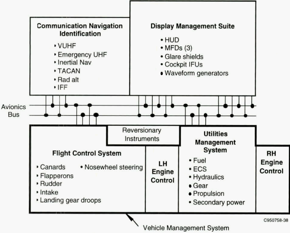
Figure 5-15. EAP Architecture
