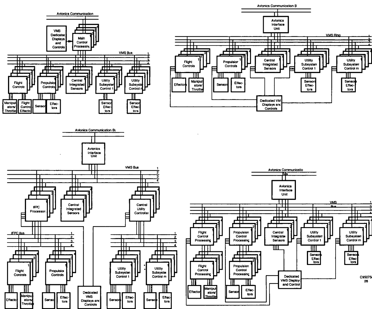
Figure 3-3. ICLE VMS Configurations
