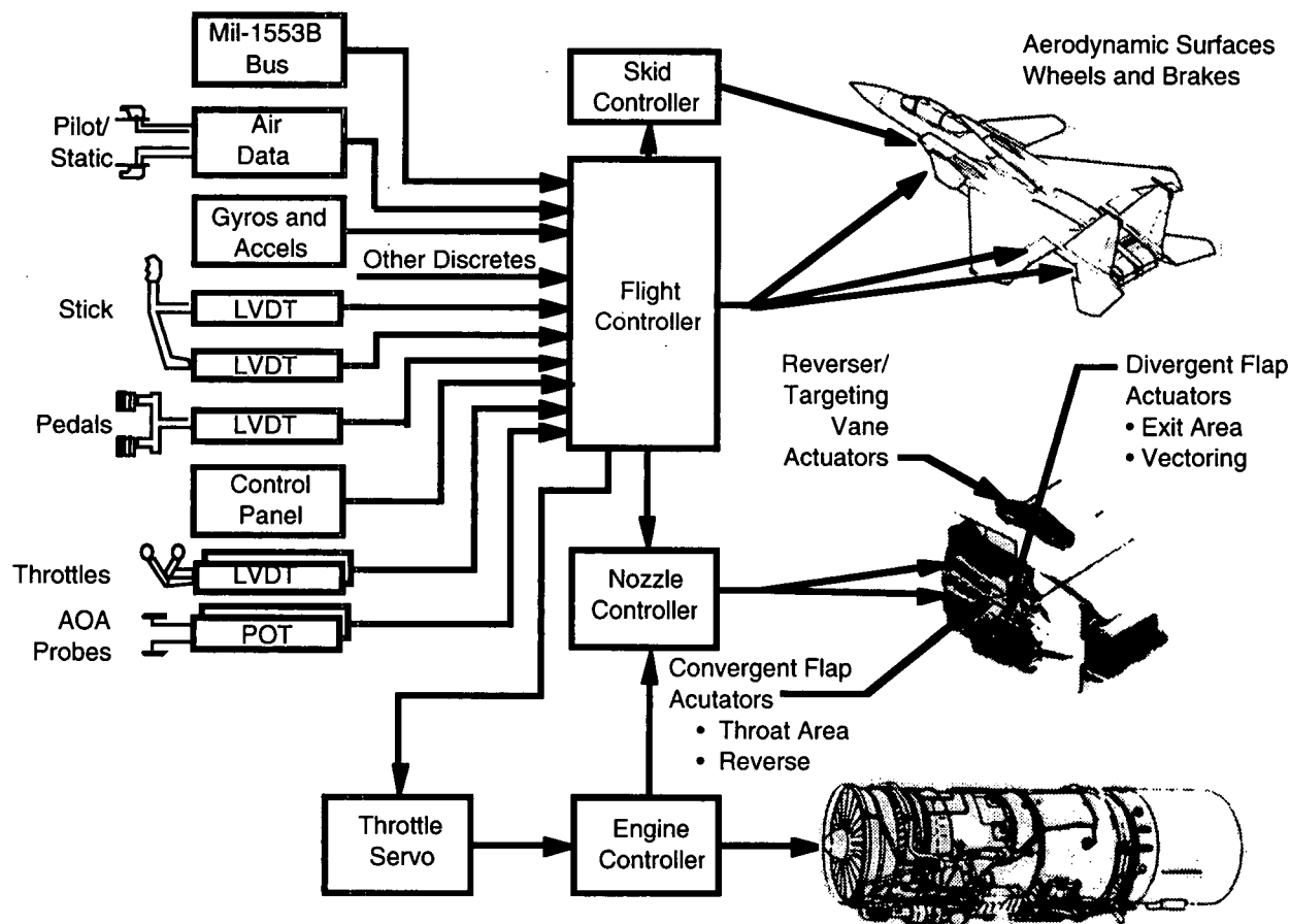
Figure 2-4. Integrated Flight/Propulsion Control [2.6]
