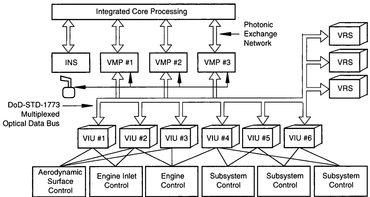
Figure 3-4. AVMS Architecture
