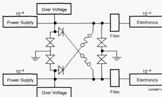
Figure 6-6D. RF Filters Added to Power Supplies
