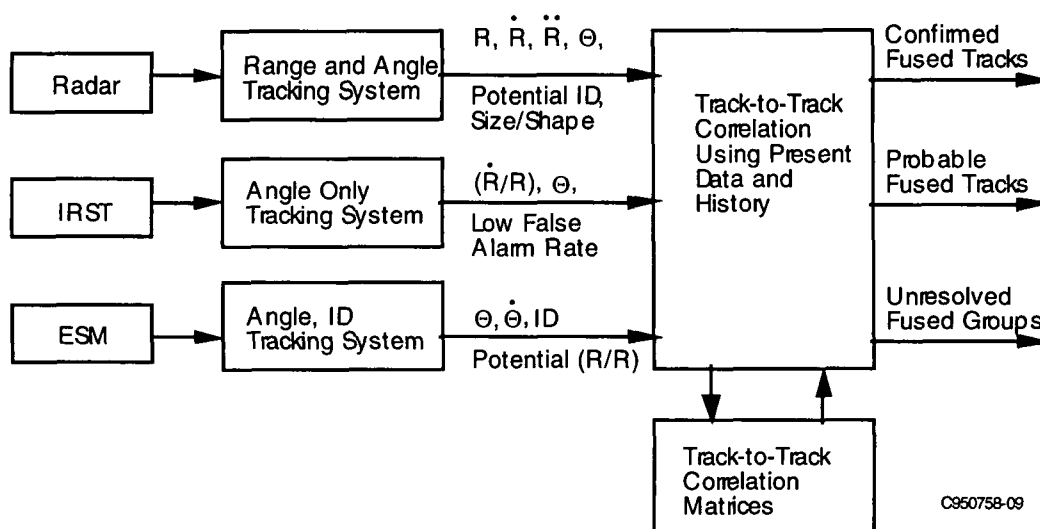
Figure 2-6. Sensor Level Tracking
