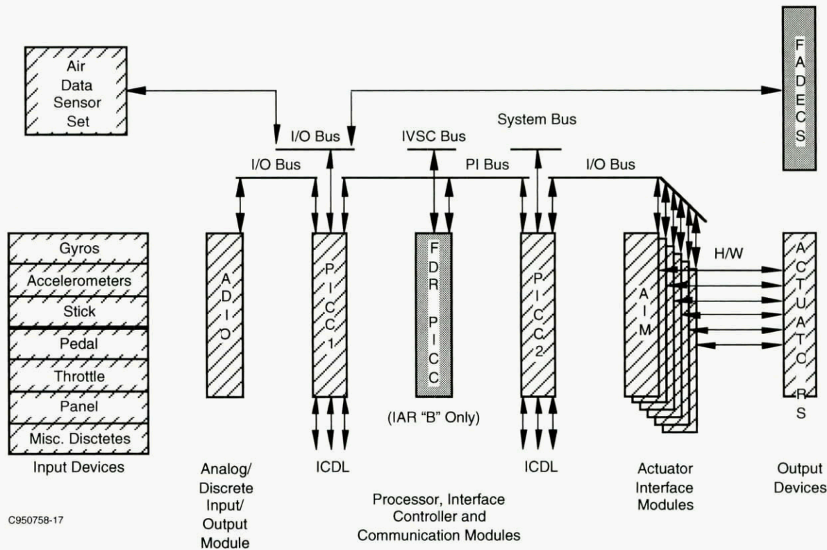
Figure 5-8. F-22 VMS Architecture
