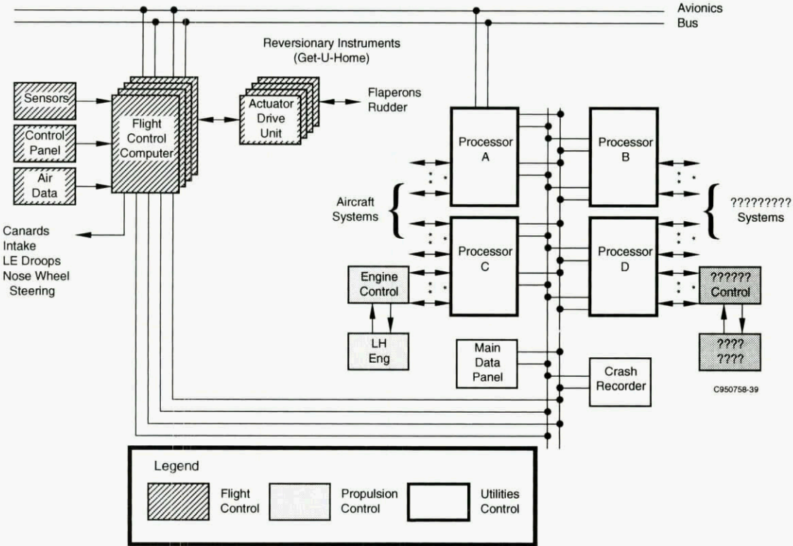
Figure 5-16. EAP VMS
