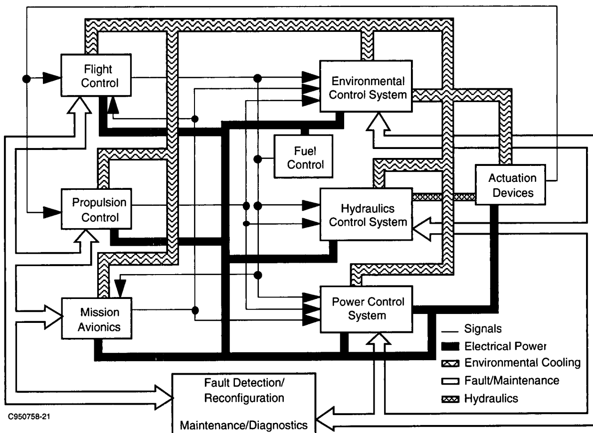
Figure 2-9. IVMS Functional Diagram
