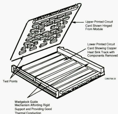
Figure 5-17. EAP Standard Module
