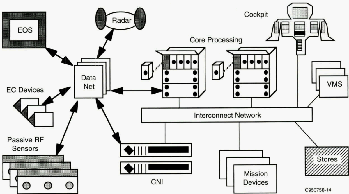
Figure 5-7. F-22 Avionics Architecture
