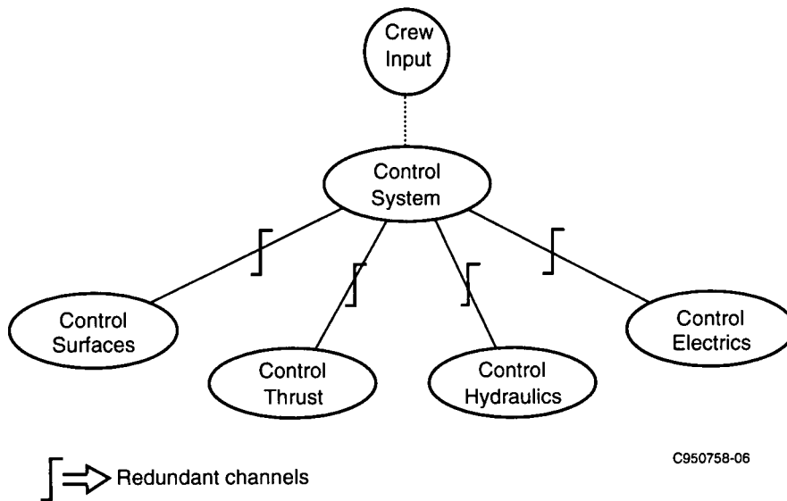
Figure 4-4. Cooperating Control Structure
