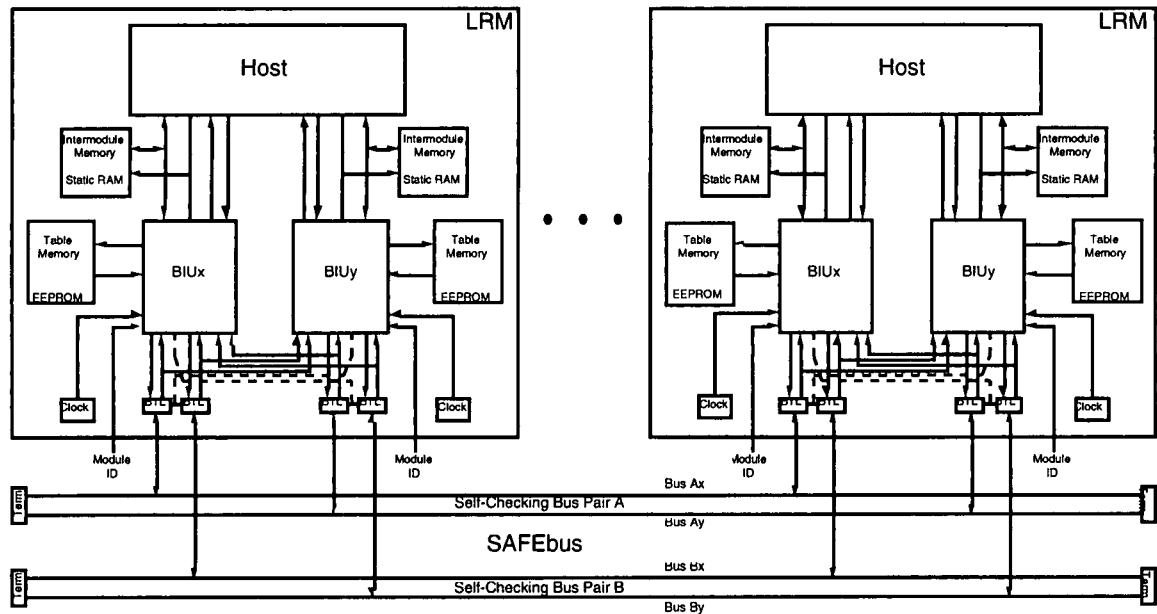
Figure 5-4. B-777 SAFEbus Implementation
