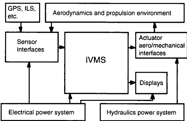
Figure 3-7. IVMS Functional Interfaces
