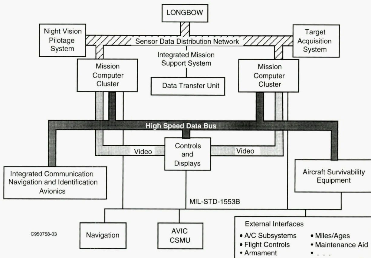
Figure 5-12. RAH-66 Avionics Architecture
