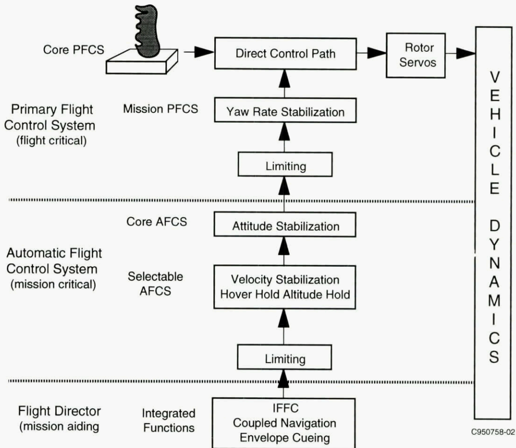
Figure 5-13. RAH-66 Flight Control Functional Diagram
