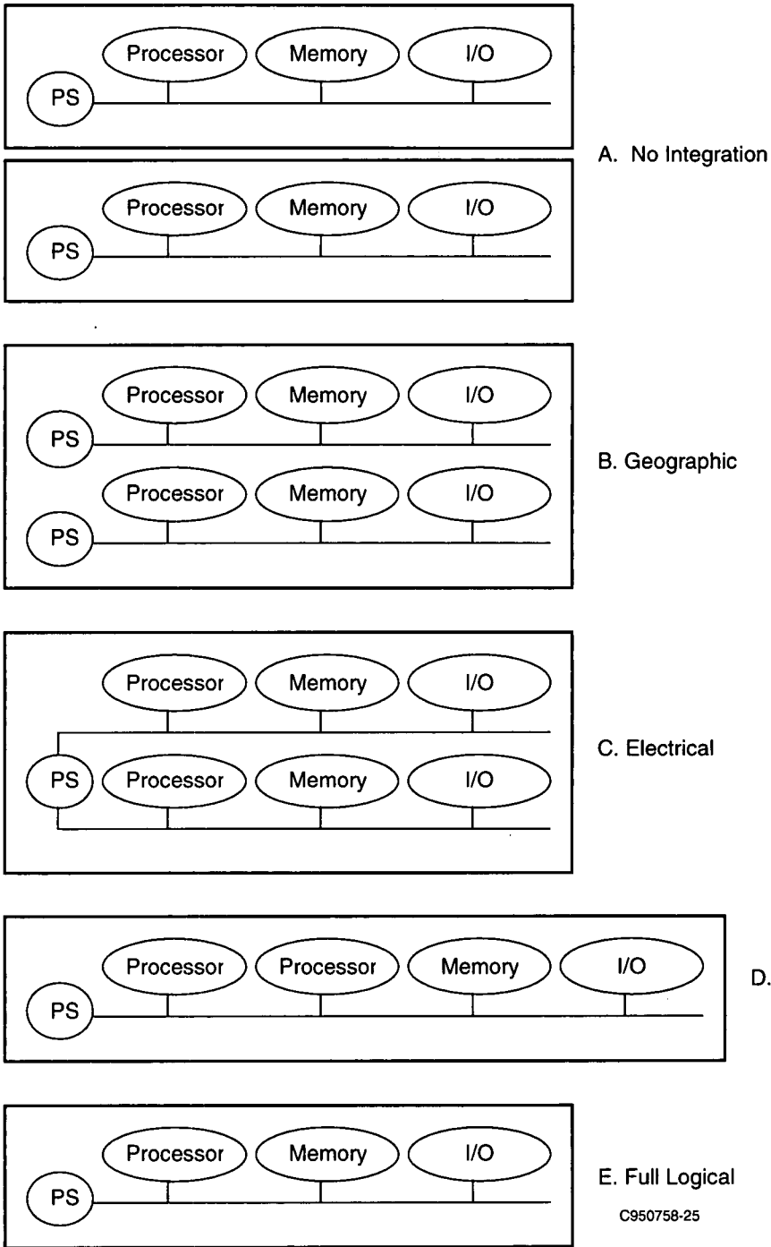
Figure 2-3. Principles of Physical Integration
