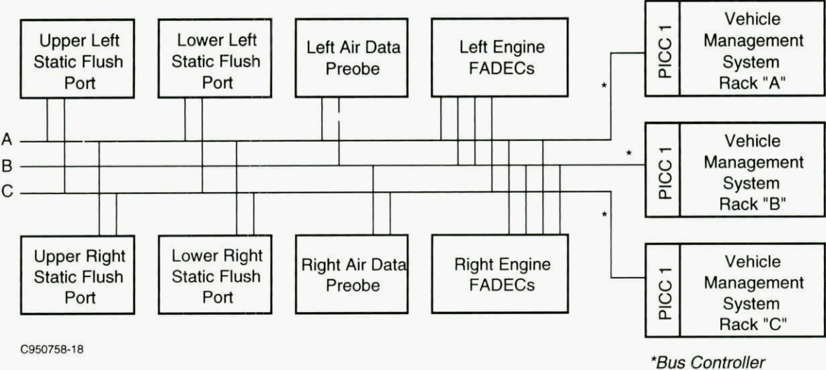
Figure 5-9. IFPC Bus Architecture
