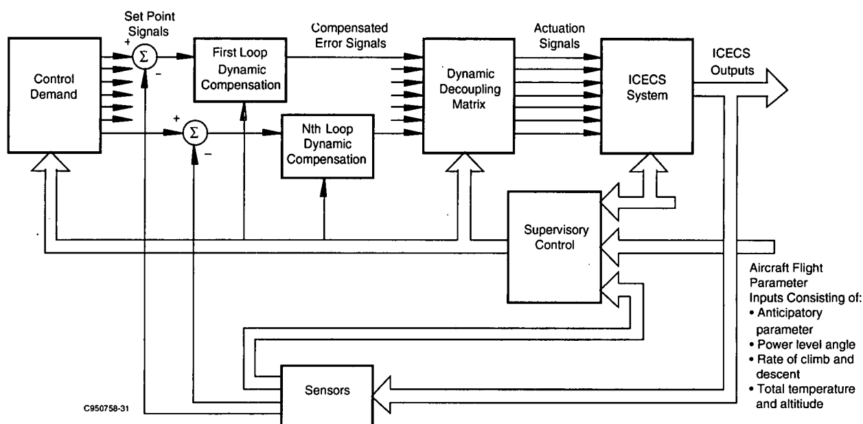
Figure 3-6. ICECS Control System
