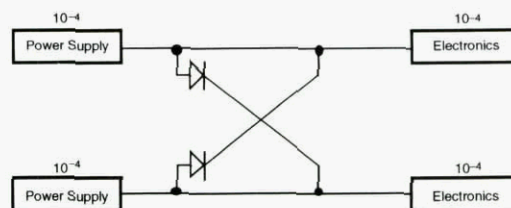
Figure 6-6B. Dual Power Supplies with Diode Protection
