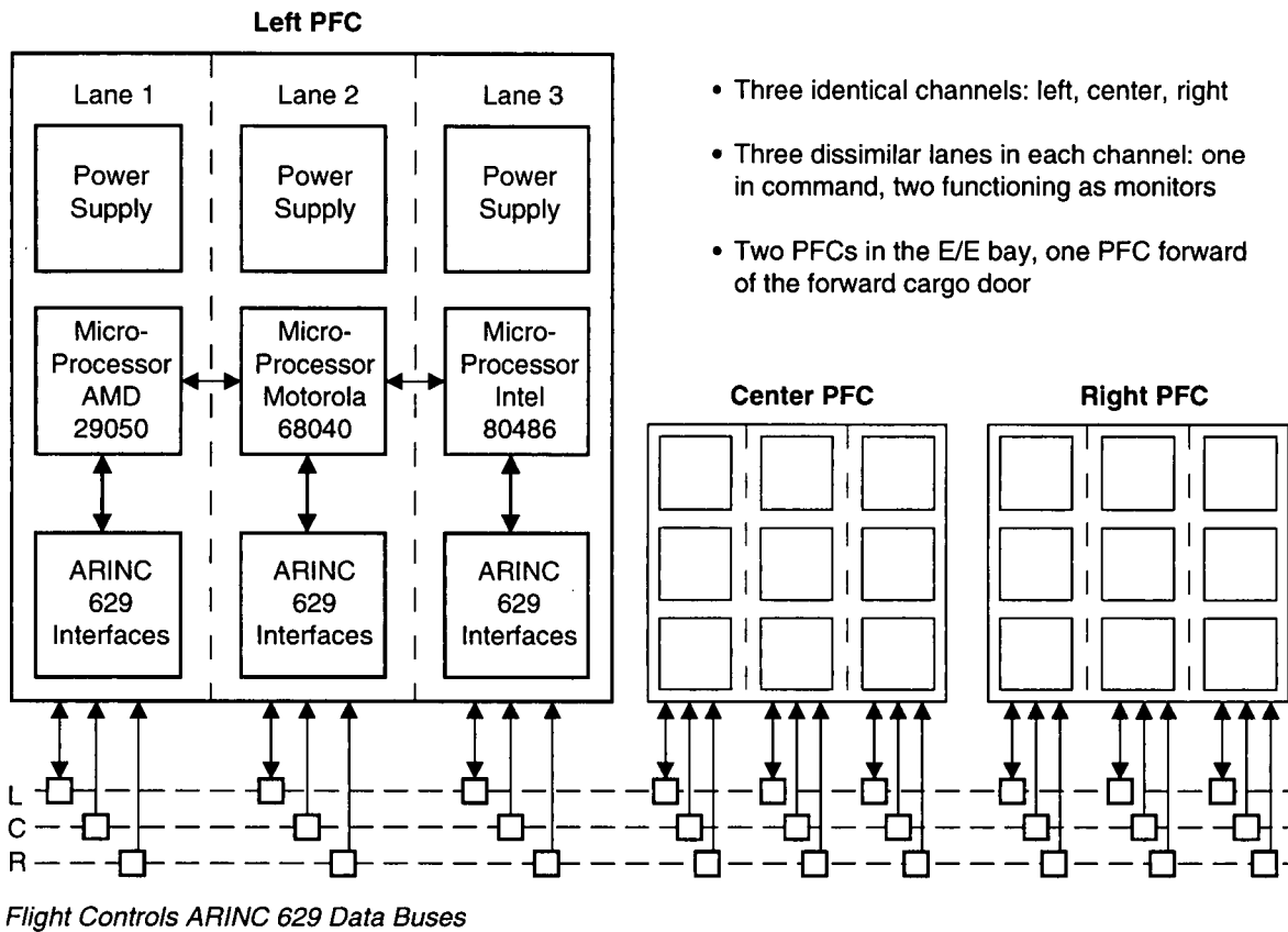
Figure 5-3. Primary Flight Computer Channel Architecture
