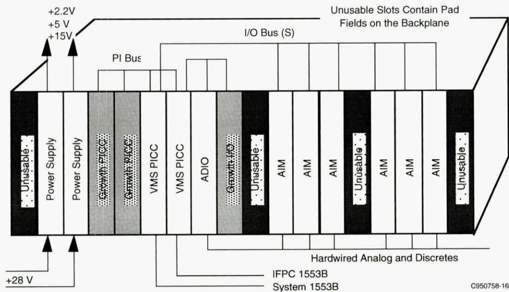
Figure 5-11. F-22 Common Module Rack
