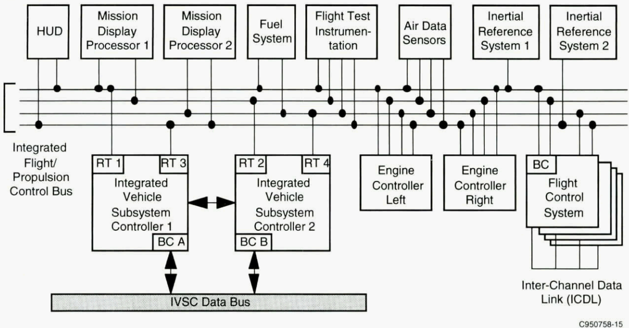
Figure 5-5. YF-22 Prototype Architecture
