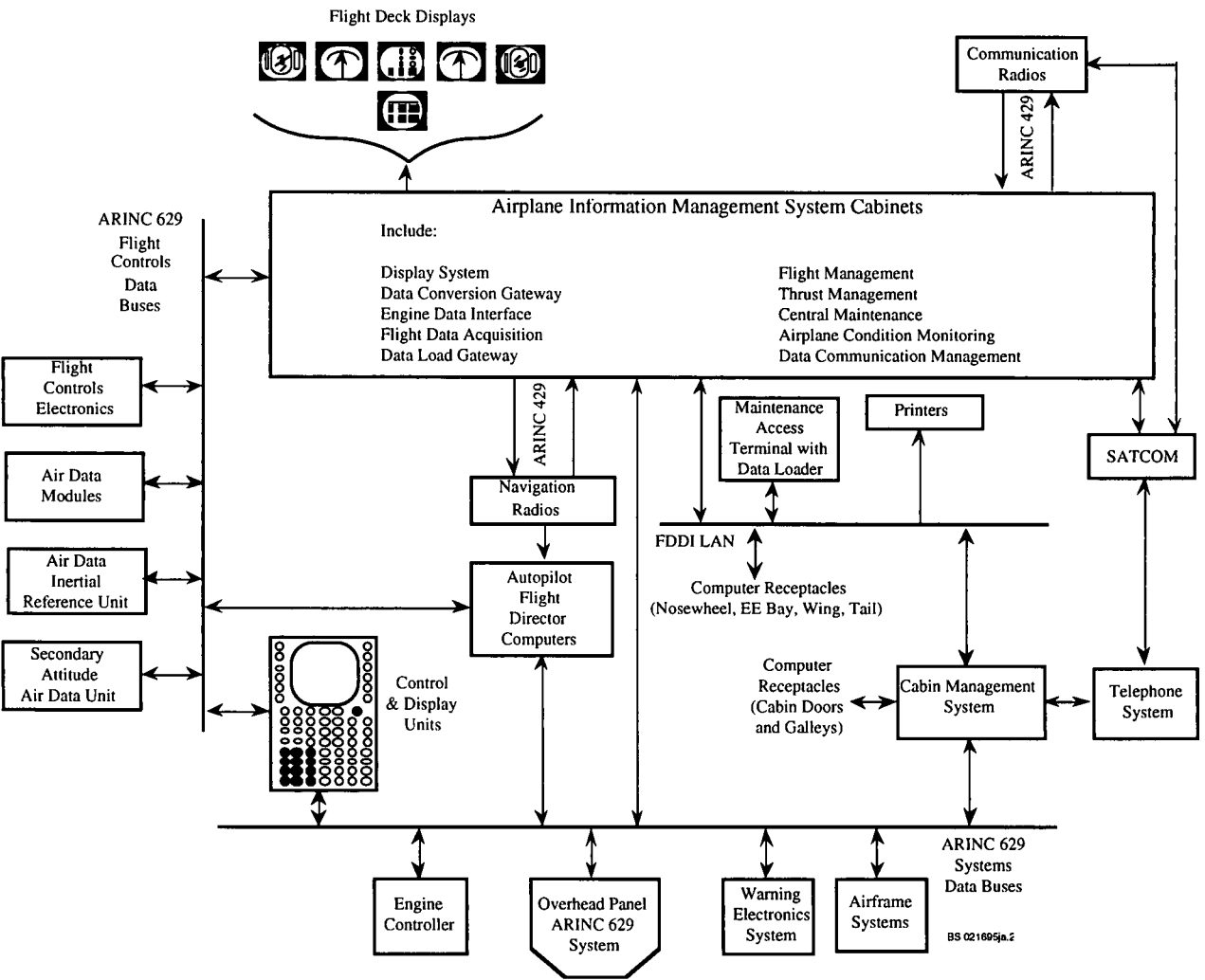
Figure 5-1. B-777 System Architecture
