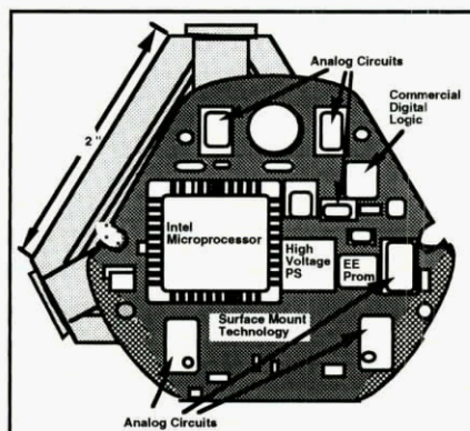
Figure 6-2. Digital RLG Electronics
