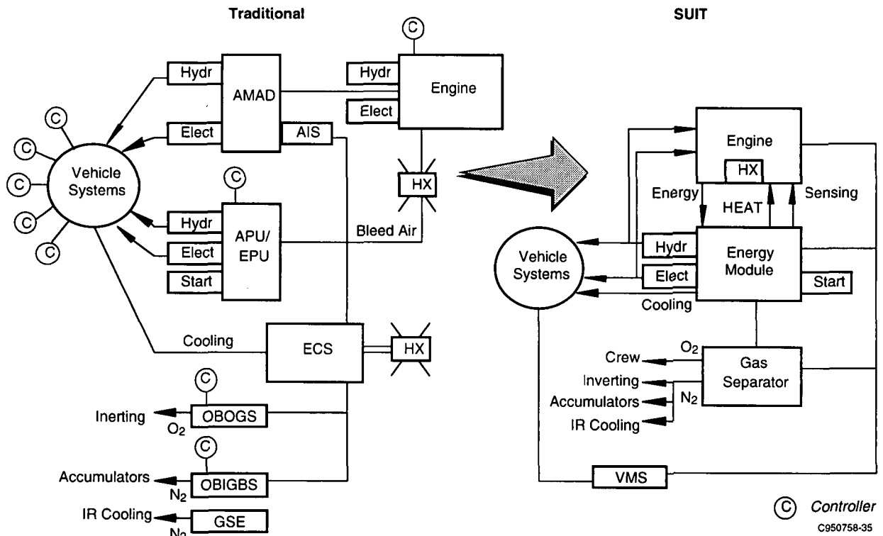
Figure 3-5. SuIT Component Reduction
