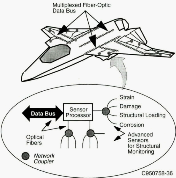
Figure 6-1. Distributed Structural Sensors
