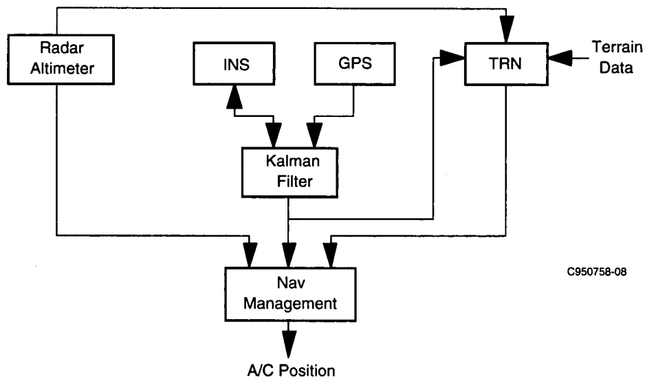
Figure 2-5. Integrated Navigation System
