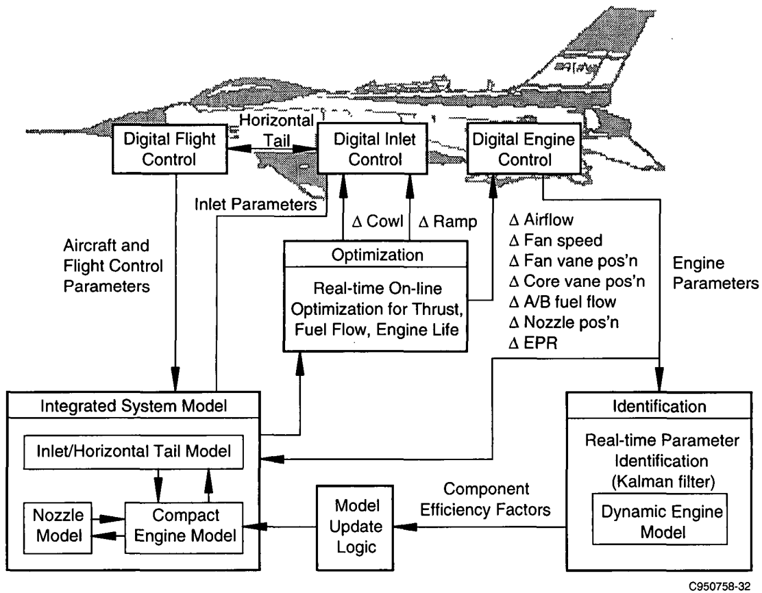
Figure 3-2. Performance-Seeking Control System
