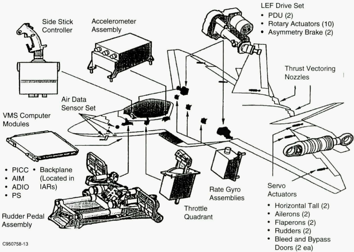
Figure 5-10. VMS Hardware
