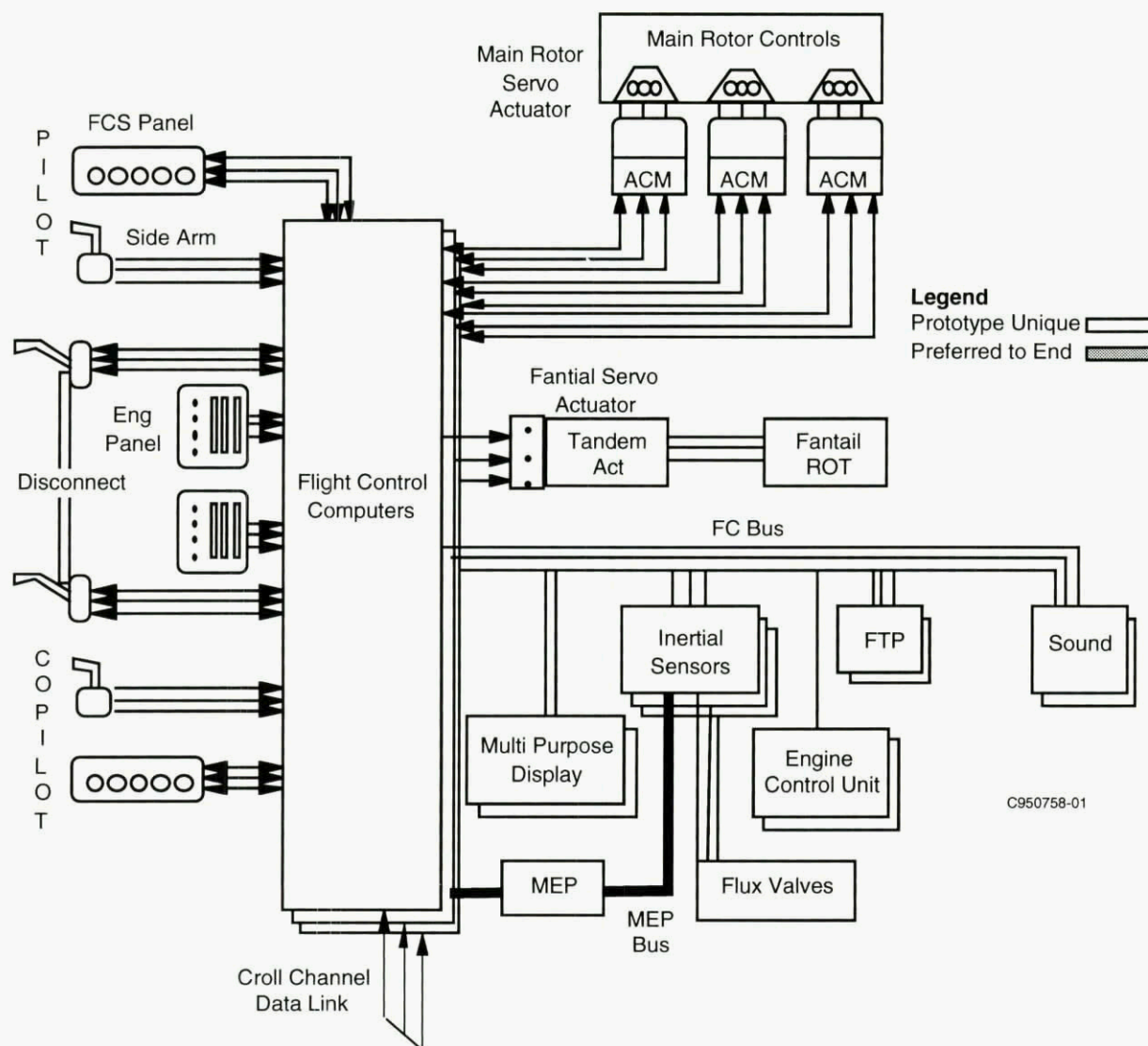
Figure 5-14. RAH-66 Flight Control System
