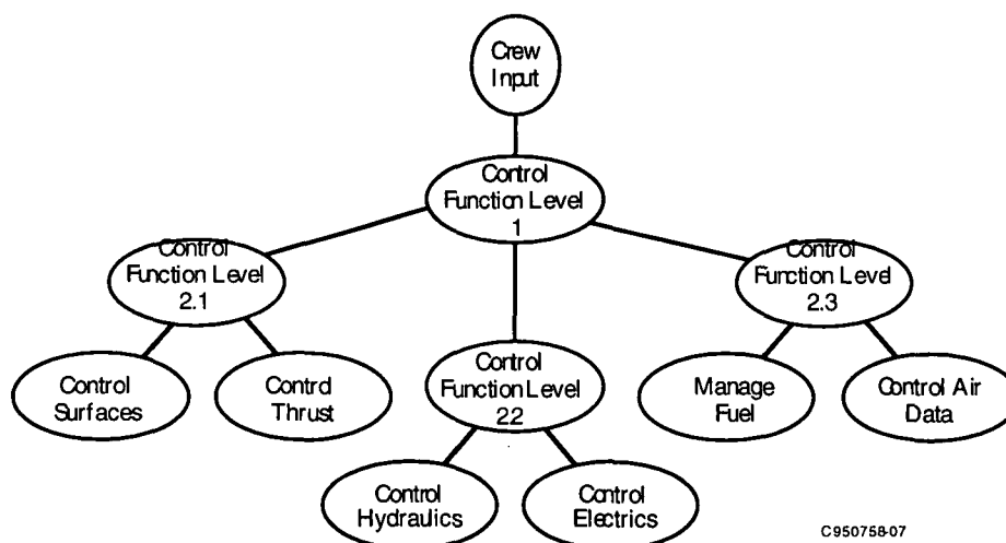
Figure 4-1. Hierarchical Control Structure
