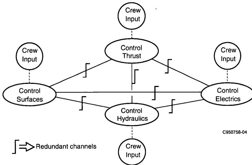
Figure 4-2. Federated Control Structure
