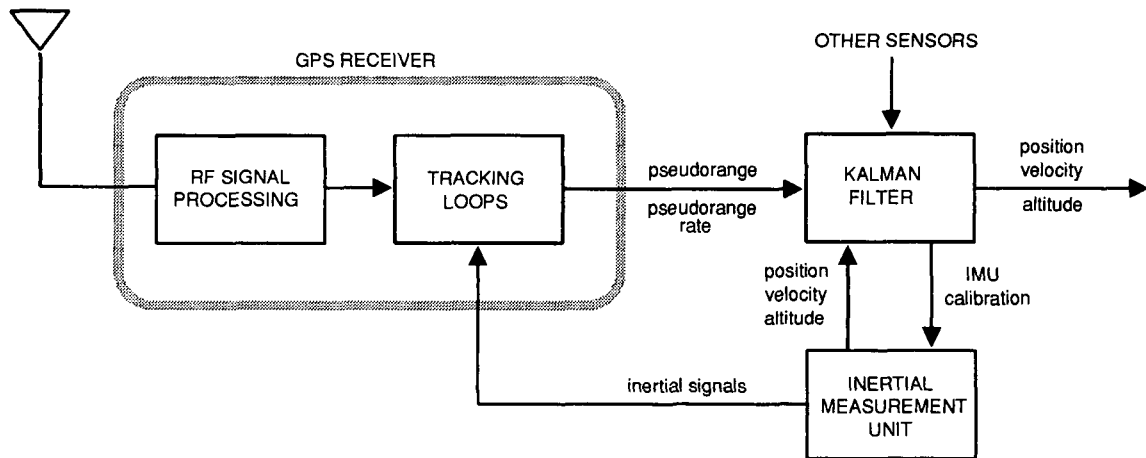
Figure 4.9. Tightly Coupled Approach
