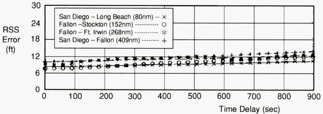
Figure D.9 Total RSS Error vs. Time Delay, West Coast Data
