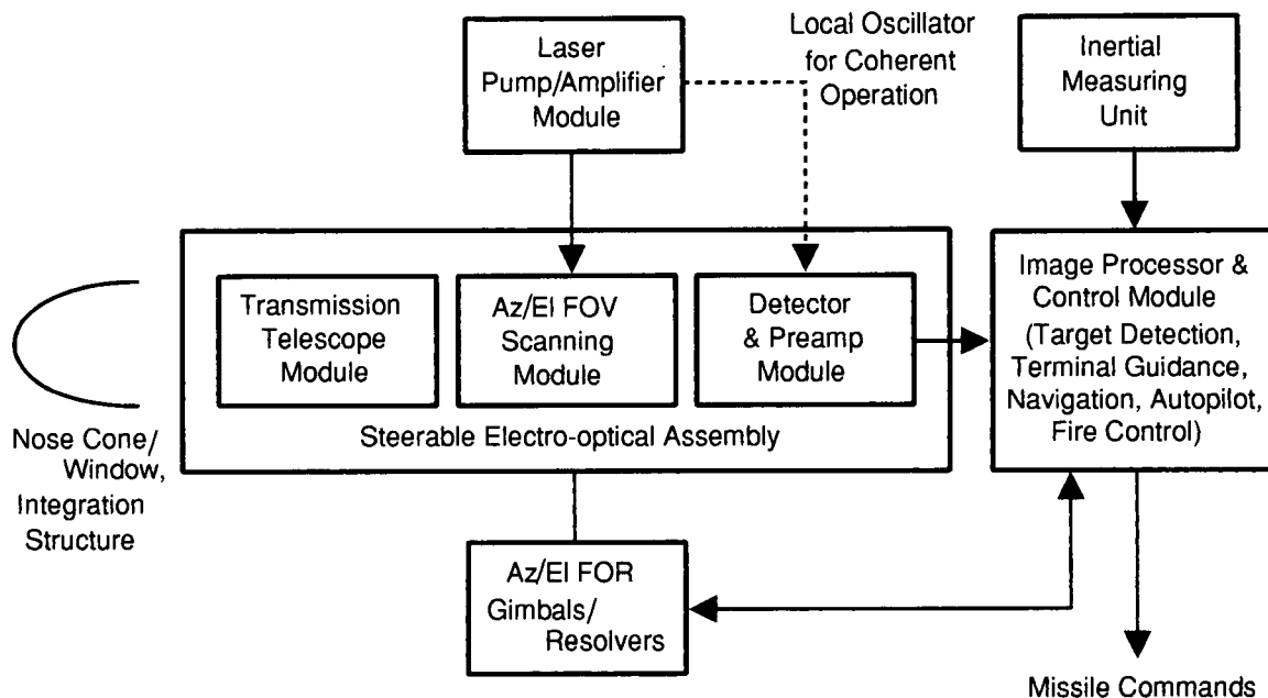
Figure 4.1. Typical Ladar Seeker Configuration
