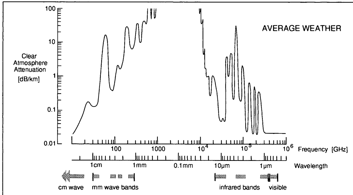
Figure 2.4. Atmospheric Attenuation
