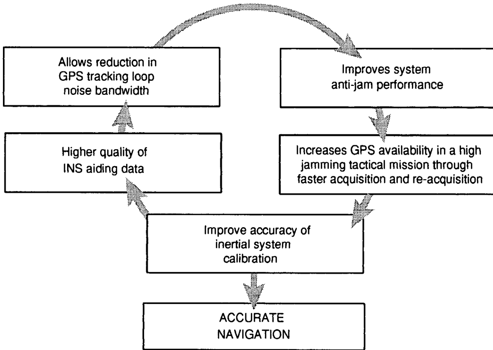
Figure 4.7. The Synergy of GPS/INS Integration
