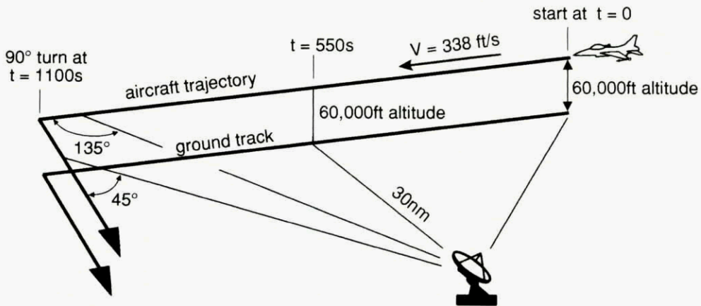
Figure D.11. Trajectory 1 Geometry
