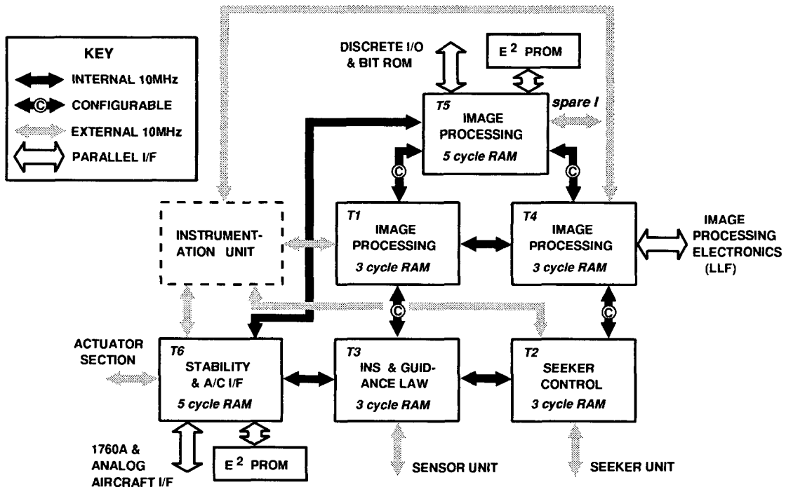
Figure 4.4. Transputer Application to Guidance Processing
