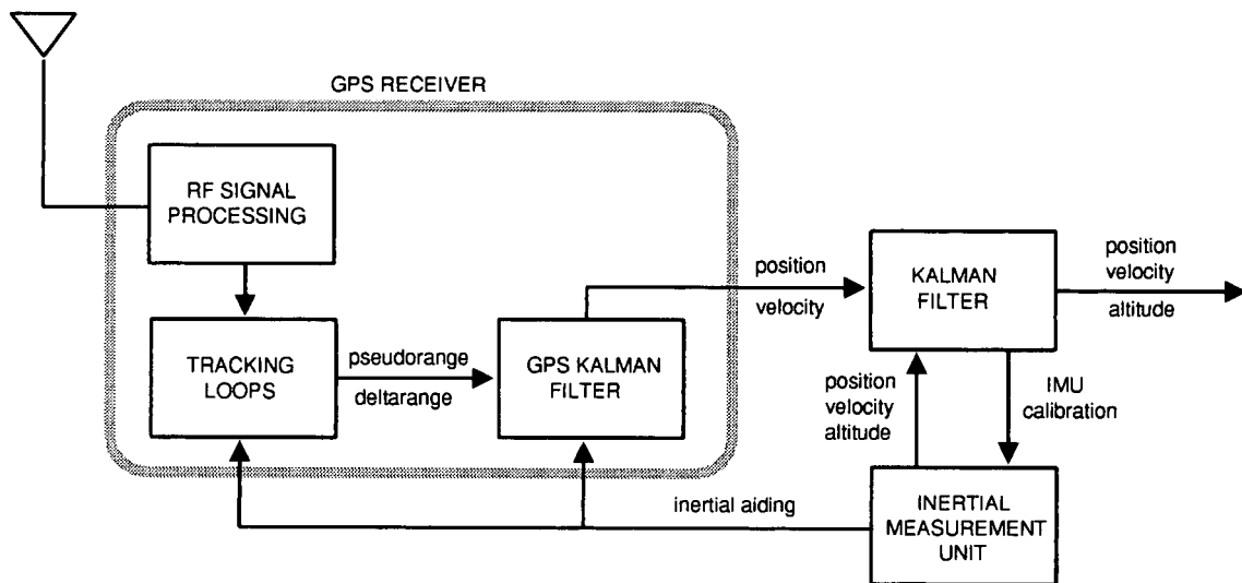
Figure 4.8. Cascaded Filter Approach
