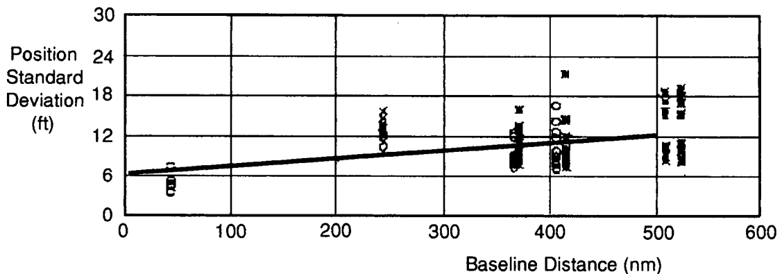
Figure D.6b. Standard Deviation Component of Error, East Coast Data
