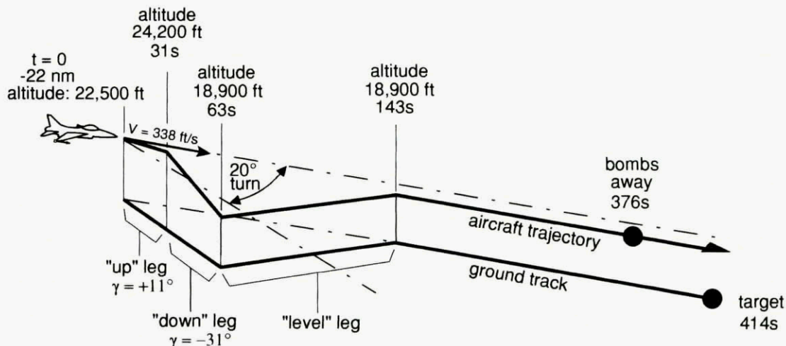
Figure D.14. Trajectory 3
