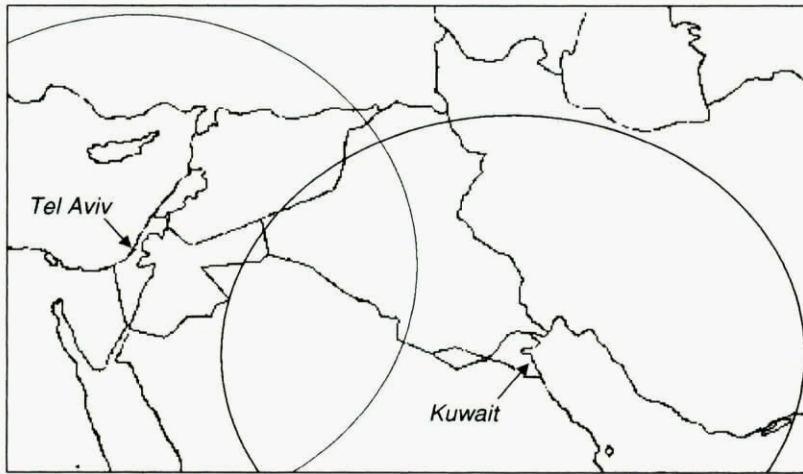
Figure D.15. 540 nm "coverage" for two cooperative GPS receiver/transmitter
