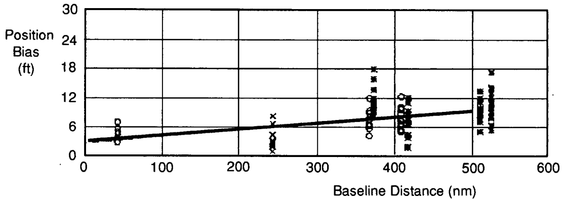
Figure D.6a. Bias Component of Error, East Coast Data
