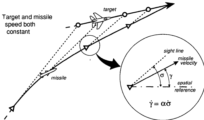
Figure 2.2 . Proportional Navigation
