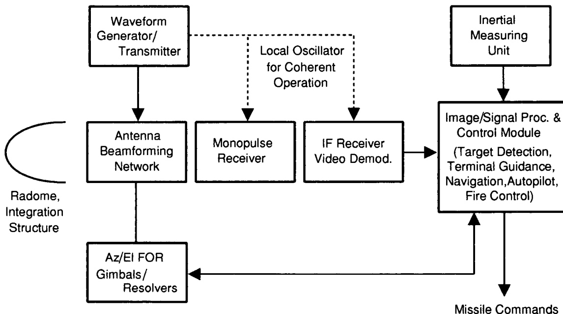
Figure 4.2. Typical SAR Seeker Configuration
