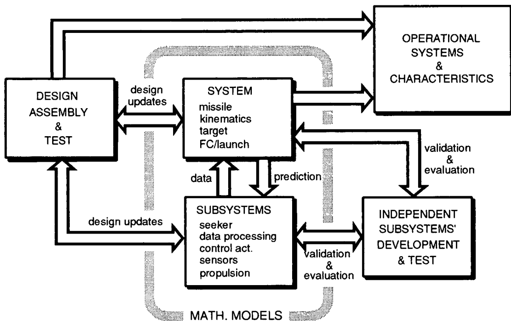
Figure 5.1. Custom Munitions Systems Process
