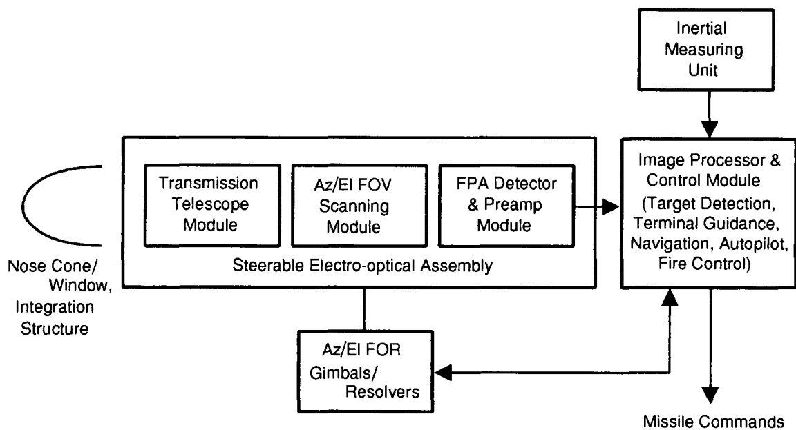
Figure 4.3. Generic Semi-Strapdown IIR Seeker Configuration
