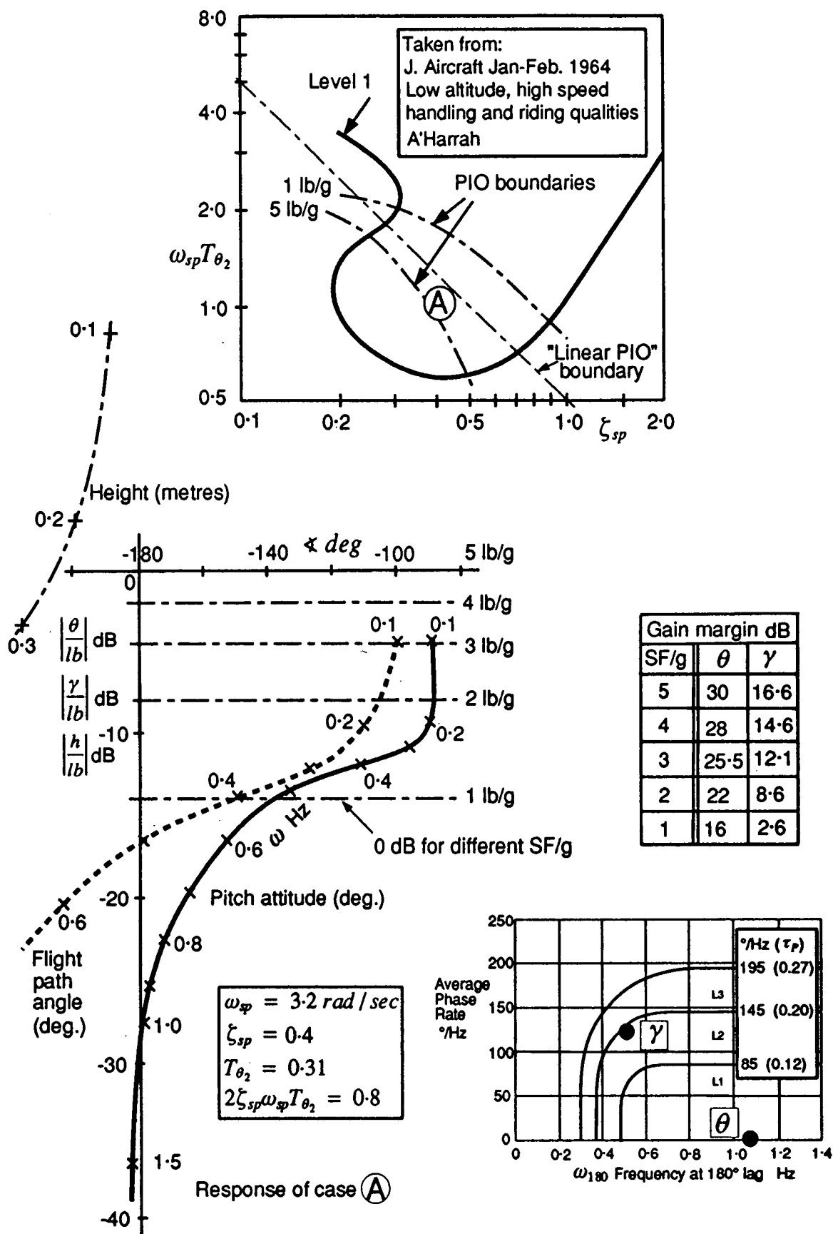
Figure 12 Probable height-related PIO
