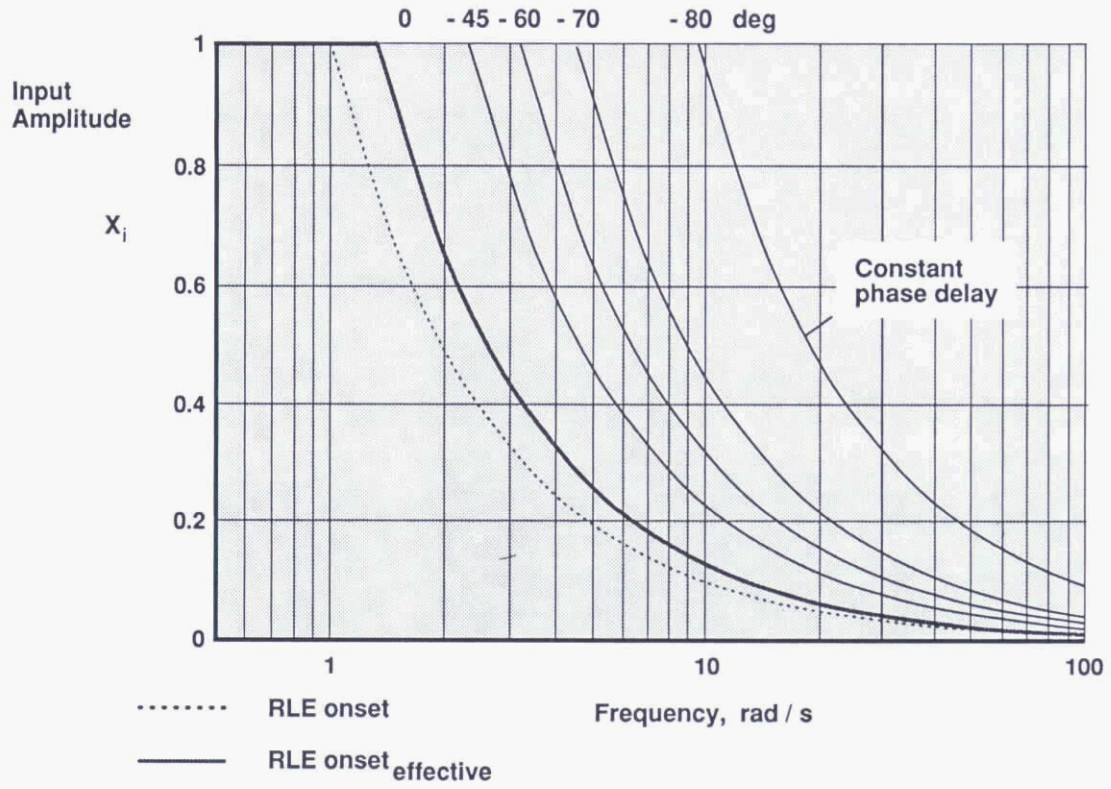
Figure 7 RLE produced phase delay
