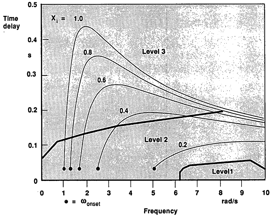
Figure 15 RLE influence on bandwidth criterion
