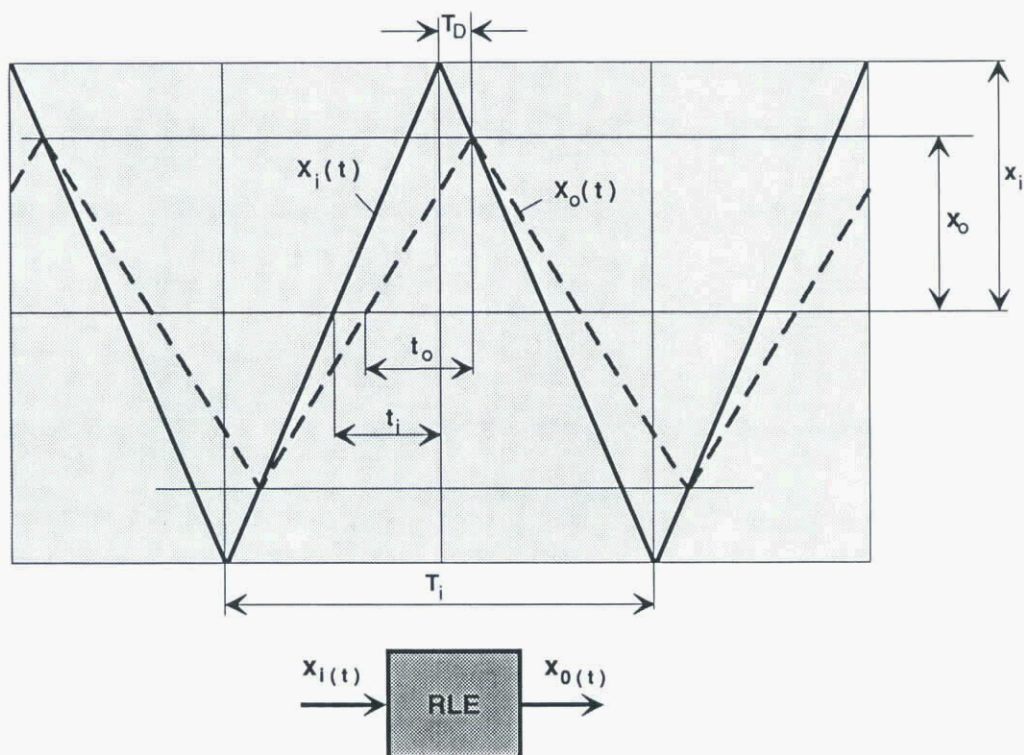
Figure 1 RLE time response (triangle type input)
