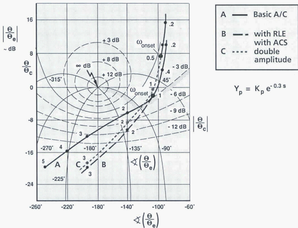
Figure 18 RLE compensated by ACS, frequency domain
