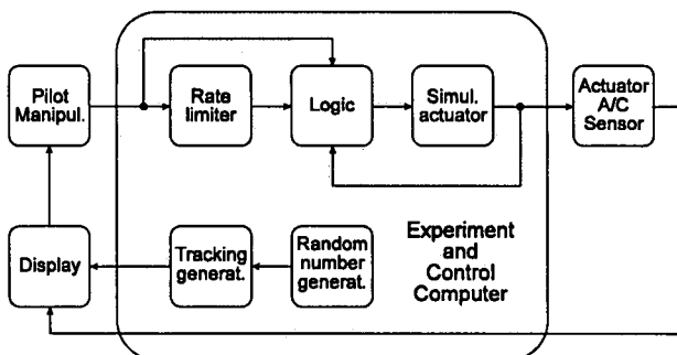
Fig 6 The experiment
