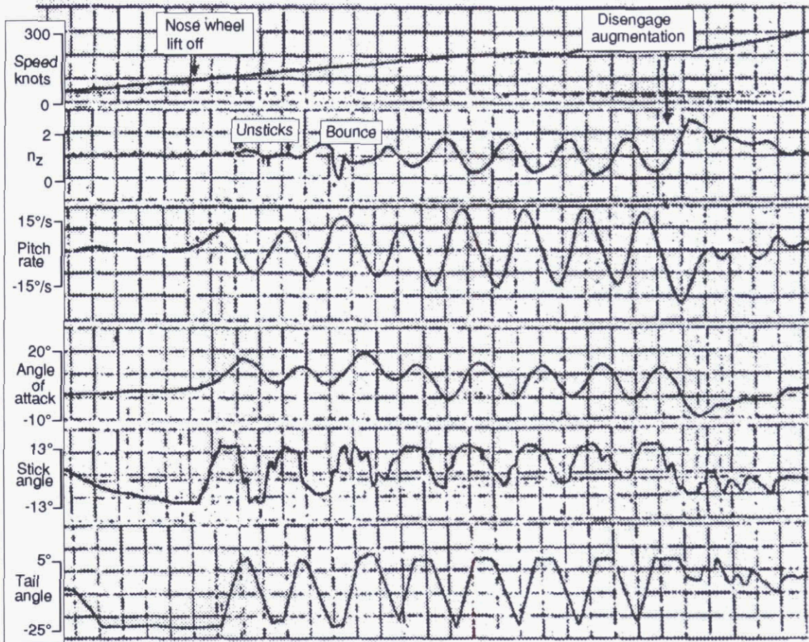
Figure 4 Tornado short take-off PIO
