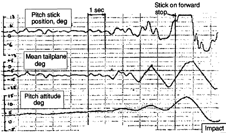
Figure 2 Landing PIO (Tornado, initial FCS)
