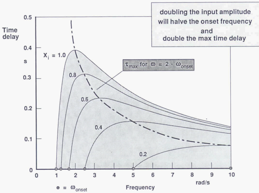
Figure 3 RLE produced time delay
