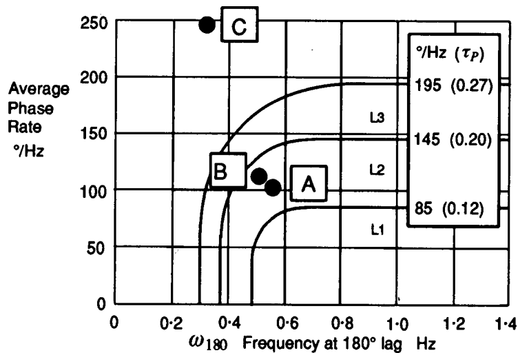
Figure 11 Shuttle orbiter PIO examples
