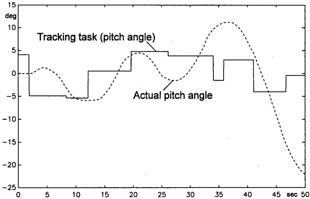
Fig 7 Conventional control scheme
