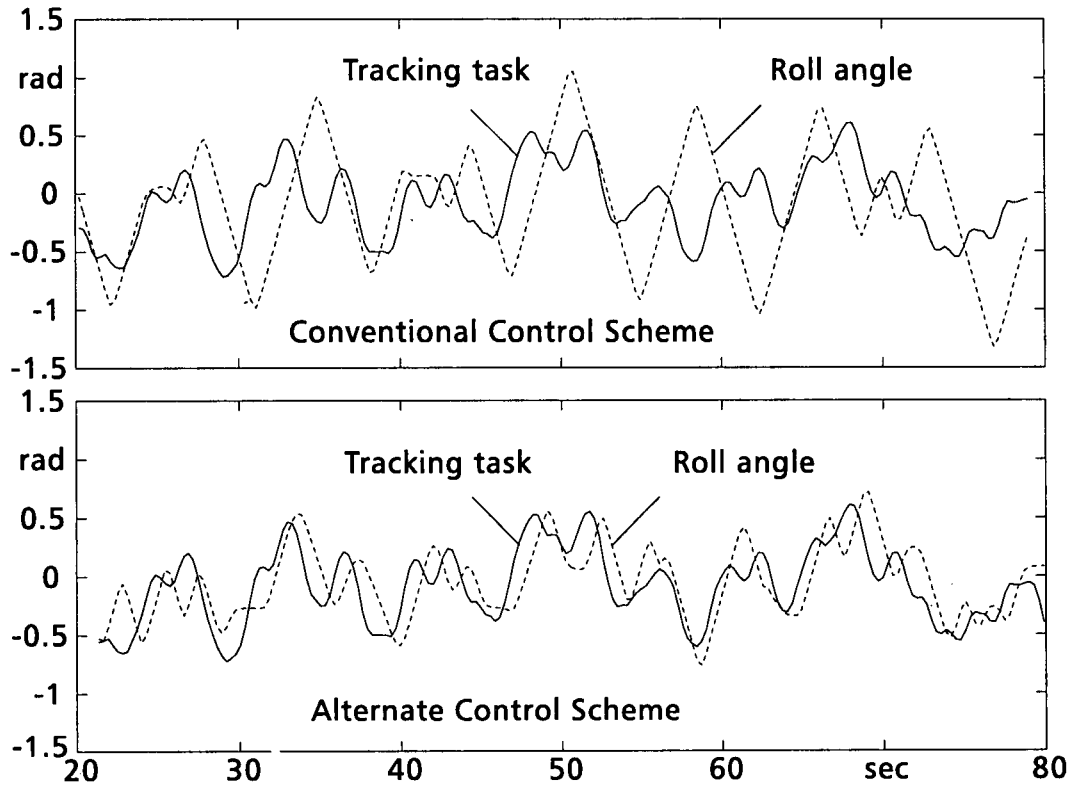
Fig 10 Pilot-in-the-loop simulation
