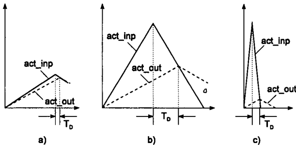
Fig 3 Different time delays
