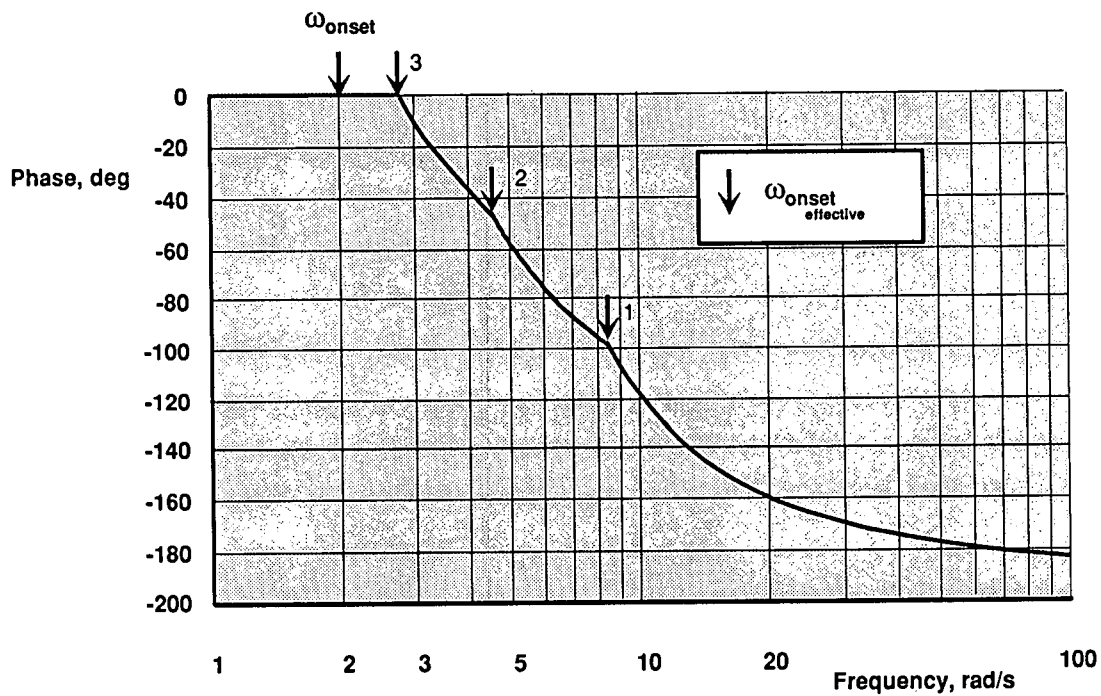
Figure 10 Cascaded RLE frequency response (sinusoidal input)
