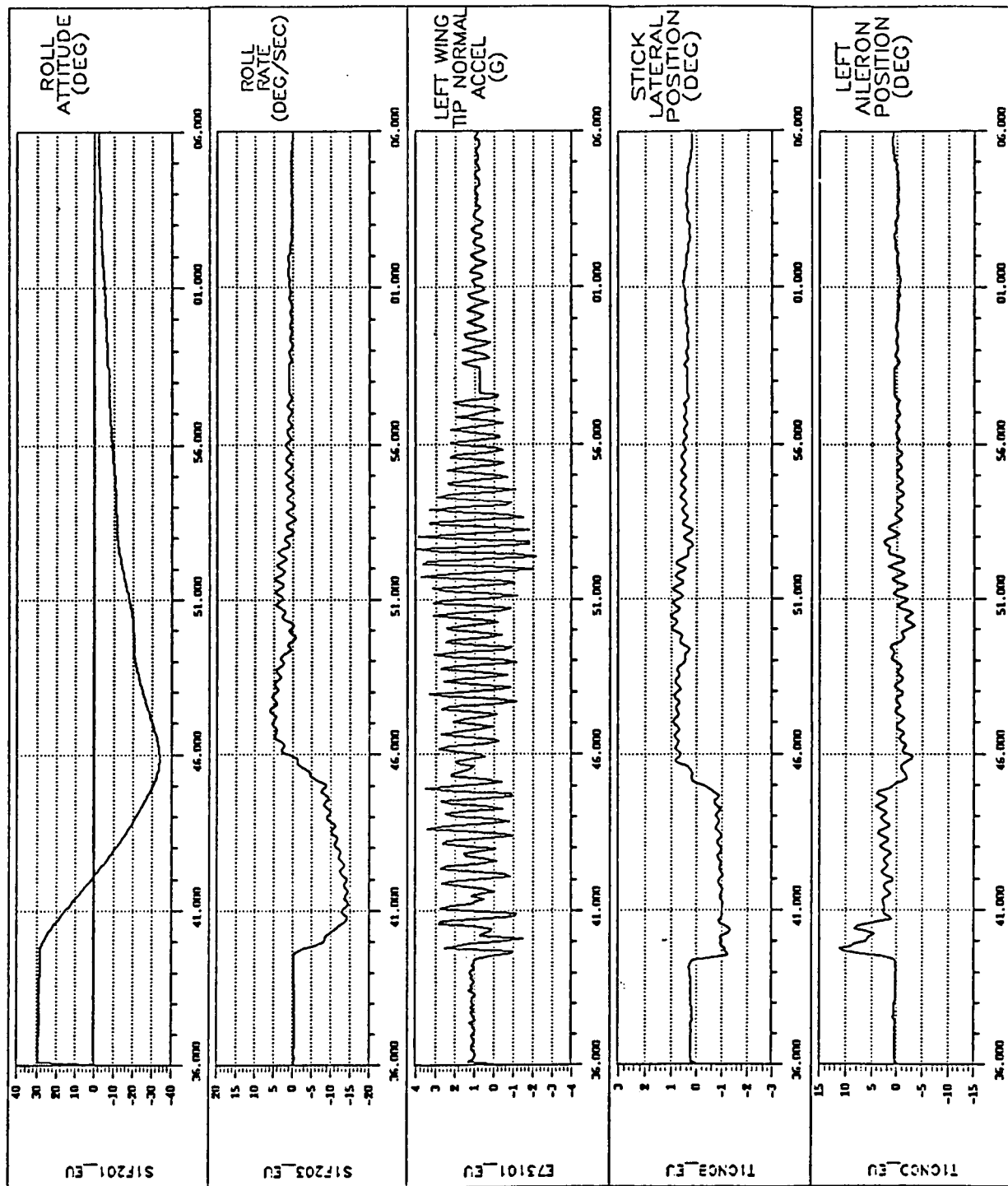
Figure C1 Example Roll Ratcheting
