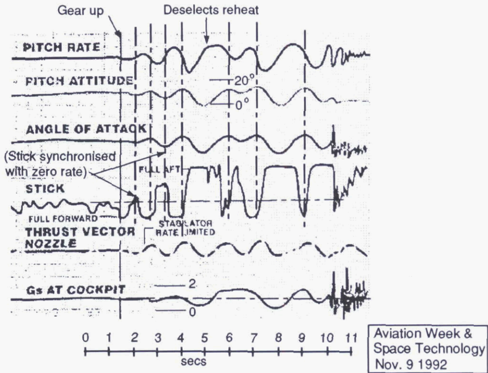
Figure 5 YF-22 landing PIO
