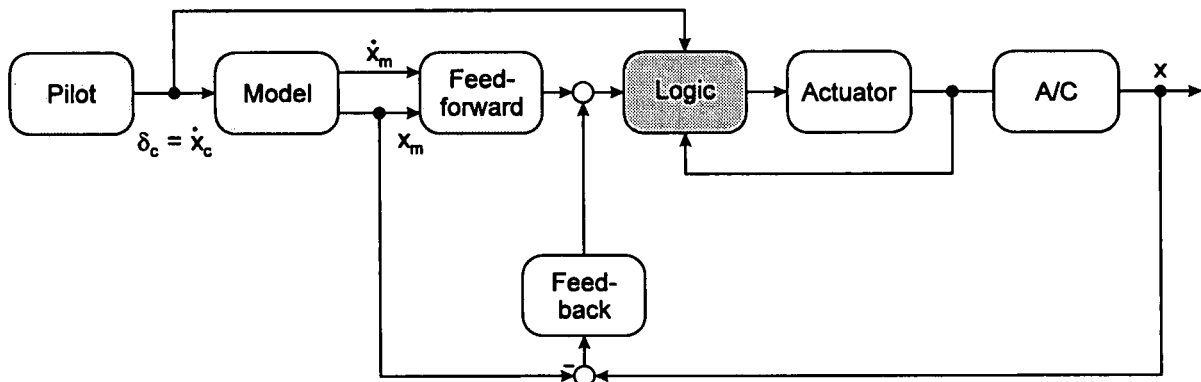
Fig 9 Model following control system
