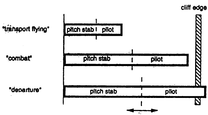
JAS 39 Flight Control System
