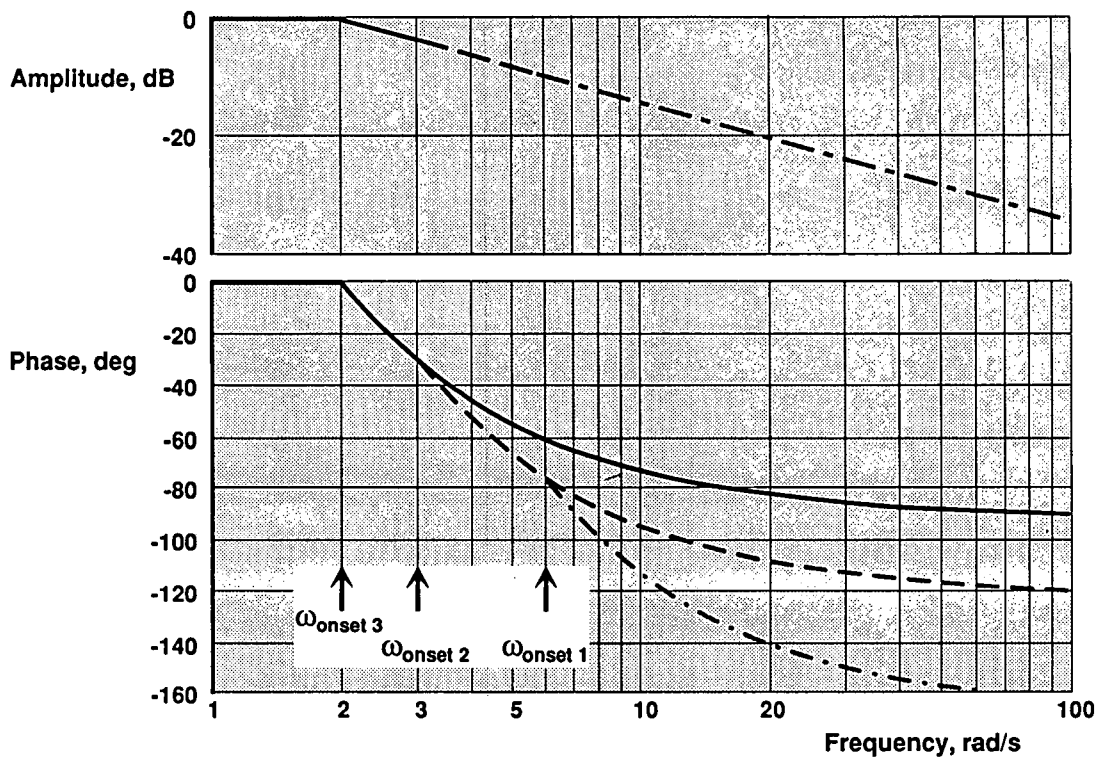
Figure 9 Cascaded RLE frequency response (triangle type input)
