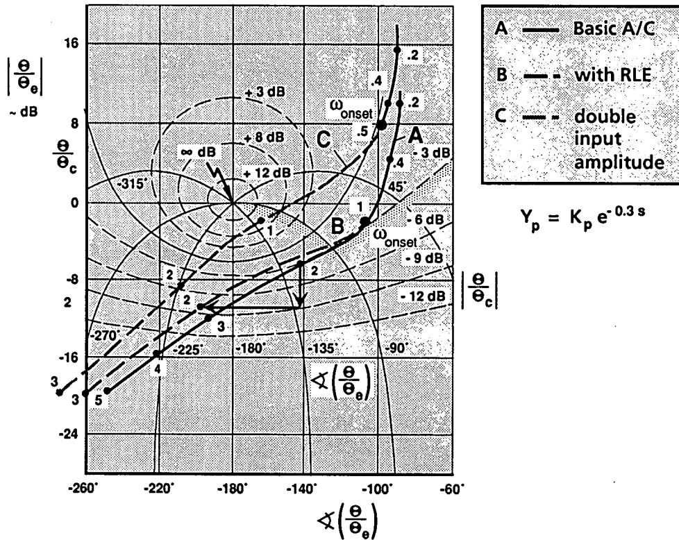
Figure 16 Influence of RLE on open/ closed loop system
