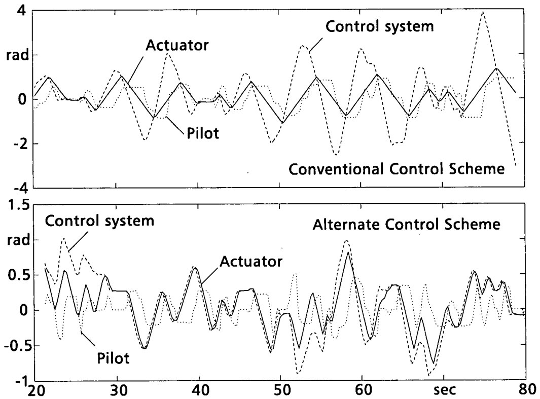
Fig 11 No time delay with alternate control scheme
