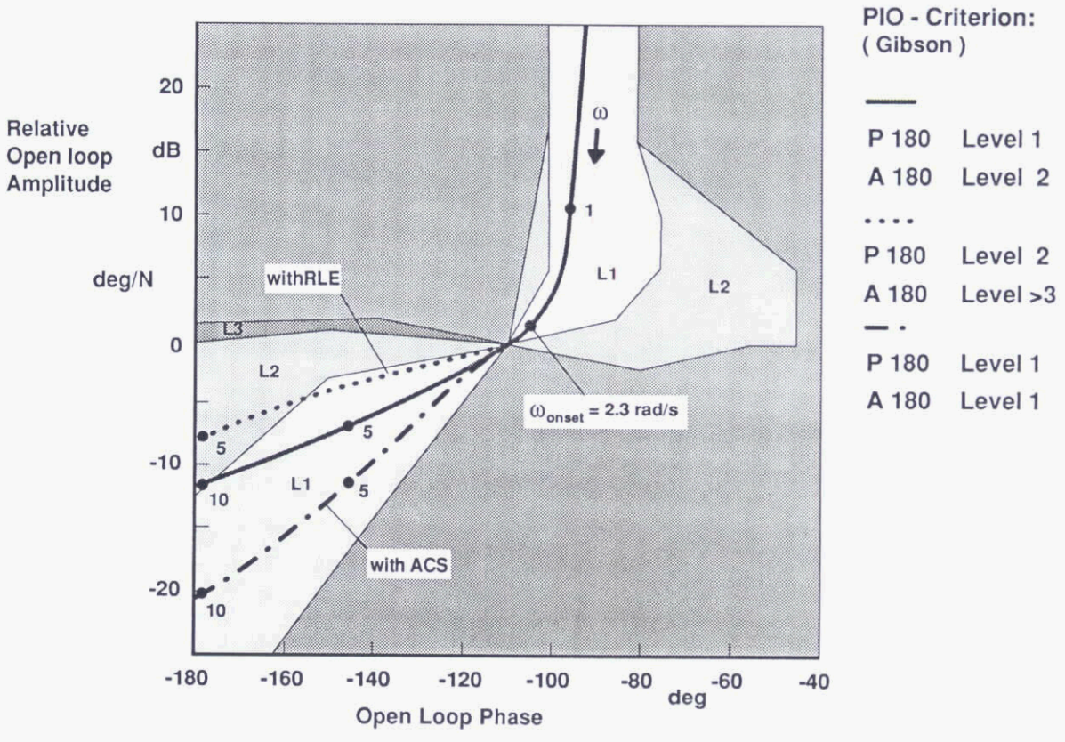
Figure 19 Pitch frequency response limits (Gibson criterion)
