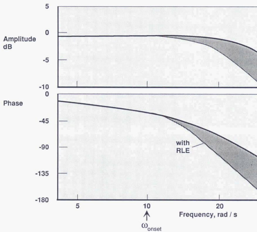
Figure 12 Actuator frequency response with input rate limitation
