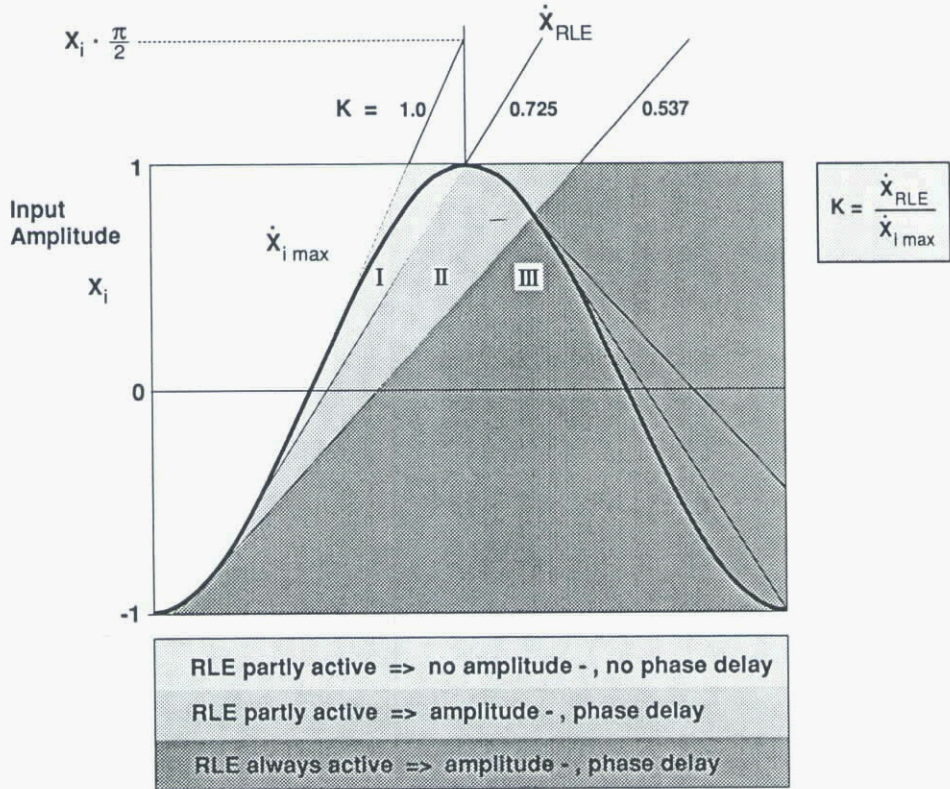
Figure 5 RLE time response (sinusoidal input)
