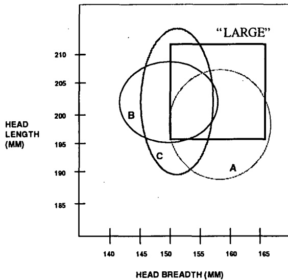
Figure 1-5. Fit regions for three size "large" helmets versus their design size "large."
