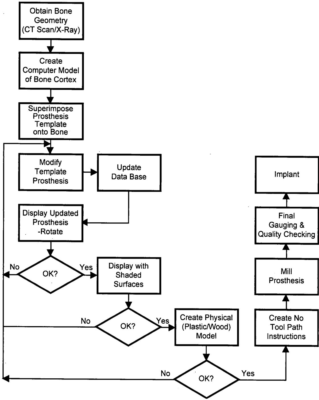
Figure 2-4. Flowchart of Design Process for Patient-Specific Prosthesis
