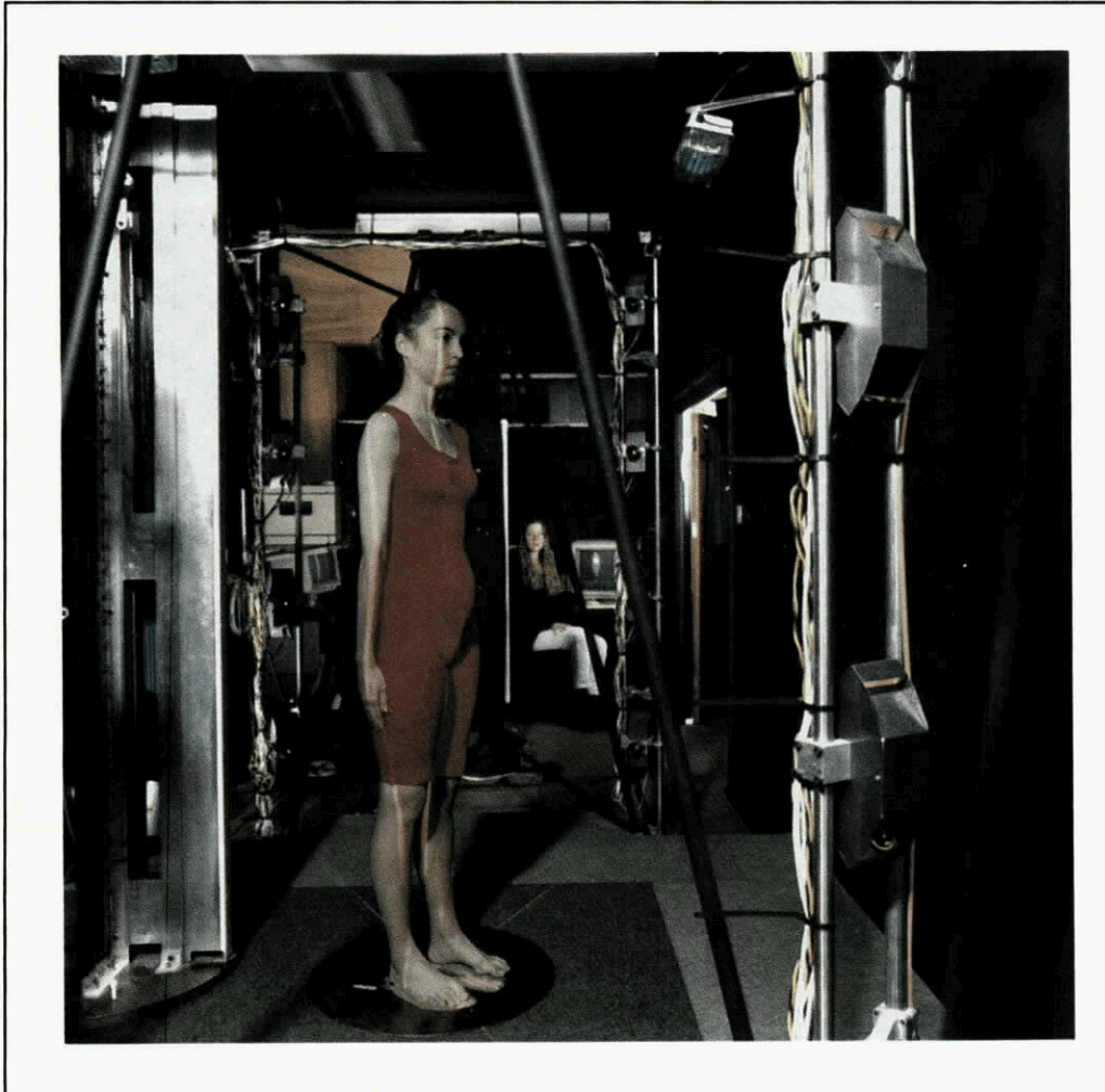
Figure 2-1. A subject being scanned in the LASS experimental rig. The narrow vertical slits of the projector light are falling on the body contours.
