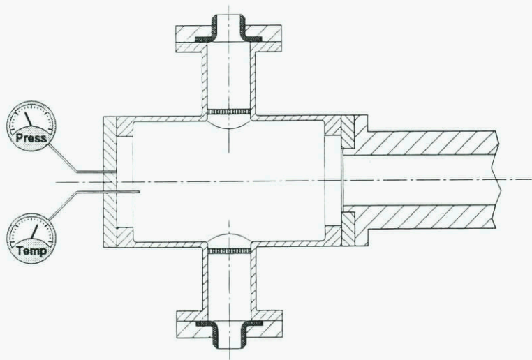
Fig. 11 - Zero thrust body for momentum tare evaluation.
