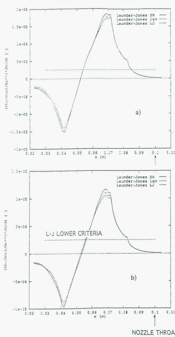
Figure 21 Axial distribution of Launder and Jones parameter a) Case 1 : Re_d = 3.8 \cdot 10^6 b) Case 2 : Re_d = 6.8 \cdot 10^6
