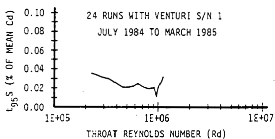
Figure 4- Repeatability of Venturi Screening Facility
