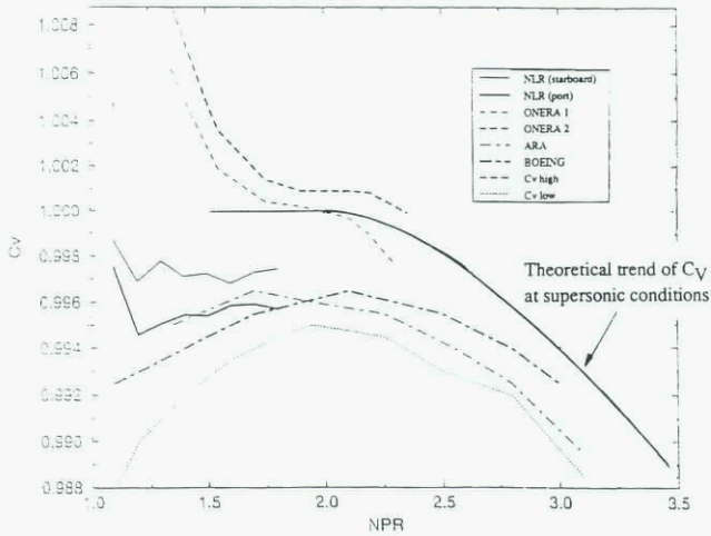
Figure 39 3" cubic nozzle Velocity coefficient
