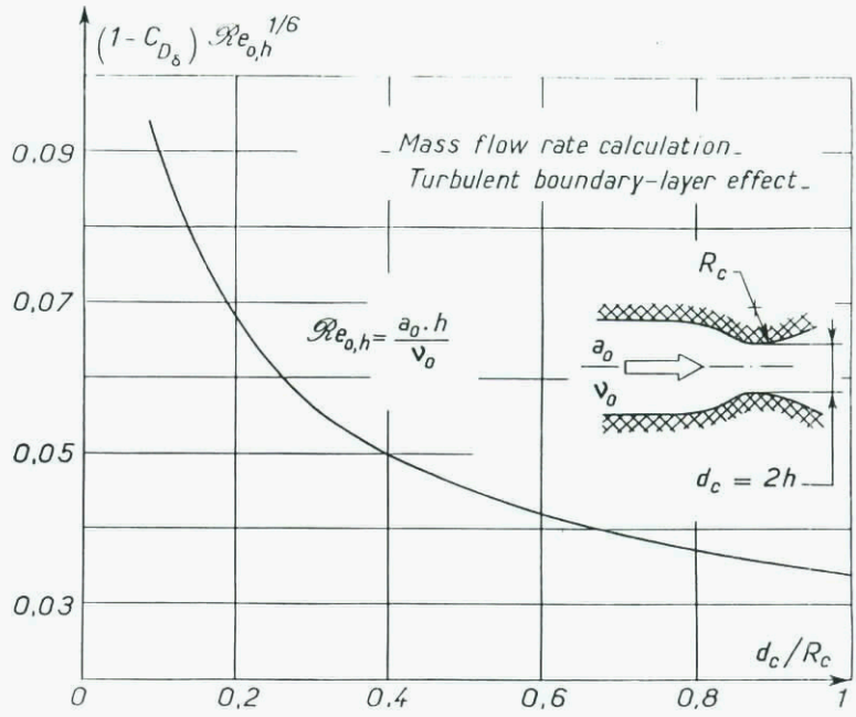
Figure 17 bis - b Mass-flow rate calculation Turbulent boundary layer effect (Masure [30])
