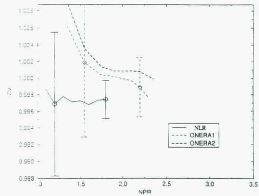
Figure 37 DNW 3" starboard cubic nozzle Velocity coefficient
