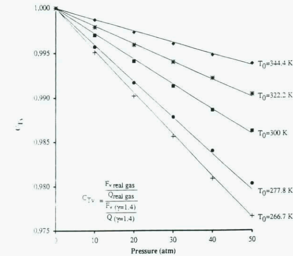
Figure 27 Real gas effect on thrust (Virial effect) for a sonic nozzle Johnson's results for C_{Tv}
