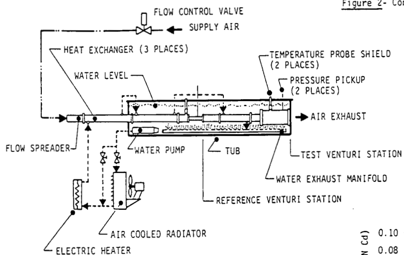
Figure 3- Venturi Screening Facility
