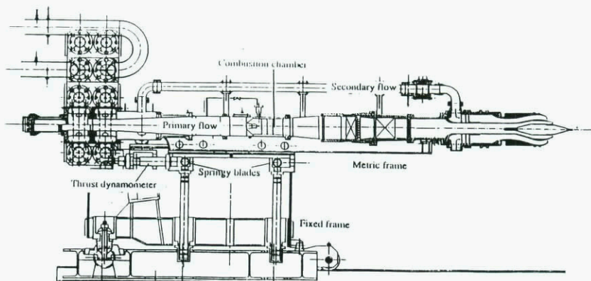
Figure A.3 ONERA dynalpy bench BD2
