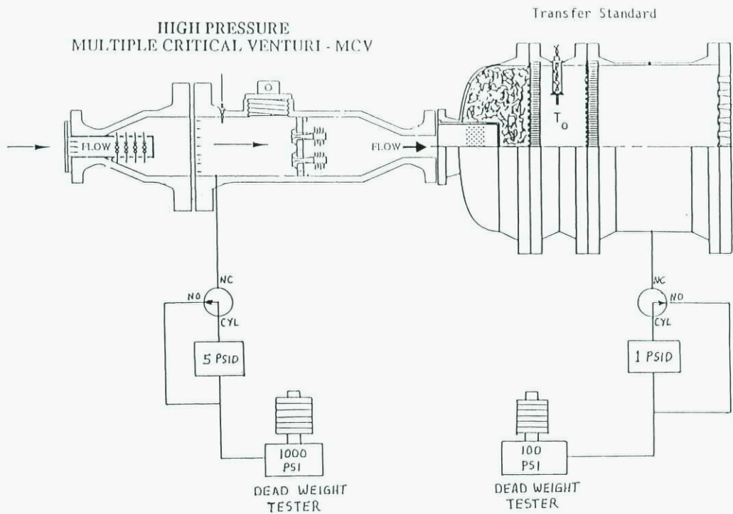
Figure 10 MCV airflow calibration Instrumentation schematic
