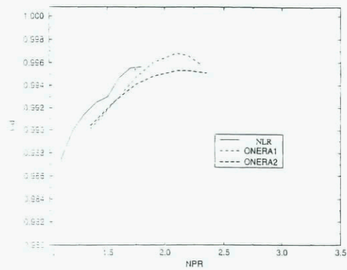
Figure 36 DNW 3" starboard cubic nozzle Flow coefficient
