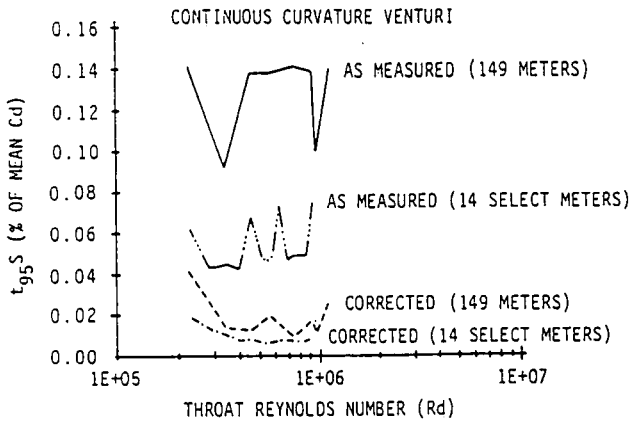
Figure 5- Throat Diameter Correction Results ( 163 Venturi Meters)
