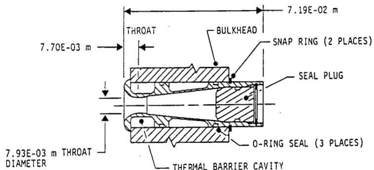
Figure 2- Continuous Curvature Venturi Configuration
