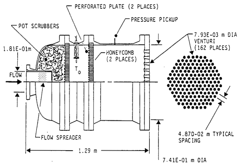
Figure 1- Transfer Standard
