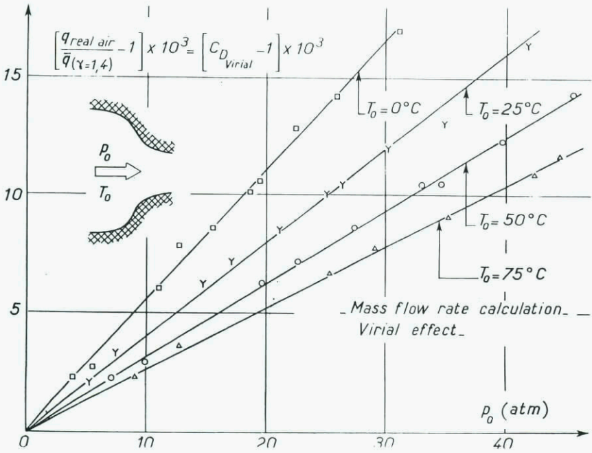
Figure 17 bis - c Mass-flow rate calculation Virial effect (Masure [30])
