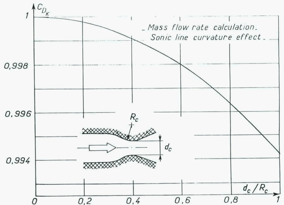
Figure 17 bis - a Mass-flow rate calculation Sonic line curvature effect (Masure [30])
