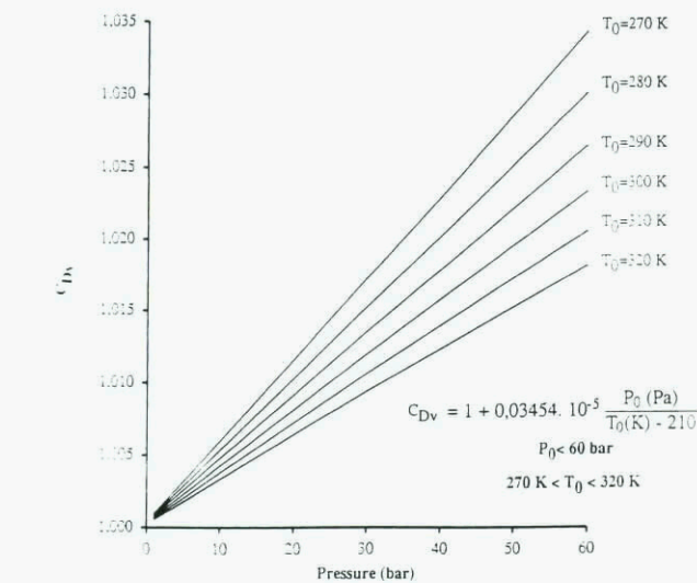
Figure 25 Real gas effect on mass flow rate (Virial effect) for a sonic venturi Masure's results for C_{Dv}
