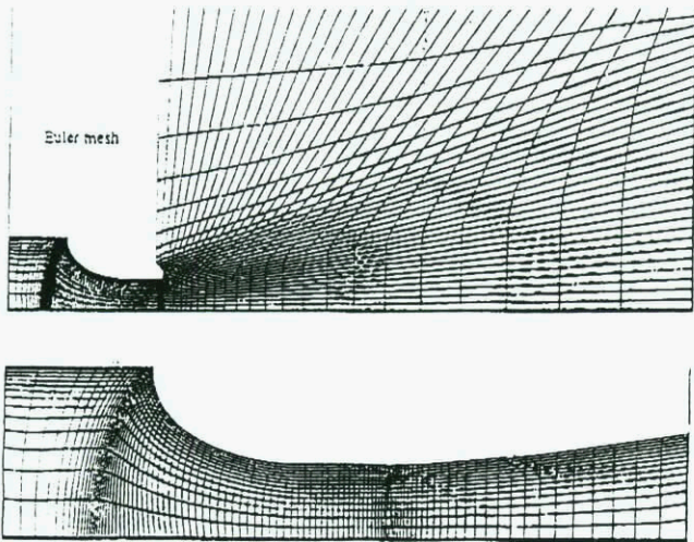
FIGURE 15 - Reference condition for reference ASME nozzle
