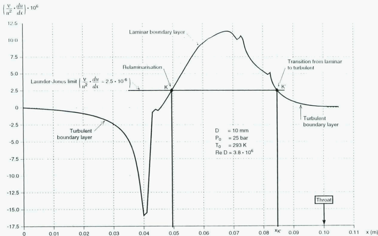
Fig. 23 - Relaminarisation criteria (Laufer-Jones) applied to ONERA short radius nozzle ( \frac{d_c}{R_c} = 2 ).
