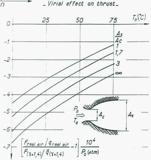
Figure 17 bis - d Virial effect on thrust
