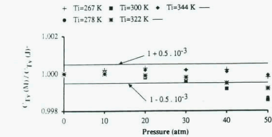
Figure 28 Real gas effect on thrust for a sonic nozzle Ratio of C_{Tv} coefficients from Masure (M) and Johnson (J)
