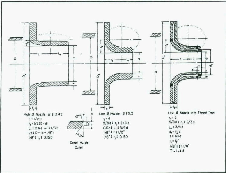
Figure 14 ASME Long Radius Nozzle (LRN)
