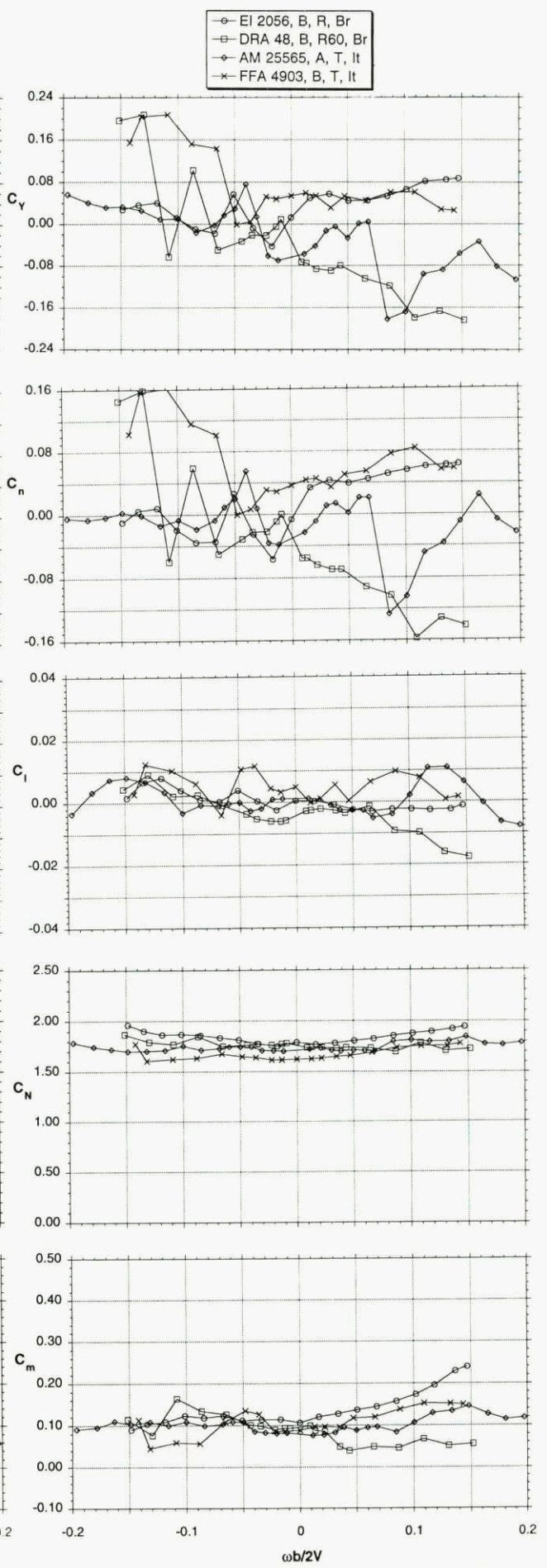
Figure 4.13 - Rotary-balance tests, BWLVHT, 50° AOA
