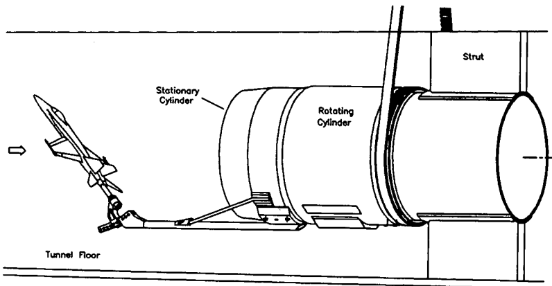
Fig A4.2.23 Orbital platform rotary apparatus
