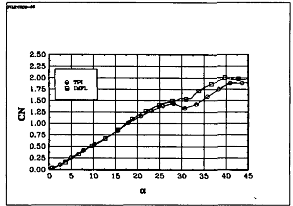
Fig 6.2 The coefficient CN: BWLVH, \beta = -10^\circ
