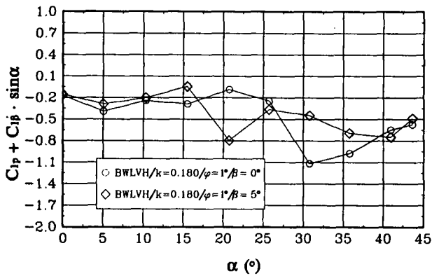
Fig. 5.18 The effect of sideslip on C_p + C_{pb} \sin \alpha ( V=30 m/s, k = 0.180 , \varphi = \pm 1^\circ ).
