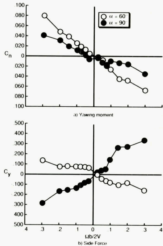
Figure 7.12. Comparison of aerodynamic characteristics for rectangular ogive at 60° and 90° angle of attack.
