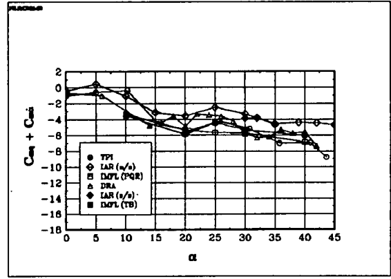
Fig 6.28 The derivative Cm q^* : BWLVHST, \beta = 0^\circ
