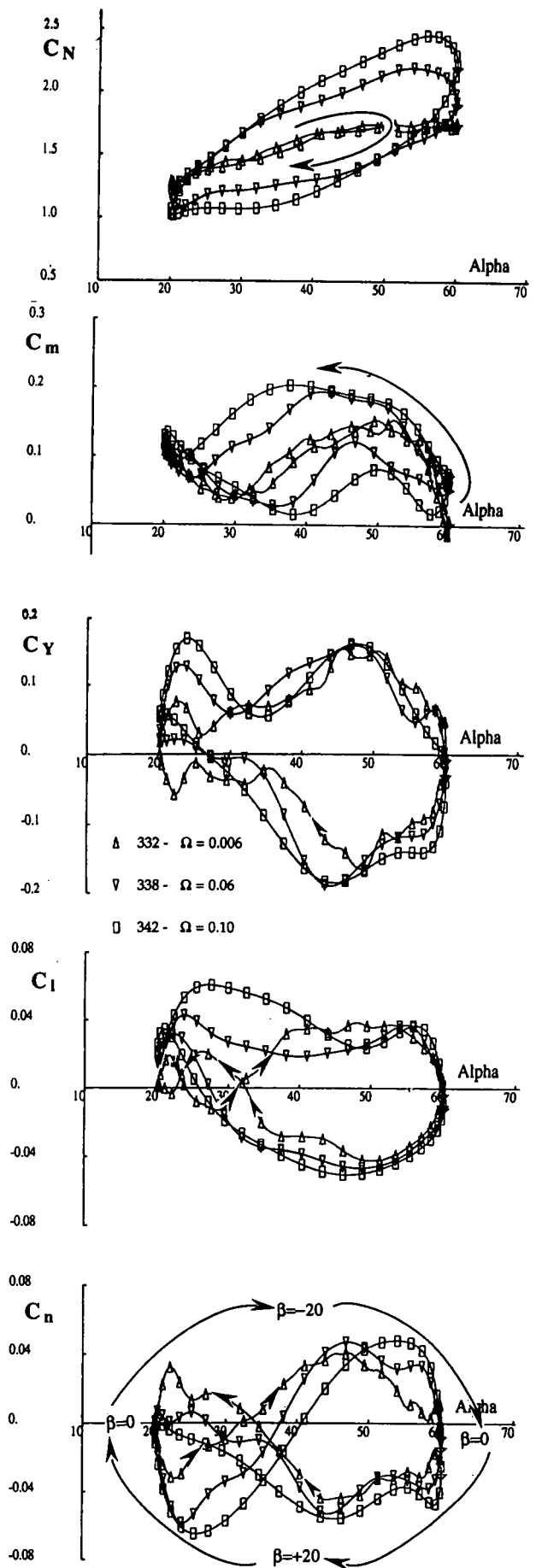
Fig 5.58 Large amplitude oscill. coning tests - Rate effect (cont.) \lambda = 20^\circ , mean \alpha = 40^\circ , mean \beta = 0^\circ BWLVHST Configuration
