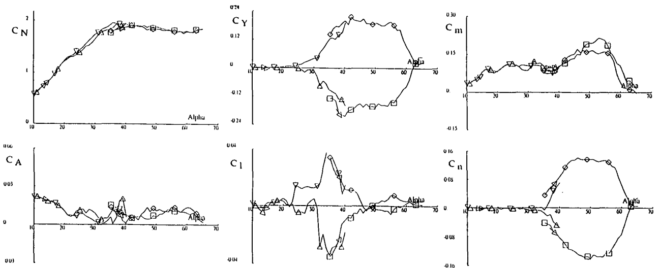
Fig 3.61 - BWLHV Configuration - slow AOA sweeps - Repeatability tests
