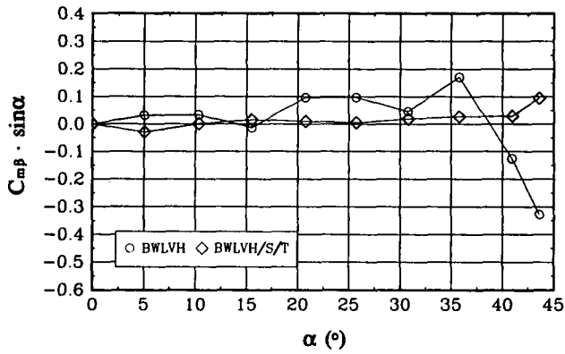
Fig. 5.16 The effect of configuration on C_{mp} \sin \alpha ( V=30 m/s, \beta = 0^\circ , k = 0.180 , \varphi = \pm 1^\circ ).
