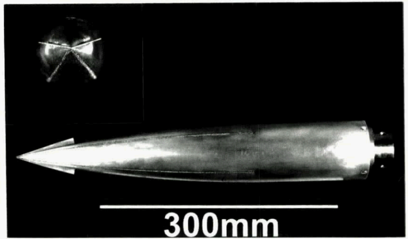
Fig 2.2 Forebody strakes and transition fixing on model WG16B
