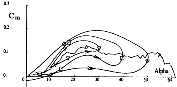
Fig. 5.47 Large amplitude pitch oscillations at \beta = 0^\circ , f = 1 Hz Amplitude effect Mean \alpha = 20^\circ BWLHVST Configuration
