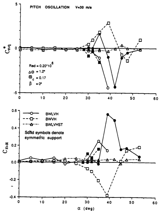
Fig. 5.31 Configurational effects on the derivatives C_{nq}^* and C_{n\alpha} .
