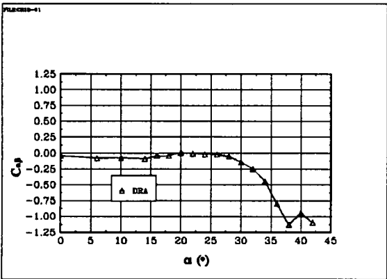
Fig 6.61 The derivative Cn_{\beta} : BWLVH, \beta = 0^{\circ}
