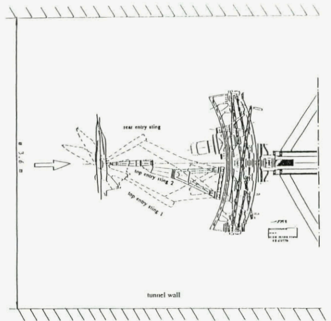
Fig 2.30 FFA rotary balance sting options
