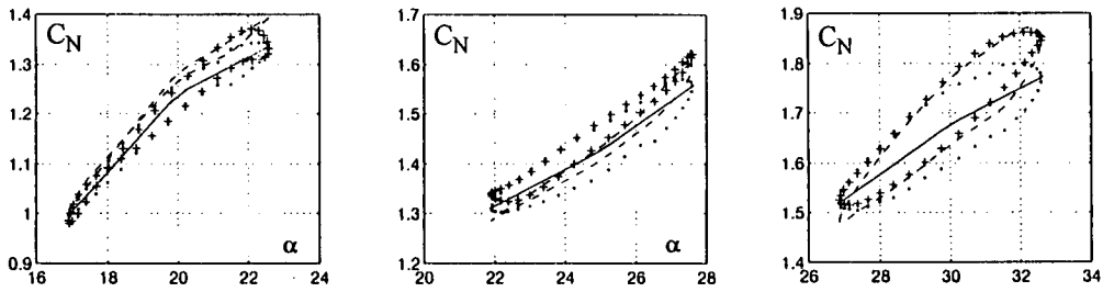
Fig 8.24 Normal force predictions of oscillatory tests ( f = 2.5 Hz).
