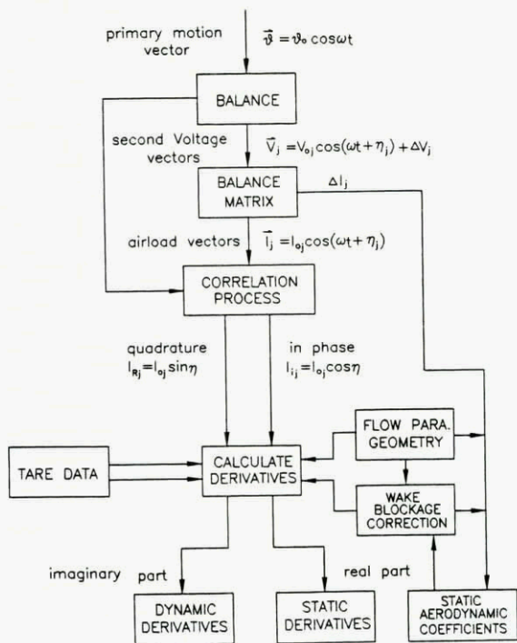
Fig 2.21 IAR data reduction for oscillatory tests
