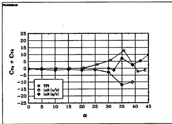
Fig 6.31 The derivative C_{Yq^*} : BWLVH, \beta = 0^\circ
