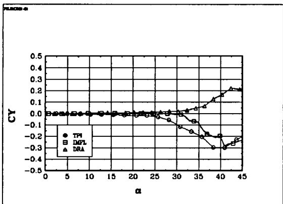
Fig 6.13 The coefficient C_Y : BWLVH, \beta = 0^\circ
