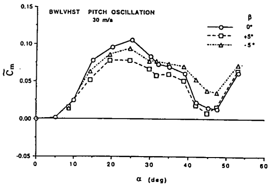
Fig A4.2.22 Effect of sideslip and motion on time-averaged pitching moment 2
