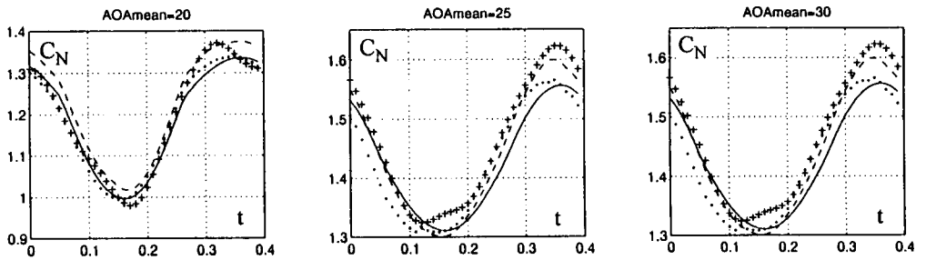
Fig 8.25 Normal force predictions as functions of time. Oscillatory tests at f = 2.5 Hz.
