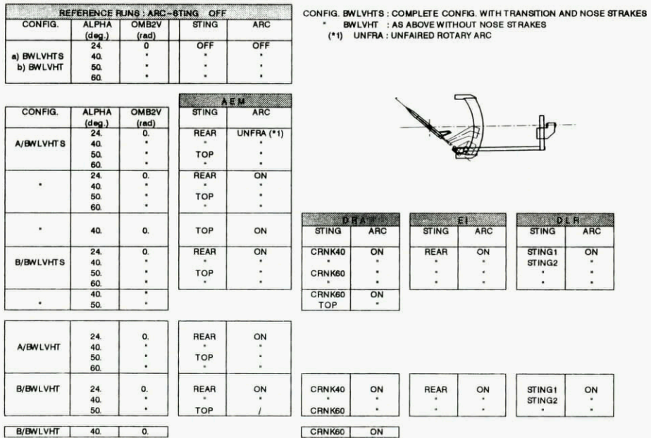
Fig 2.12 Flow analysis with rotary rig in AEM water tunnel
