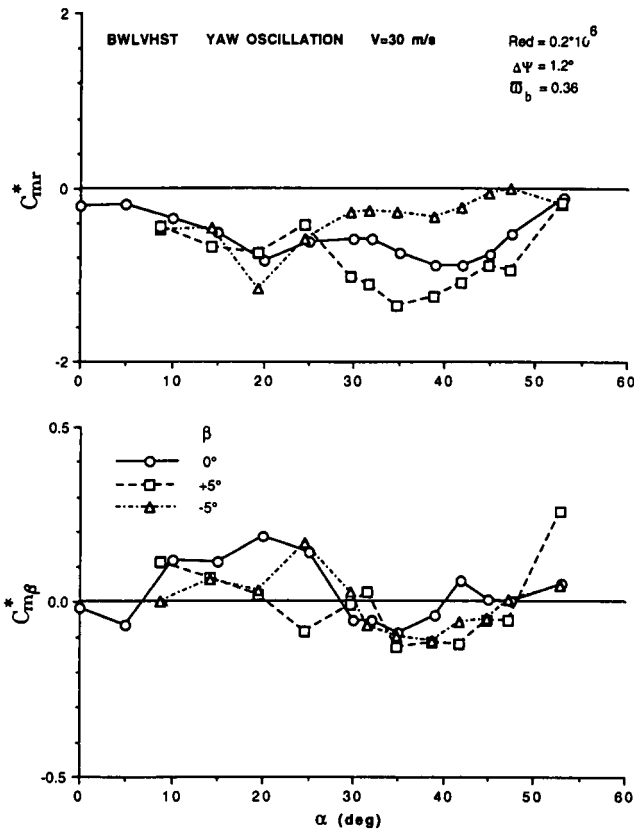
Fig 5.38 The effect of sideslip on derivatives C_{mr}^* and C_{mp}^* for BWLVHST configuration in yaw oscillation.
