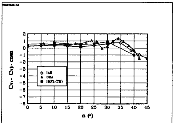
Fig 6.64 The derivative CYr^* : BWLVHST, \beta = 0^{\circ}
