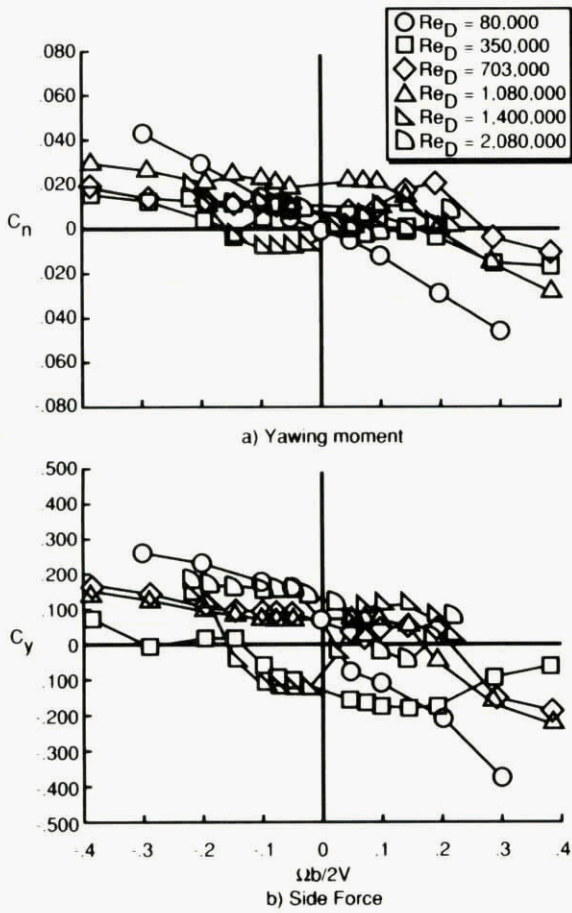
Figure 7.13. Effect of rotation rate and Reynolds number on aerodynamic characteristics for the circular ogive at 60^\circ angle of attack.
