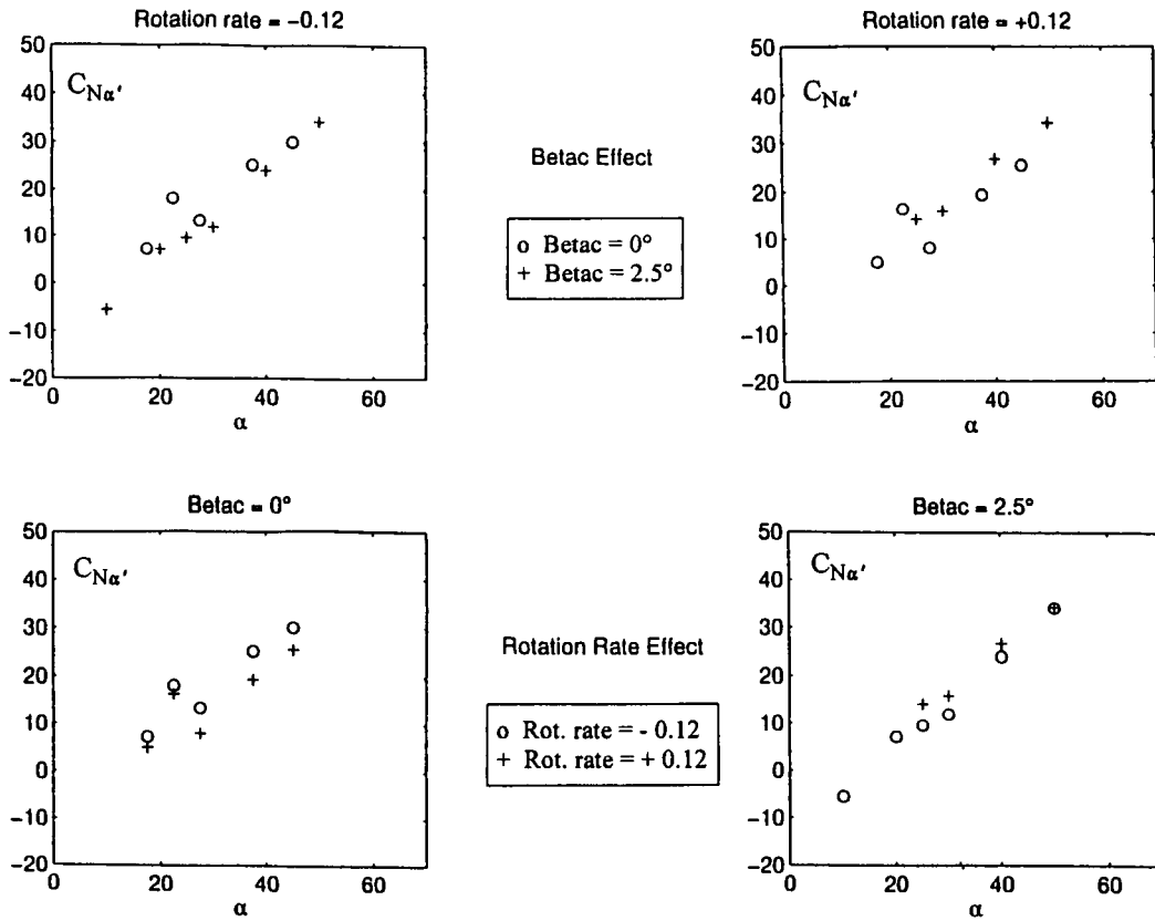
Fig 8.5 Small amplitude oscillatory coning derivatives. Sideslip and rotation rate effects on C_{N\alpha'} .
