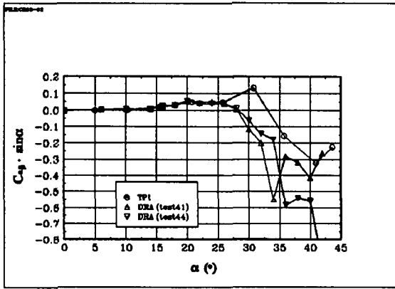
Fig 6.49 The derivative Cn\beta \sin\alpha : BWLVH, \beta = 0^\circ
