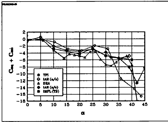
Fig 6.27 The derivative Cm q^* : BWLVH, \beta = 0^\circ
