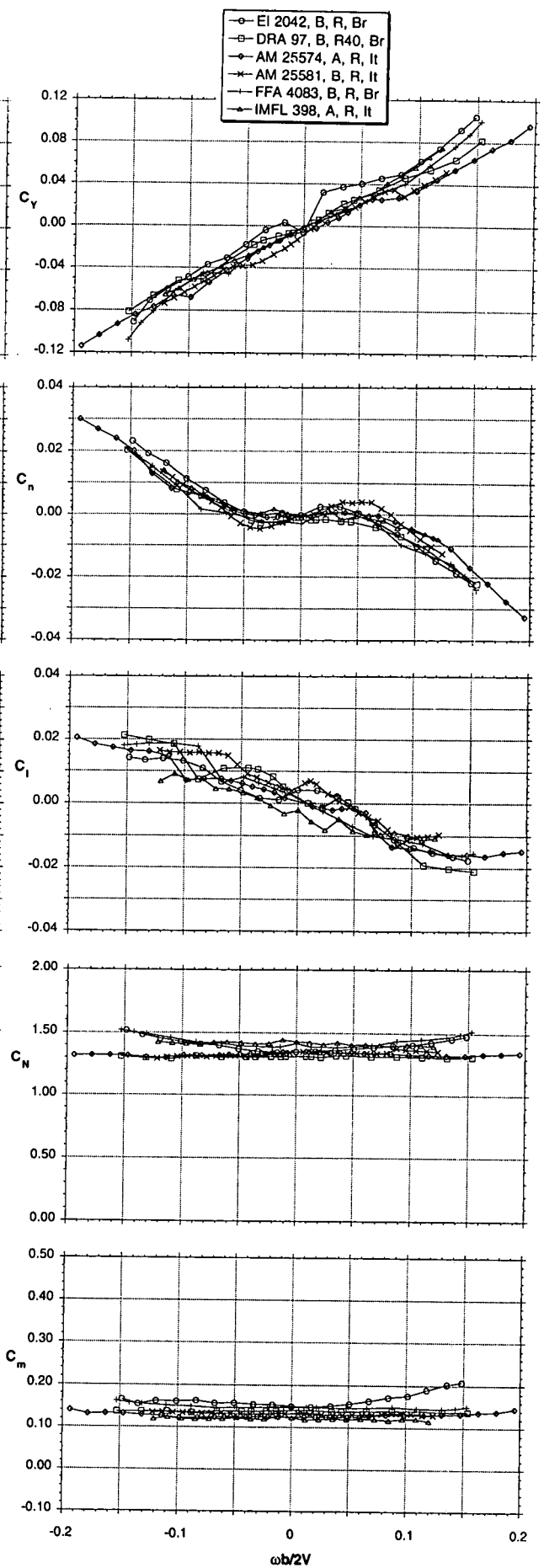
Figure 4.7 - Rotary-balance tests, BWLVHST, 24^\circ AOA
