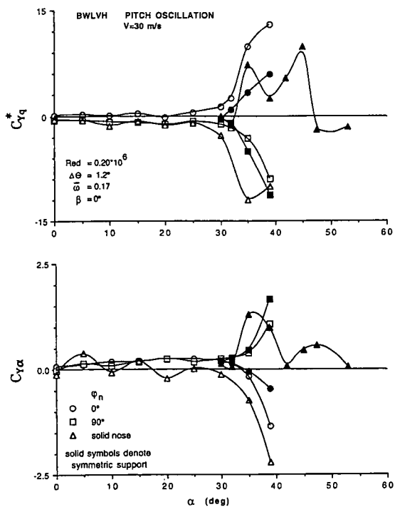
Fig A4.2.20 Effect of rotating nose tip on derivatives C_{Yq}^* and C_{Yq}
