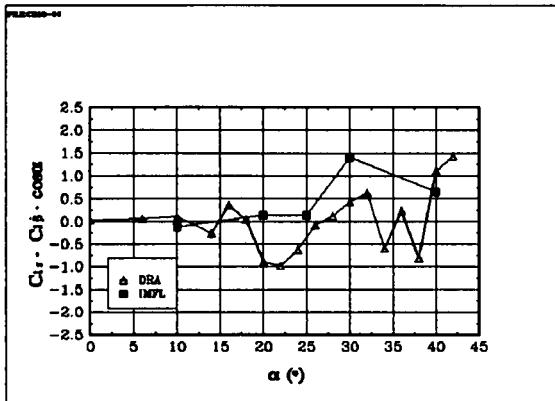
Fig 6.67 The derivative Cl_r : BWLVH, \beta = 0^\circ
