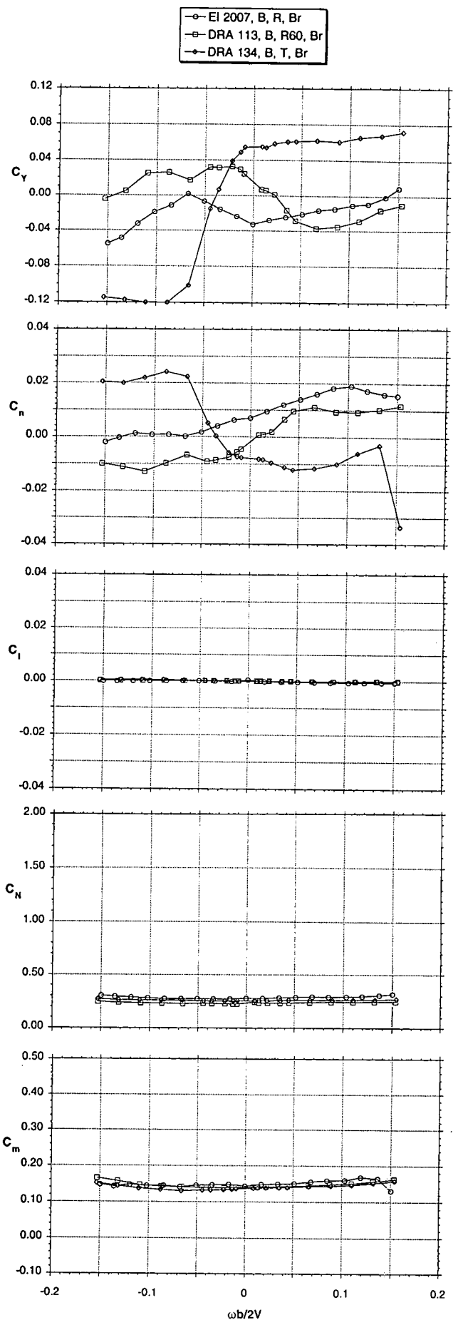
Figure 4.3 - Rotary-balance tests, BST, 50° AOA
