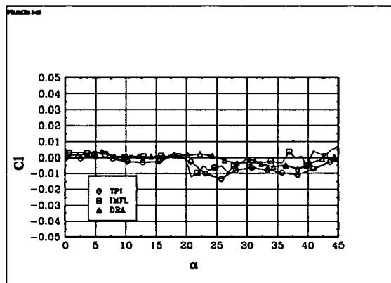
Fig 6.12 The coefficient C_i : BWLVHST, \beta = 0^\circ
