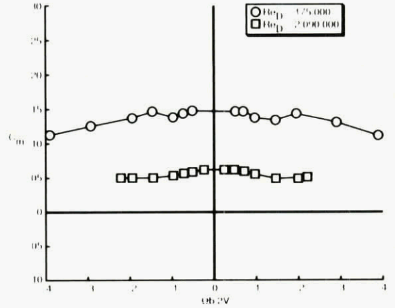
Figure 7.6. Effect of rotation rate and Reynolds number on pitching moment characteristics for the rectangular ogive at 60° angle of attack.
