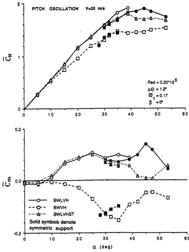
Fig. 5.28 Configurational effects on the longitudinal aerodynamic coefficients.
