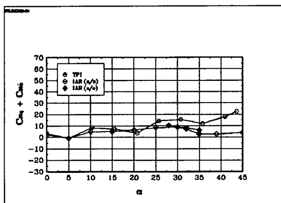
Fig 6.43 The derivative C_{Nq} : BWVH, \beta = 0^\circ
