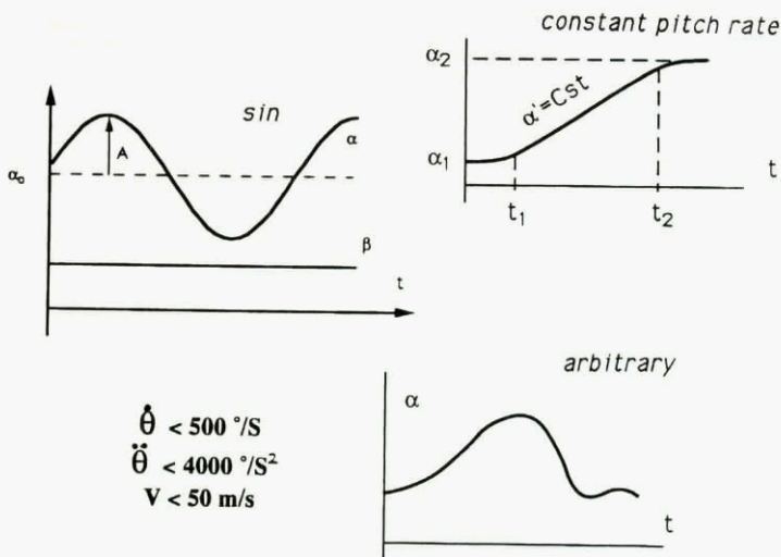
Fig 2.24 Typical motion time-histories for PQR rig
