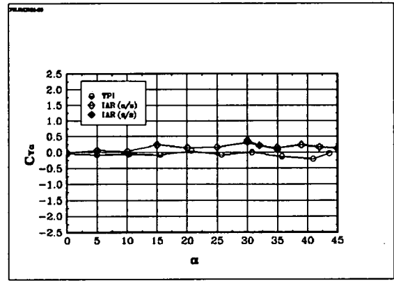
Fig 6.30 The derivative C_{Y\alpha} : BWLVHST, \beta = 0^\circ
