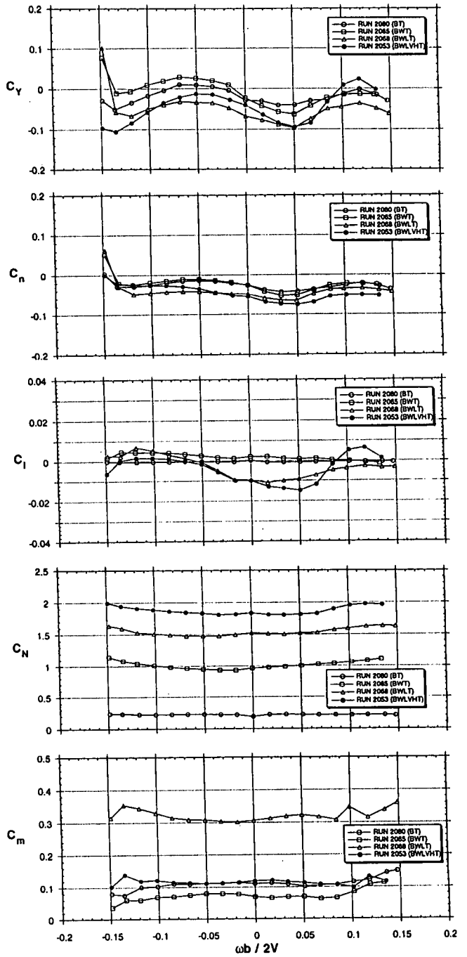
Fig 3.28 - Configuration buildup effects at \alpha = 39^\circ , R=0.955 \times 10^6 , strakes off
