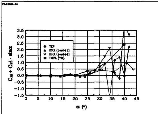
Fig 6.53 The derivative Cy\beta^* : BWLVH, \beta = 0^\circ
