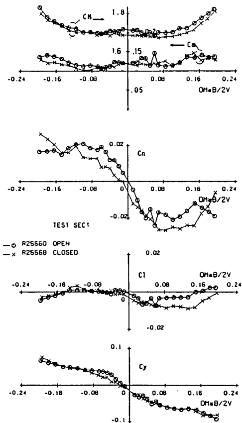
Fig 3.56 - Open versus closed test section walls BWLHVST Configuration - AeM tests - \alpha = 50^\circ
