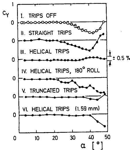
Fig A4.3.5 Effect of helical and straight body trips on side force of ogive-cylinder body 38
