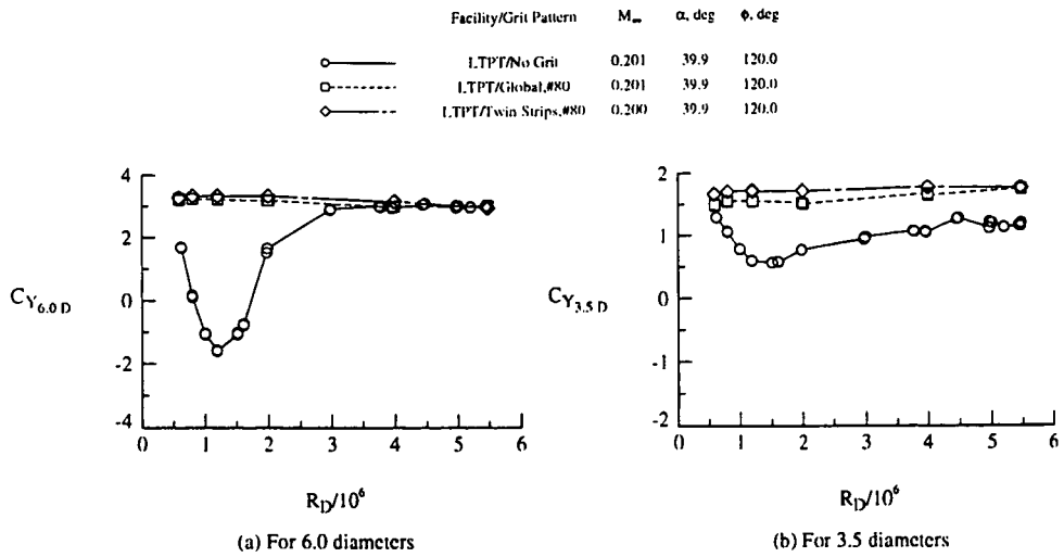
Fig A3.4 - NASA Langley experiment - Effect of transition tripping pattern on variation of total integrated side force with Reynolds number for ogive/cylinder model and two model lengths.
