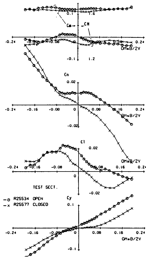
Fig 3.58 - Open versus closed test section walls BWLHVT Configuration - AeM tests - \alpha = 24^\circ
