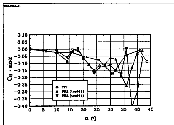
Fig 6.47 The derivative C_{l\beta \sin \alpha} : BWLVH, \beta = 0^\circ
