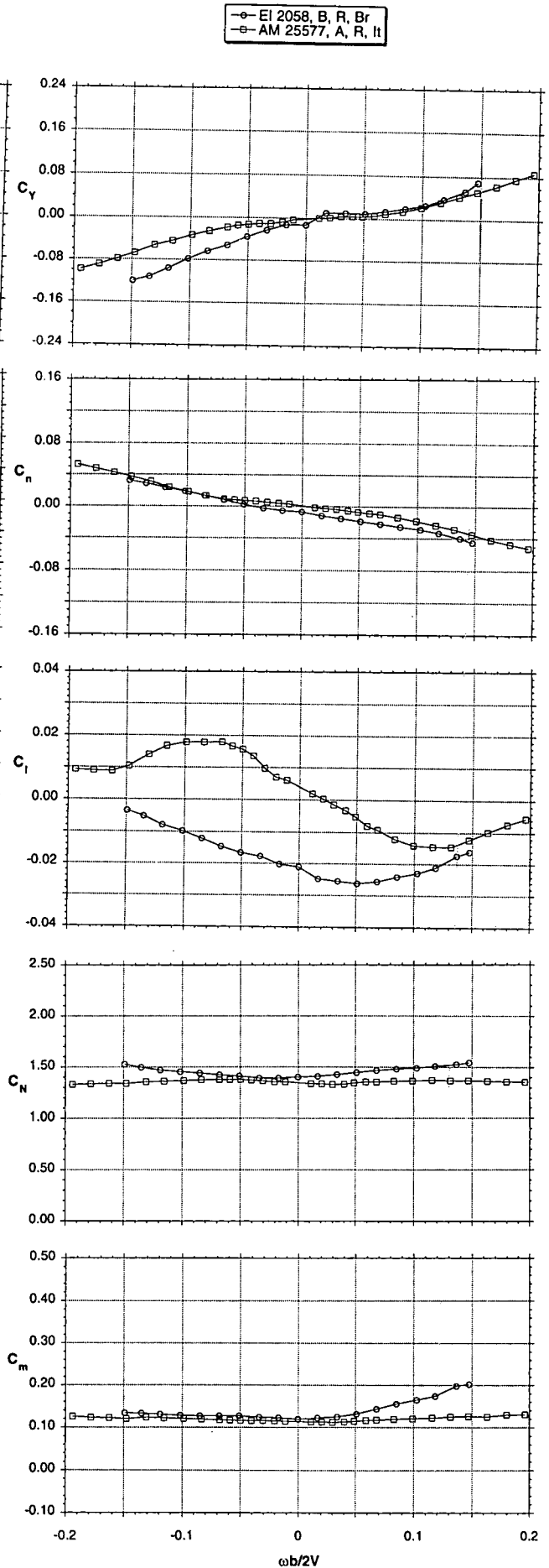
Figure 4.11 - Rotary-balance tests, BWLVHT, 24° AOA
