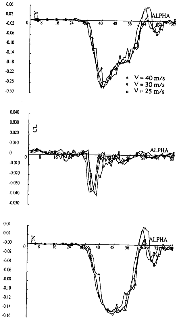
Fig. A4.3.8 Effect of Reynolds number on the lateral characteristics of the basic configuration (BC) 40
