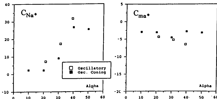
Fig 8.11 Comparison of oscillatory and oscillatory coning derivatives. Amplitude = 20°.
