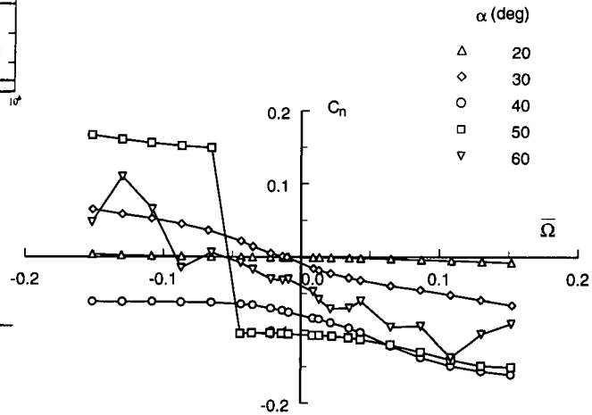
Fig A4.4.5 Body-alone characteristics at Re_d = 0.3 \times 10^6
