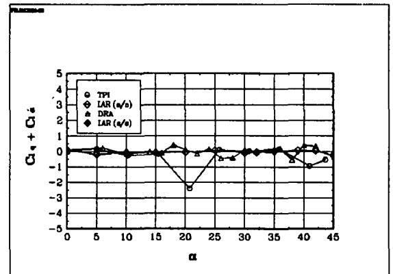
Fig 6.36 The derivative Cl_\alpha^* : BWLVHST, \beta = 0^\circ
