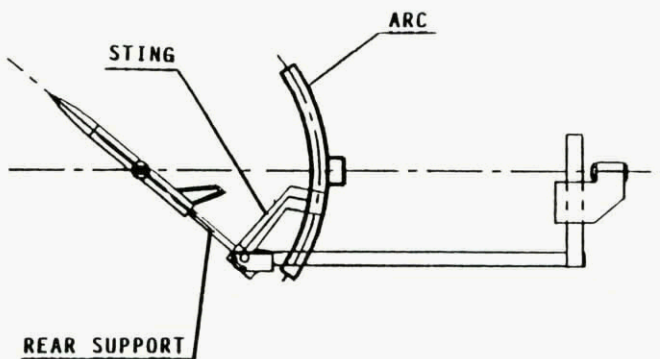
Figure 4.20(a) - AerMacchi water tunnel rotary-rig
