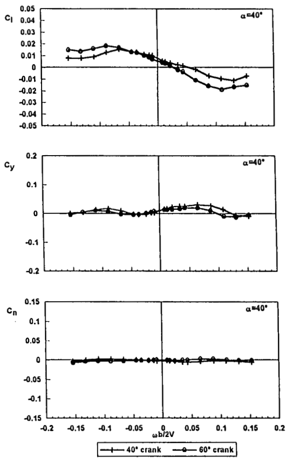
Fig 3.50.b - BWLHVST Configuration
