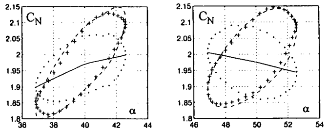
Fig 8.24 Normal force predictions of oscillatory tests ( f = 2.5 Hz).
