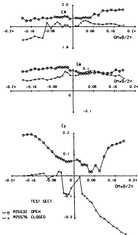
Fig 3.59 - Open versus closed test section walls, BWLHVT Config. - AeM tests - \alpha = 40^\circ
