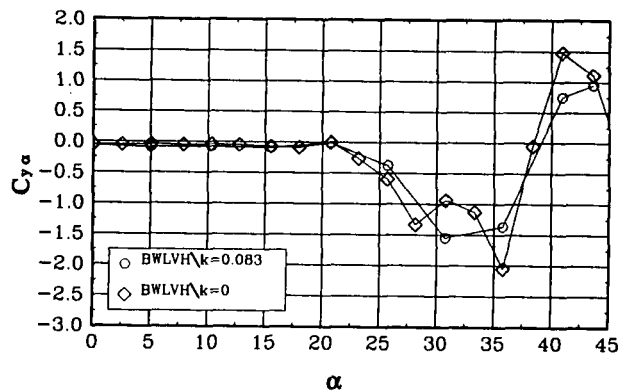
Fig. 5.19 The effect of oscillation frequency on C_{y\alpha} : comparison with static data.
