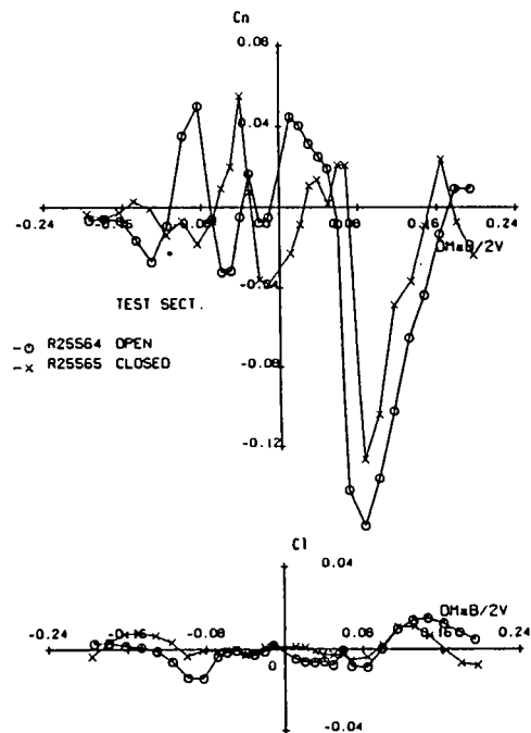
Fig 3.59 - Open versus closed test section walls, BWLHVT Config. - AeM tests - \alpha = 40^\circ
