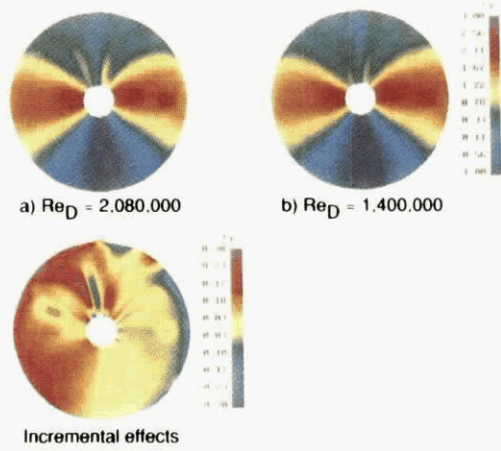
Figure 7.15. Comparison of the pressure distribution at \Omega b/2V = -0.1 for the circular ogive at 60^\circ angle of attack for two Reynolds numbers.
