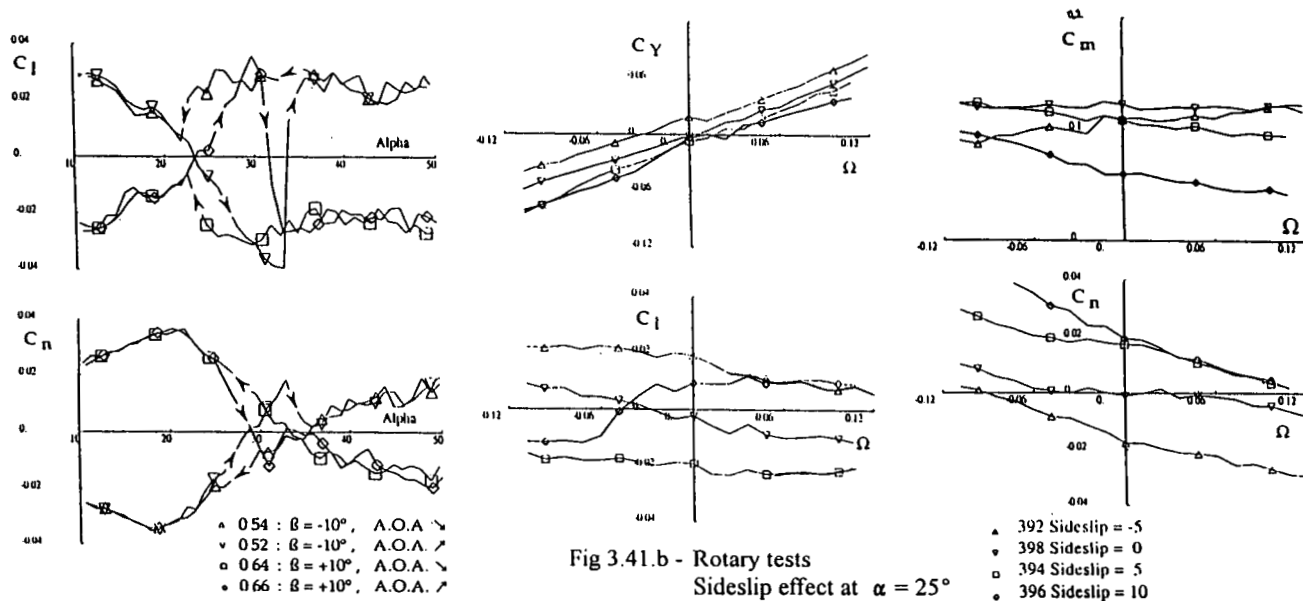
Fig 3.41 - BWLHVST Configuration
