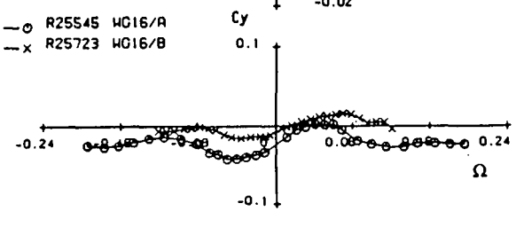
Fig 3.26 - Model A vs. Model B results - BWLVHST conf. AeM tests - \alpha = 40^\circ
