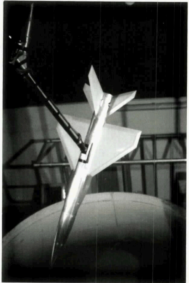
Fig 2.7 WG16A model on rotary balance in AEM wind tunnel
