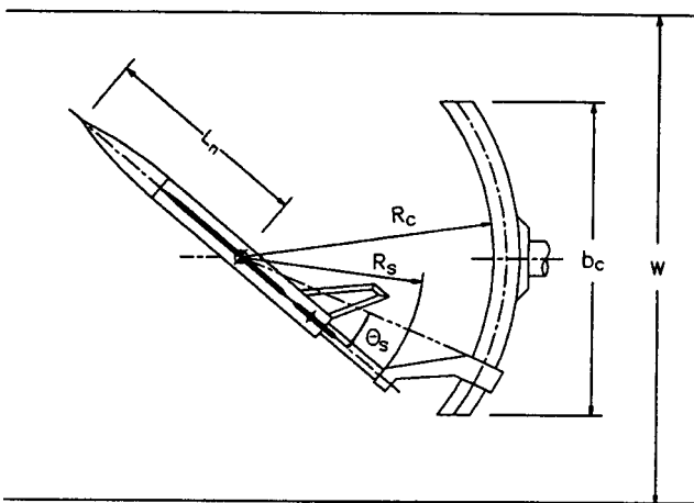
Fig A4.4.3 Schematic of test installation
