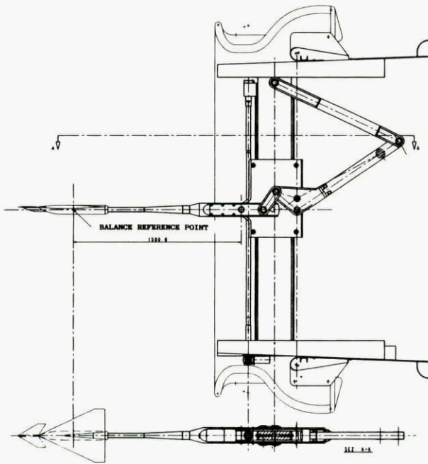
Fig 2.5 AEM static balance
