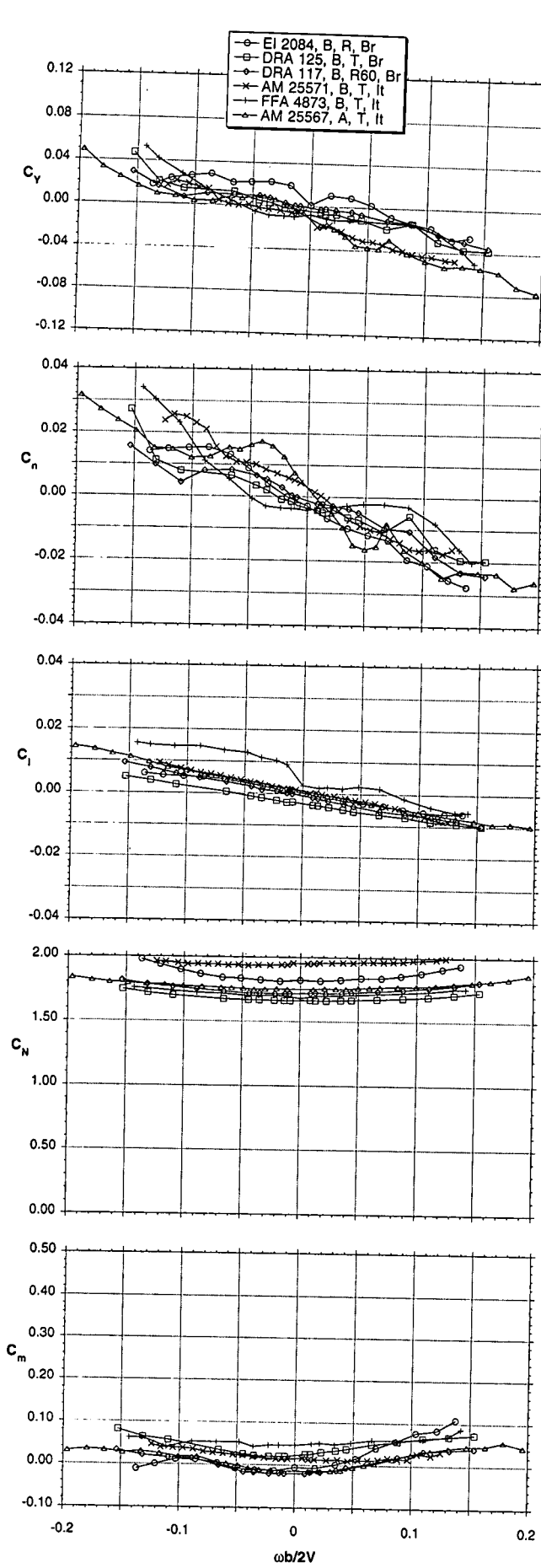
Figure 4.10 - Rotary-balance tests, BWLVHST, 60° AOA
