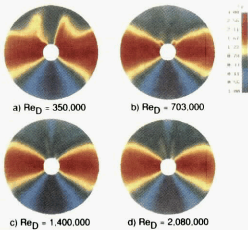
Figure 7.14. Pressure distribution for the circular ogive at 60^\circ angle of attack and \Omega b/2V = 0.0 .
