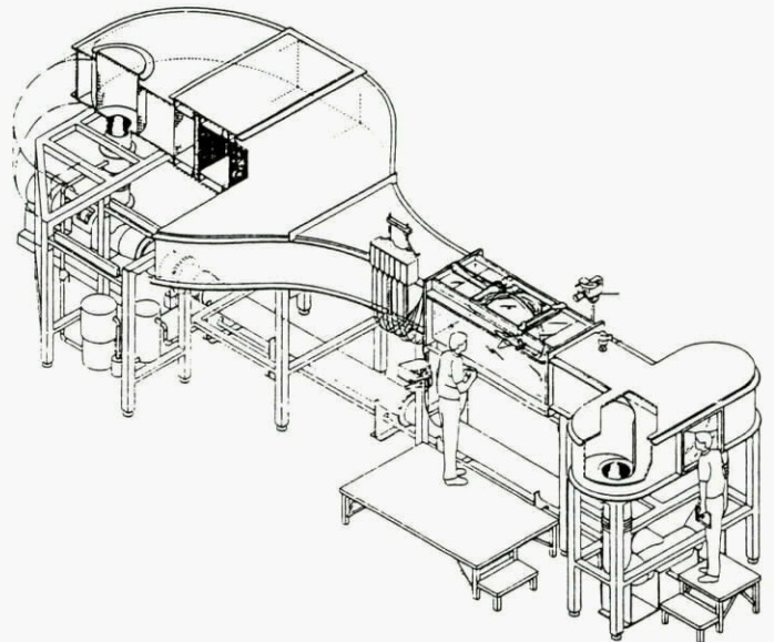
Fig 2.9 Eidetics EI2436 water tunnel at AEM
