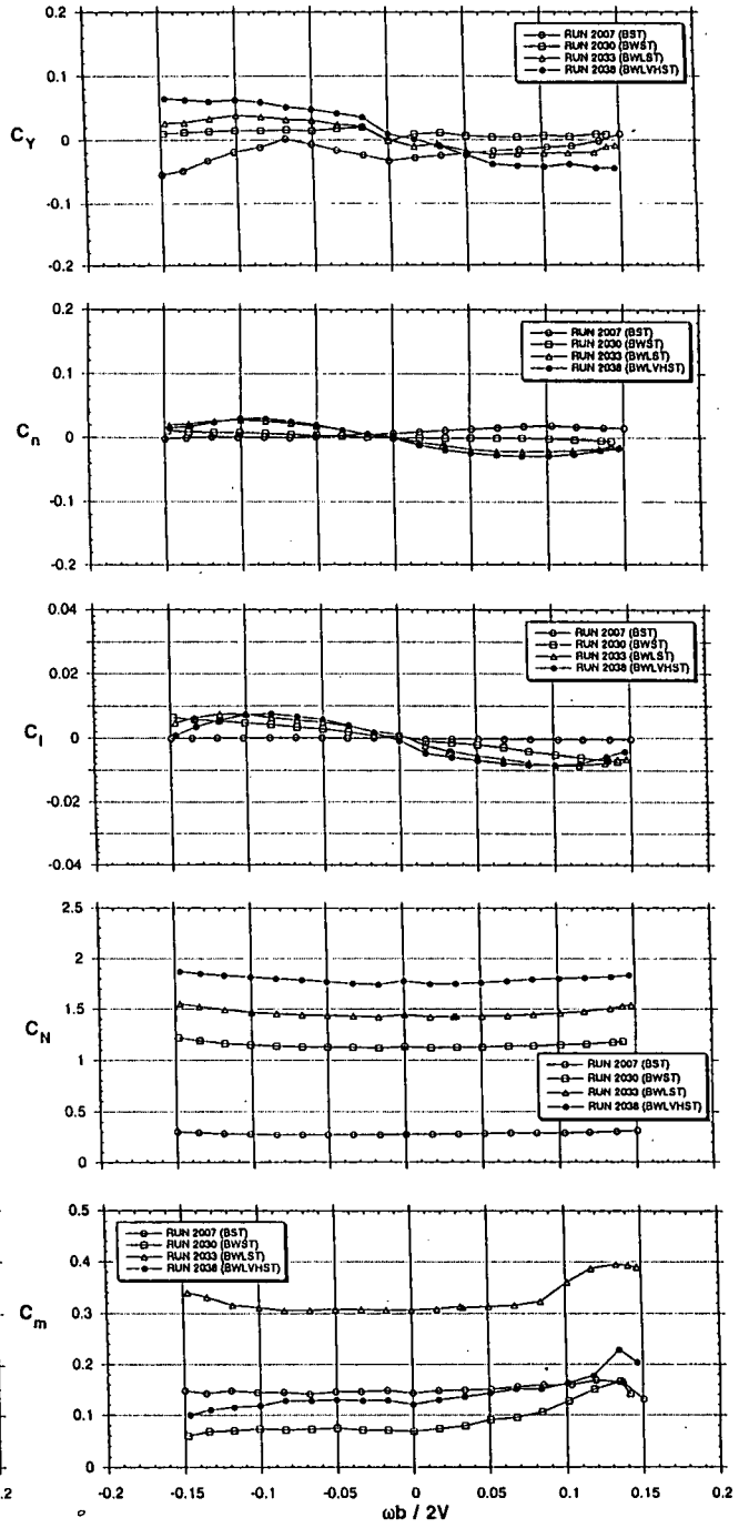
Fig 3.32 - Configuration buildup effects at \alpha = 51^\circ , R=0.955 \times 10^6 , strakes on
