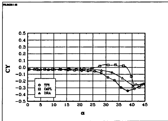
Fig 6.16 The coefficient C_Y : BWLVH, \beta = 5^\circ
