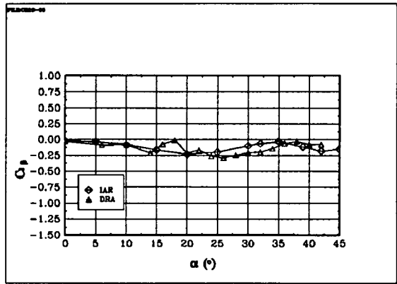
Fig 6.60 The derivative Cj_{\beta} : BWLVHST, \beta = 0^{\circ}
