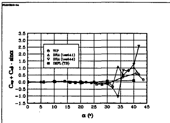
Fig 6.55 The derivative Cnp\beta^* : BWLVH, \beta = 0^\circ
