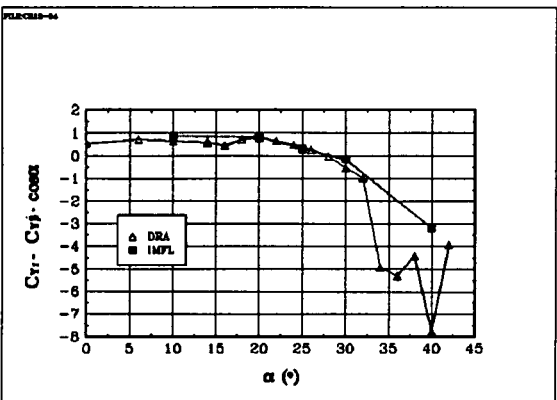
Fig 6.63 The derivative CYr^* : BWLVH, \beta = 0^{\circ}
