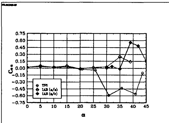
Fig 6.37 The derivative Cn_\alpha : BWLVH, \beta = 0^\circ
