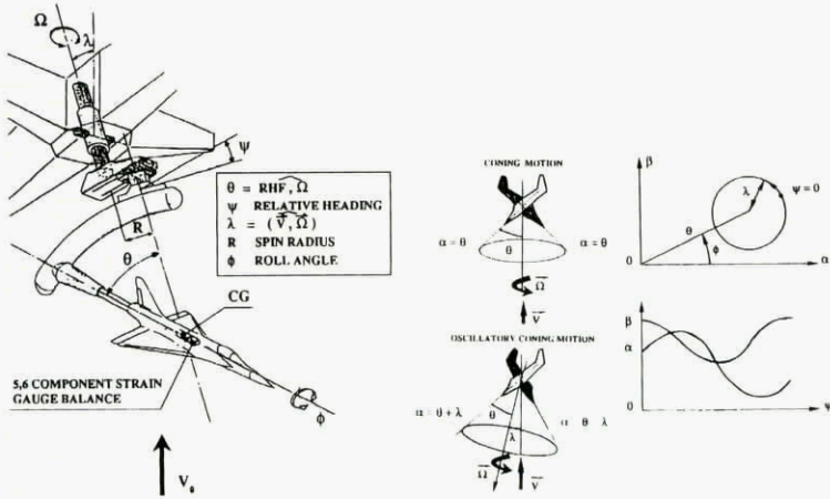
Fig 2.25 ONERA-IMFL 'Toune-Broche' oscillatory coning rig installed in 4m vertical wind tunnel 'SV4'
