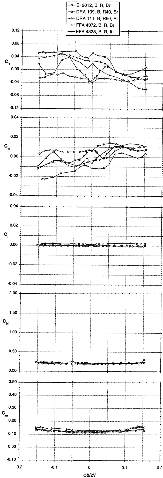
Figure 4.2 - Rotary-balance tests, BST, 40° AOA
