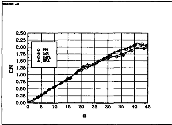
Fig 6.1 The coefficient CN: BWLVH, \beta = 0^\circ
