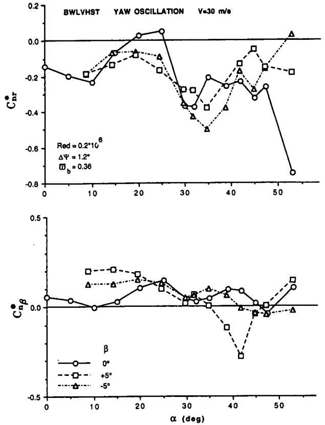
Fig 5.37 The effect of sideslip on derivatives C_{ar}^* and C_{ap}^* for BWLVHST configuration in yaw oscillation.
