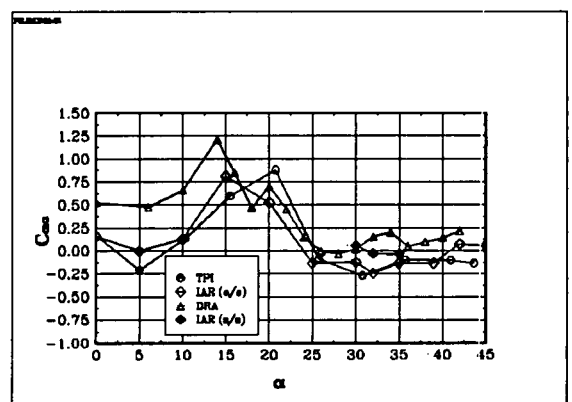
Fig 6.24 The derivative C_{m\alpha} : BWLVHST, \beta = 0^\circ
