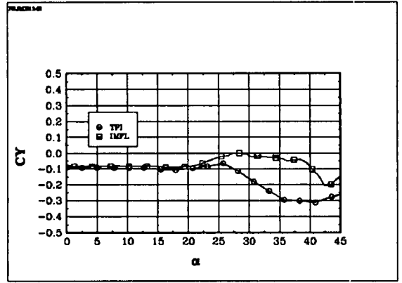
Fig 6.18 The coefficient C_Y : BWLVH, \beta = 10^\circ
