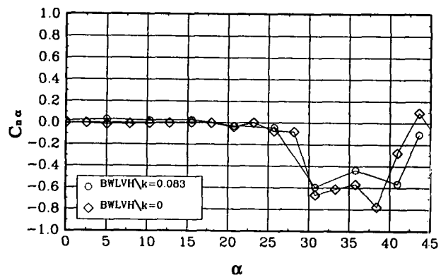
Fig. 5.21 The effect of oscillation frequency on C_{na} : comparison with static data.
