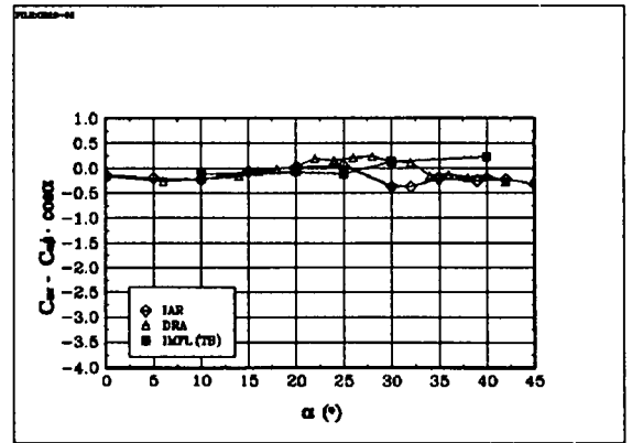
Fig 6.66 The derivative C_{nr} : BWLVHST, \beta = 0^\circ
