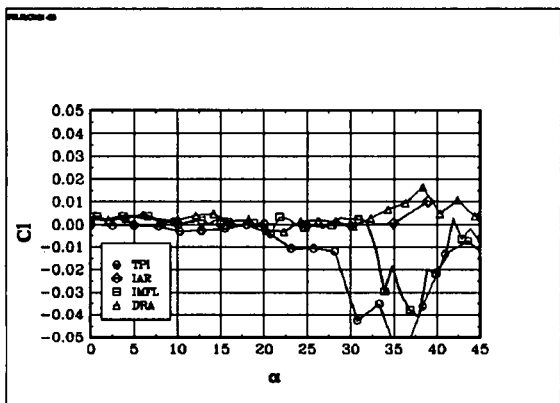
Fig 6.11 The coefficient C_i : BWLVH, \beta = 0^\circ
