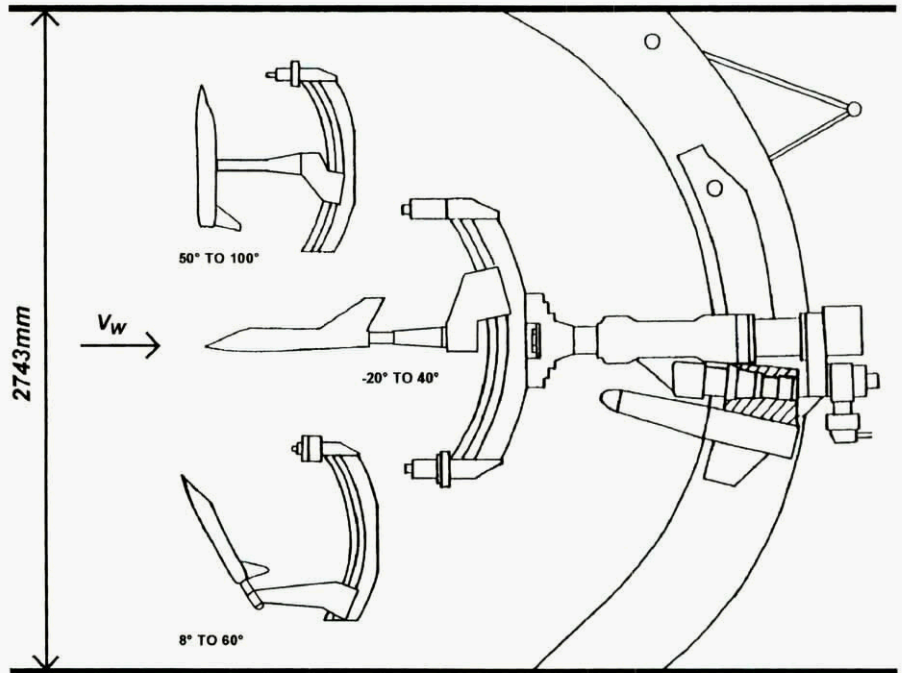
Fig 2.13 General arrangement of DRA Inexorable Drive Rig
