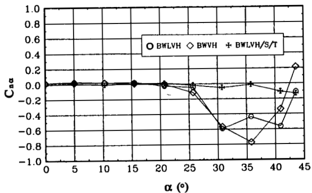
Fig. 5.14 The effect of configuration on C_{n\alpha} ( V=30 m/s, \beta=0^\circ , k=0.083 , \theta=\pm 1^\circ ).
