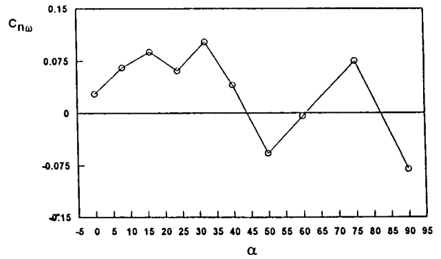
Fig 3.37 - BWLHVST Configuration, Effect of Angle of Attack on C_n and C_{n\omega}
