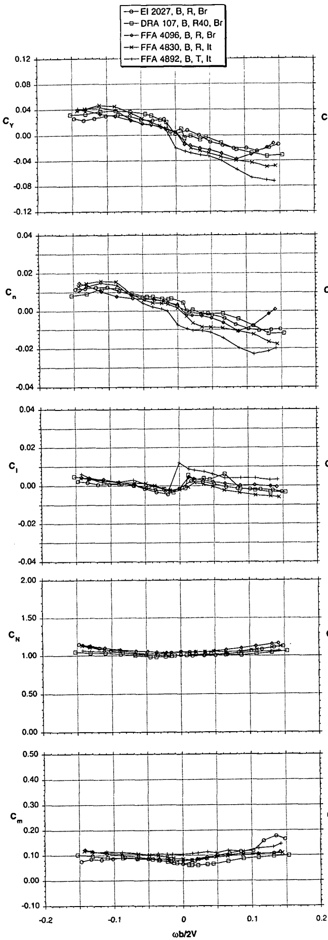
Figure 4.4 - Rotary-balance tests, BWST, 40° AOA
