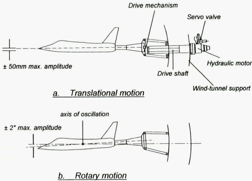
Fig 2.13 General arrangement of DRA Inexorable Drive Rig
