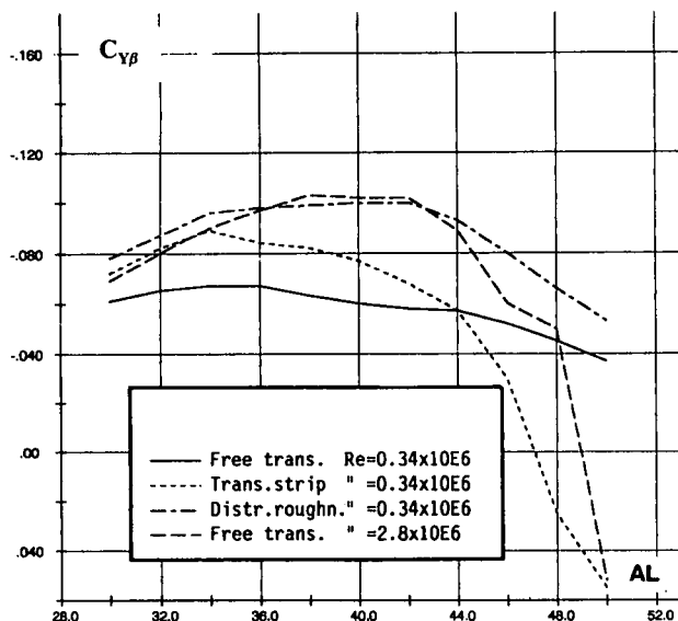
Fig A3.10 - AEM/NLR experiment - Effectiveness of transition tripping techniques in simulating Re-number effects on side force gradient due to sideslip.
