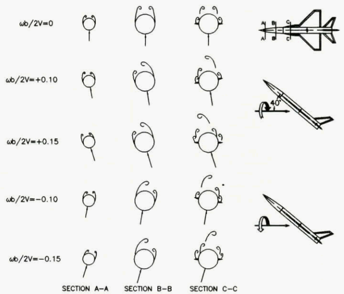
Fig A4.2.16 Analysis of flow visualization data in Fig 4.21
