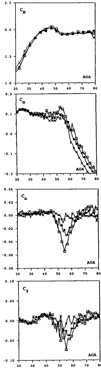
Fig 3.11 - BVLHVST Configuration - Effect of Reynolds Number, Slow Sweeps in angle of attack
