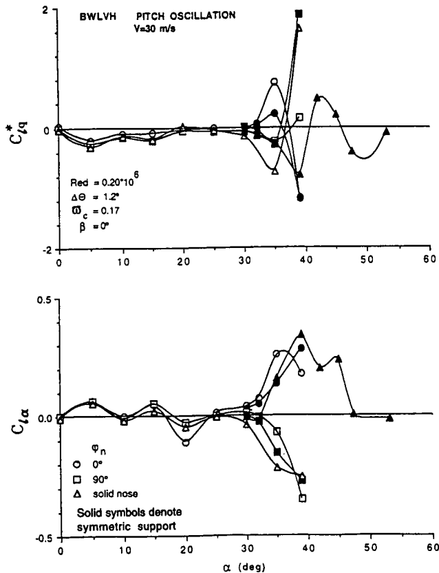
Fig. 5.26 Effect of rotating nose tip on the derivatives C_{lq}^* and C_{la} .
