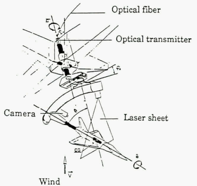
Fig 2.26 Flow visualization on Toune-Broche
