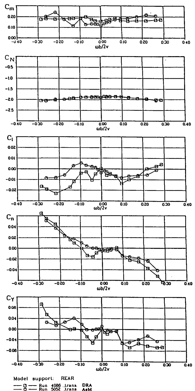
Fig 3.9.b - BWLHVST Configuration Effect of transition fixing type at \alpha = 40^\circ , V = 30 m/s
