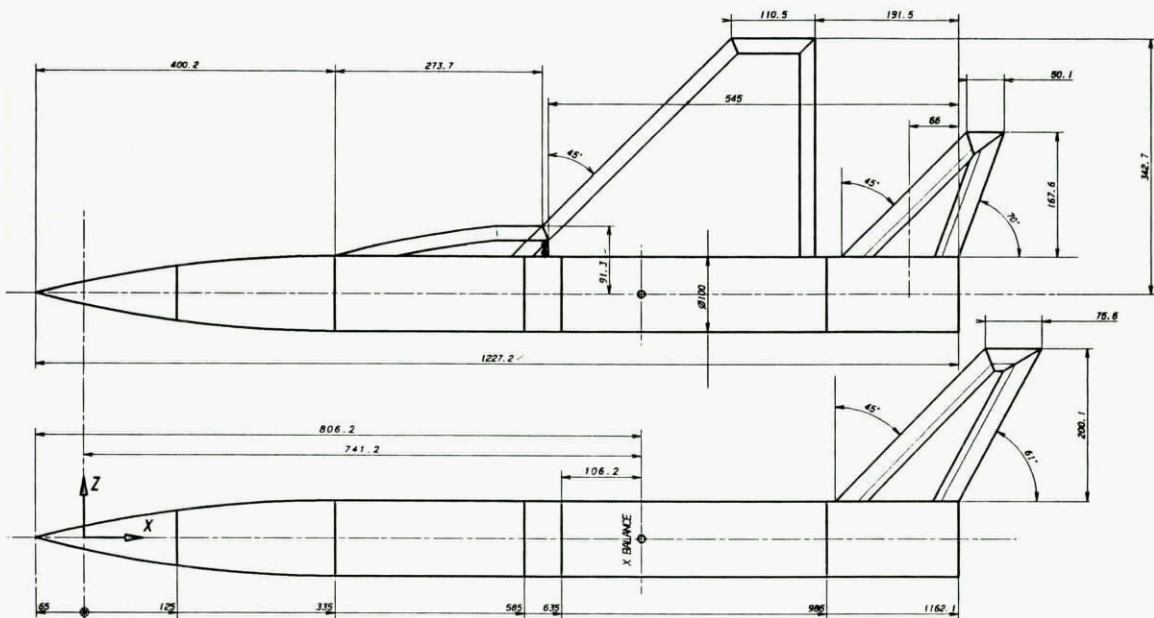
Fig 2.3 Model WG16A
