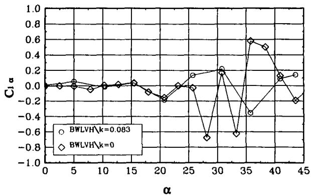
Fig. 5.20 The effect of oscillation frequency on C_{z\alpha} : comparison with static data.
