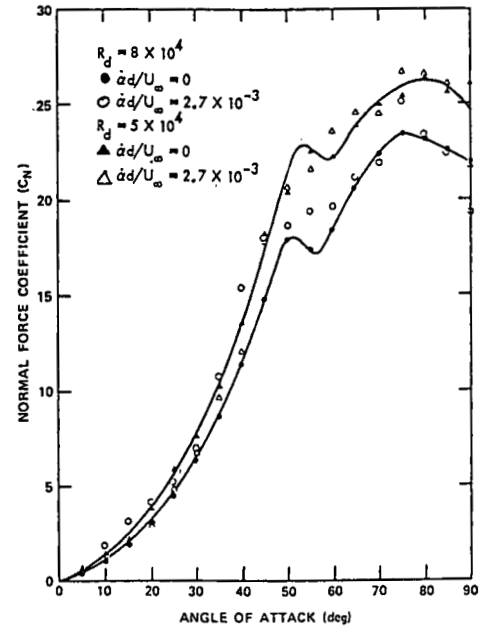
Fig A4.4.24 Pitch rate effect on ogive-cylinder normal force at critical flow conditions 67
