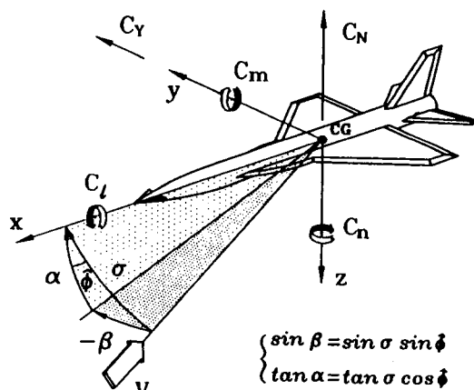
Fig. 5.1 The body axes reference system
