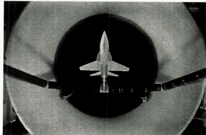
Fig 2.23 WG16A model on PQR rig
