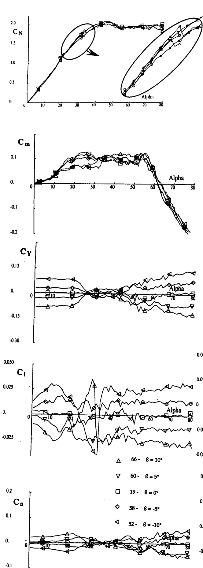
Fig. 5.42 Slow Alpha-sweeps - BWLHVST Configuration - Sideslip effect.
