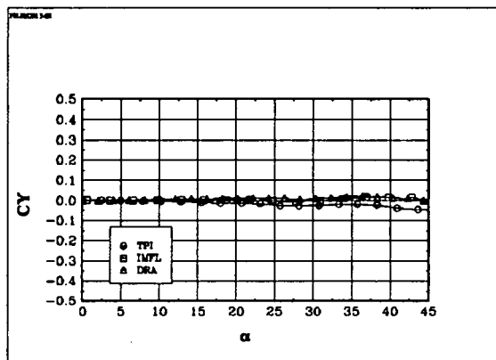
Fig 6.14 The coefficient C_Y : BWLVHST, \beta = 0^\circ
