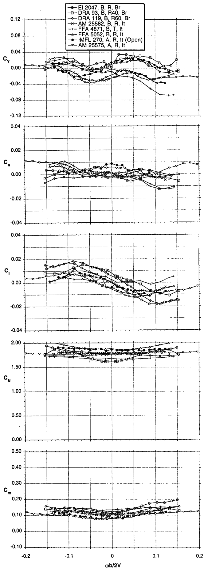
Figure 4.8 - Rotary-balance tests, BWLVHST, 40° AOA
