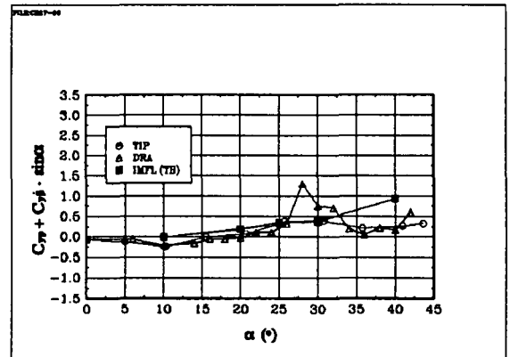
Fig 6.54 The derivative Cy\beta^* : BWLVHST, \beta = 0^\circ
