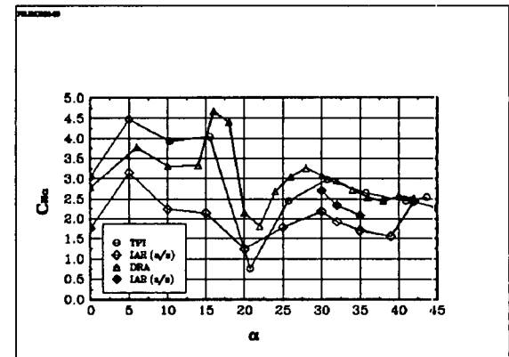
Fig 6.22 The derivative C_{n\alpha} : BWLVHST, \beta = 0^\circ
