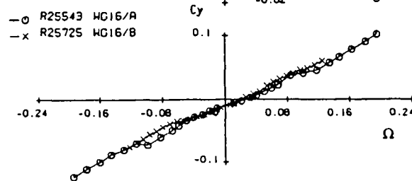
Fig 3.25 - Model A vs. Model B results - BWLVHST conf. AeM tests - \alpha = 24^\circ
