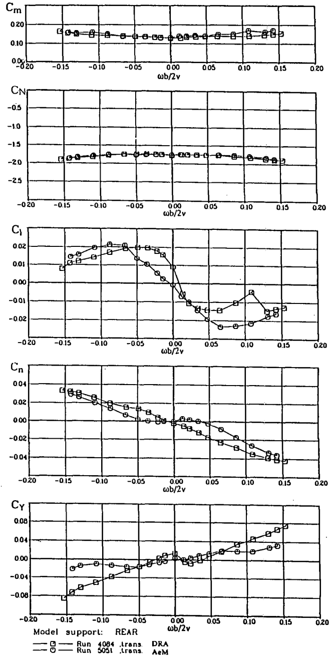
Fig 3.8 - BWLHVST Configuration Effect of transition fixing type at \alpha = 32^\circ , V = 60 m/s
