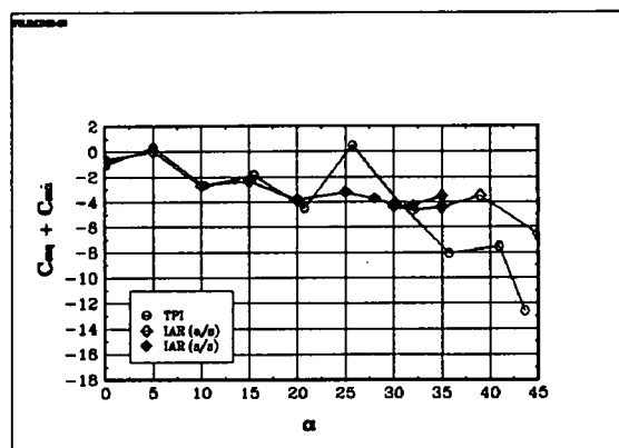
Fig 6.44 The derivative C_{mq} : BWVH, \beta = 0^\circ
