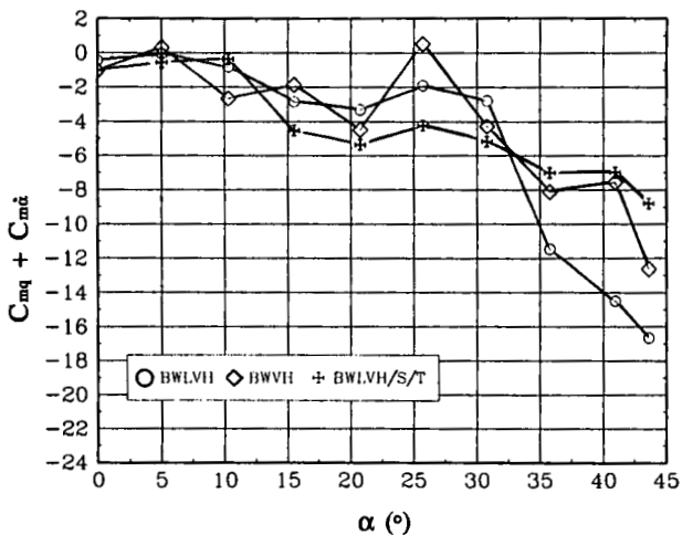
Fig. 5.11 The effect of configuration on C_{mq} + C_{m\dot{\alpha}} ( V=30 m/s, \beta=0^\circ , k=0.083 , \theta=\pm 1^\circ ).
