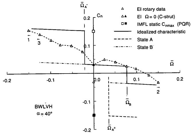
Fig A4.4.13 Interpretation of water tunnel rotary data at \alpha = 40^\circ
