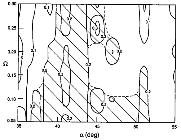
Fig A4.2.24 Incremental effect of support on vortex breakdown on coning cone-cylinder
