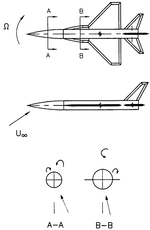
Fig A4.3.12 Forebody-LEX vortex interaction at \Omega > 0
