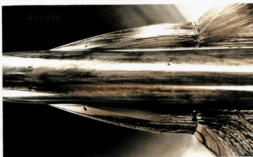
Fig A4.2.8 Forebody/LEX flow pattern at \alpha = 49^\circ , \phi_m = 180^\circ
