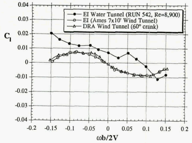
Figure 4.19 - Water/wind tunnel test comparisons, BWLVHS (strakes on), 50° AOA
