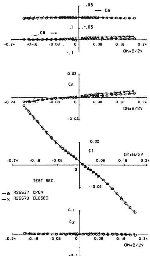
Fig 3.57 - Open versus closed test section walls BWLHVT Configuration - AeM tests - \alpha = 0^\circ
