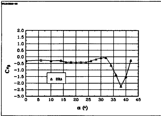
Fig 6.57 The derivative CY_{\beta} : BWLVH, \beta = 0^{\circ}
