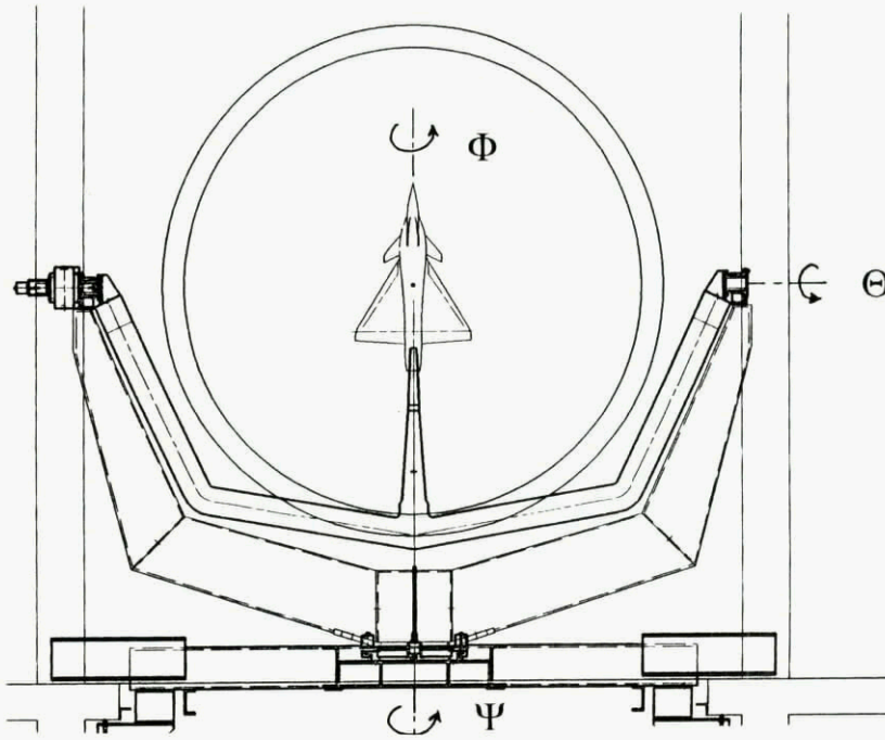
Fig 2.22 ONERA-IMFL 'PQR' rig in open-section wind tunnel
