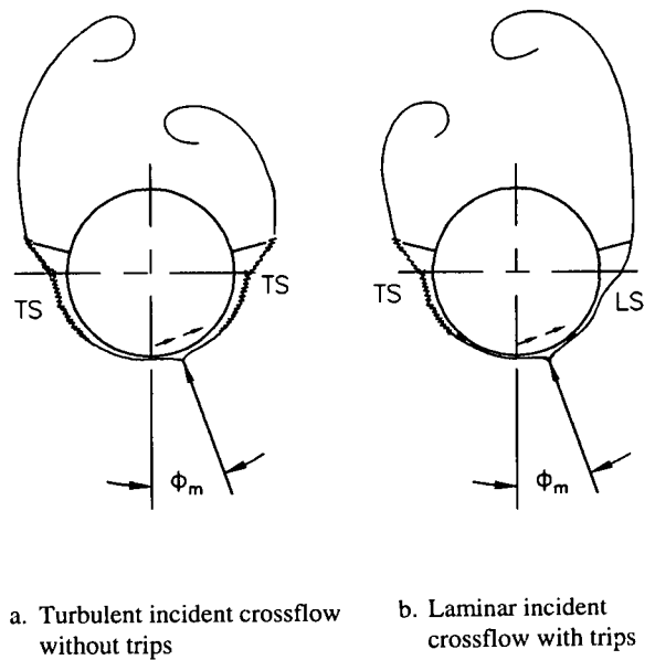
Fig A4.3.13 Crossflow characteristics of translating circular cross-section with strakes
