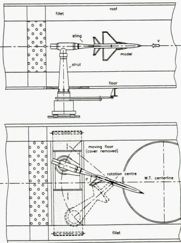
Fig 2.19 IAR asymmetric support system for oscillatory tests
