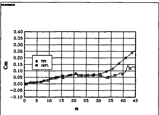
Fig 6.7 The coefficient Cm: BWLVH, \beta = -10^\circ
