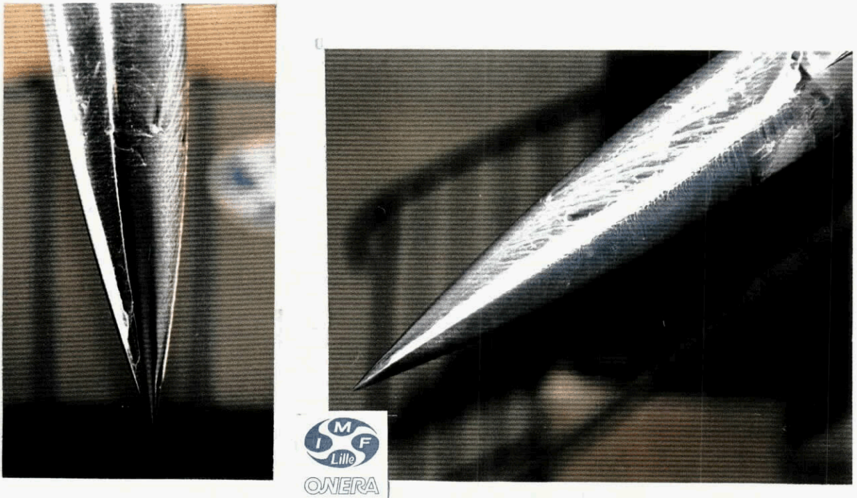
Fig A4.2.10 Oil flow visualization on BWLVH at \alpha = 53^\circ
