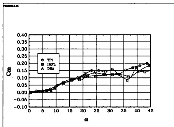
Fig 6.10 The coefficient C_m : BWLVH, \beta = 5^\circ
