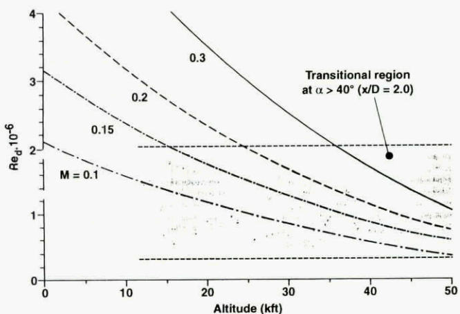
Fig A4.5.11 Typical forebody crossflow Reynolds number in full-scale flight
