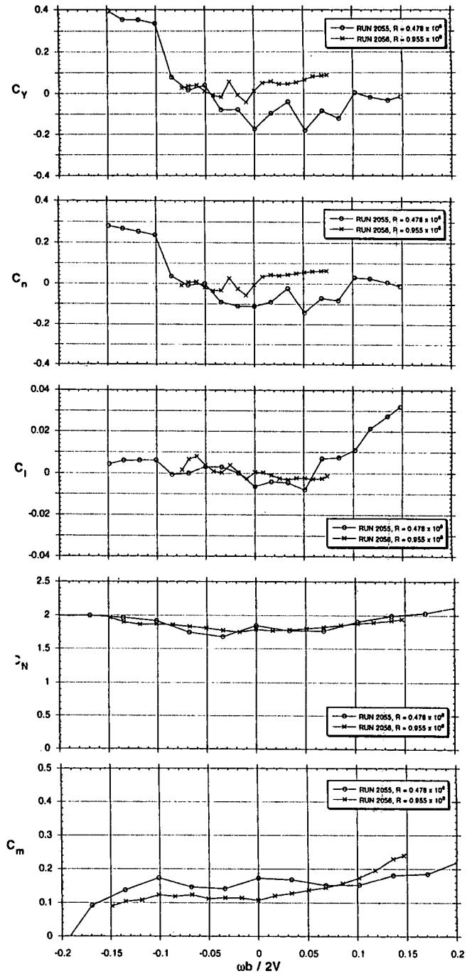
Fig 3.20 - Effects of Reynolds No. body-wing-LEX-tails (BWL VHT), \alpha = 51^\circ (R=0.478, 0.955 x 10 6 for V=100, 200 ft/s)
