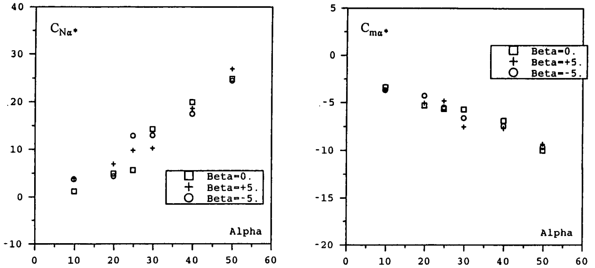
Fig 8.3 Small amplitude oscillatory derivatives
