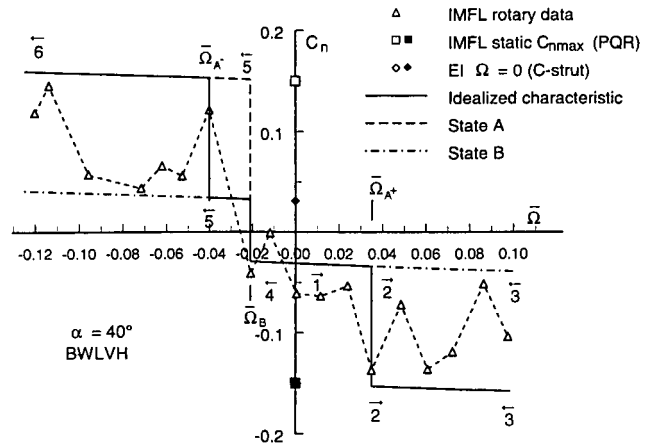
Fig A4.4.12 Interpretation of rotary characteristics of baseline configuration
