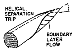
Fig A4.3.4 Crossflow characteristics of translating circular cross-section for laminar flow conditions
