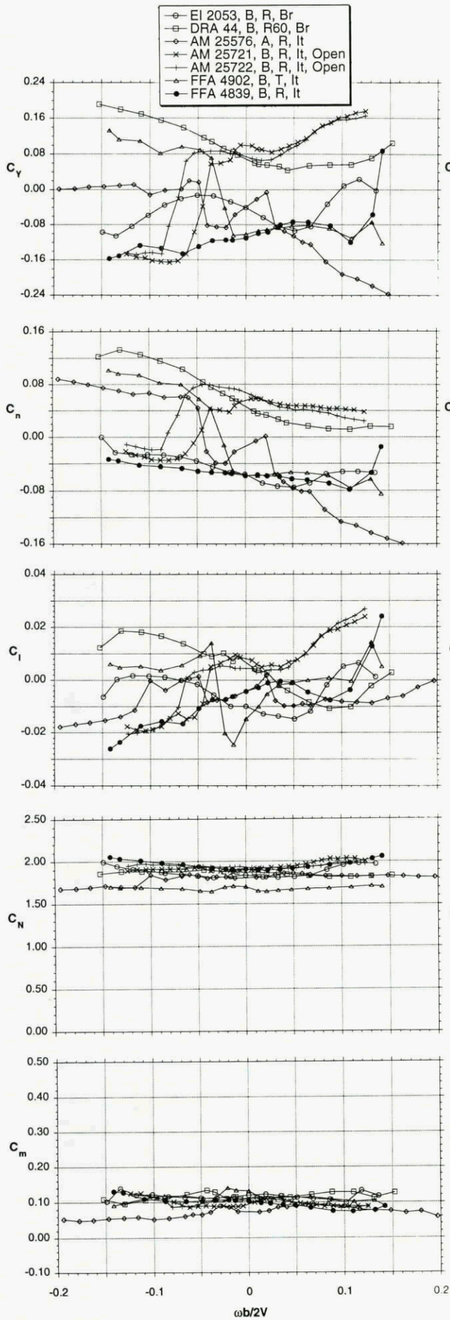
Figure 4.12 - Rotary-balance tests, BWLVHT, 40° AOA
