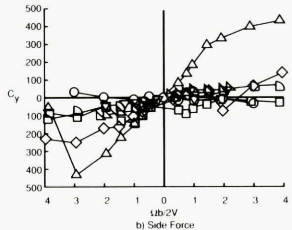
Figure 7.7. Effect of rotation rate and Reynolds number on aerodynamic characteristics for the rectangular ogive at 90° angle of attack.
