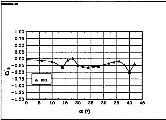
Fig 6.59 The derivative Cj_{\beta} : BWLVH, \beta = 0^{\circ}
