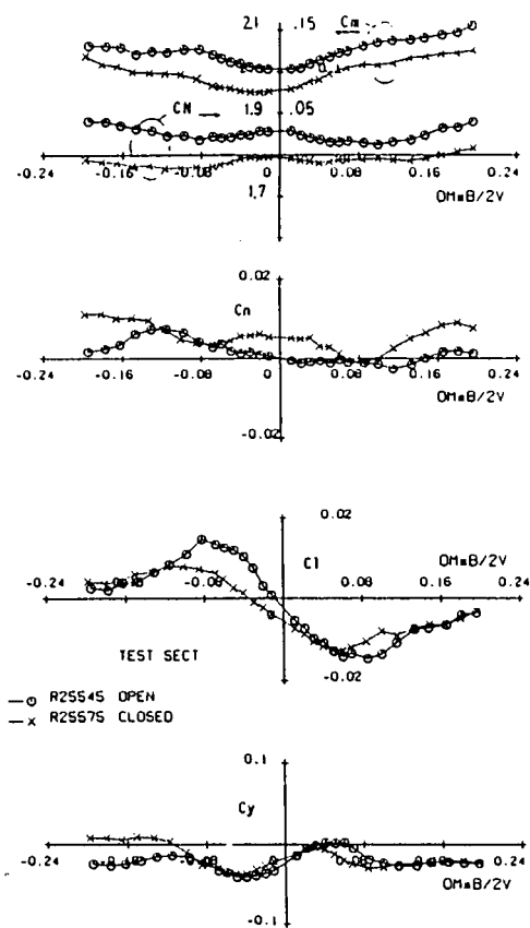
Fig 3.55 - Open versus closed test section walls BWLHVST Configuration - AeM tests - \alpha = 40^\circ
