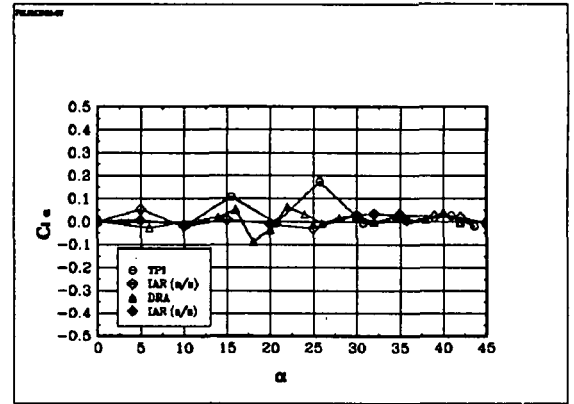
Fig 6.34 The derivative Cl_\alpha : BWLVHST, \beta = 0^\circ
