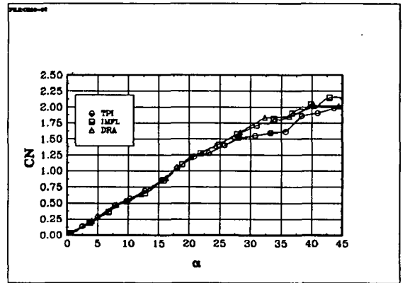
Fig 6.4 The coefficient CN: BWLVH, \beta = -5^\circ
