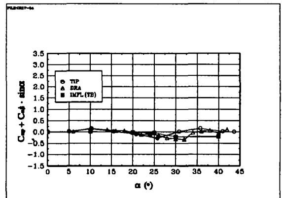
Fig 6.56 The derivative Cnp\beta^* : BWLVHST, \beta = 0^\circ
