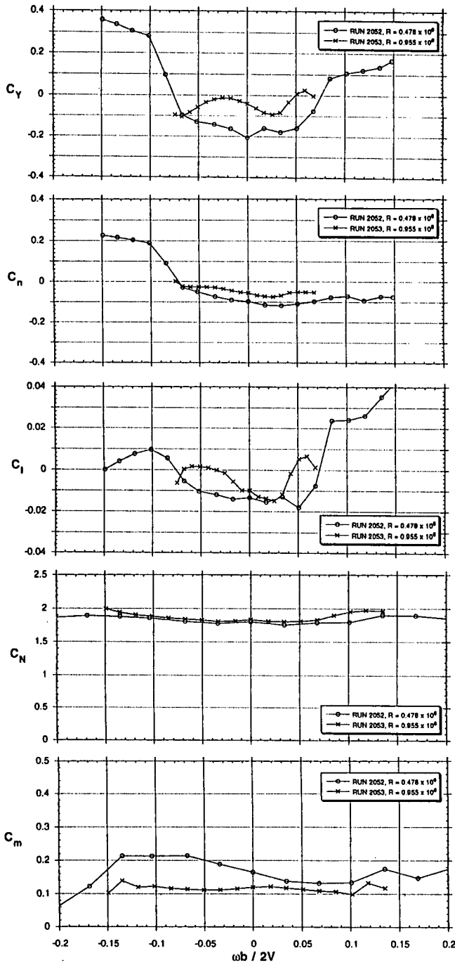
Fig 3.19 - Effects of Reynolds No. body-wing-LEX-tails (BWL VHT), \alpha = 39^\circ (R=0.478, 0.955 x 10 6 for V=100, 200 ft/s)
