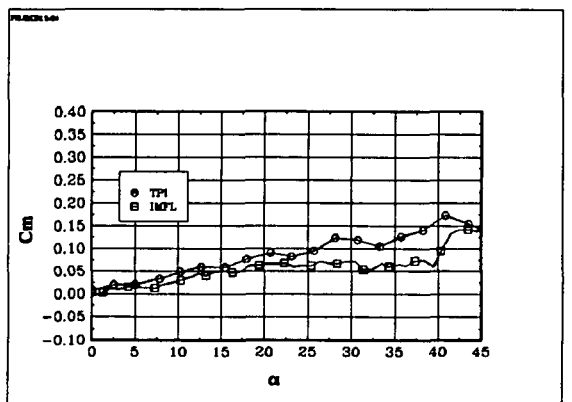
Fig 6.8 The coefficient Cm: BWLVH, \beta = 10^\circ
