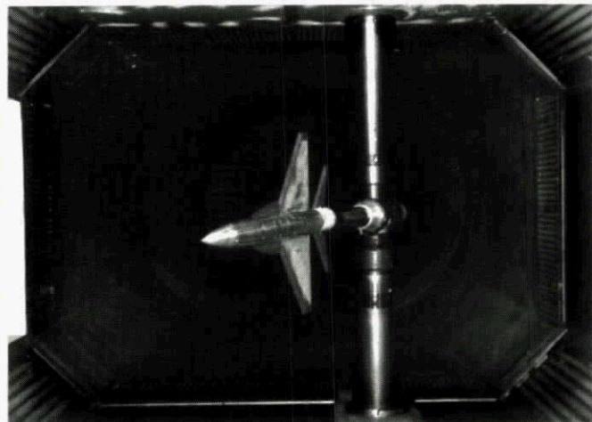
Fig 2.20 IAR oscillatory rig with image strut fitted in wind tunnel
