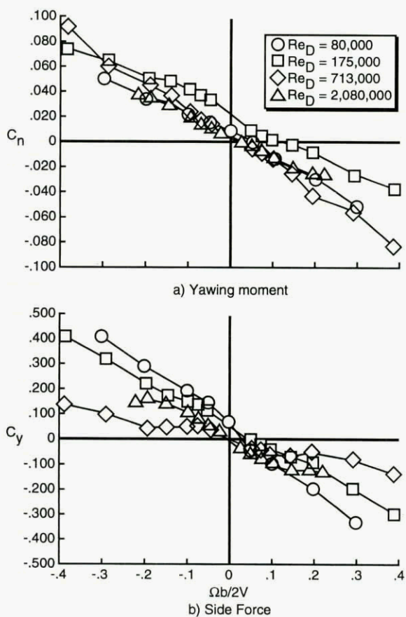
Figure 7.2. Effect of rotation rate and Reynolds number on aerodynamic characteristics for the rectangular ogive at 60° angle of attack.
