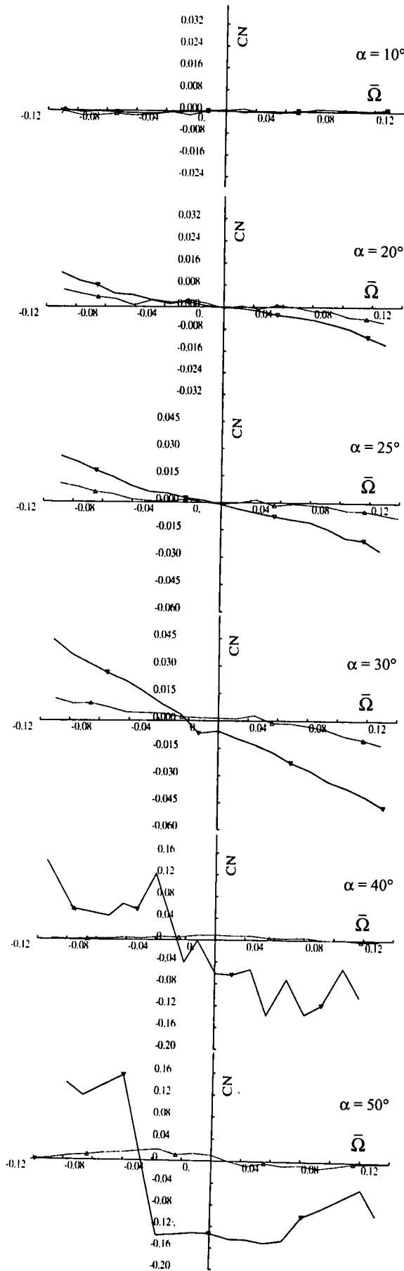
Fig A4.3.7 Effect of strakes and trips on C_n(\Omega) characteristics for the AGARD WG16 model 40
