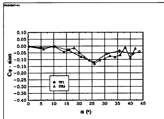
Fig 6.48 The derivative C_{l\beta \sin \alpha} : BWLVHST, \beta = 0^\circ
