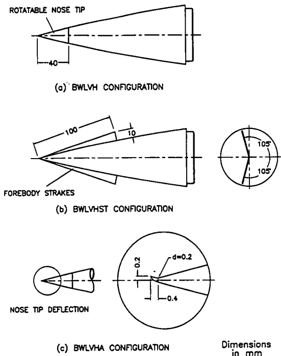
Fig. 5.24 WG16CA forebody configurations.
