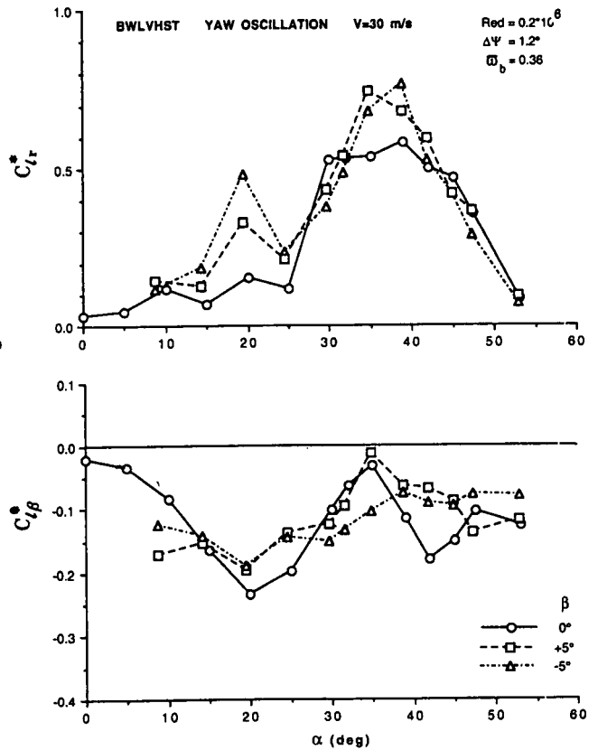
Fig 5.39 The effect of sideslip on derivatives C_{tr}^* and C_{tp}^* for BWLVHST configuration in yaw oscillation.
