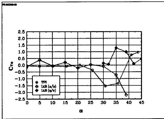
Fig 6.29 The derivative C_{Y\alpha} : BWLVH, \beta = 0^\circ
