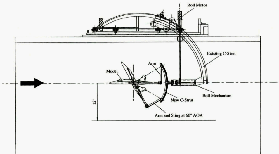
Fig 2.18 Eidetics rotary rig in EI2436 water tunnel
