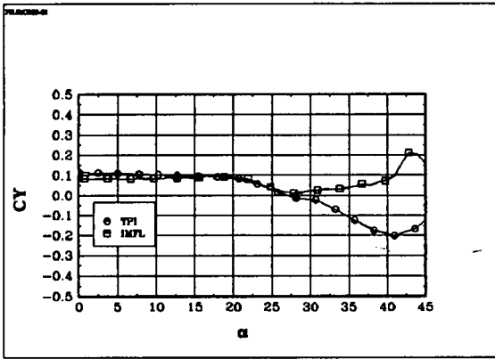
Fig 6.17 The coefficient C_Y : BWLVH, \beta = -10^\circ
