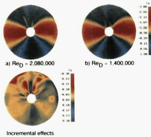
Figure 7.16. Comparison of the pressure distribution at \Omega d/2V = -0.2 for the circular ogive at 60^\circ angle of attack for two Reynolds numbers.
