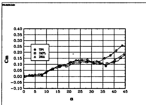
Fig 6.9 The coefficient C_m : BWLVH, \beta = -5^\circ
