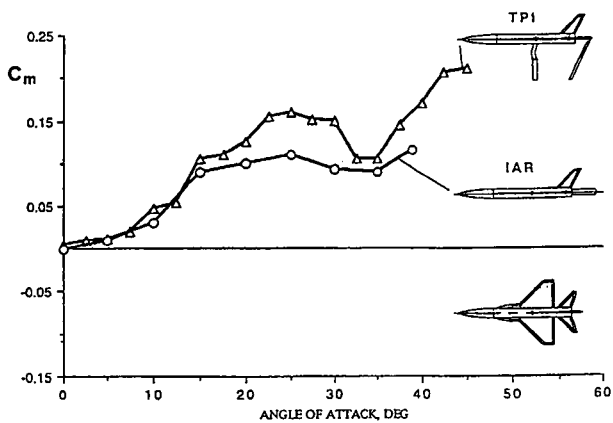
Fig A4.2.19 Strut-induced support interference
