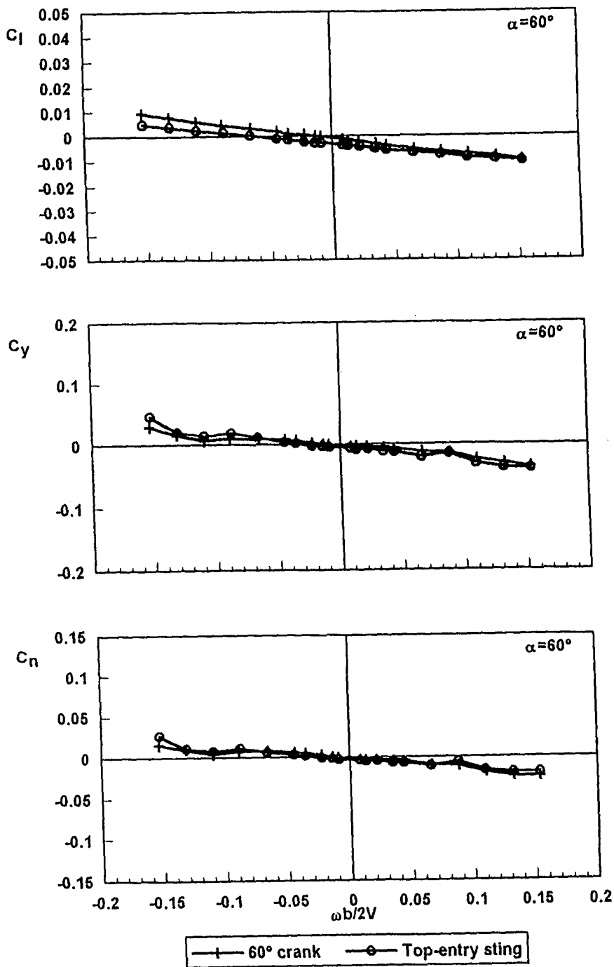
Fig 3.52 - BWLHVST Configuration. Effect of top-entry sting - \alpha = 60^\circ
