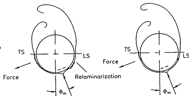
a. Trips at \phi_t = \pm 40^\circ b. Trips at \phi_t = \pm 70^\circ
