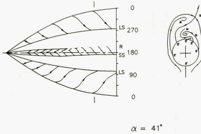
Fig A4.2.4 Asymmetric vortex flow topology
