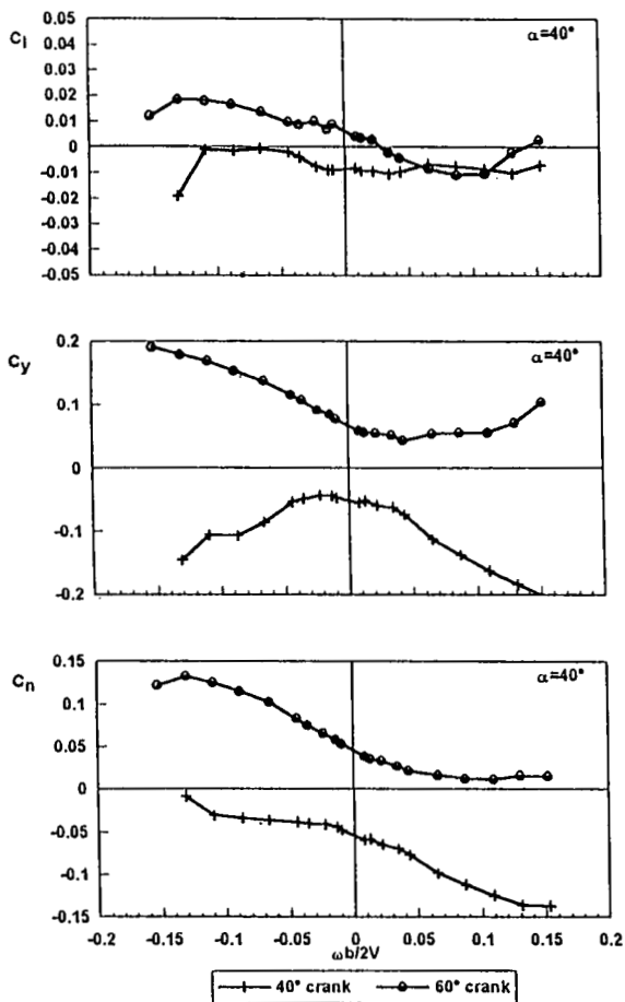
Fig 3.50.a - BWLHVT Configuration
