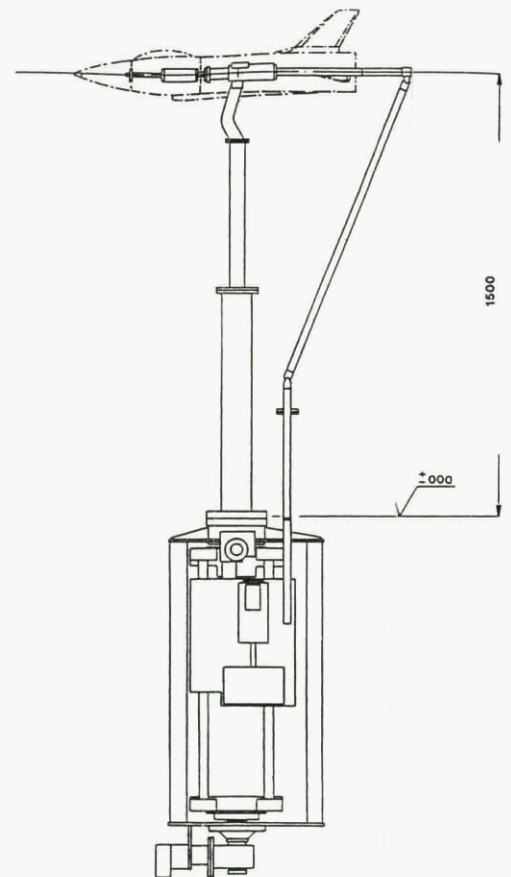
Fig 2.28 The TPI oscillatory balance
