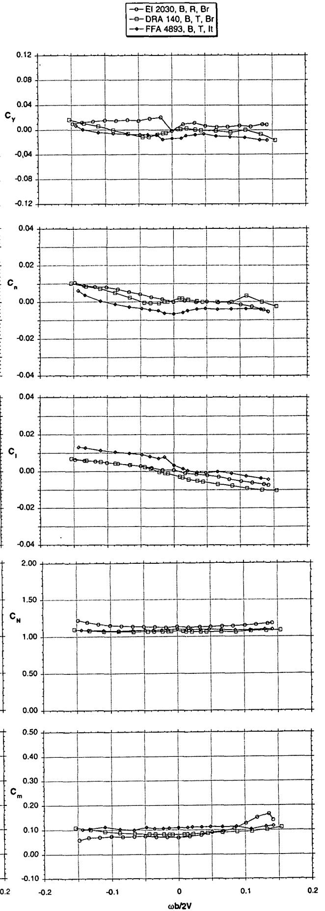
Figure 4.5 - Rotary-balance tests, BWST, 50° AOA
