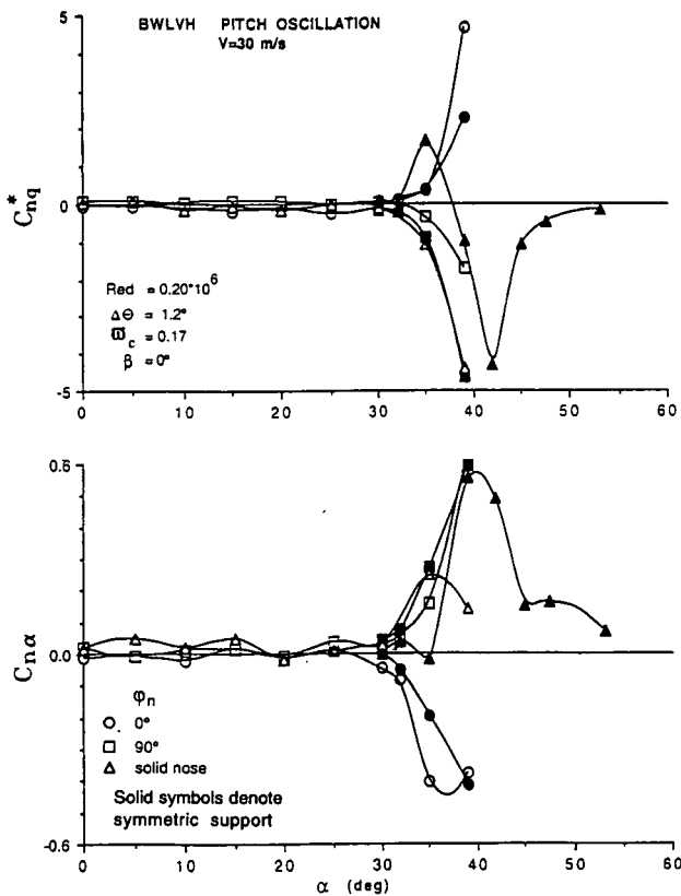
Fig. 5.25 Effect of rotating nose tip on the derivatives C_{nq}^* and C_{na}
