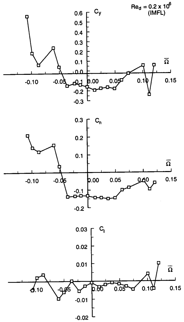
Fig A4.4.7 Rotary data on BWLVH at \alpha = 50^\circ and subcritical conditions
