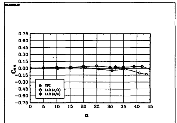
Fig 6.38 The derivative Cn_\alpha : BWLVHST, \beta = 0^\circ
