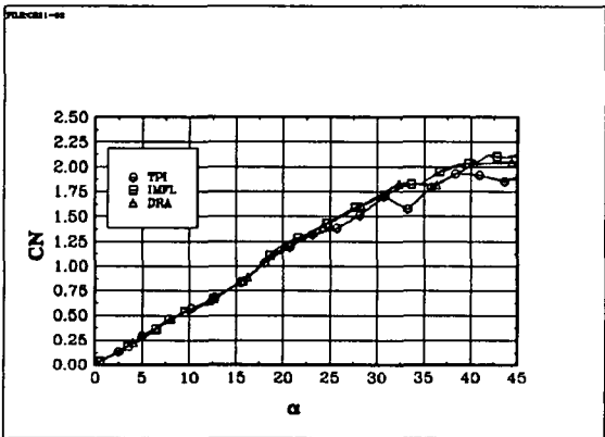
Fig 6.5 The coefficient CN: BWLVH, \beta = 5^\circ
