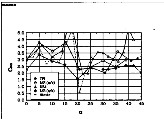
Fig 6.21 The derivative C_{n\alpha} : BWLVH, \beta = 0^\circ
