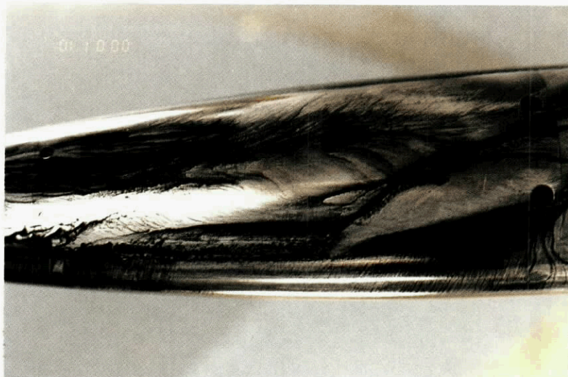
Fig A4.2.6 Forebody flow pattern at \alpha = 47^\circ , \phi_m = 135^\circ
