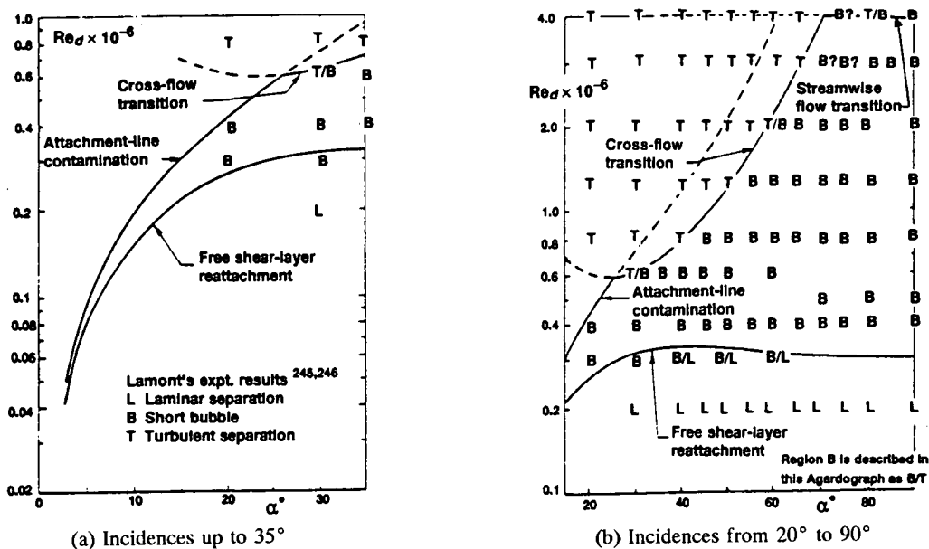
Fig A3.1 - Illustration of the types of transition on cylindrical bodies and a comparison of predicted and measured results (from Ref 10).
