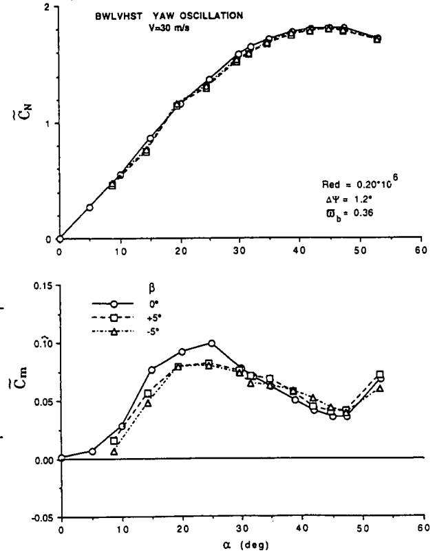
Fig 5.35 The effect of sideslip on the longitudinal aerodynamic coefficients for BWLVHST configuration in yaw oscillation.
