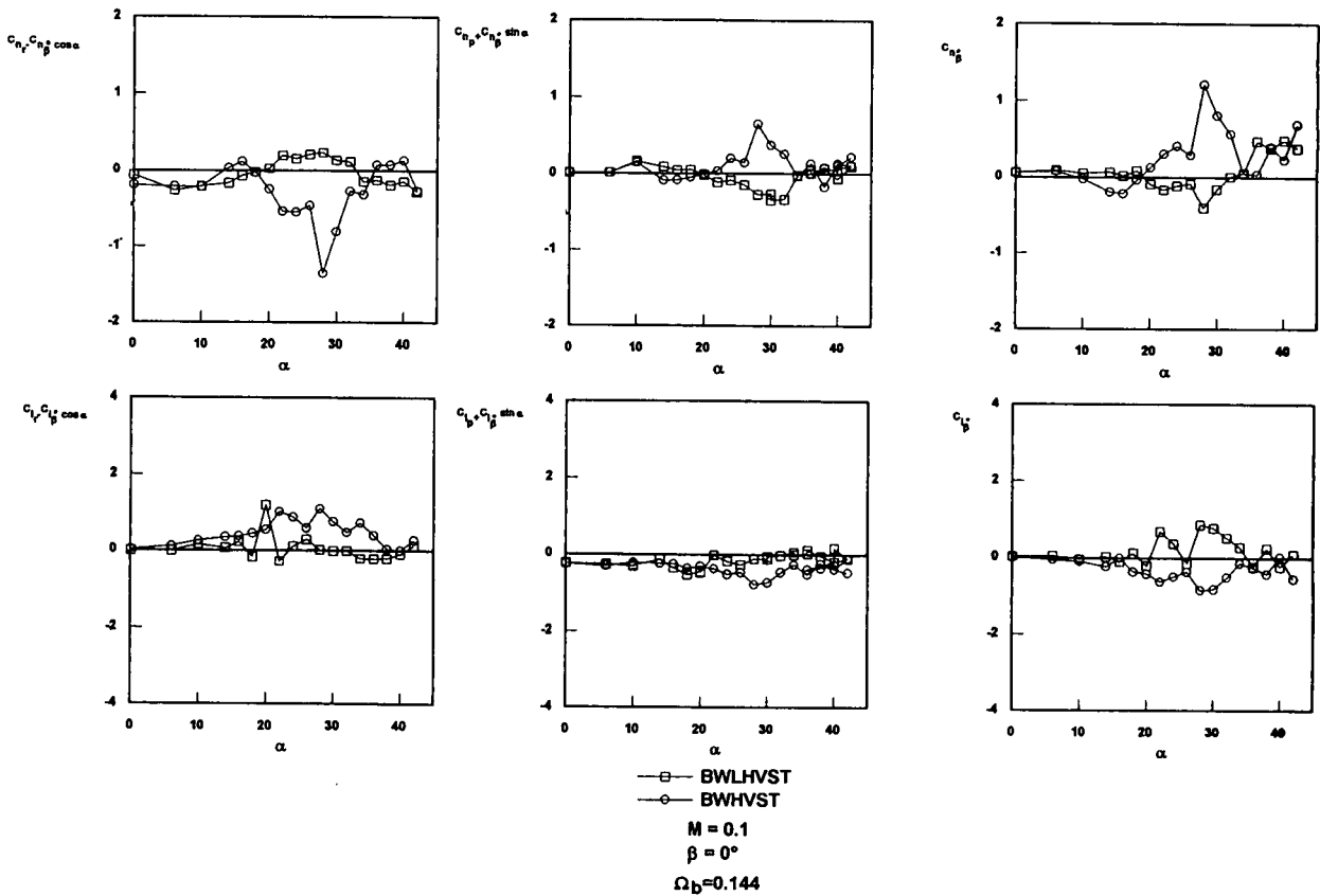
Fig. 5.7 Effect of LEX on derivatives from yawing, swaying and rolling modes.
