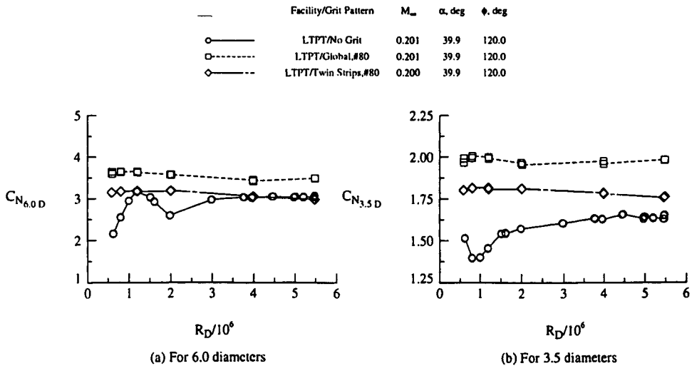
Fig A3.5 - NASA Langley experiment - Effect of transition tripping pattern on variation of total integrated normal force with Reynolds number for ogive/cylinder model and two model lengths.
