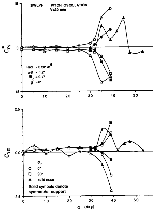
Fig. 5.27 Effect of rotating nose tip on derivatives C_{yq}^* and C_{ya} .
