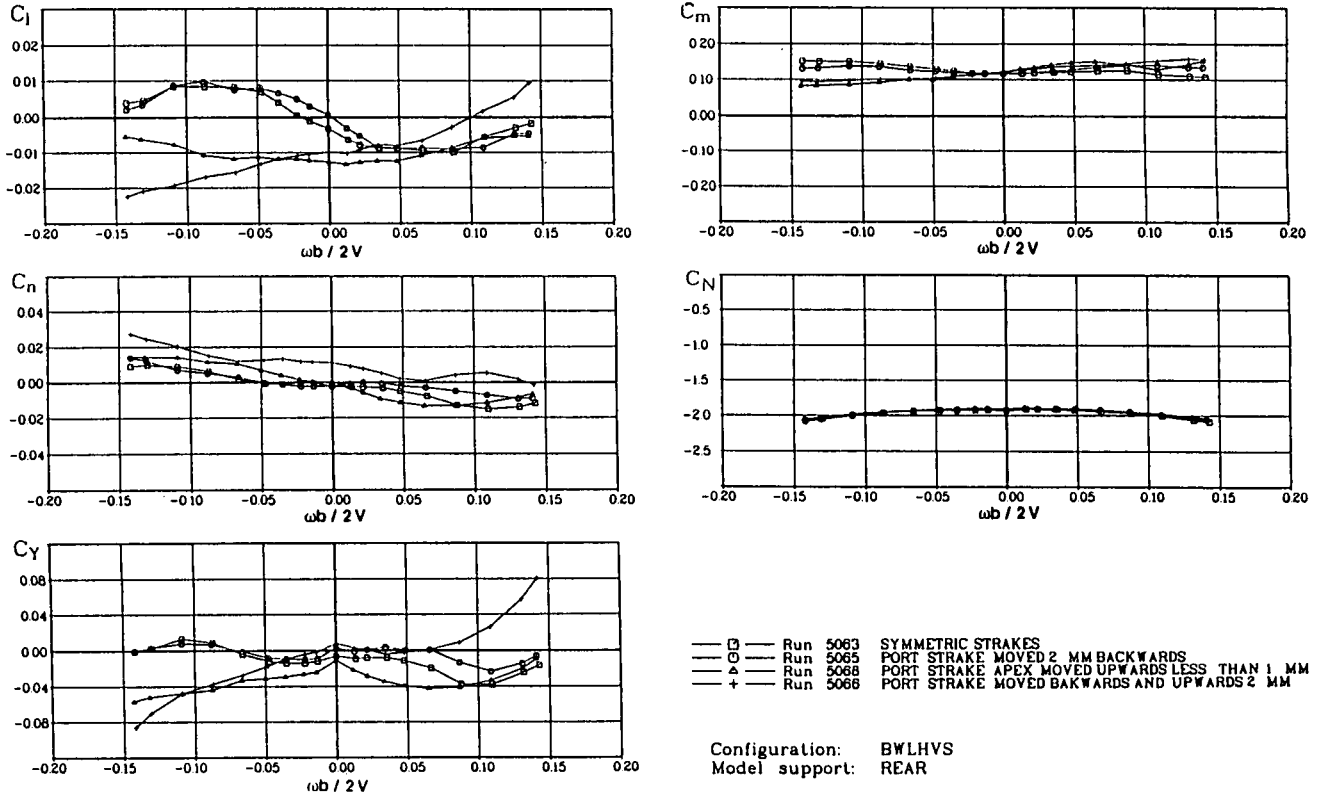
Fig 3.34 - Sensitivity to the nose strake position
