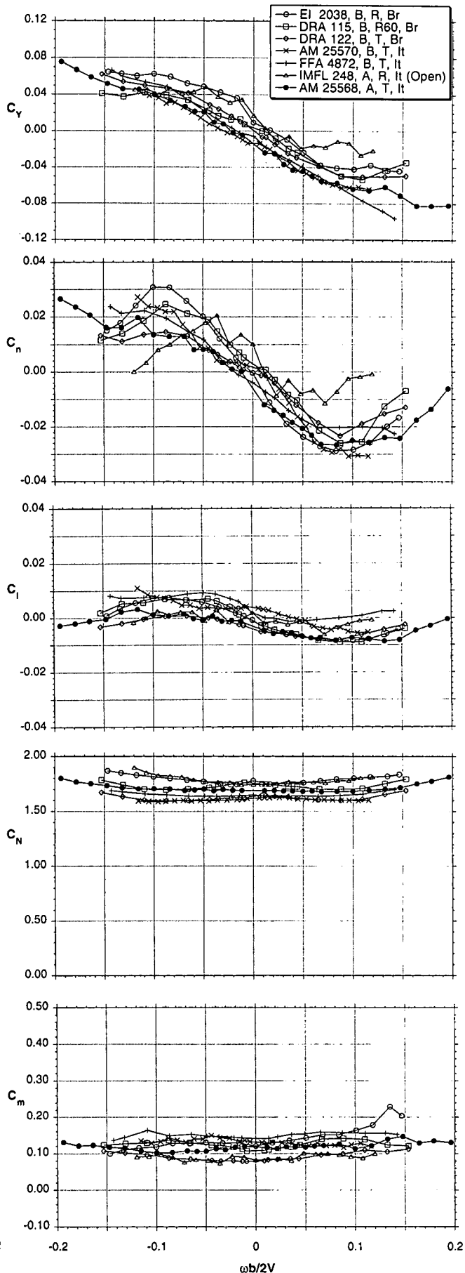
Figure 4.9 - Rotary-balance tests, BWLVHST, 50° AOA
