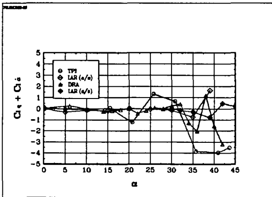
Fig 6.35 The derivative Cl_\alpha^* : BWLVH, \beta = 0^\circ
