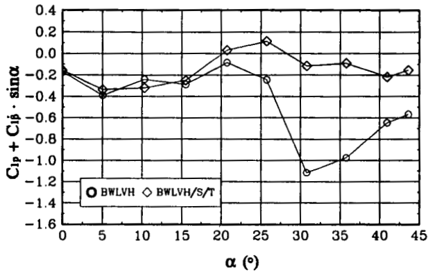
Fig. 5.13 The effect of configuration on C_{lP} + C_{l\beta} \sin\alpha ( V=30 m/s, \beta=0^\circ , k=0.180 , \varphi=\pm 1^\circ ).
