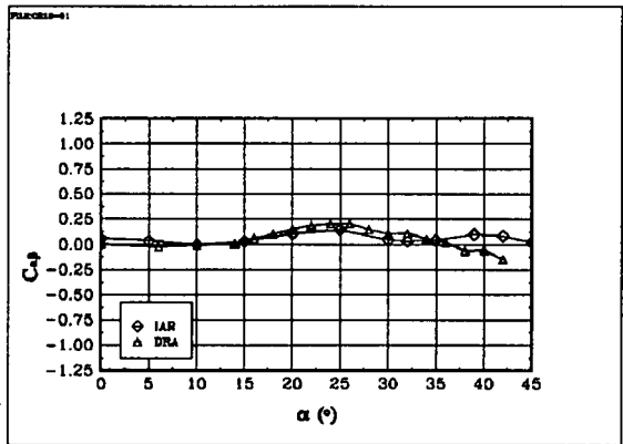
Fig 6.62 The derivative Cn_{\beta} : BWLVHST, \beta = 0^{\circ}
