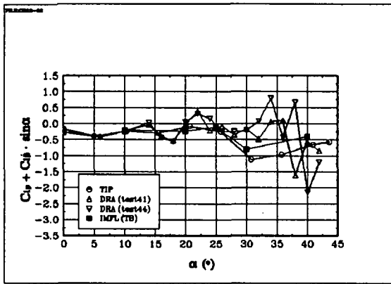
Fig 6.51 The derivative Cp\beta^* : BWLVH, \beta = 0^\circ
