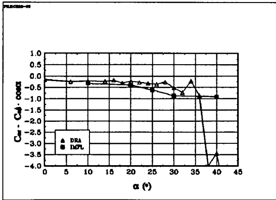
Fig 6.65 The derivative C_{nr} : BWLVH, \beta = 0^\circ
