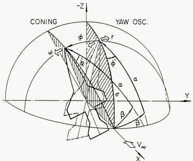
Fig A4.5.3 Relationships between characteristic motions
