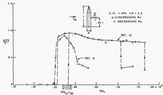
Fig A4.5.8 Flat spin characteristics of cone-cylinder 78
