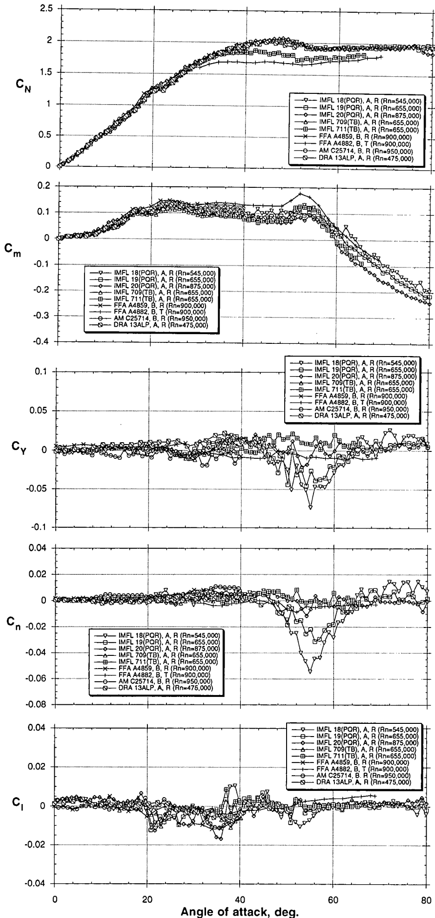
Figure 4.1 - Static data for complete configuration, BWLVHST
