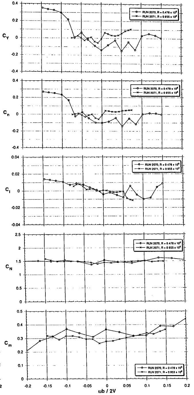
Fig 3.18 - Effects of Reynolds No. body-wing-LEX (BWL), \alpha = 51^\circ ( R=0.478, 0.955 \times 10^6 for V=100, 200\text{ft/s} )
