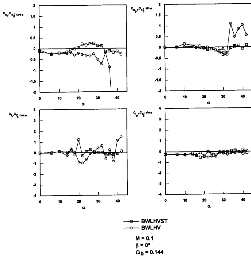
Fig. 5.5 Effect of forebody strakes and grit strips on derivatives from yawing and rolling modes.
