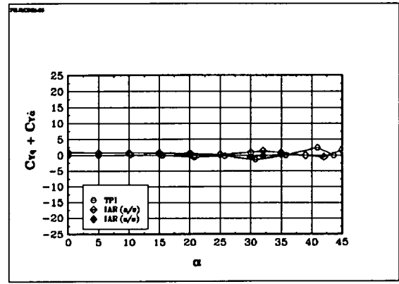
Fig 6.32 The derivative C_{Yq^*} : BWLVHST, \beta = 0^\circ
