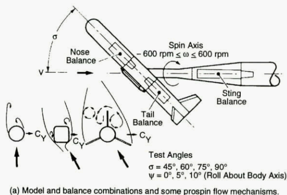
(a) Model and balance combinations and some prospin flow mechanisms.
