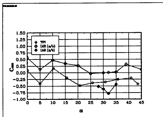
Fig 6.42 The derivative C_{m\alpha} : BWVH, \beta = 0^\circ
