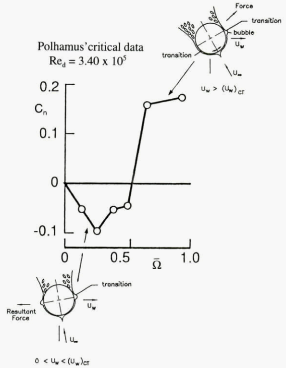
Fig A4.5.7 Flat-spin yawing moment at critical flow conditions 46
