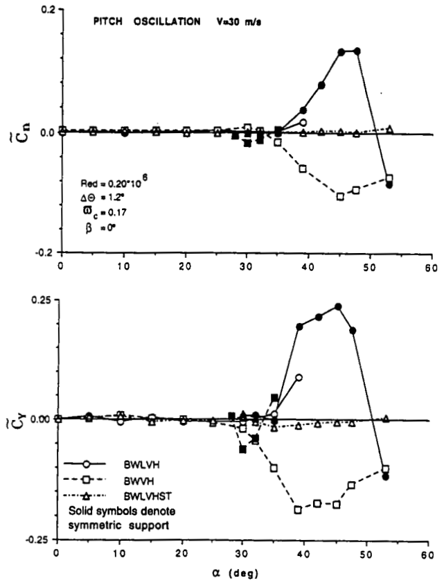
Fig. 5.29 Configurational effects on the lateral-directional aerodynamic coefficients.
