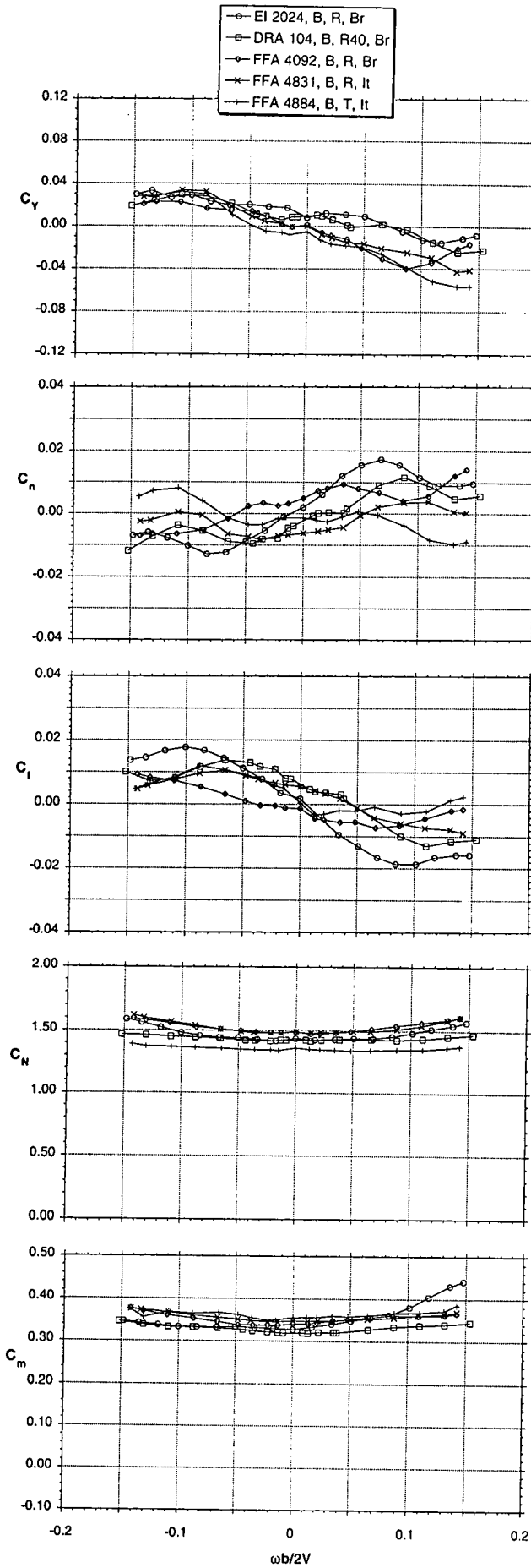
Figure 4.6 - Rotary-balance tests, BWLST, 40^\circ AOA
