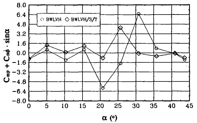
Fig. 5.17 The effect of configuration on C_{mp} + C_{mp} \sin \alpha ( V=30 m/s, \beta = 0^\circ , k = 0.180 , \varphi = \pm 1^\circ ).
