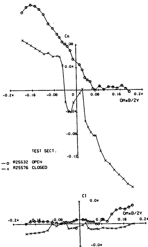
Fig 3.59 - Open versus closed test section walls, BWLHVT Config. - AeM tests - \alpha = 40^\circ
