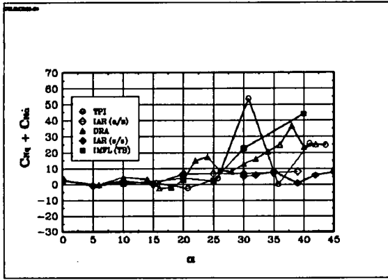
Fig 6.25 The derivative CNq^* : BWLVH, \beta = 0^\circ
