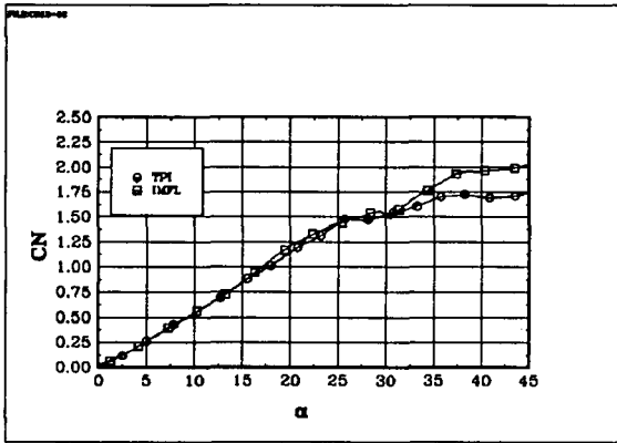
Fig 6.3 The coefficient CN: BWLVH, \beta = 10^\circ
