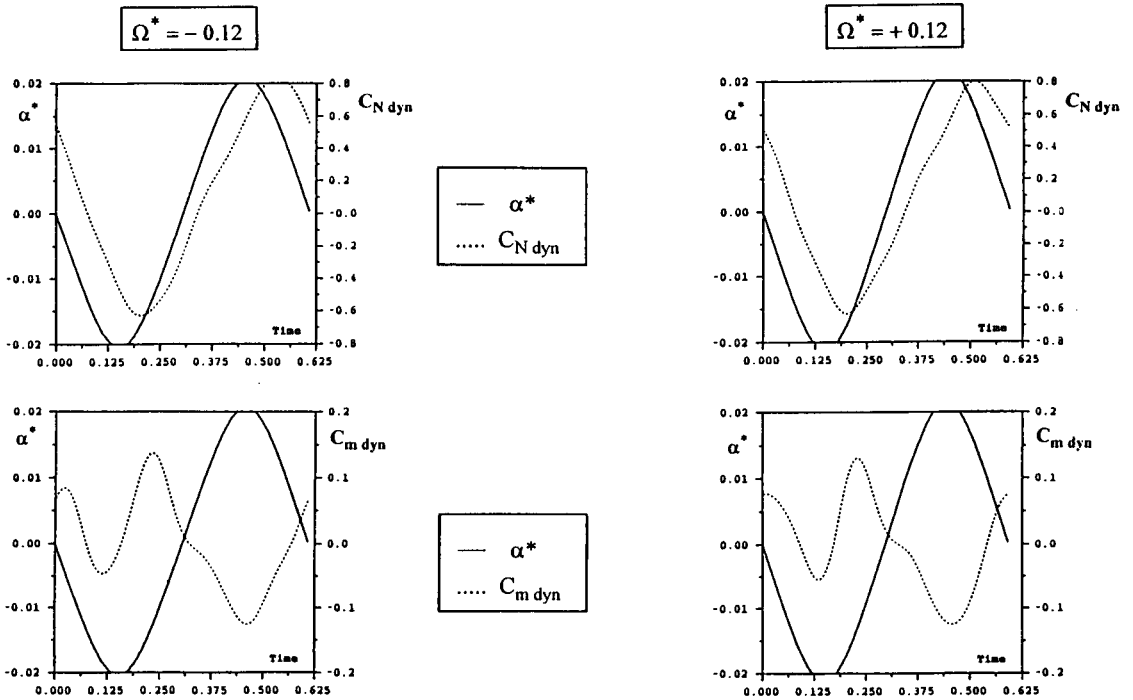
Fig 8.22 Time histories of dynamic contributions in Normal force and pitching moment for large amplitude oscillatory coning tests ( \lambda = 20^\circ , mean \alpha = 50^\circ ).
