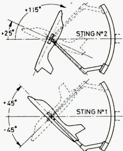
Fig 2.6 AEM rotary balance stings
