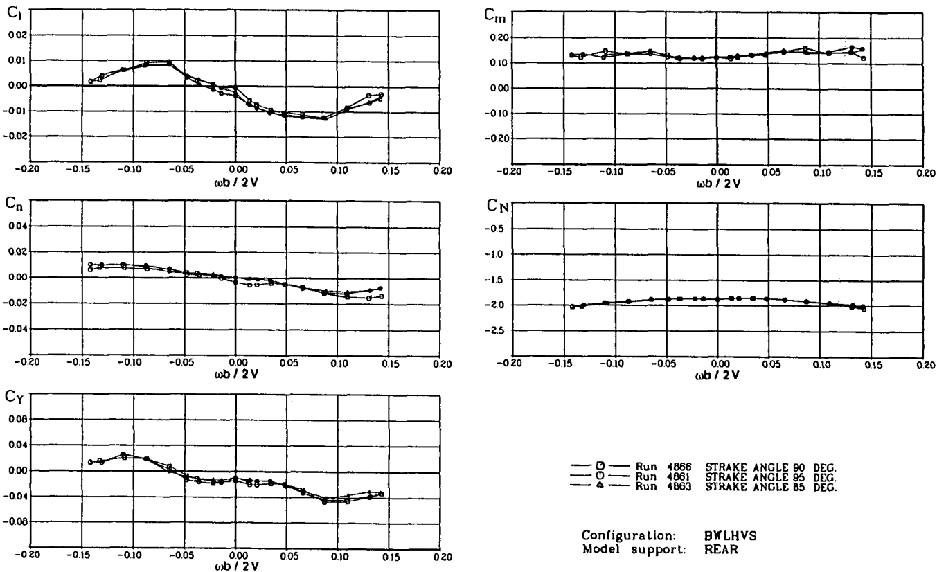
Fig 3.33 - Sensitivity to the nose strake position
