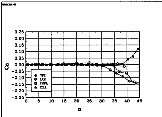
Fig 6.19 The coefficient C_n : BWLVH, \beta = 0^\circ
