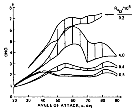
Fig 3.12 - Reynolds Number effect on an ogive cylinder (Ref 3.3)
