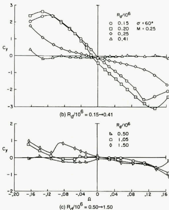
Figure 7.3. Side-force coefficient on the nose section; effect of Reynolds number at \sigma = 60 deg, M = 0.25 .
