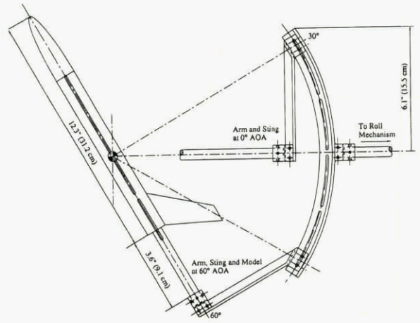
Figure 4.15 - Eidetics Water Tunnel Rotary-Balance Rig
