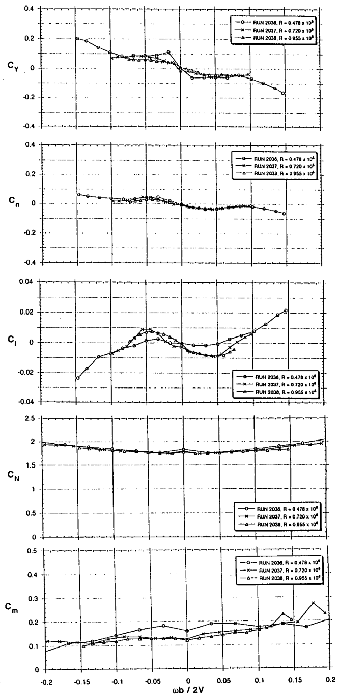
Fig 3.22 - Effects of Reynolds No. body-wing-LEX-tails-strakes (BWL VHST) \alpha = 51^\circ ( R=0.478, 0.955 \times 10^6 for V=100, 200 ft/s)
