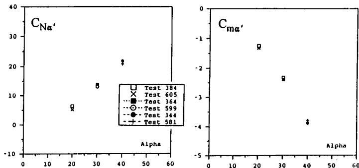
Fig 8.7 Repeatability of mean oscillatory coning derivatives. Amplitude = 20°.
