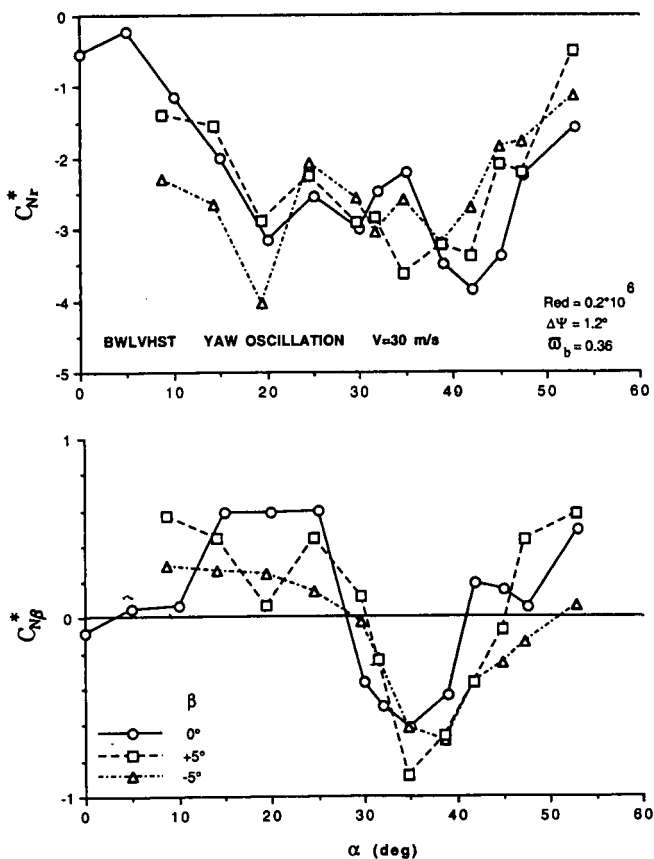
Fig 5.41 The effect of sideslip on derivatives C_{Nr}^* and C_{N\beta}^* for BWLVHST configuration in yaw oscillation.
