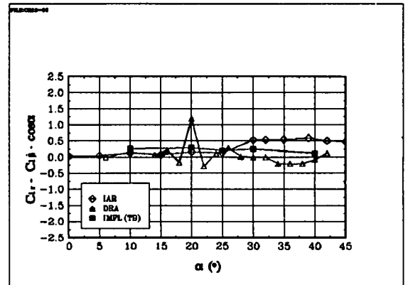
Fig 6.68 The derivative Cl_r : BWLVHST, \beta = 0^\circ
