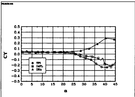
Fig 6.15 The coefficient C_Y : BWLVH, \beta = -5^\circ
