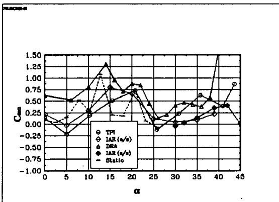
Fig 6.23 The derivative C_{m\alpha} : BWLVH, \beta = 0^\circ
