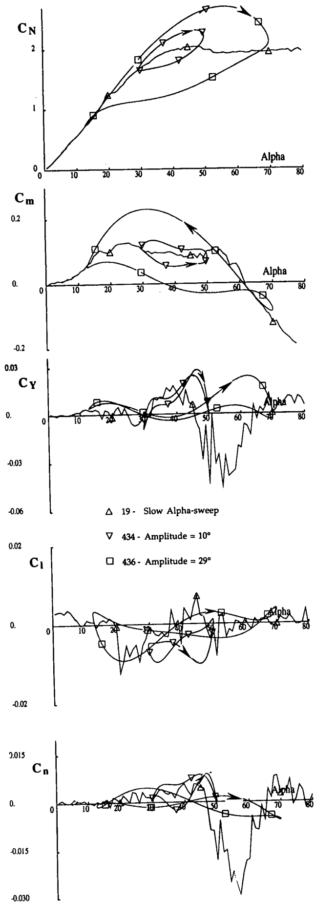
Fig. 5.49 Large amplitude pitch oscillations at \beta = 0^\circ , f = 1 Hz Amplitude effect - Mean \alpha = 40^\circ - BWLHVST Configuration
