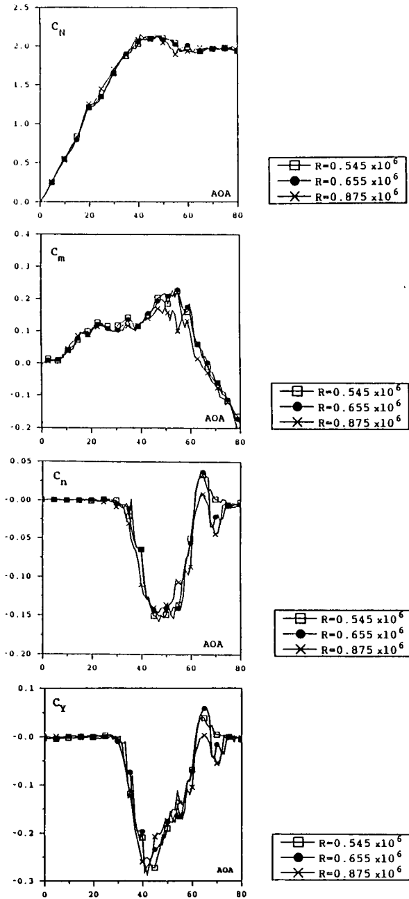
Fig 3.10 - BVLHV Configuration - Effect of Reynolds Number, Slow Sweeps in angle of attack
