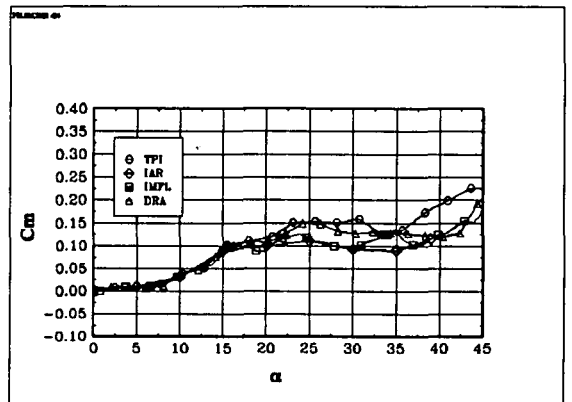
Fig 6.6 The coefficient Cm: BWLVH, \beta = 0^\circ
