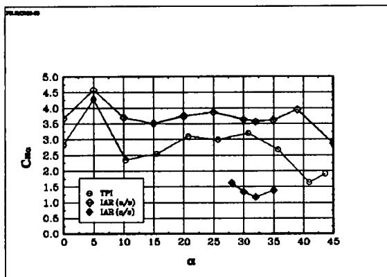
Fig 6.41 The derivative C_{N\alpha} : BWVH, \beta = 0^\circ
