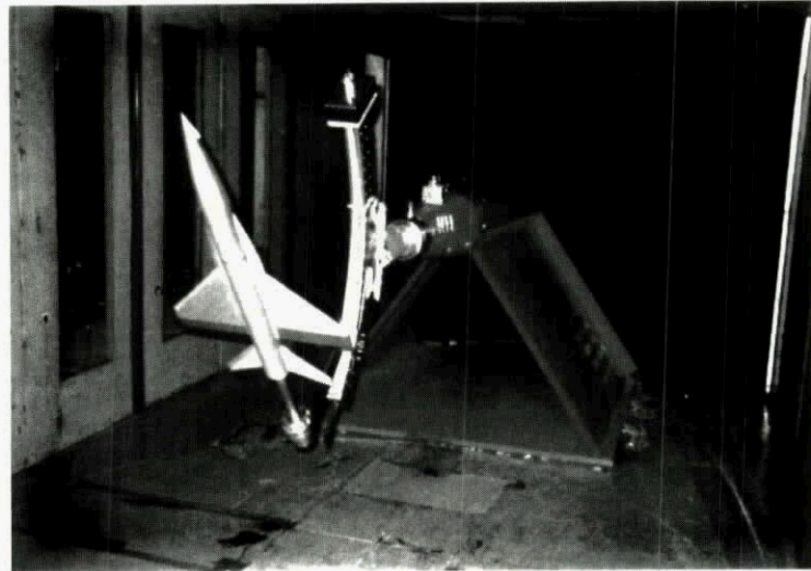
Fig 2.17 WG16B model on NASA Ames/Eidetics rotary balance
