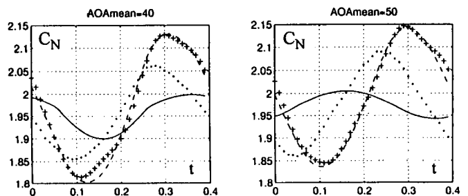
Fig 8.25 Normal force predictions as functions of time. Oscillatory tests at f = 2.5 Hz.
