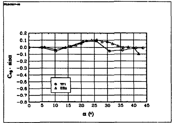
Fig 6.50 The coefficient Cn\beta \sin\alpha : BWLVHST, \beta = 0^\circ
