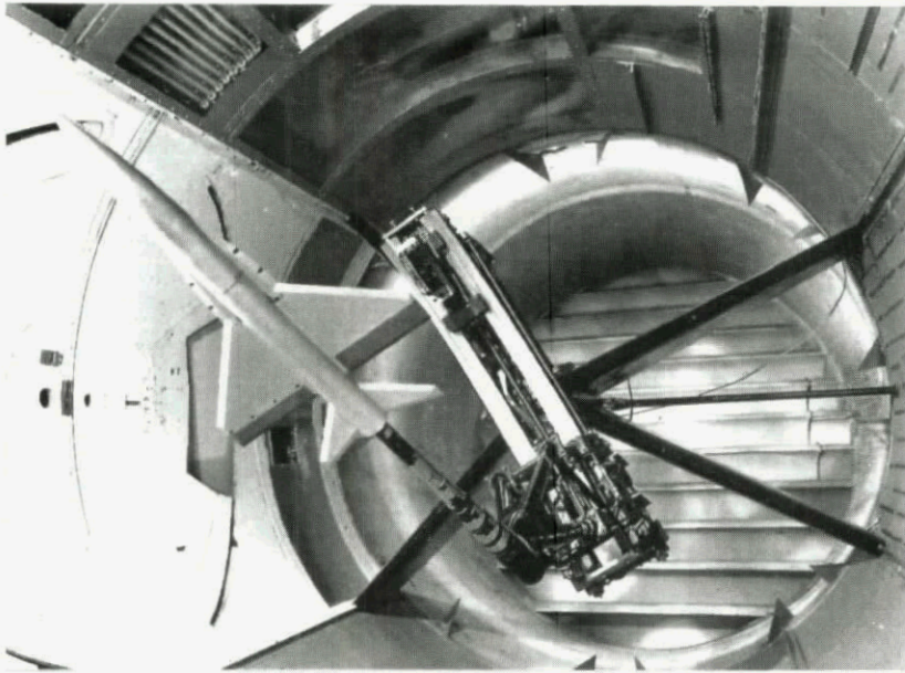
Fig 2.29 FFA rotary balance in LT1 wind tunnel
