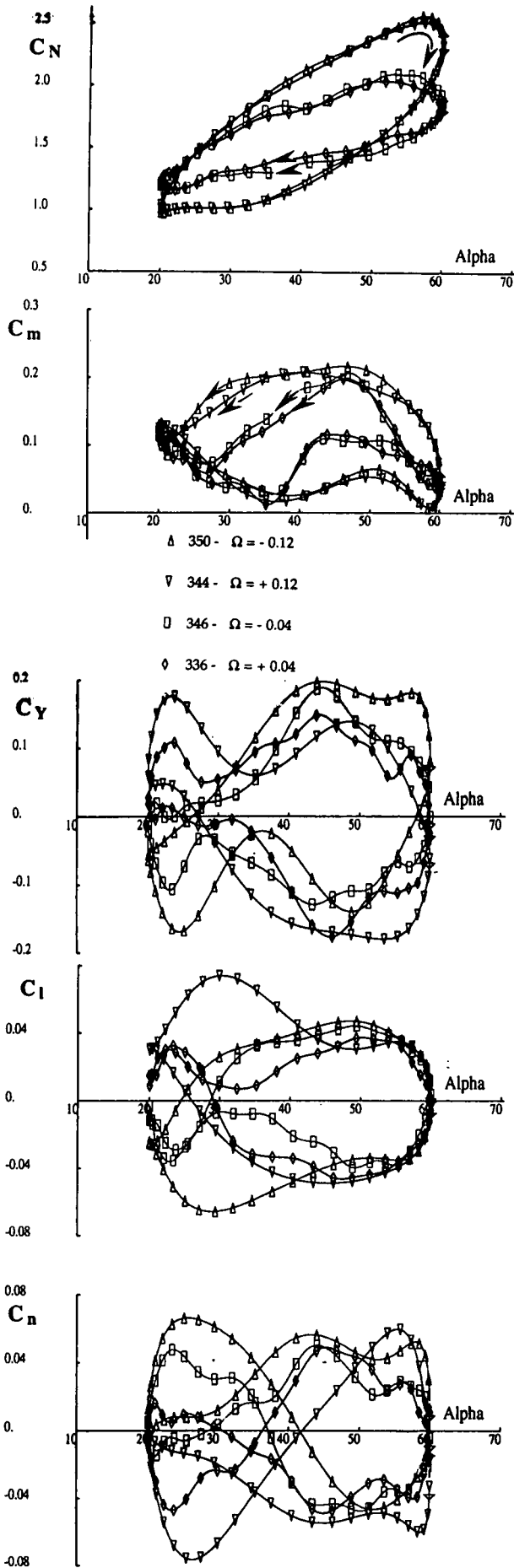
Fig 5.57 Large amplitude oscillatory coning tests - Rate effect \lambda = 20^\circ , mean \alpha = 40^\circ , mean \beta = 0^\circ BWLVHST Configuration
