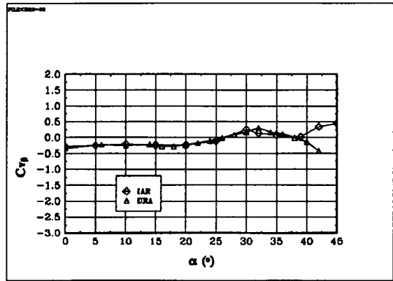
Fig 6.58 The derivative CY_{\beta} : BWLVHST, \beta = 0^{\circ}
