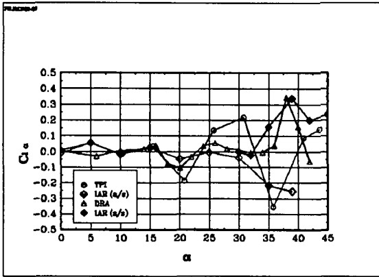
Fig 6.33 The derivative Cl_\alpha : BWLVH, \beta = 0^\circ
