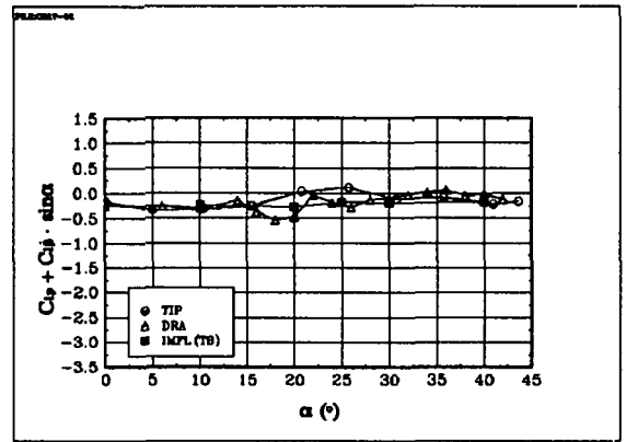
Fig 6.52 The derivative Cp\beta^* : BWLVHST, \beta = 0^\circ
