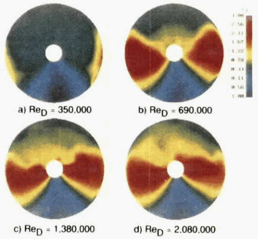
Figure 7.19. Frontal view of pressure distribution for the circular ogive at 90° angle of attack; \Omega b/2V = -0.2 .
