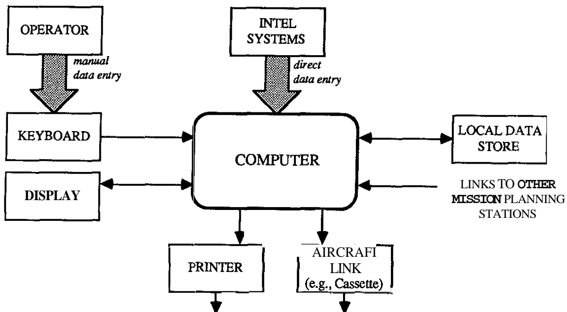
Figure 2-1. Schematic of a Typical Mission Planning System.
