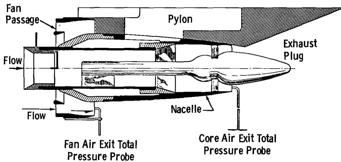
Fig.4.2.5 Schematic of dual stream turbofan engine
