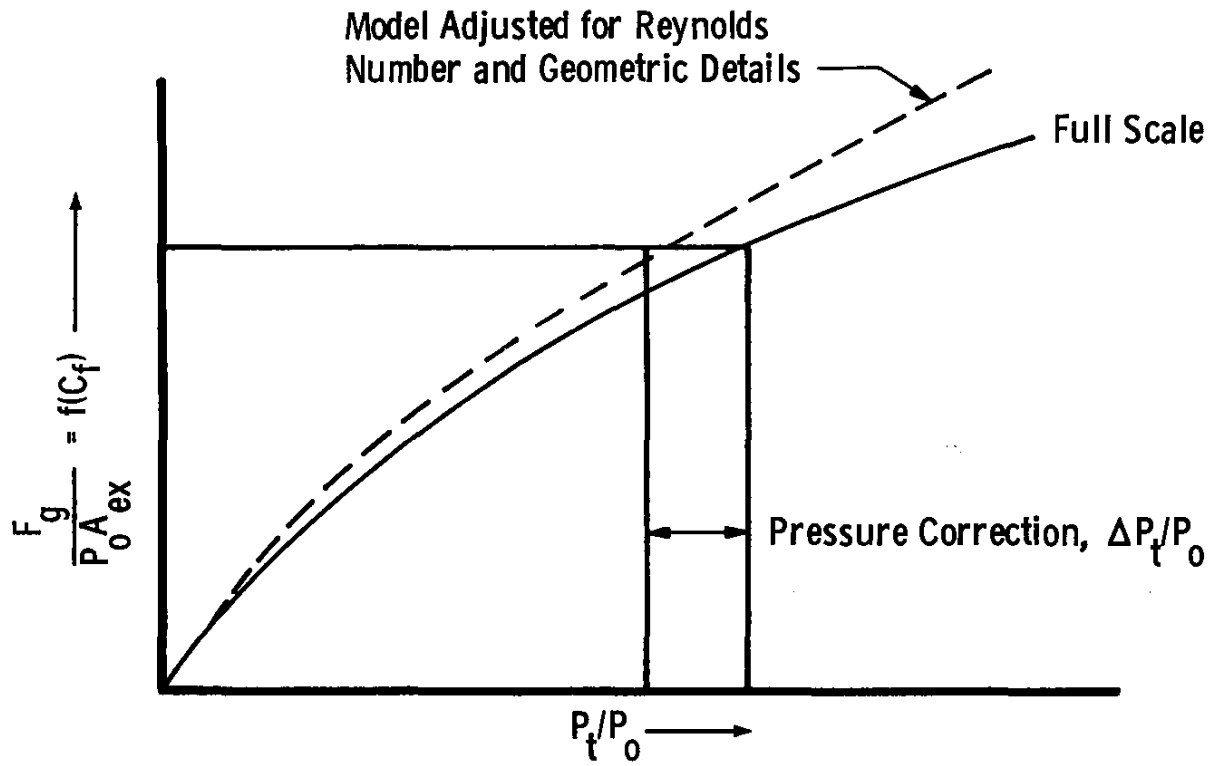
Fig.4.2.8 (Ref.4.2.4) Model to full-scale pressure correction
