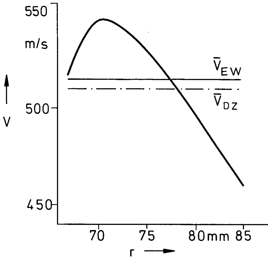
Fig.4.3.7 Section 2, velocity
