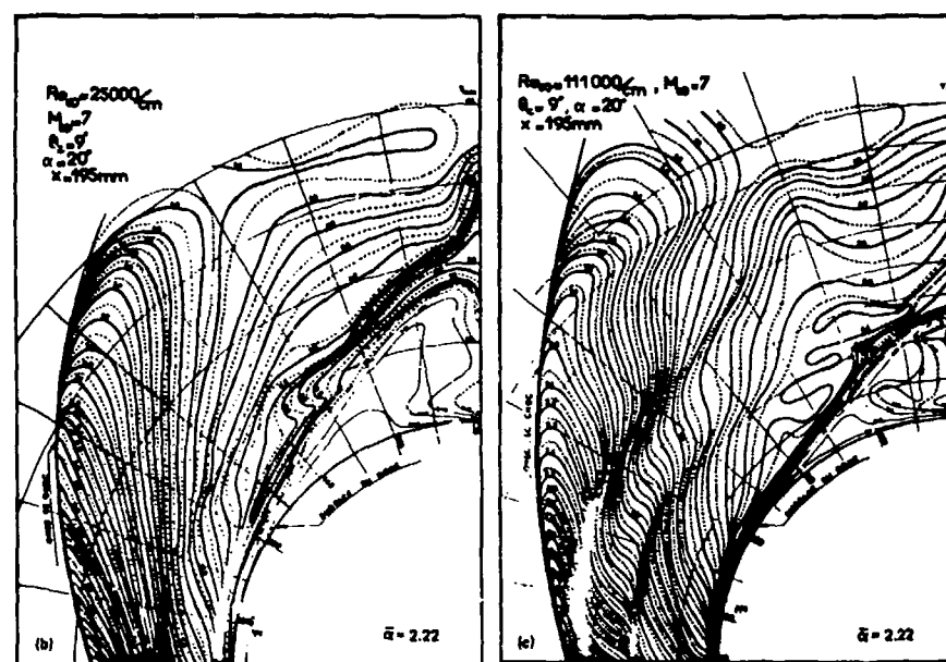
(b), (c) PITOT PRESSURE CONTOURS IN FLOWFIELD ABOUT CIRCULAR CONE AT RELATIVE INCIDENCE \bar{\alpha} = 2.22 , AT M_\infty = 7 (b) R_{x_{min}} = 4.9 \times 10^5 AND (c) R_{x_{min}} = 21.6 \times 10^5 (GUFFROY ET AL. 1968)
