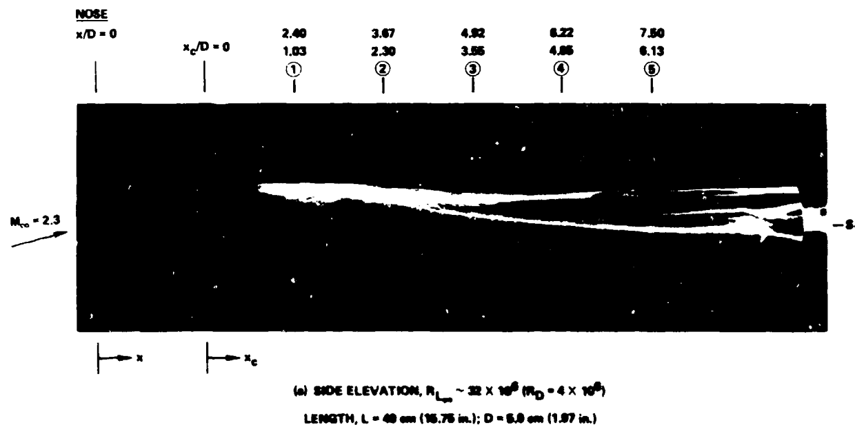
Fig. 95 Surface oil-flow patterns and circumferential pressures on \theta_c = 20^\circ pointed cone-cylinder at \alpha = 0.6 , M_\infty = 2.3 with turbulent boundary layers (Boersen 1975).
