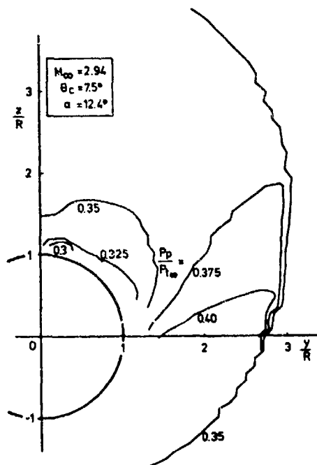
(b) LINES OF CONSTANT PITOT PRESSURE
