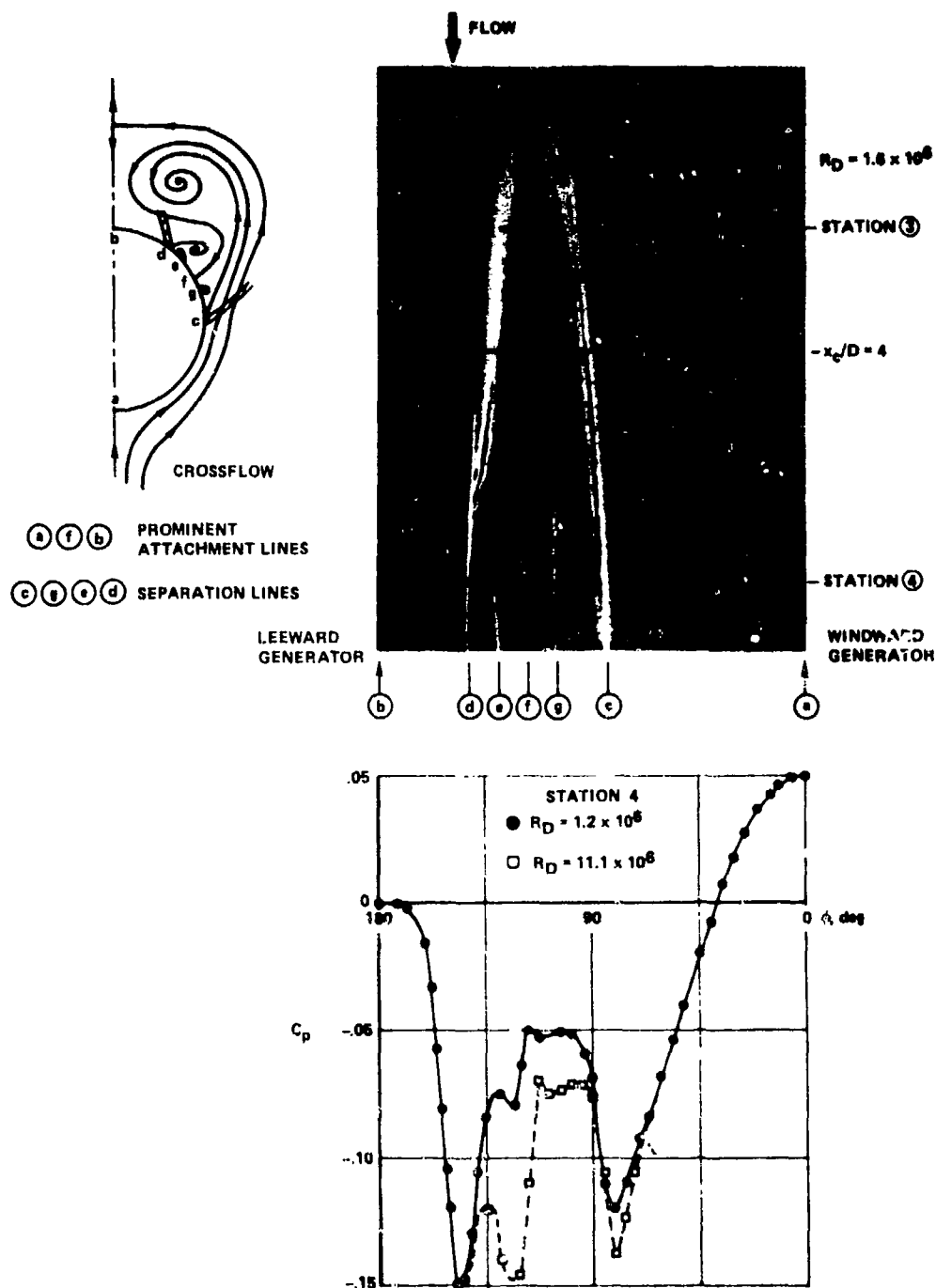
(c) OCL FLOW AND SURFACE PRESSURES ON DOWNSTREAM PART OF AFTERBODY
