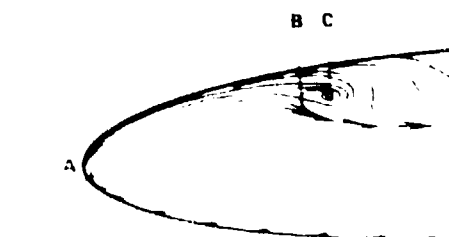
(a) ORIGINAL SKETCH OF SKIN-FRICTION LINES BY LEGENDRE 1985 A: NODAL ATTACHMENT POINT B: SADDLE POINT C: FOCUS OF SEPARATION
