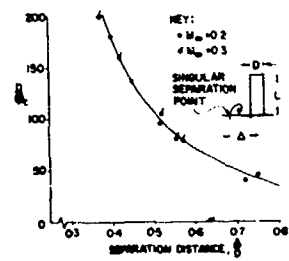
(b) DEPENDENCE OF SEPARATION DISTANCE A/D UPON D/\delta^* RATIO
