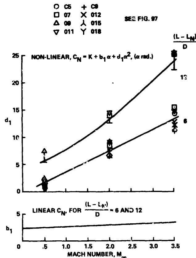
Fig. 99 Linear and nonlinear lift on long, pointed slender bodies at R_D = 1 \times 10^6 to 4 \times 10^6 (Peake, Rainbird, and Atraghji 1972).
