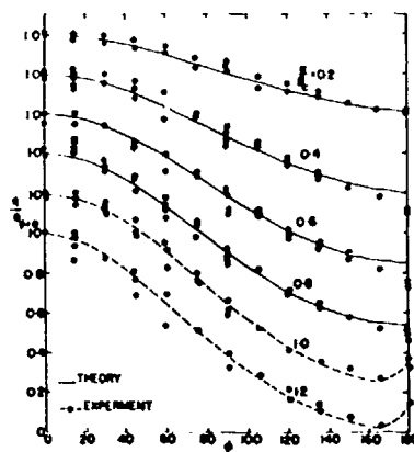
(c) HEAT-TRANSFER DISTRIBUTIONS ON A 15^\circ CIRCULAR CONE AT M_\infty = 10.4 , R_{x_m} = 10^6
