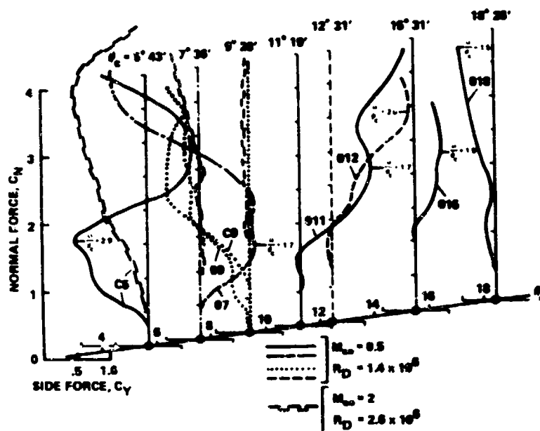
Fig. 101 Influence of semi-nose angle \theta_c on side-force-normal-force polar for afterbody length of 12D at R_D = 1 \times 10^6 to 4 \times 10^6 (Peake, Rainbird, and Atraghji 1972).
