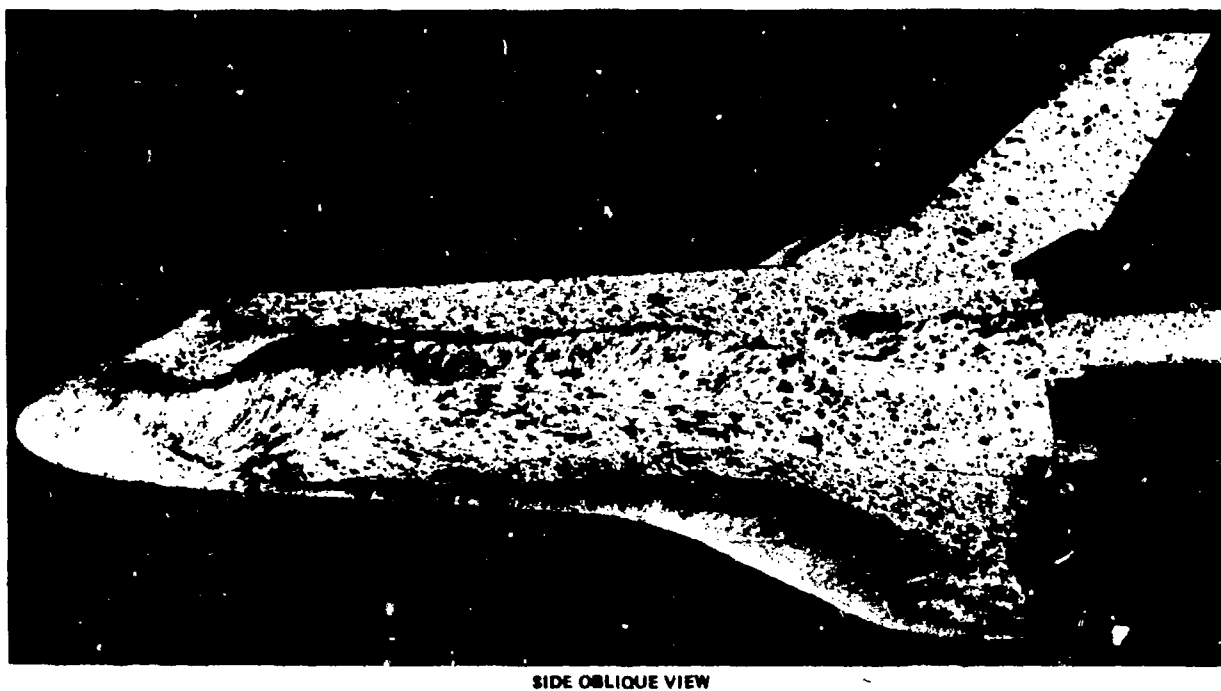
Fig. 201 Space Shuttle Orbiter at 30^\circ angle of attack: M_\infty = 20 and R_{L_\infty} \sim 1 \times 10^6 (Stone and Mulfinger 1974).
