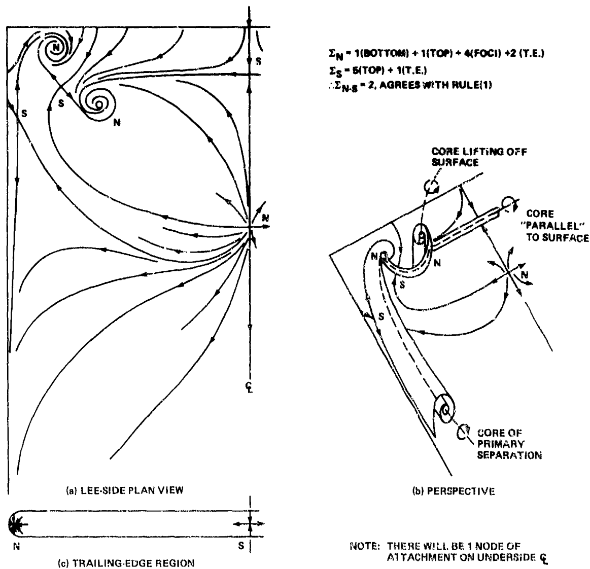
Fig. 21 Interpretation of skin-friction lines on slender, rectangular wing.
