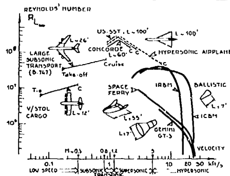
Fig. 3 Flight domains.
