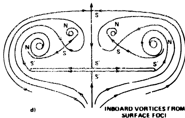
Fig. 25 Cross-flow streamlines about slender configuration at angle of attack.
