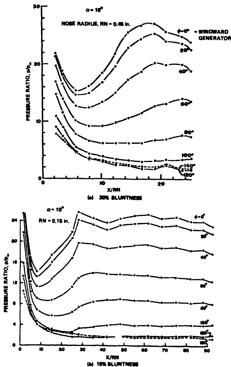
Fig. 76 Longitudinal pressure distributions on \theta_c = 5.6^\circ blunt cones at M_\infty = 14.2 and R_{L_\infty} \sim 0.4 \times 10^6 ; laminar, \gamma = 1.79 (Statson 1971).
