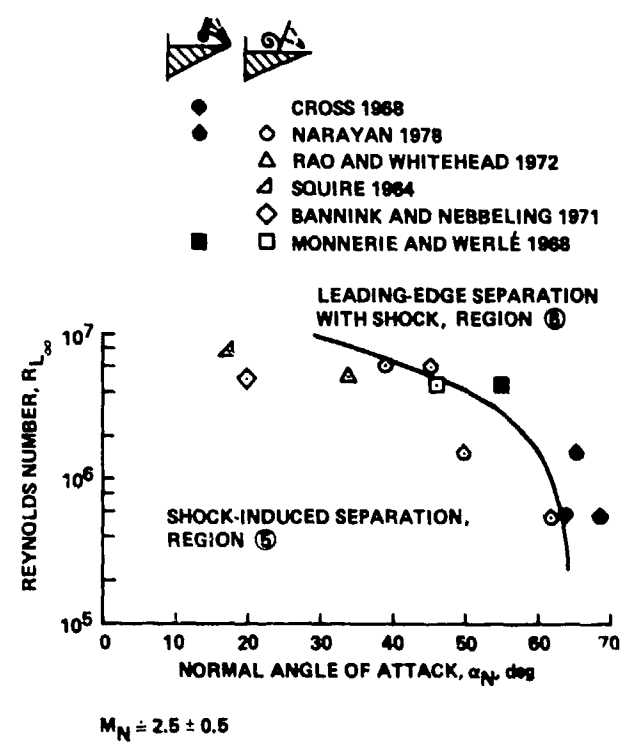
Fig. 172 Influence of Reynolds number on flow types and boundaries at M_N \sim \text{constant} (Szodruch and Peake 1980).
