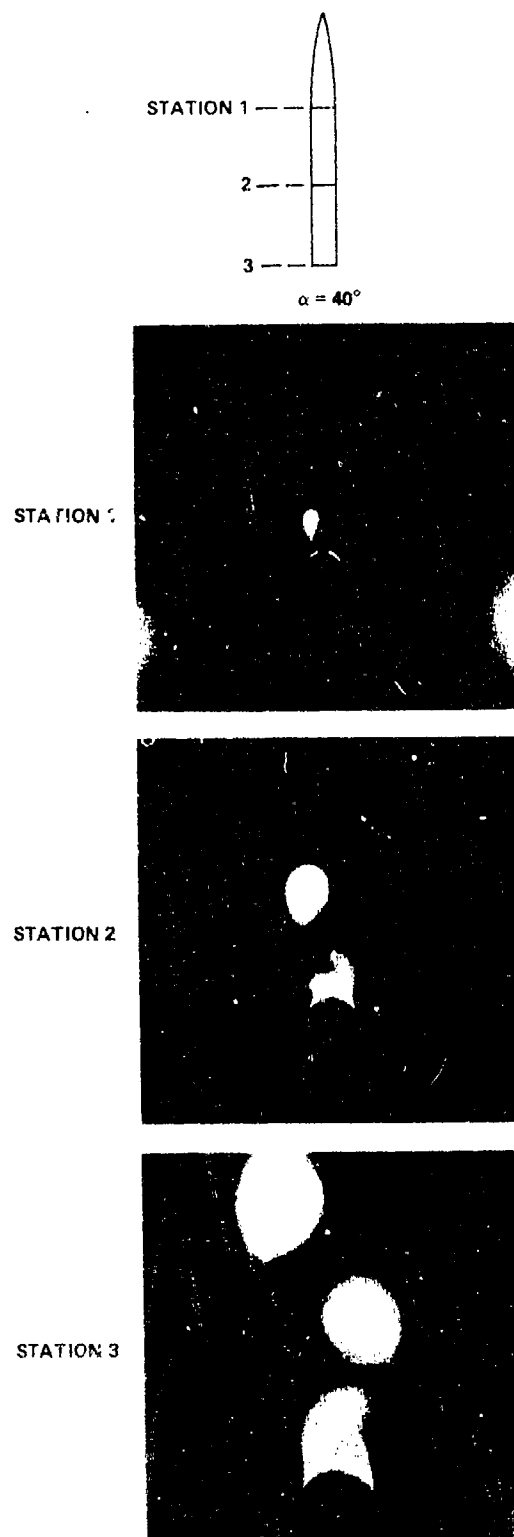
Fig. 31 Vapor-screen photographs of asymmetric flow along ogive-cylinder at M_\infty = 0.6 (Jorgensen 1977).
