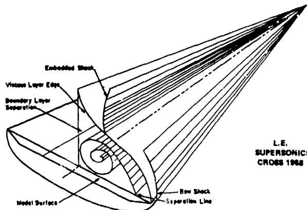
(b) DOMINANT FEATURES OF LEE SIDE FLOW FIELD ABOUT 75° DELTA WING
