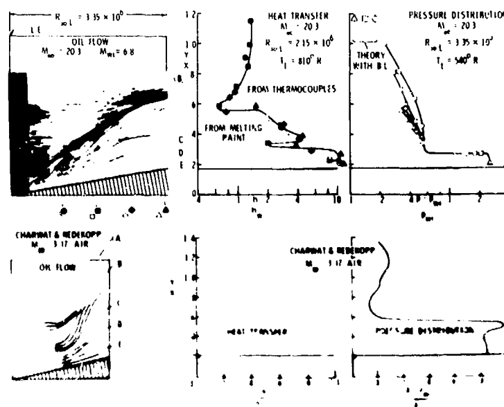
Fig. 149 Oil flow, heat transfer, and pressure distributions from experiments in helium with \theta_1 = \theta_2 = 10^\circ and from the work of Charvat and Redhepp (1966) in air with \theta_1 = \theta_2 = 12.2^\circ (Bortman and Anderson 1969).
