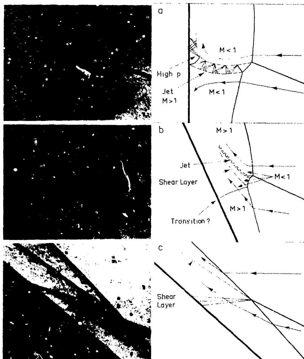
(a) TYPE IV INTERFERENCE. (b) TYPE V INTERFERENCE. (c) TYPE VI INTERFERENCE. M_{\infty} = 4.6 , \theta = 5^\circ (SHOCK GENERATOR DEFLECTION)
