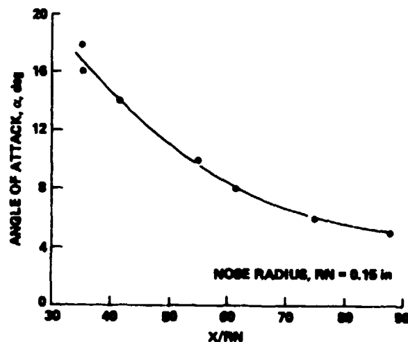
Fig. 75 Distance to return to conical (laminar) flow conditions on leeward side of \theta_c = 5.6^\circ blunt cone (10% bluntness) at M_\infty = 14.2 , R_{L_\infty} \sim 0.4 \times 10^6 (Statson 1971).
