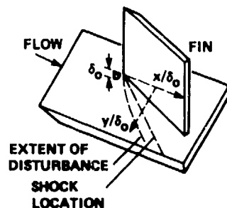
FLAT PLATE MODEL
