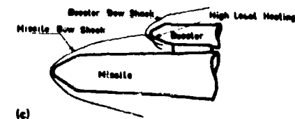
Fig. 156 Practical examples of shock-impingement heating (Edney 1968).
