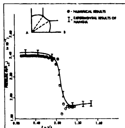
Fig. 148 Inviscid corner flow calculations of Shankar, Anderson, and Kutler (1975) compared with turbulent flow experimental result of Nangia (1974).
