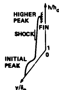
SURFACE HEAT- TRANSFER PROFILE
