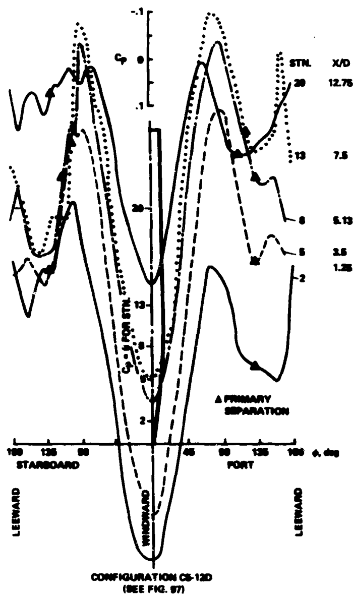
Fig. 104 Circumferential pressures on a 5.7^\circ cone-cylinder at \alpha = 25^\circ , M_\infty = 0.5 , and R_0 = 1.4 \times 10^6 with asymmetric separation line positions.
