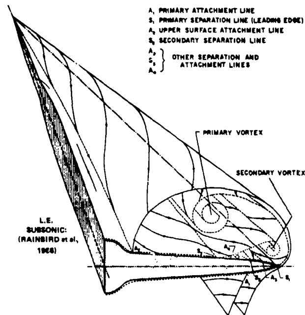
(a) INTERPRETATION OF FLOW ABOUT 70° DELTA WING AT 16.5° ANGLE OF ATTACK
