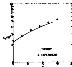
(b) HEAT-TRANSFER COEFFICIENT (STANTON NUMBER) AT THE MOST WINDWARD GENERATOR ON A 15^\circ CIRCULAR CONE AT M_\infty = 10.4 , R_{x_m} = 10^6
