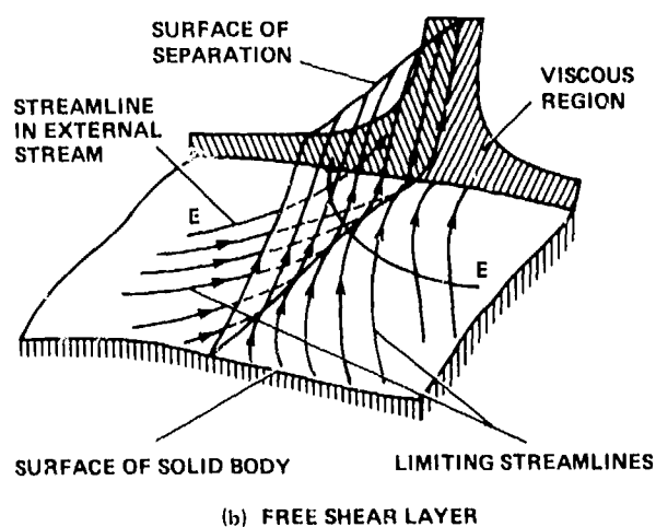
Fig. 9 3D separations (after Maskell 1955).
