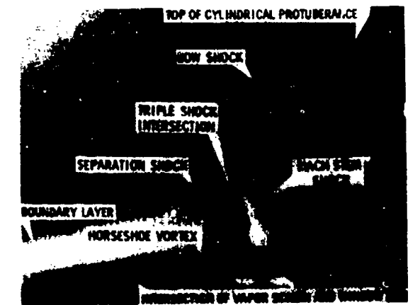
VAPOR SCREEN PHOTOGRAPH FOR LARGE PROTUBERANCE, WITH LIGHT SHEET IN SYMMETRY PLANE AND CAMERA AT 30^\circ TO SHEET, M_\infty = 2.50 , R/\ell = 9.3 \times 10^6/m
