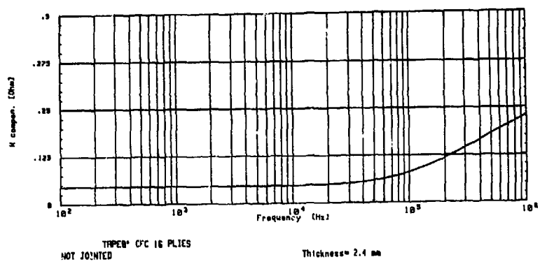
Fig.9 A.C. measurements on CFRP UD laminates (0° fiber direction)
