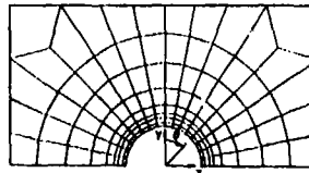
FIG. 9: NASTRAN MODEL OF THE REGION IN THE VICINITY OF THE FASTENER HOLE (REF. 39)
