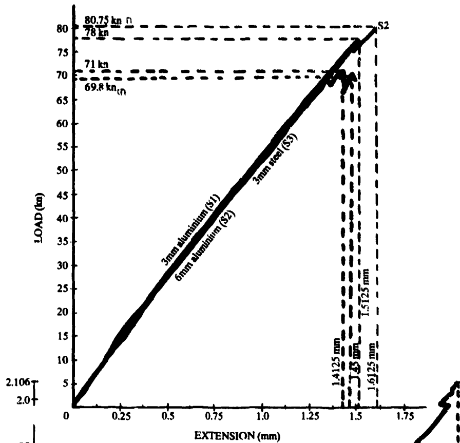
FIG.11 LOAD EXTENSION CURVES FOR S1 TO S3 (A06 TO A08)
