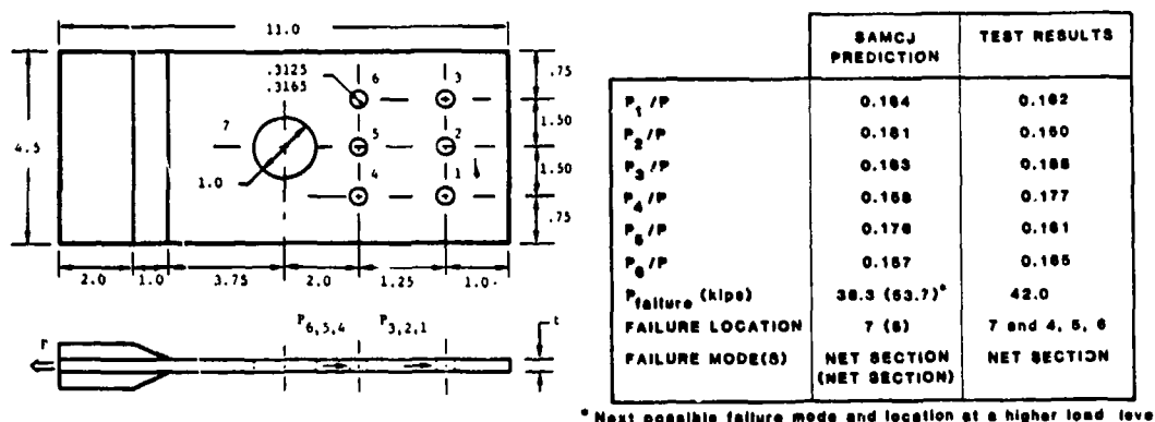
Figure 17. SAMCJ Predictions and Test Results for Test Case 243 ( Ref.6 ).
