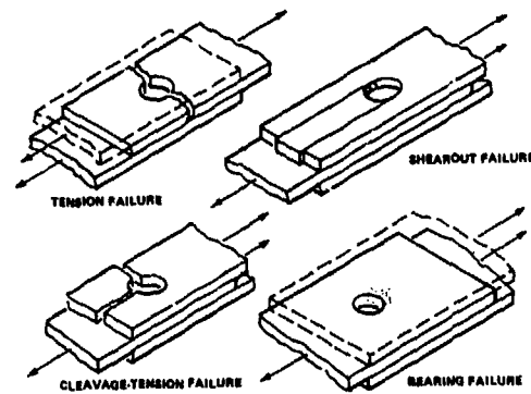
FIG. 7: MODES OF FAILURE FOR BOLTED COMPOSITE JOINTS
