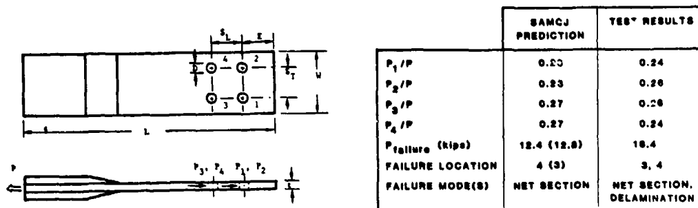
Figure 16. SAMCJ Predictions and Test Results for Test Case 320 ( Ref.6 ).
