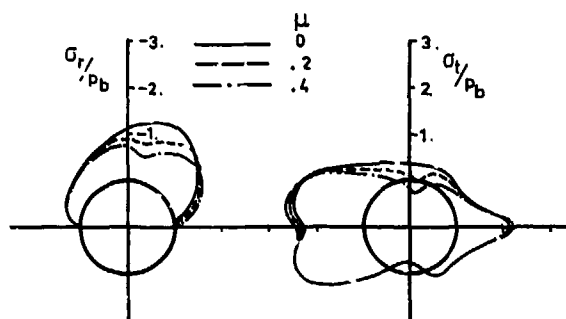
Figure 15: The effects of the friction coefficient \mu on the stresses around a pin-loaded hole in the [0_3/\pm 45]_s - laminate for s/D = 3 and \varphi = 30^\circ .
