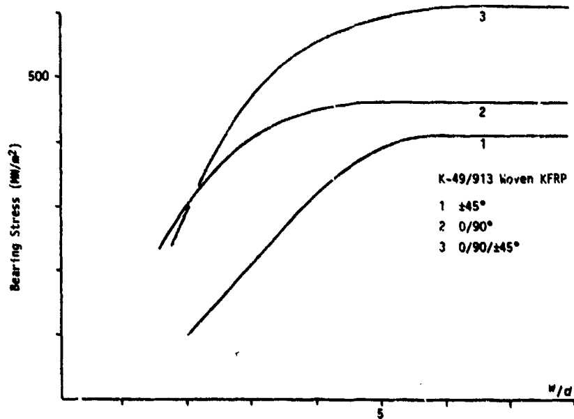
Figure 1. Variation of Failure Bearing Stress with w/d for 'Kevlar' Fibre Laminates
