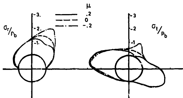
Figure 13: The effects of the friction coefficient \mu on the stresses around a pin-loaded hole in the [0_4/\pm 45]_s - laminate for s/D = 3 and \varphi = 30^\circ .
