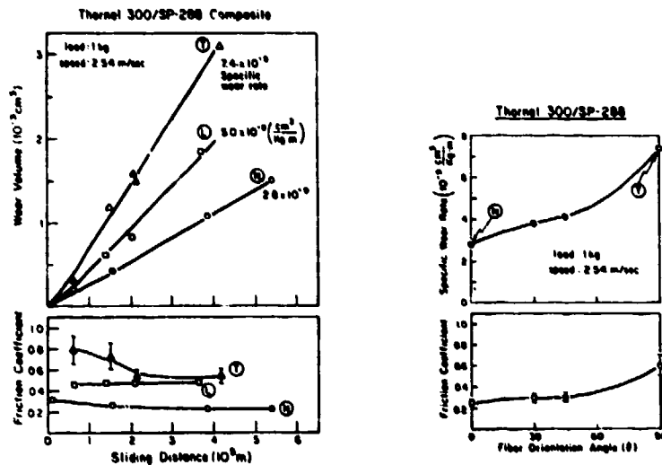
FIG. 4: FRICTION COEFFICIENTS AND WEAR VOLUME AS A FUNCTION OF SLIDING DISTANCE IN UNIAXIAL GRAPHITE FIBER-SPOKY COMPOSITE. SLIDING AGAINST S2100 STEEL, WITH FIBER ORIENTATIONS NORMAL, LONGITUDINAL AND TRANSVERSE TO THE SLIDING DIRECTION (REF. 11)
