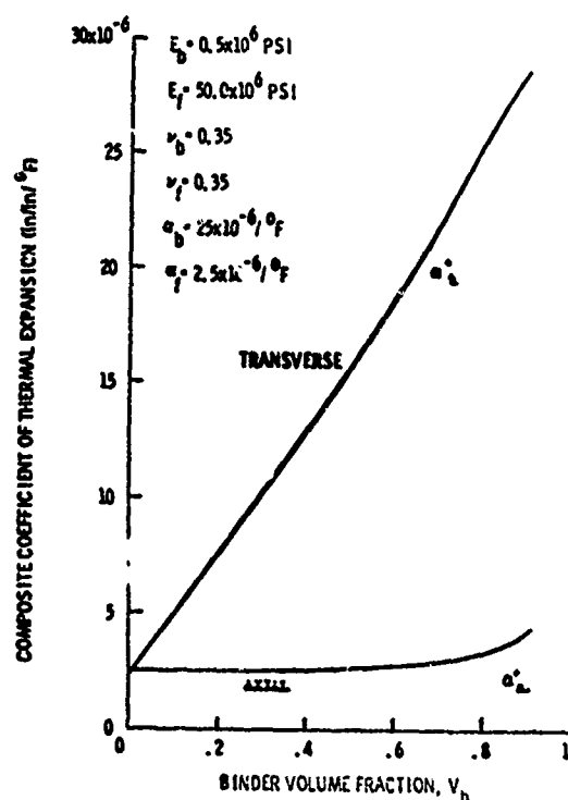
Fig. 8 Effective Composite Thermal Expansion Coefficients.
