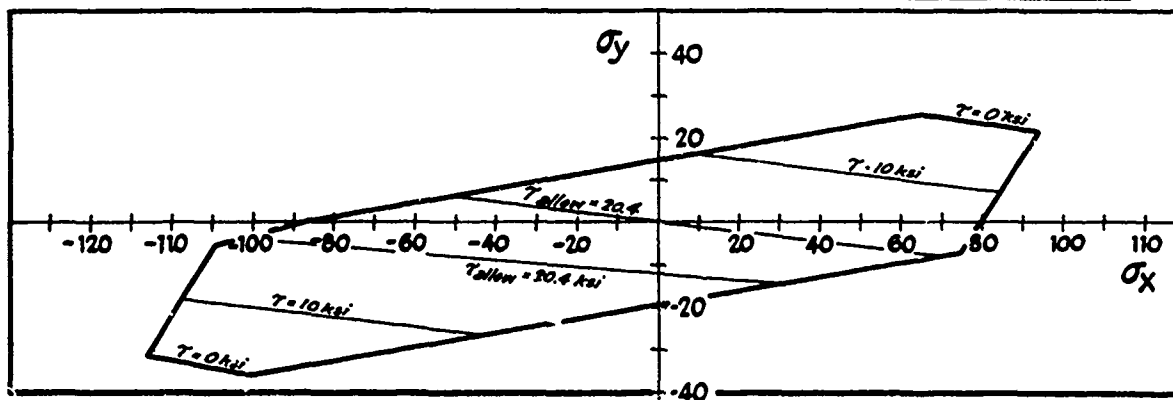
Figure 8 Limit-Interaction Curve
