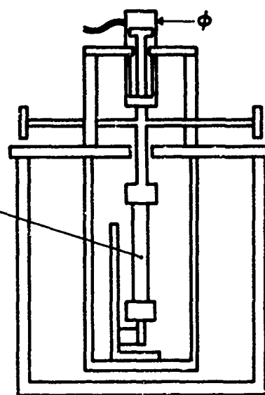
FIG.13 TORSION PENDULUM
