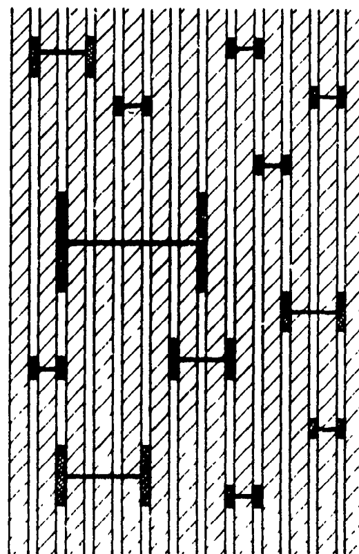
Fig. 10 Distribution of Damage in a Fiber Composite Material Resulting from an Applied Tensile Load.
