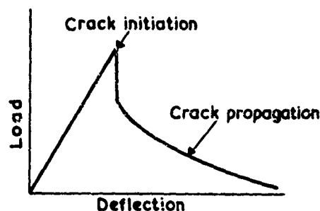
FIG.26 LOAD-DEFLECTION CURVE FOR SLOW BEND TEST
