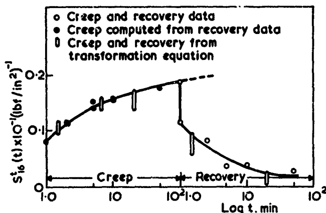
FIG.8 CREEP AND RECOVERY FOR NYLON IN RUBBER
