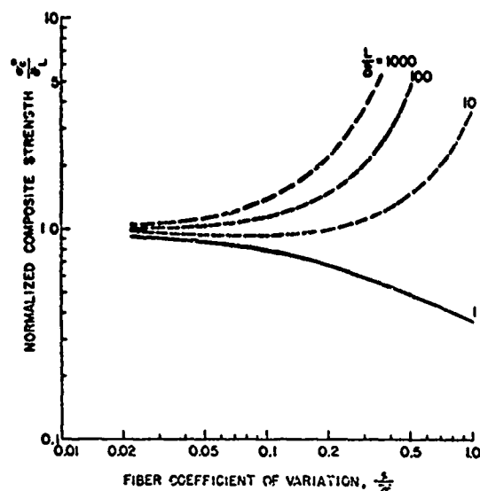
Fig. 12 Effect of Fiber Strength Properties upon Composite Tensile Strength for Cumulative Weakening Failure Model.
