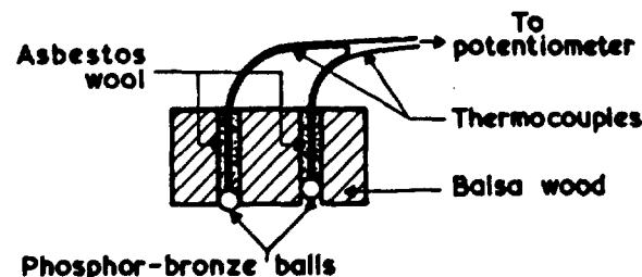
FIG.31 THERMAL COMPARATOR
