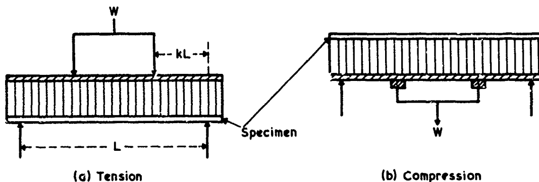
FIG.5 HONEYCOMB SANDWICH
