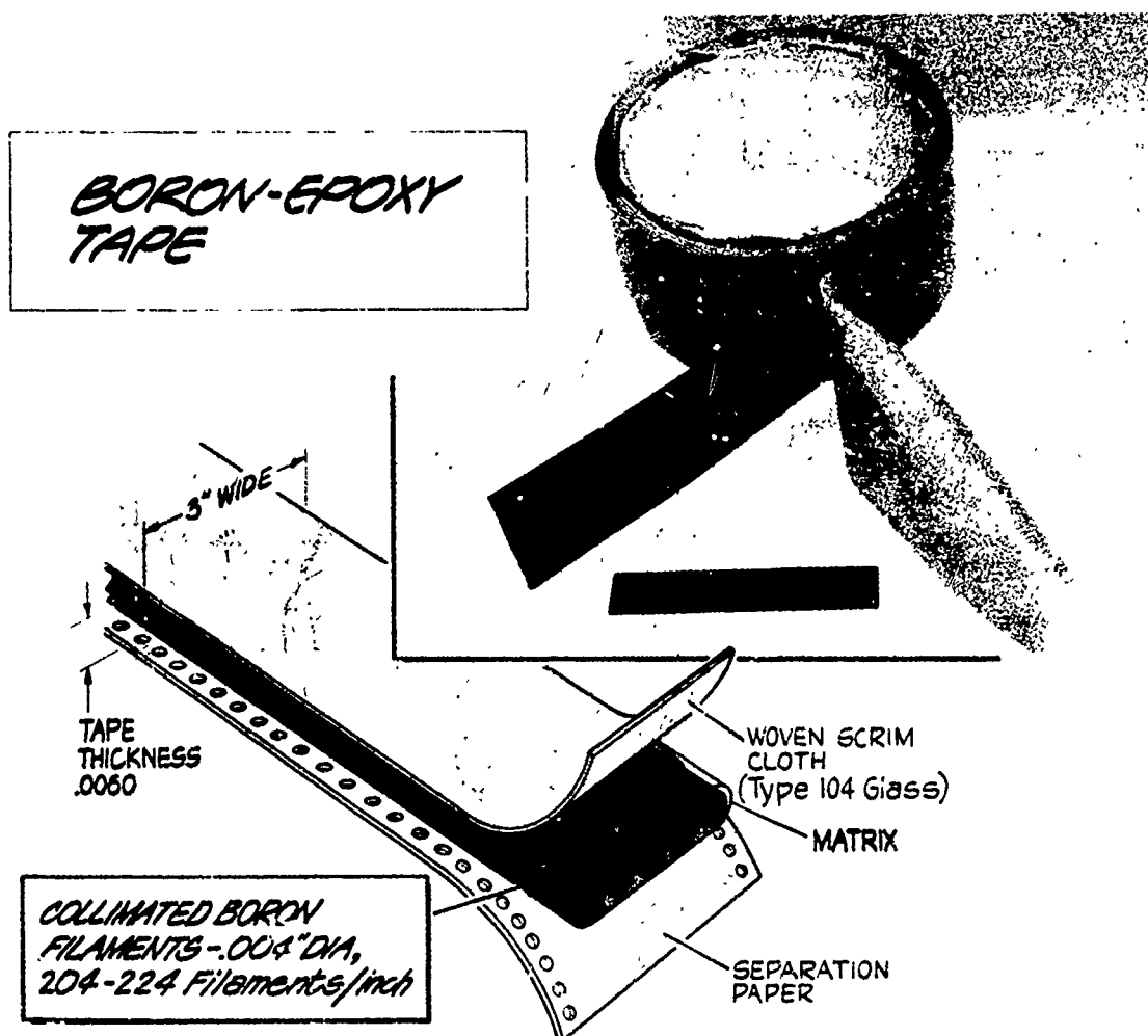
Figure 1 Boron-Epoxy Tape
