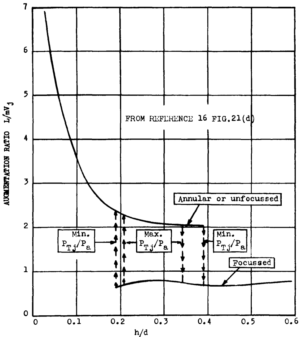
Fig.14 Lift hysteresis
