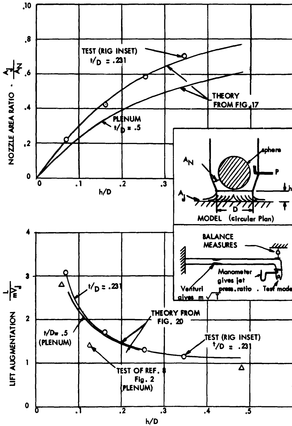
Fig.66 Plenum chamber lift data
