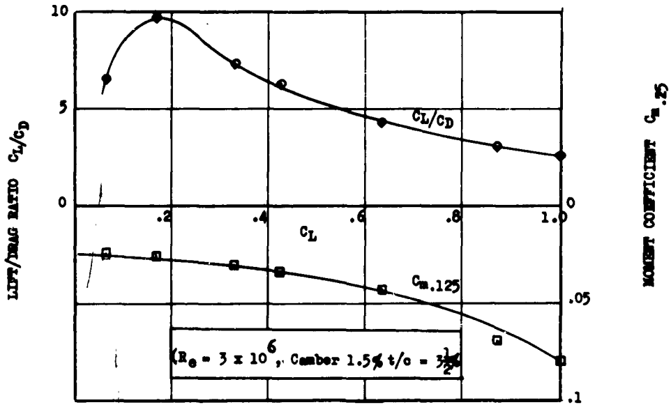
Fig. 78 Measured subsonic characteristics for a thin cambered biconvex aerofoil of circular planform
