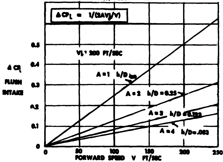
Fig. 76 Air intake pitching moment
