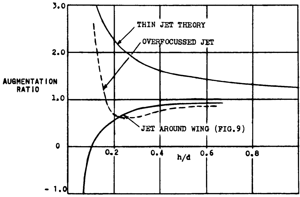
Fig.13 Overfocused jet
