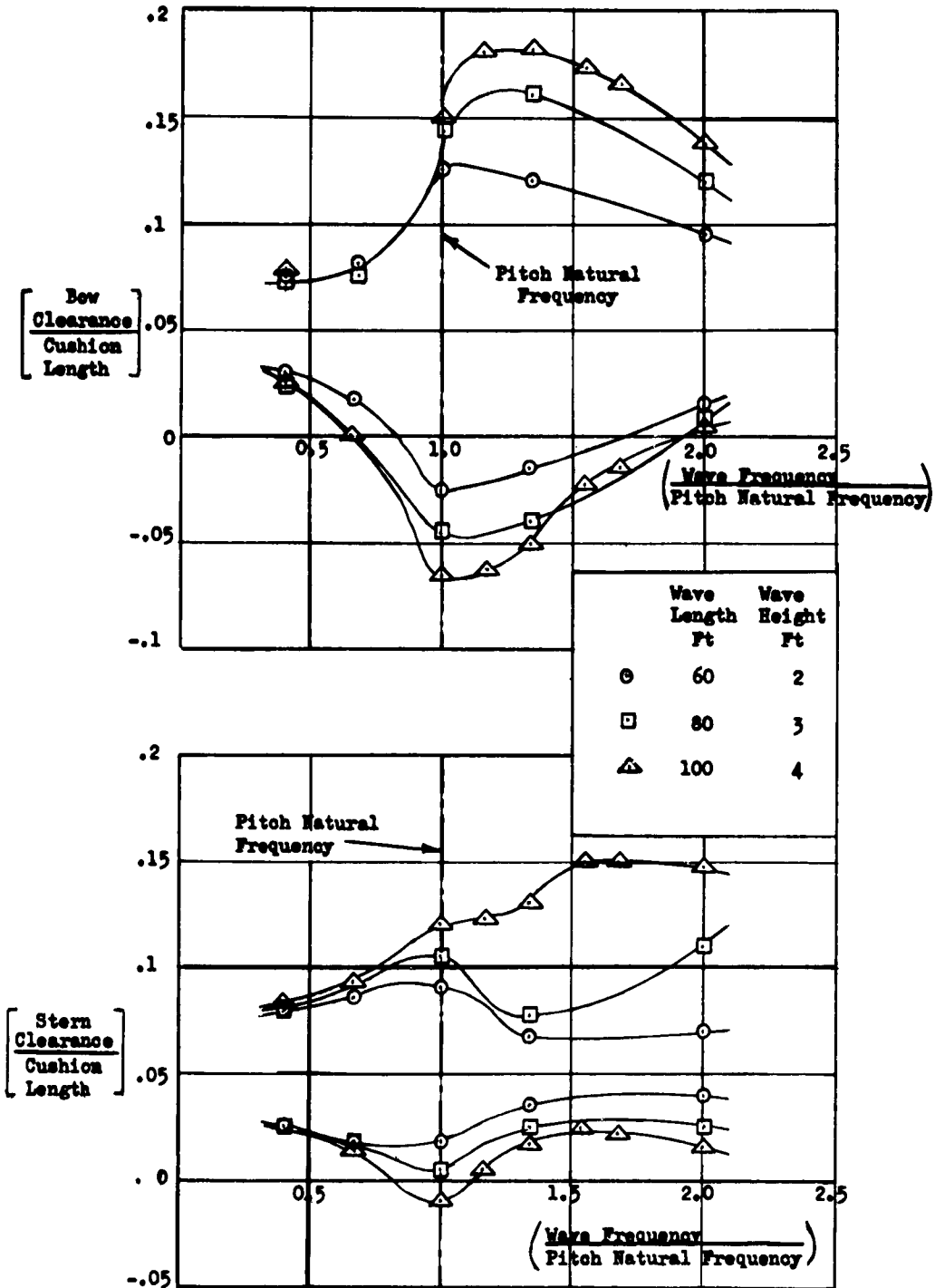
Fig. 39 Wave clearance
