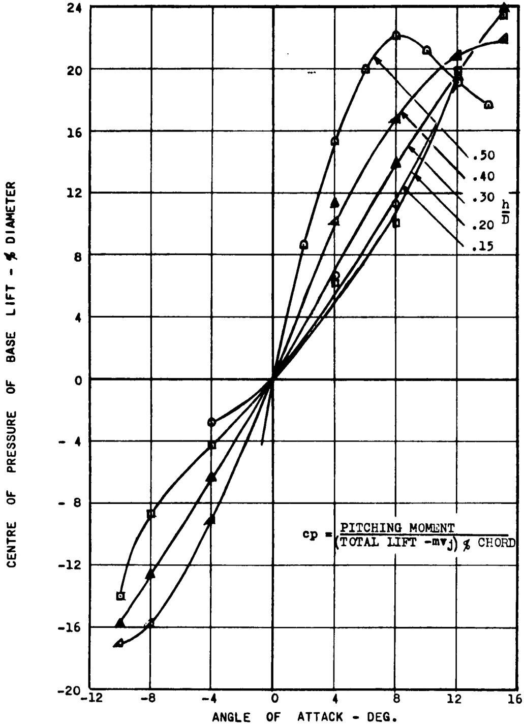
Fig.29 Half-plane model data; variation of base lift c.p. with ground angle and h/D
