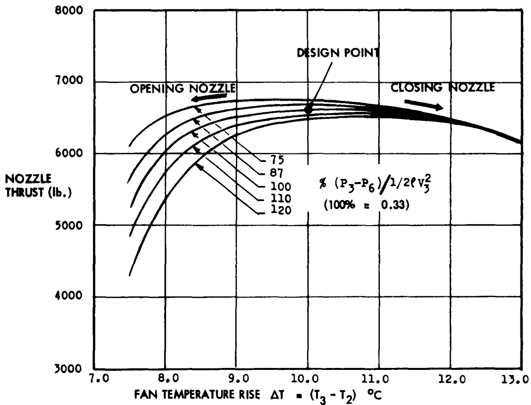
Fig. 55 Avrocar: estimated variation of nozzle thrust with fan temperature rise for different duct loss assumptions
