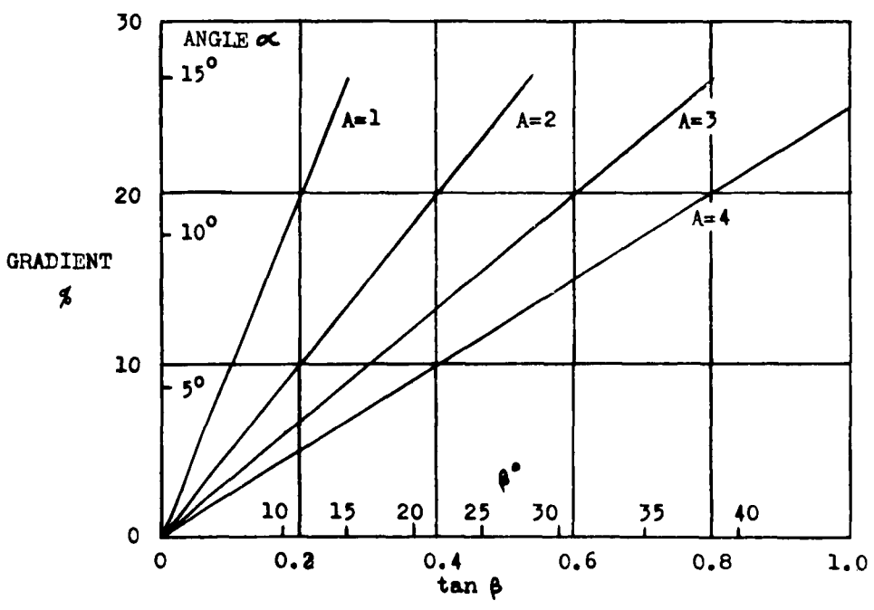
Fig. 89 Hill climb capability
