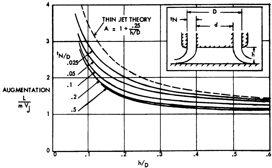
Fig. 20 Variation of augmentation with jet thickness
