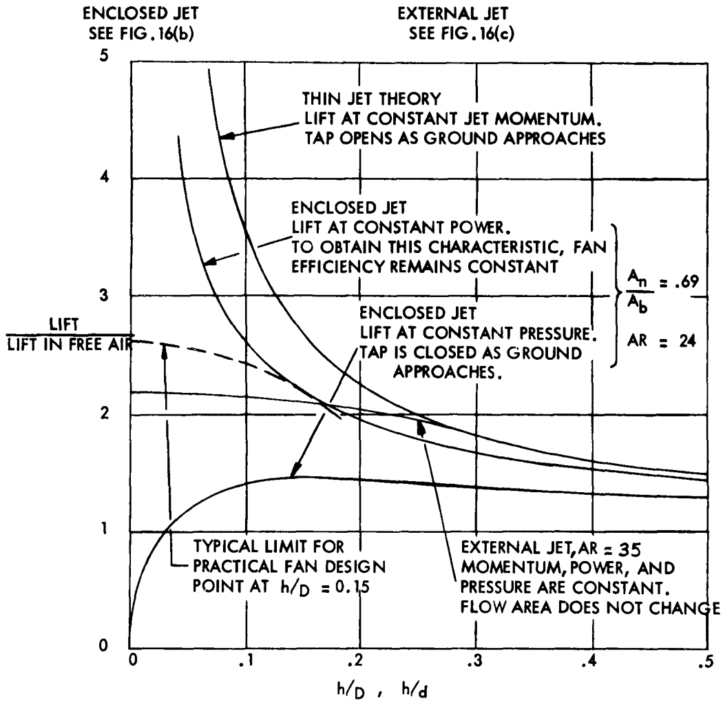
Fig. 50 Lift vs h/D and h/d for different modes of operation
