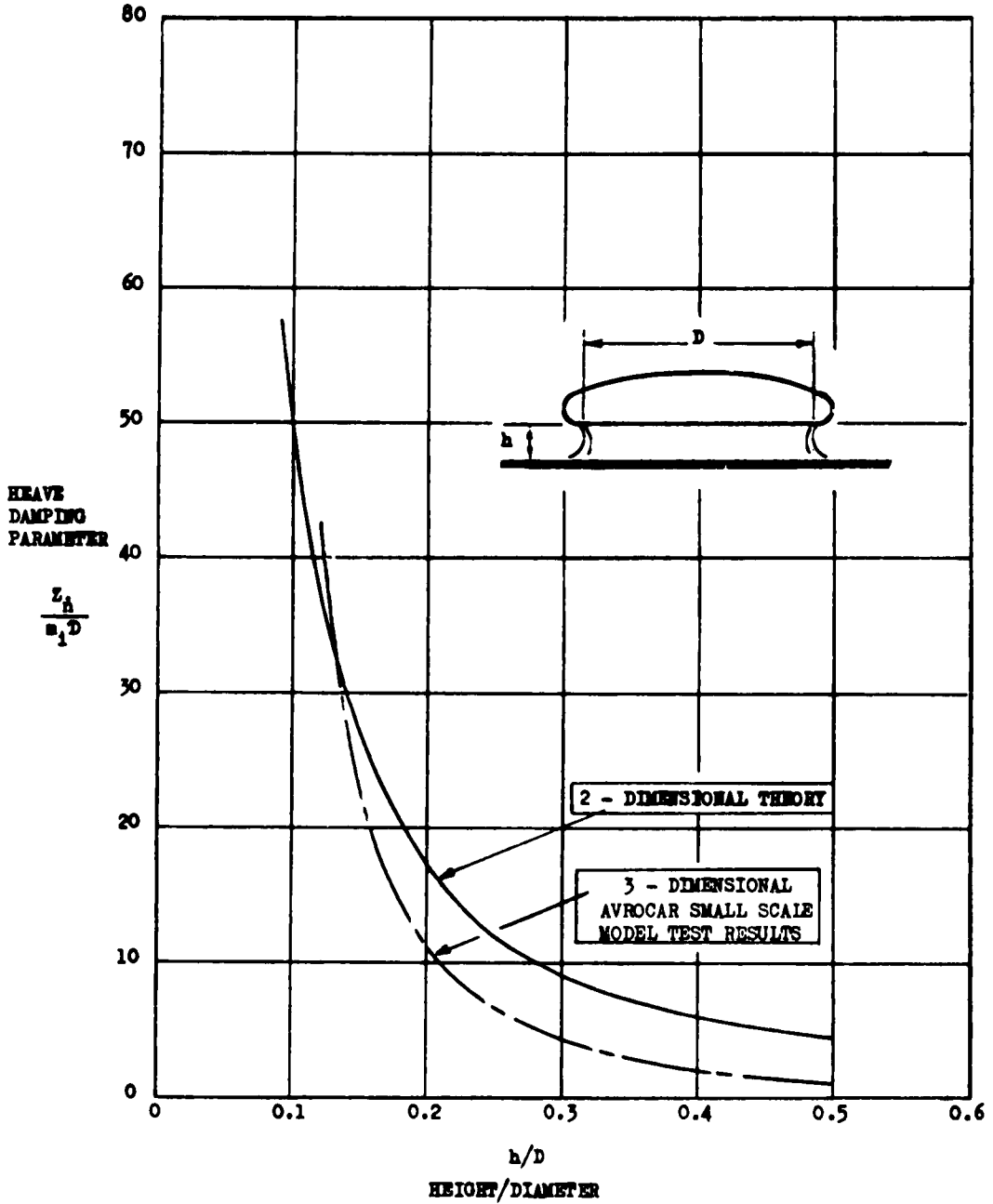
Fig.38 Heave damping
