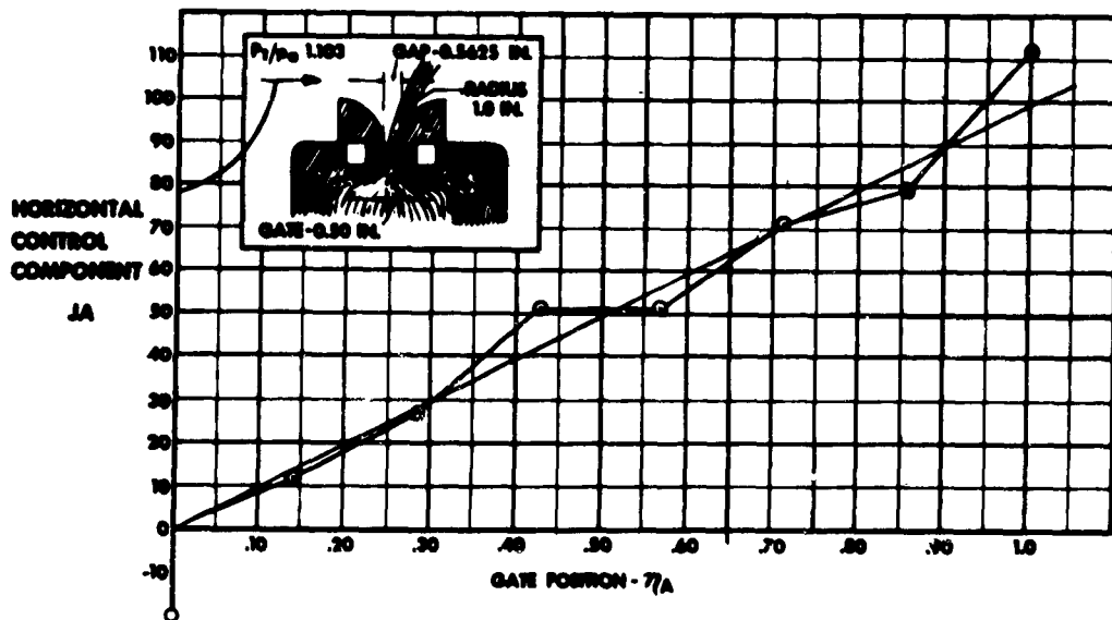
Fig.83 Spoiler control linearity
