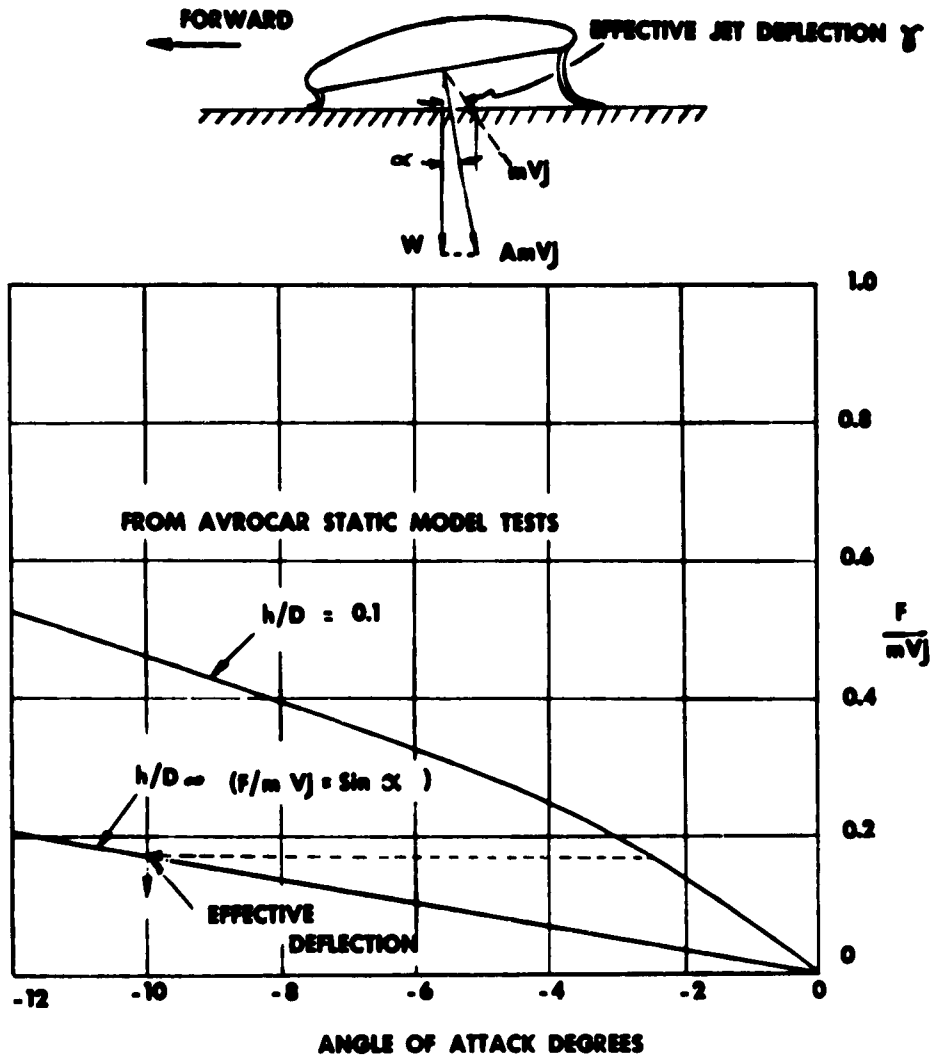
Fig. 49 Thrust recovery from inclination of cushion base
