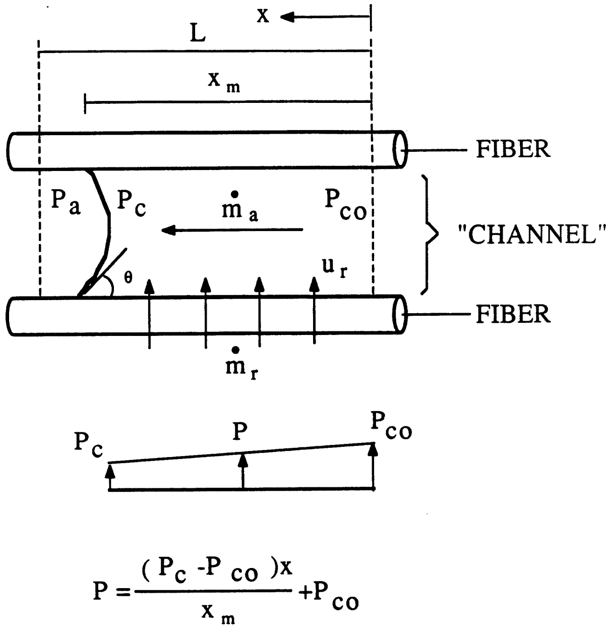
Figure 3. Annular channel used in modeling the matrix flow inside a tow.
