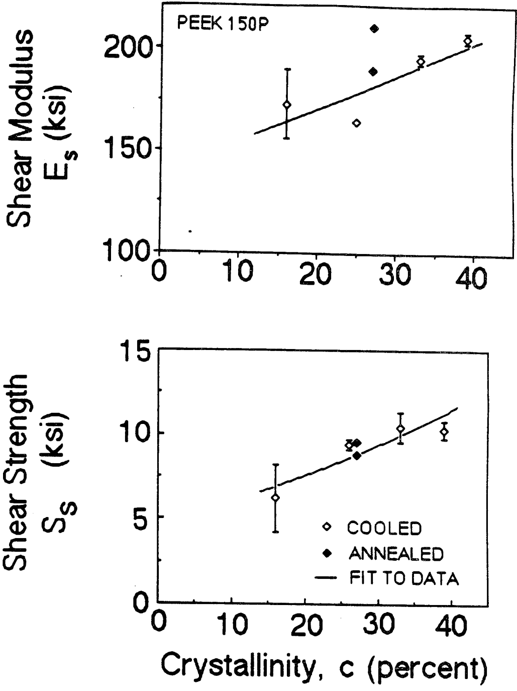
Figure 38. Shear properties of PEEK 150P as functions of crystallinity. The error bars represent the standard deviation of the data.
