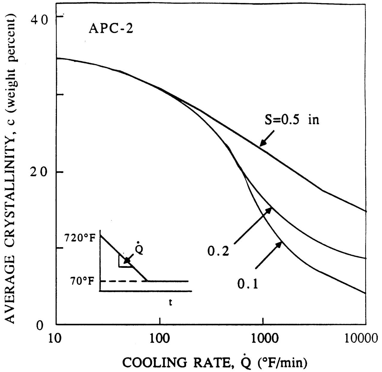
Figure 25. Average crystallinity as a function of surface cooling rate for an APC-2 composite. Results of the model.
