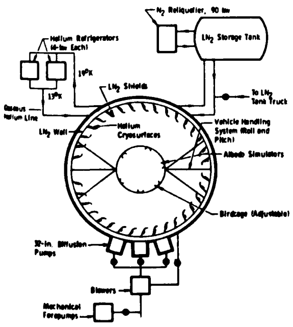
Mark I Schematic
