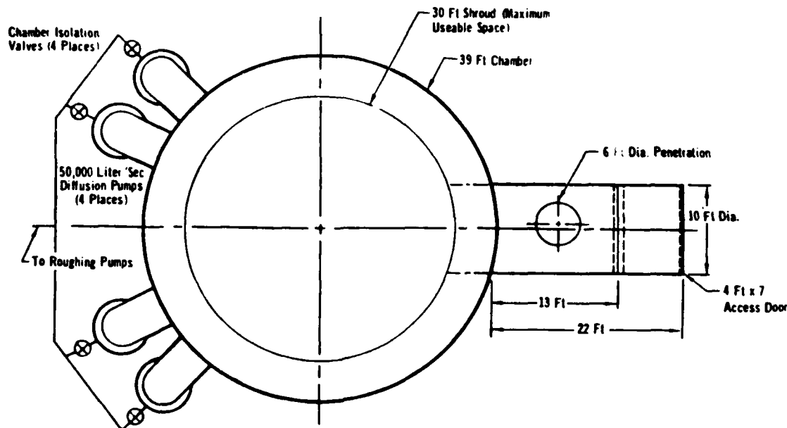
SCHMATIC
