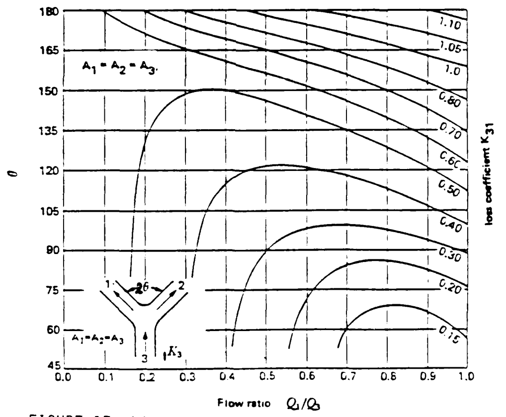
FIGURE 15 DIVIDING FLOW-SYMMETRICAL 'Y' JUNCTION REFERENCE (5)
