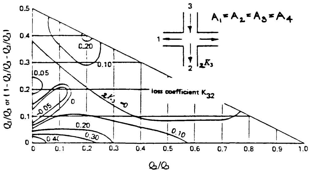
FIGURE 16 4-WAY DIVIDING JUNCTION. REFERENCE (5)
