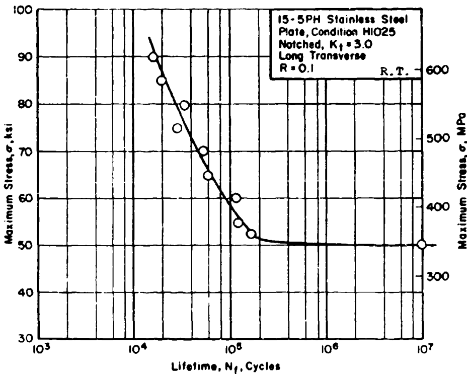
Figure B-4. Axial load fatigue data of notched 15-5PH stainless steel (H1025, long transverse).
