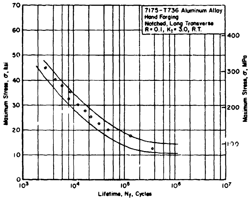
Figure B-8. Axial load fatigue data (one heat only).
