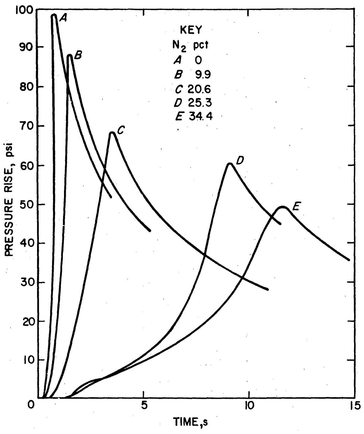
Figure 49. Explosion Pressure Histories for Stoichiometric Methane-Air Mixtures with Added Nitrogen at 25°C (77°F) and 1 atm (920 ft. 3 vessel).
