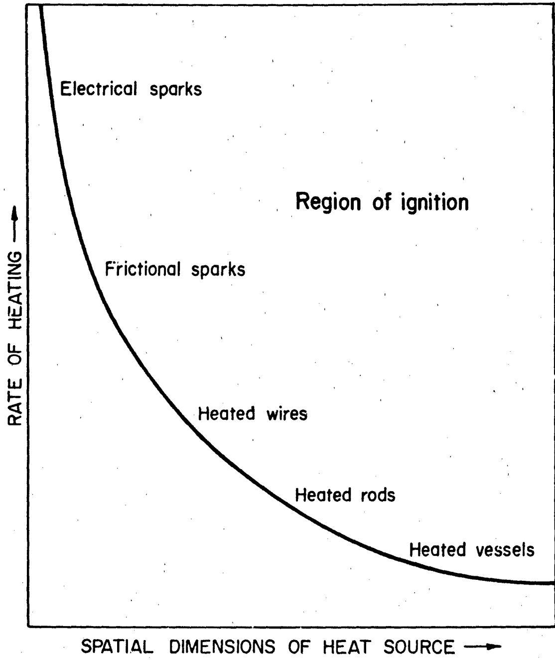
Figure 17. Temporal and Spatial Characterization of Various Ignition Sources
