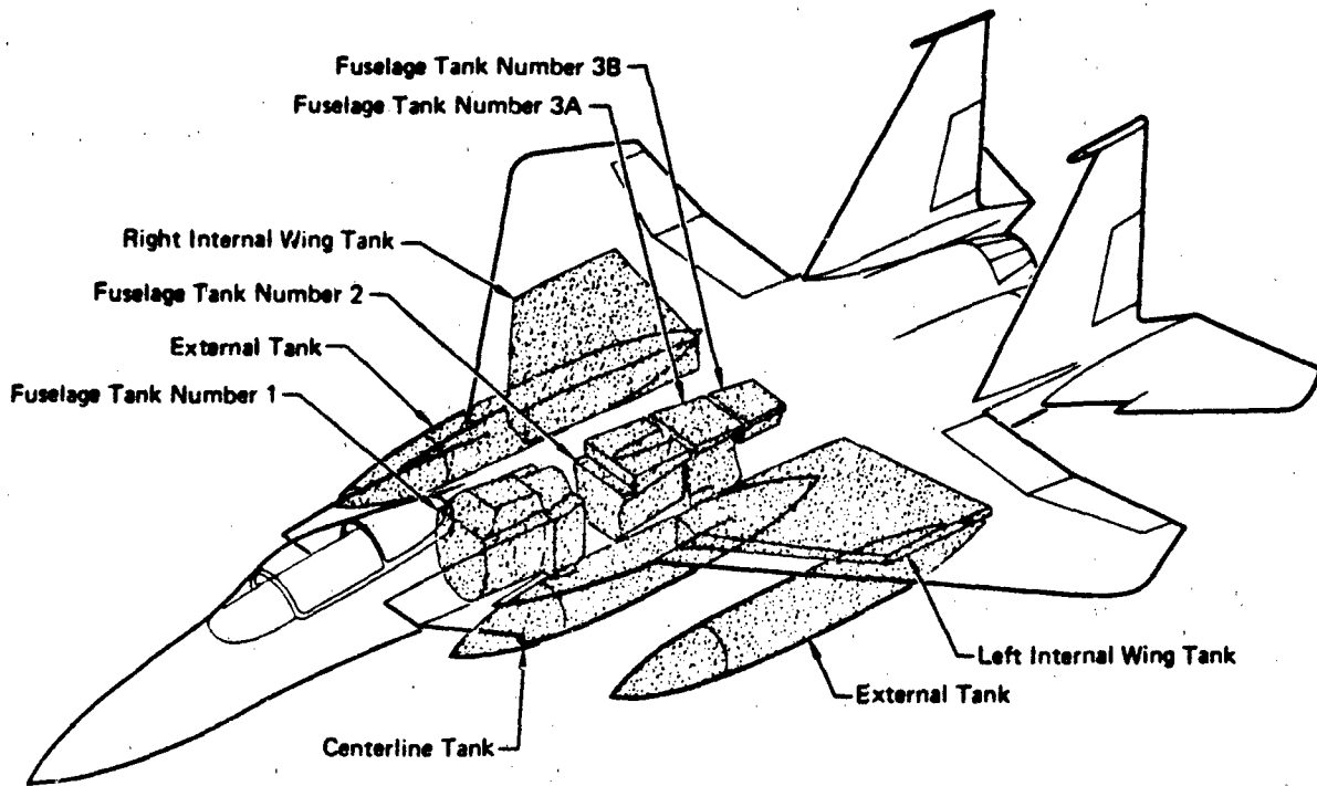
F-15A FUEL TANK ARRANGEMENT
