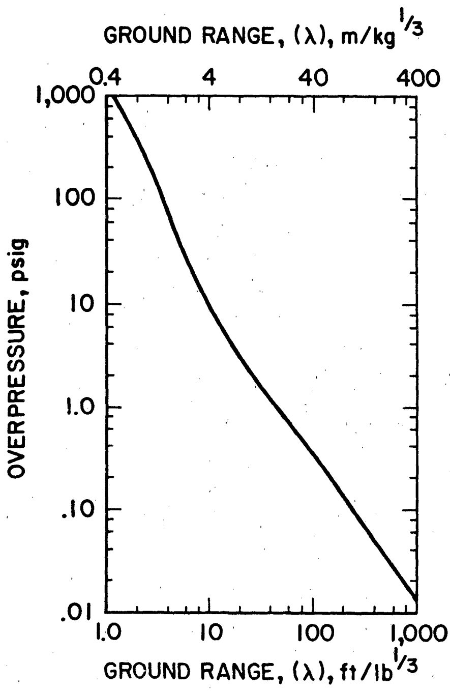
Figure 62. Peak Overpressure vs. Scaled Distance for Hemispherical TNT Surface Bursts
