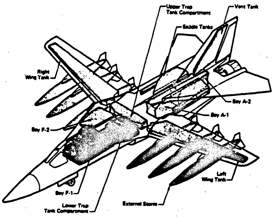
F-111 FUEL TANK ARRANGEMENT
