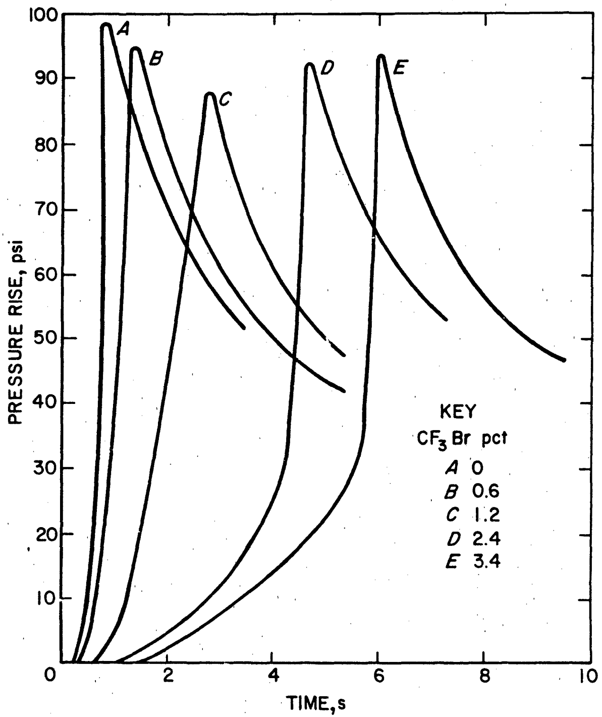
Figure 50. Explosion Pressure Histories for Stoichiometric Methane-Air Mixtures with Added Halon 1301 (CF 3 Br) at 25°C (77°F) and 1 atm (920 ft. 3 vessel).
