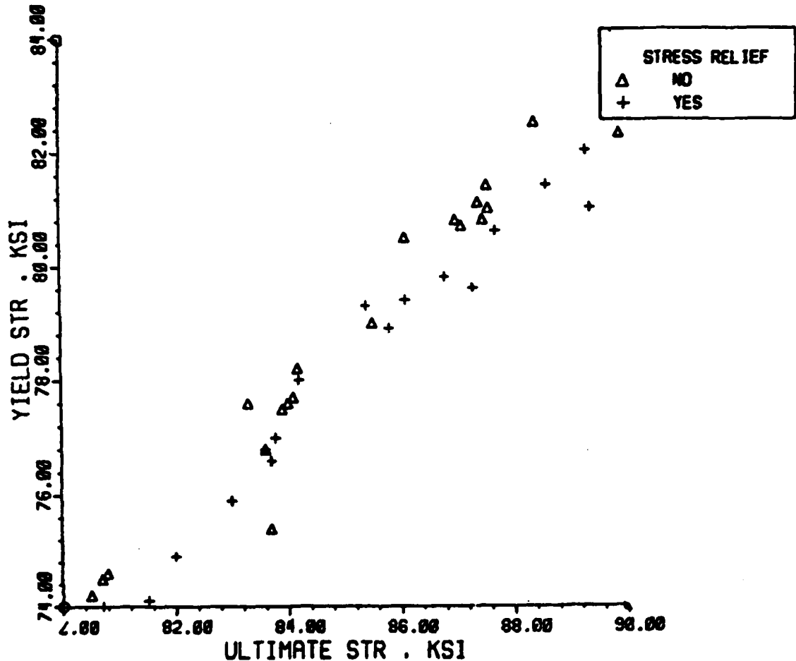
Figure 48. Effect of Stress Relief on Strength.
