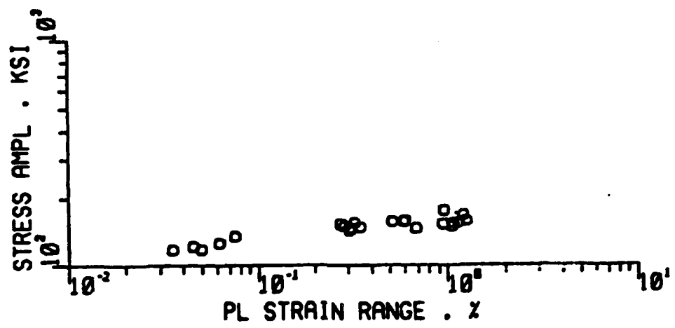
(a) o All data n' = 0.085 .
