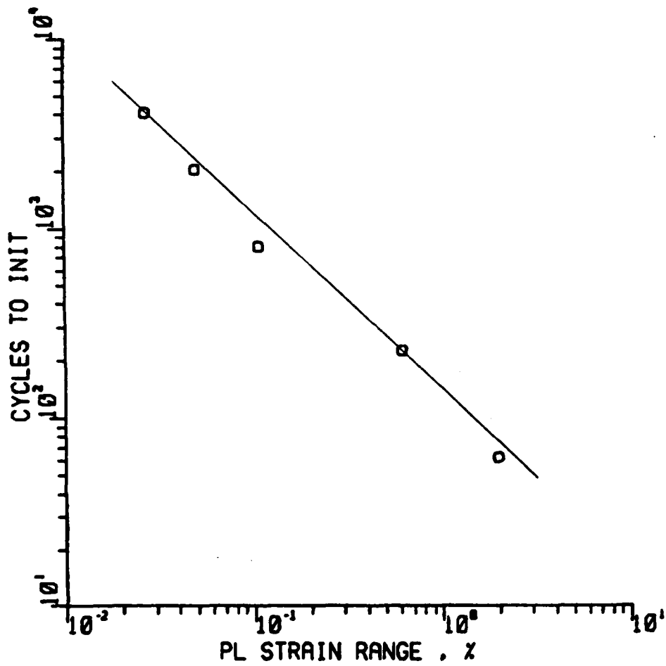
Figure 74. Typical Coffin-Manson Plot. This curve is for Condition 111 (64% upset, 0.4% Co, stress relieved). The slope is - 0.938 and \beta = 1/m = 1.07 . There is no indication of dual slope behavior.
