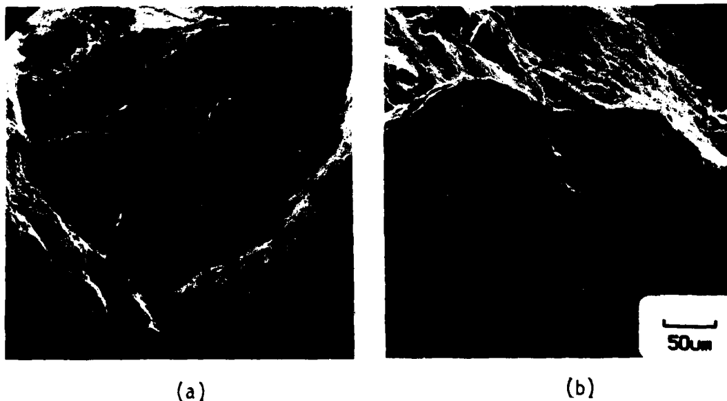
Figure 97. In Spite of Running Tests at A_c = 0.95 , Smearing is Occasionally Encountered in High Strain Tests. (a), (b), and (c) are increasing magnification SEM fractographs showing the smeared initiation site. Condition 001, Sample DD1R-2, 0.638%, N_i = 165 .
