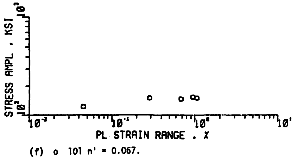
Figure A2 Continued.
