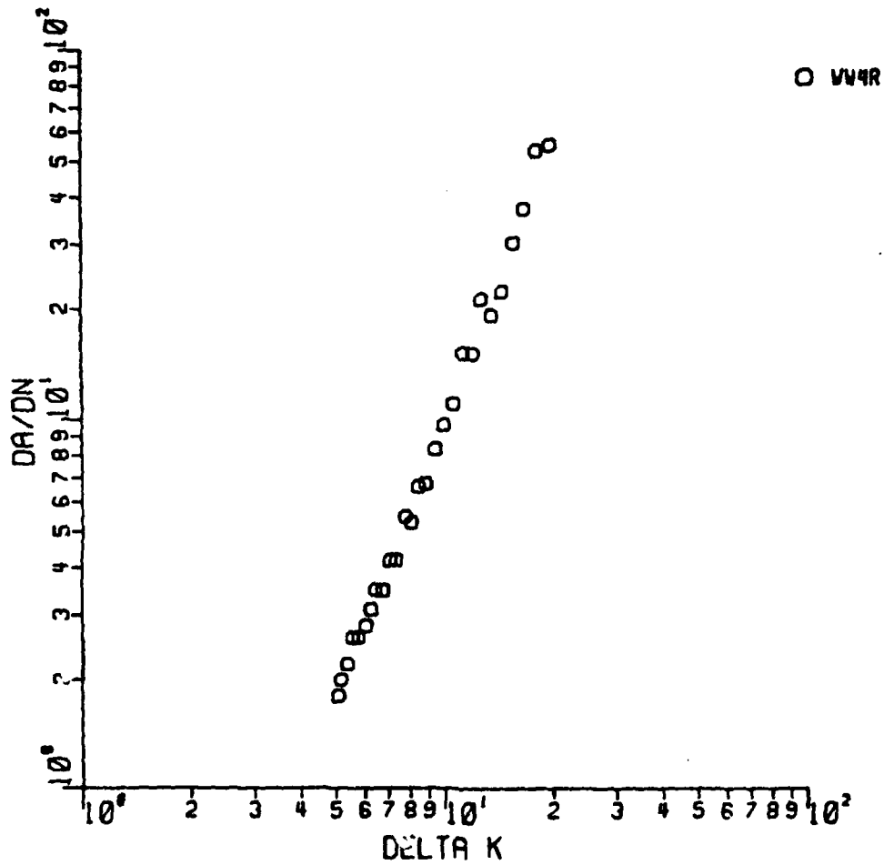
Figure 61. FCP Data for O11 Condition Using T-L CT Specimen.
