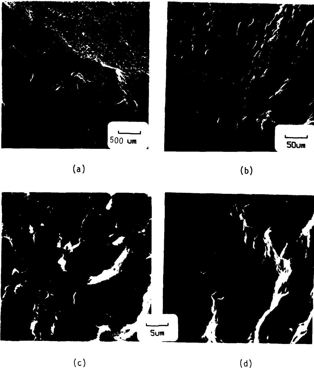
Figure 86. (a) Typical Initiation Site. (b) Higher Magnification of (a). (c) Close to the Initiation No Striations are Observed. (d) A Short Distance Away Striations are Observed. Condition 011, Sample TT4R-3, 0.042%, N_i = 3756 .
