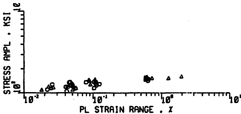
(b) o 38% upset n' = 0.076 ; \Delta 64% upset n' = 0.077 .
