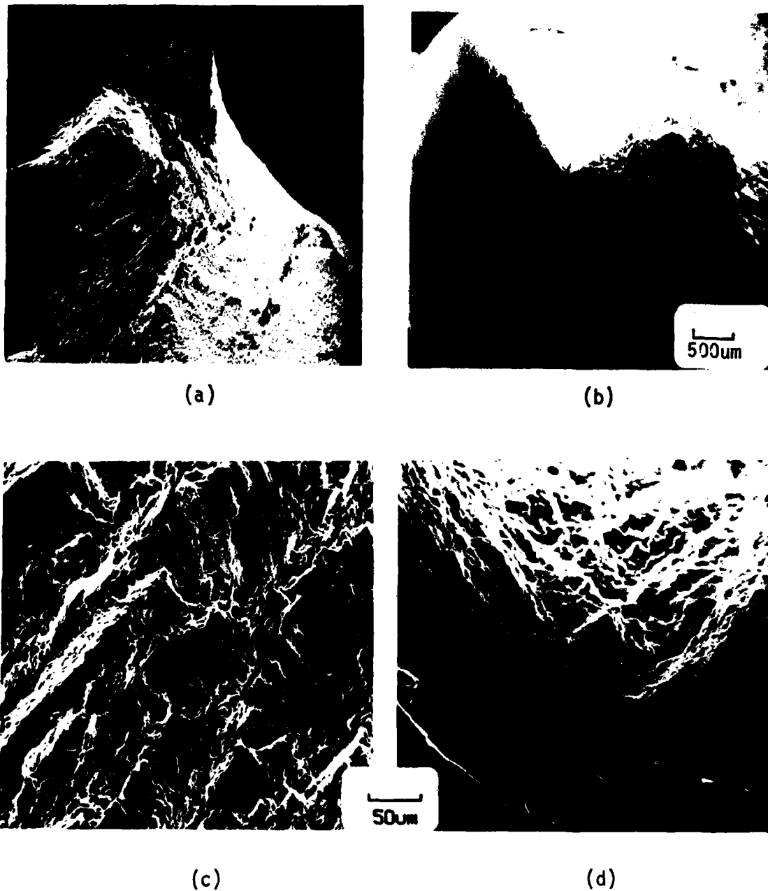
Figure 98. Three Regions of Initiation Can be Seen in (a) and (b). (c) and (d) are higher magnification SEM fractographs showing secondary cracking and smearing. Condition 001, Sample DD2R-2, 0.585%, N_j = 225 .
