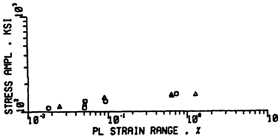
(f) o 100 n' = 0.92; Δ 101 n' = 0.069.
