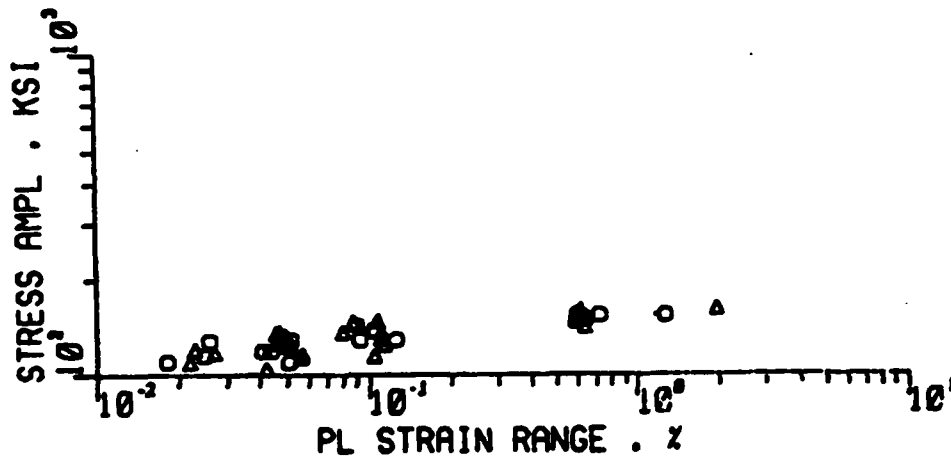
(c) o 0% Co n' = 0.076 ; Δ 0.4% Co n' = 0.077 .
