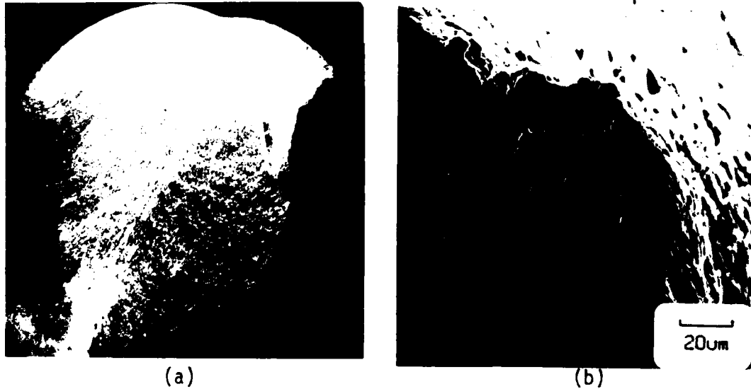
Figure 95. (a) Although Initiation Sites are more Difficult to Find in High Strain Tests, They are Present. (b) The initiation region is somewhat smaller but otherwise similar in appearance. Condition 101, Sample 23-3, 0.570%, N_i = 447 .
