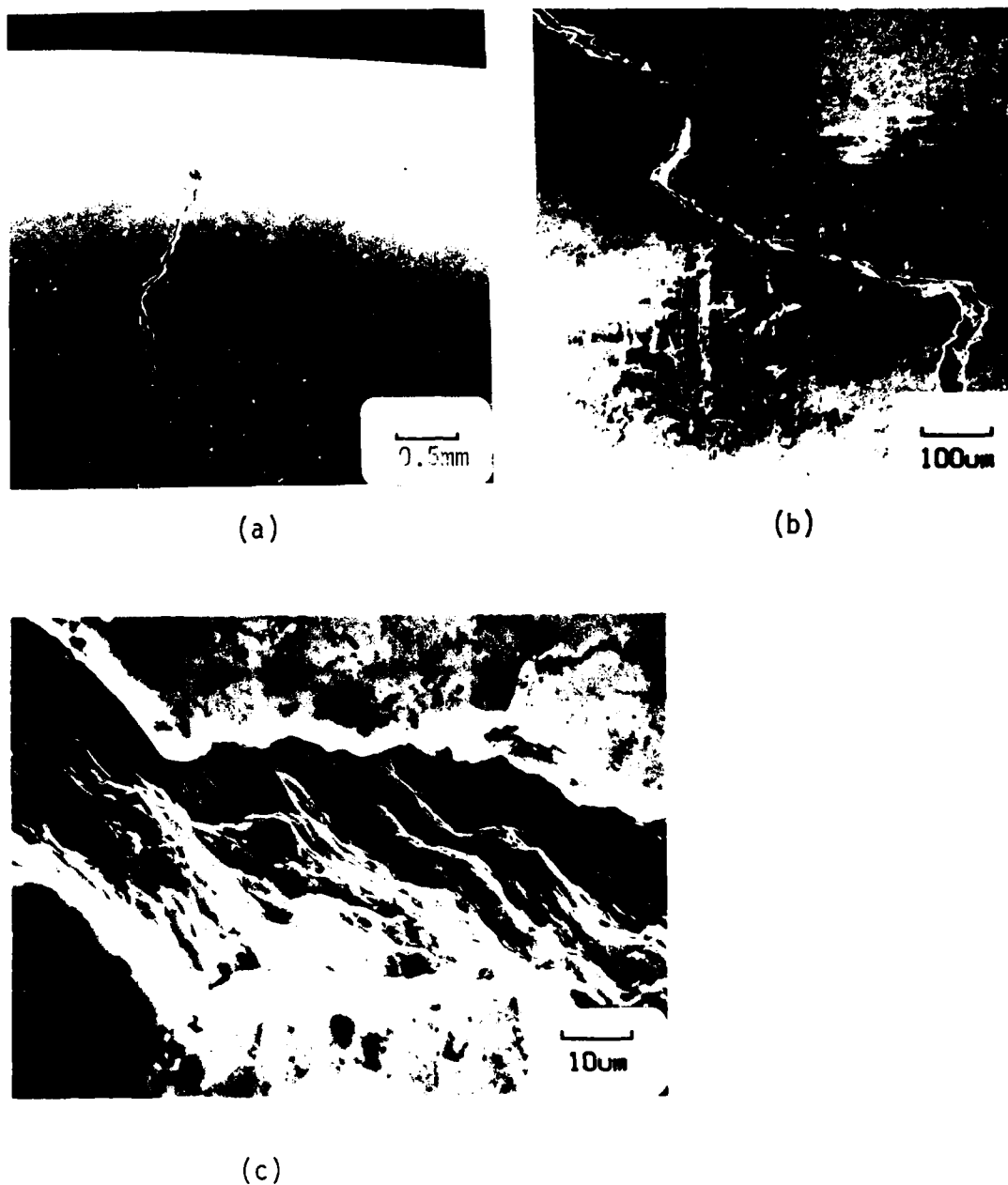
Figure 78. Typical Nature of Surface Cracking. (a) Overall view in 010. (b) Debris in crack believed at original initiation. (c) Crack away from initiation site with evidence of striations. Condition 010, Sample WW1-4, 0.024%, N_j = 1100 .
