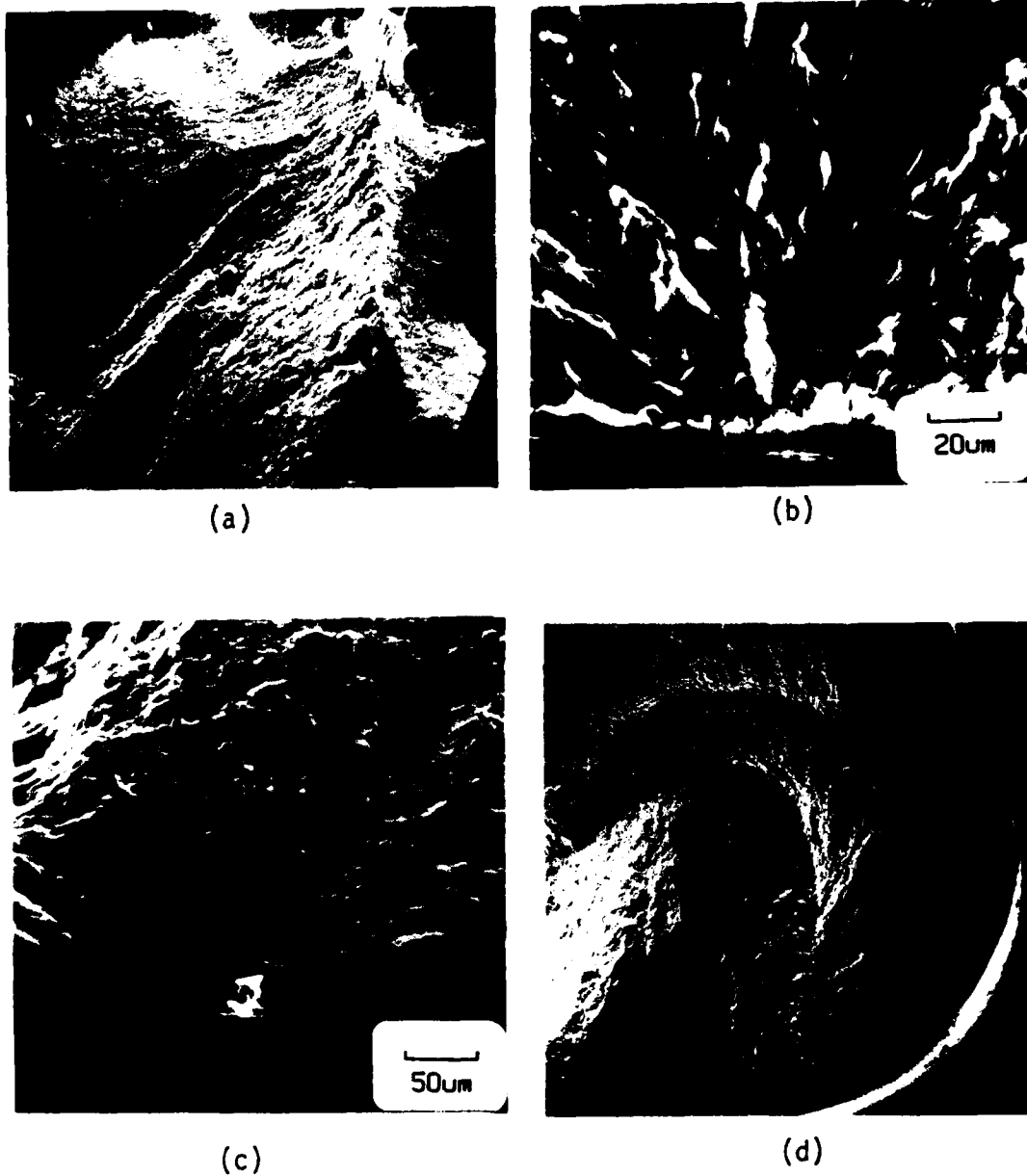
Figure 84. There are Three Kinds of Initiations Typically Found. (a) and (b) Initiations associated with a boundary weakness and surface instability; (c) surface particles, and (d) subsurface particles.
