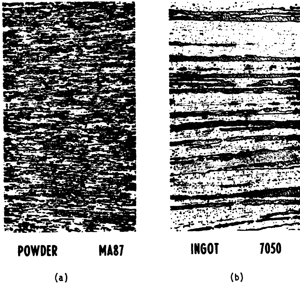
Figure 4. Microstructures of Al Die Forgings [64]. (a) Fine structure of P/M alloy MA87 and (b) coarse structure of I/M alloy 7050. Both microstructures were originally 100x.
