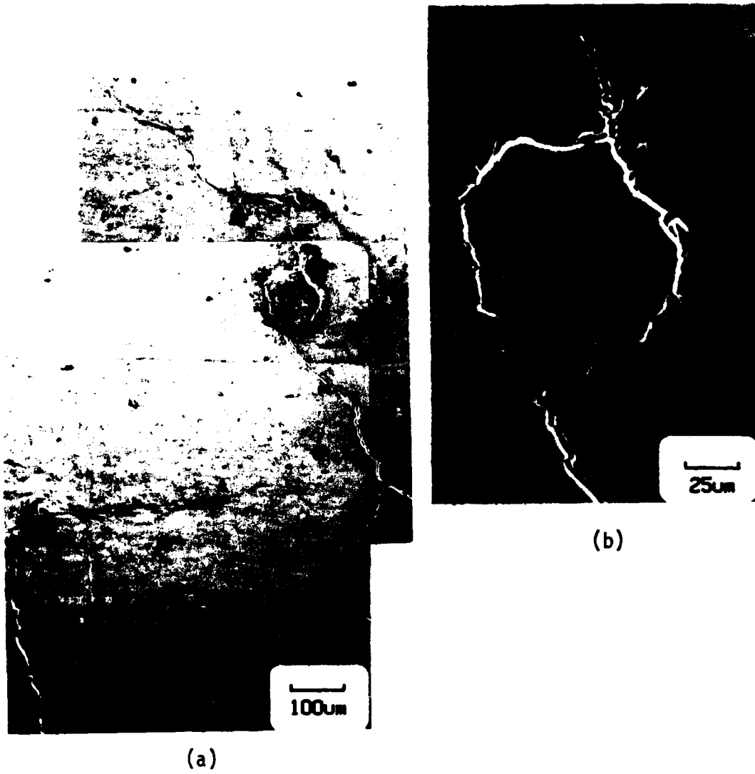
Figure 82. Surface Cracking in 110 Type Specimen. (a) Over-all view, (b) close-up of what is believed to be an original powder particle. Condition 110, Sample 19-4, 0.020% Ni = 2515.
