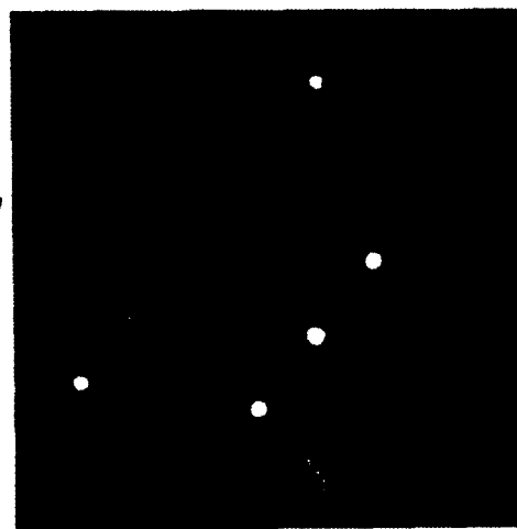
Figure 110. Typical Deformation Structure at Low Plastic Strain Amplitudes When Slip Bands are not Observed. (a) the active plane, (\bar{1}11) , is edge on; (b) the same grain tilted and rotated near a [211] zone axis with (\bar{1}11) approximately 2^\circ off edge. (c) and (d) are the diffraction patterns for (a) and (b) respectively. Sample TT3-2, \Delta\epsilon_p = 0.049\% , N_i = 3921 , Condition 010.
