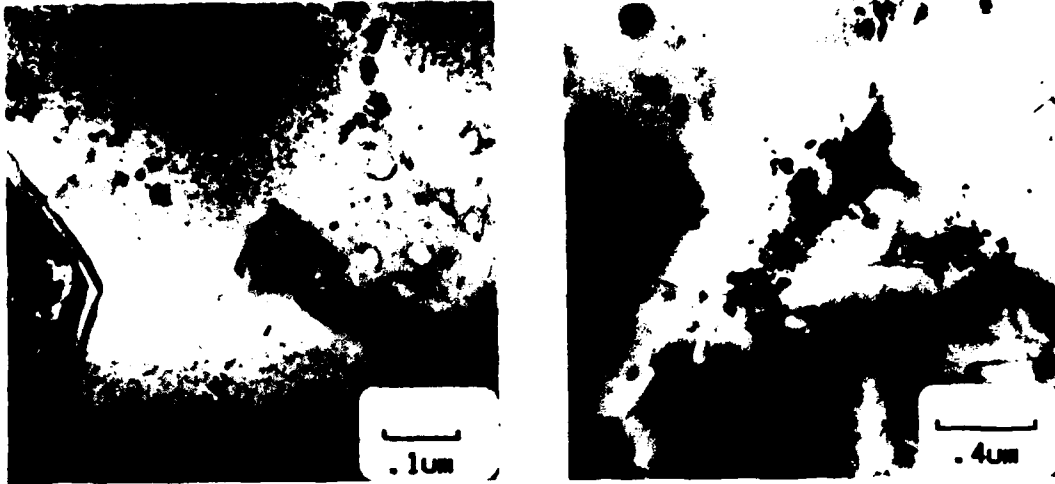
Figure 42. Individual Oxide Arrays in CT91 Forgings. (a) T-L plane of a 38% upset forging with 0% Co and stress relieved; (b) S-L plane of a 64% upset forging with 0.4% Co and not stress relieved.
