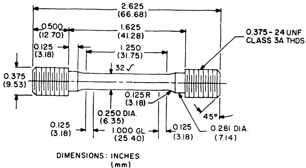
Figure 2. Tensile Specimen Geometry.
