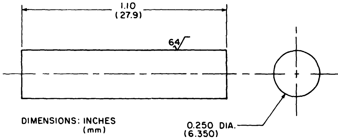
Figure 4. Pin-Shear Specimen Geometry.
