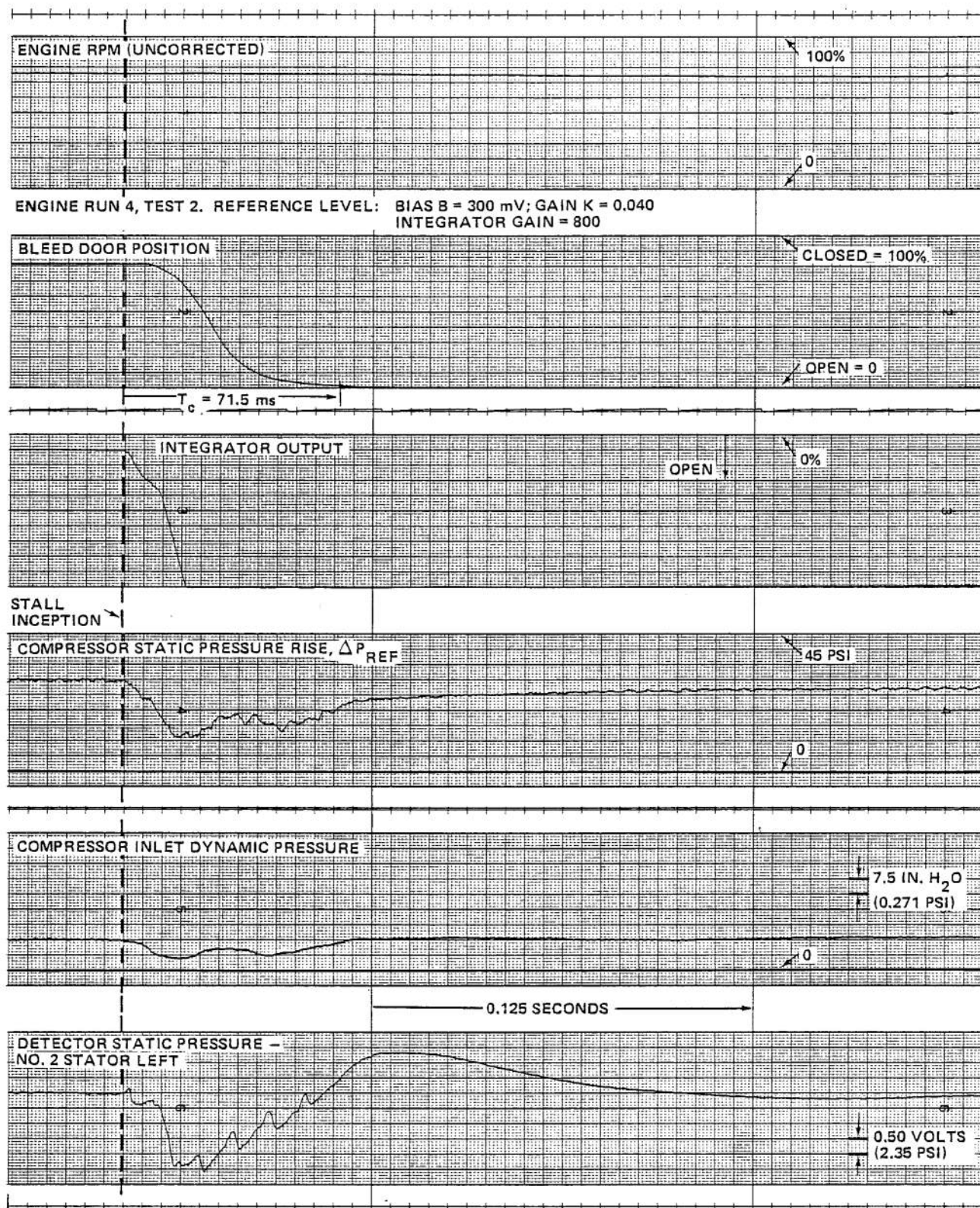
Figure 35 J-85 COMPRESSOR RESPONSE TO ROTATING STALL AT NOMINAL ENGINE SPEED OF 75% (EXPANDED TIME SCALE)
