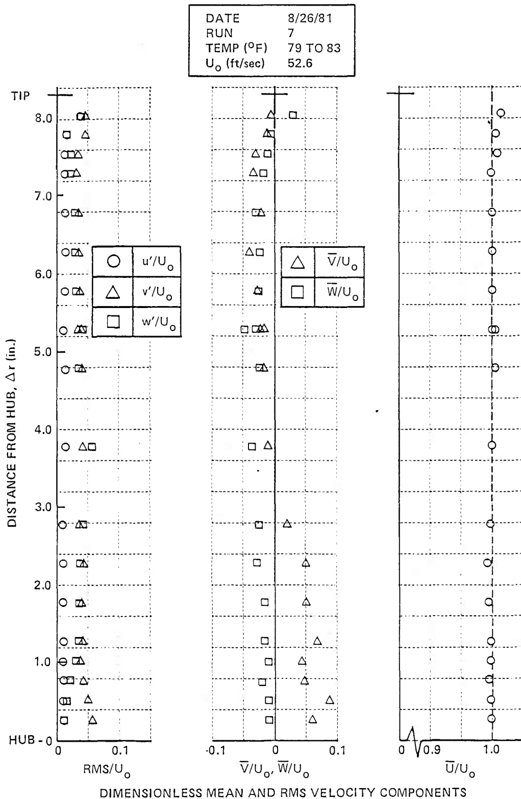
Figure 4 (Cont.) RADIAL DISTRIBUTIONS OF VELOCITY COMPONENTS FAR UPSTREAM OF ROTOR
