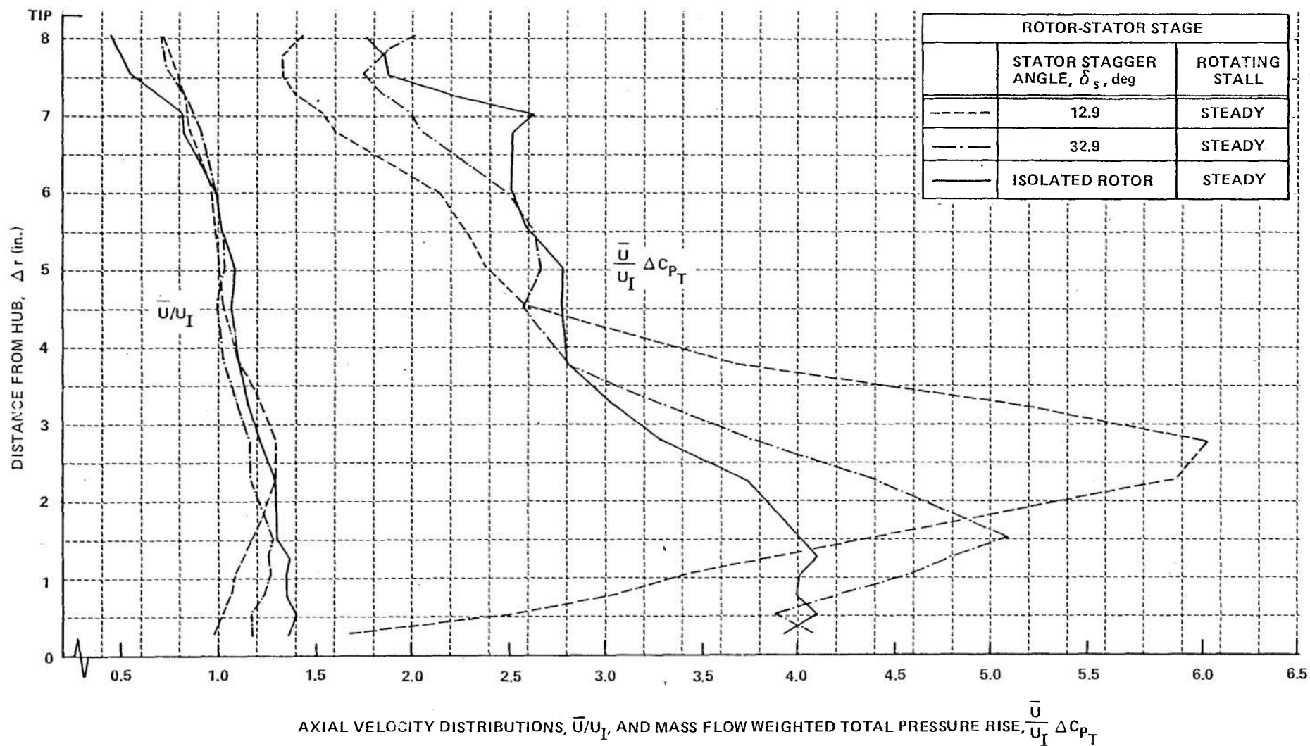
Figure 15 (Cont.) RADIAL DISTRIBUTIONS OF AXIAL VELOCITY AND MASS FLOW WEIGHTED TOTAL PRESSURE RISE DOWNSTREAM OF ISOLATED ROTOR AND THE SAME ROTOR IN A ROTOR-STATOR STAGE
