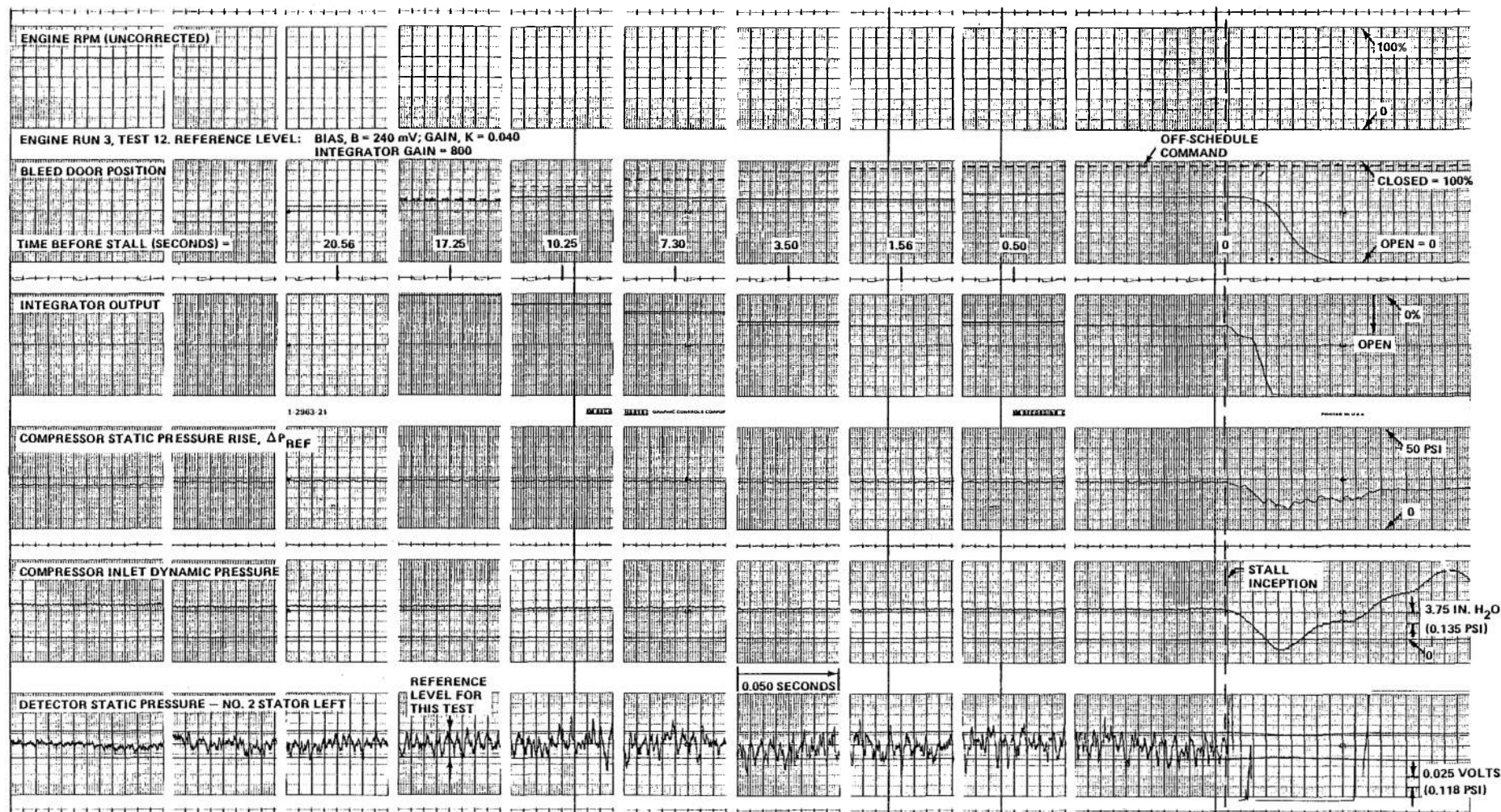
Figure 38 J-85 COMPRESSOR PARAMETERS PRIOR TO ROTATING STALL. STALL CONTROL ADJUSTED TO ALMOST PREVENT STALL. CORRECTED ENGINE SPEED AT STALL INCEPTION (N/N^* \sqrt{\theta}) = 70.5\%
