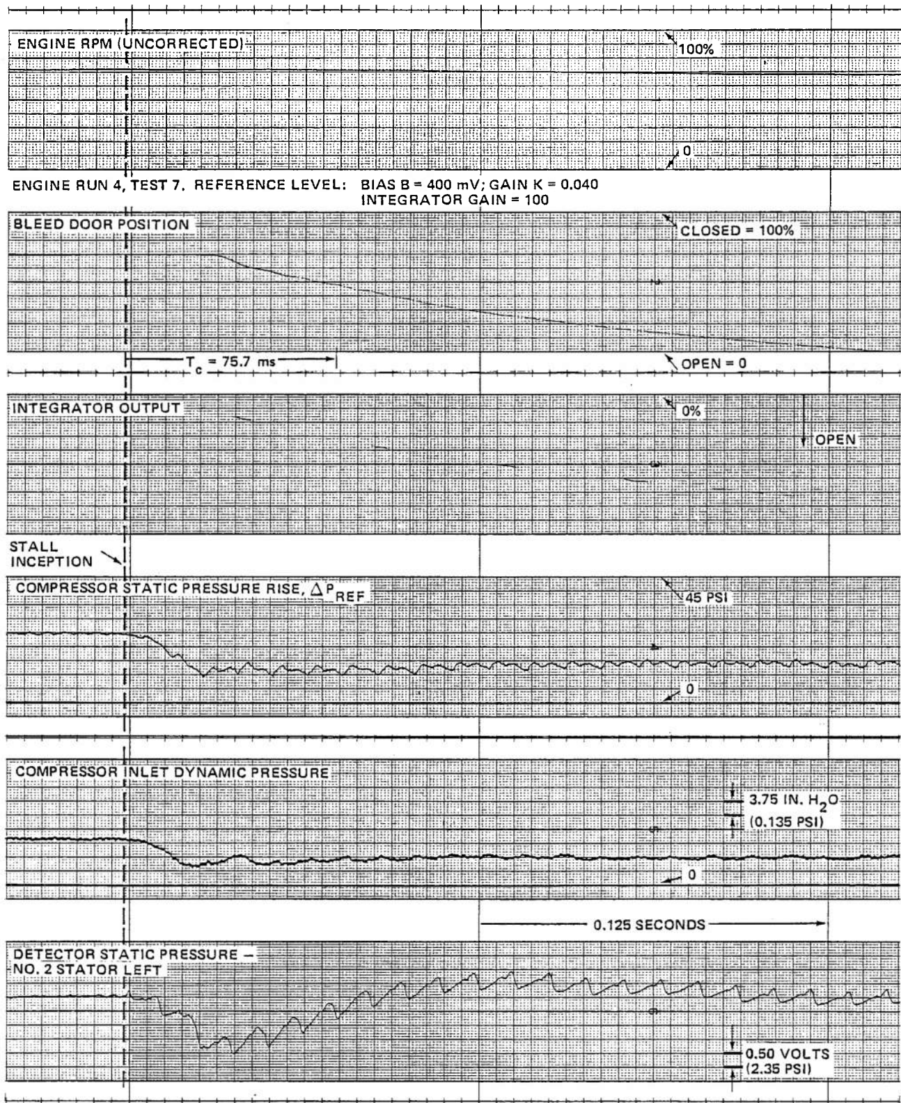
Figure 34 (Cont.) J-85 COMPRESSOR RESPONSE TO ROTATING STALL AT NOMINAL ENGINE SPEED OF 70% (EXPANDED TIME SCALE) d. INTEGRATOR GAIN = 100; CORRECTED ENGINE SPEED AT STALL INCEPTION, (N/N^* \sqrt{\theta}) = 71.1\%
