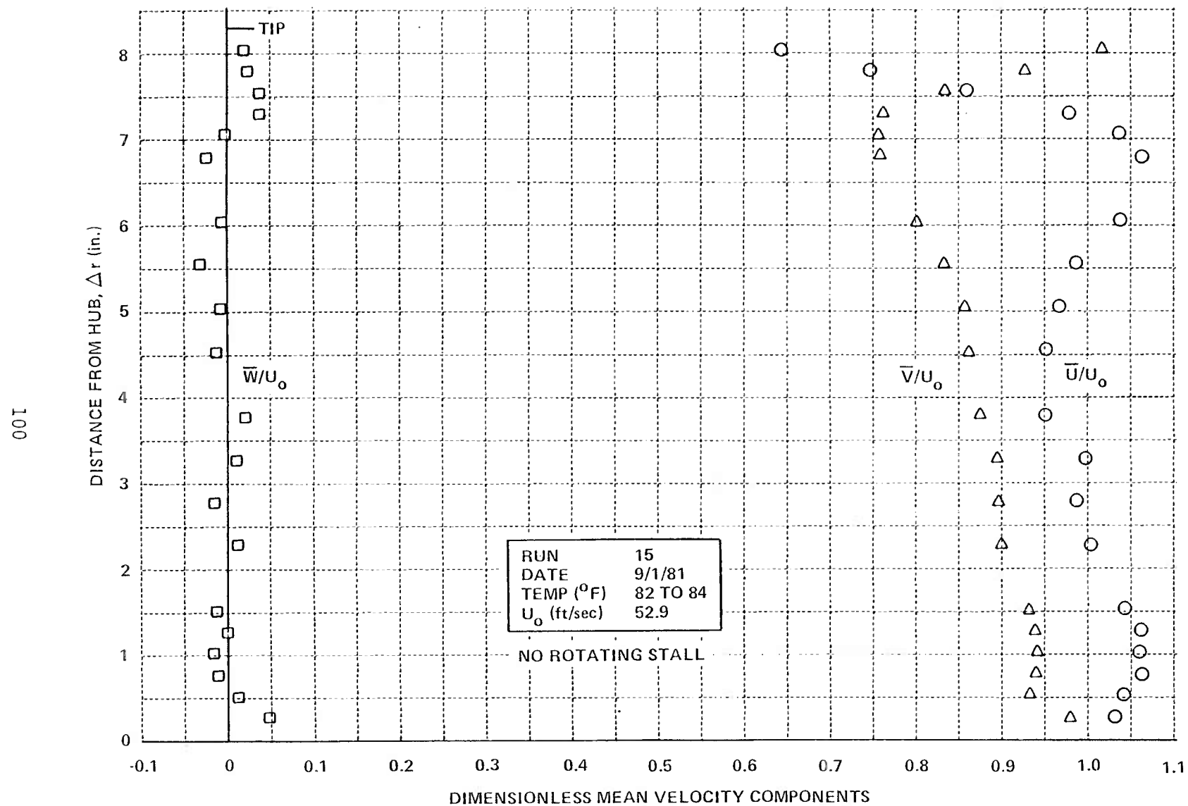
Figure 5 (Cont.) RADIAL DISTRIBUTIONS OF MEAN VELOCITY COMPONENTS DOWNSTREAM OF ISOLATED ROTOR d. ROTOR RPM = 900
