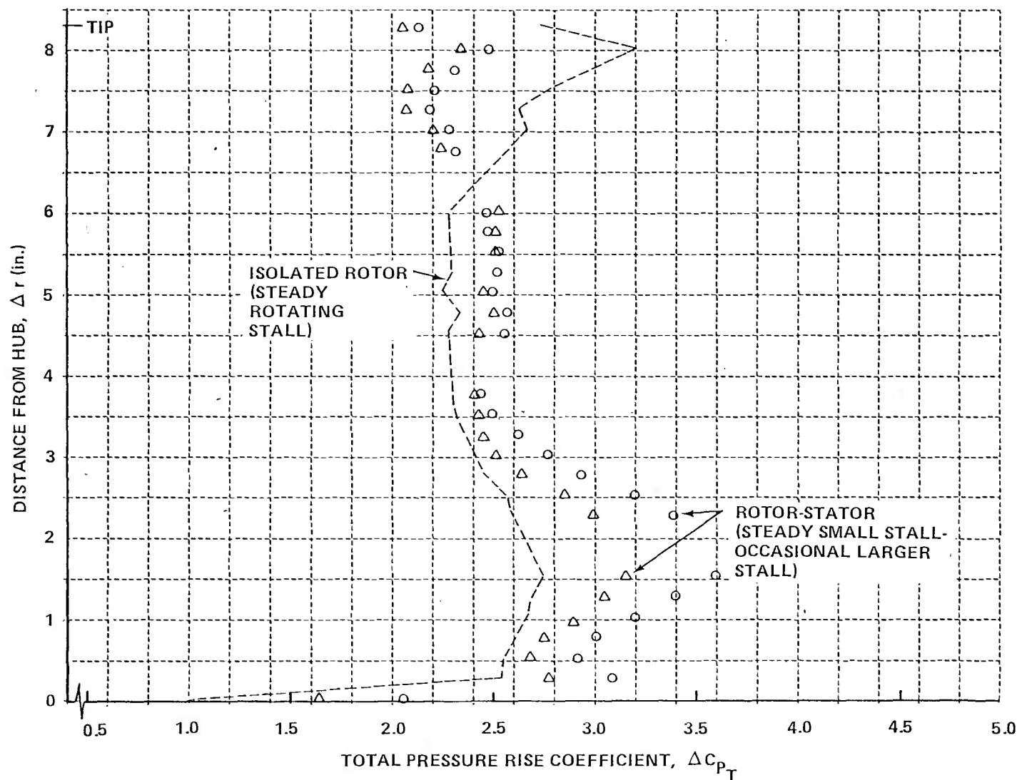
Figure 14 (Cont.) RADIAL DISTRIBUTIONS OF TOTAL PRESSURE COEFFICIENT IMMEDIATELY DOWNSTREAM OF ISOLATED ROTOR AND THE SAME ROTOR IN ROTOR-STATOR STAGE. STATOR STAGGER ANGLE AT MEAN RADIUS, \delta_s = 32.9 deg.
