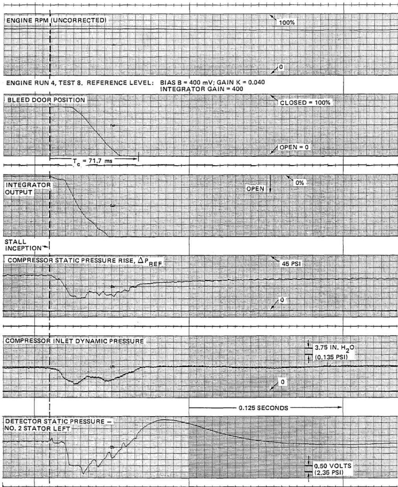
Figure 35 (Cont.) J-85 COMPRESSOR RESPONSE TO ROTATING STALL AT NOMINAL ENGINE SPEED OF 75% (EXPANDED TIME SCALE) b) INTEGRATOR GAIN = 400; CORRECTED ENGINE SPEED AT STALL INCEPTION, (N/N * \sqrt{\theta}) = 75.0\%
