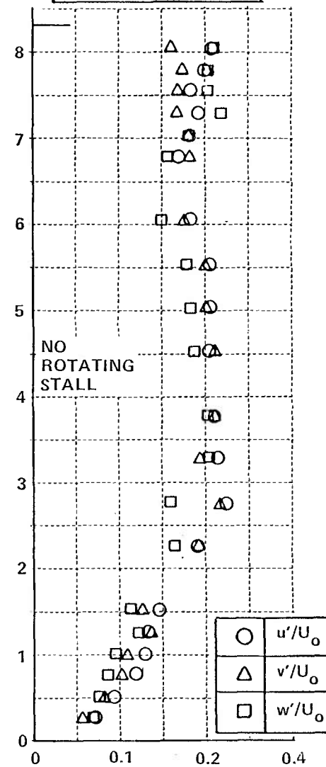
Figure 6 (Cont.) DIMENSIONLESS RMS VELOCITY COMPONENTS DOWNSTREAM OF ISOLATED ROTOR b. ROTOR RPM = 800, 850, 900
