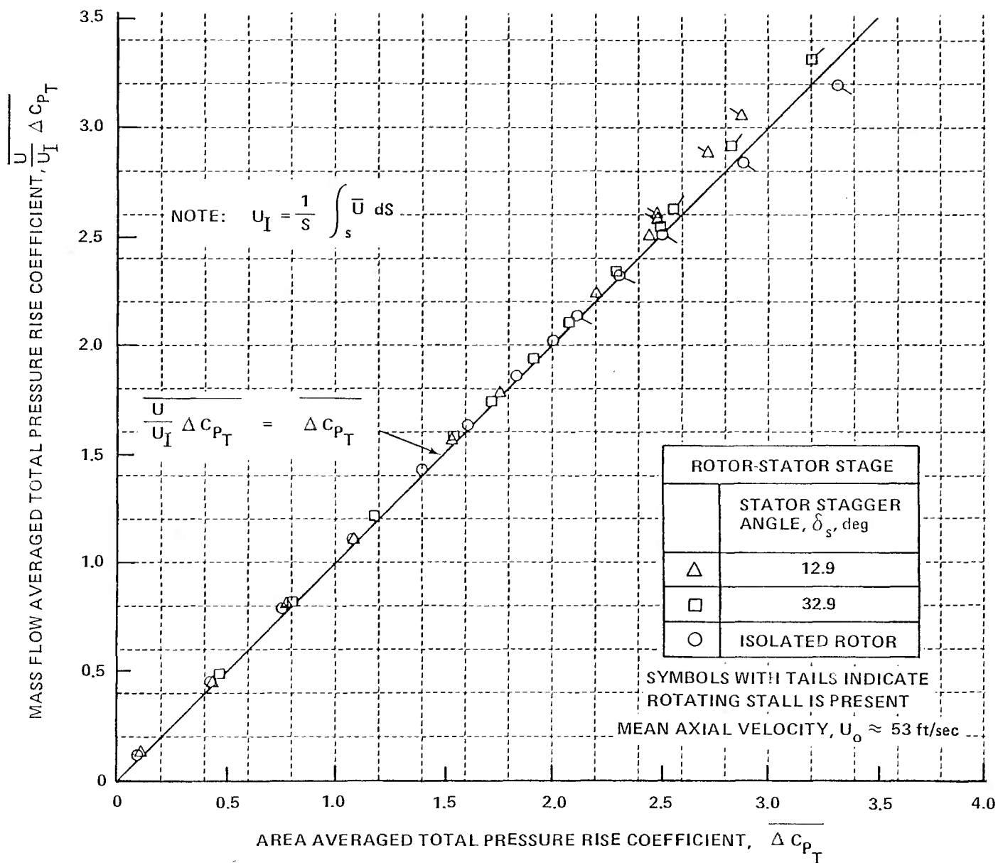
Figure 17 COMPARISON OF AREA AVERAGED AND MASS-FLOW AVERAGED TOTAL PRESSURE RISE ACROSS ROTOR
