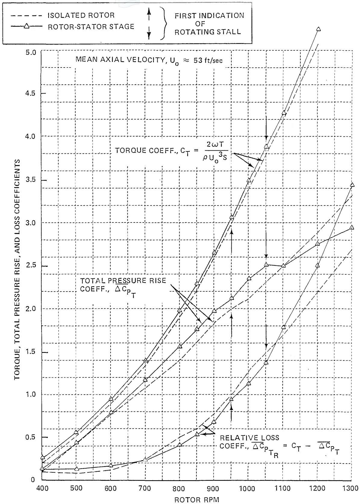
Figure 19 TORQUE COEFFICIENT AND AREA-AVERAGED TOTAL PRESSURE RISE, AND LOSS COEFFICIENTS FOR ROTOR IN LOW HUB/TIP RATIO ROTOR-STATOR STAGE. STATOR STAGGER ANGLE AT MEAN RADIUS, \delta_s = 22.9 deg.
