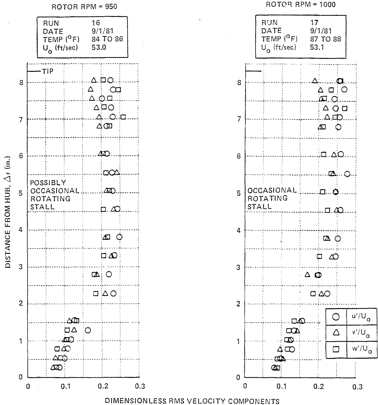
Figure 6 (Cont.) DIMENSIONLESS RMS VELOCITY COMPONENTS DOWNSTREAM OF ISOLATED ROTOR
