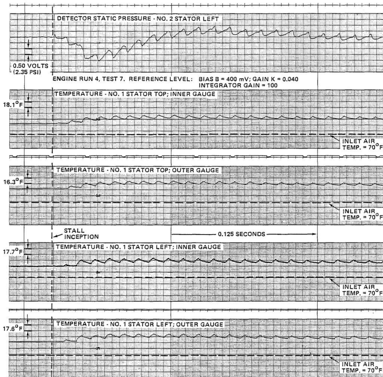
Figure 40 UNSTEADY TEMPERATURE MEASUREMENTS IN J-85 COMPRESSOR DURING ROTATING STALL (EXPANDED TIME SCALE) a. CORRECTED ENGINE SPEED AT STALL INCEPTION, (N/N^* \sqrt{\theta}) = 71.1\%
