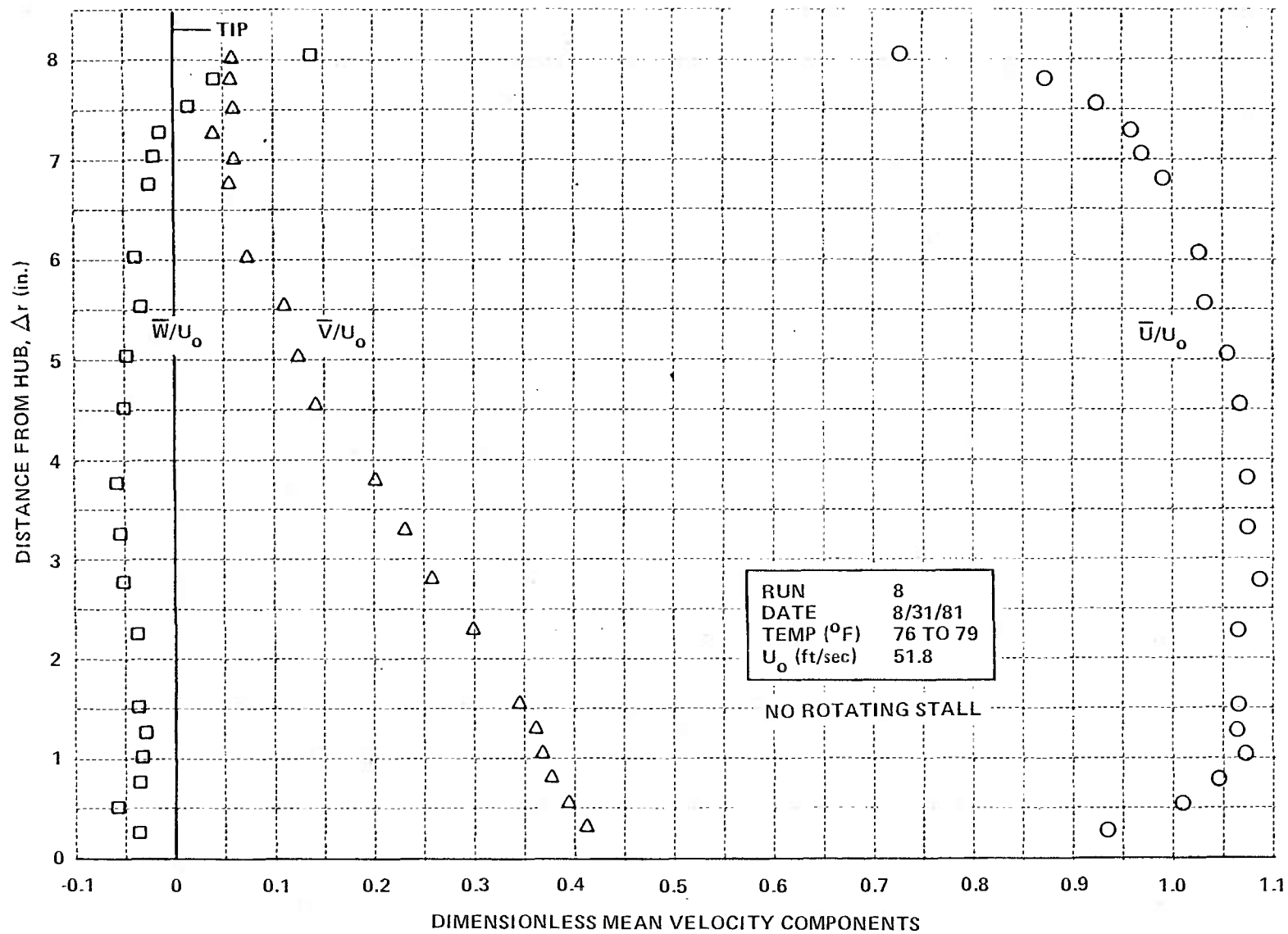
Figure 5 RADIAL DISTRIBUTIONS OF MEAN VELOCITY COMPONENTS DOWNSTREAM OF ISOLATED ROTOR a. ROTOR RPM = 400
