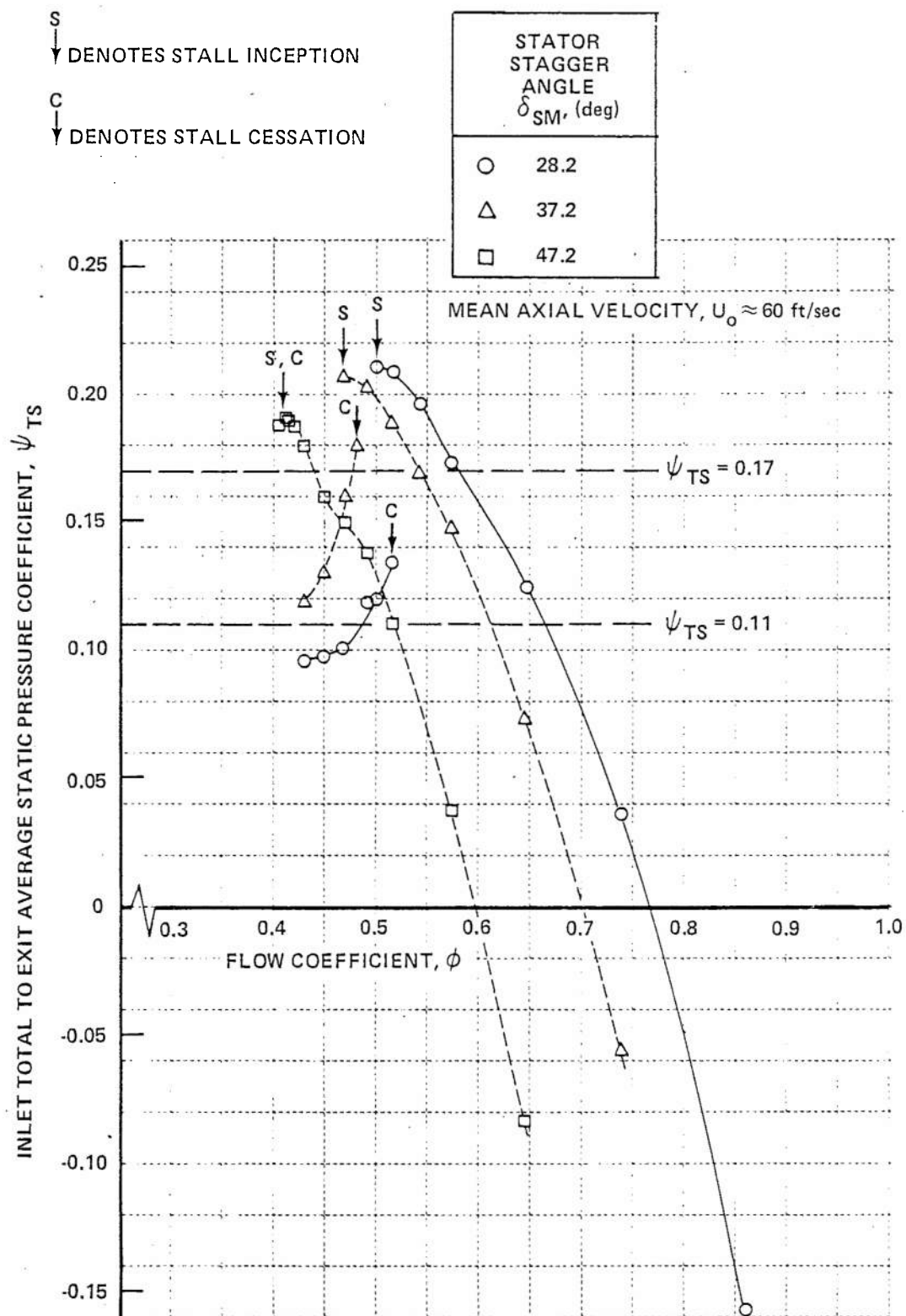
Figure 26 INLET TOTAL TO EXIT AVERAGE STATIC PRESSURE RISE PERFORMANCE OF HIGH HUB-TO-TIP RATIO STAGE IN ANNULAR CASCADE
