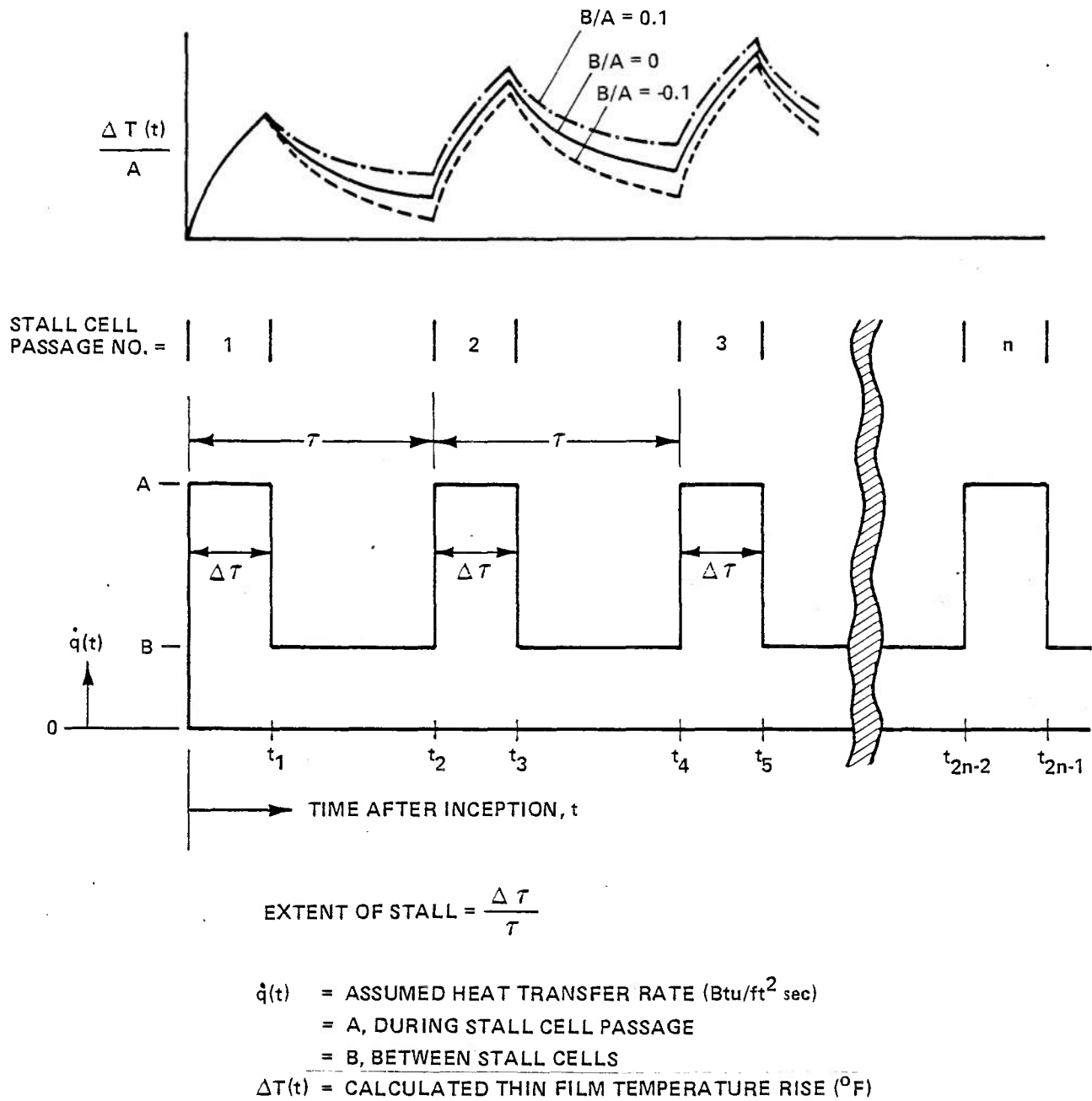
Figure 42 ASSUMED MODEL FOR HEAT TRANSFER RATE DURING ROTATING STALL
