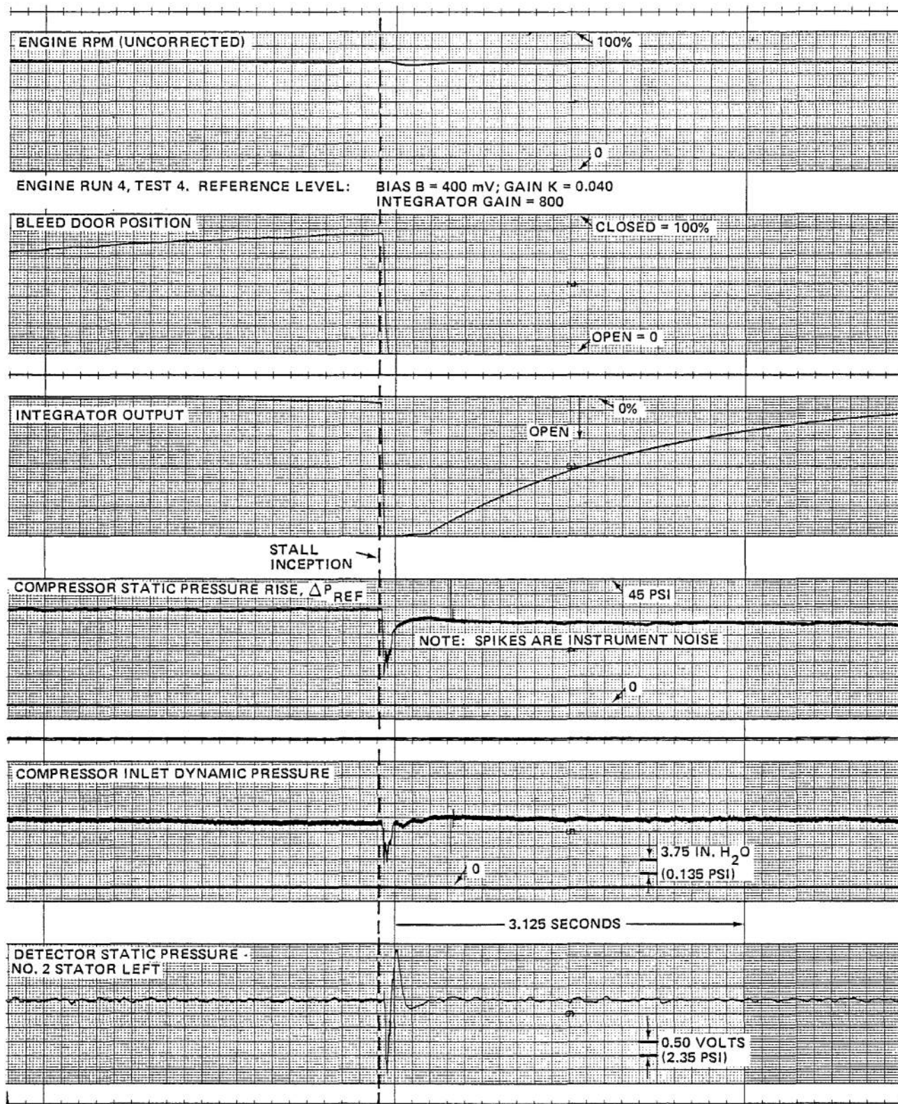
Figure 33 J-85 COMPRESSOR RESPONSE TO ROTATING STALL AT NOMINAL ENGINE SPEED OF 78%
