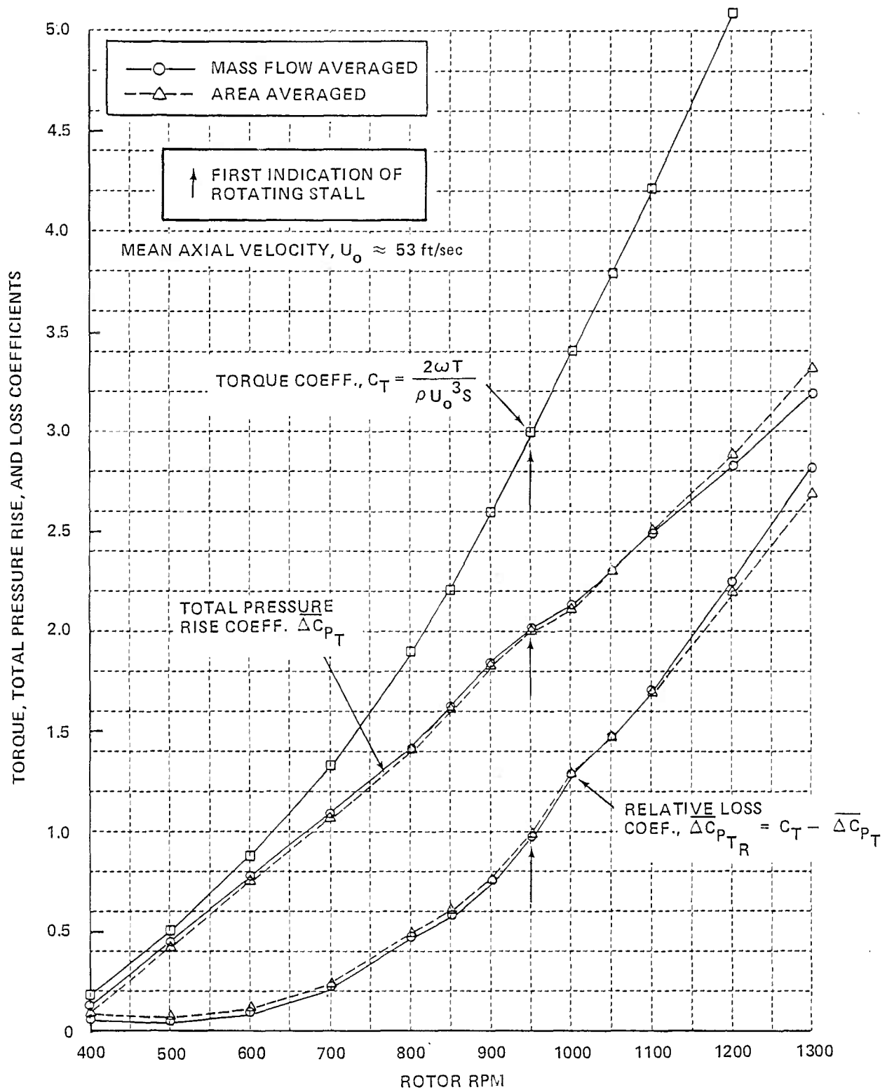
Figure 11 AVERAGED TORQUE, TOTAL PRESSURE RISE, AND LOSS COEFFICIENTS ON LOW HUB-TIP RATIO ISOLATED ROTOR
