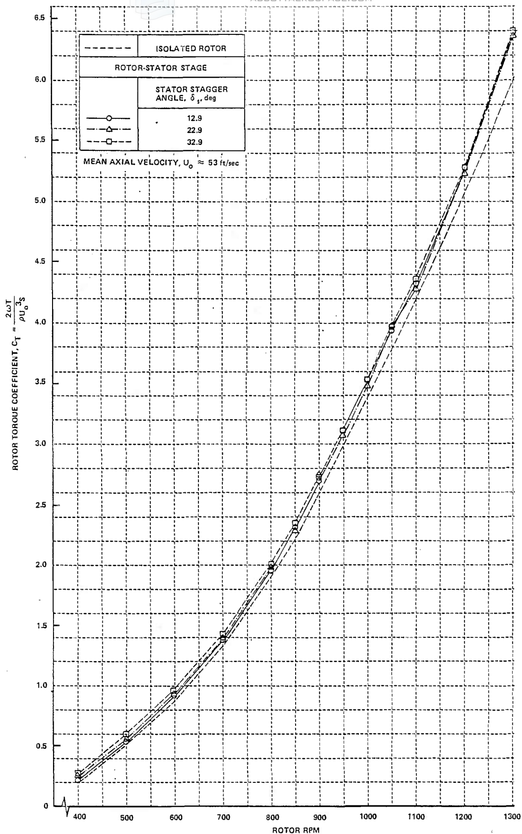
Figure 12 COMPARISON OF ROTOR TORQUE COEFFICIENTS MEASURED ON ISOLATED ROTOR AND ON THE SAME ROTOR IN A ROTOR-STATOR STAGE
