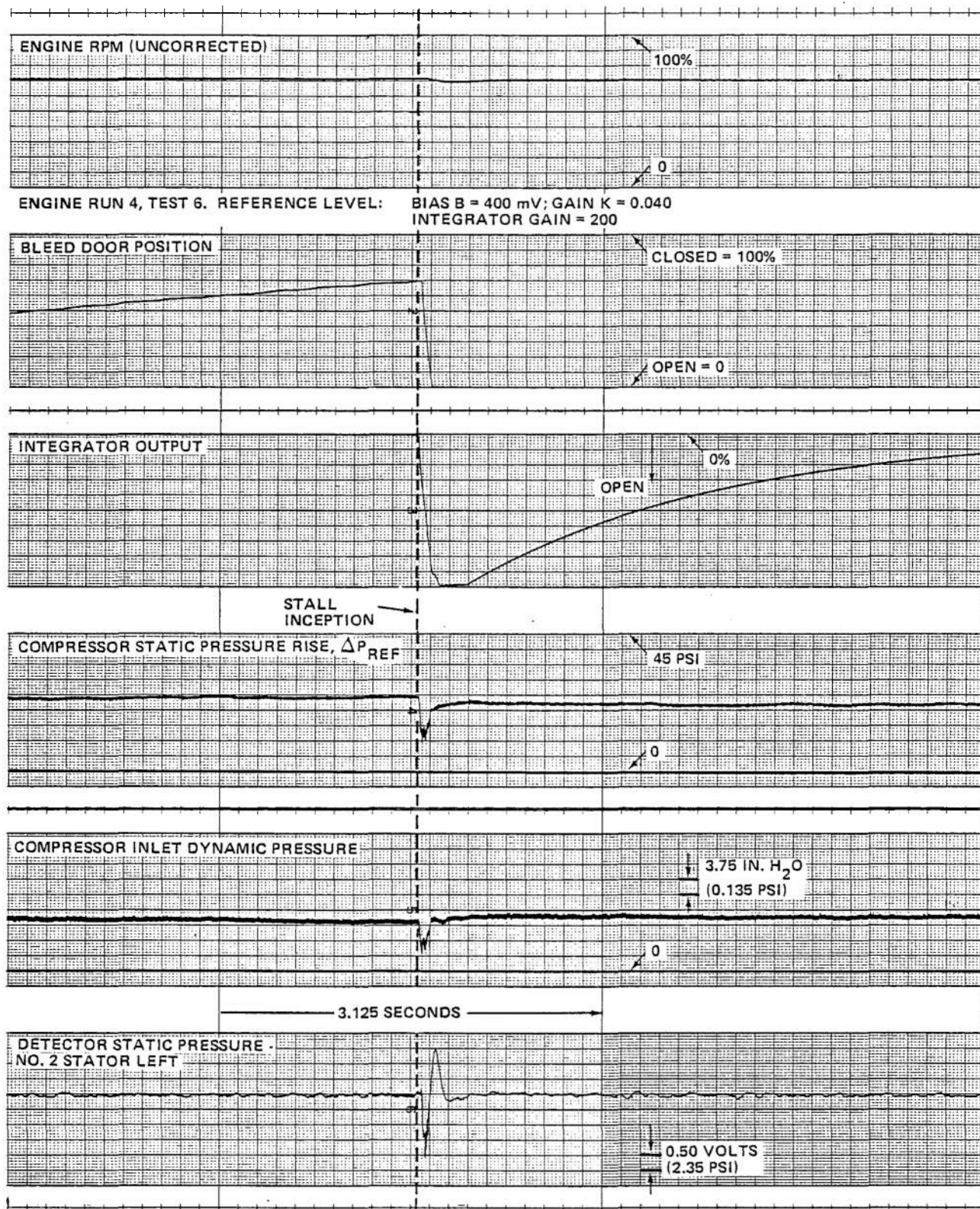
Figure 31 (Cont.) J-85 COMPRESSOR RESPONSE TO ROTATING STALL AT NOMINAL ENGINE SPEED OF 70%
