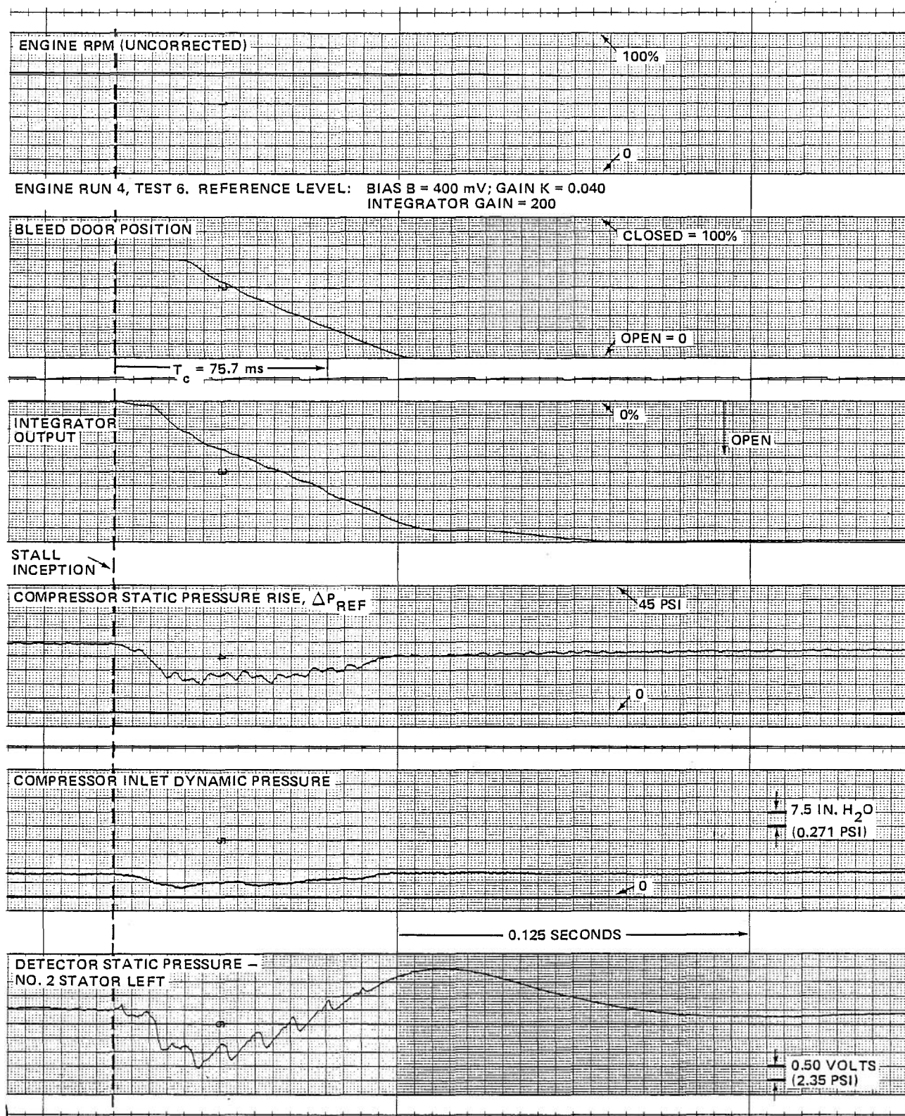
Figure 34 (Cont.) J-85 COMPRESSOR RESPONSE TO ROTATING STALL AT NOMINAL ENGINE SPEED OF 70% (EXPANDED TIME SCALE) c. INTEGRATOR GAIN = 200; CORRECTED ENGINE SPEED AT STALL INCEPTION, (N/N^* \sqrt{\theta}) = 71.1\%
