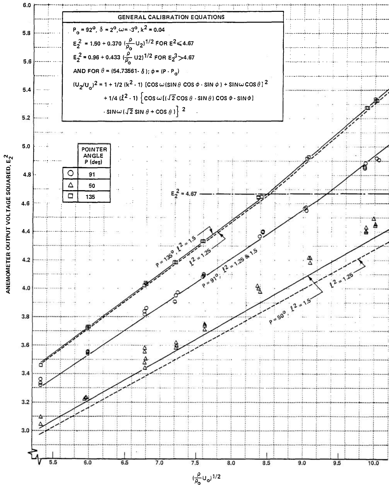
Figure A-5 (Cont.) TRIPLE PROBE VELOCITY CALIBRATION
