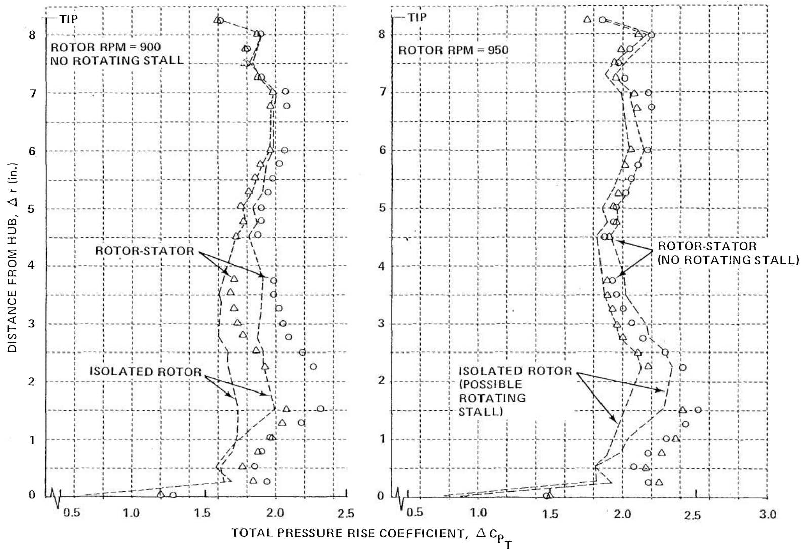
Figure 14 (Cont.) RADIAL DISTRIBUTIONS OF TOTAL PRESSURE COEFFICIENT IMMEDIATELY DOWNSTREAM OF ISOLATED ROTOR AND THE SAME ROTOR IN ROTOR-STATOR STAGE. STATOR STAGGER ANGLE AT MEAN RADIUS, \delta_s = 32.9 deg.
