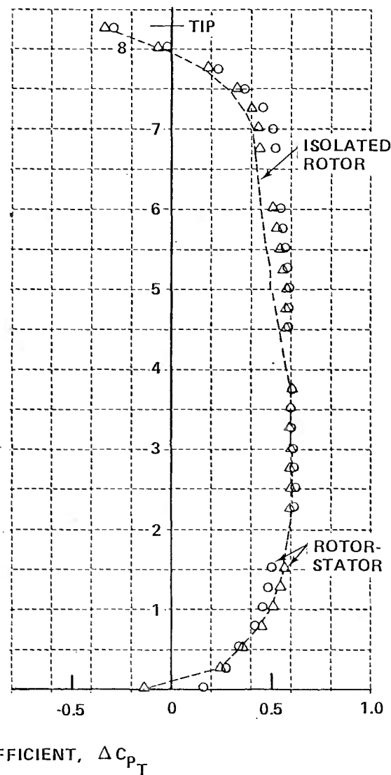
Figure 14 RADIAL DISTRIBUTIONS OF TOTAL PRESSURE COEFFICIENT IMMEDIATELY DOWNSTREAM OF ISOLATED ROTOR AND THE SAME ROTOR IN ROTOR-STATOR STAGE. STATOR STAGGER ANGLE AT MEAN RADIUS, \delta_s = 32.9 deg.
