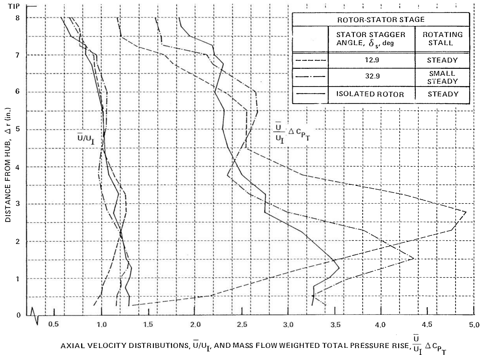
Figure 15 (Cont.) RADIAL DISTRIBUTIONS OF AXIAL VELOCITY AND MASS FLOW WEIGHTED TOTAL PRESSURE RISE DOWNSTREAM OF ISOLATED ROTOR AND THE SAME ROTOR IN A ROTOR-STATOR STAGE. (g) ROTOR RPM = 1100
