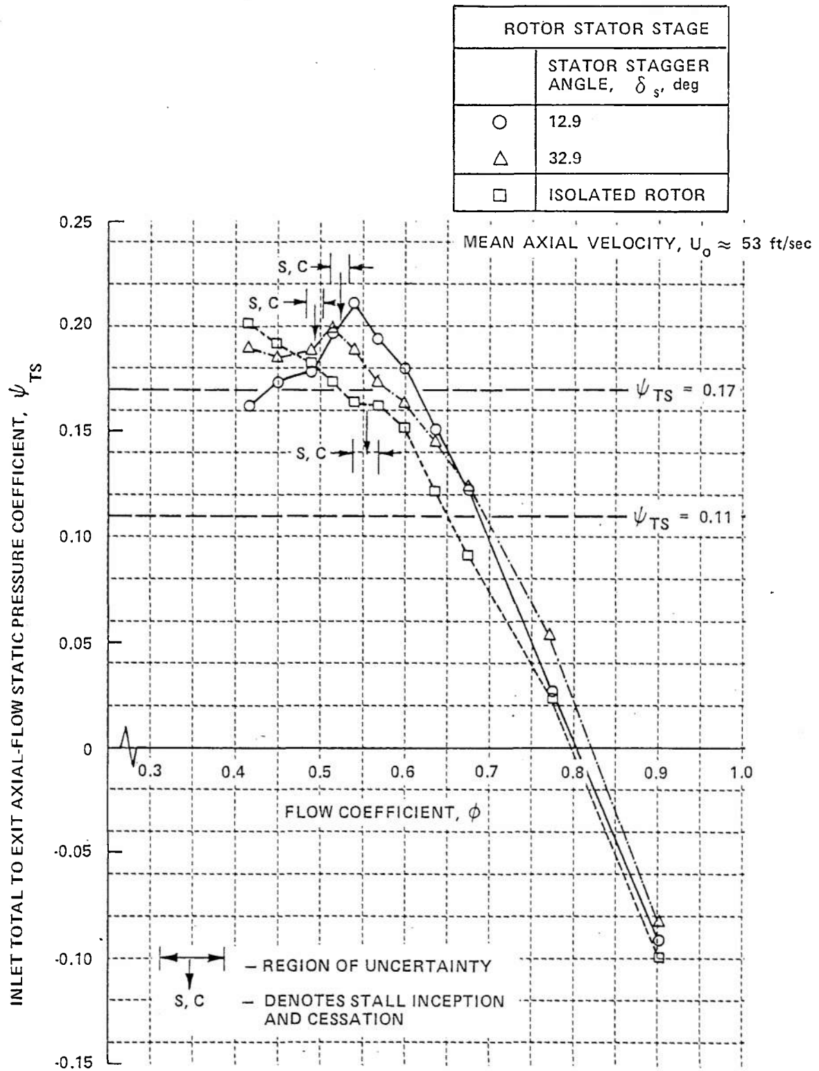
Figure 28 INLET TOTAL TO EXIT AXIAL-FLOW STATIC PRESSURE RISE PERFORMANCE OF LOW HUB-TO-TIP RATIO ISOLATED ROTOR AND THE SAME ROTOR IN A ROTOR-STATOR STAGE
