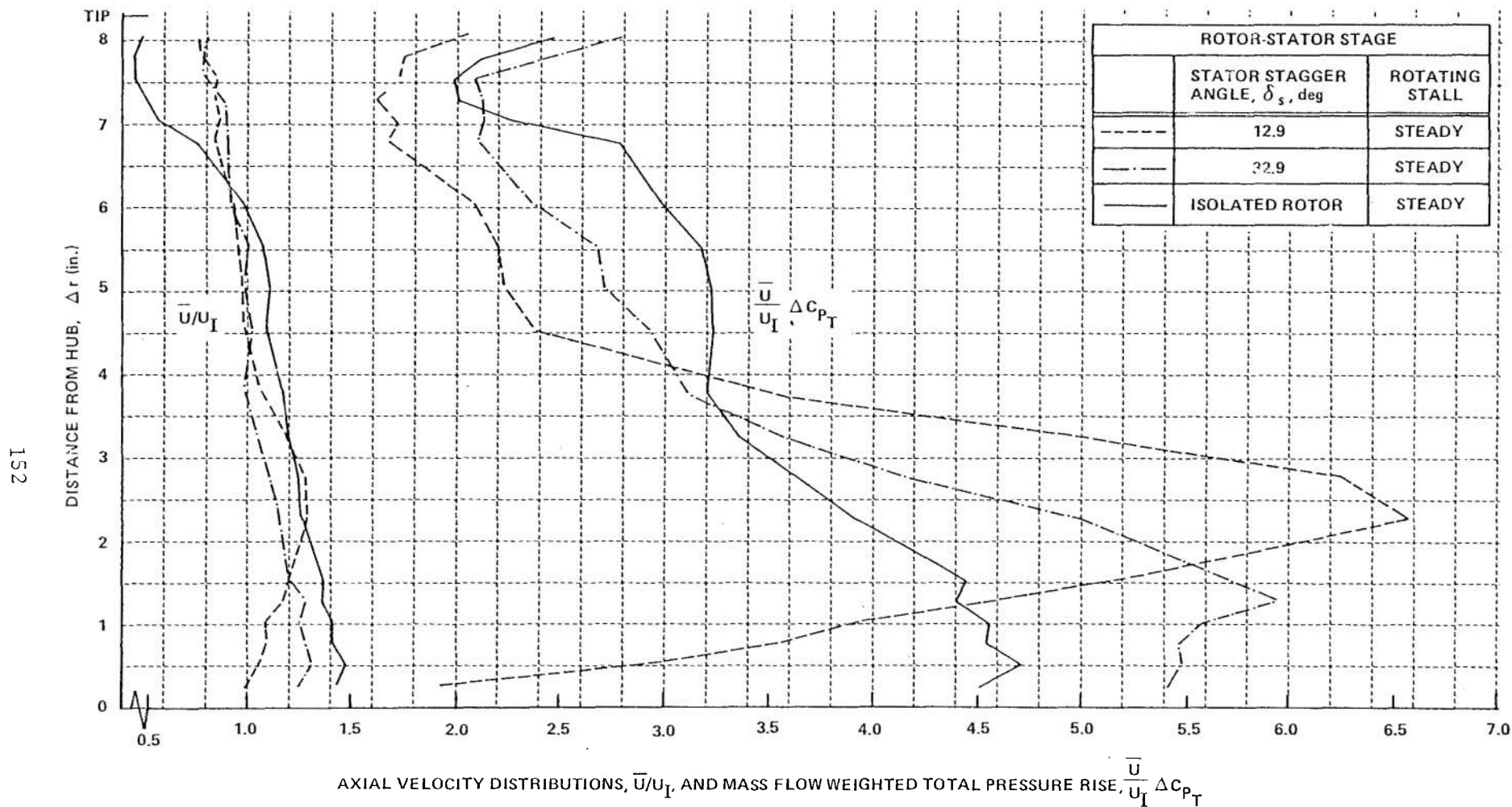
Figure 15 (Cont.) RADIAL DISTRIBUTIONS OF AXIAL VELOCITY AND MASS FLOW WEIGHTED TOTAL PRESSURE RISE DOWNSTREAM OF ISOLATED ROTOR AND THE SAME ROTOR IN A ROTOR-STATOR STAGE
