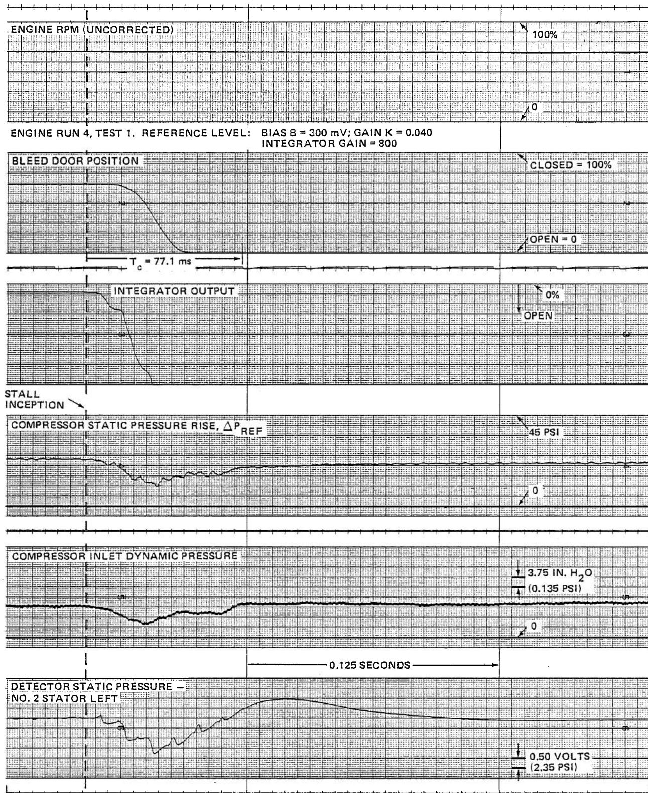
Figure 34 J-85 COMPRESSOR RESPONSE TO ROTATING STALL AT NOMINAL ENGINE SPEED OF 70% (EXPANDED TIME SCALE) a. INTEGRATOR GAIN = 800; CORRECTED ENGINE SPEED AT STALL INCEPTION, (N/N * \sqrt{\theta}) = 69.8\%
