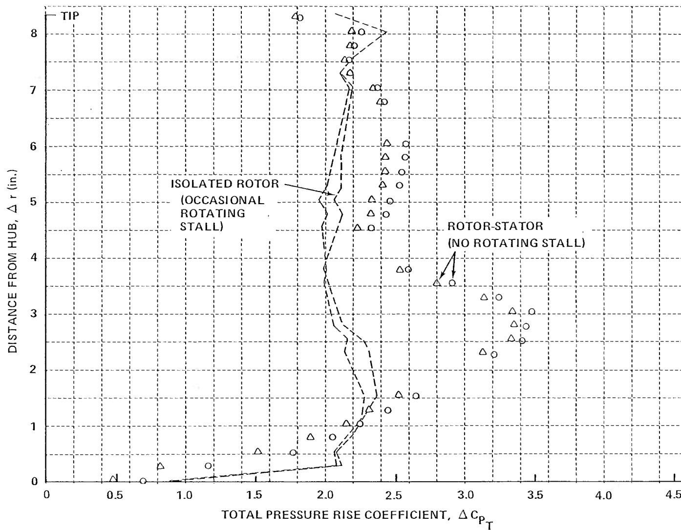
Figure 13 (Cont.) RADIAL DISTRIBUTIONS OF TOTAL PRESSURE COEFFICIENT IMMEDIATELY DOWNSTREAM OF ISOLATED ROTOR AND THE SAME ROTOR IN ROTOR-STATOR STAGE. STATOR STAGGER ANGLE AT MEAN RADIUS, \delta_s = 12.9 deg.
