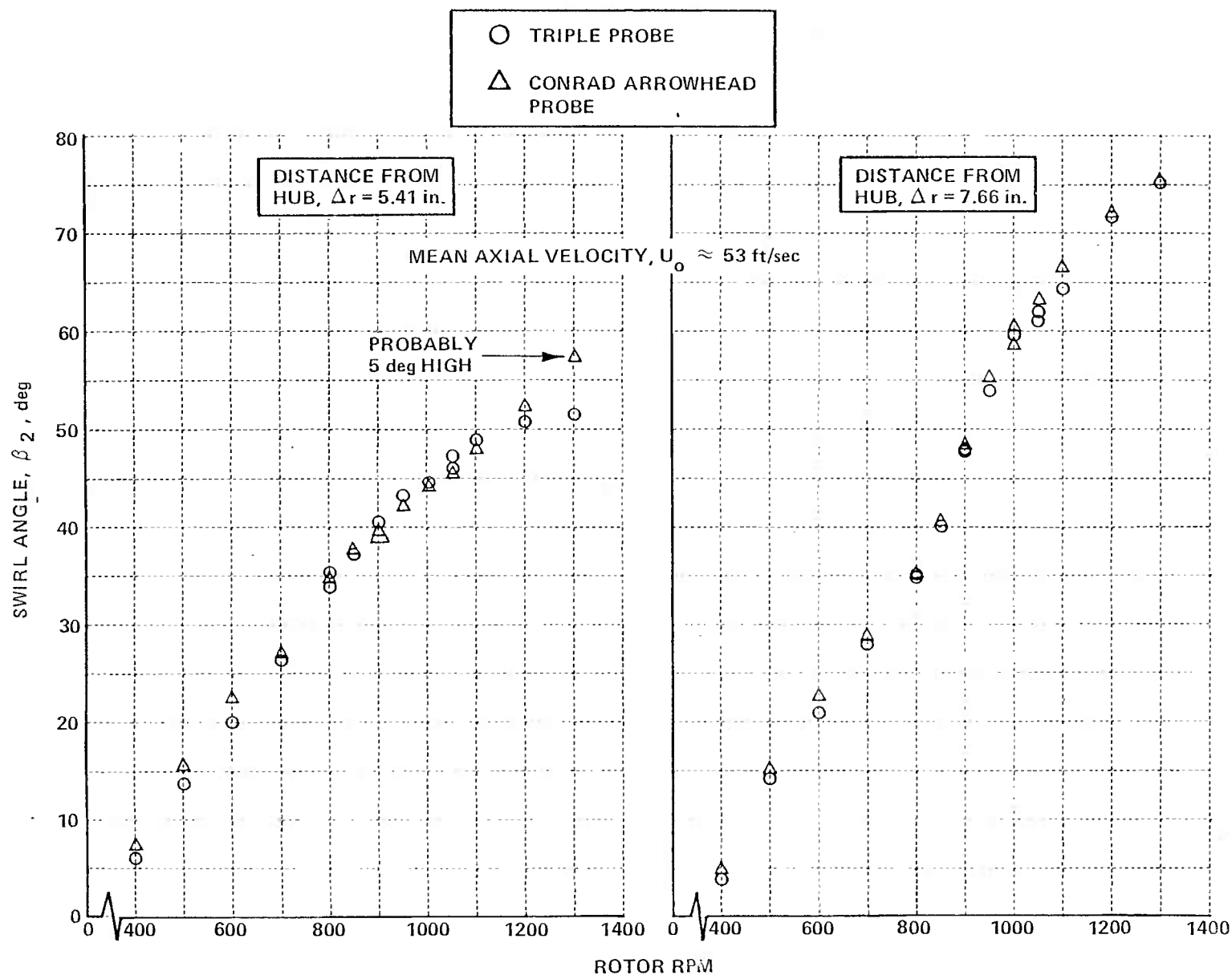
Figure 7 (Cont.) COMPARISON OF SWIRL ANGLES MEASURED BY CONRAD ARROWHEAD PROBE WITH SWIRL ANGLES CALCULATED FROM TRIPLE PROBE MEAN VELOCITY DATA
