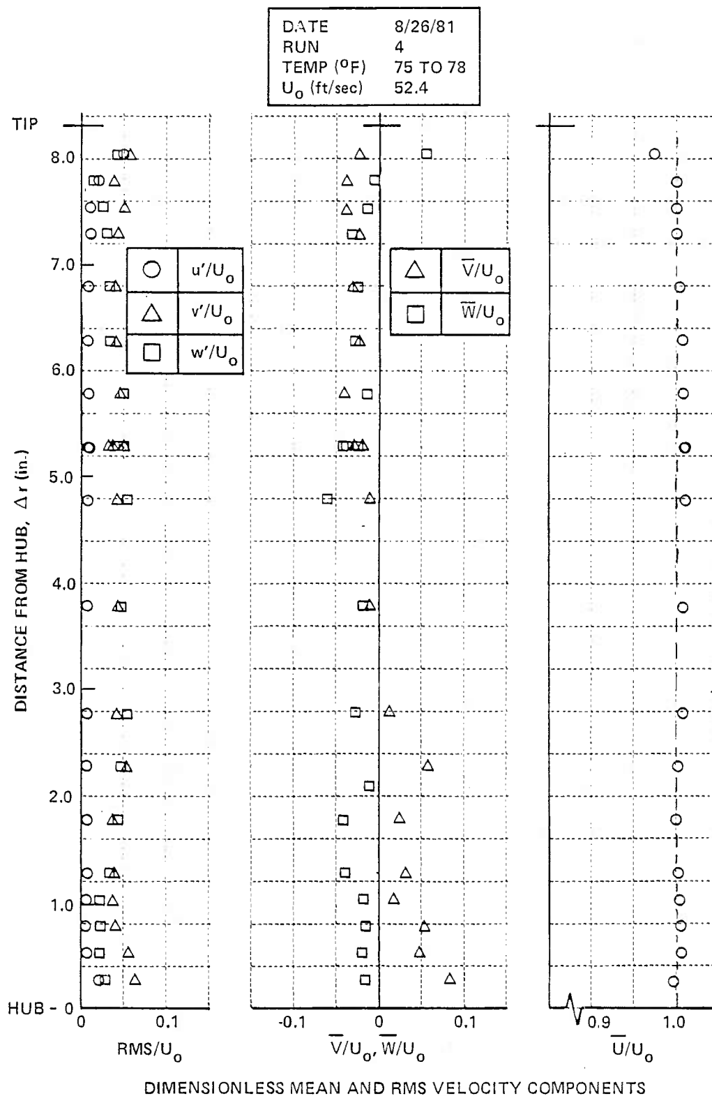
Figure 4 RADIAL DISTRIBUTIONS OF VELOCITY COMPONENTS FAR UPSTREAM OF ROTOR
