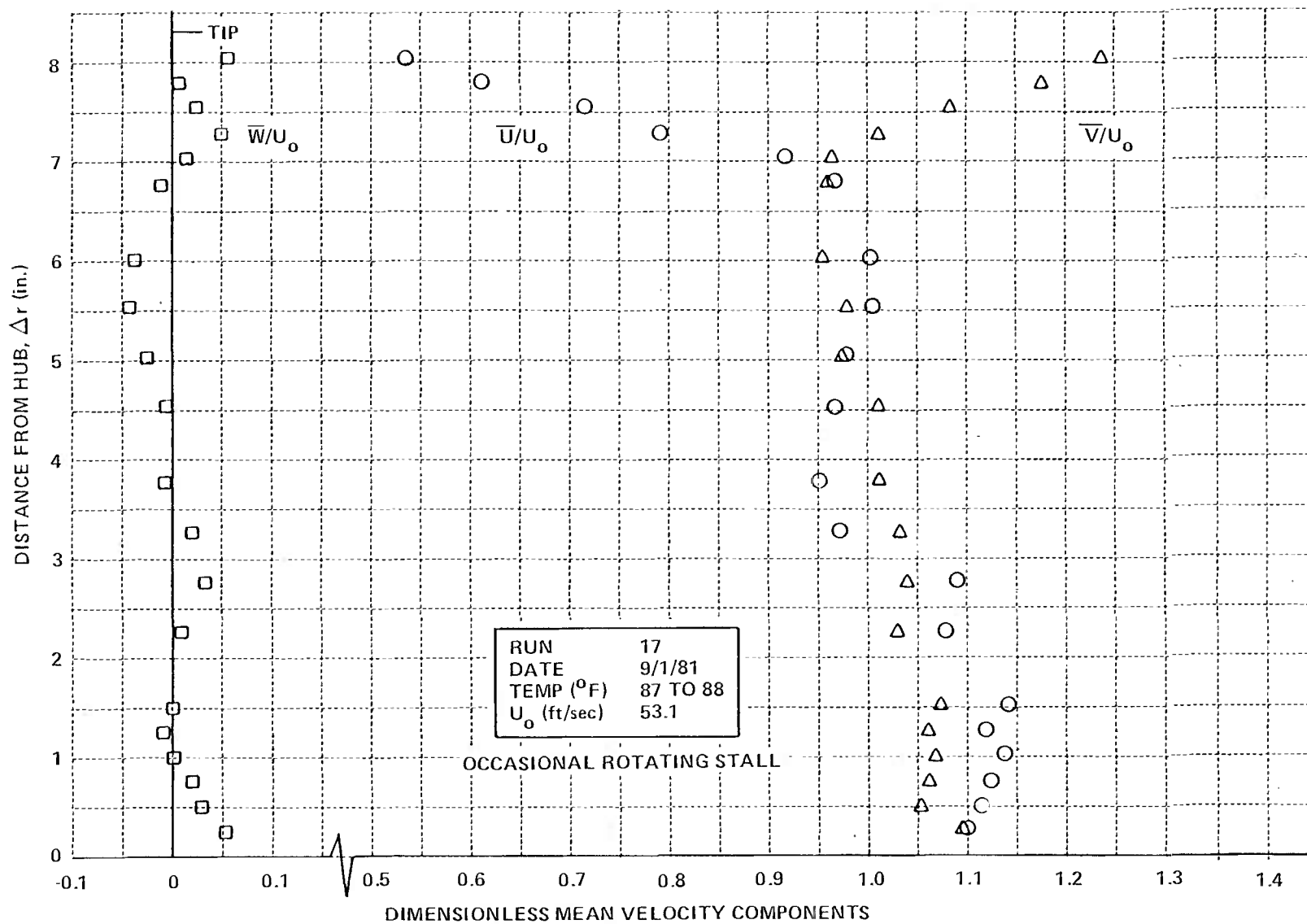
Figure 5 (Cont.) RADIAL DISTRIBUTIONS OF MEAN VELOCITY COMPONENTS DOWNSTREAM OF ISOLATED ROTOR f. ROTOR RPM = 1000
