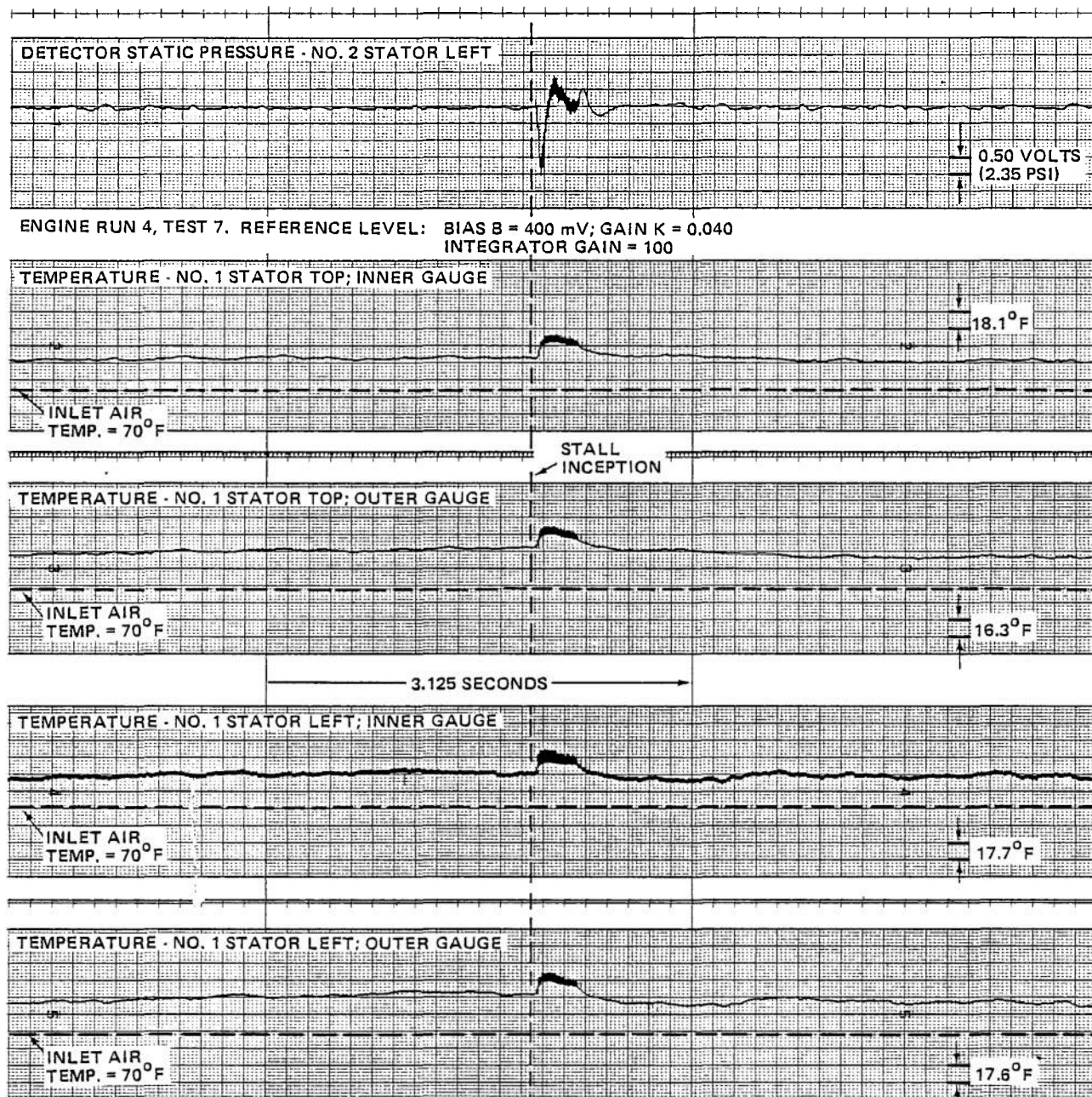
Figure 39 UNSTEADY TEMPERATURE MEASUREMENTS IN J-85 COMPRESSOR DURING ROTATING STALL a. CORRECTED ENGINE SPEED AT STALL INCEPTION, (N/N^* \sqrt{\theta}) = 71.1\%
