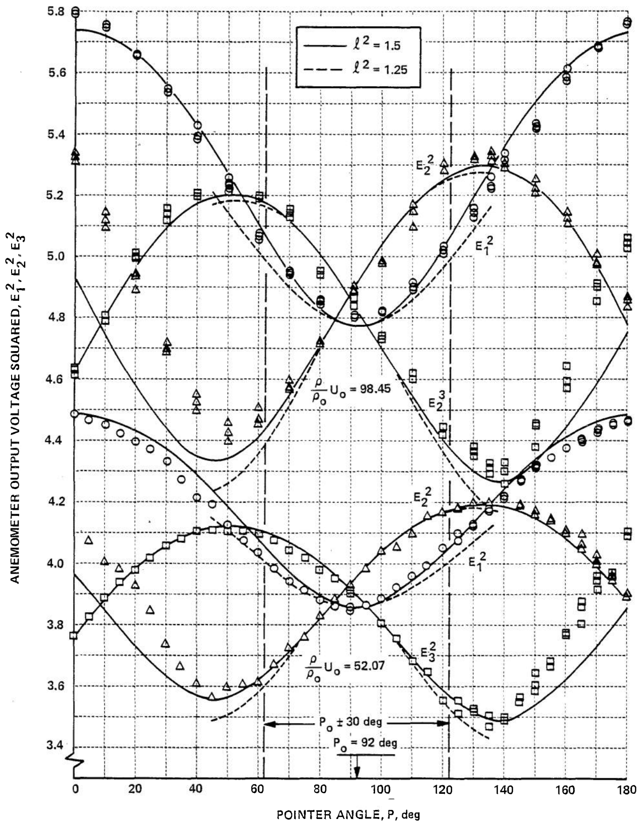
Figure A-6 TRIPLE PROBE ANGLE CALIBRATIONS PROBE NO. 2, ALL SENSORS
