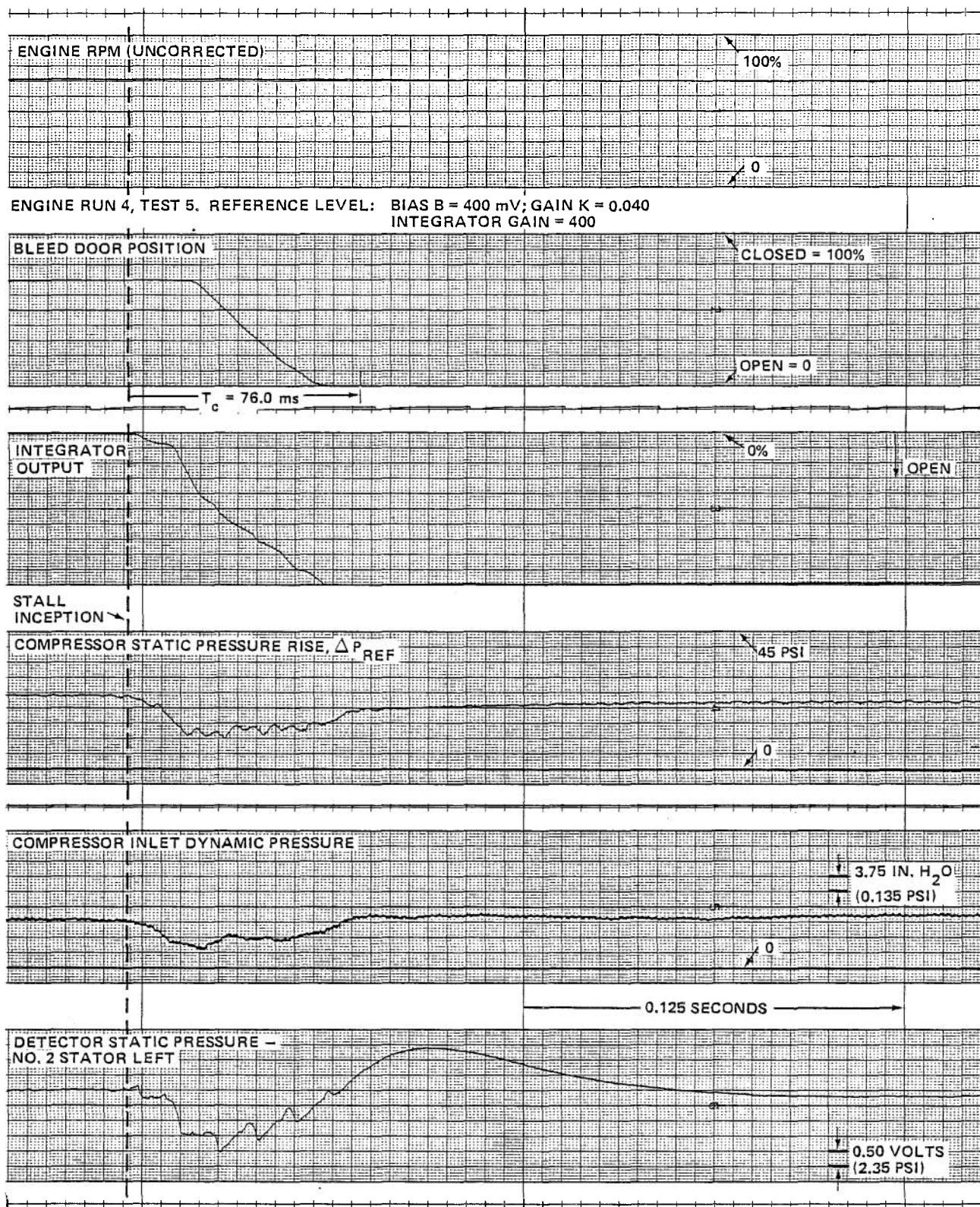
Figure 34 (Cont.) J-85 COMPRESSOR RESPONSE TO ROTATING STALL AT NOMINAL ENGINE SPEED OF 70% (EXPANDED TIME SCALE) b. INTEGRATOR GAIN = 400; CORRECTED ENGINE SPEED AT STALL INCEPTION, (N/N * \sqrt{\theta}) = 70.8\%
