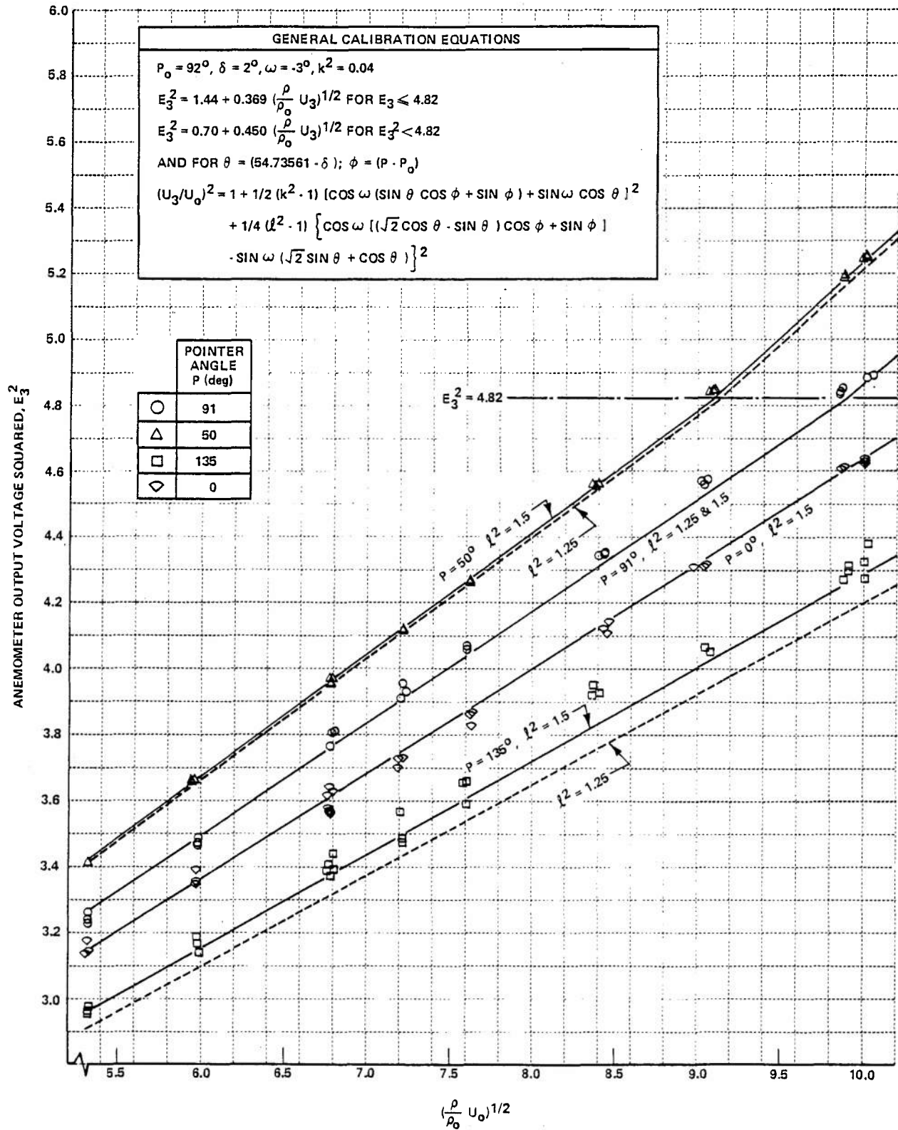
Figure A-5 (Cont.) TRIPLE PROBE VELOCITY CALIBRATION
