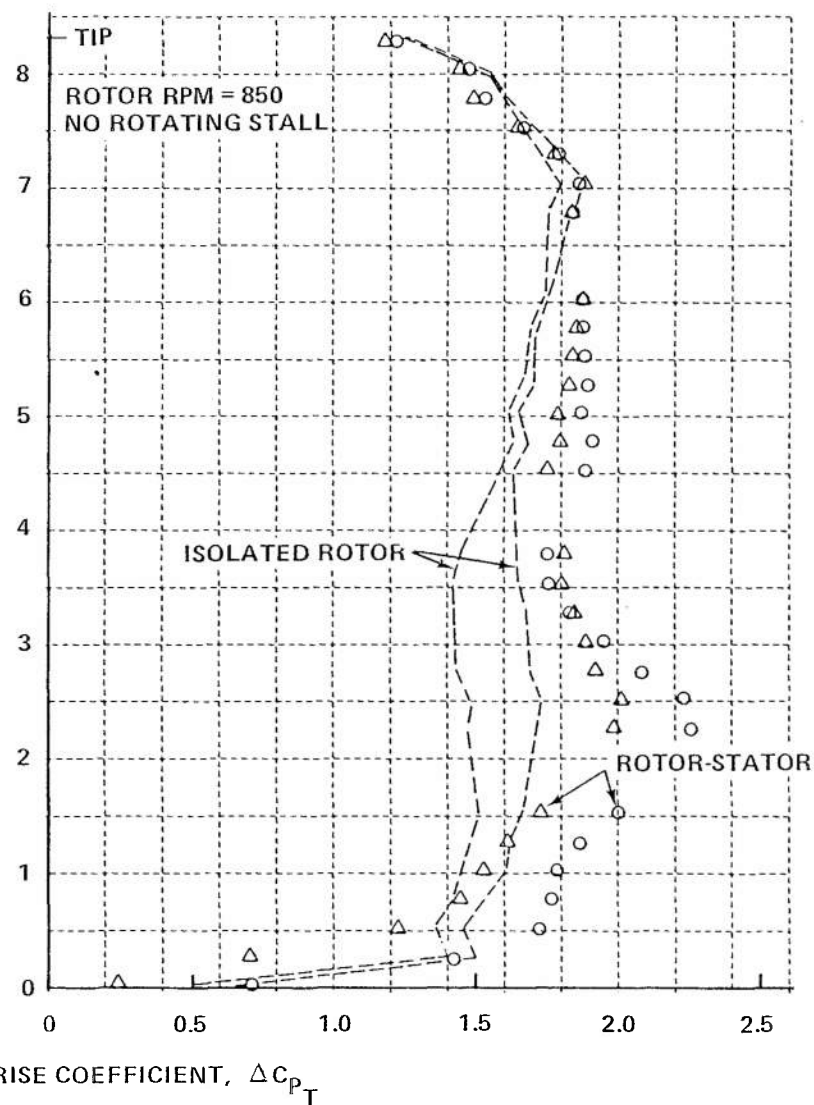
Figure 13 (Cont.) RADIAL DISTRIBUTIONS OF TOTAL PRESSURE COEFFICIENT IMMEDIATELY DOWNSTREAM OF ISOLATED ROTOR AND THE SAME ROTOR IN ROTOR-STATOR STAGE. STATOR STAGGER ANGLE AT MEAN RADIUS, \delta_s = 12.9 deg
