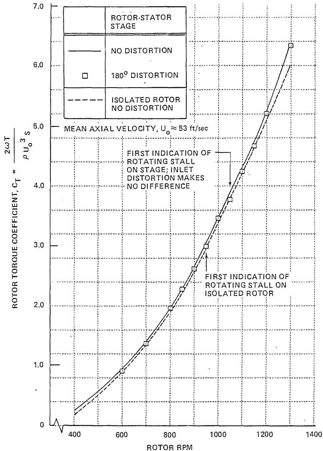
Figure 21 (Cont.) ROTOR TORQUE COEFFICIENTS FOR A ROTOR-STATOR STAGE WITH AND WITHOUT INLET DISTORTION b. STATOR STAGGER ANGLE, \delta_s = 22.9 deg
