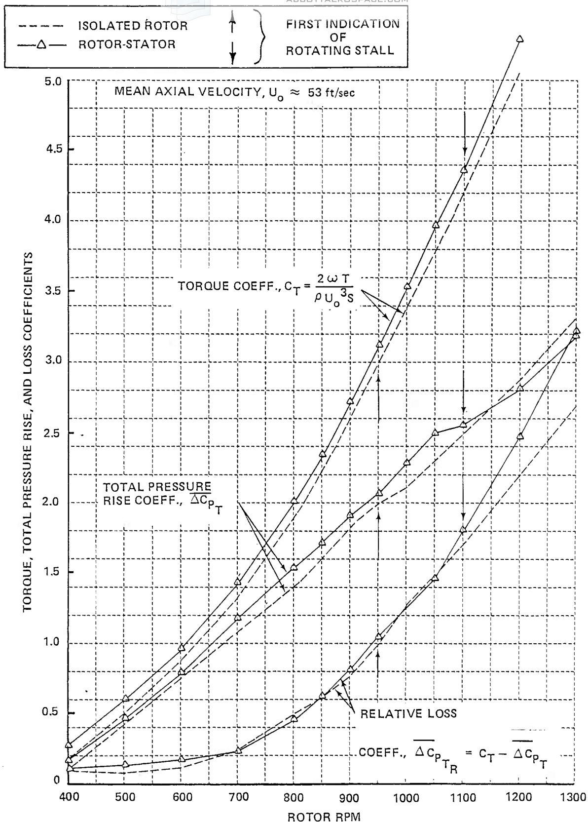
Figure 20 TORQUE COEFFICIENT AND AREA-AVERAGED TOTAL PRESSURE RISE, AND LOSS COEFFICIENTS FOR ROTOR IN LOW HUB/TIP RATIO ROTOR-STATOR STAGE. STATOR STAGGER ANGLE AT MEAN RADIUS, \delta_s = 32.9 deg.
