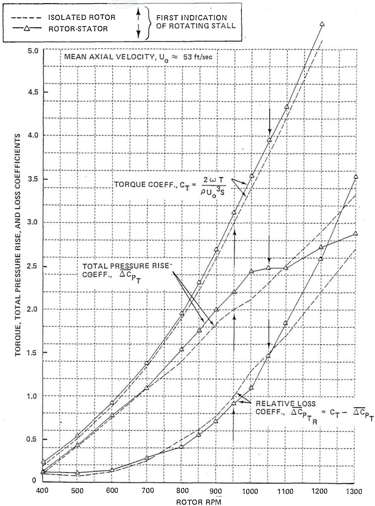
Figure 18 TORQUE COEFFICIENT AND AREA-AVERAGED TOTAL PRESSURE RISE, AND LOSS COEFFICIENTS FOR ROTOR IN LOW HUB/TIP RATIO ROTOR-STATOR STAGE. STATOR STAGGER ANGLE AT MEAN RADIUS \delta_s = 12.9 deg.
