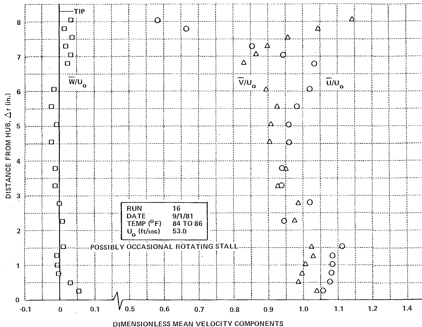
Figure 5 (Cont.) RADIAL DISTRIBUTIONS OF MEAN VELOCITY COMPONENTS DOWNSTREAM OF ISOLATED ROTOR e. ROTOR RPM = 950
