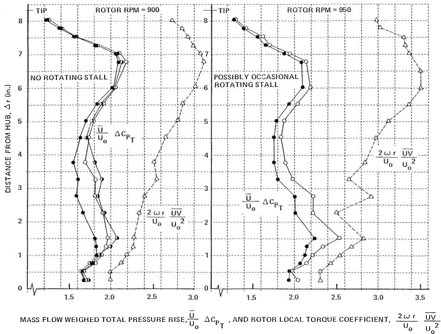
Figure 10 (Cont.) COMPARISONS OF RADIAL DISTRIBUTIONS OF MASS FLOW WEIGHTED TOTAL PRESSURE RISE ACROSS ISOLATED ROTOR WITH ROTOR TORQUE COEFFICIENT
