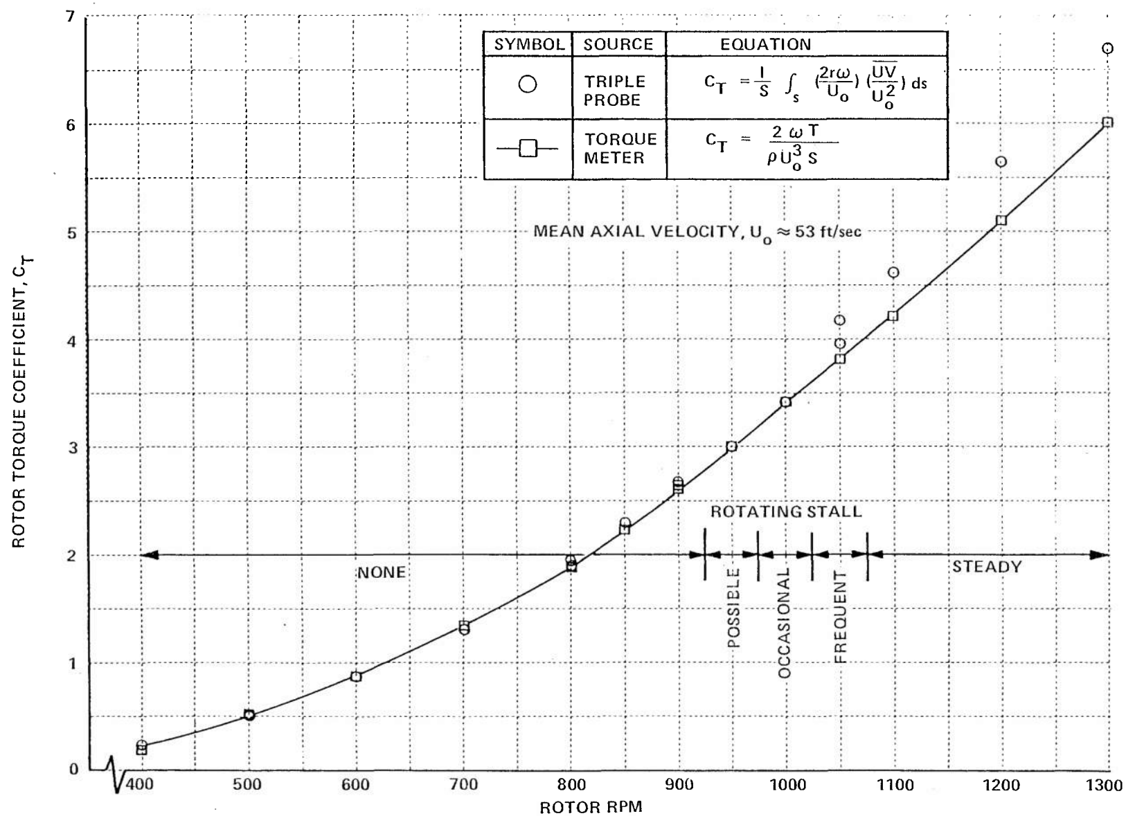
Figure 9 COMPARISON OF ROTOR TORQUE COEFFICIENTS CALCULATED FROM TRIPLE PROBE DATA WITH THOSE CALCULATED FROM TORQUE METER DATA
