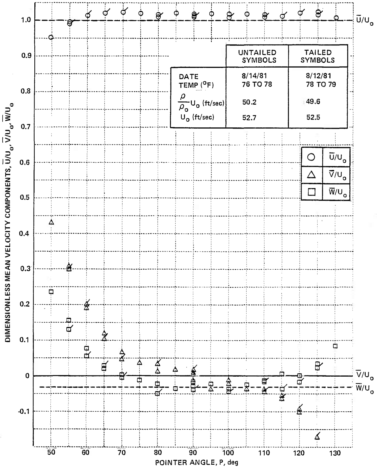
Figure A-8 TRIPLE PROBE ANGLE CALIBRATION CHECK, MEAN VELOCITY COMPONENTS
