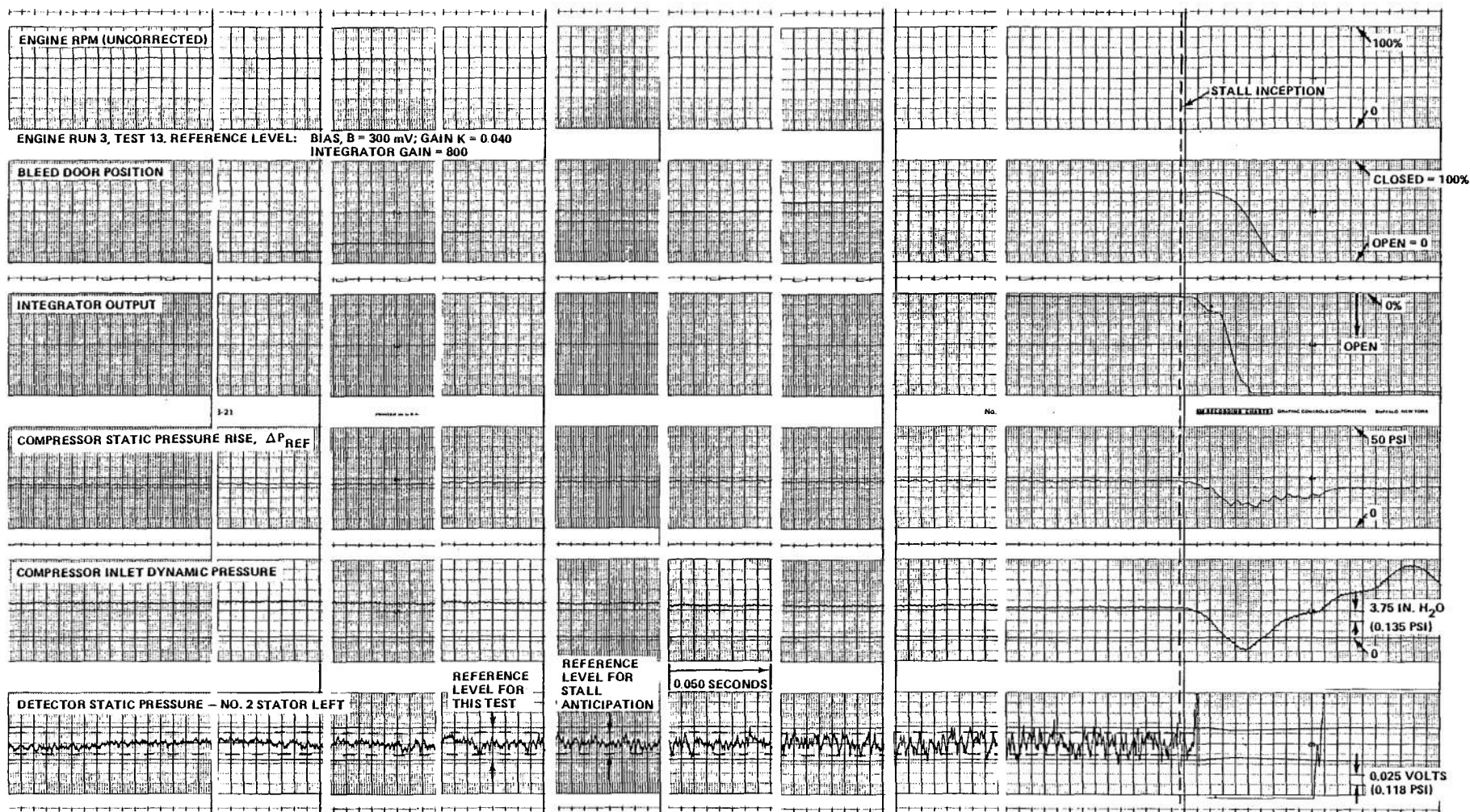
Figure 37 J-85 COMPRESSOR PARAMETERS PRIOR TO ROTATING STALL. STALL CONTROL DETUNED TO ALLOW STALL. CORRECTED ENGINE SPEED AT STALL INCEPTION ( N/N^* \sqrt{\theta} ) = 70.1%
