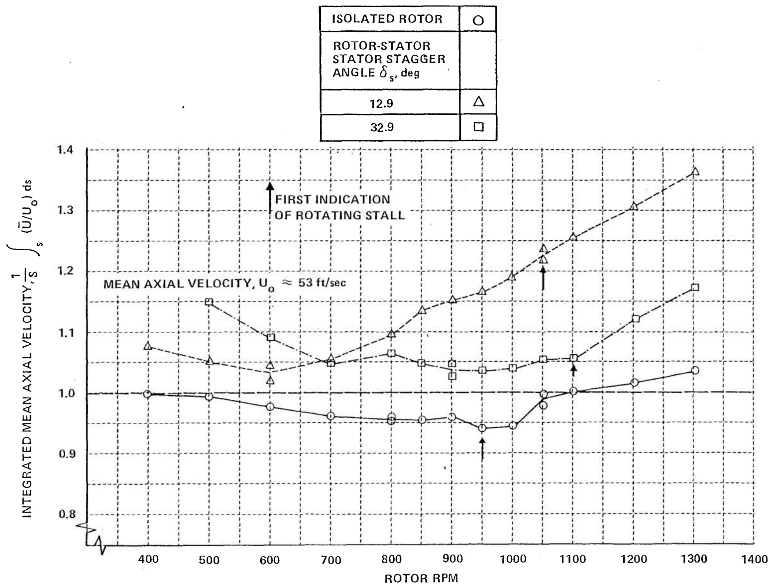
Figure 16 AREA WEIGHTED INTEGRALS OF DIMENSIONLESS MEAN AXIAL FLOW VELOCITY
