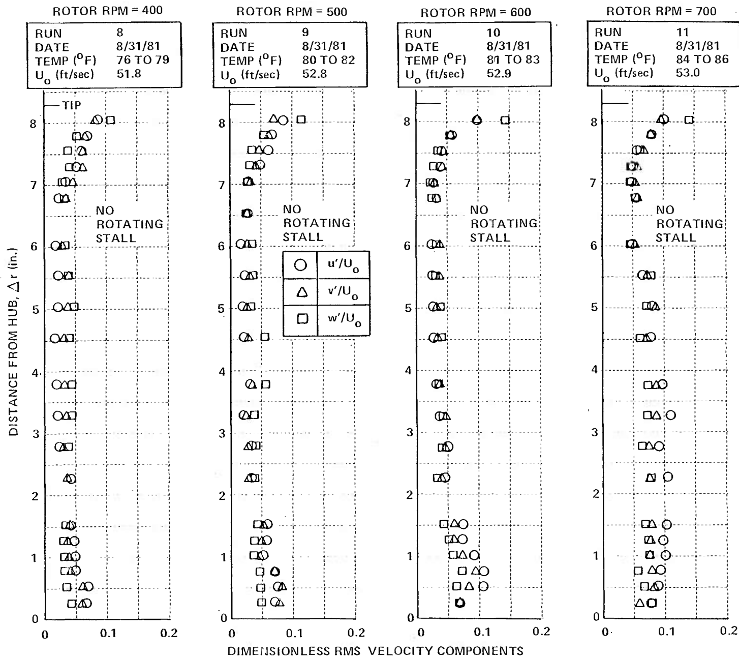
Figure 6 DIMENSIONLESS RMS VELOCITY COMPONENTS DOWNSTREAM OF ISOLATED ROTOR
