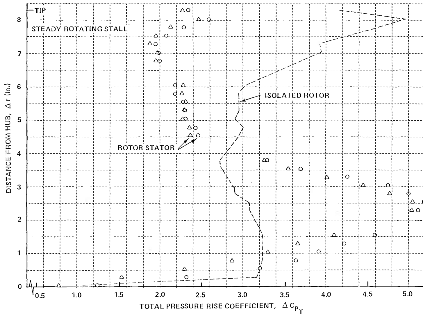
Figure 13 (Cont.) RADIAL DISTRIBUTIONS OF TOTAL PRESSURE COEFFICIENT IMMEDIATELY DOWNSTREAM OF ISOLATED ROTOR AND THE SAME ROTOR IN ROTOR-STATOR STAGE. STATOR STAGGER ANGLE AT MEAN RADIUS, \delta_s = 12.9 deg.
