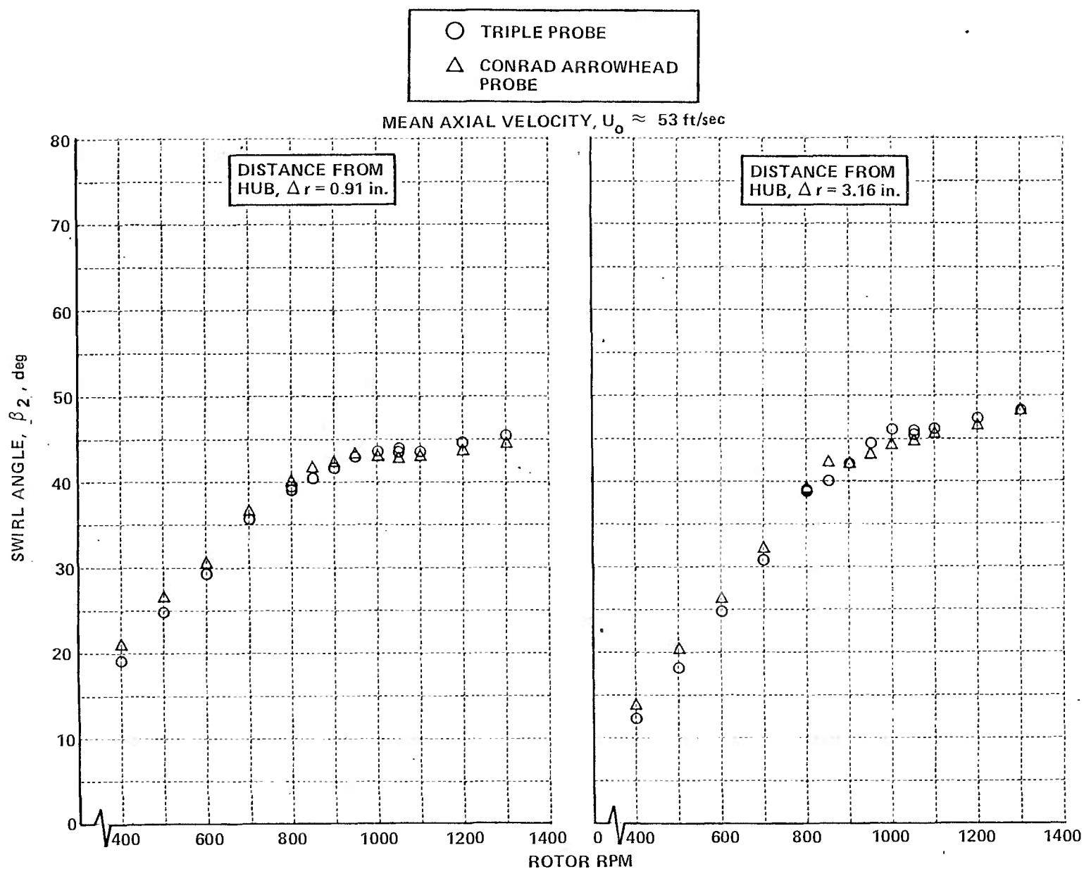
Figure 7 COMPARISON OF SWIRL ANGLES MEASURED BY CONRAD ARROWHEAD PROBE WITH SWIRL ANGLES CALCULATED FROM TRIPLE PROBE MEAN VELOCITY DATA
