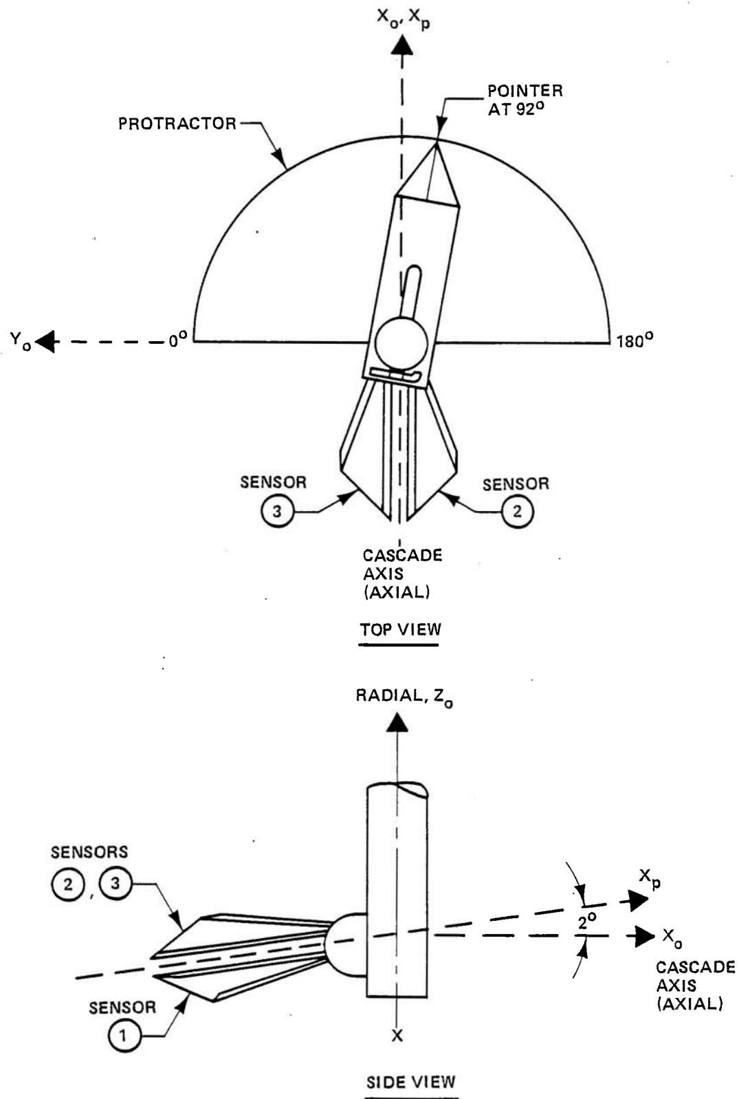
Figure A-3. RELATIONSHIP BETWEEN PROBE AXIS OF SYMMETRY AND ANNULAR CASCADE AXIS
