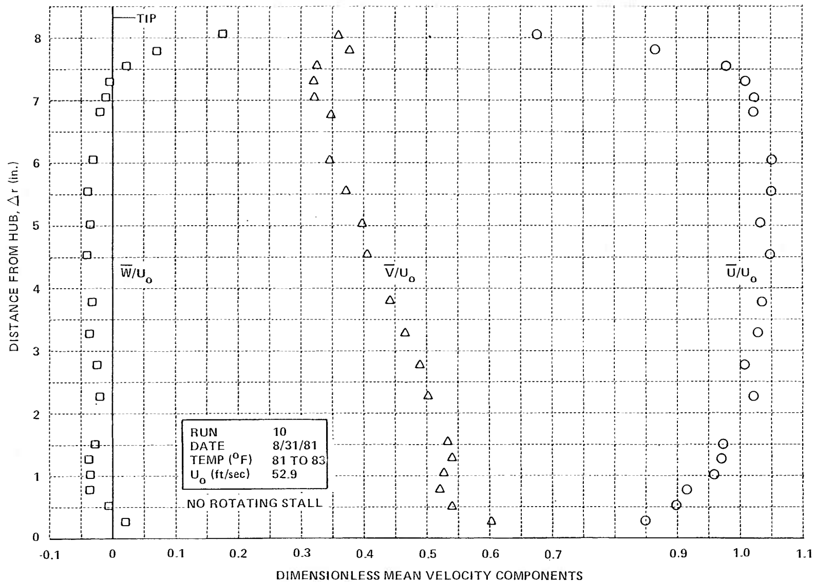
Figure 5 (Cont.) RADIAL DISTRIBUTIONS OF MEAN VELOCITY COMPONENTS DOWNSTREAM OF ISOLATED ROTOR b. ROTOR RPM = 600
