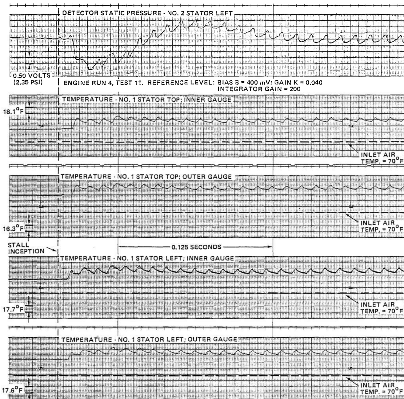
Figure 40 (Cont.) UNSTEADY TEMPERATURE MEASUREMENTS IN J-85 COMPRESSOR DURING ROTATING STALL (EXPANDED TIME SCALE) c. CORRECTED ENGINE SPEED AT STALL INCEPTION, (N/N * \sqrt{\theta}) = 78.7\%
