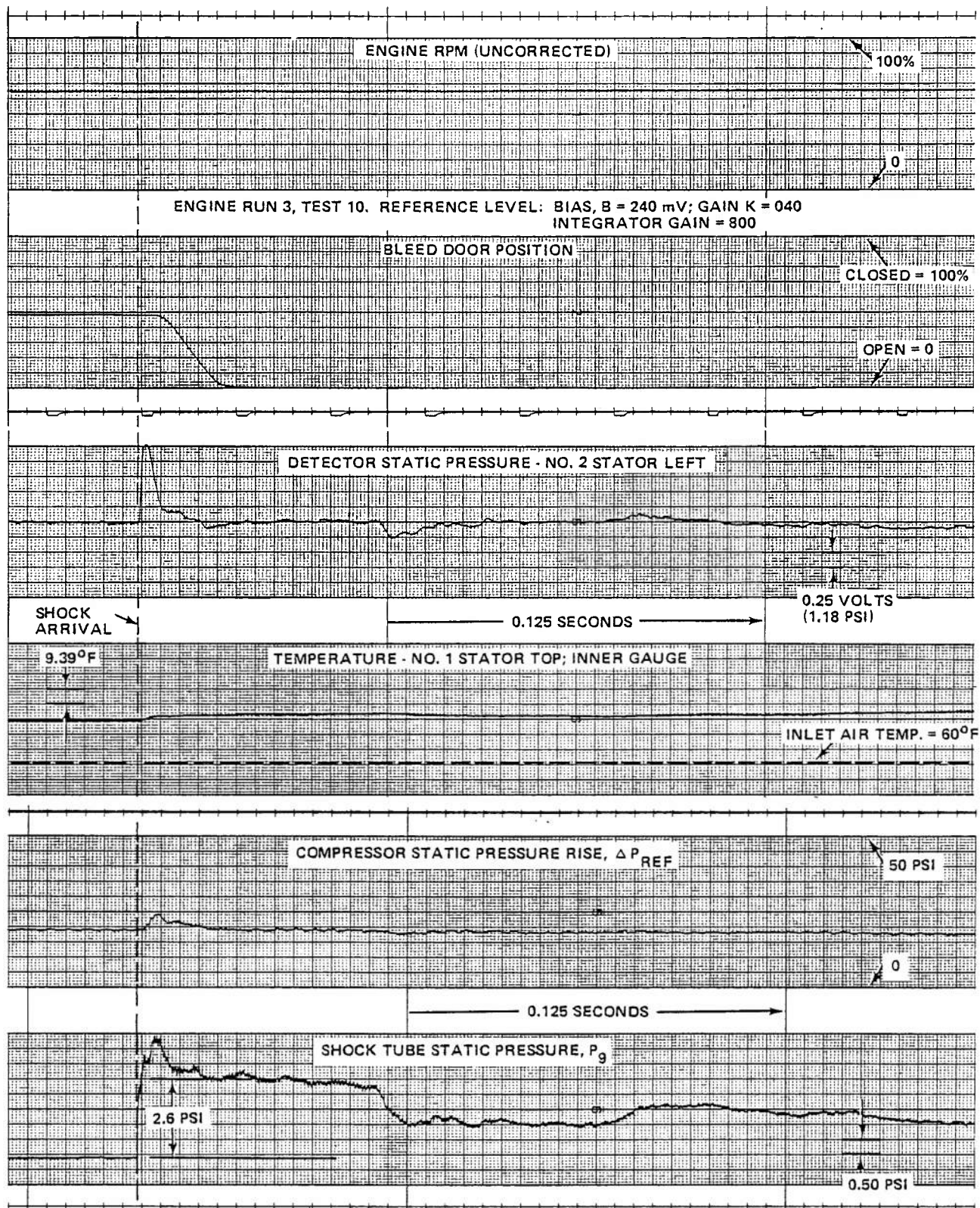
Figure 45 J-85 COMPRESSOR RESPONSE TO INCIDENT SHOCK WAVE. STALL CONTROL ACTIVE. CORRECTED ENGINE SPEED N/N^* \sqrt{\theta} = 64.4\%
