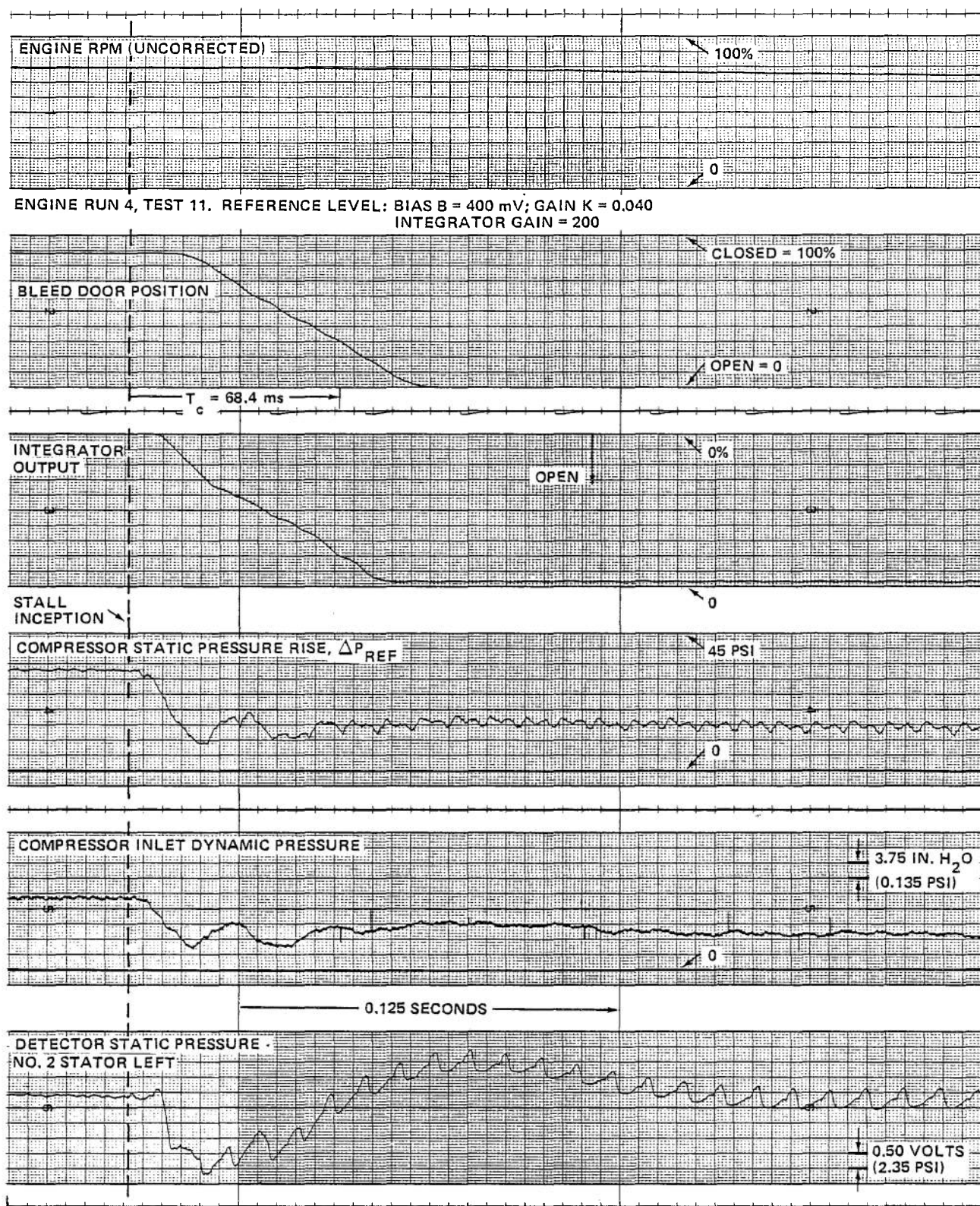
Figure 36 (Cont.) J-85 COMPRESSOR RESPONSE TO ROTATING STALL AT NOMINAL ENGINE SPEED OF 78% (EXPANDED TIME SCALE) b. INTEGRATOR GAIN = 200; CORRECTED ENGINE SPEED AT STALL INCEPTION, (N/N * \sqrt{\theta}) = 78.7\%
