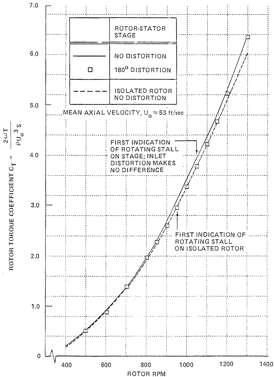
Figure 21 ROTOR TORQUE COEFFICIENTS FOR A ROTOR-STATOR STAGE WITH AND WITHOUT INLET DISTORTION a. STATOR STAGGER ANGLE, \delta_s = 12.9 \text{ deg}
