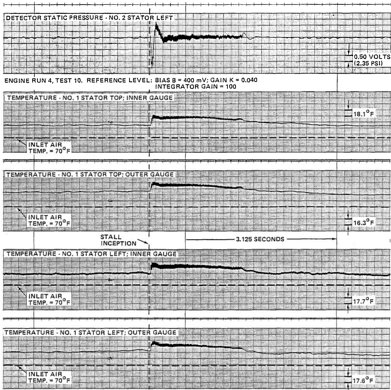
Figure 39 (Cont.) UNSTEADY TEMPERATURE MEASUREMENTS IN J-85 COMPRESSOR DURING ROTATING STALL b. CORRECTED ENGINE SPEED AT STALL INCEPTION, (N/N * \sqrt{\theta}) = 75.5\%
