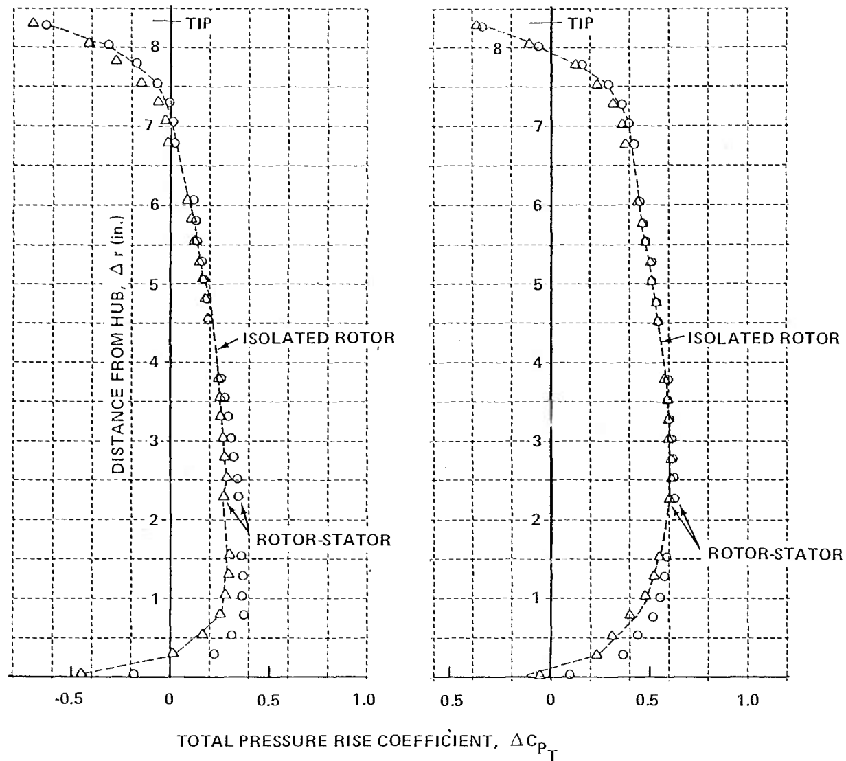
Figure 13 RADIAL DISTRIBUTIONS OF TOTAL PRESSURE COEFFICIENT IMMEDIATELY DOWNSTREAM OF ISOLATED ROTOR AND THE SAME ROTOR IN ROTOR-STATOR STAGE. STATOR STAGGER ANGLE AT MEAN RADIUS, \delta_s = 12.9 deg
