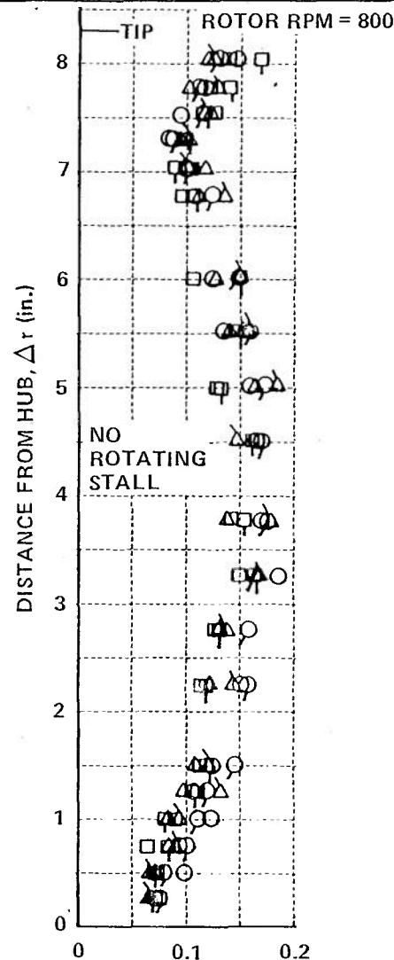
Figure 6 (Cont.) DIMENSIONLESS RMS VELOCITY COMPONENTS DOWNSTREAM OF ISOLATED ROTOR b. ROTOR RPM = 800, 850, 900
