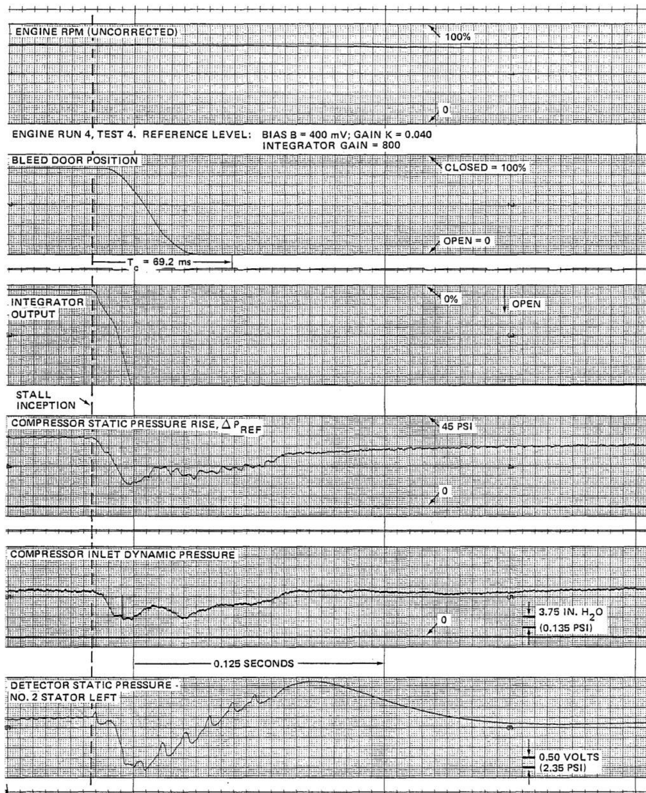
Figure 36 J-85 COMPRESSOR RESPONSE TO ROTATING STALL AT NOMINAL ENGINE SPEED OF 78% (EXPANDED TIME SCALE) a. INTEGRATOR GAIN = 800; CORRECTED ENGINE SPEED AT STALL INCEPTION, (N/N * \sqrt{\theta}) = 77.7\%
