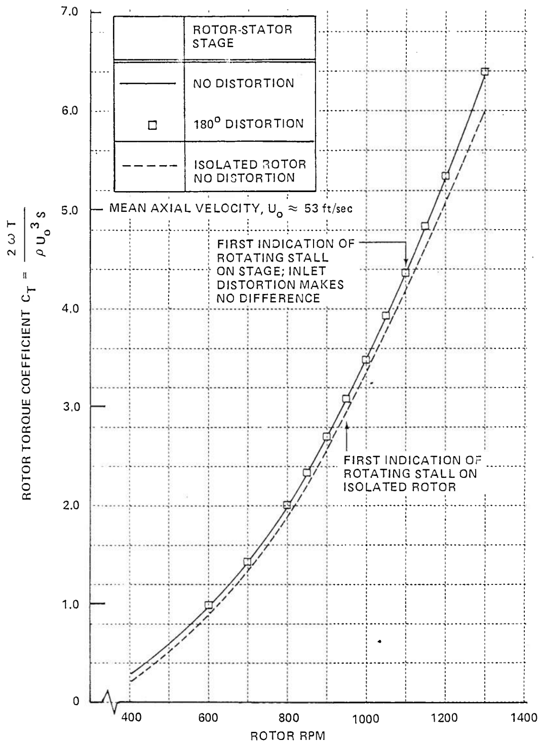
Figure 21 (Cont.) ROTOR TORQUE COEFFICIENTS FOR A ROTOR-STATOR STAGE WITH AND WITHOUT INLET DISTORTION
