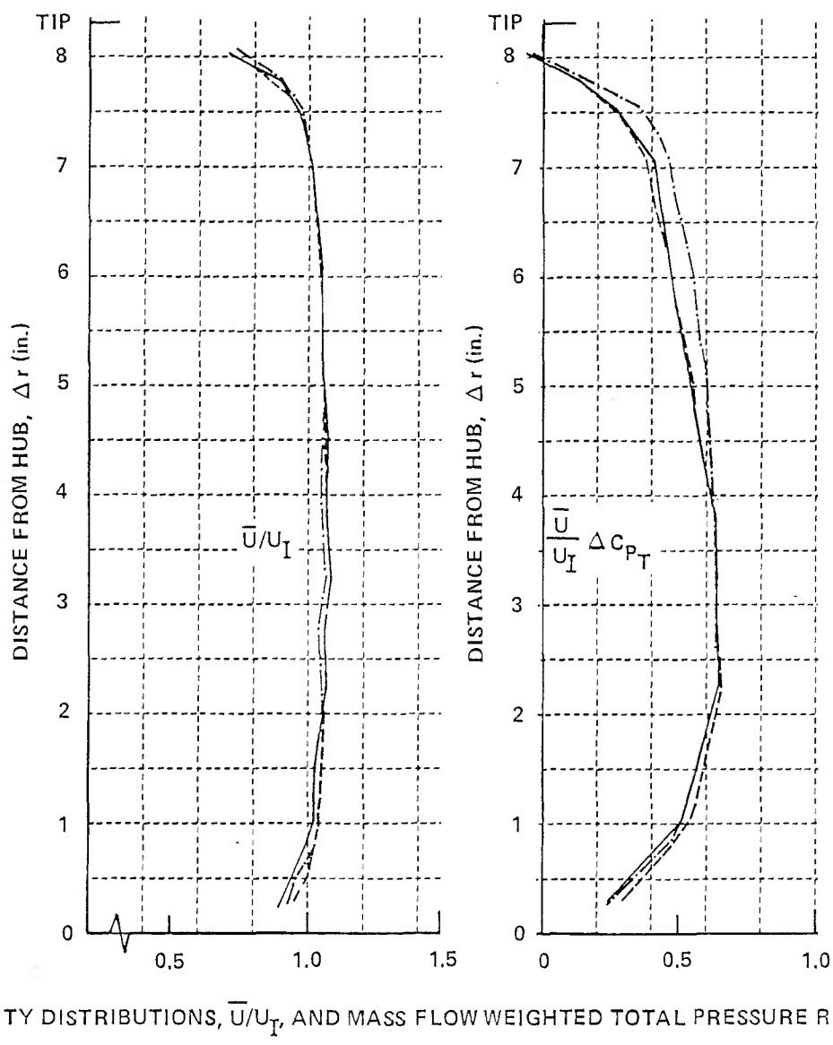
Figure 15 RADIAL DISTRIBUTIONS OF AXIAL VELOCITY AND MASS FLOW WEIGHTED TOTAL PRESSURE RISE DOWNSTREAM OF ISOLATED ROTOR AND THE SAME ROTOR IN A ROTOR-STATOR STAGE. (a) ROTOR RPM = 500
