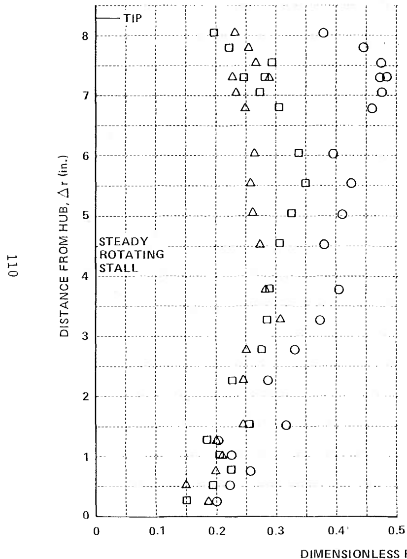
Figure 6 (Cont.) DIMENSIONLESS RMS VELOCITY COMPONENTS DOWNSTREAM OF ISOLATED ROTOR
