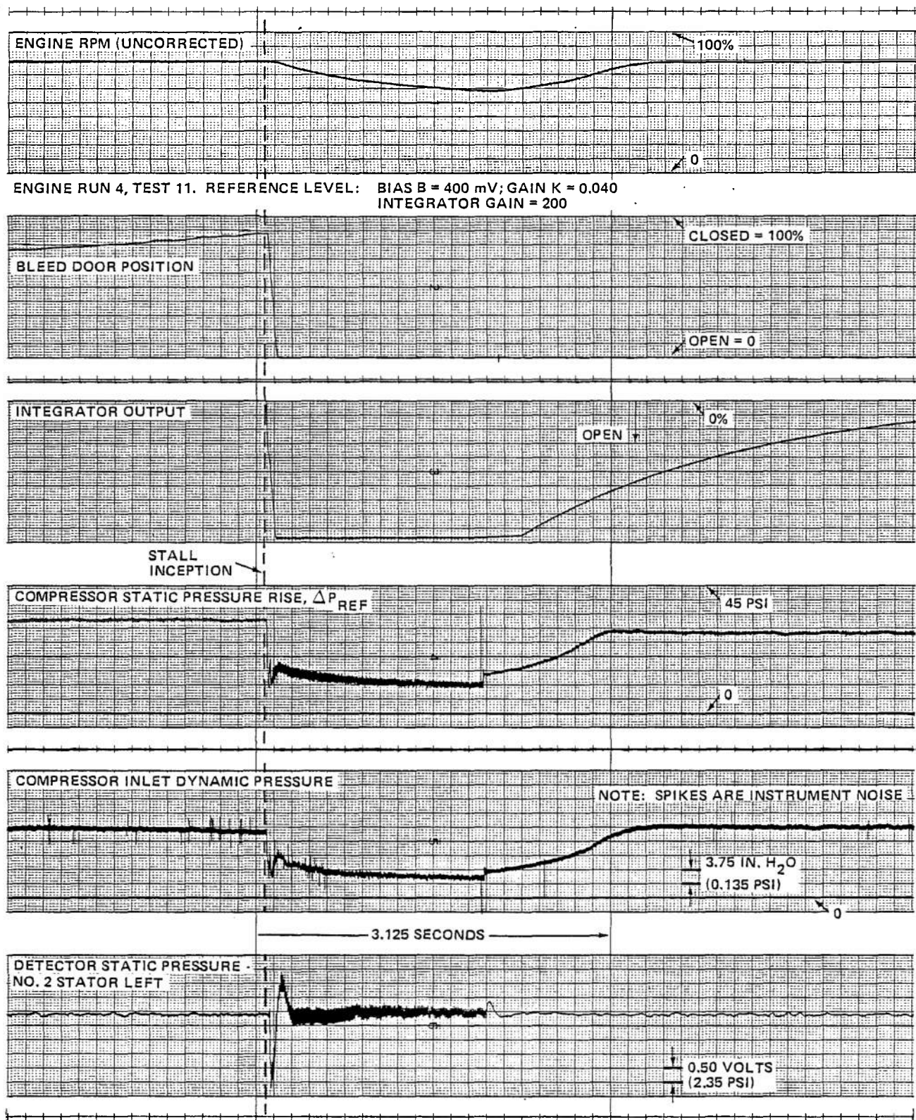
Figure 33 (Cont.) J-85 COMPRESSOR RESPONSE TO ROTATING STALL AT NOMINAL ENGINE SPEED OF 78% b. INTEGRATOR GAIN = 200; CORRECTED ENGINE SPEED AT STALL INCEPTION, (N/N * \sqrt{\theta}) = 78.7\%
