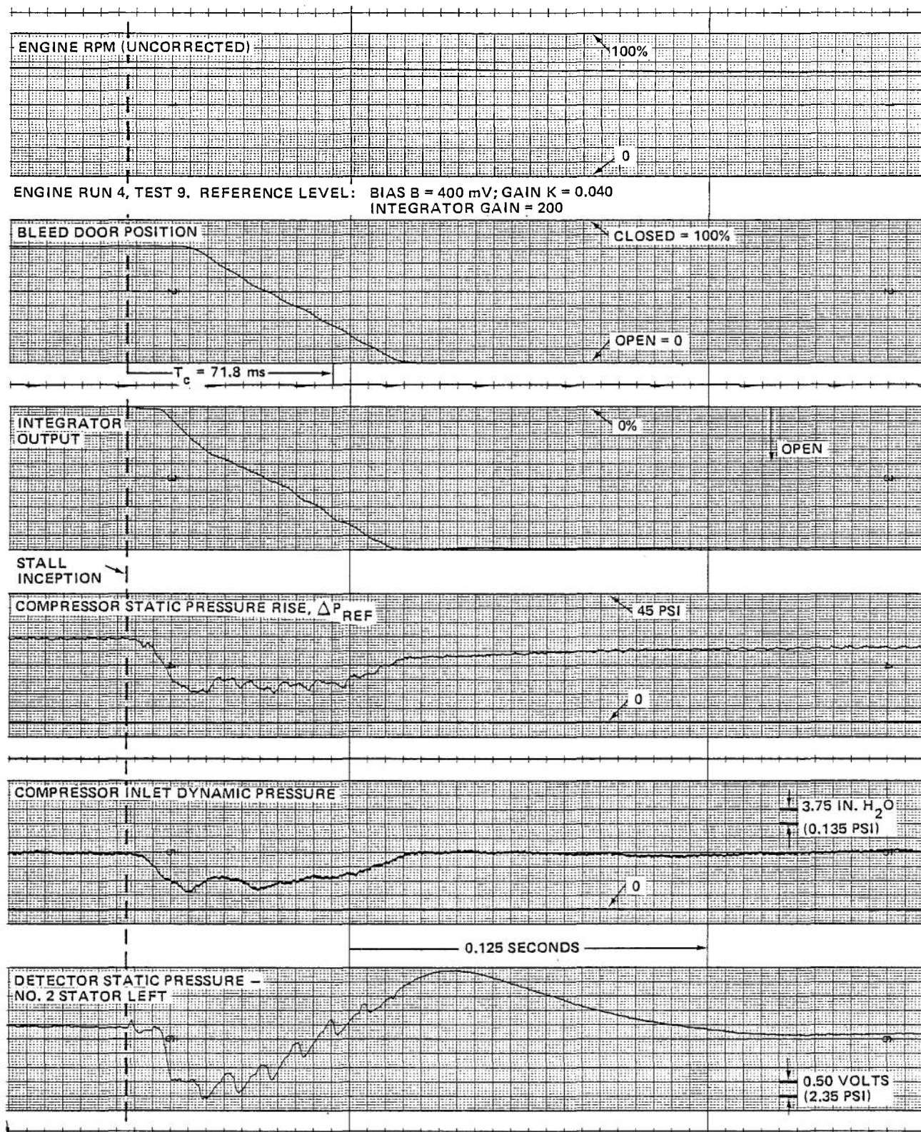
Figure 35 (Cont.) J-85 COMPRESSOR RESPONSE TO ROTATING STALL AT NOMINAL ENGINE SPEED OF 75% (EXPANDED TIME SCALE) c) INTEGRATOR GAIN = 200; CORRECTED ENGINE SPEED AT STALL INCEPTION, (N/N^* \sqrt{\theta}) = 74.9\%
