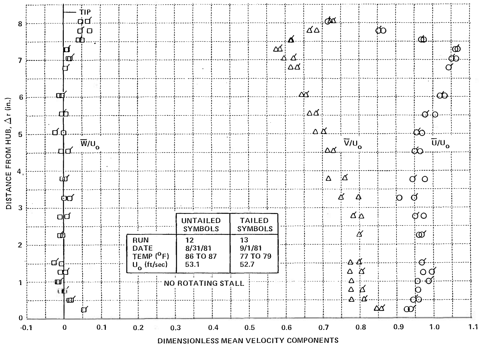
Figure 5 (Cont.) RADIAL DISTRIBUTIONS OF MEAN VELOCITY COMPONENTS DOWNSTREAM OF ISOLATED ROTOR c. ROTOR RPM = 800
