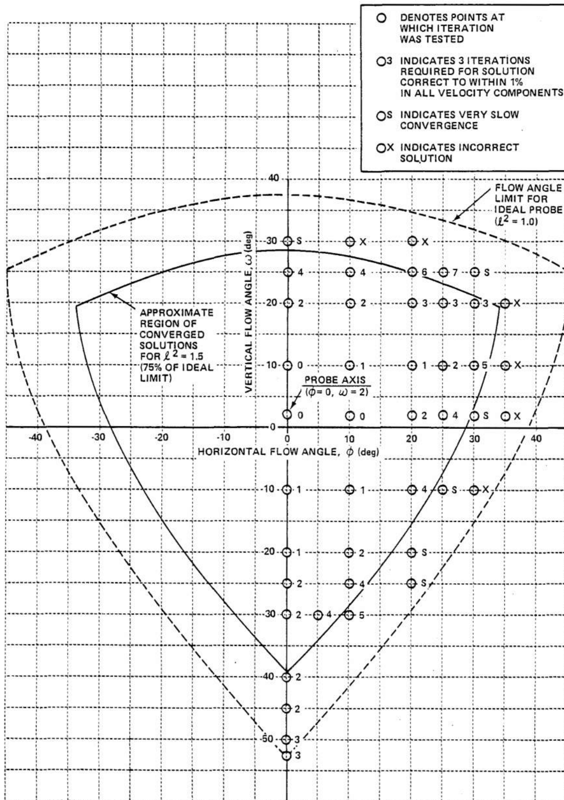
Figure A-4 SUMMARY OF CONVERGENCE TESTS FOR ITERATIVE SOLUTION OF NONLINEAR ANEMOMETER EQUATIONS
