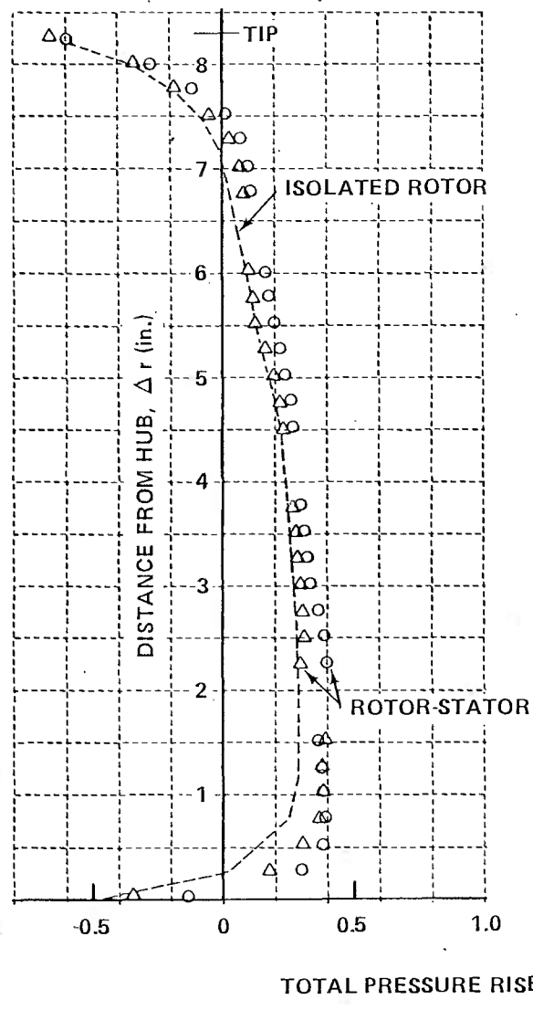
Figure 14 RADIAL DISTRIBUTIONS OF TOTAL PRESSURE COEFFICIENT IMMEDIATELY DOWNSTREAM OF ISOLATED ROTOR AND THE SAME ROTOR IN ROTOR-STATOR STAGE. STATOR STAGGER ANGLE AT MEAN RADIUS, \delta_s = 32.9 deg.
