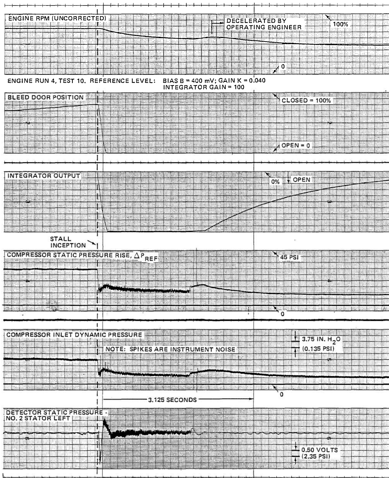
Figure 32 (Cont.) J-85 COMPRESSOR RESPONSE TO ROTATING STALL AT NOMINAL ENGINE SPEED OF 75%
