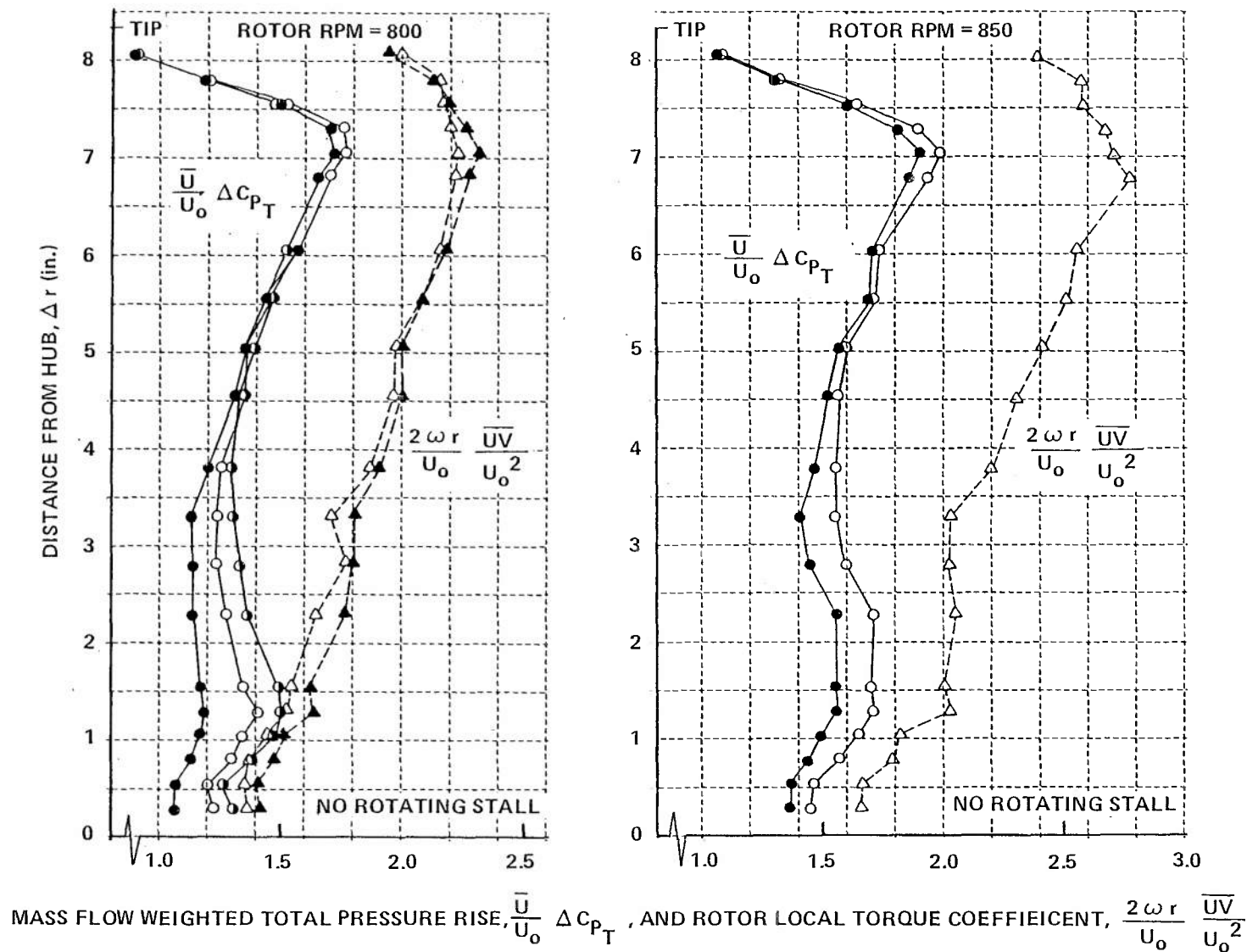
Figure 10 (Cont.) COMPARISONS OF RADIAL DISTRIBUTIONS OF MASS FLOW WEIGHTED TOTAL PRESSURE RISE ACROSS ISOLATED ROTOR WITH ROTOR TORQUE COEFFICIENT
