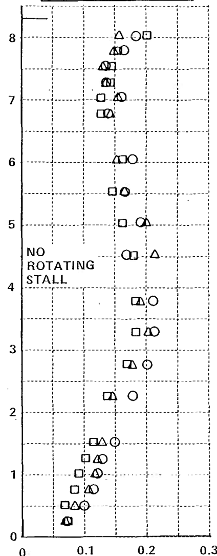
Figure 6 (Cont.) DIMENSIONLESS RMS VELOCITY COMPONENTS DOWNSTREAM OF ISOLATED ROTOR b. ROTOR RPM = 800, 850, 900
