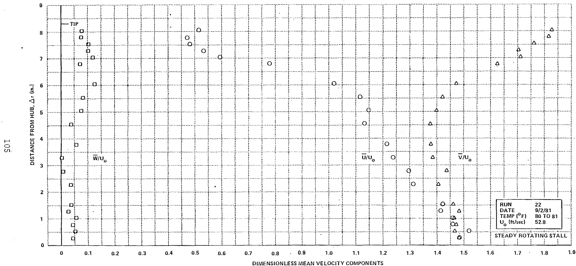
Figure 5 (Cont.) RADIAL DISTRIBUTIONS OF MEAN VELOCITY COMPONENTS DOWNSTREAM OF ISOLATED ROTOR
