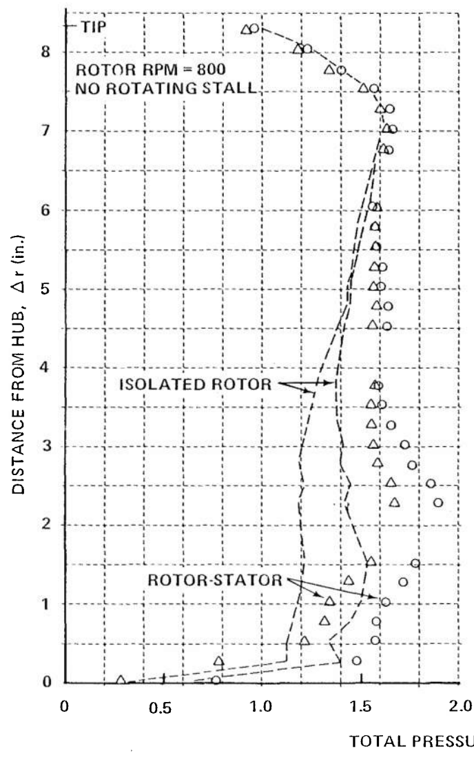
Figure 13 (Cont.) RADIAL DISTRIBUTIONS OF TOTAL PRESSURE COEFFICIENT IMMEDIATELY DOWNSTREAM OF ISOLATED ROTOR AND THE SAME ROTOR IN ROTOR-STATOR STAGE. STATOR STAGGER ANGLE AT MEAN RADIUS, \delta_s = 12.9 deg
