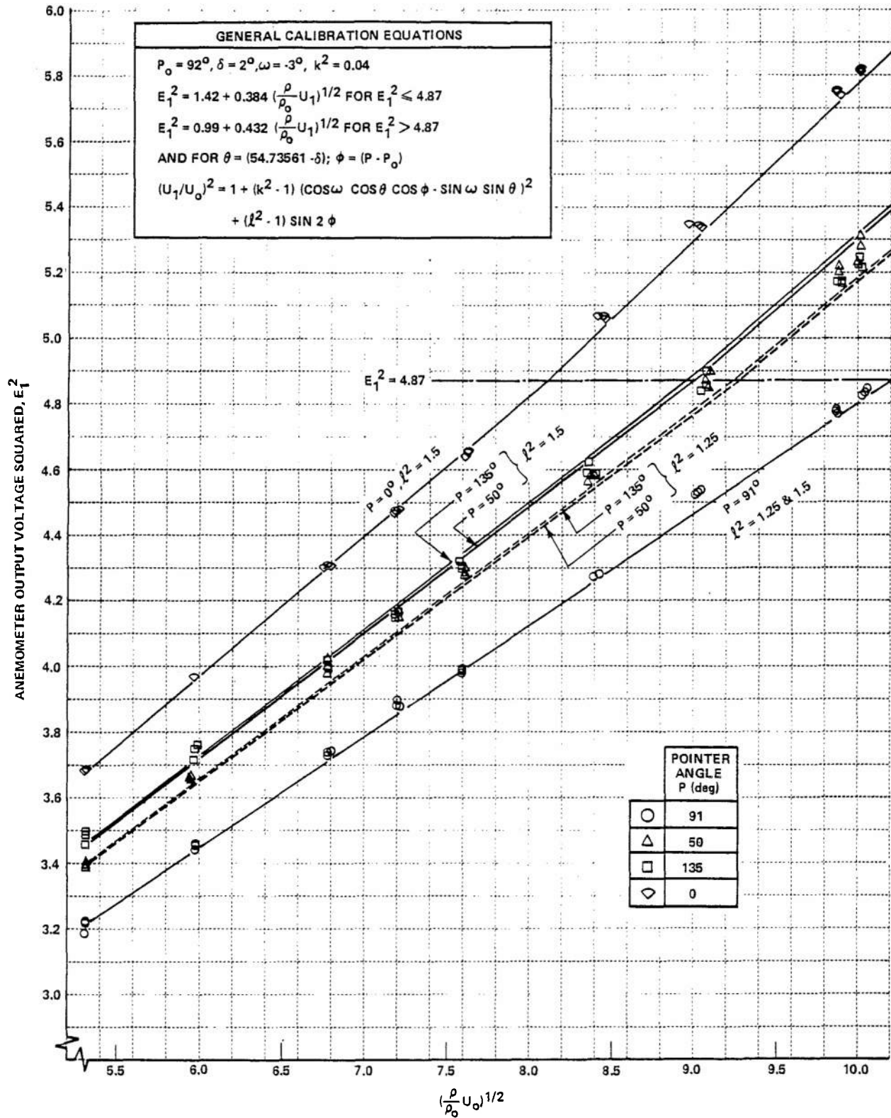
Figure A-5 TRIPLE PROBE VELOCITY CALIBRATION
