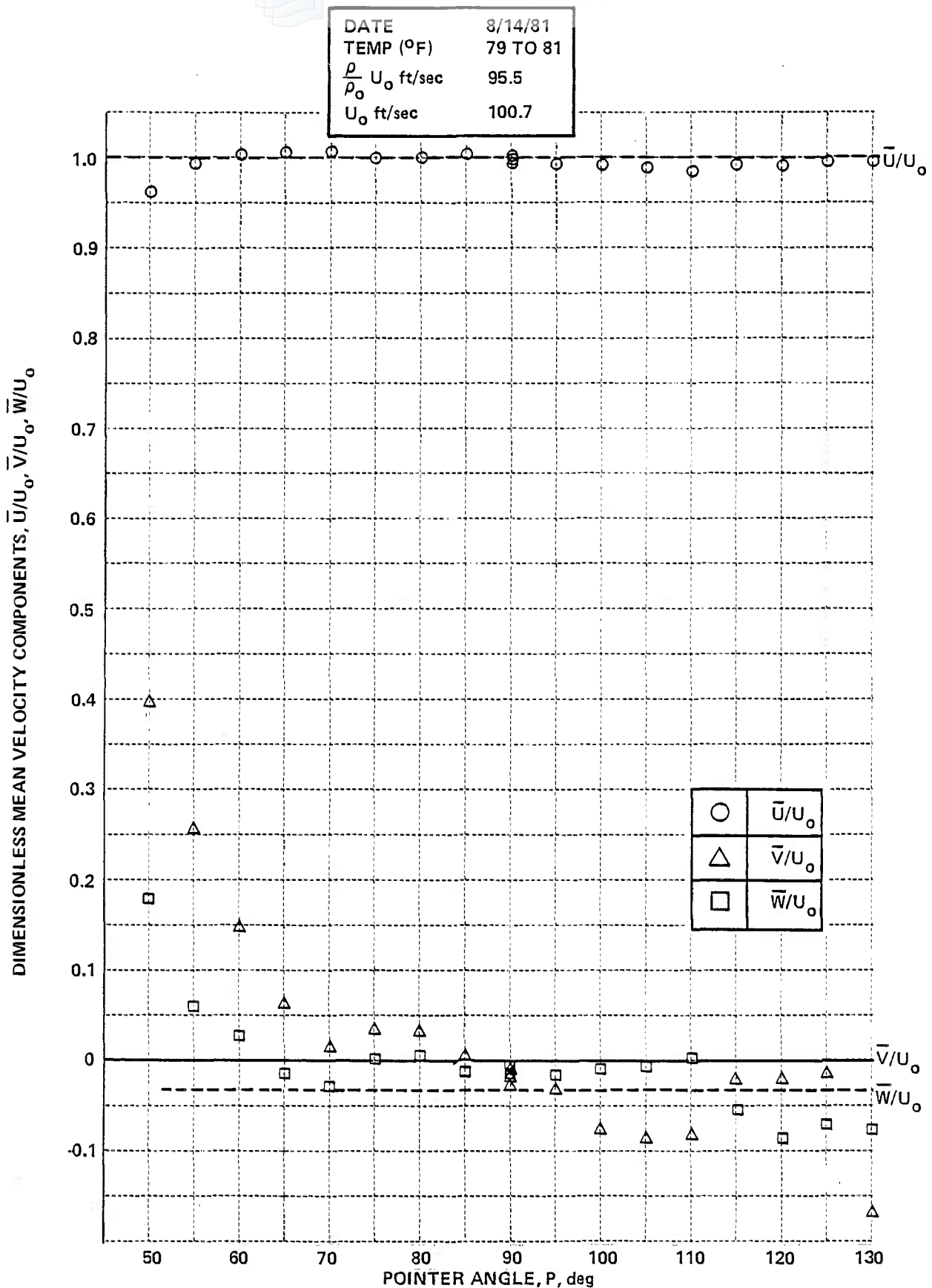
Figure A-8 (Cont.) TRIPLE PROBE ANGLE CALIBRATION CHECK, MEAN VELOCITY COMPONENTS
