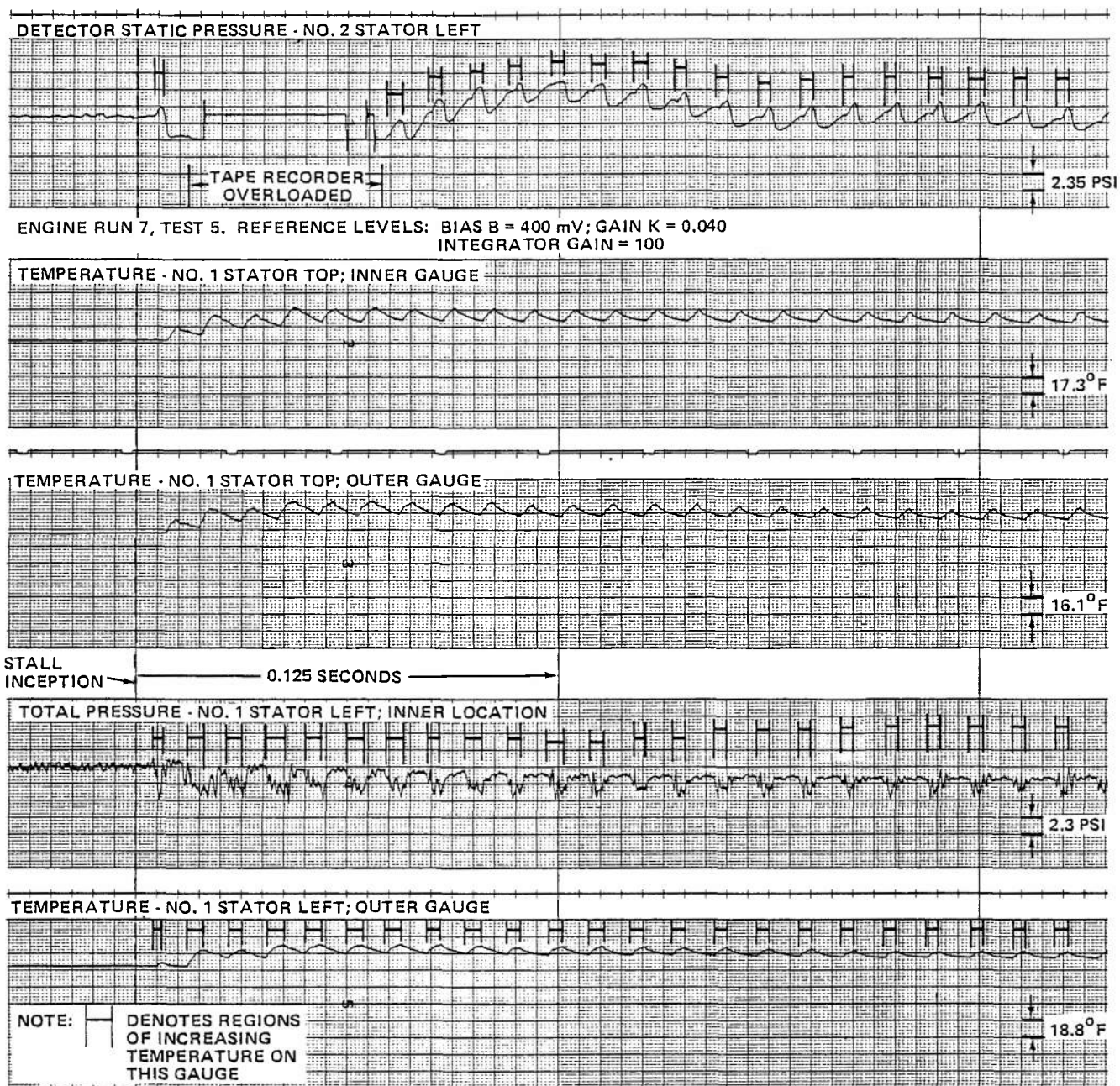
Figure 41 CORRELATION BETWEEN TEMPERATURE AND TOTAL PRESSURE FLUCTUATIONS IN J-85 COMPRESSOR DURING ROTATING STALL. CORRECTED ENGINE SPEED AT STALL INCEPTION, (N/N^* \sqrt{\theta}) = 74.6\%
