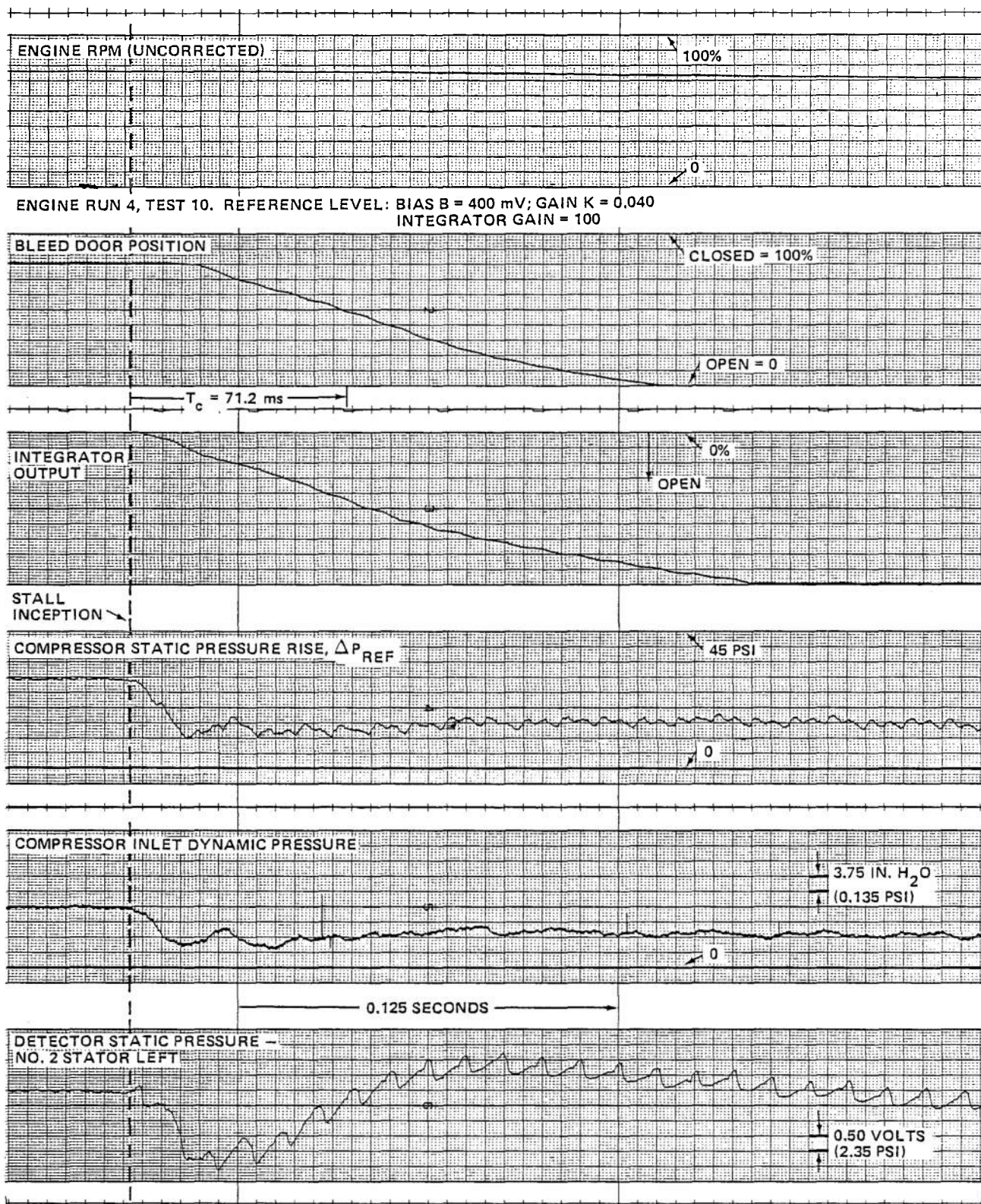
Figure 35 (Cont.) J-85 COMPRESSOR RESPONSE TO ROTATING STALL AT NOMINAL ENGINE SPEED OF 75% (EXPANDED TIME SCALE) d. INTEGRATOR GAIN = 100; CORRECTED ENGINE SPEED AT STALL INCEPTION, (N/N * \sqrt{\theta}) = 75.5\%
