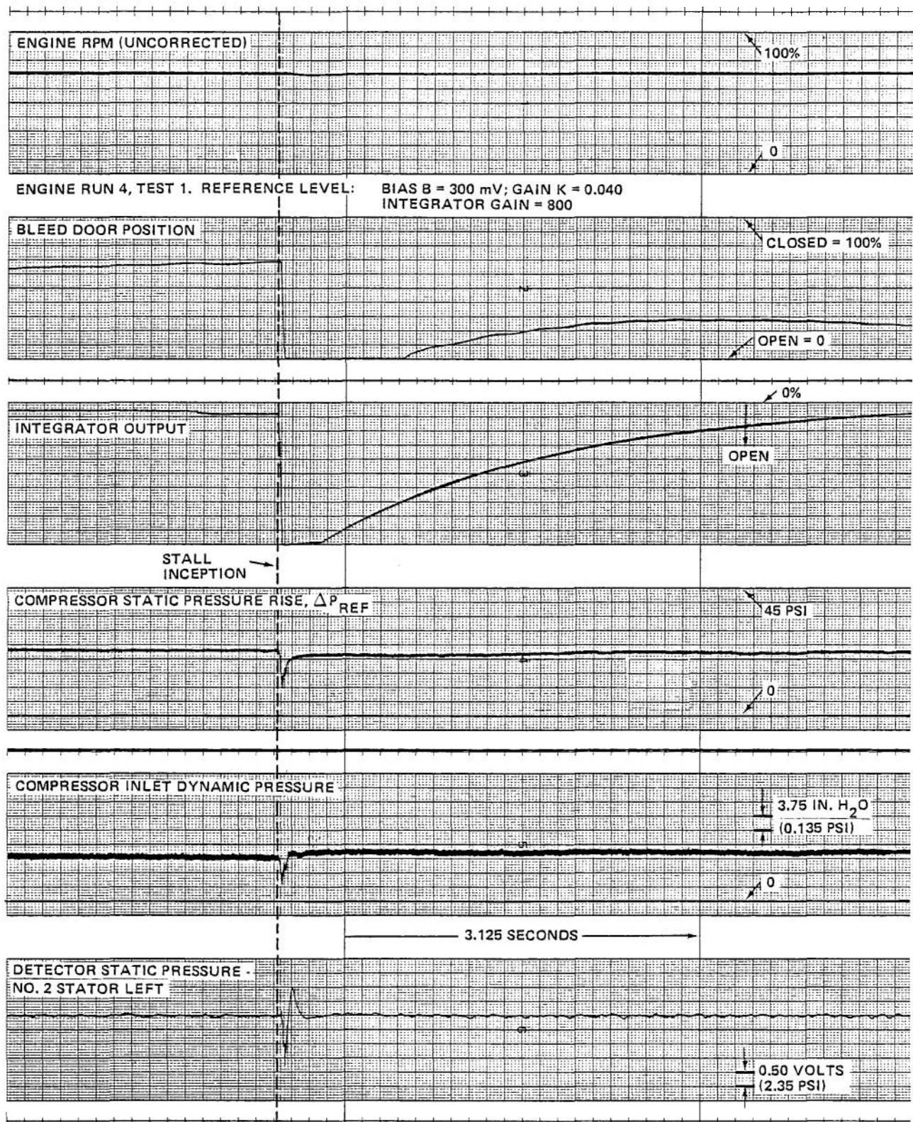
Figure 31 J-85 COMPRESSOR RESPONSE TO ROTATING STALL AT NOMINAL ENGINE SPEED OF 70%
