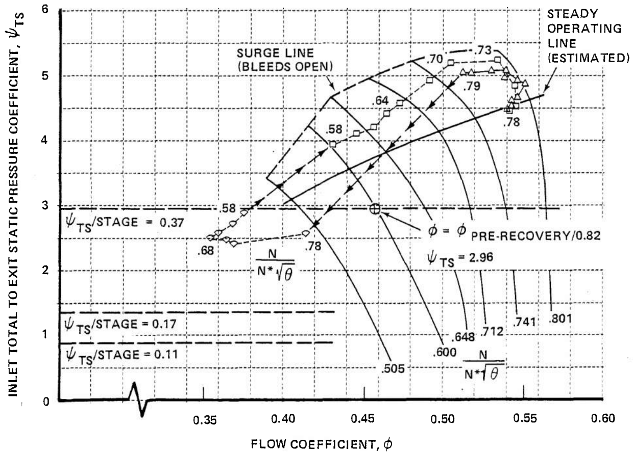
Figure 46 (Cont.) J85 POST-STALL BEHAVIOR
