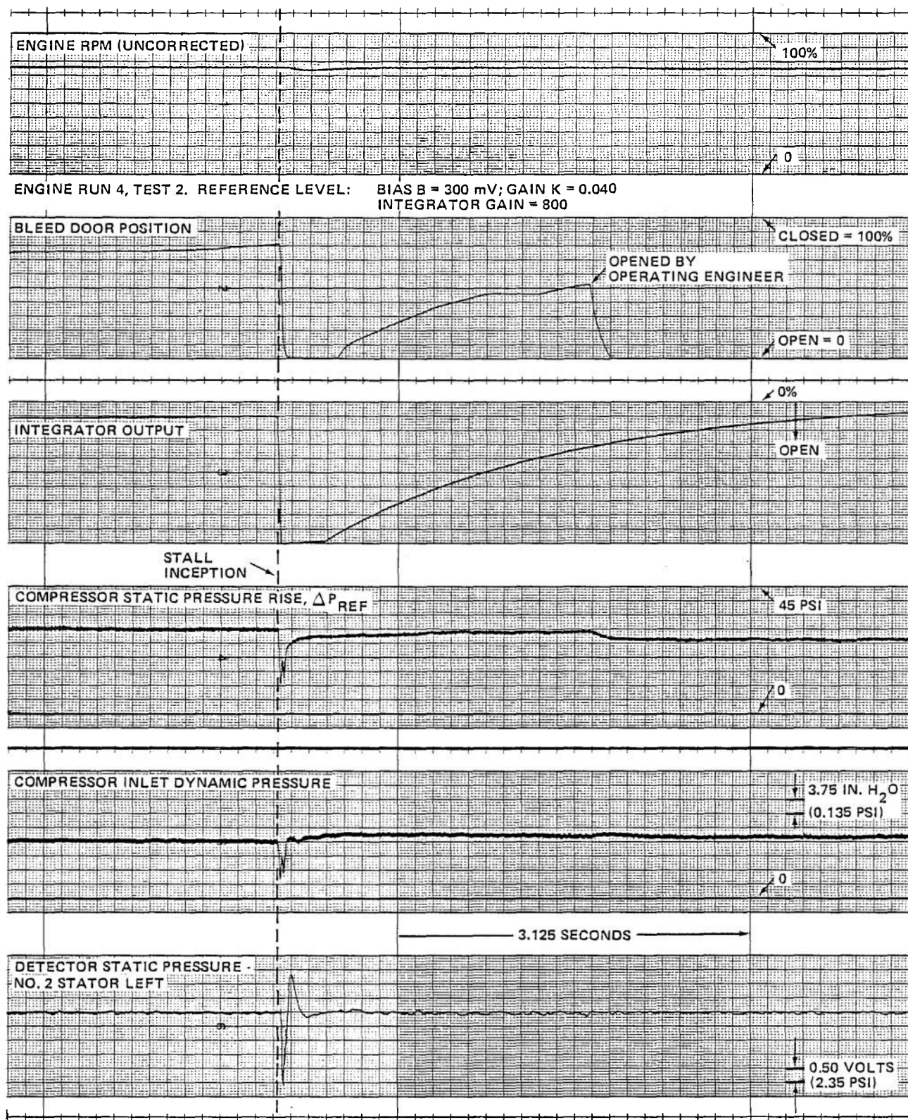
Figure 32 J-85 COMPRESSOR RESPONSE TO ROTATING STALL AT NOMINAL ENGINE SPEED OF 75%
