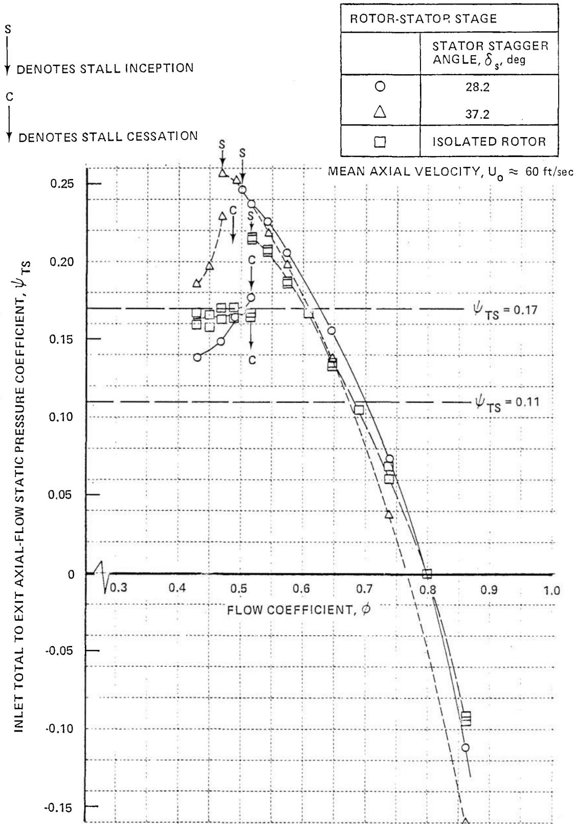
Figure 27 INLET TOTAL TO EXIT AXIAL-FLOW STATIC PRESSURE RISE PERFORMANCE OF HIGH HUB-TO-TIP RATIO ISOLATED ROTOR AND ROTOR-STATOR STAGE
