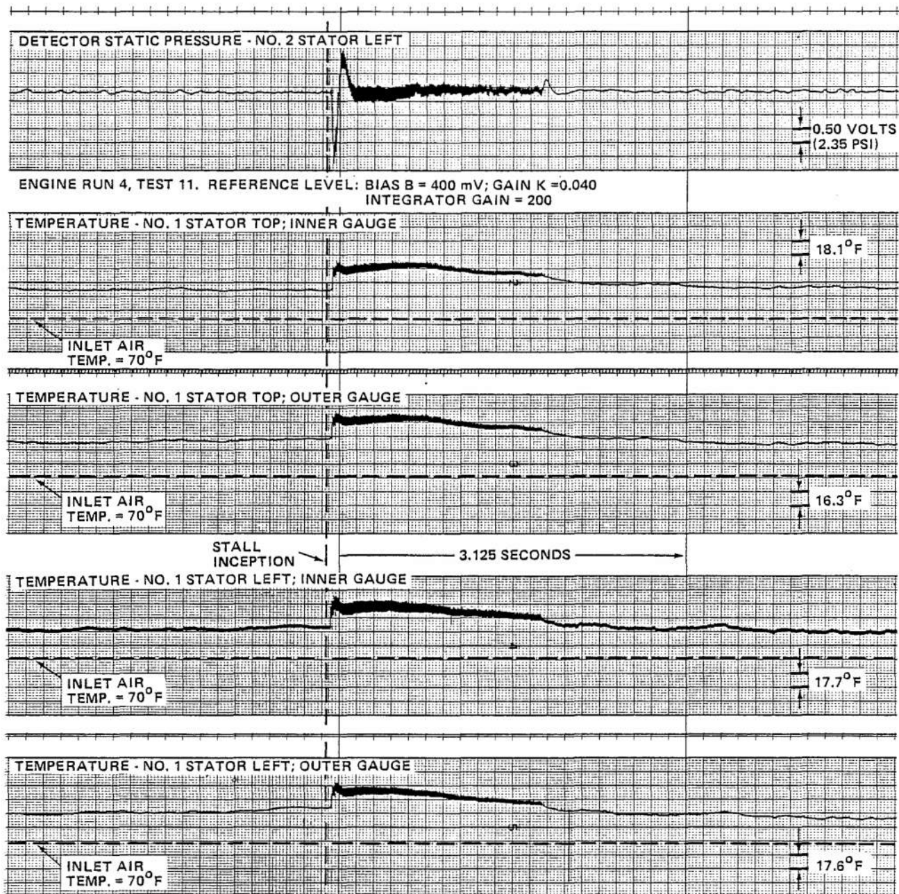
Figure 39 (Cont.) UNSTEADY TEMPERATURE MEASUREMENTS IN J-85 COMPRESSOR DURING ROTATING STALL c. CORRECTED ENGINE SPEED AT STALL INCEPTION; (N/N * \sqrt{\theta}) = 78.7\%
