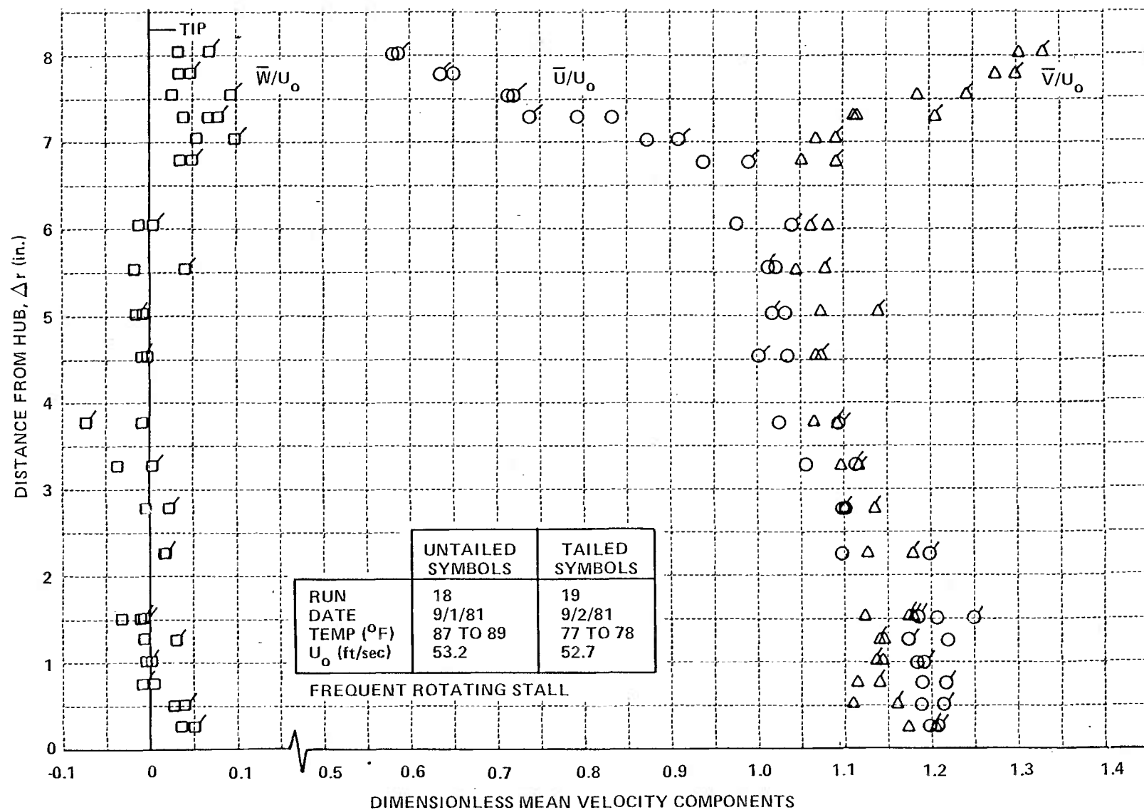
Figure 5 (Cont.) RADIAL DISTRIBUTIONS OF MEAN VELOCITY COMPONENTS DOWNSTREAM OF ISOLATED ROTOR g. ROTOR RPM = 1050
