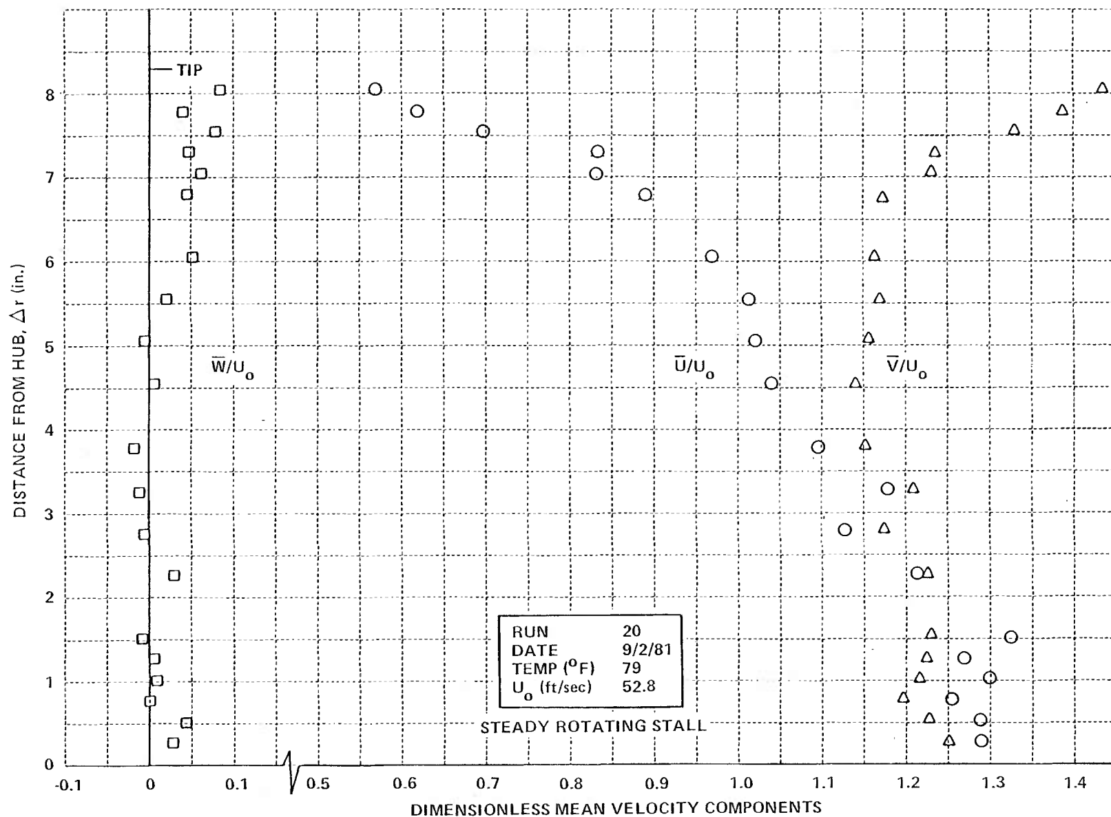
Figure 5 (Cont.) RADIAL DISTRIBUTIONS OF MEAN VELOCITY COMPONENTS DOWNSTREAM OF ISOLATED ROTOR h. ROTOR RPM = 1100
