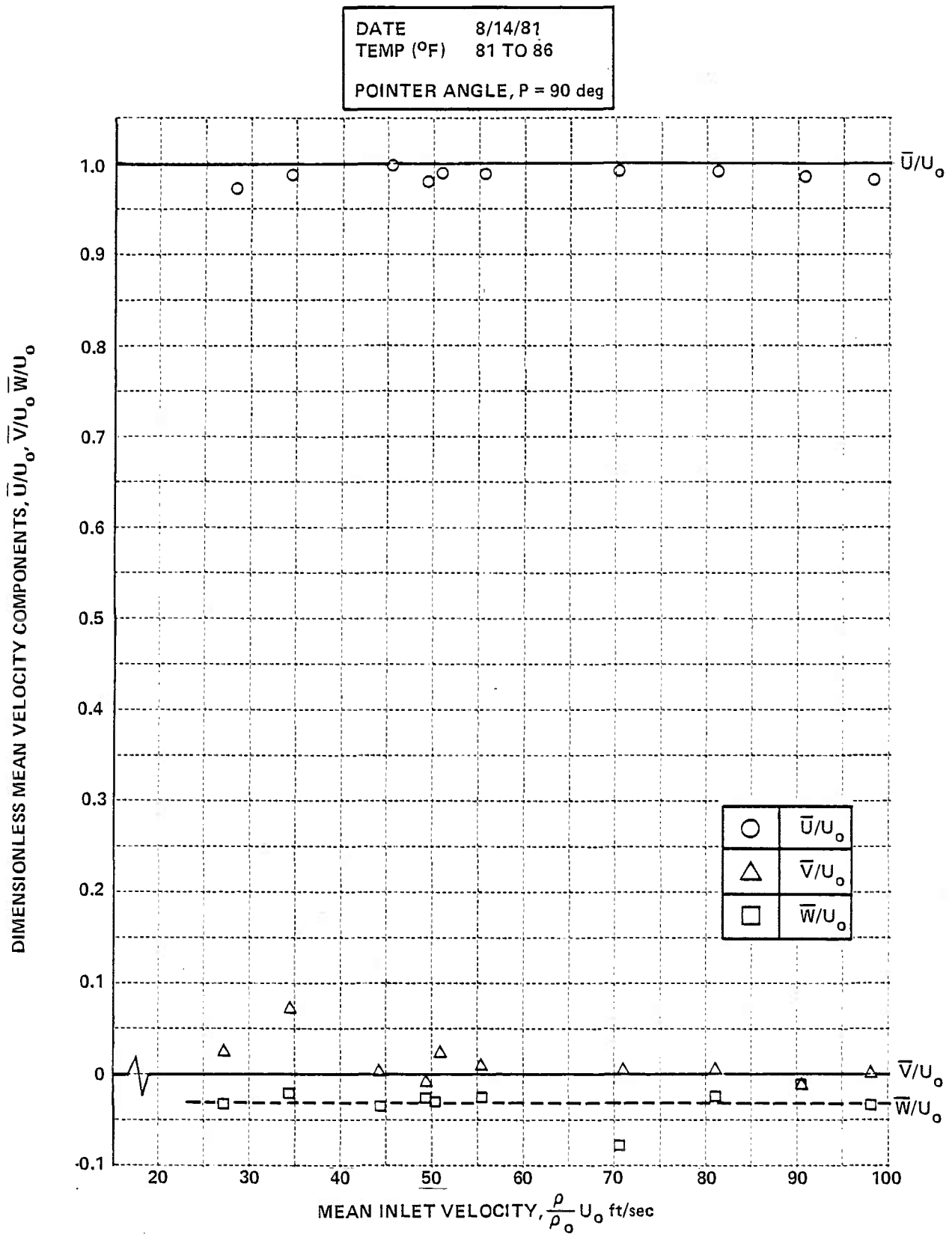
Figure A-7 TRIPLE PROBE VELOCITY CALIBRATION CHECK, MEAN VELOCITY COMPONENTS
