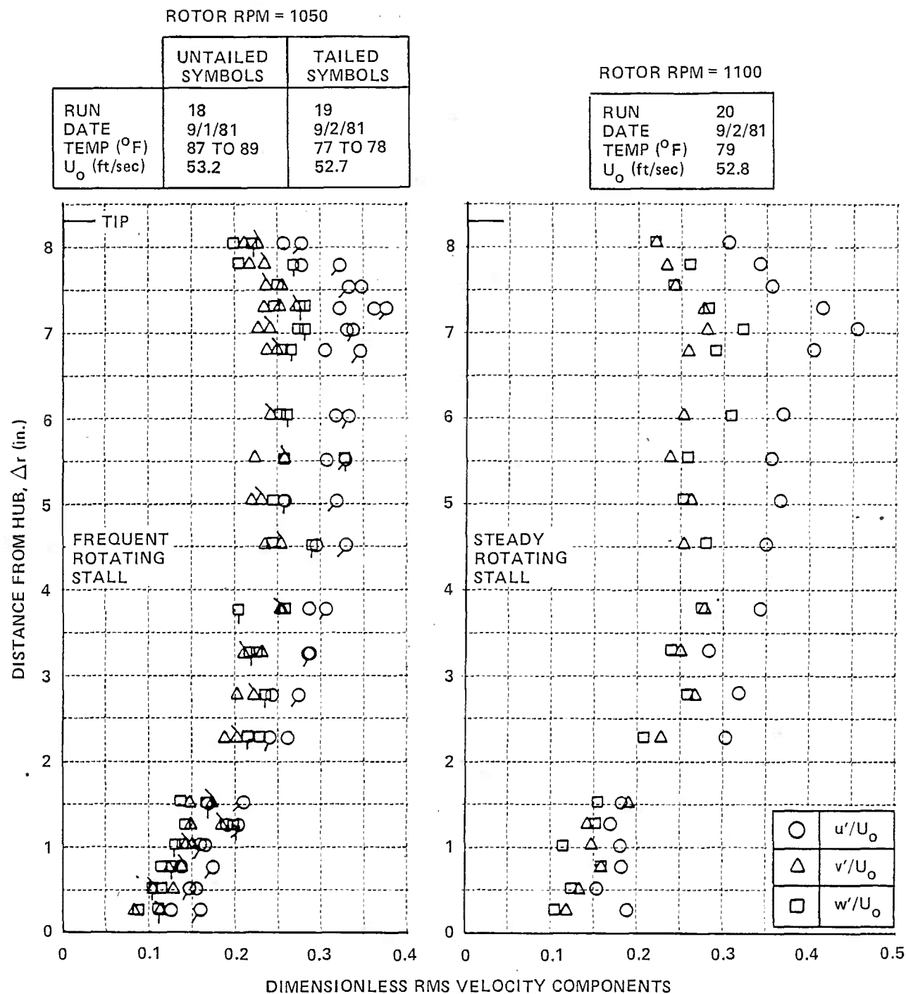
Figure 6 (Cont.) DIMENSIONLESS RMS VELOCITY COMPONENTS DOWNSTREAM OF ISOLATED ROTOR
