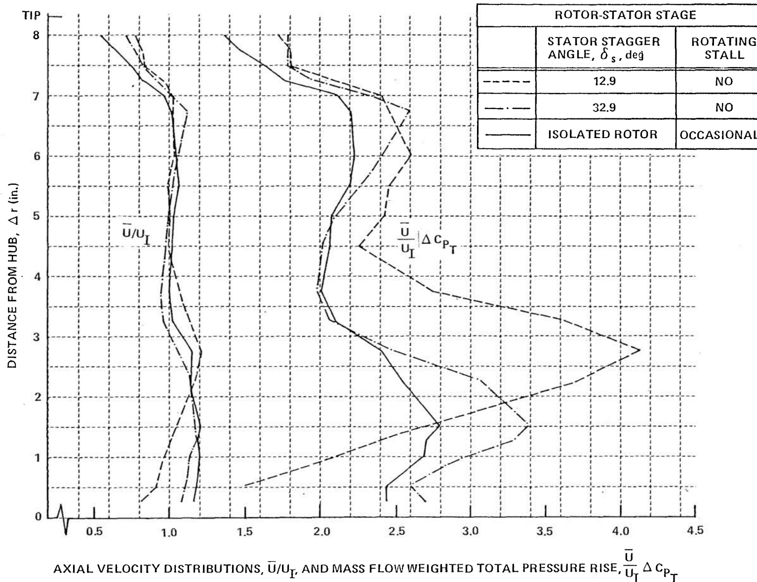
Figure 15 (Cont.) RADIAL DISTRIBUTIONS OF AXIAL VELOCITY AND MASS FLOW WEIGHTED TOTAL PRESSURE RISE DOWNSTREAM OF ISOLATED ROTOR AND THE SAME ROTOR IN A ROTOR-STATOR STAGE.
