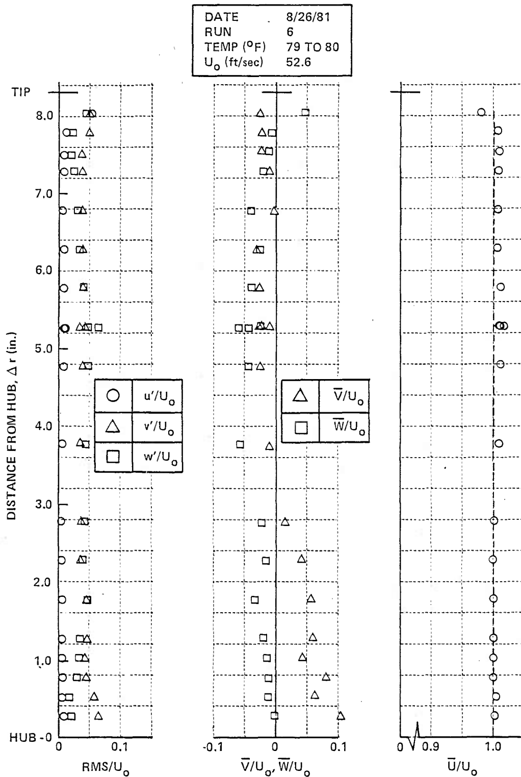
Figure 4 (Cont.) RADIAL DISTRIBUTIONS OF VELOCITY COMPONENTS FAR UPSTREAM OF ROTOR
