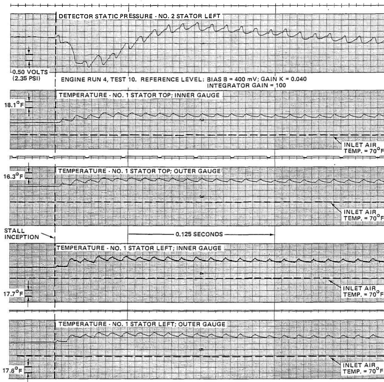
Figure 40 (Cont.) UNSTEADY TEMPERATURE MEASUREMENTS IN J-85 COMPRESSOR DURING ROTATING STALL (EXPANDED TIME SCALE) b. CORRECTED ENGINE SPEED AT STALL INCEPTION, (N/N * \sqrt{\theta}) = 75.5\%
