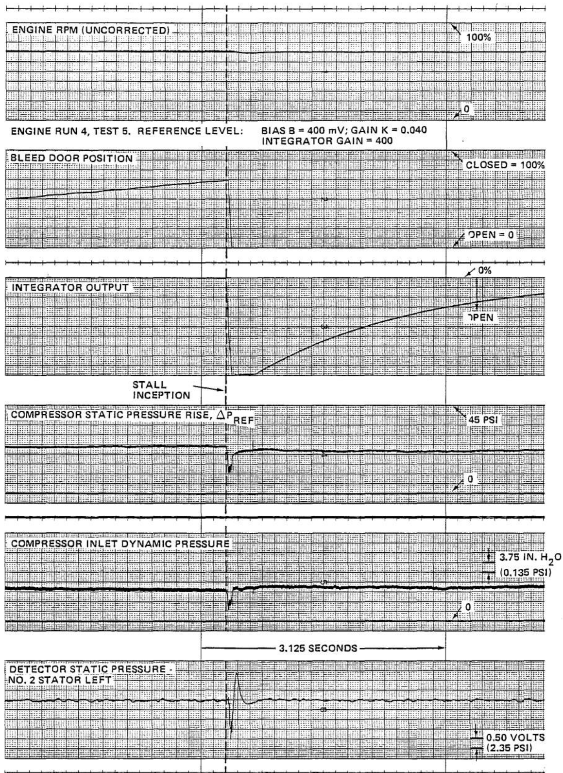
Figure 31 (Cont.) J-85 COMPRESSOR RESPONSE TO ROTATING STALL AT NOMINAL ENGINE SPEED OF 70%
