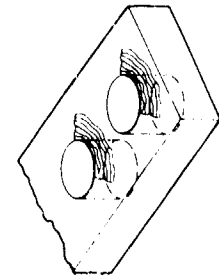
4 Bearing mode. Failure localized directly in front of bolt.
