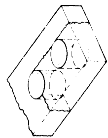
2 Tension-cleavage mode. Net section and shearout combination. Failure extends along shearout path and net section path.
