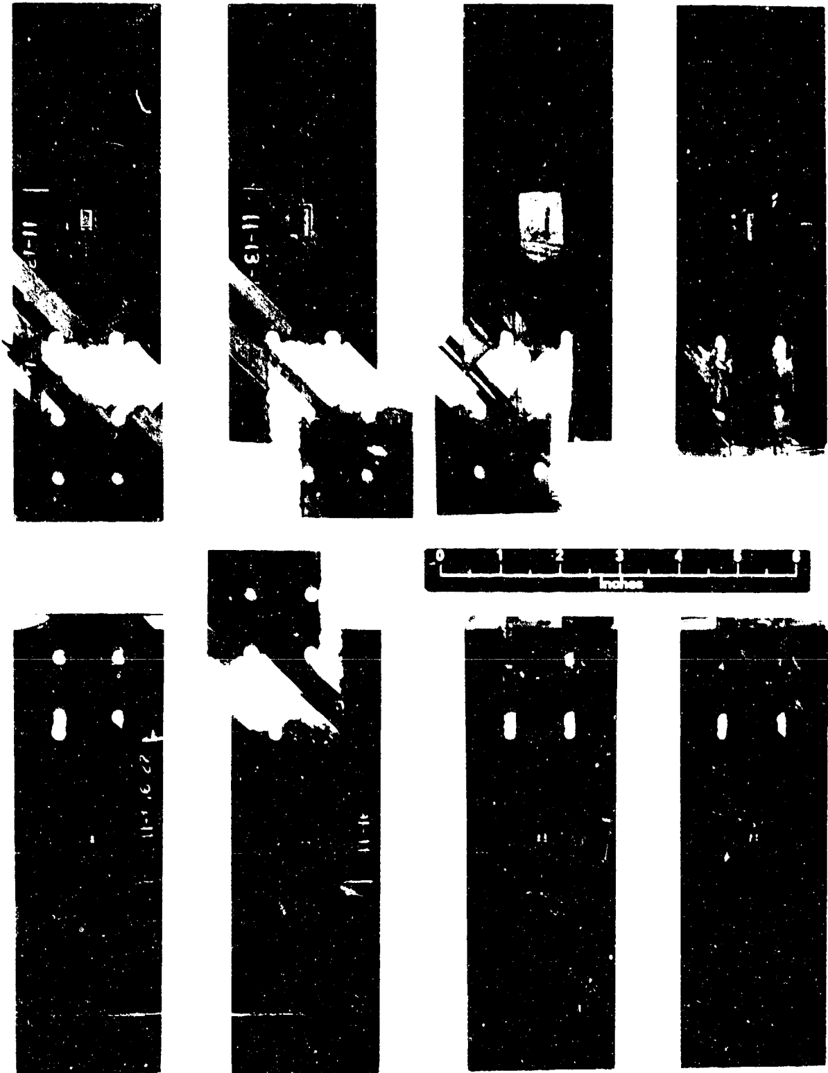
Figure 25. Fastener Pattern Tension Test Specimens After Testing
