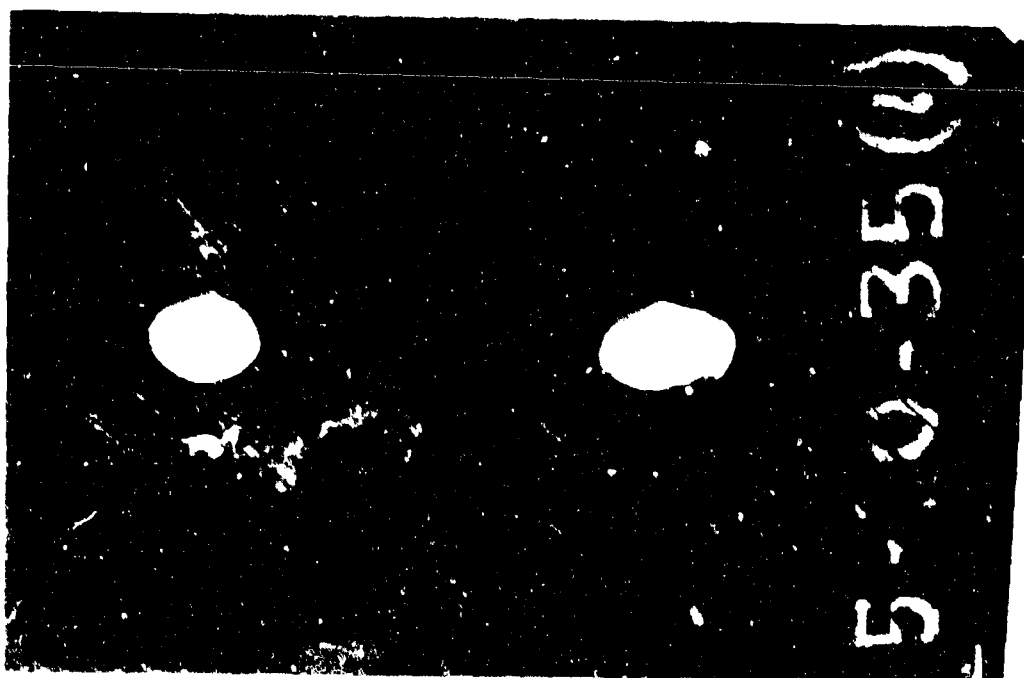
Tilted Countersink - Away from Bearing Surface
