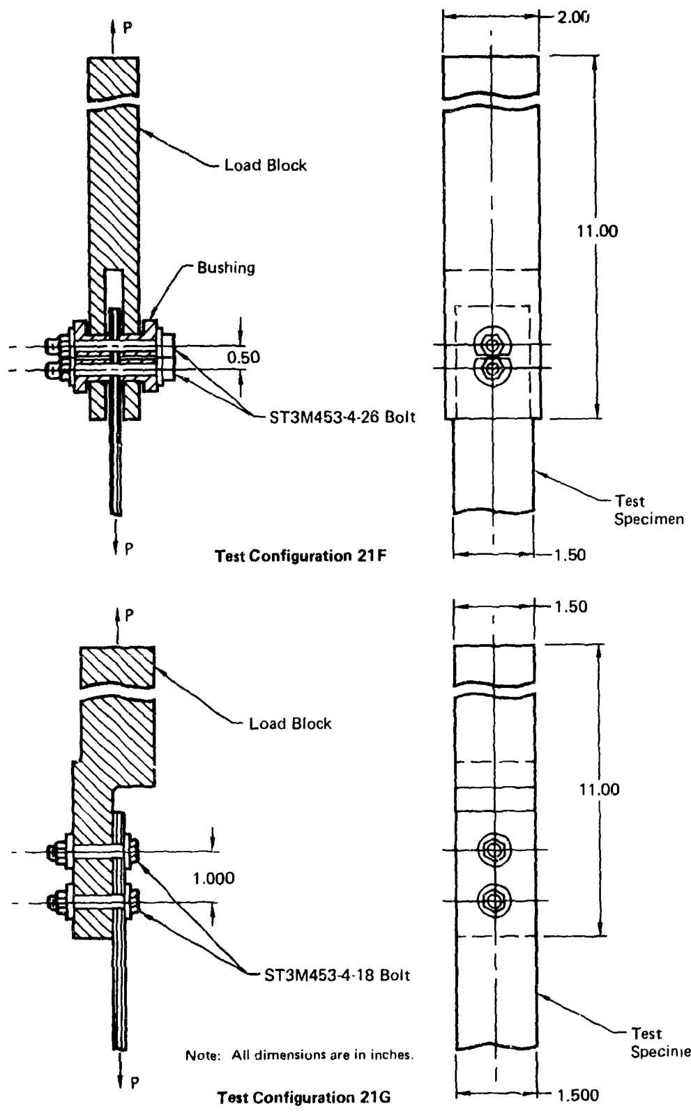
Figure 21. (Continued) Multiple Fastener Test Setups
