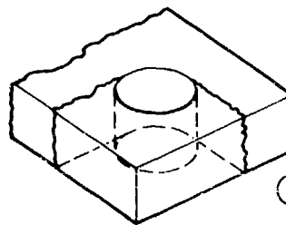
① Shearout mode 0° and 90° plies "pushed" out in front of bolt hole
