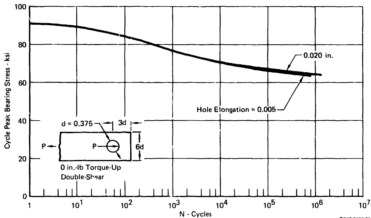
Figure 120. Effect of Stacking Sequence - Hole Elongation Levels 50/40/10 Layup
