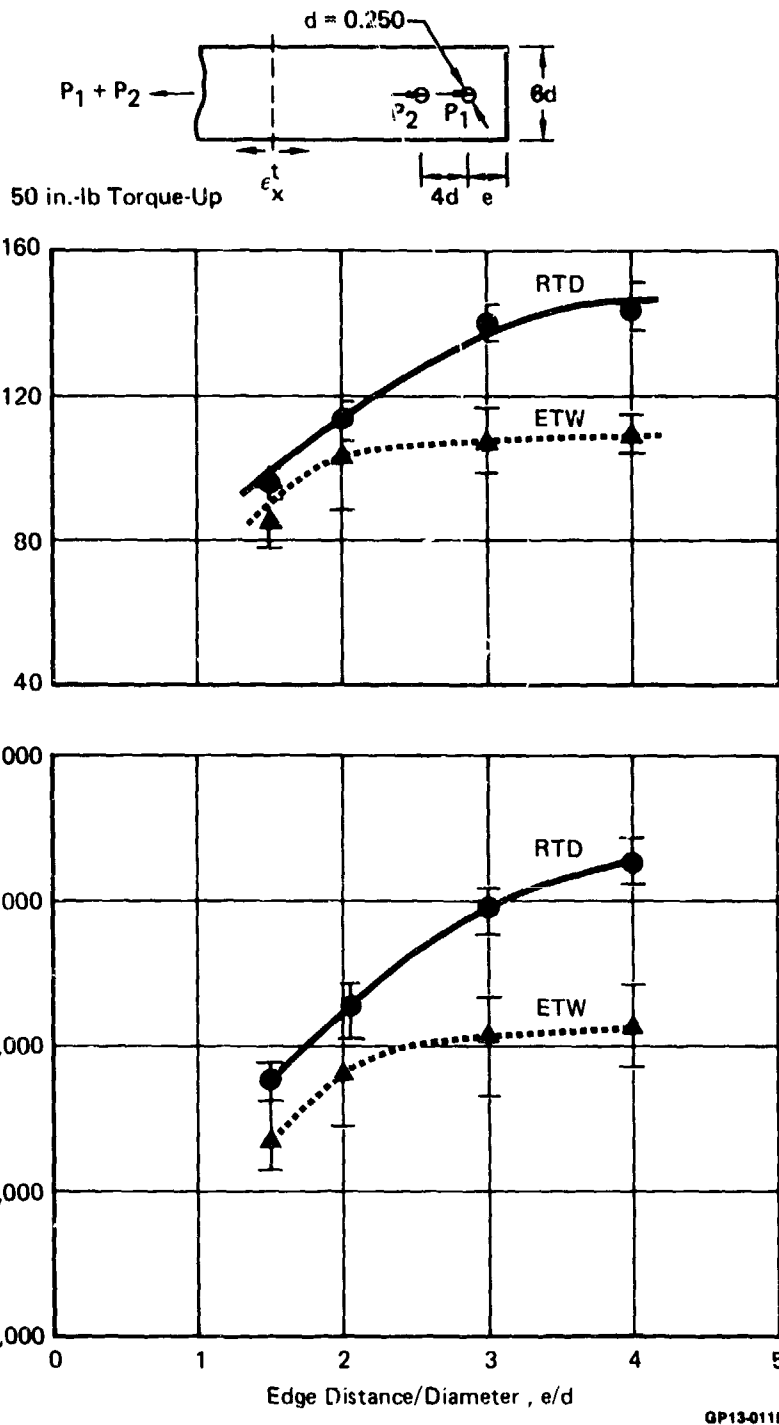
Figure 47. Effect of Edge Distance on Joint Tensile Strength
