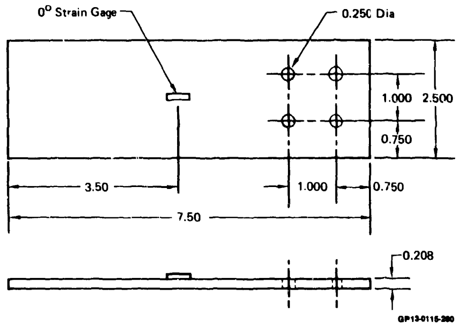
Figure 41. Fastener Pattern Specimen Geometry
