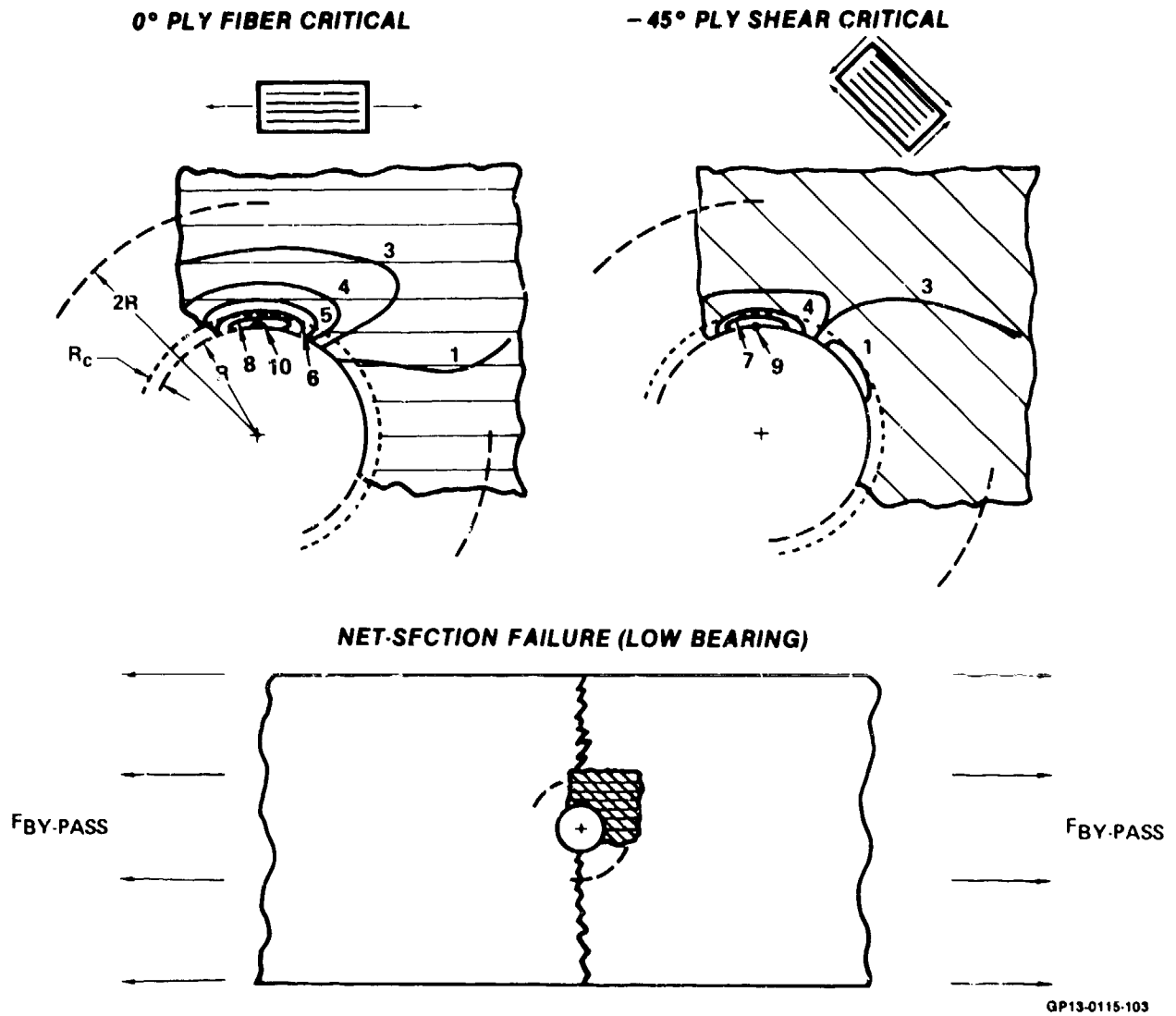
Figure 58. Predicted Critical Plies for Net-Section Failures
