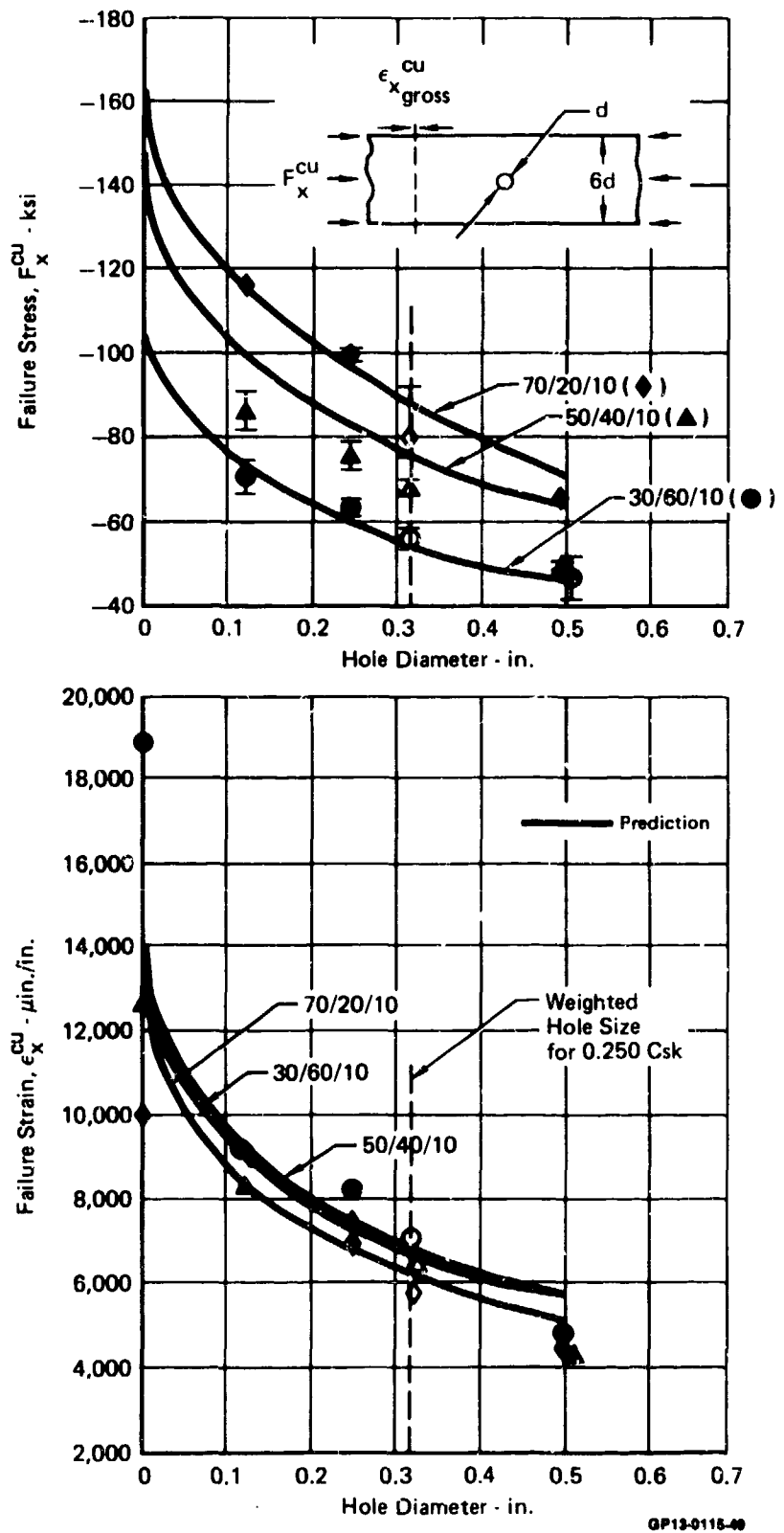
Figure 34. Effect of Hole Size on Unloaded Hole Compressive Strength
