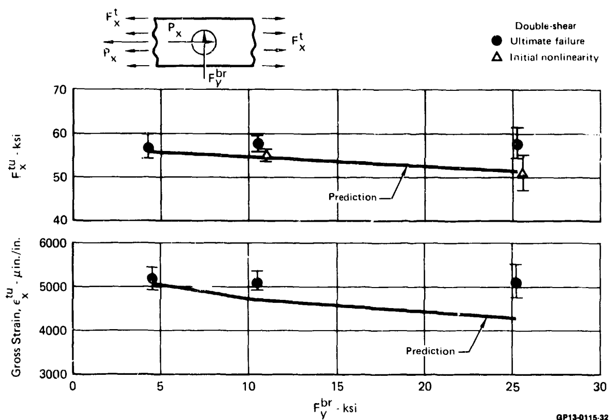
Figure 62. Effect of Off-Axis Bearing Loads on Bypass Strength
