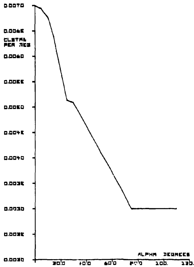
Figure 6. C_{L_{stab}}(\alpha)
