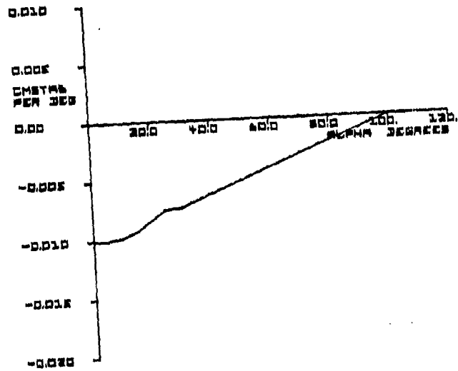
Figure 20. C_{m_{bstab}} (\alpha)
