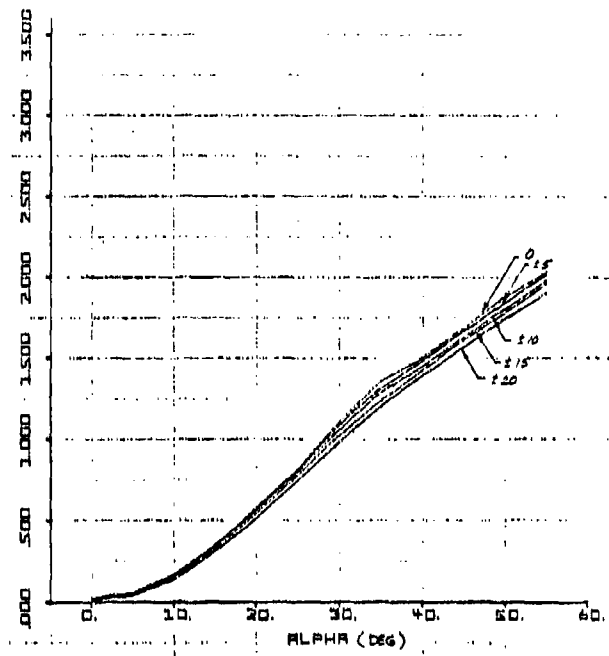
Figure 40. C_{DBASIC}(\alpha, \beta)
