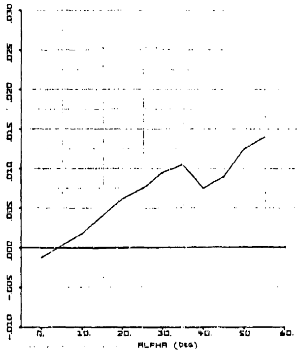
Figure 42. CD_{\delta s_1}(\alpha) - 1/\text{deg}
