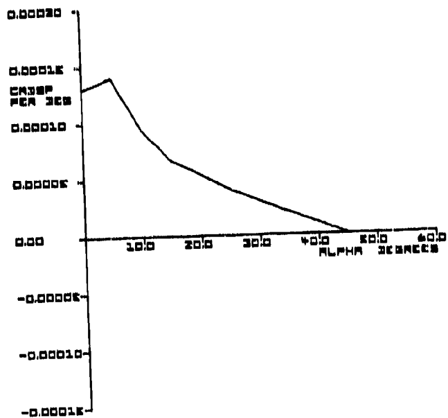
Figure 14. C_{l\delta_{sp}}(\alpha)
