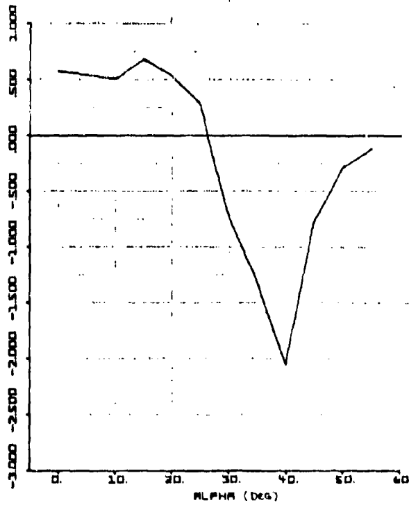
Figure 47. C_{Yr}(\alpha) - 1/\text{rad}
