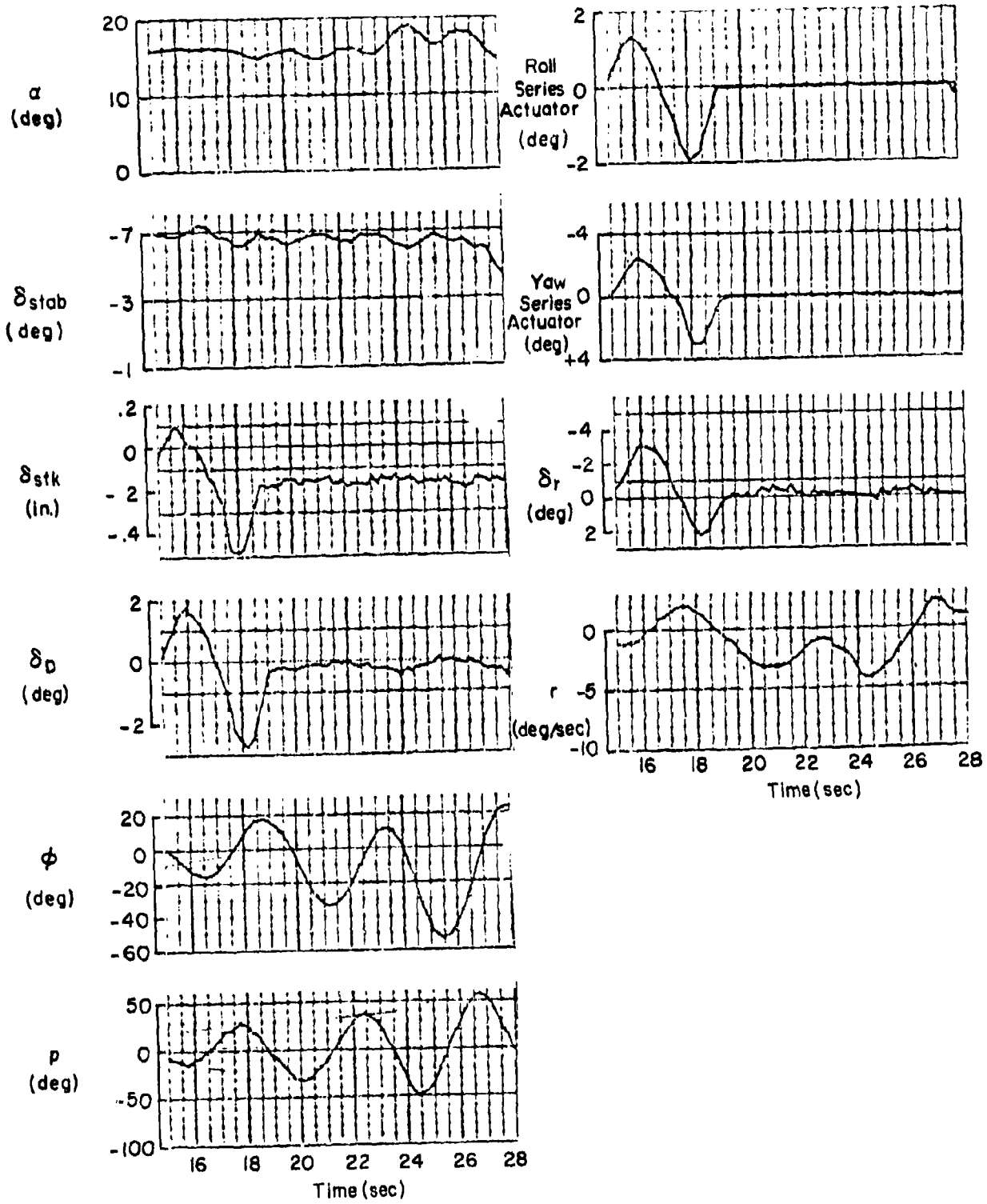
Figure 78. Flight 234-1 Traces
