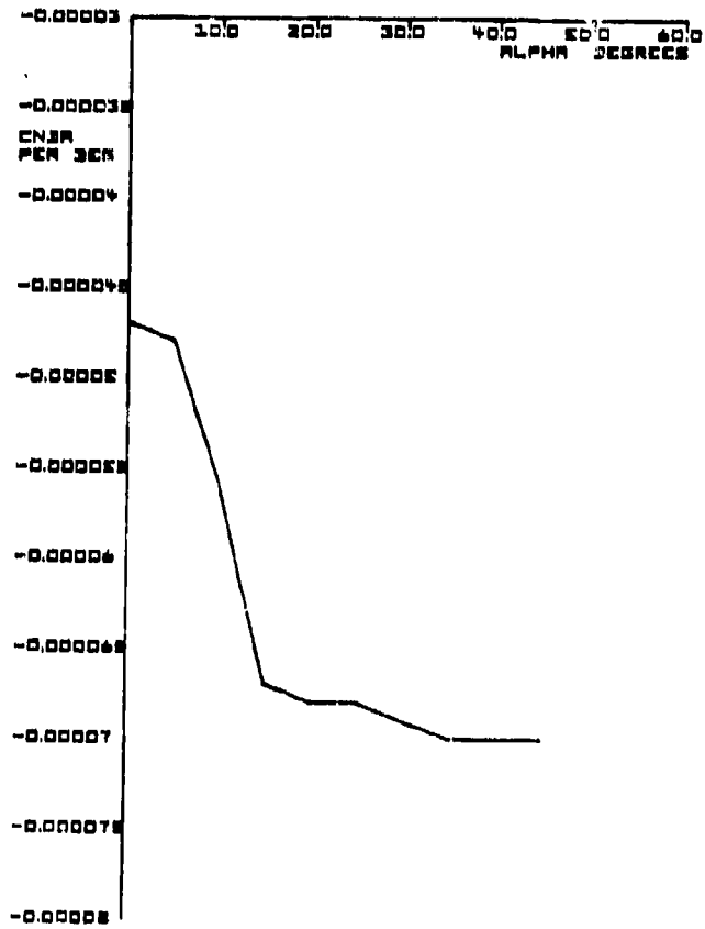
Figure 26. C_{n\delta_a}(\alpha)
