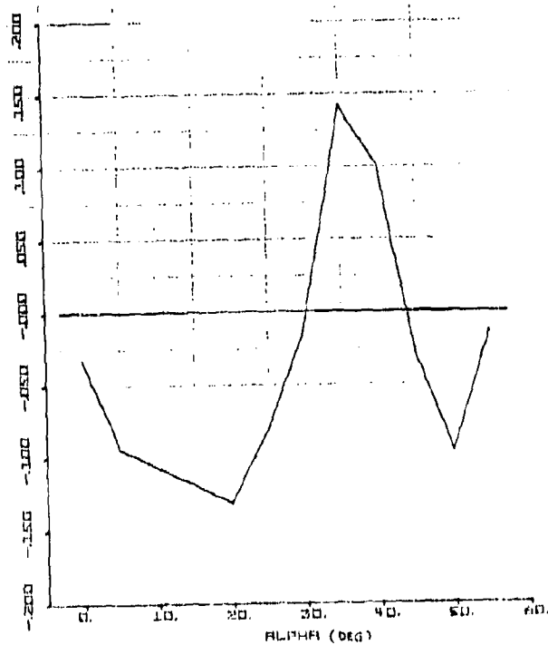
Figure 67. Cn_{\beta}(\alpha) - 1/\text{rad}
