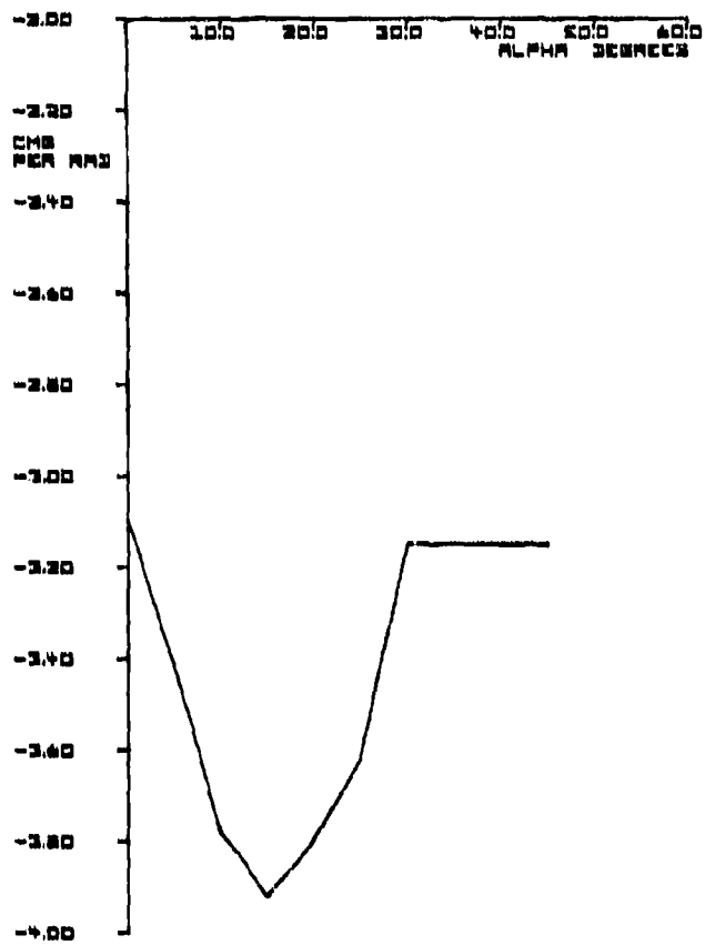
Figure 18. C_{m_2}(\alpha)
