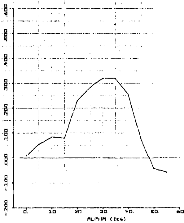
Figure 59. C_{lr}(\alpha) - 1/\text{rad}
