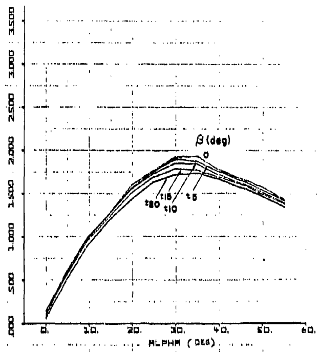
Figure 36. C_{LBASIC}(\alpha, \beta)
