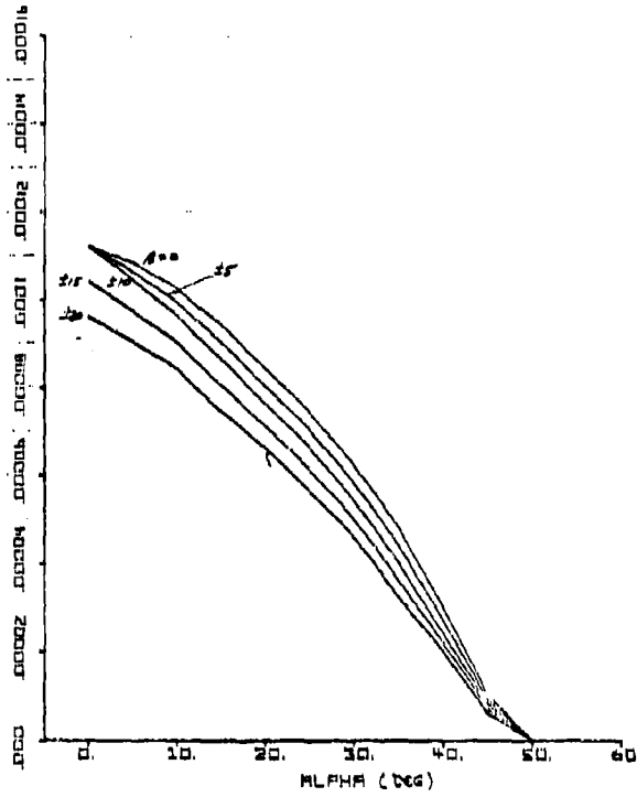
Figure 62. C_{l\beta}(\alpha, \beta) - 1/\text{deg}
