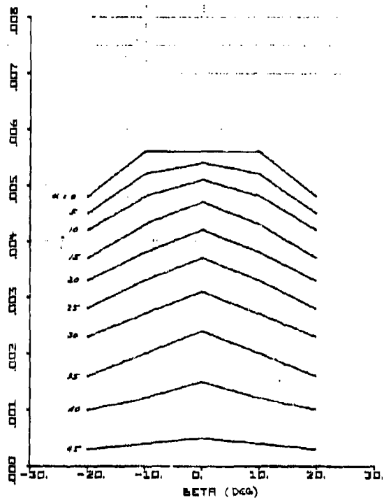
Figure 50. CY_{Dr}(\alpha, \beta) - 1/deg
