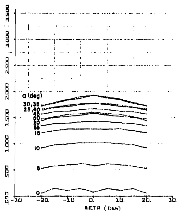
Figure 37. C_{LBASIC}(\alpha, \beta)
