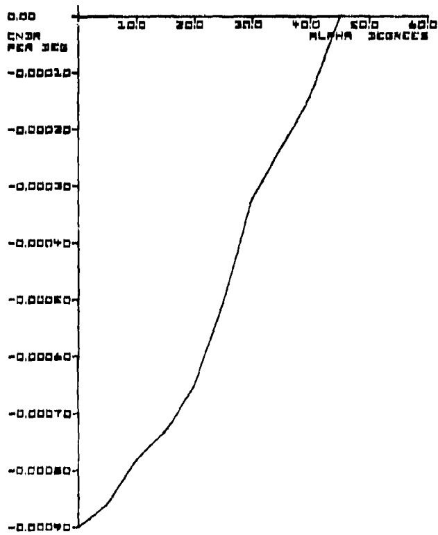
Figure 28. C_{n\delta_r} (\alpha)
