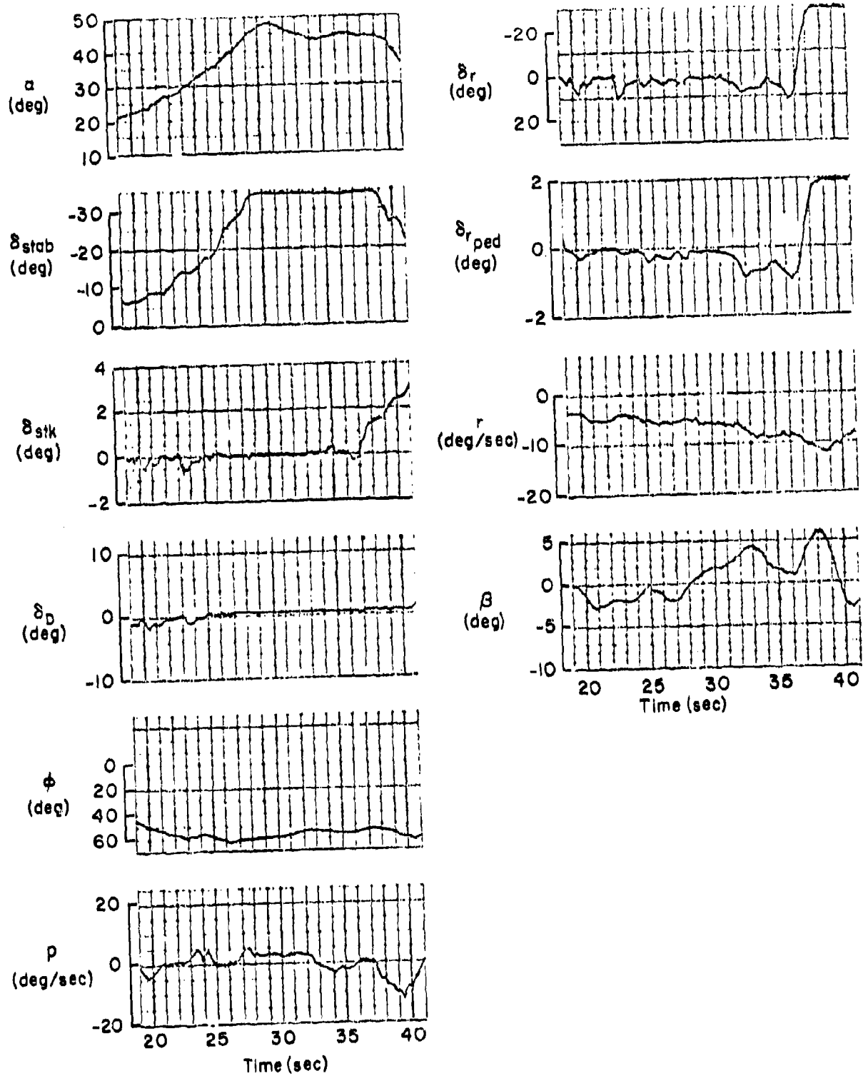
Figure 84. Flight 230-6 Traces
