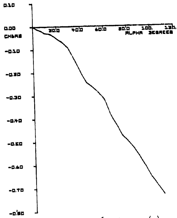
Figure 16. C_{m_{BASIC}} ( \alpha )
