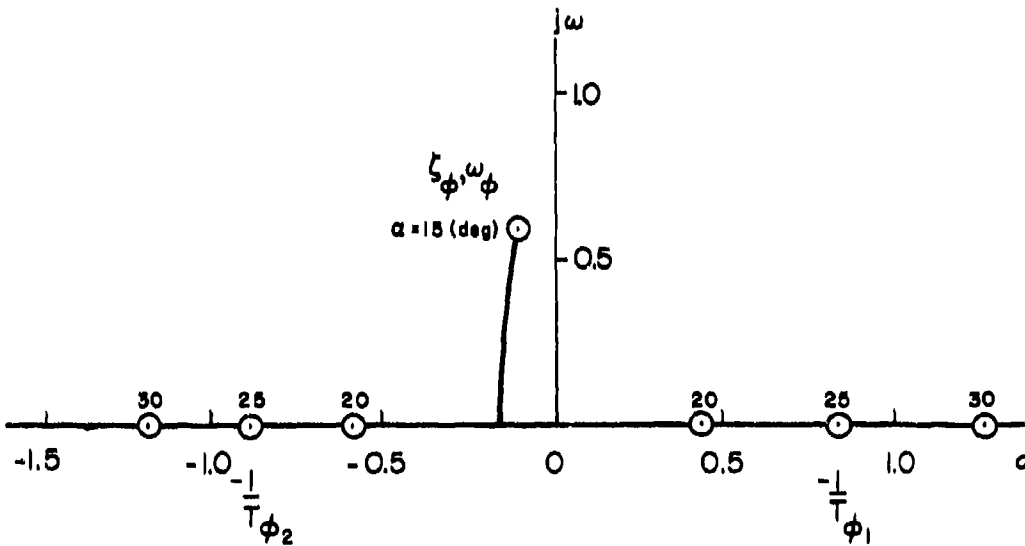
Figure 85. Migration of N_{\delta_a}^\phi Zeros With Angle of Attack, \beta_0 = 0
