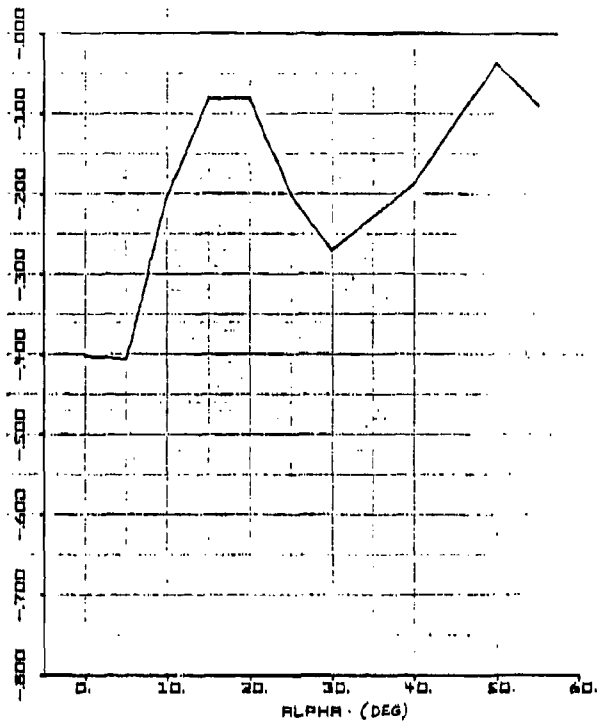
Figure 58. C_{lp}(\alpha) - 1/\text{rad}
