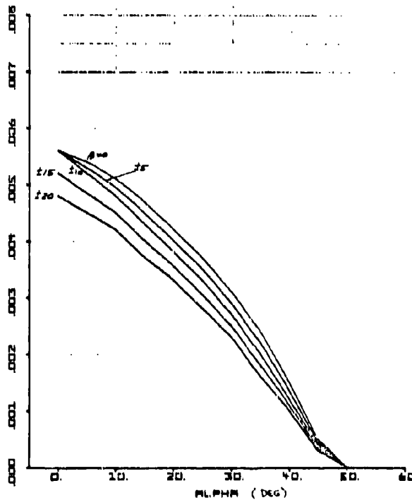
Figure 49. CY_{\Delta B r}(\alpha, \beta) - 1/\text{deg}
