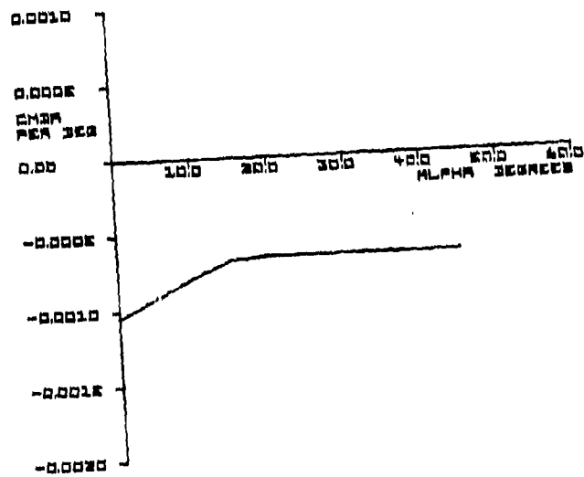
Figure 21. C_{m_{BA}} (\alpha)
