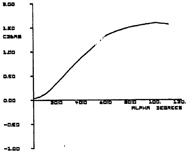
Figure 7. C_{D\text{BASIC}}(\alpha)
