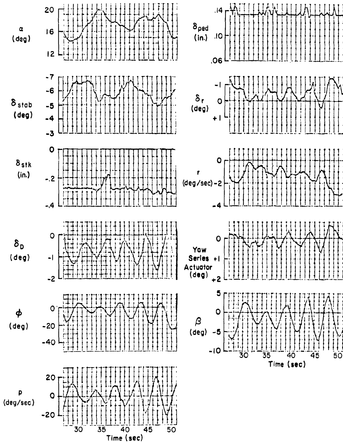
Figure 75. Flight 243 Traces
