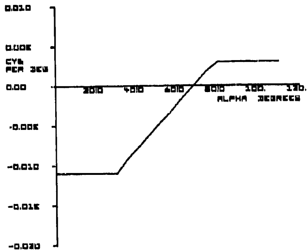
Figure 8. C_{y_p}(\alpha)
