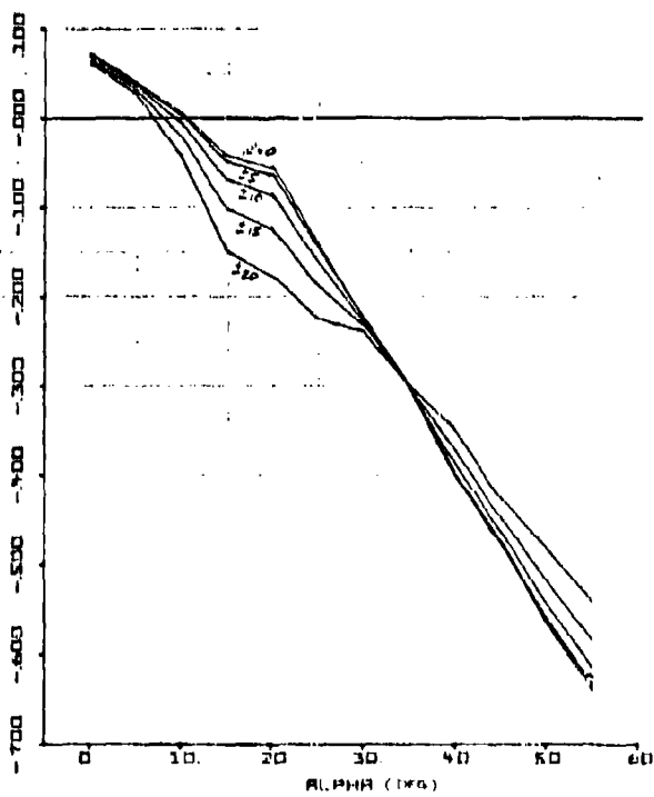
Figure 51. Cm_{BASIC}(\alpha, \beta)
