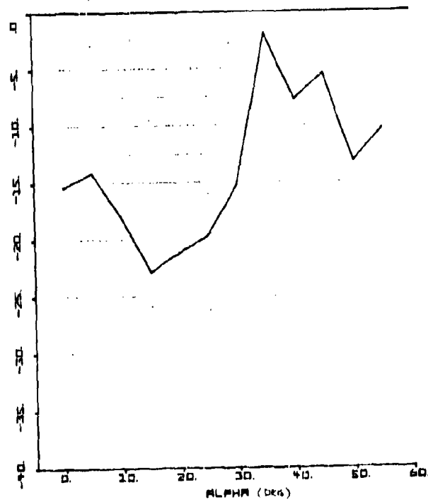
Figure 53. C_{m\_q}(\alpha) - 1/\text{rad}
