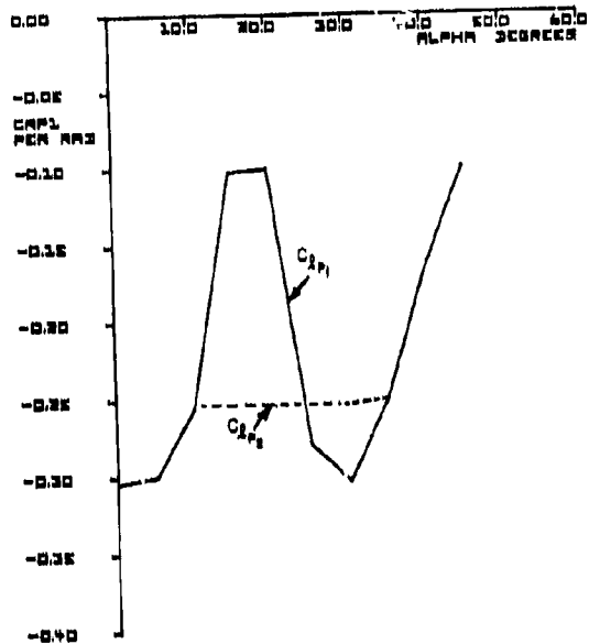
Figure 11. C_{dp}(\alpha)
