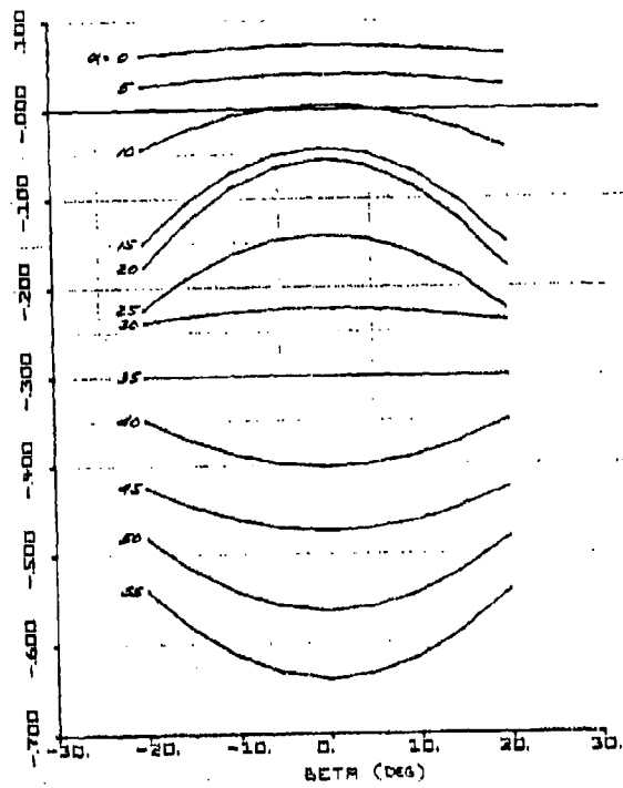
Figure 52. C_{m\_BASIC}(\alpha, \beta)
