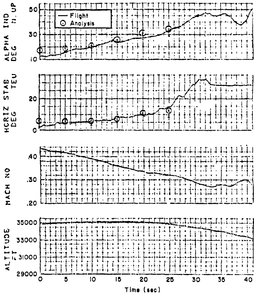
Figure 74. Flight 199 Traces
