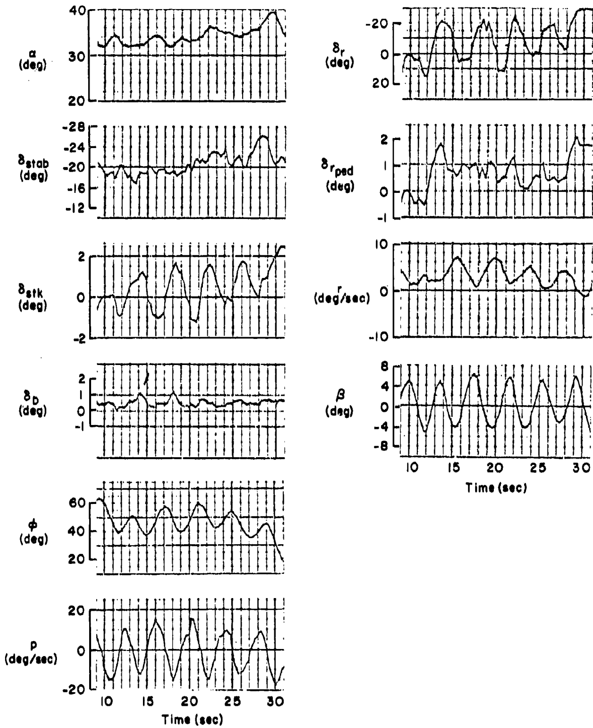
Figure 82. Flight 230-5 Traces
