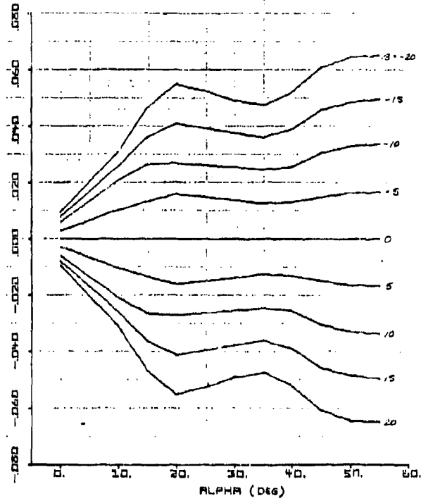
Figure 56. C_L BASIC( \alpha, \beta ) - 1/deg
