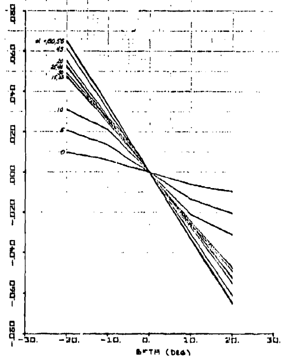
Figure 57. C_L BASIC( \alpha, \beta )
