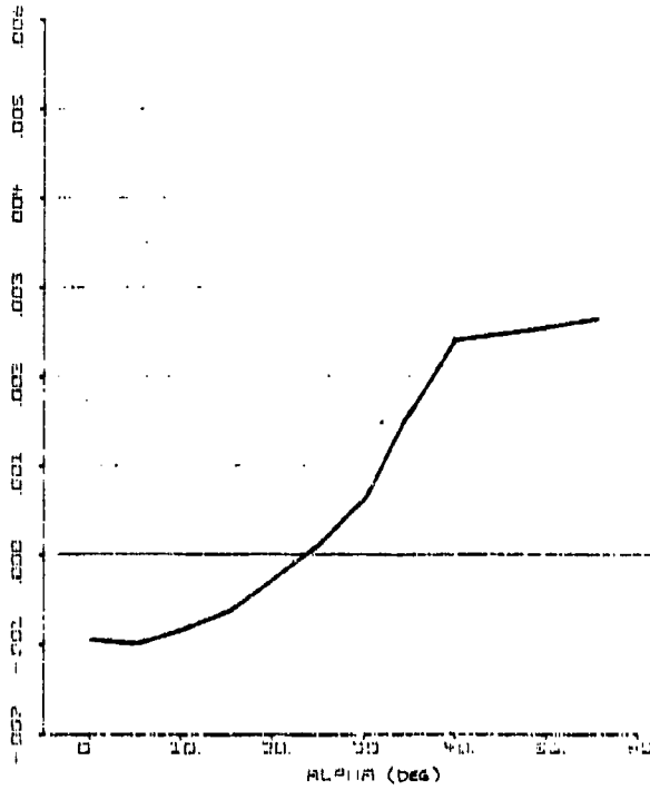
Figure 48. CY_{\Delta B A}(\alpha) - 1/\text{deg}
