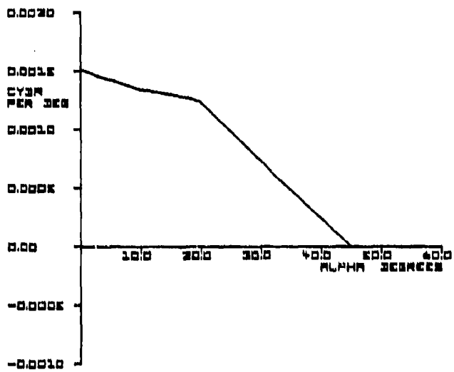
Figure 9. C_{Y\beta_r}(\alpha)
