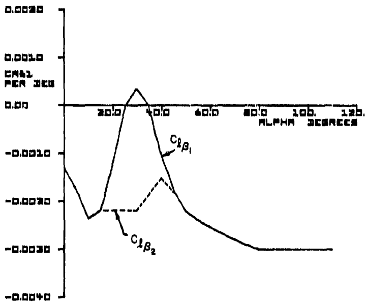
Figure 10. C_{L\beta}(\alpha)
