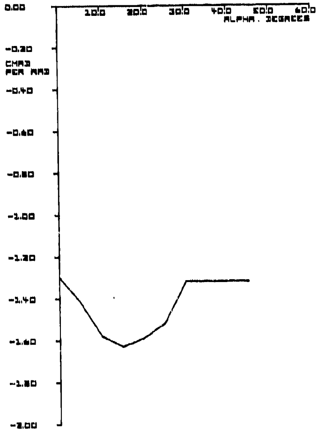
Figure 19. C_{m\alpha}(\alpha)
