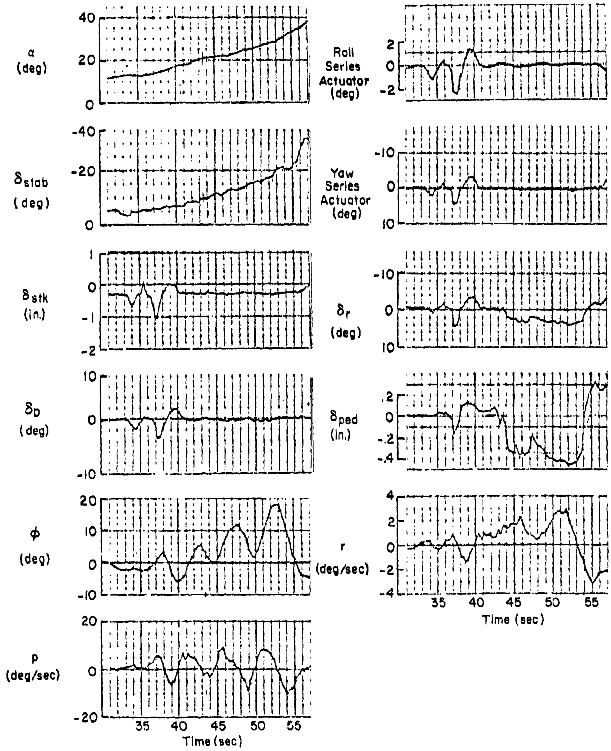
Figure 80. Flight 236-1 Traces
