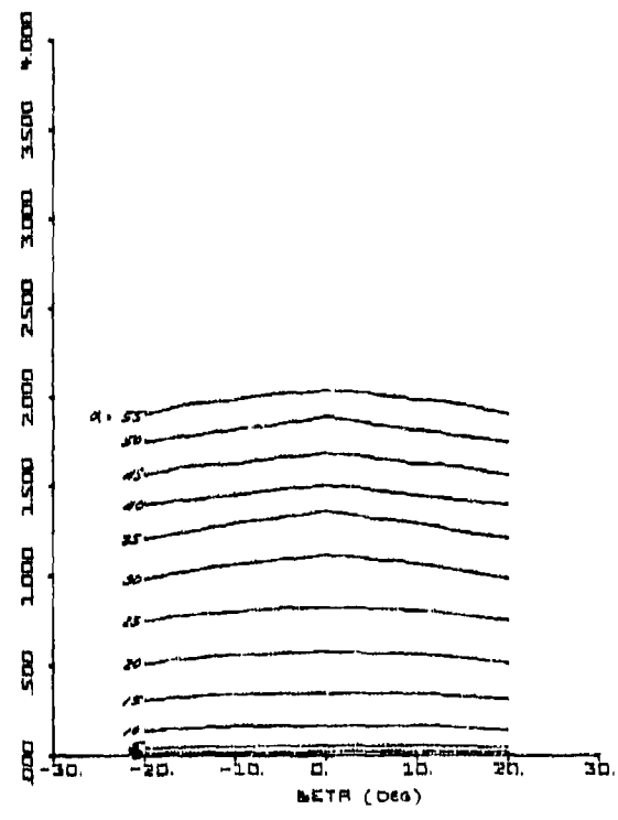
Figure 41. C_{DBASIC}(\alpha, \beta)
