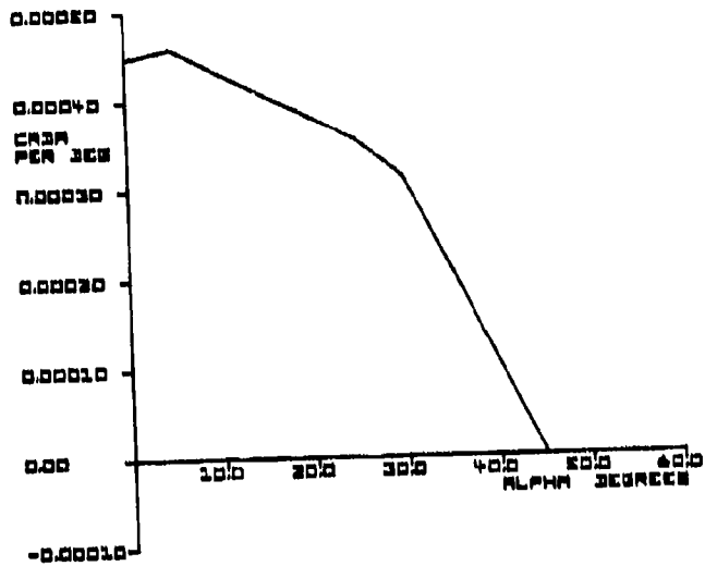
Figure 13. C_{l\delta_a}(\alpha)
