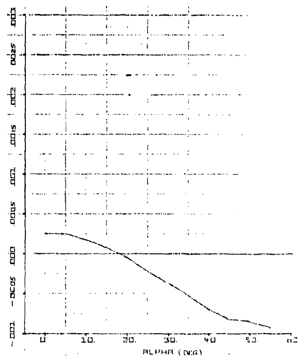
Figure 69. C_{n\delta_1}(\alpha) - 1/\text{deg}
