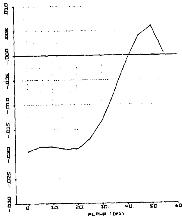
Figure 55. C_{m\delta\beta_2}(\alpha) - 1/\text{deg}
