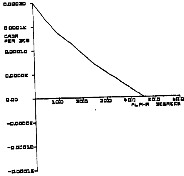
Figure 15. C_{L_{\alpha}} ( \alpha )
