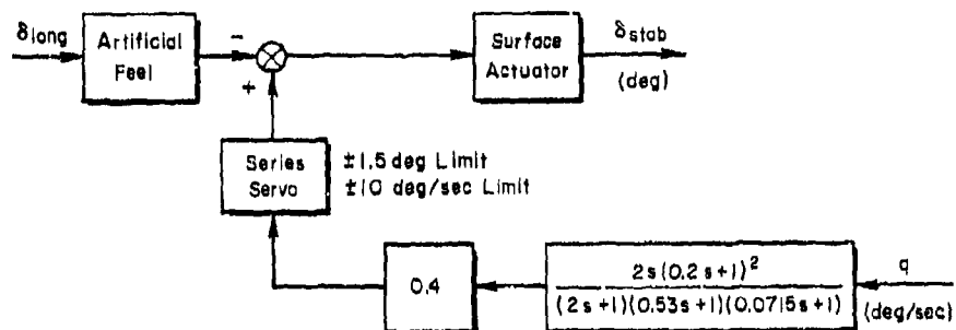
Figure 26. F-14A Longitudinal Control System
