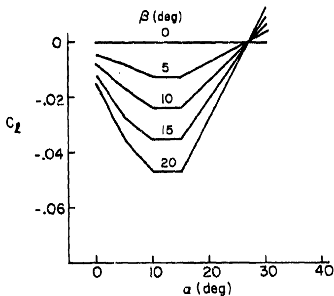
Figure 7. F-4J Roll Coefficient Variation with \alpha , \beta
