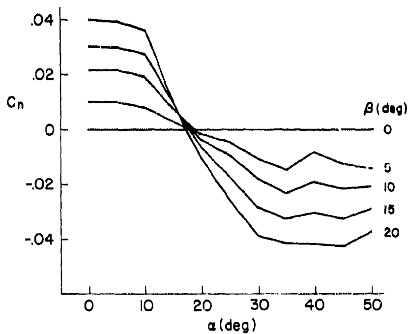
Figure 24. F-14A Yaw Coefficient Variation with \alpha , \beta
