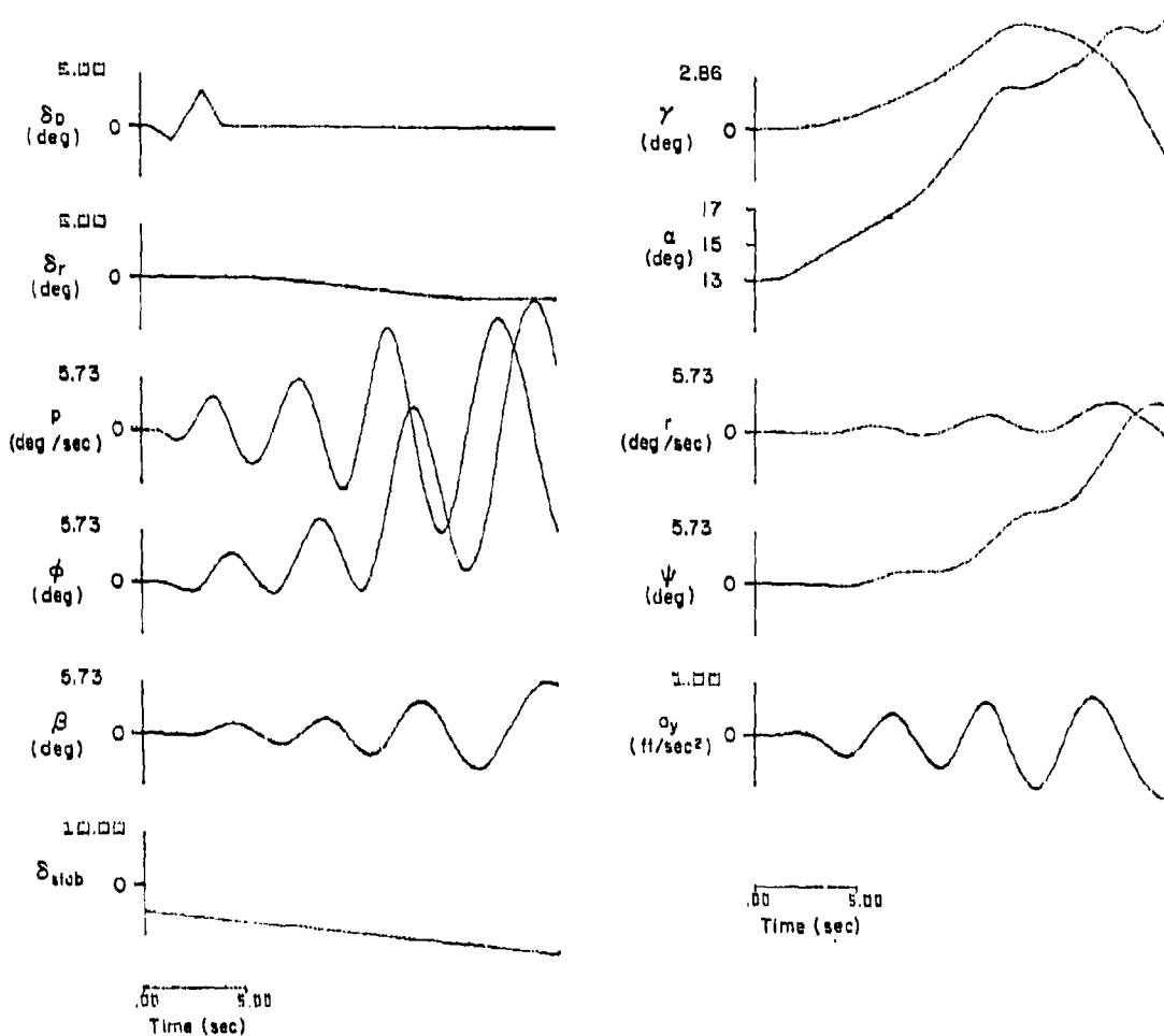
Figure 34. F-14A Model Simulation of Flight 236-1 Pullup
