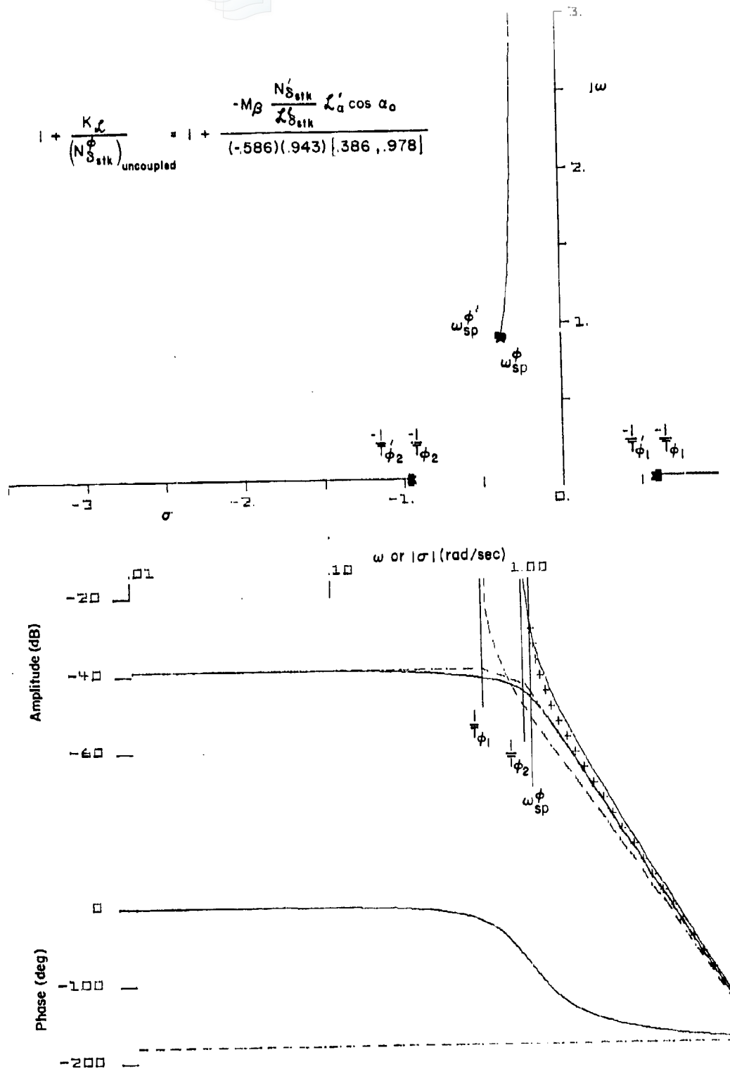
Figure 48. System Survey of Effect of L_{\alpha}^{\phi} on N_{\delta_{stk}}^{\phi} ; F-4J; N_{\alpha}^{\phi} = 0 , \alpha_0 = 21 deg, \beta_0 = 5.5 deg
