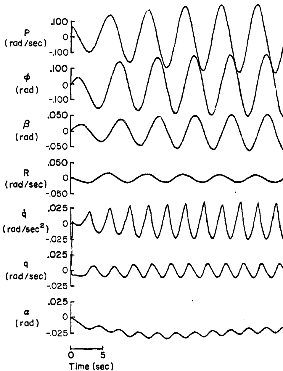
Figure 12. F-4J Open-Loop Nonlinear Airframe Response to Pulse Aileron; \alpha_0 = 21 deg, \beta_0 = 0 deg
