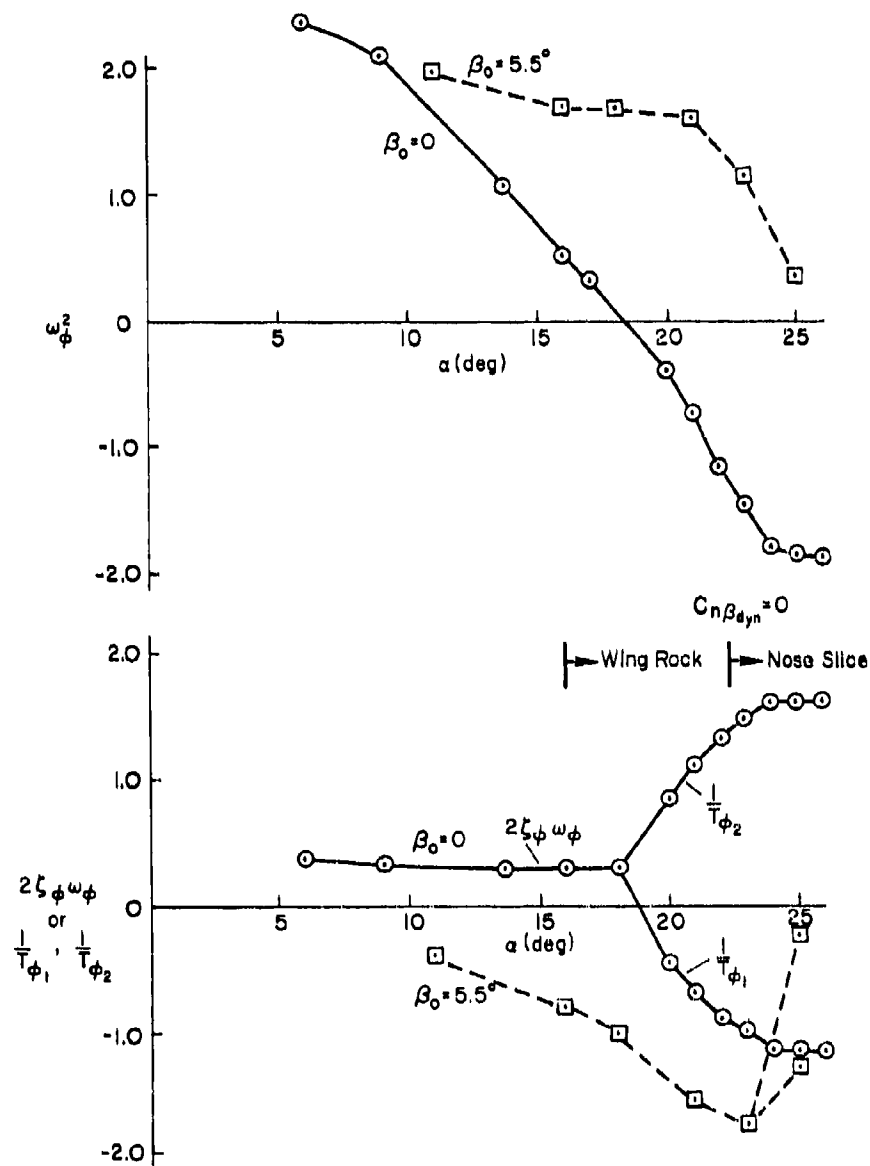
Figure 17. N_{\delta_{stk}}^{\phi} Root Migration with AOA; F-4J
