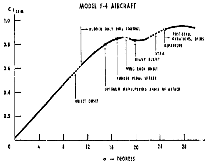
Figure 1. Basic F-4 Trimmed Lift Curve (from Ref. 7)
