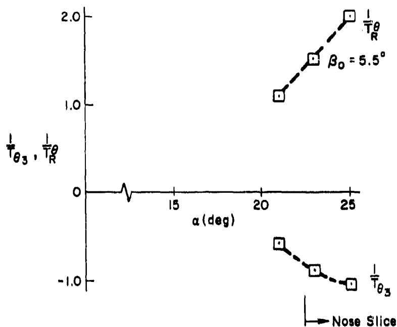
Figure 21. N_{\delta_{stab}}^{\theta} First-Order Root Migrations with AOA; F-4J
