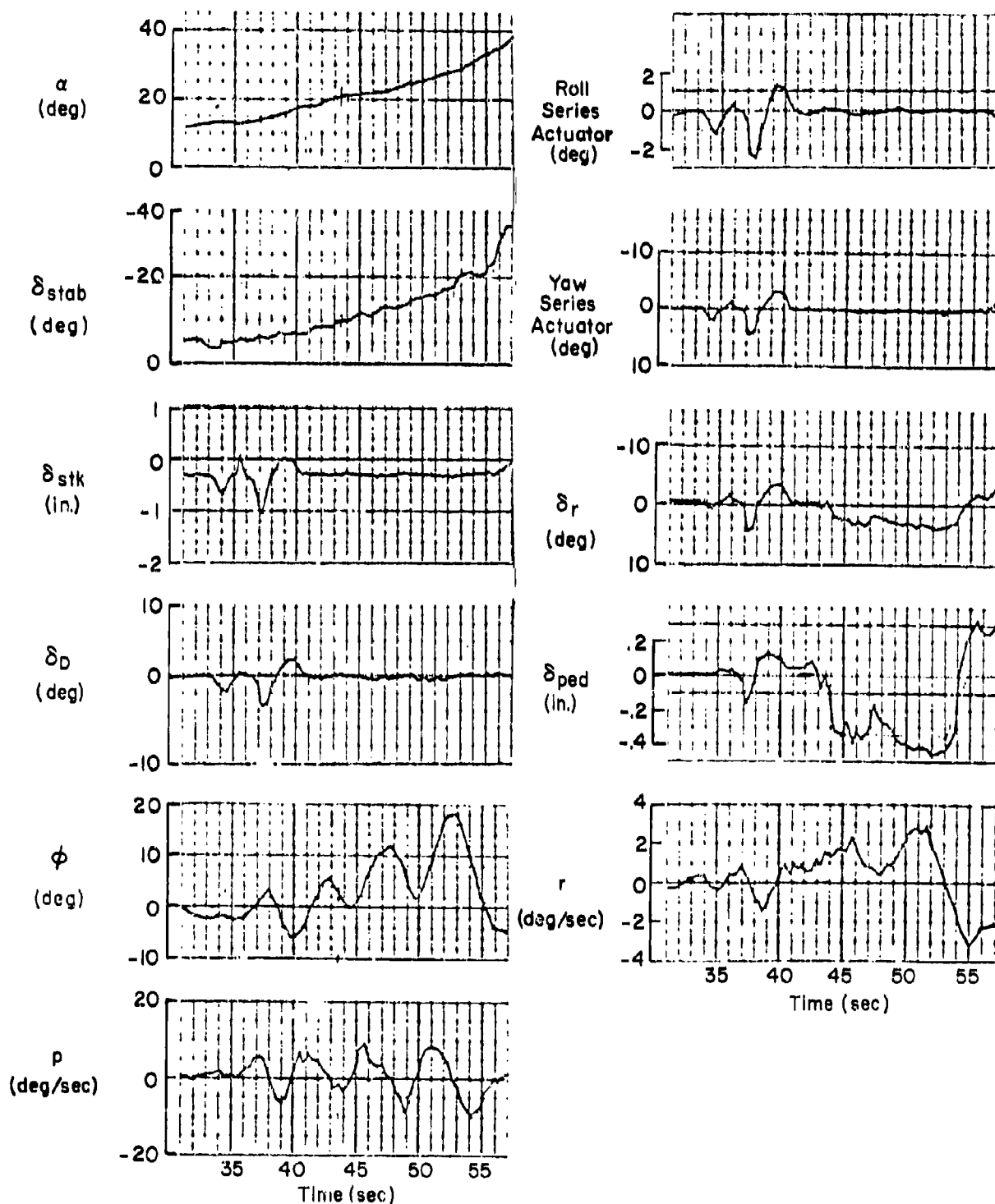
Figure 33. F-14A Flight 276-1 Pullup
