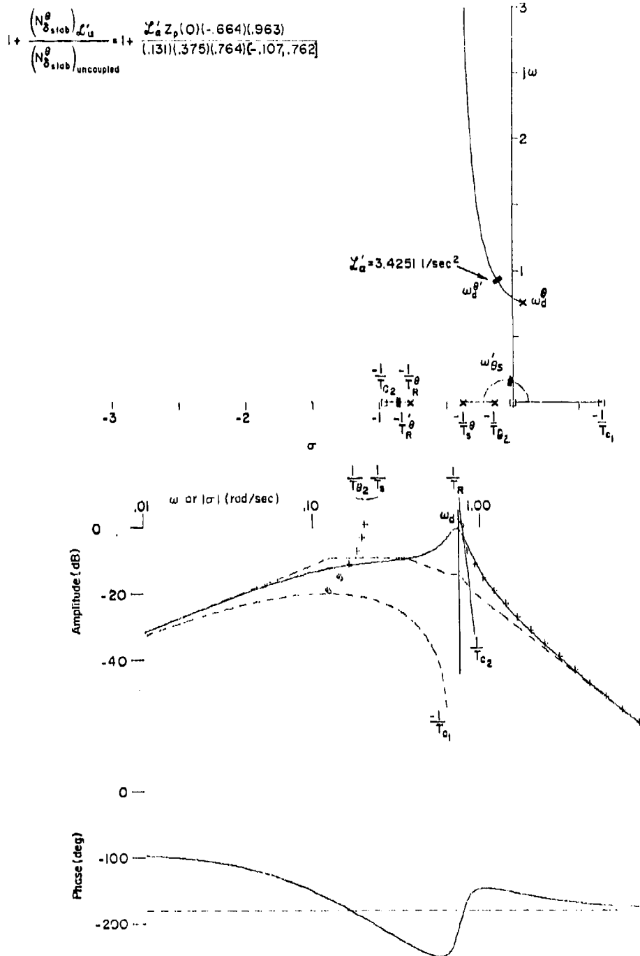
Figure 52. System Survey for Effect of \mathcal{L}'_{\alpha} on N_{\delta_{stab}}^{\theta} ; N_{\alpha}^{\theta} = 0 ; \alpha = 21 deg, \beta = 5.5 deg
