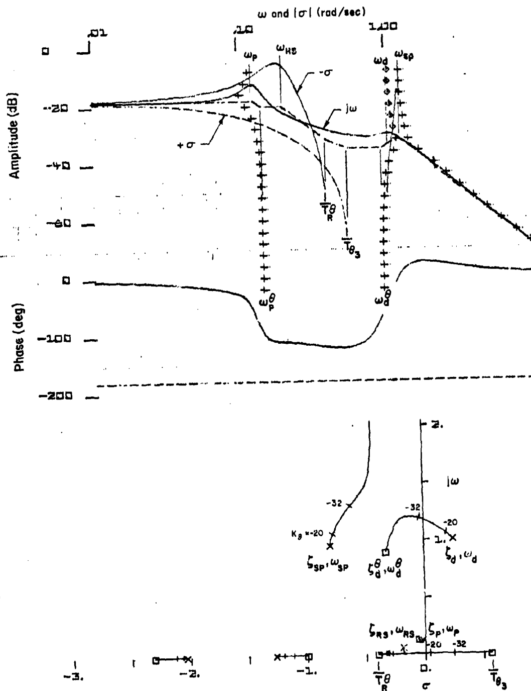
Figure 20. System Survey for \theta + \delta stab Closure; \alpha_0 = 23 deg, \beta_0 = 5.5 deg
