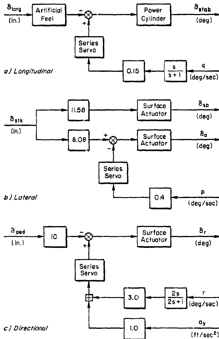
Figure 2. F-4J Flight Control System
