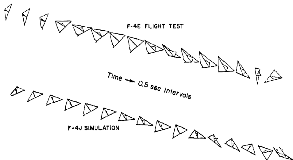
Figure 5. Departure During Left Turn
