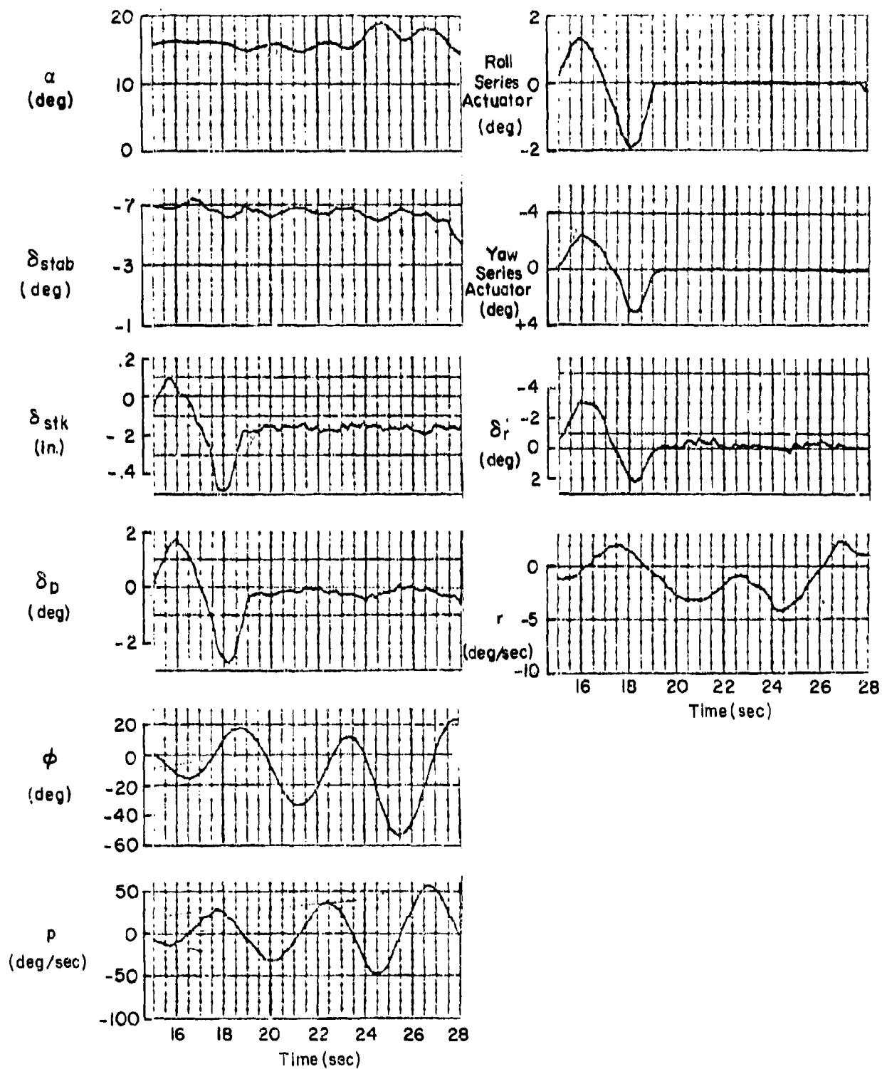
Figure 30. F-14A Flight 234-1 Traces
