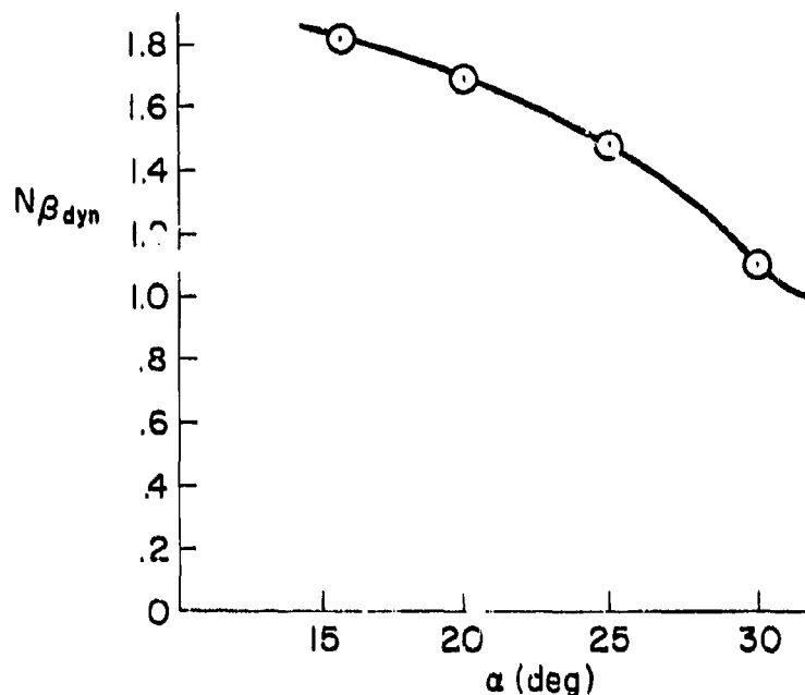
Figure 36. N_{\beta_{dyn}} Variation with AOA; F-14A
