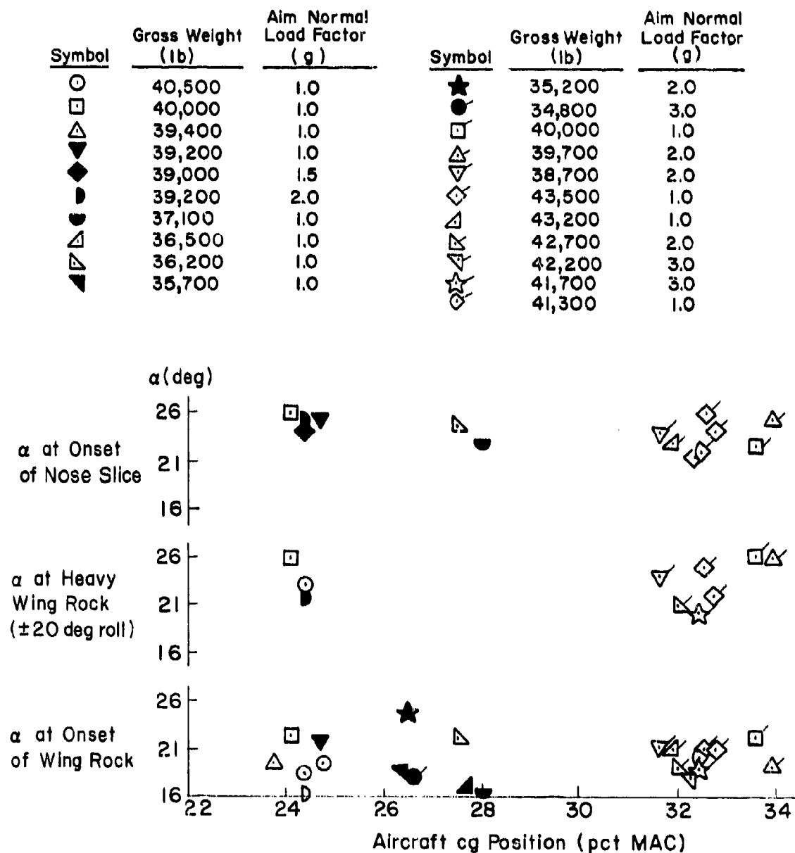
Figure 10. F-4E Stall Approach Characteristics (From Ref. 19)
