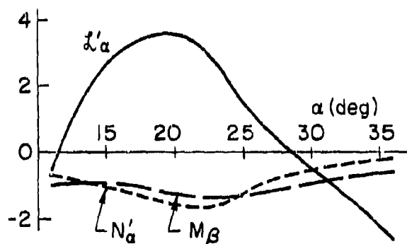
Figure 22. F-4J Static Aerodynamic Cross-Coupling Derivatives; \beta_0 = 5.5 deg
