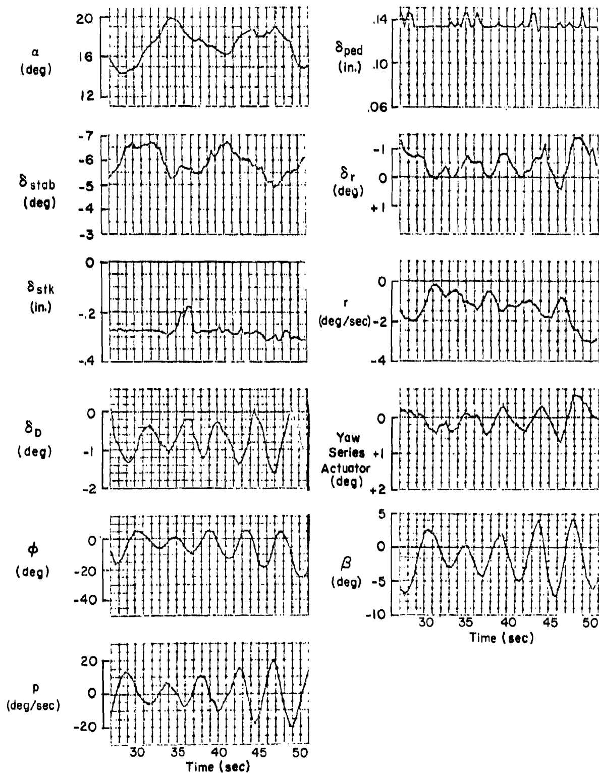
Figure 32. F-14A Flight 243 Traces
