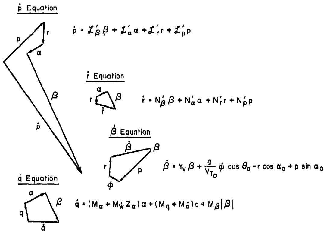
Figure 15. F-4J Force Vector Polygons; \alpha_0 = 21 \text{ deg} , \beta_0 = 1.5 \text{ deg}
