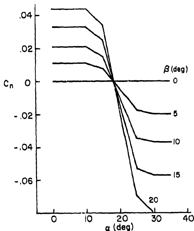
Figure 8. F-4J Yaw Coefficient Variation with \alpha , \beta
