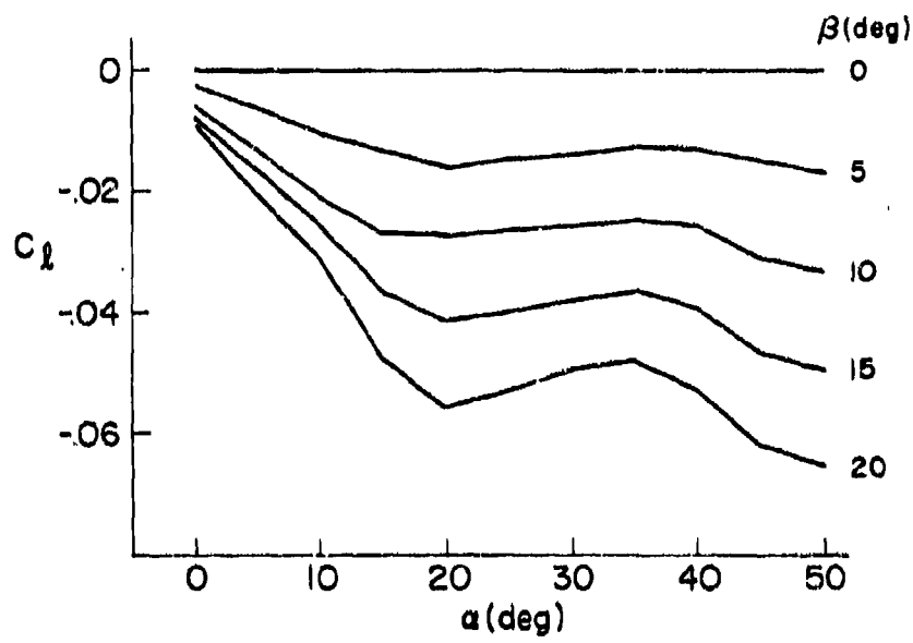
Figure 23. F-14A Roll Coefficient Variation with \alpha , \beta
