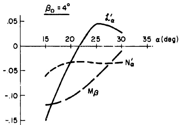
Figure 41. F-14A Static Aerodynamic Cross-Coupling Derivatives
