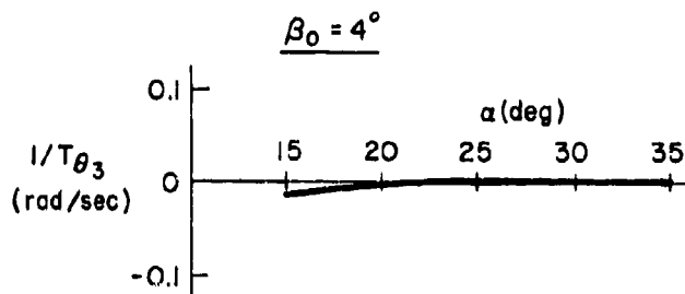
Figure 40. N_{\delta_{stab}}^{\theta} First-Order Root Migration with AOA, F-14A
