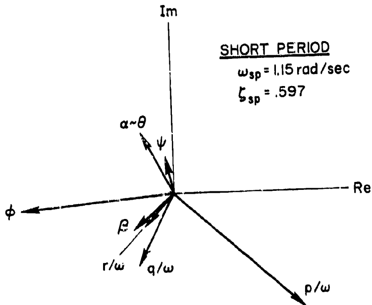
Figure 14. F-4J Eigenvectors; \alpha_0 = 21 \text{ deg} , \beta_0 = 1.5 \text{ deg}
