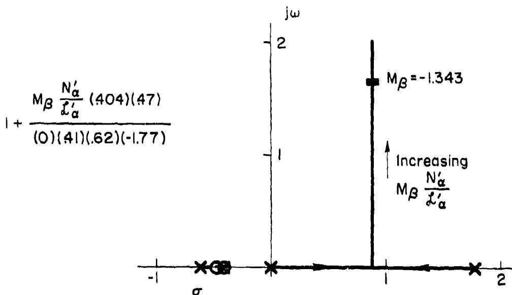
Figure 42. Migration of Roots of K(\beta_0)\Delta_{\text{coup1}} with Increasing M_\beta ( \alpha_0 = 21 deg, \beta_0 = 5.5 deg)
