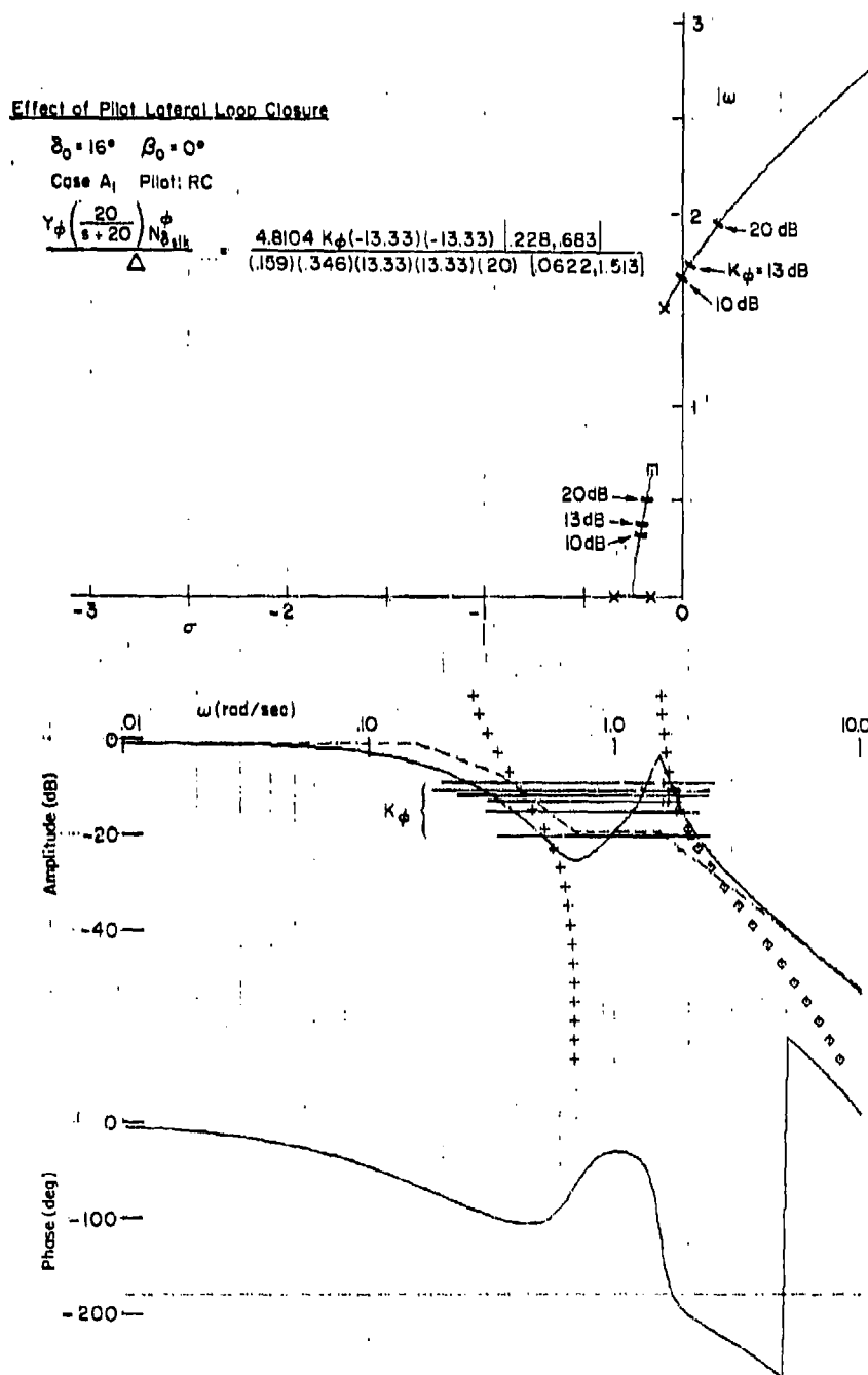
Figure 79. Survey Plot for Roll Loop Closure; \alpha_0 = 16 deg, \beta_0 = 0 deg
