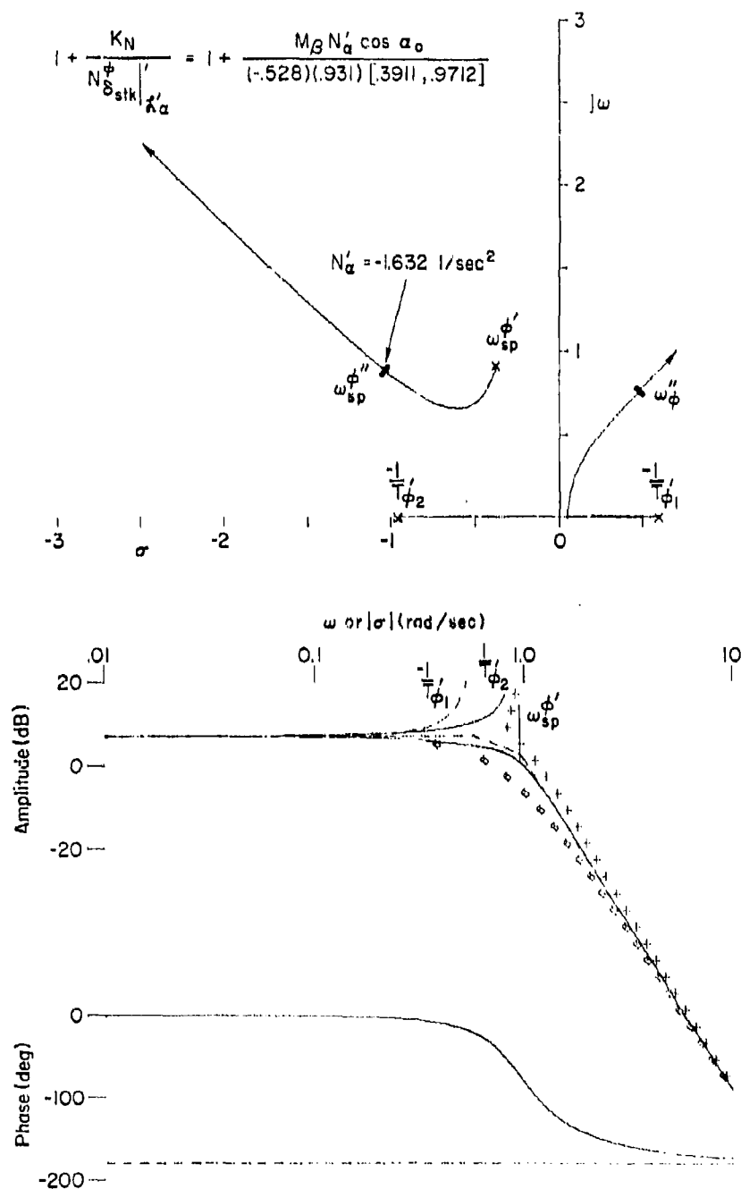
Figure 49. System Survey for Effect of N'_\alpha on N_{\delta_{stk}} (with L'_\alpha = 3.4251 \text{ 1/sec}^2 ), F-4J; \alpha_0 = 21 \text{ deg} , \beta_0 = 5.5 \text{ deg}
