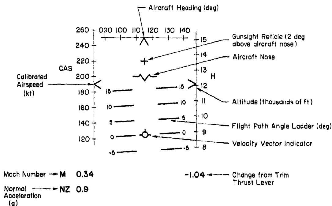
Figure 68. Head-Up Display (HUD) Used in Simulation
