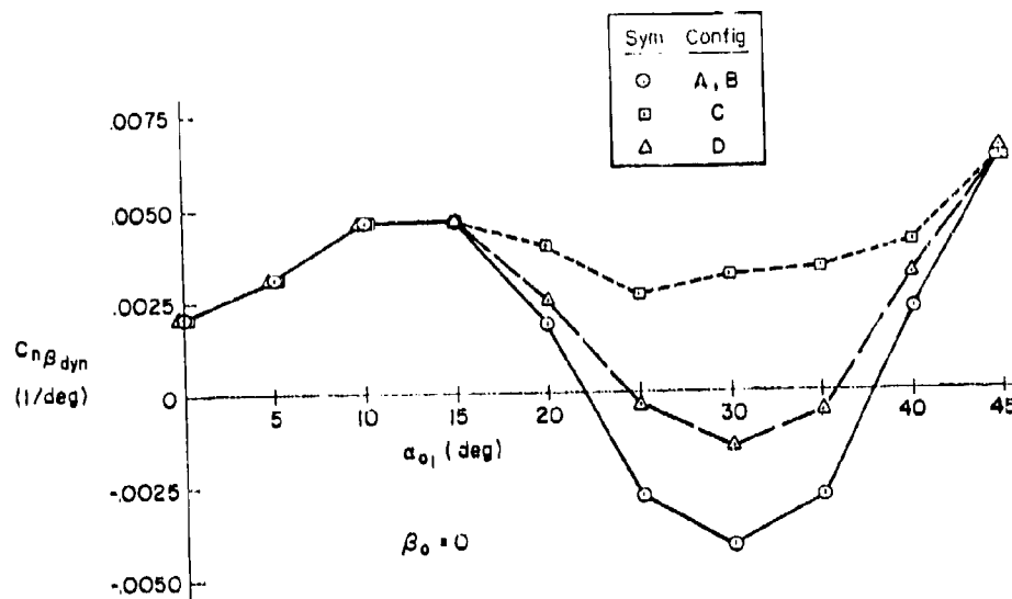
Figure 62. C_{n\beta_{dyn}} for Configurations Simulated
