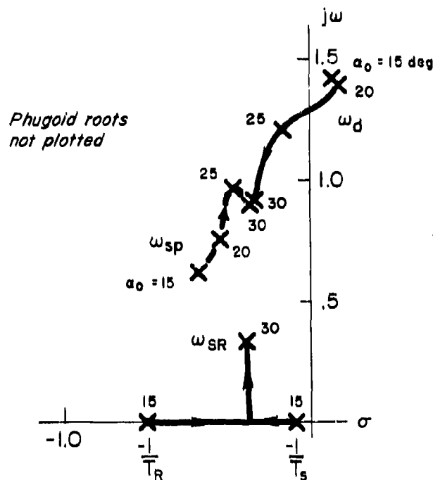
Figure 35. F-14A Root Migrations with AOA
