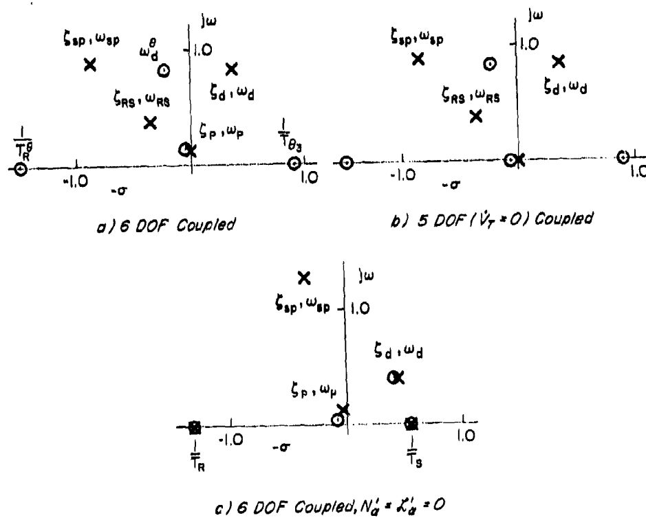
Figure 19. Effect of Lateral-Longitudinal Coupling on N_{stab}^{\theta}/\Delta Roots; \alpha_0 = 23 \text{ deg} , \beta_0 = 5.5 \text{ deg}
