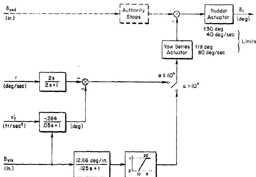
Figure 28. F-14A Directional Control System
