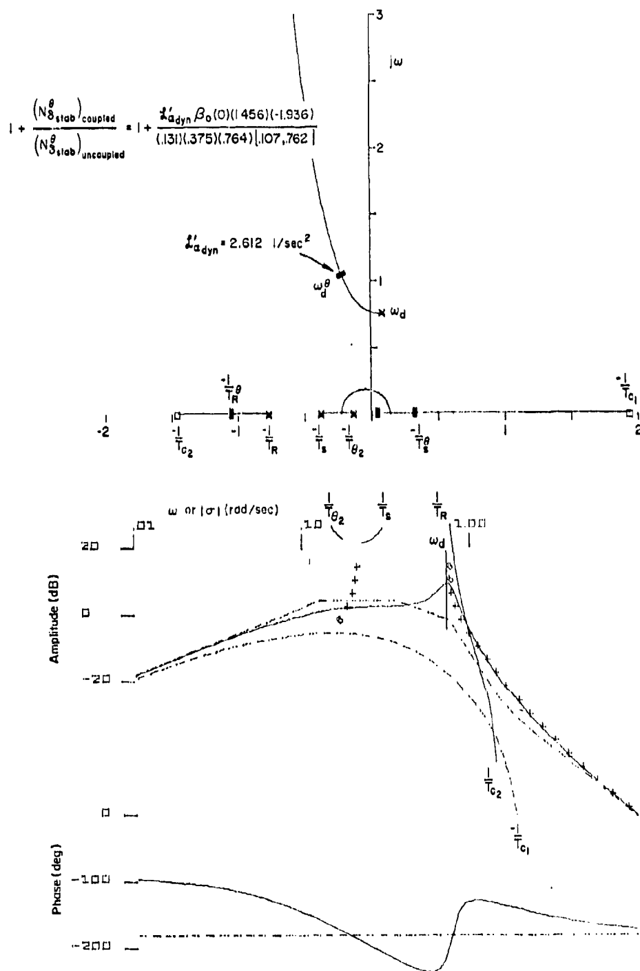
Figure 54. System Survey for Effect of Combined Cross-Coupling on N_{stab}^{\theta} ; F-4J; \alpha_o = 21 \text{ deg} , \beta_o = 5.5 \text{ deg}
