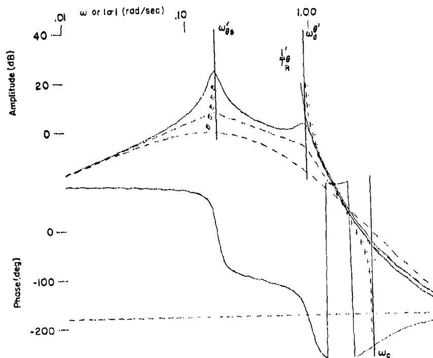
Figure 53. System Survey for Effect of N'_a on N_{stab}^{\theta} ; L'_{\alpha} = 3.4251 \text{ 1/sec}^2 ; F-4J; \alpha = 21 \text{ deg} , \beta = 5.5 \text{ deg}
