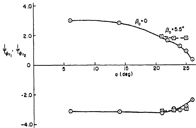
Figure 18. N_{\delta_r}^\phi Root Migration with AOA; F-4J
