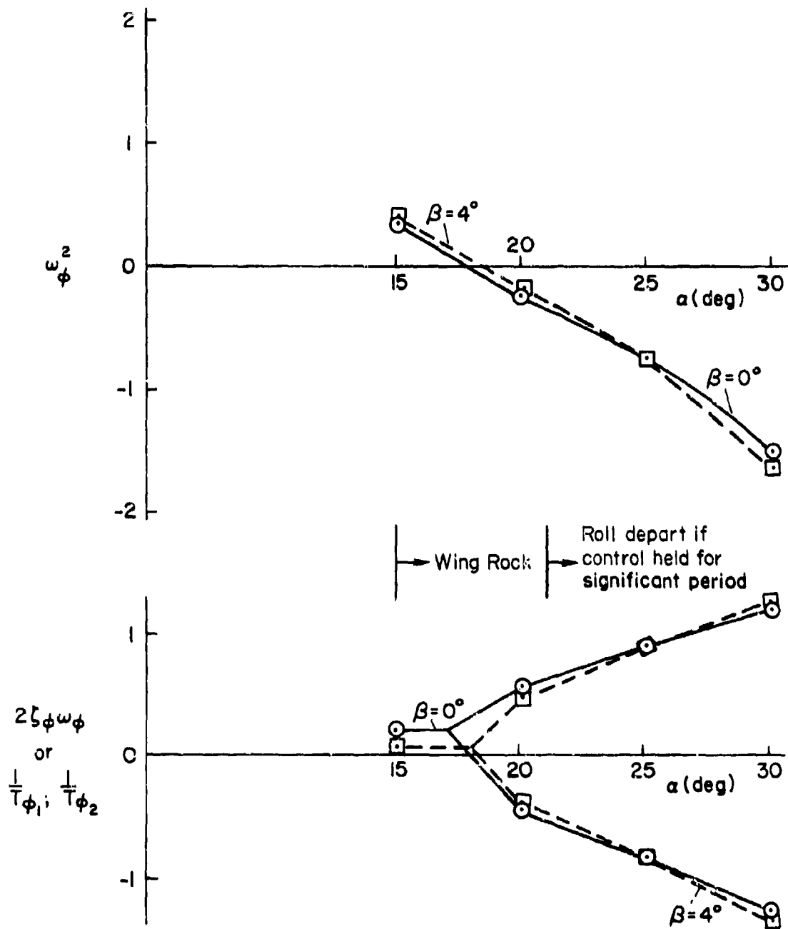
Figure 39. N_{\delta\phi}^\phi Root Migration with AOA; F-14A
