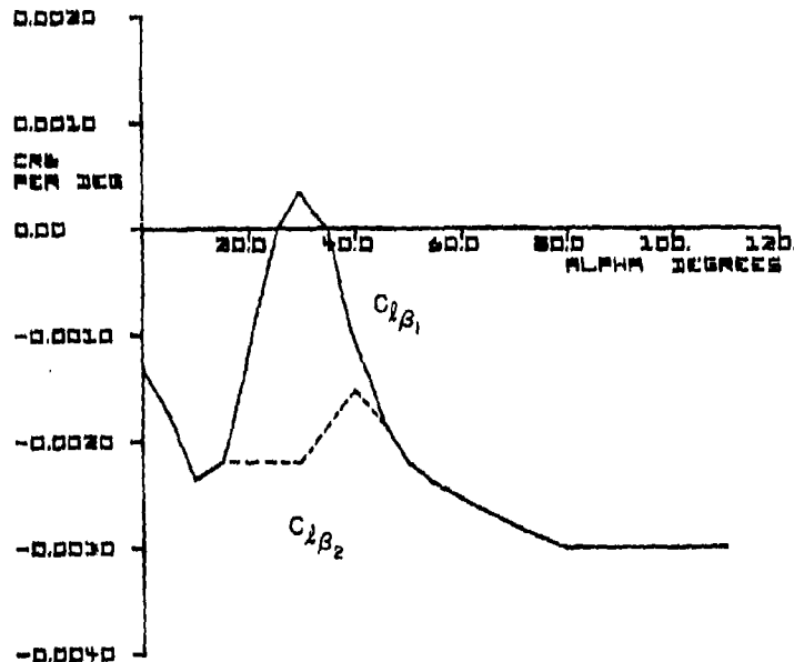
Figure 58. Change in C_{l\beta} for Configuration C
