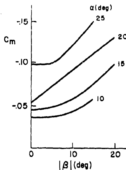
Figure 6. F-4J Pitch Coefficient Variation with \alpha , \beta
