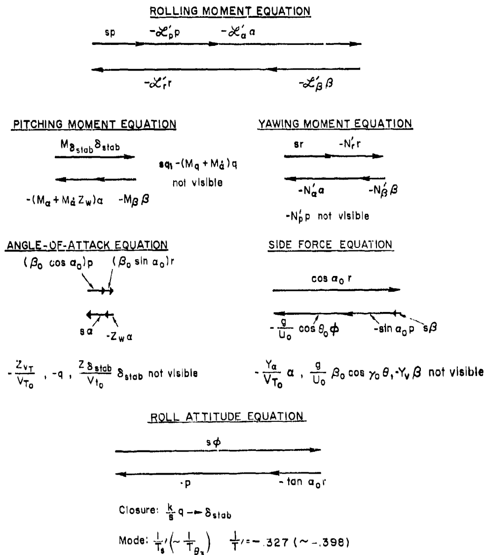
Figure 50. Time Vectors for Closed-Loop Mode 1/T_s (Approximating 1/T_{\theta_3} ), F-4J; \alpha = 21 \text{ deg} , \beta = 5.5 \text{ deg}
