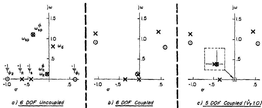
Figure 44. N_{\text{stk}}^{\phi} / \Delta Pole-Zero Locations, Coupled vs. Uncoupled, F-4J, \alpha_0 = 21 \text{ deg} , \beta_0 = 5.5 \text{ deg}
