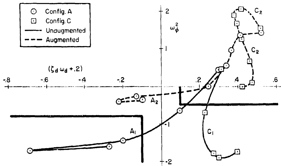
Figure 66. \omega_\phi^2 Versus \zeta_d \omega_d for Augmented and Unaugmented Configurations A and C
