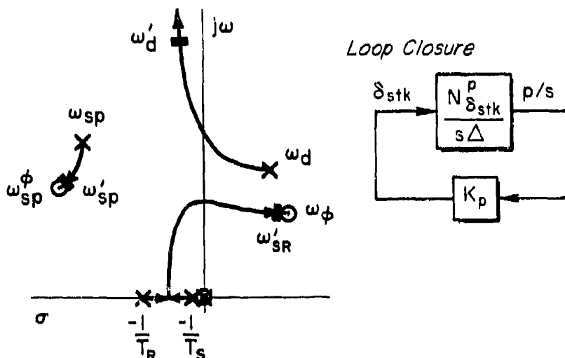
Figure 45. Closure of p/s + \delta_{stk} to Obtain Time Vectors, F-4J, \alpha_0 = 21 \text{ deg} , \beta_0 = 5.5 \text{ deg}
