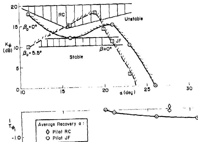
Figure 86. Roll Loop Closure Gains Employed with Configuration D
