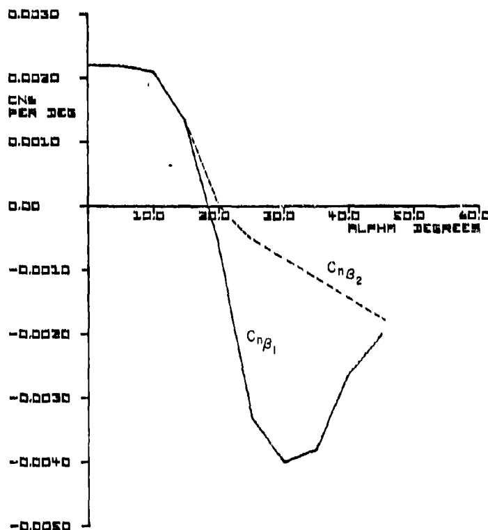
Figure 60. Change in C_{n\beta} for Configuration D
