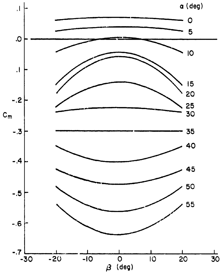
Figure 25. F-14A Pitch Coefficient Variation with \alpha , \beta
