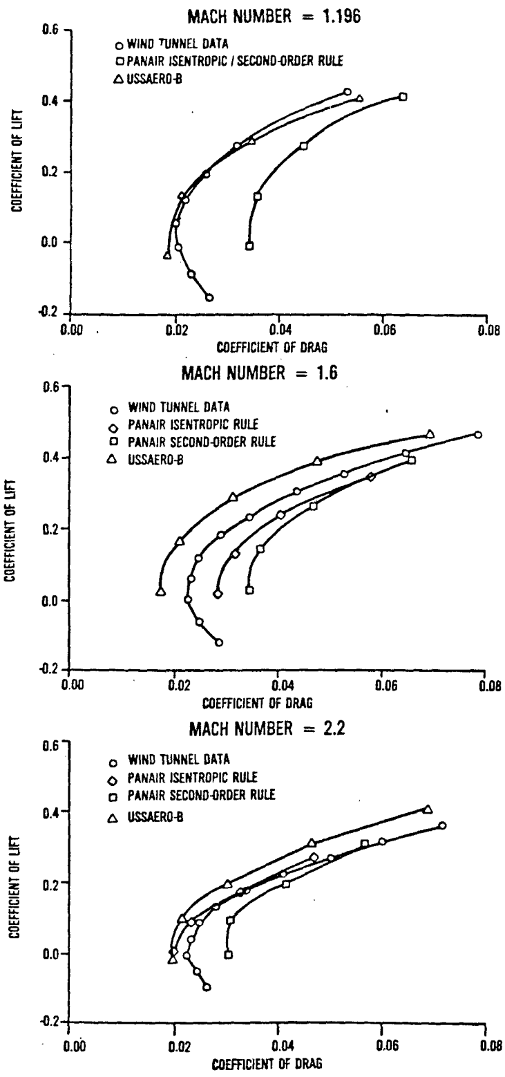
Figure 33. Drag Polars, CDAF Configuration
