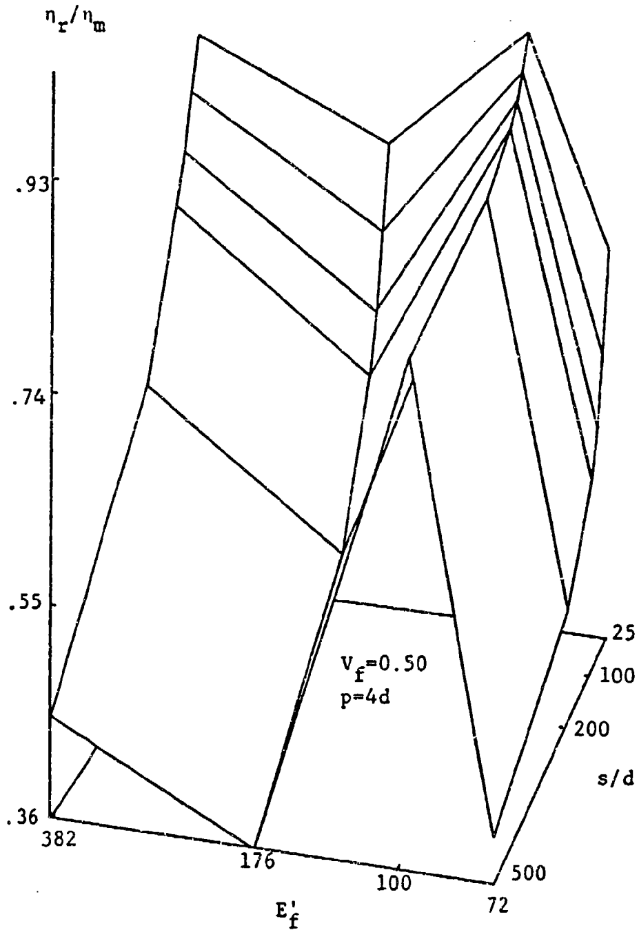
Figure 9.26: Three-Dimensional Plots of \eta_x/\eta_m vs s/d and E'_x for Randomly Oriented Fiber Composites
