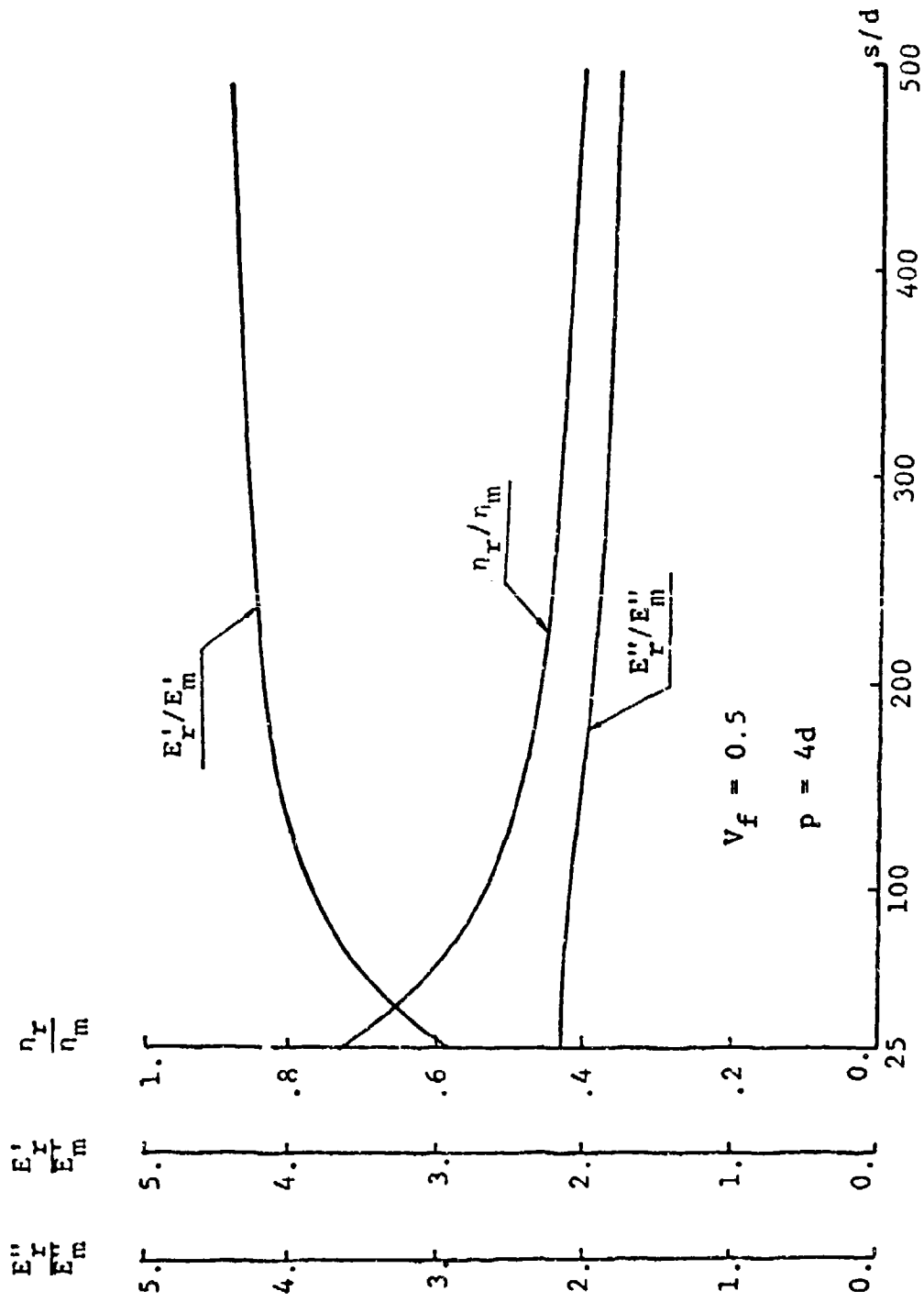
Figure 9.18: Plots of n_I/n_m , E_I'/E_m' and E_I''/E_m'' vs s/d for Randomly Oriented Glass Epoxy Composites
