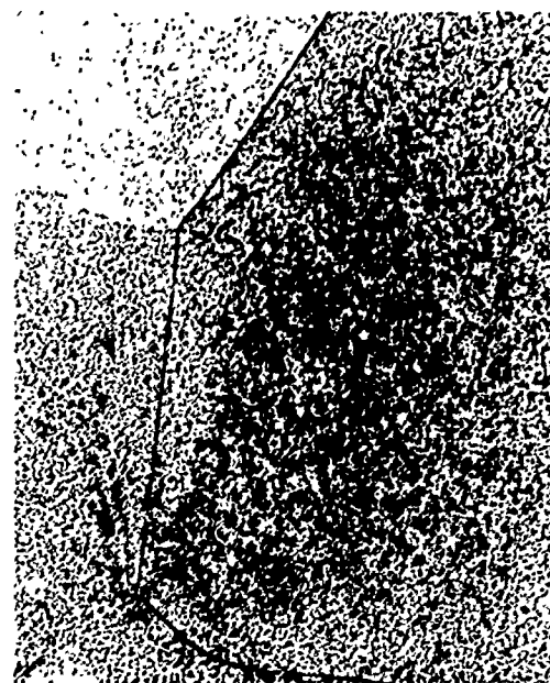
(n) Heat 24222 (9481) Ti-7Fe-0.03Y 1525F-1hr-WQ + 1025F-24hr-AC
