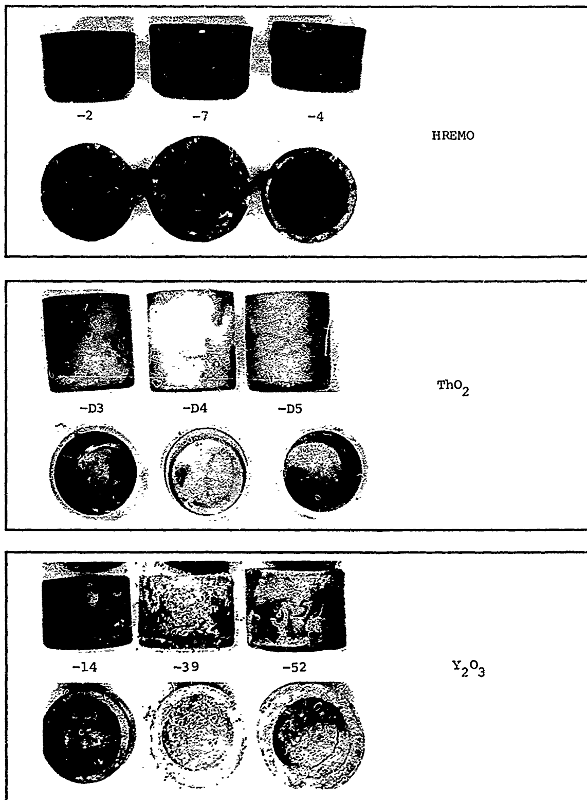
Figure 12. Side and Top Views of the Special Fired Crucibles. Used in Task II Melting Experiments.
