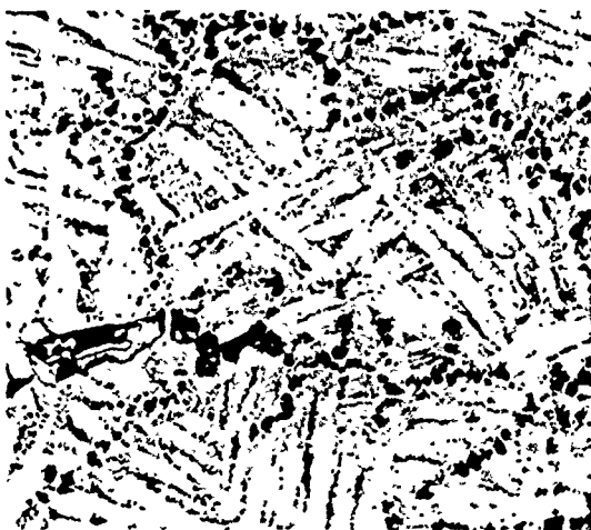
(u) Heat 24107 (9274) Ti-2.7Be-5Zr 1775°F-1Hr-FC
