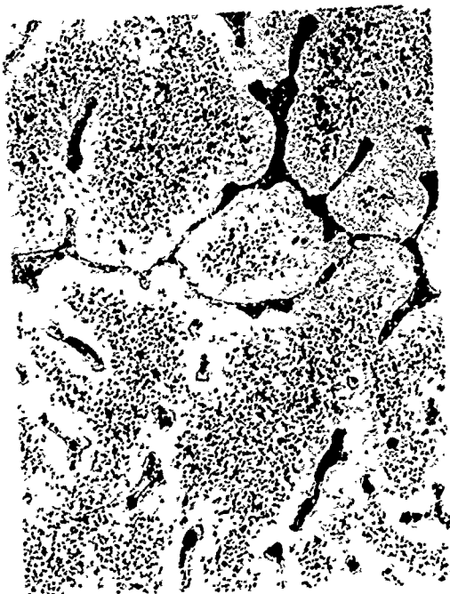
(c) HEAT 24268 (9554) Ti-7Fe-1Be-0.03Y 1525F-1 hr-FC
