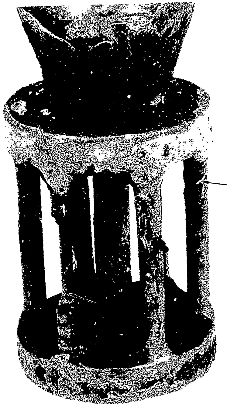
Figure 45. Appearance of Ti-13Cu-1.5Al Alloy Cast into the Howmet Monograf Mold (P-19). Note Good Fill but Surface Cold Shuts (Arrows).
