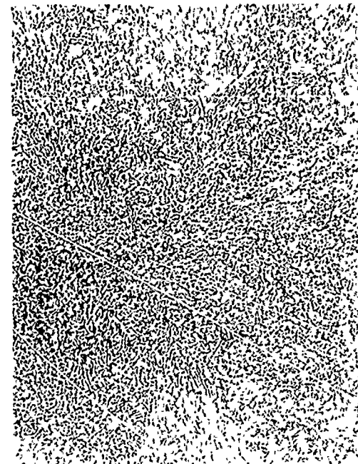
(f) HEAT 24275 (9567) Ti-13Cu-2Al 1760F-1 hr-AC +1450F-8 hr-AC
