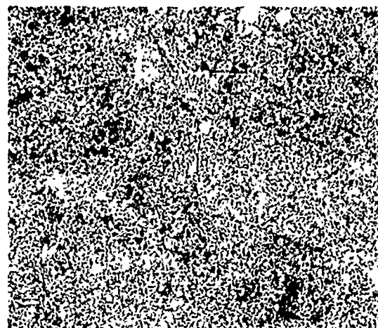
(b) Heat 24033 (8782) Ti-11Co 1225°F-1Hr-FC
