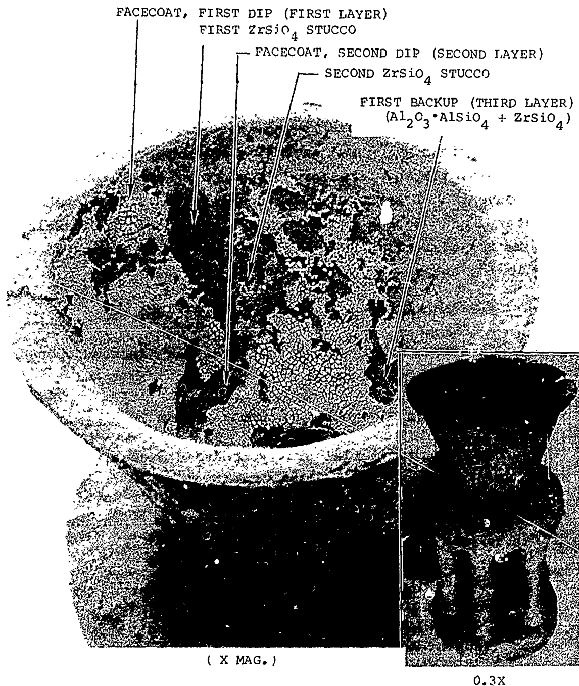
Figure 29. Typical Appearance of Experimental Molds (Composition CC2) Illustrating Severe Spalling of Facecoats in Cup Area. Molds Fired at 1900°F for 1-Hour Were all Unusable for Further Casting Operations.
