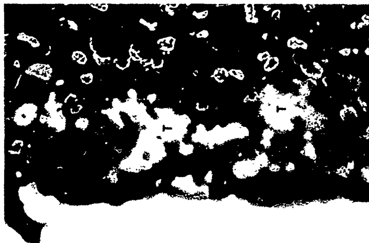
(B) I.D. EPCF SHOWING TITANIUM ALLOY INFILTRATION
