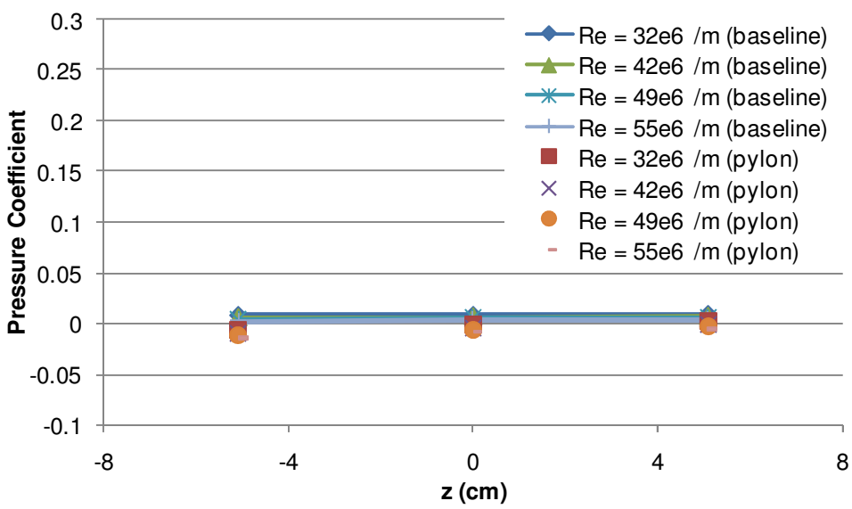
Figure 100. Surface pressure coefficients with and without a pylon installed (x = 3.4 cm, y = -2.54 cm)
