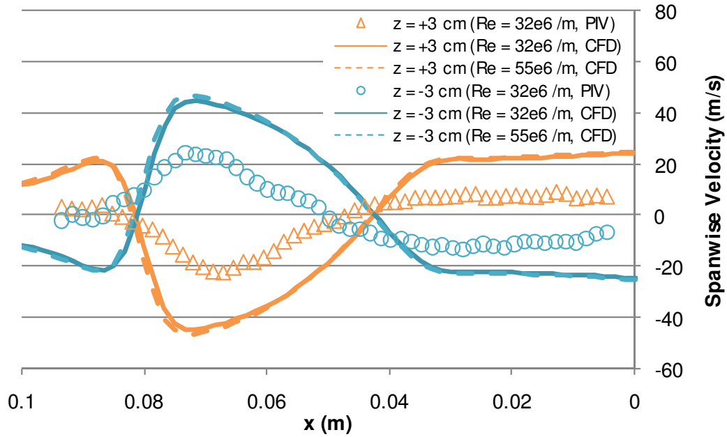
Figure 49. Spanwise velocities at z = \pm 3 cm
