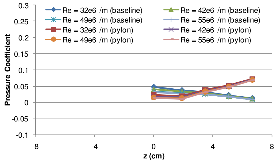
Figure 103. Surface pressure coefficients with and without a pylon installed (x = 9.2 cm, y = -1.6 cm)
