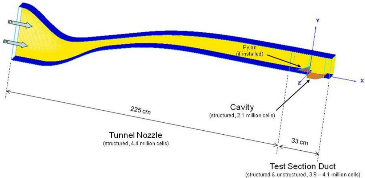
Figure 26. Computational domains
