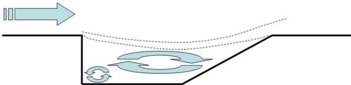
Figure 8. Inclined cavity flameholder
