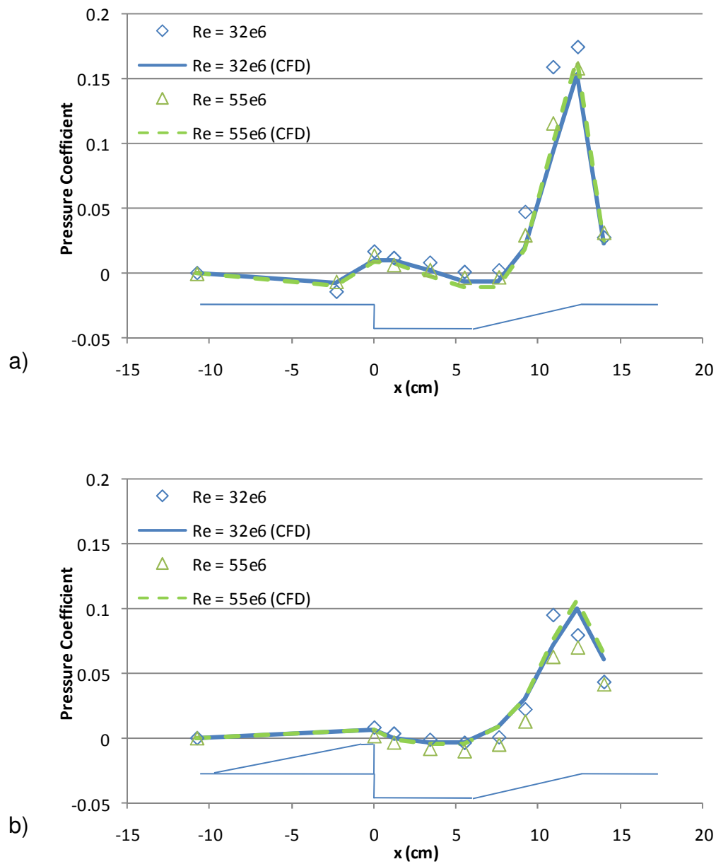
Figure 37. Wind tunnel and CFD centerline surface pressure coefficients at Re \approx 32 \times 10^6 \text{ m}^{-1} and Re \approx 55 \times 10^6 \text{ m}^{-1} , a) without pylon and b) with pylon
