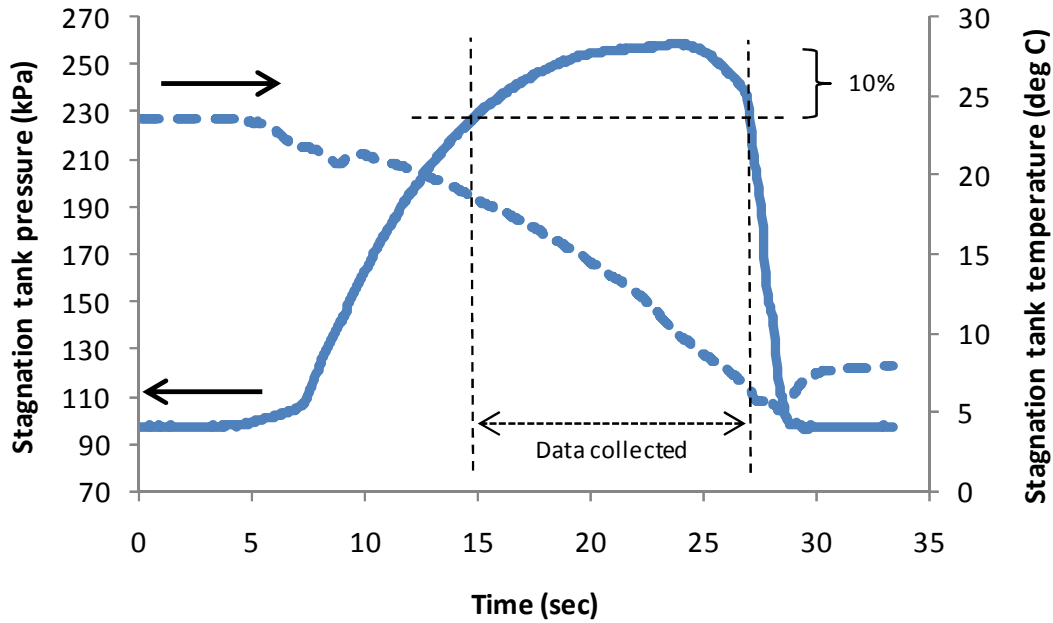
Figure 15. Stagnation tank pressure and temperature traces (stagnation pressure setting = 241 kPa, peak stagnation pressure = 258 kPa)
