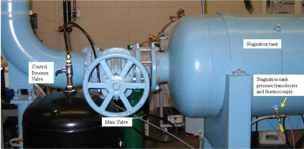
Figure 81. Main and pressure control valves
