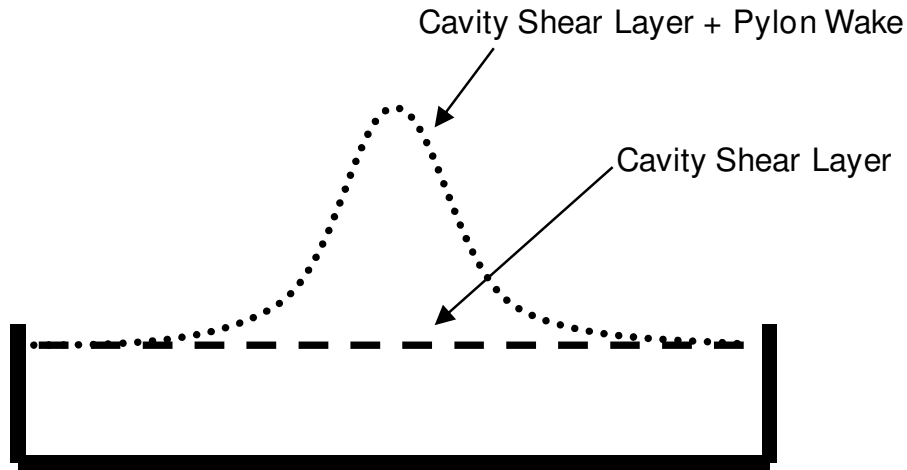
Figure 13. Comparison of cavity shear layer and cavity shear layer plus pylon wake
