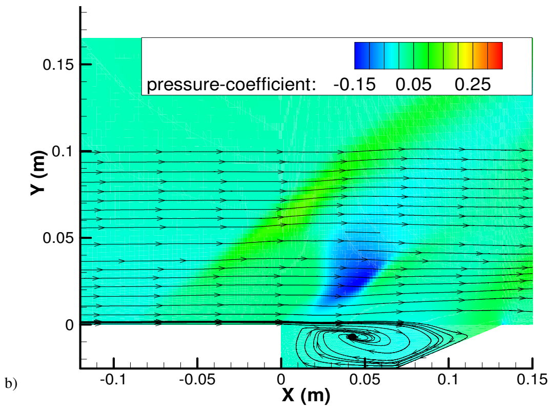
Figure 42. CFD off-centerline pressure coefficient with streamlines ( Re \approx 32 \times 10^6 m^{-1} ): a) z = 0.5 cm; and b) z = 2 cm
