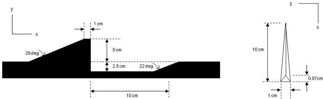
Figure 18. Test article geometry
