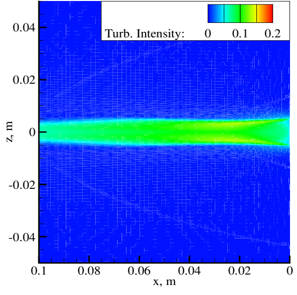
Figure 90. Turbulence intensity behind pylon 3.7 cm above the cavity (CFD; Re \approx 32 \times 10^6 \text{ m}^{-1} ; corresponds to Figure 46)
