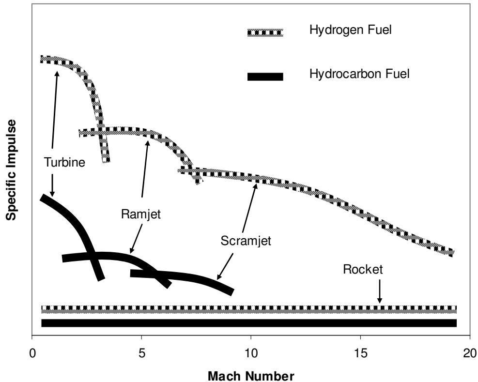
Figure 2. Air-breathing propulsion specific impulse trends [based on Ref. 3]
