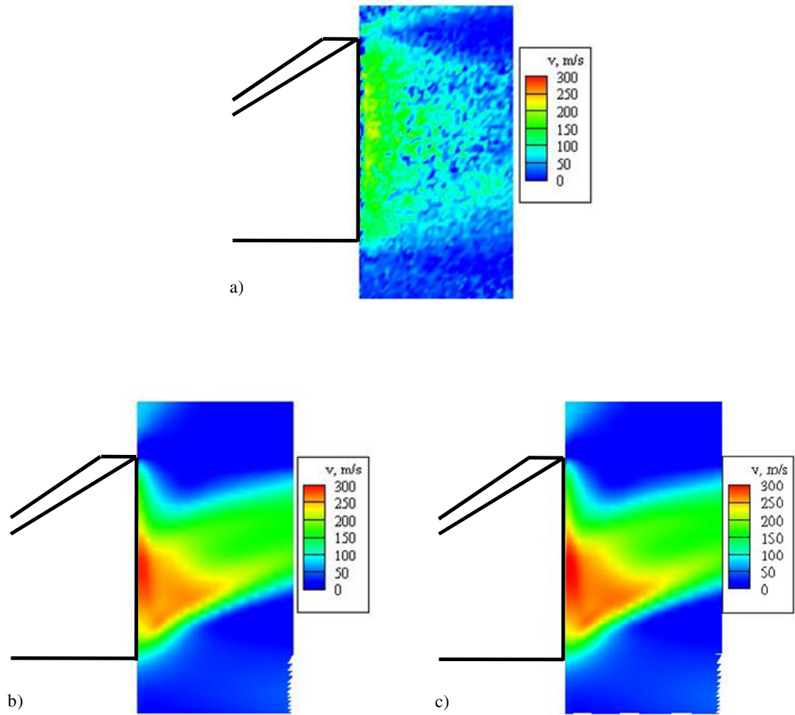
Figure 43. Vertical velocity on centerline a) PIV data ( Re \approx 32 \times 10^6 \text{ m}^{-1} ); b) CFD data ( Re \approx 32 \times 10^6 \text{ m}^{-1} ); and c) CFD data ( Re \approx 55 \times 10^6 \text{ m}^{-1} )
