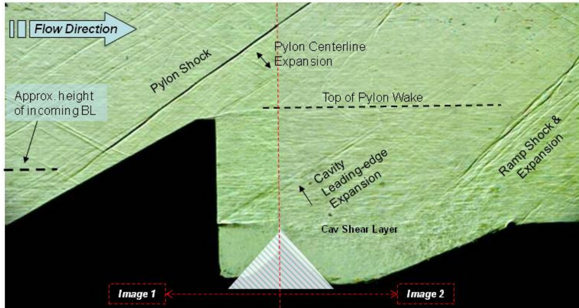
Figure 31. Shadowgraph image of significant features ( Re\# \approx 42 \times 10^6 \text{ m}^{-1} , M = 2 ; hatched area unusable)
