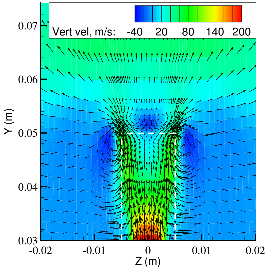
Figure 33. Flowfield behind the top of the pylon in the plane x = 1 cm (contours of vertical velocity; dashed line represents the pylon)
