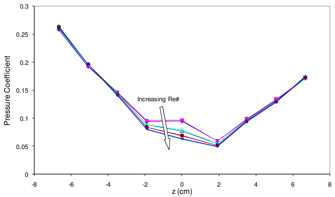
Figure 40. Cross ramp surface pressure coefficients with pylon installed
