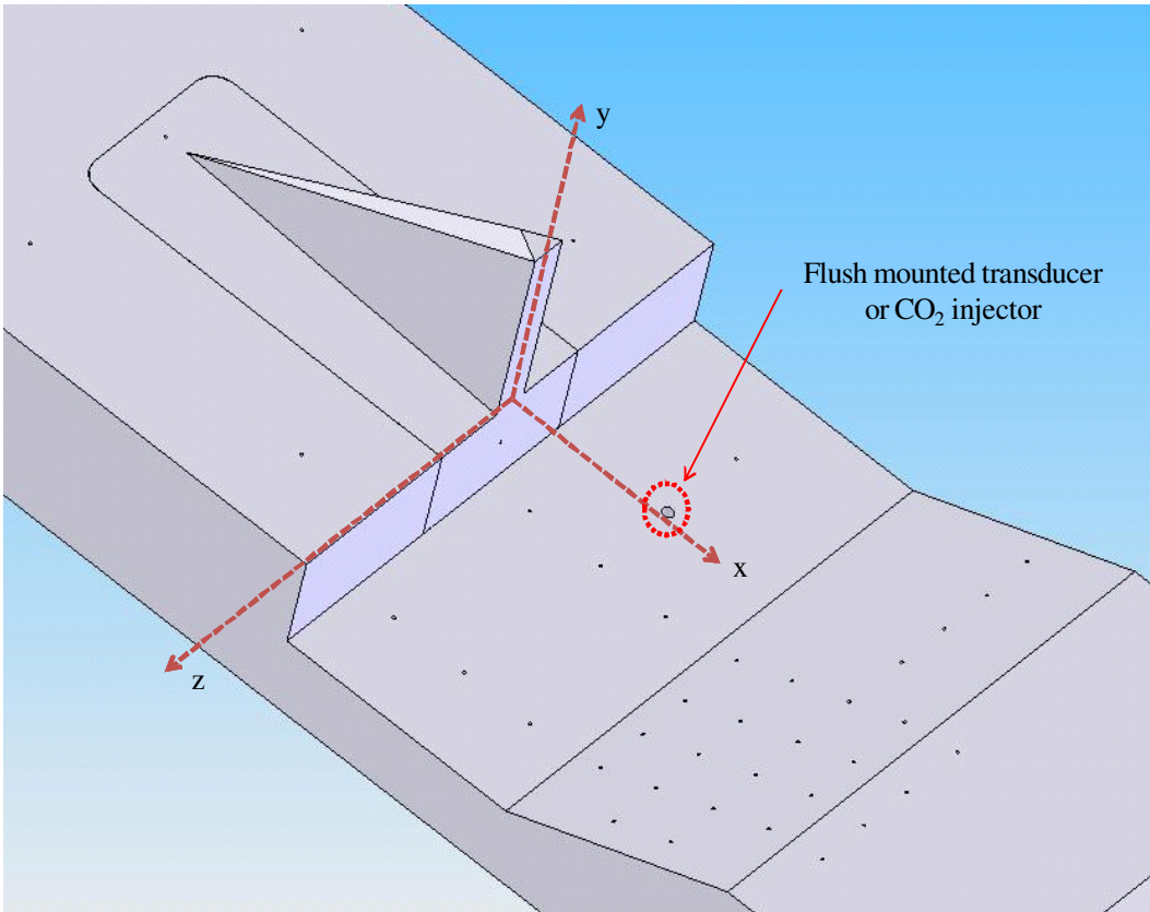
Figure 19. Coordinate system and pressure tap placement
