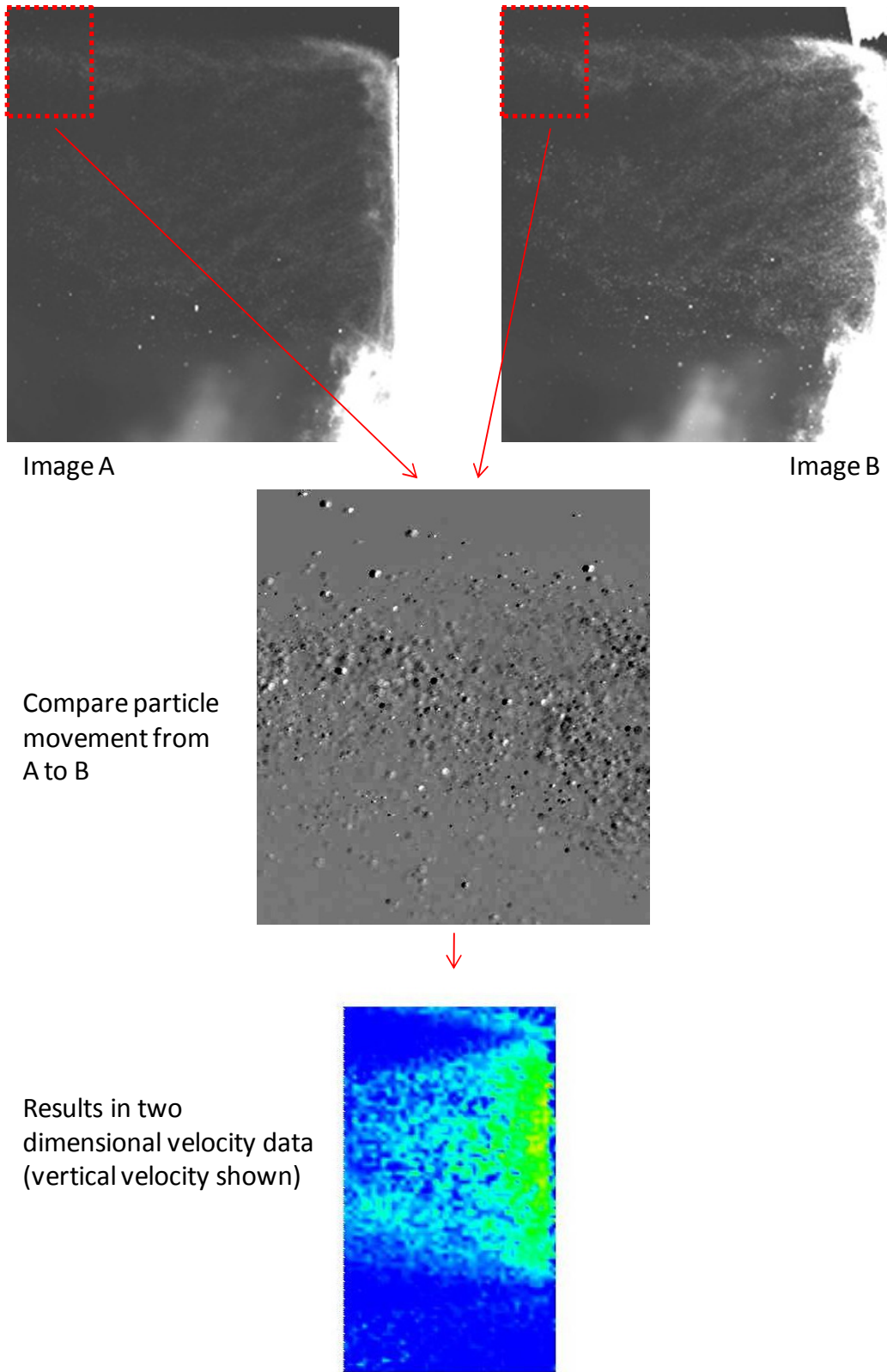
Figure 23. PIV data reduction flow (flow from right; details in App. A)
