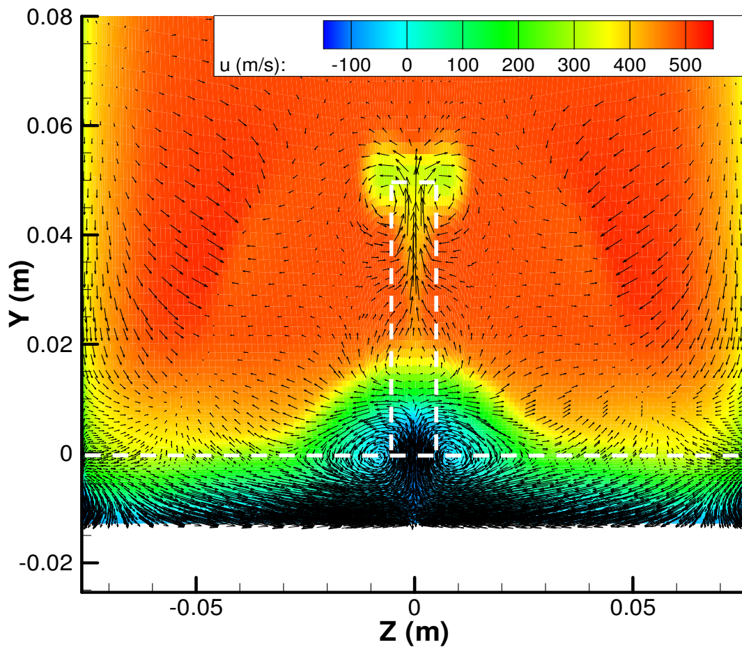
Figure 54. Velocity vectors in y-z plane at x = 10 cm across full span of test section (contours of x velocity; Re \approx 32 \times 10^6 m^{-1} )
