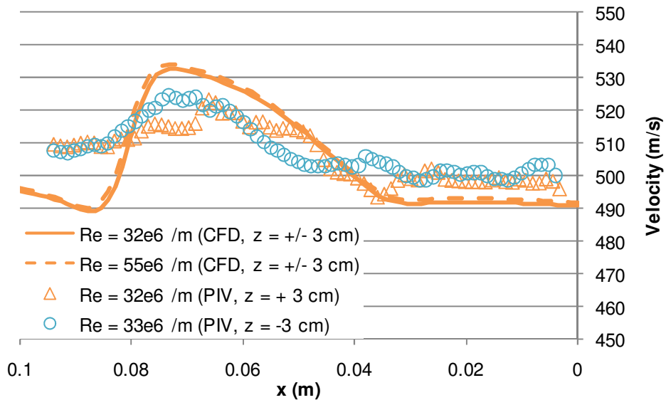
Figure 48. Profile of velocity magnitude on either side of wake ( y = 3.7 \text{ cm} , z = +/- 3 \text{ cm} ; CFD velocities corrected for temperature differences)
