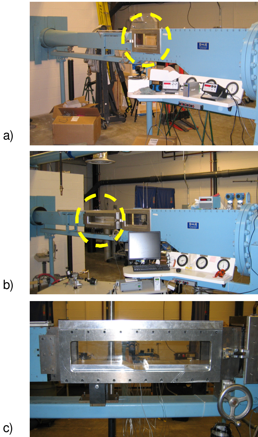
Figure 65. AFIT 6" x 6" Supersonic Wind Tunnel: a) original test section; b) new Test section inserted behind old test section; c) closeup of new test section with baseline cavity test article installed
