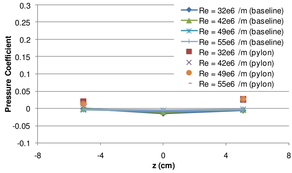
Figure 97. Surface pressure coefficients with and without a pylon installed (x = -2.3 cm, y = 0 cm)
