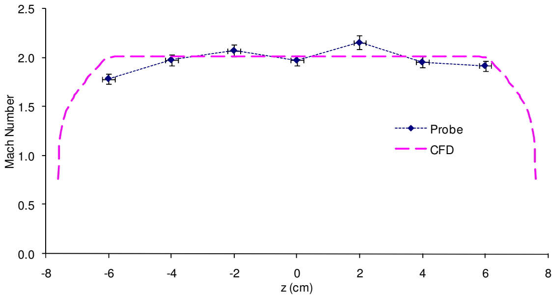
Figure 17. Mach number profile across the test section entrance ( x = -22 \text{ cm} , y = 3.7 \text{ cm} ; Re \approx 32 \times 10^6 \text{ m}^{-1} )
