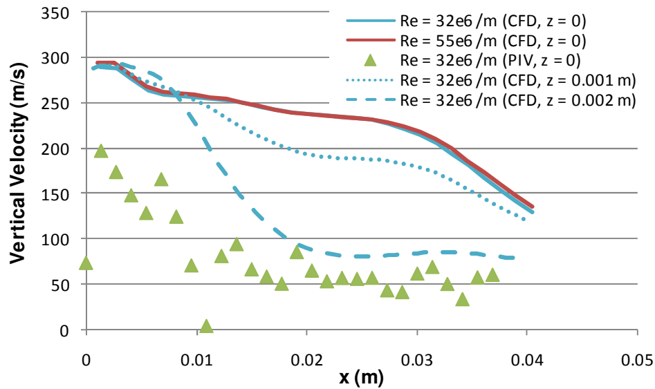
Figure 44. Centerline vertical velocities behind pylon pressure tap ( y = 1.9 cm)
