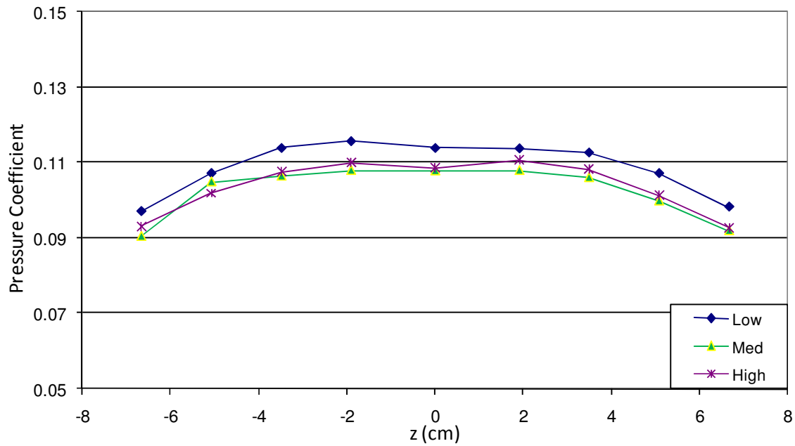
Figure 93. Grid convergence (cross ramp pressure coefficient)
