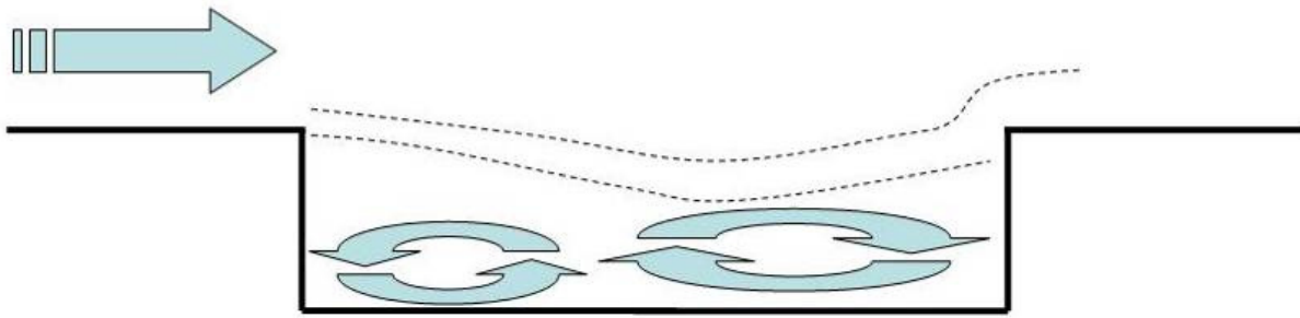
Figure 6. Rectangular cavity flameholder
