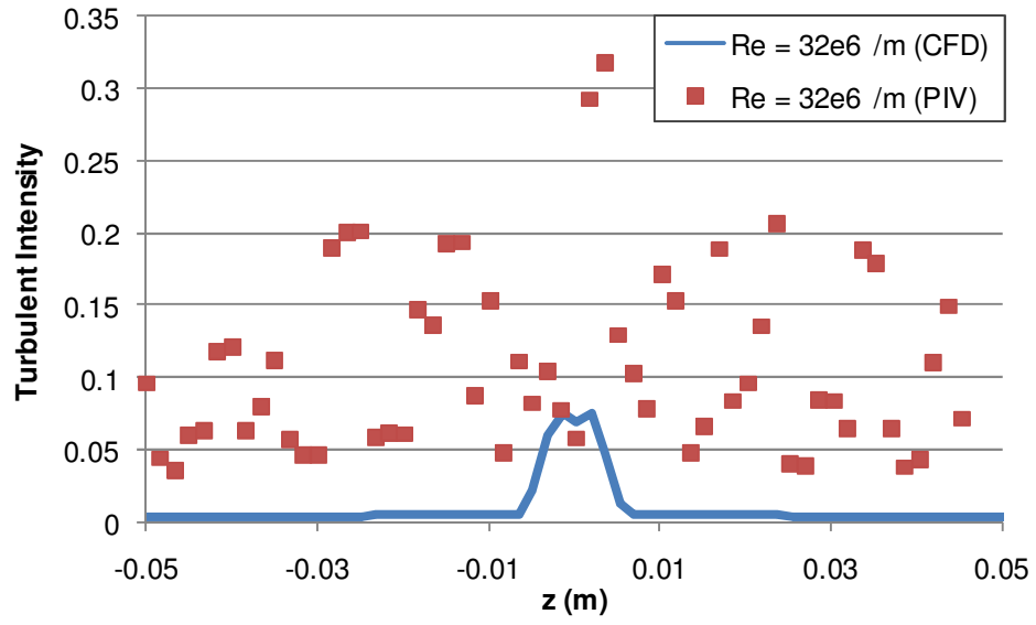
Figure 92. Turbulence intensity profile across test section (x = 8.8 cm, y = 3.7 cm)
