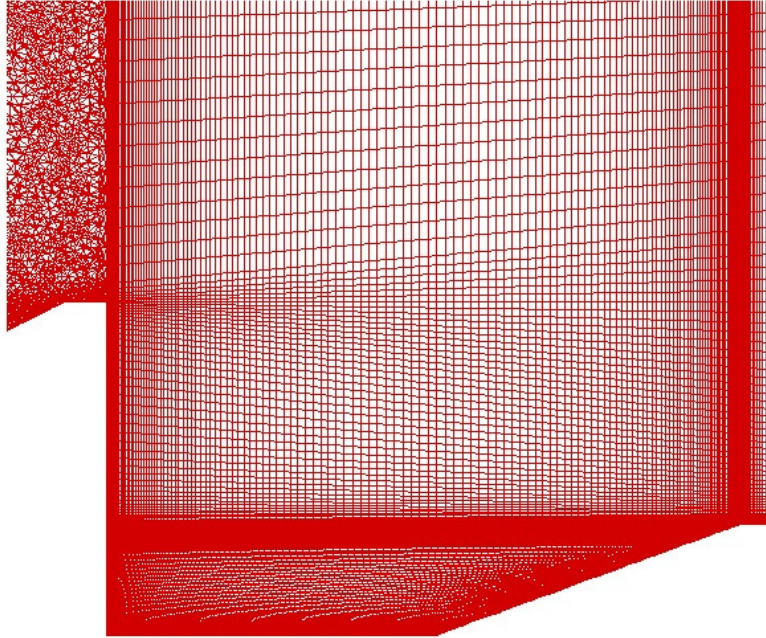
Figure 27. Close-up of mesh on centerline ( z = 0 cm)
