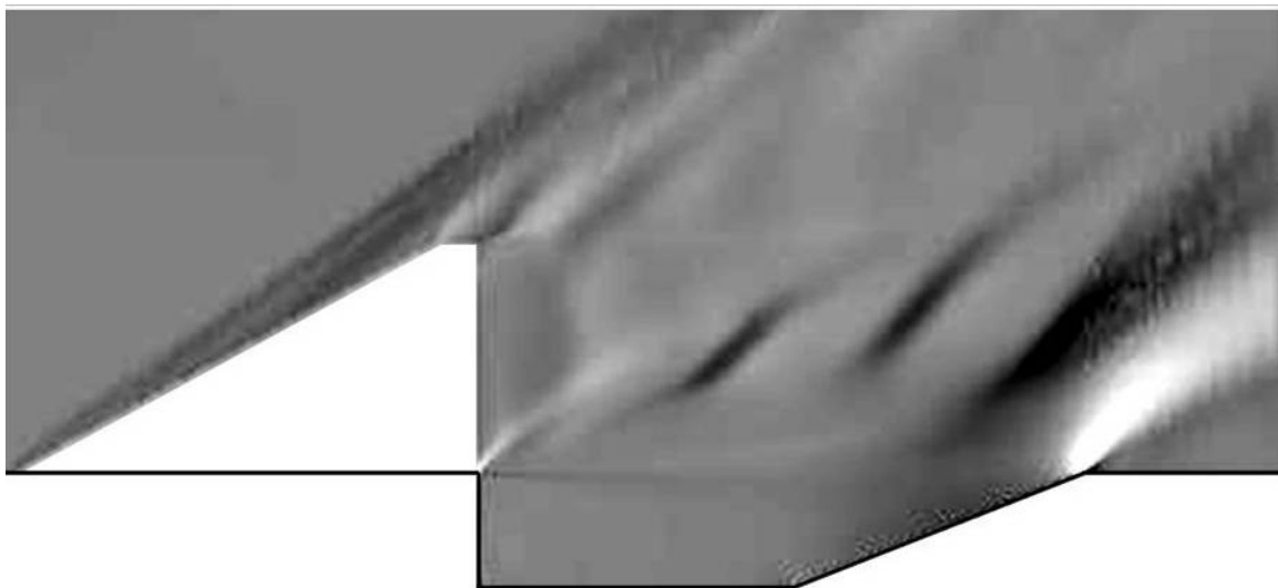
Figure 32. CFD density gradient (data from z = 0, 2, 4, 6 \text{ cm} ; grey scale of dp/dx ; Re\# \approx 42 \times 10^6 \text{ m}^{-1} , M = 2 )
