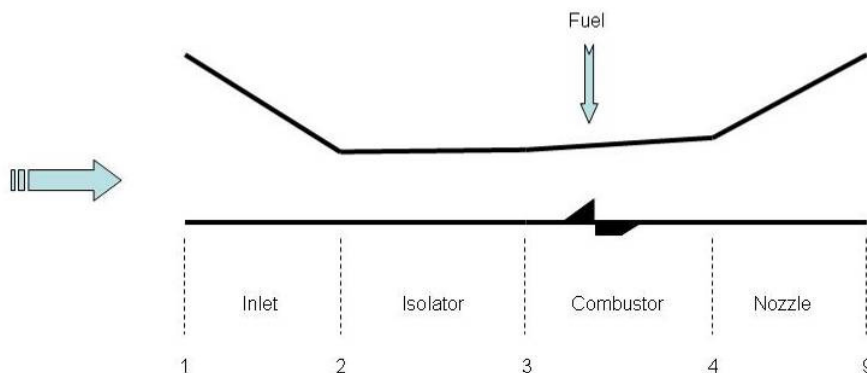
Figure 4. Scramjet engine reference stations
