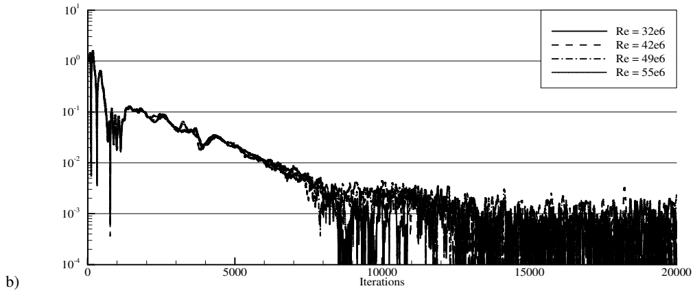
Figure 30. Test section convergence history a) without pylon and b) with pylon {plot of |\dot{m}_{in} - \dot{m}_{out}| / |\dot{m}_{in} - \dot{m}_{out}|_{n=1} }
