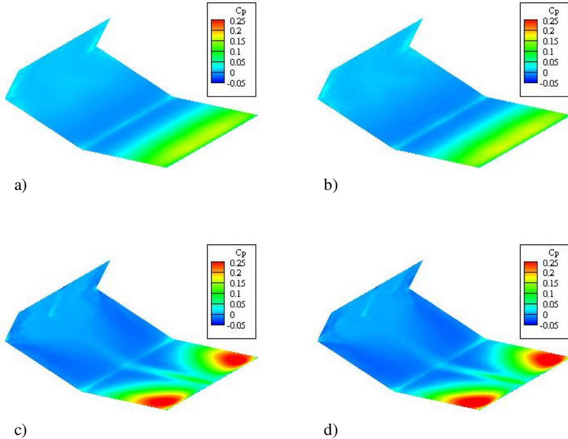
Figure 36. CFD cavity surface pressure coefficient a) cavity-only, Re \approx 32 \times 10^6 \text{ m}^{-1} ; b) cavity-only, Re \approx 55 \times 10^6 \text{ m}^{-1} ; c) pylon-cavity, Re \approx 32 \times 10^6 \text{ m}^{-1} ; and d) pylon-cavity, Re \approx 55 \times 10^6 \text{ m}^{-1}
