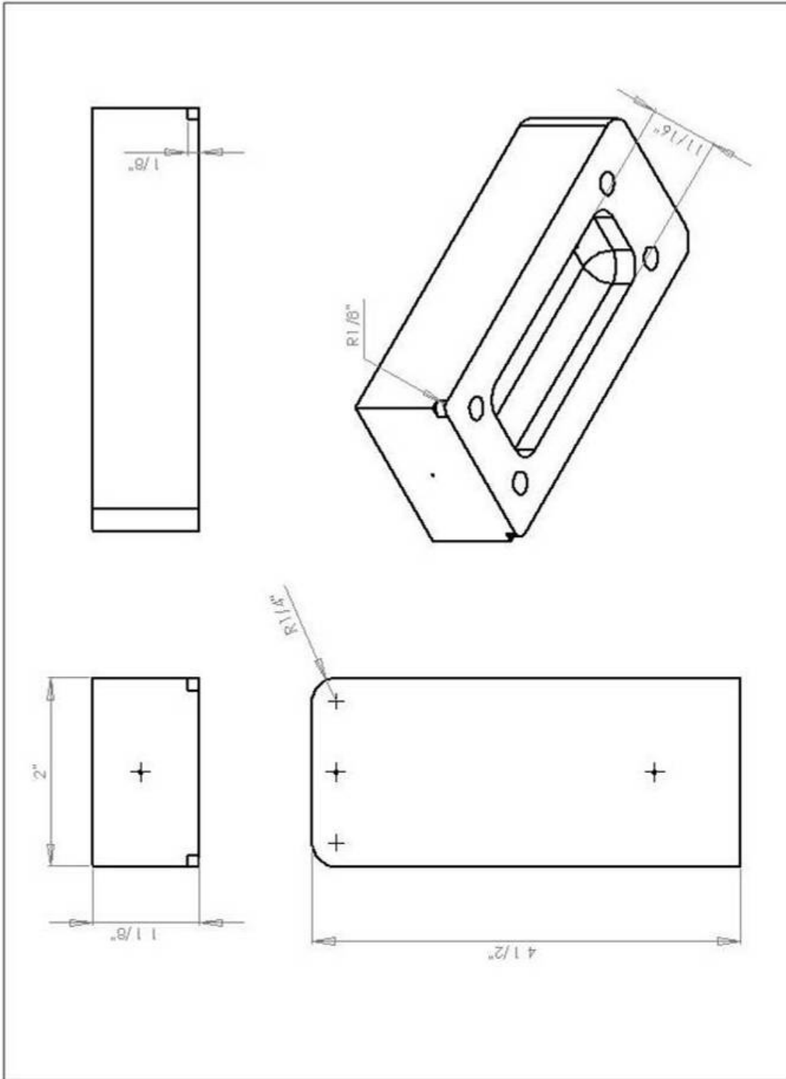
Figure 75. Plain insert
