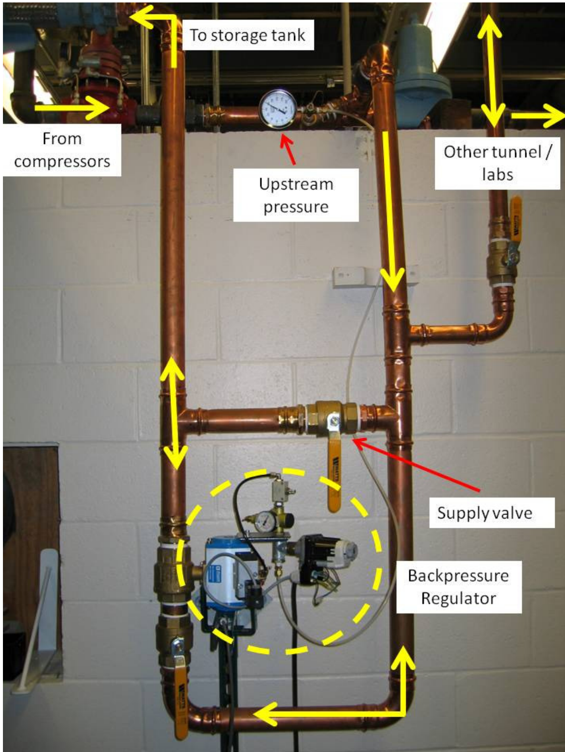
Figure 80. Supply valves configured for operation with the backpressure regulator
