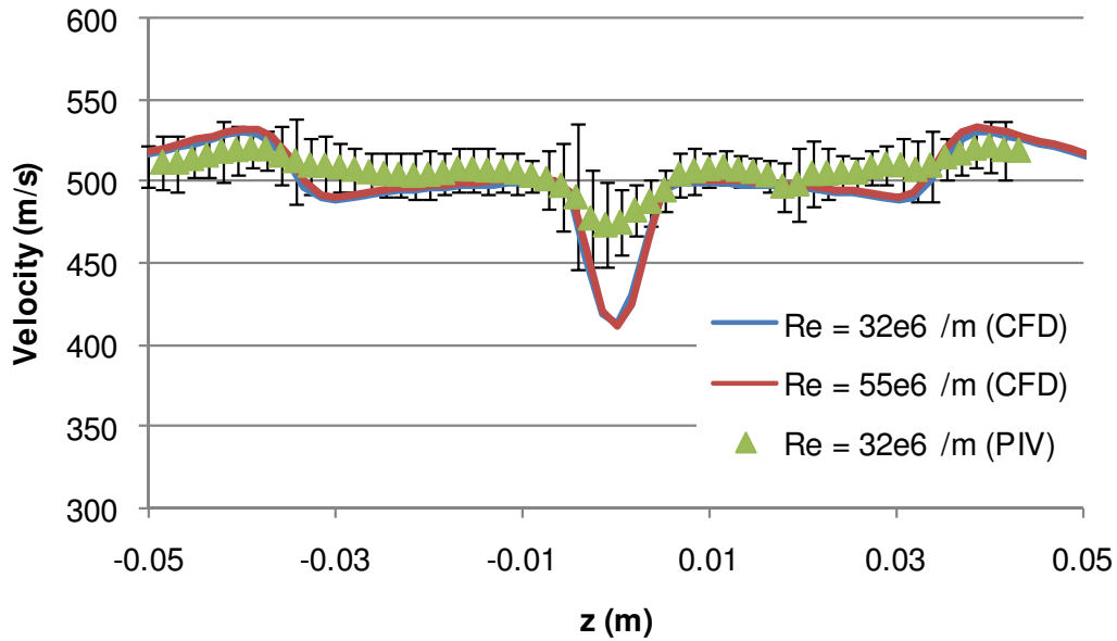
Figure 50. PIV and CFD velocity magnitude across test section with pylon ( x = 8.8 cm, y = 3.7 cm, CFD velocities corrected for temperature differences)
