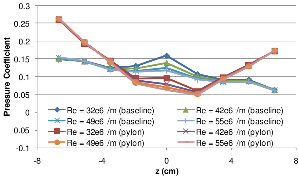
Figure 104. Surface pressure coefficients with and without a pylon installed (x = 10.9 cm, y = -0.95 cm)
