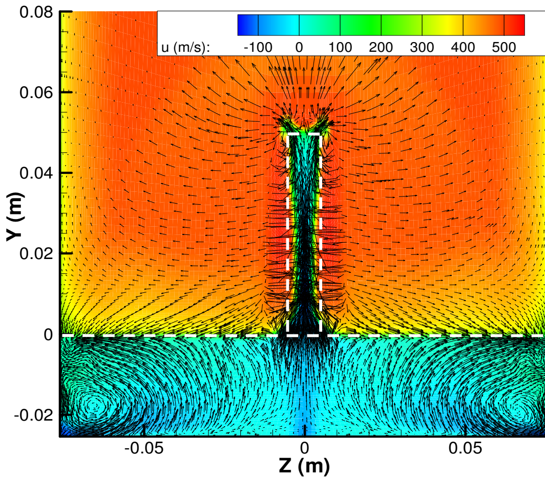
Figure 52. Velocity vectors in y-z plane at x = 1 cm across full span of test section (contours of x velocity; Re \approx 32 \times 10^6 \text{ m}^{-1} )
