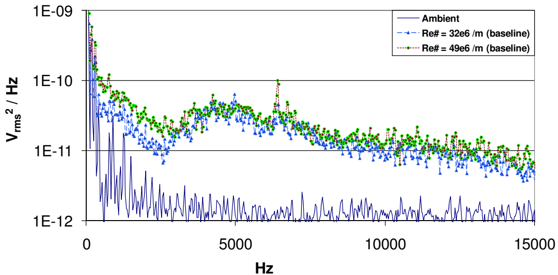
Figure 59. Pressure fluctuation power spectrum at ambient conditions (baseline cavity)
