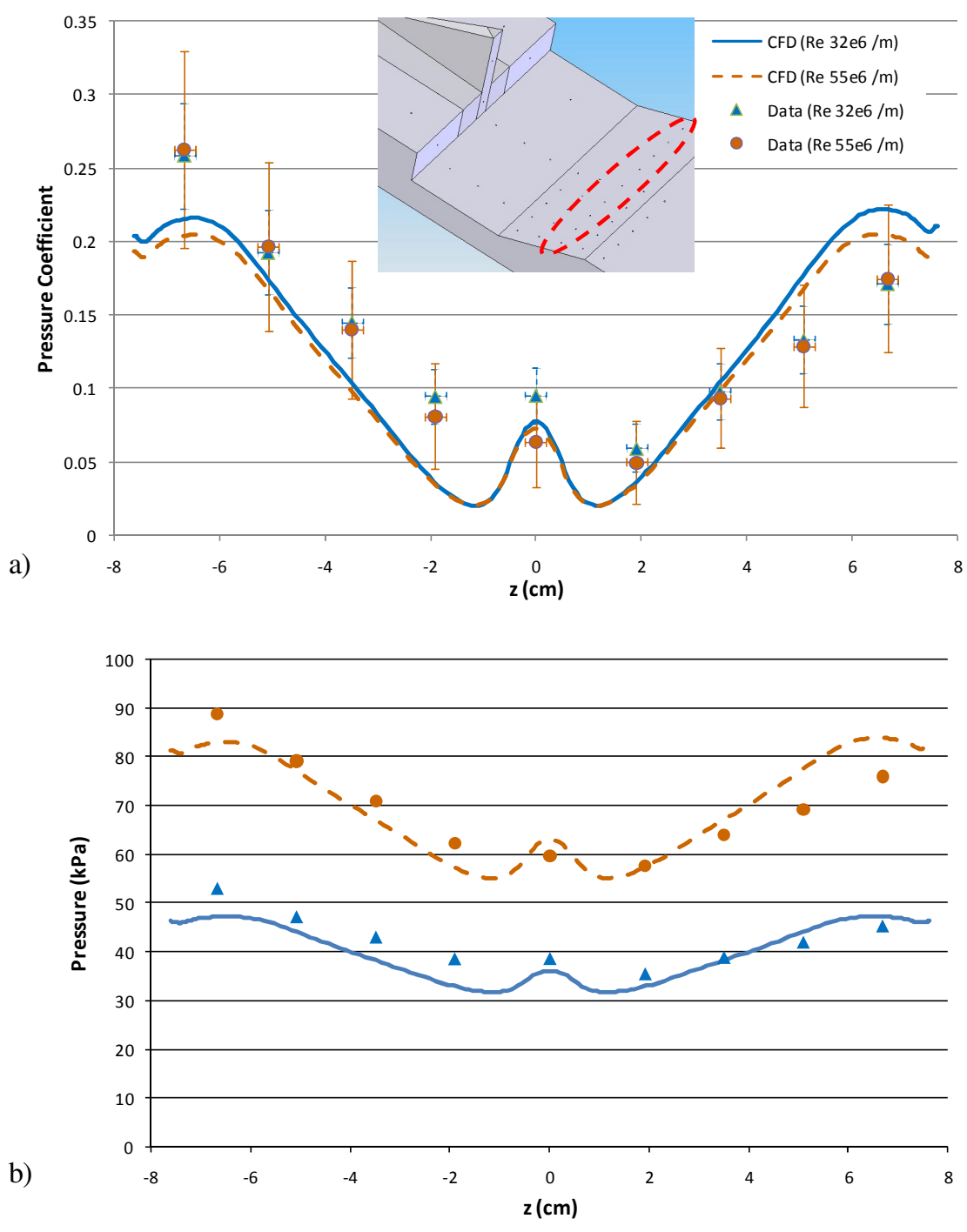
Figure 38. Cross ramp pressures near shear layer impingement: a) pressure coefficient and b) absolute pressure ( x = 10.8 cm, y = -0.94 cm)
