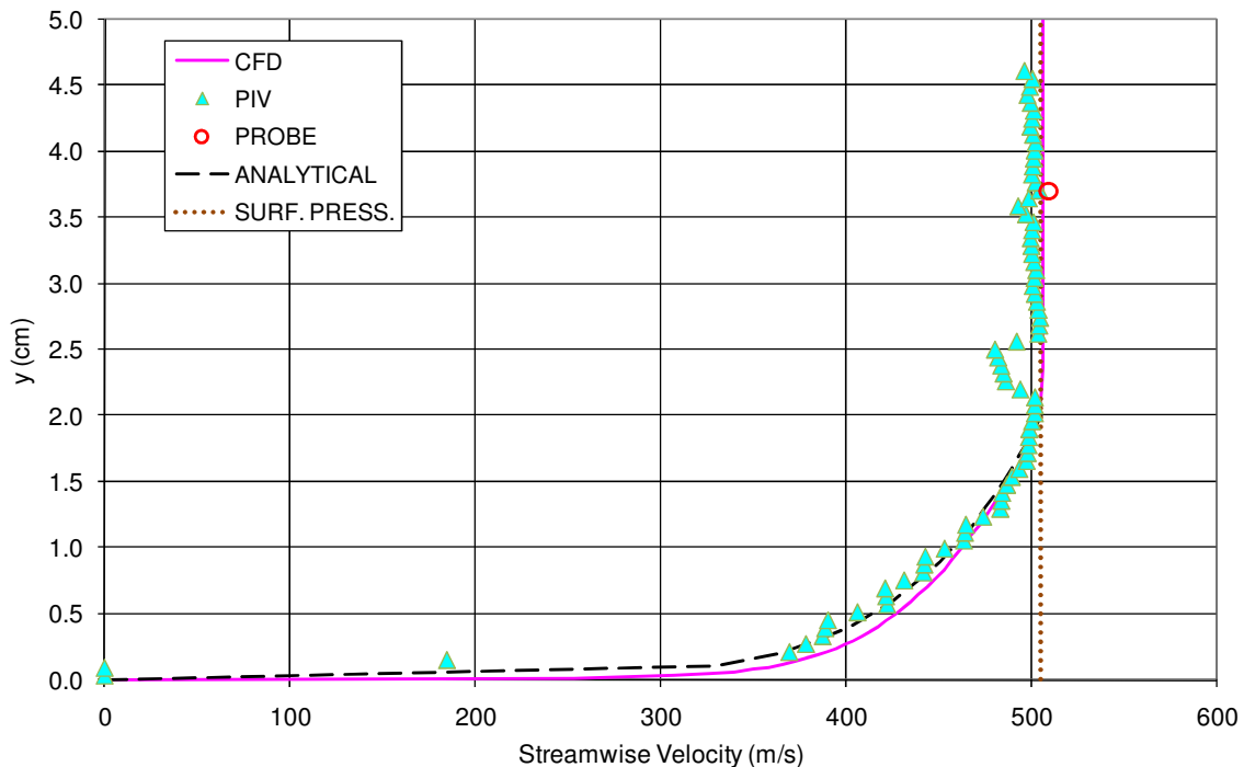
Figure 25. Boundary layer entering the test section ( x \approx -12 cm, z \approx 2.5 cm; Re \approx 32 \times 10^6 \text{ m}^{-1} ; probe data at x = -22 cm; surface pressure data at x = -10.8 cm; velocity corrected for temperature variation)
