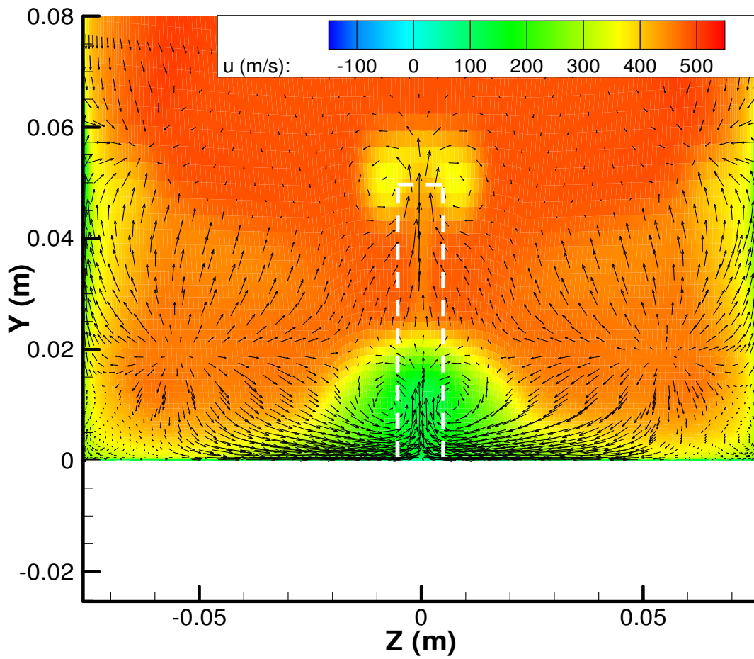
Figure 55. Velocity vectors in y-z plane at x = 15 cm across full span of test section (contours of x velocity; Re \approx 32 \times 10^6 m^{-1} )
