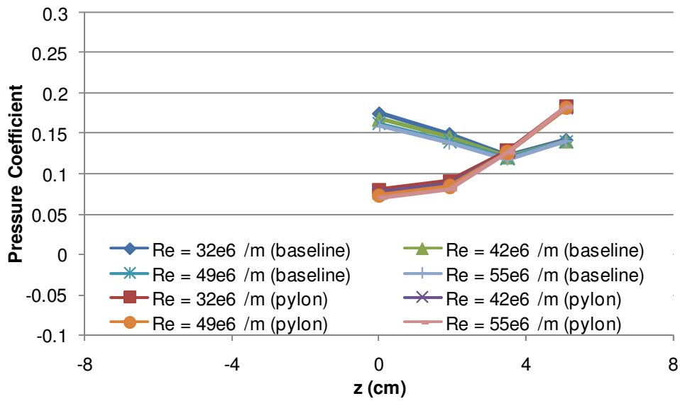
Figure 105. Surface pressure coefficients with and without a pylon installed (x = 12.4 cm, y = -0.32 cm)
