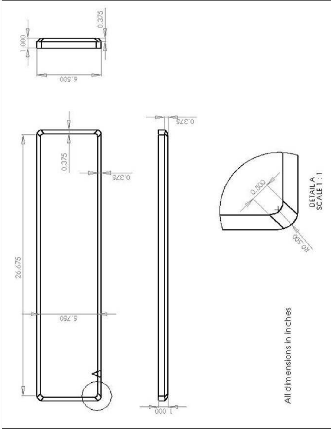
Figure 71. Test section side window
