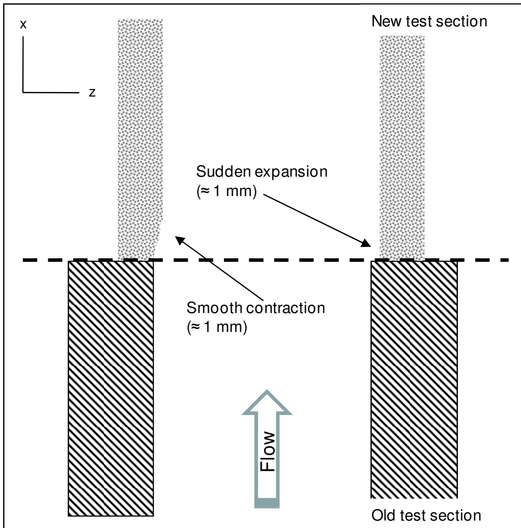
Figure 77. Representation of the new test section junction (not to scale)
