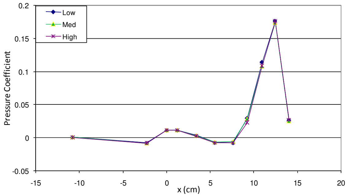
Figure 94. Grid convergence (centerline pressure coefficient)
