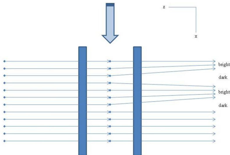
Figure 21. Refraction of parallel light beams passing through the test section used in Shadowgraph/Schlieren photography [56]
