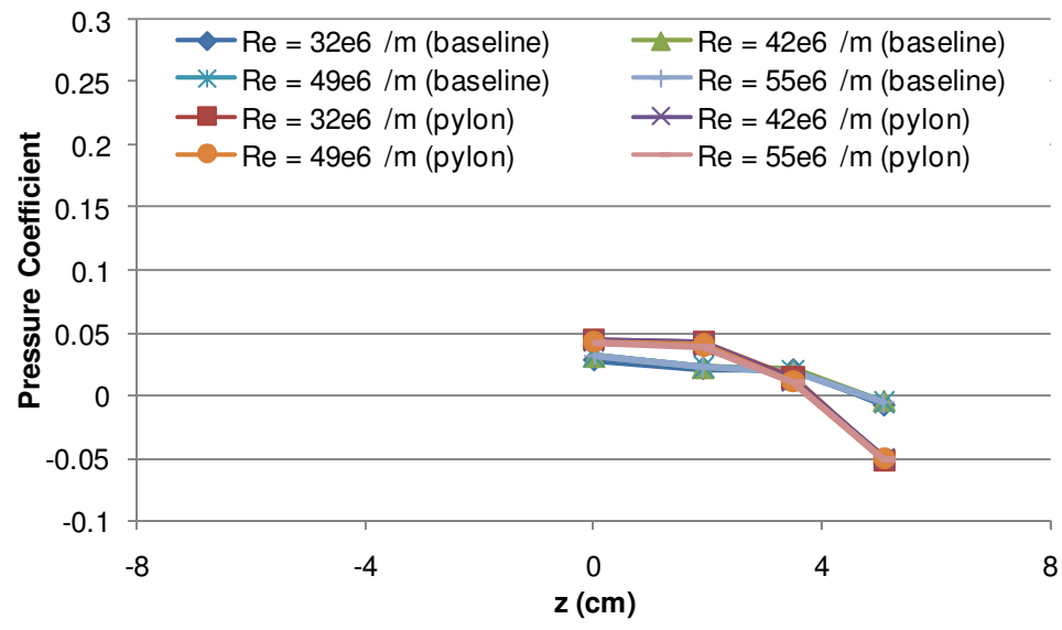
Figure 106. Surface pressure coefficients with and without a pylon installed (x = 14.0 cm, y = 0 cm)
