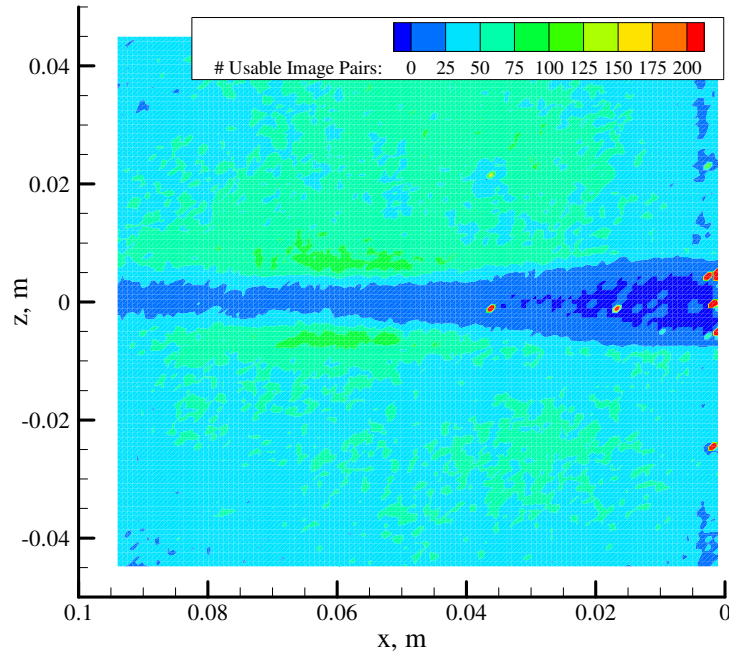
Figure 47. Number of usable PIV image pairs in wake flow 3.7 cm above the cavity (corresponds to Figure 46a; Re \approx 32 \times 10^6 \text{ m}^{-1} )
