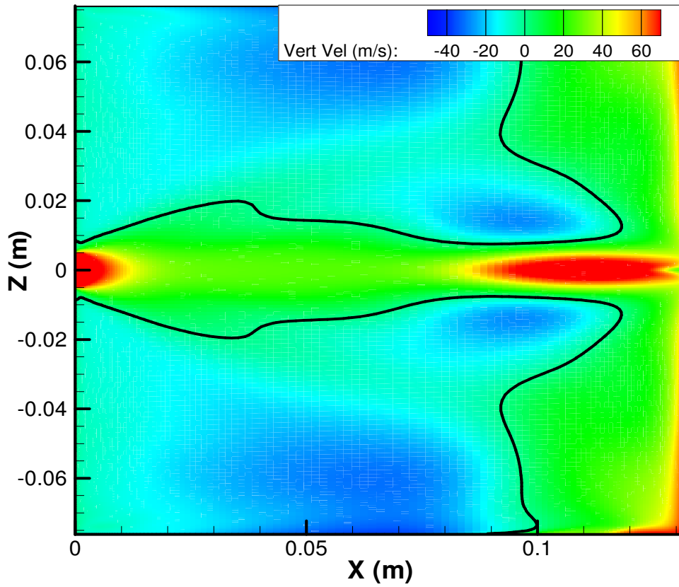
Figure 62. Vertical velocity contours at the top cavity boundary ( y = 0 cm) for Re\# \approx 32 \times 10^6 \text{ m}^{-1} (pylon installed; black line indicates zero vertical velocity)
