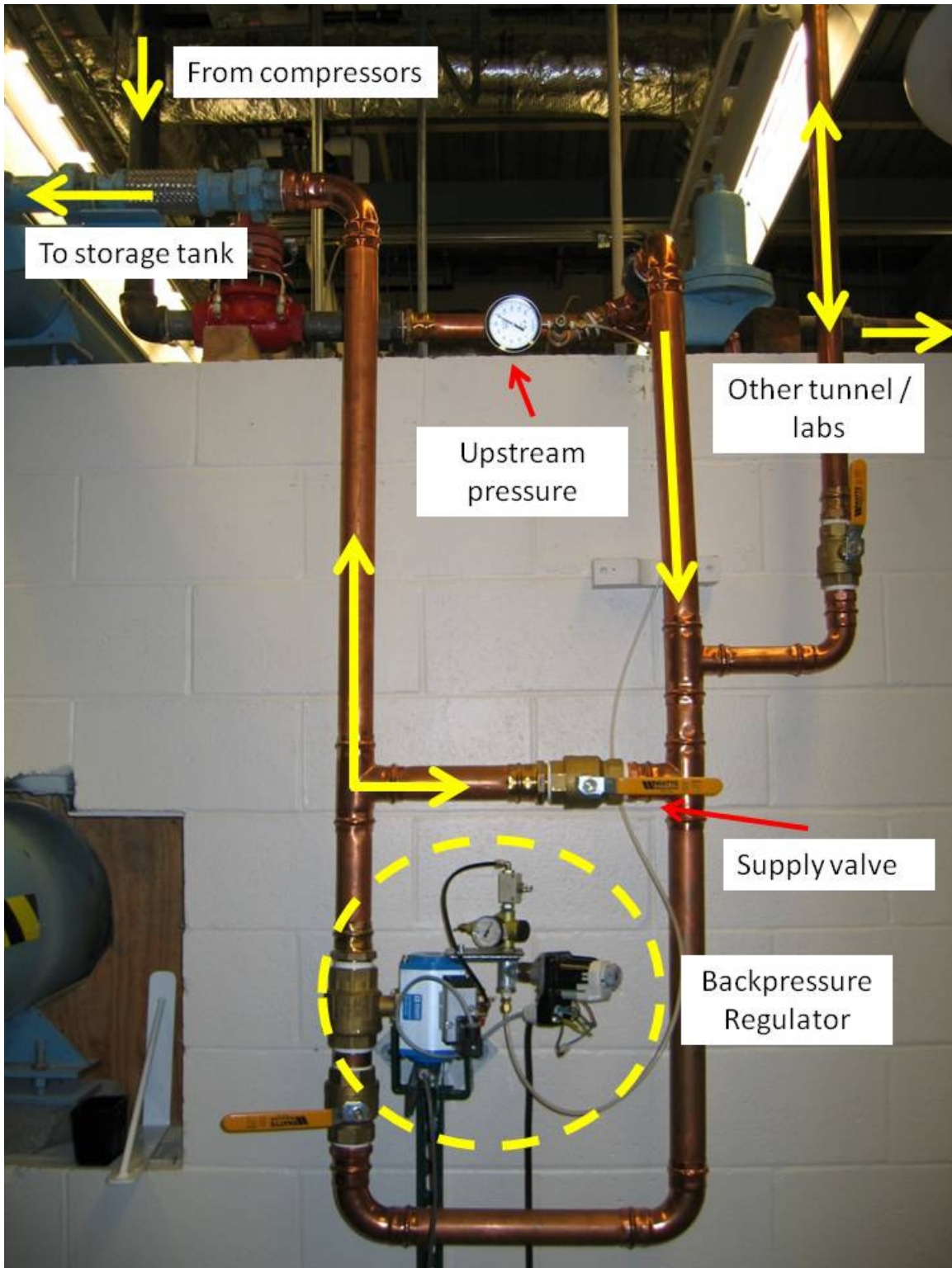
Figure 79. Supply valves configured for operation without the backpressure regulator
