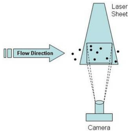
Figure 22. Two-dimensional PIV component relationships
