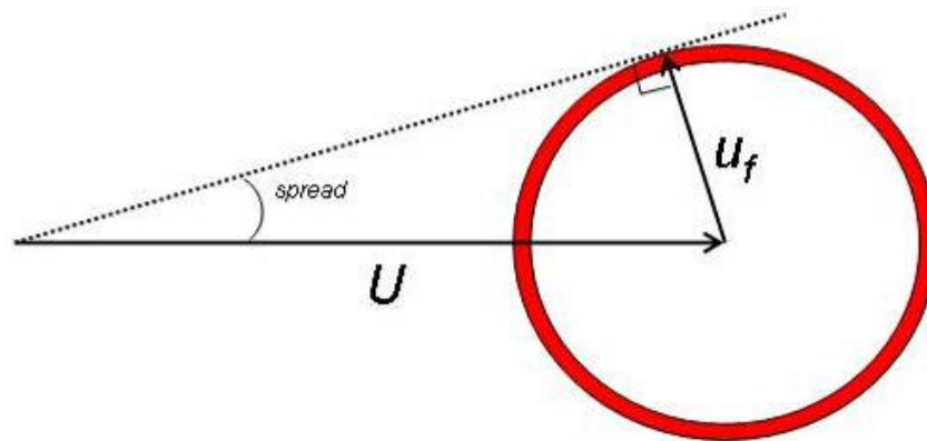
Figure 10. Flame spread geometry
