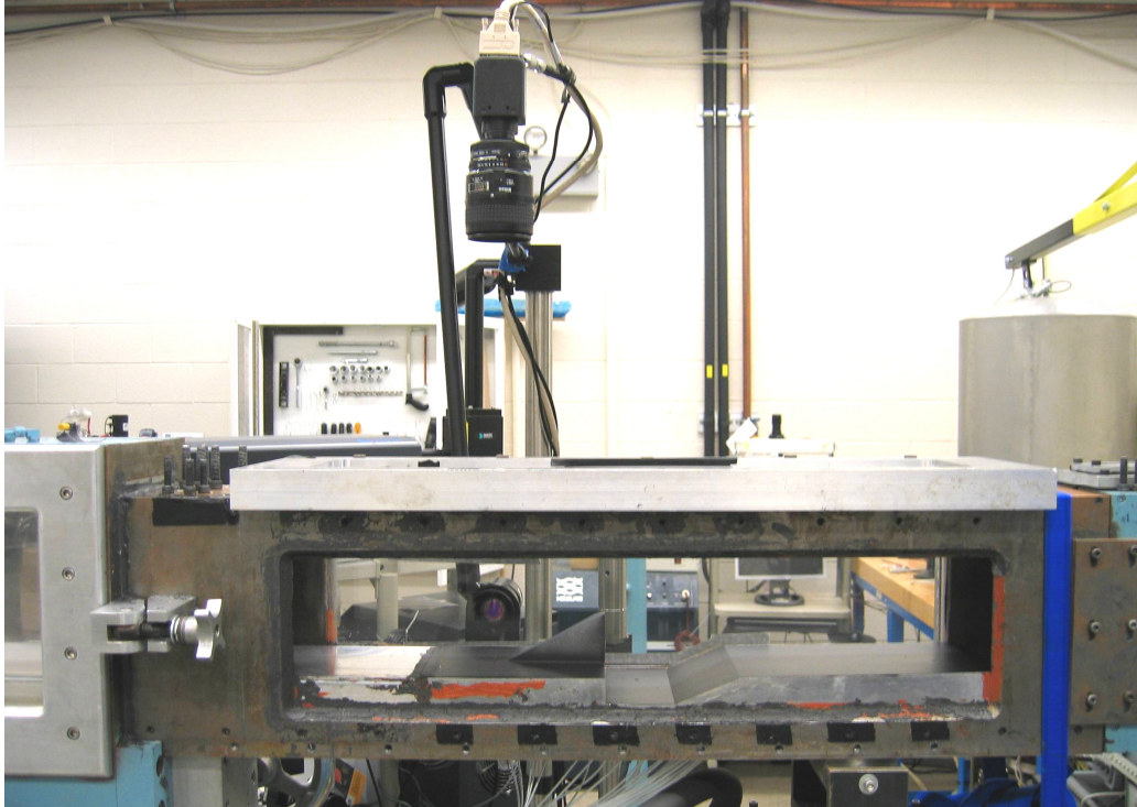
Figure 16. AFIT 6' x 6' Supersonic Wind Tunnel add-on test section with pylon installed and configured for PIV (near-side window and probe plate removed)
