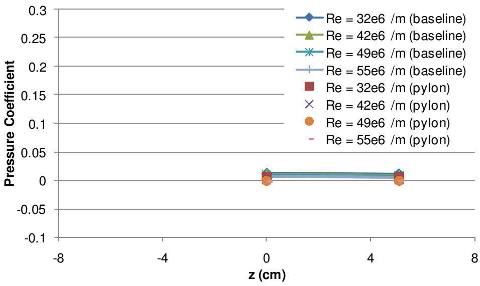
Figure 99. Surface pressure coefficients with and without a pylon installed (x = 1.2 cm, y = -2.54 cm)
