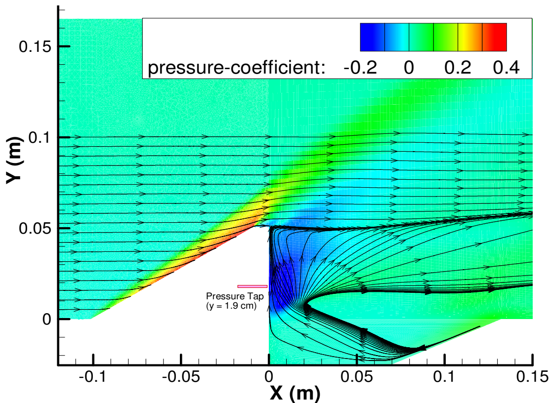
Figure 41. CFD centerline pressure coefficient with streamlines ( Re \approx 32 \times 10^6 \text{ m}^{-1} )
