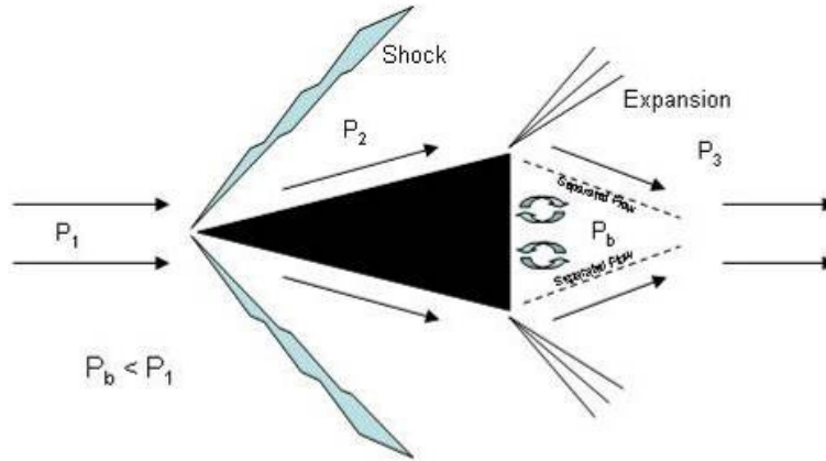
Figure 12. Two-dimensional pylon shock/expansion system
