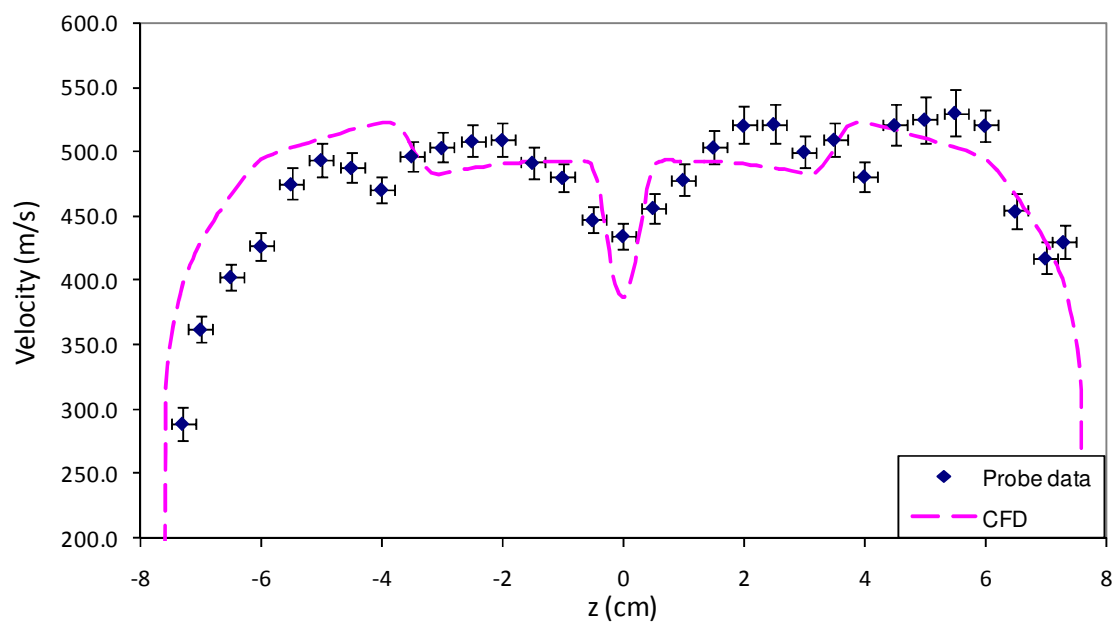
Figure 39. Streamwise velocities measured above the cavity ramp (probe data, x = 8.8 cm, y = 3.7 cm, Re \approx 32 \times 10^6 \text{ m}^{-1} )
