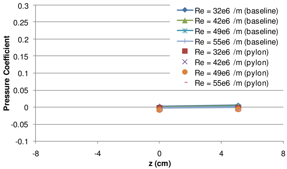
Figure 101. Surface pressure coefficients with and without a pylon installed (x = 5.5 cm, y = -2.54 cm)
