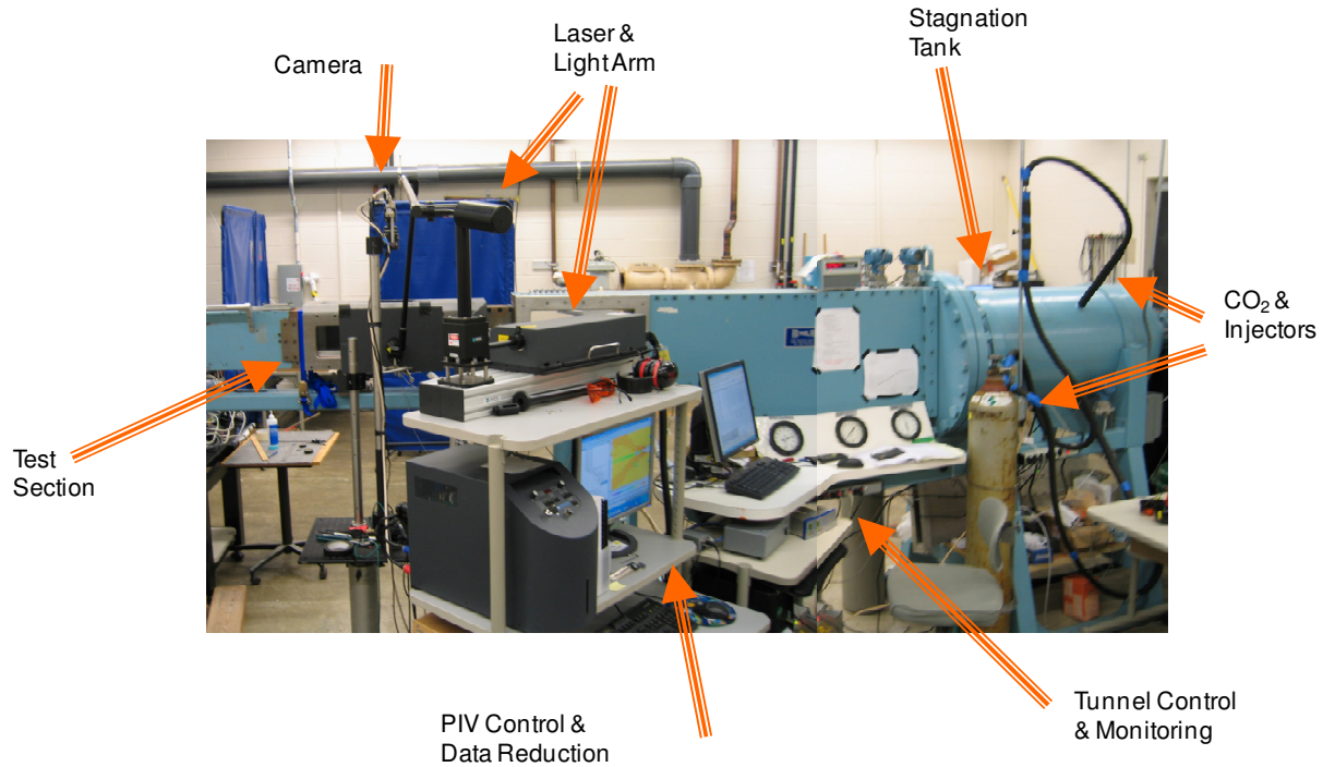
Figure 14. AFIT 6' x 6' Supersonic Wind Tunnel
