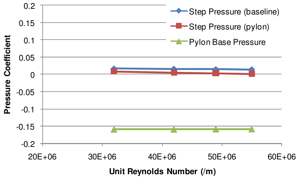
Figure 98. Cavity step pressure (with and without pylon installed) and pylon base pressure
