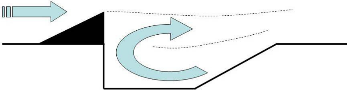
Figure 11. Cavity flameholder with inclined downstream ramp and leading edge pylon (on centerline)
