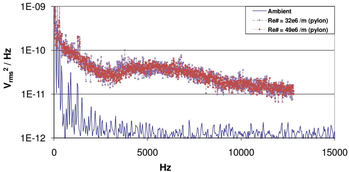
Figure 60. Pressure fluctuation power spectrum at ambient conditions (pylon-cavity)
