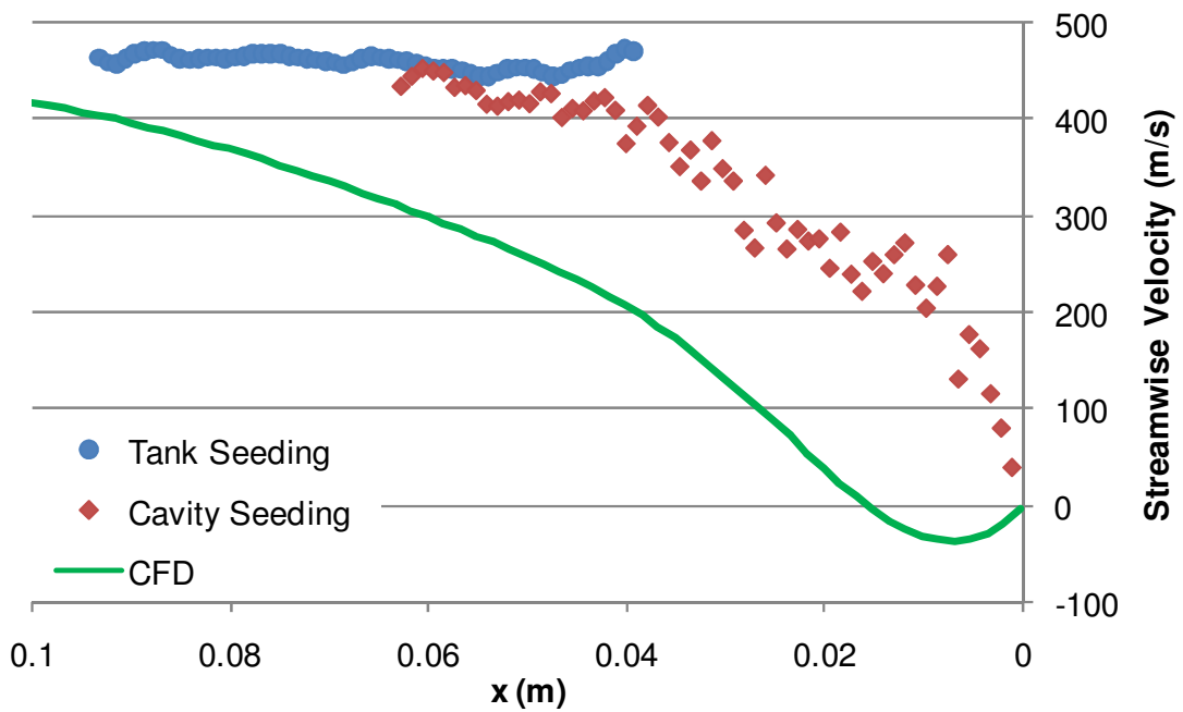
Figure 51. Streamwise velocity behind pylon ( y = 3.7 \text{ cm} , z = 0 \text{ cm} , Re \approx 32 \times 10^6 \text{ m}^{-1} )
