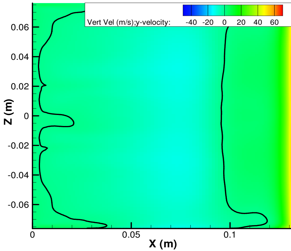
Figure 63. Vertical velocity contours at the top cavity boundary ( y = 0 cm) for Re\# \approx 32 \times 10^6 \text{ m}^{-1} (baseline cavity; black line indicates zero vertical velocity)
