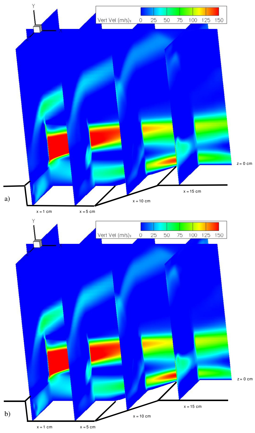
Figure 45. CFD vertical velocity contours a) Re \approx 32 \times 10^6 \text{ m}^{-1} ; and b) Re \approx 55 \times 10^6 \text{ m}^{-1}
