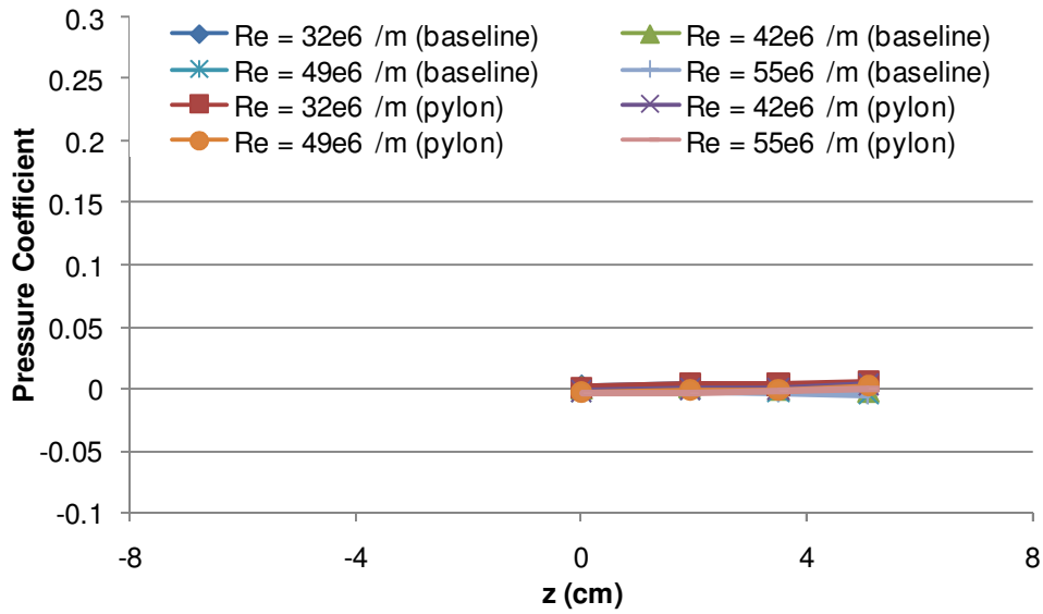
Figure 102. Surface pressure coefficients with and without a pylon installed (x = 7.6 cm, y = -2.2 cm)
