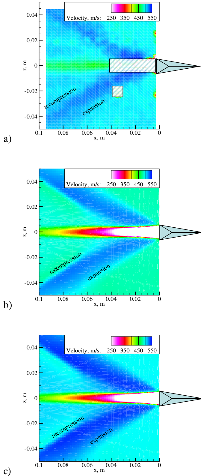
Figure 46. Velocity magnitude behind pylon 3.7 cm above the cavity a) PIV data ( Re \approx 32 \times 10^6 \text{ m}^{-1} ); b) CFD data ( Re \approx 32 \times 10^6 \text{ m}^{-1} and T_t = 273 \text{ K} ); c) CFD data ( Re \approx 55 \times 10^6 \text{ m}^{-1} and T_t = 287 \text{ K} ) (flow from right; hatched area unusable due to low particle density and surface reflections )
