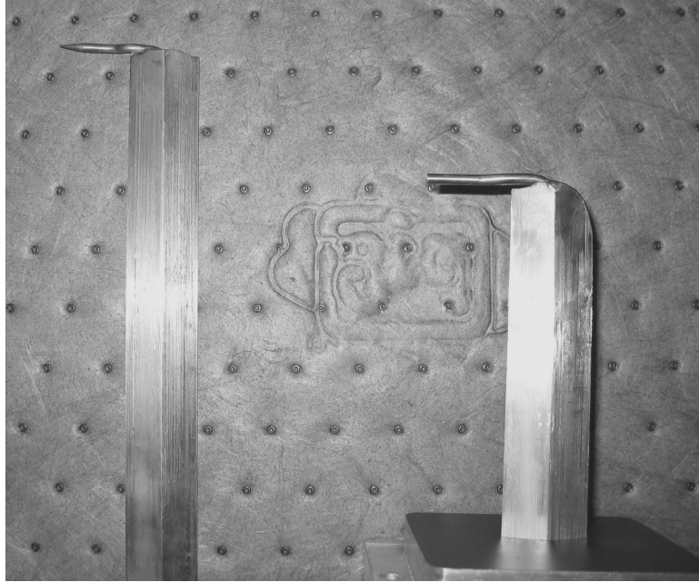
Figure 20. Static and pitot probes
