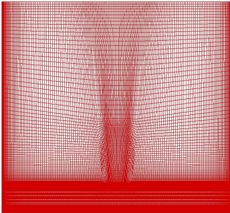
Figure 28. Cross-stream mesh from cavity floor to tunnel ceiling ( x = 5 cm)
