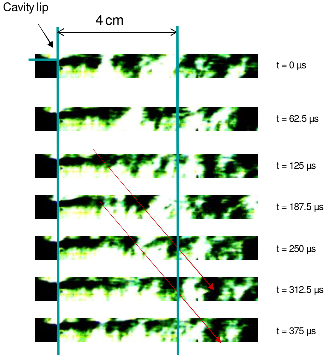
Figure 61. High-speed Schlieren frames of flow separating at the leading edge of the cavity showing structures propagating downstream (baseline cavity, Re\# \approx 42 \times 10^6 \text{ m}^{-1} )
