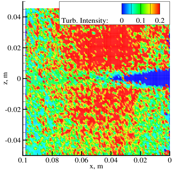
Figure 91. Turbulence intensity behind pylon 3.7 cm above the cavity (PIV; Re \approx 32 \times 10^6 \text{ m}^{-1} ; corresponds to Figure 46)
