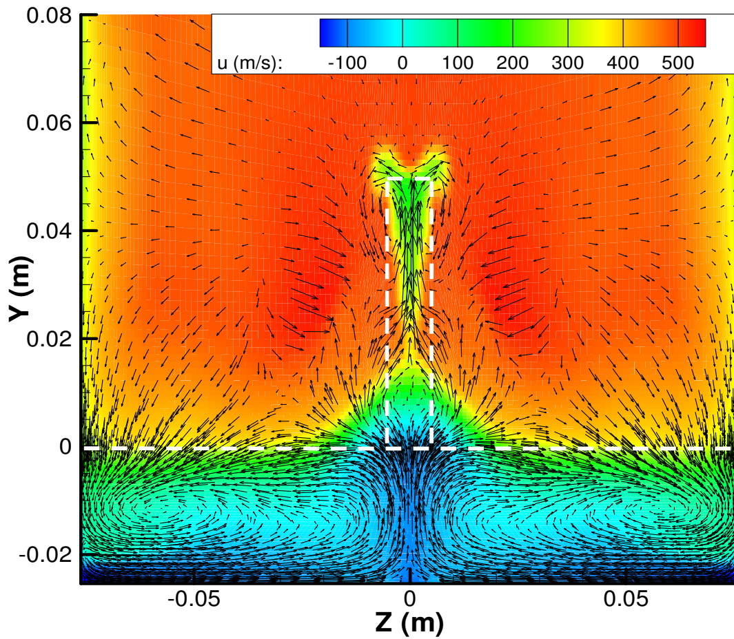
Figure 53. Velocity vectors in y-z plane at x = 5 cm across full span of test section (contours of x velocity; Re \approx 32 \times 10^6 \text{ m}^{-1} )
