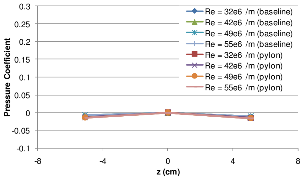
Figure 96. Surface pressure coefficients with and without a pylon installed ( x = -10.8 cm)
