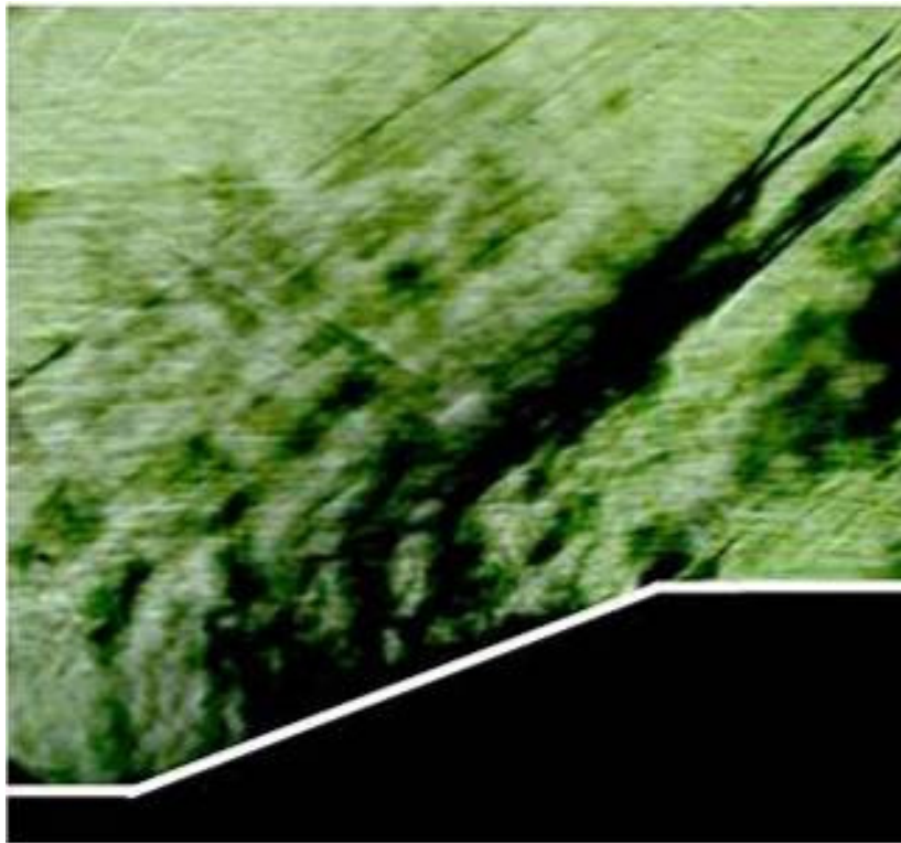
Figure 35. Instantaneous Schlieren photograph of flow over the downstream ramp ( Re\# \approx 42 \times 10^6 \text{ m}^{-1} ; 1/64000 sec exposure time)
