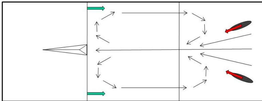
Figure 64. Notional cavity fuel-air injection scheme
