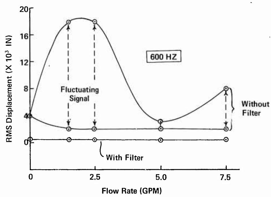
Figure 9. Vibration Displacement Measurements At Resonant Frequencies and 600 Hz With and Without an 110 Hz High-Pass Filter
