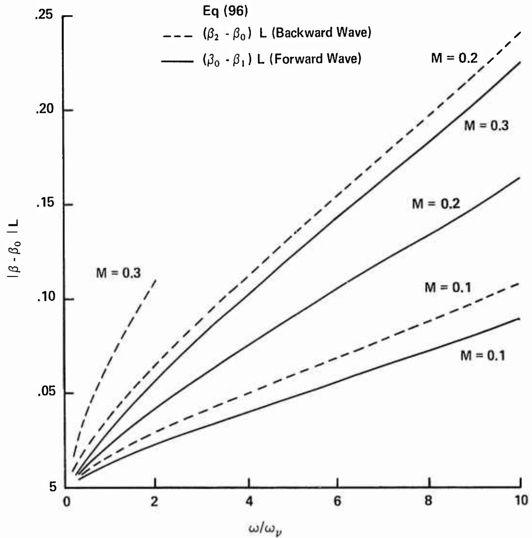
Figure 52. Phase Constant Deviation Versus \omega/\omega_p (AIR, T = 50°F, ID = 1/8 In, L = 23.245 In)
