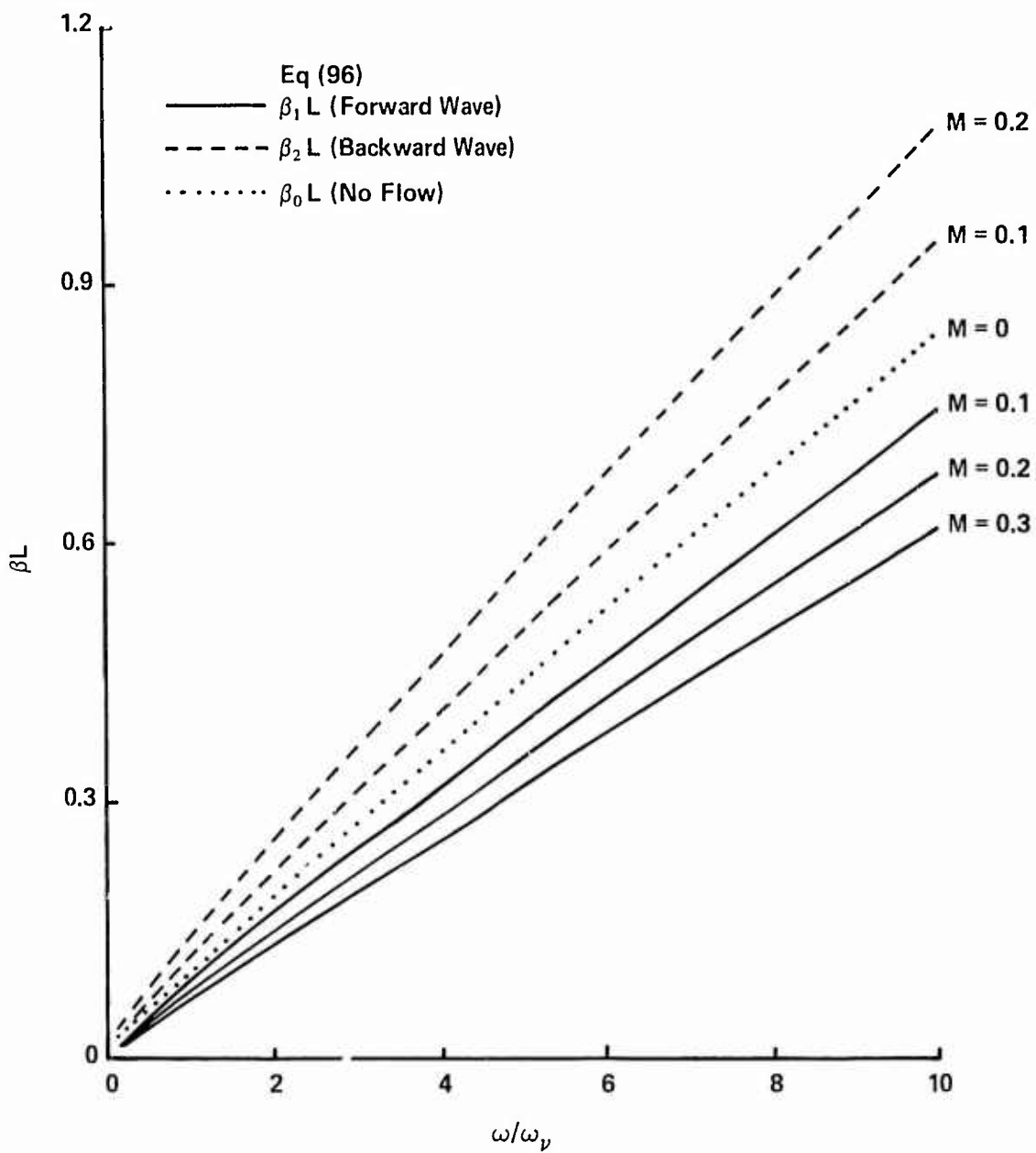
Figure 49. Phase Constant Versus \omega/\omega_p For Mach Numbers From 0 to 0.3 (AIR, T = 59° F, ID = 1/8 In, L = 23.245 In)
