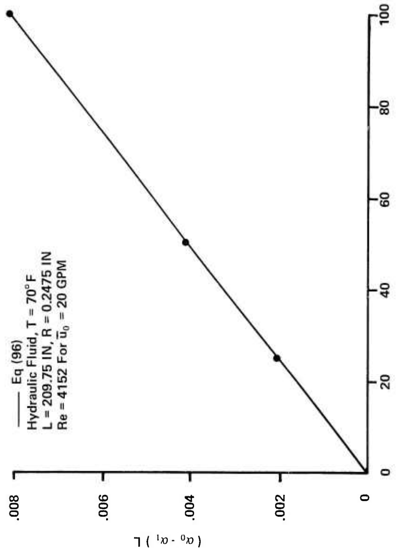
Figure 29. Attenuation Deviation For Large Flow Rates (Turbulent) \omega_y = 1.0 Hz, \omega/\omega_p = 183.5
