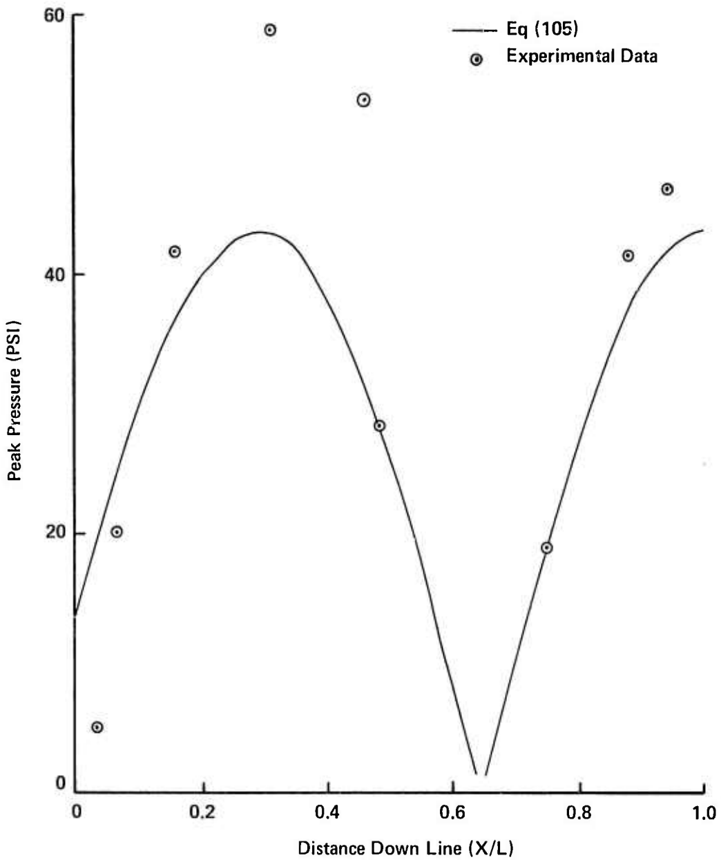
Figure 42. Standing Pressure Half Wave For A Mean Flow Of 0 GPM (Straight Hydraulic Line, \omega = 180 Hz, T = 75^\circ F, L = 209.75 In, R = 0.2475 In)
