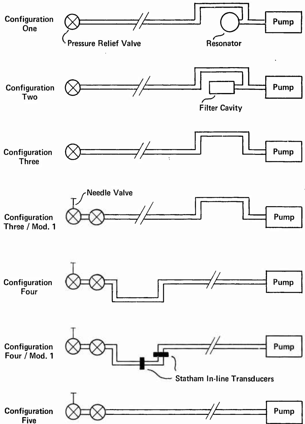
Figure 3. Line Configurations
