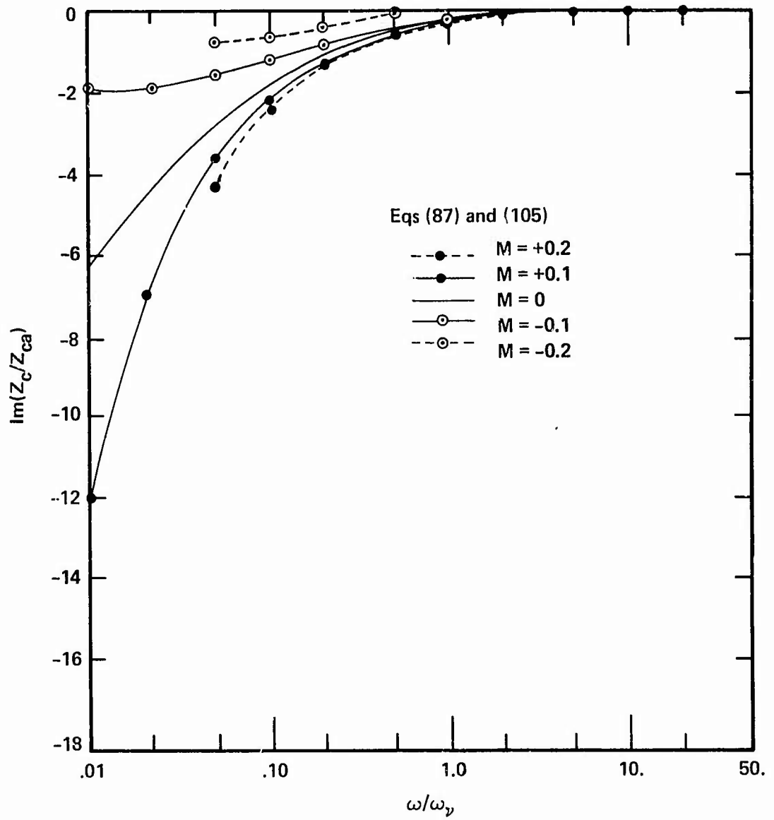
Figure 68. Imaginary Part Of The Normalized Characteristic Impedance Versus \omega/\omega_y
