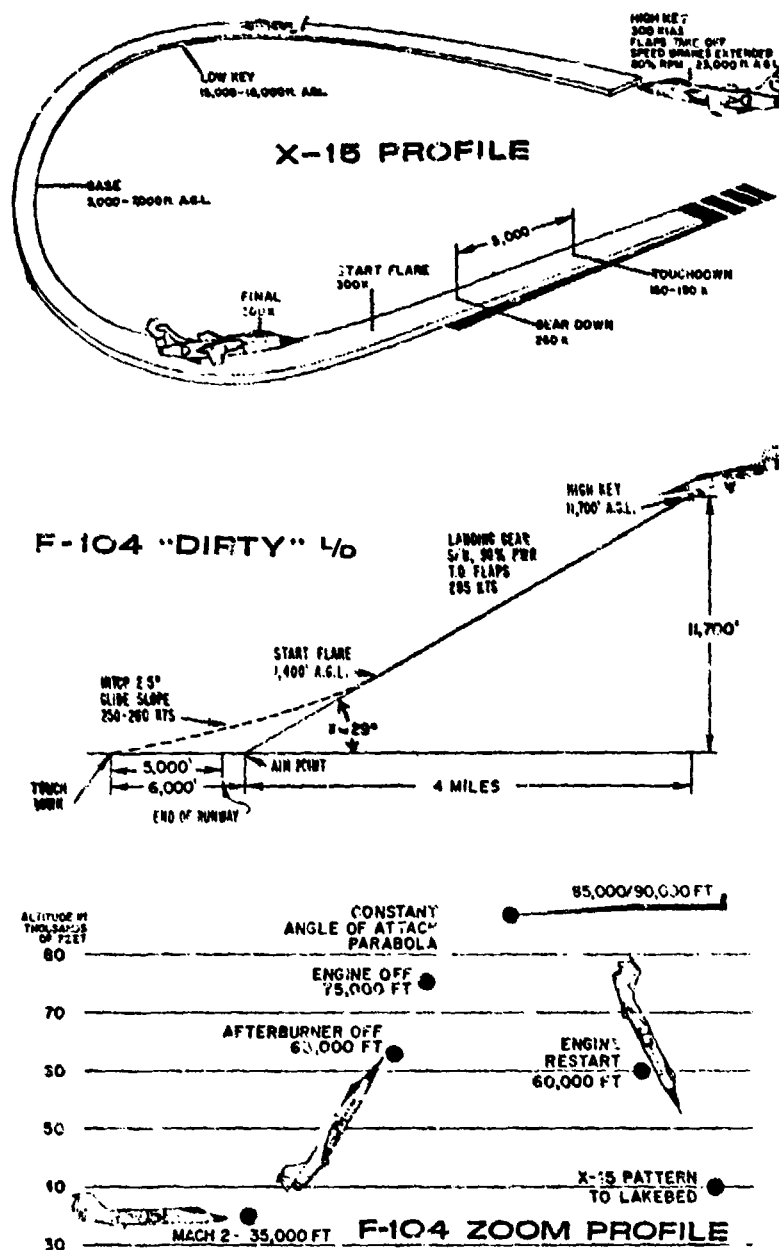
Figure 1: Some F-104D SSCE Evaluation Tasks (Illustrations from Ref. 12)
