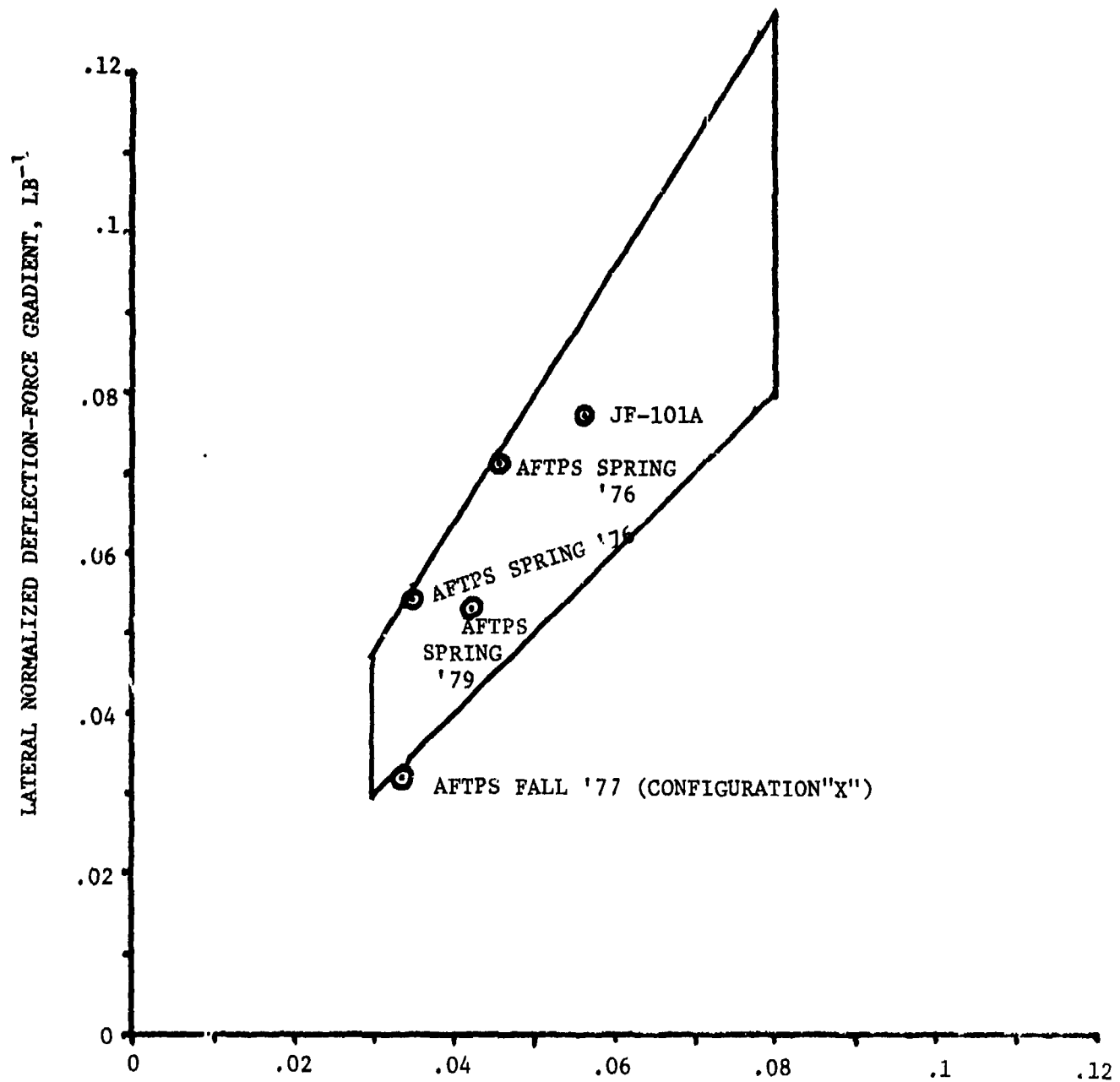
FIGURE 13: PREFERRED CONTROL HARMONY
