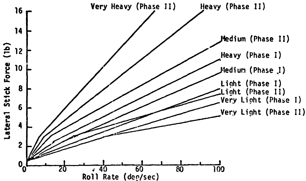
FIG 10: LATERAL CONFIGURATIONS EVALUATED IN REFS 2 AND 3 (FIG FROM REF 7)
