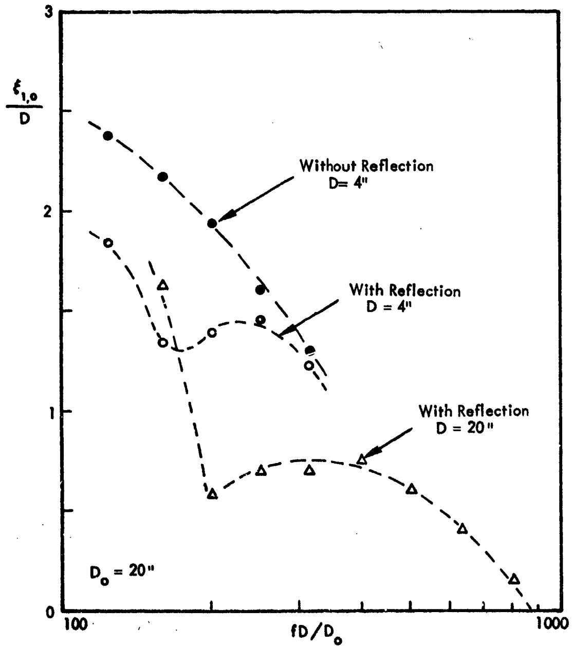
FIG. 44. EFFECT OF REFLECTION FROM PERPENDICULAR PLANE ON ZERO CROSSING POINT OF CORRELATION COEFFICIENT IN LONGITUDINAL DIRECTION [65].
