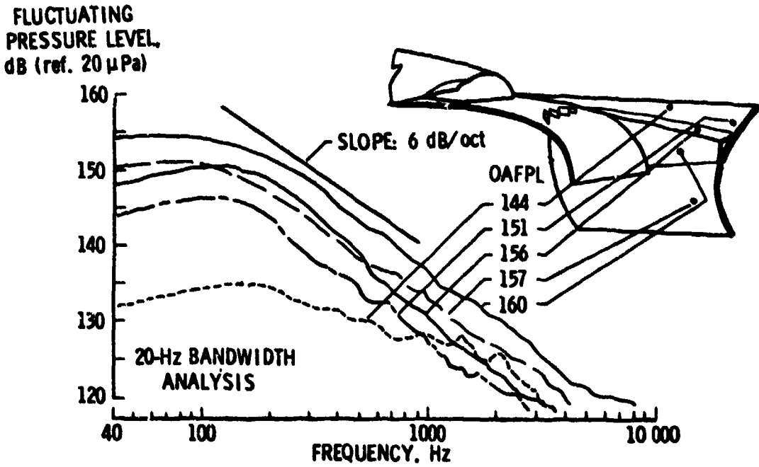
FIG. 61. FLUCTUATING PRESSURES ON FUSELAGE SIDEWALL OF YC-14 SCALE MODEL [79].
