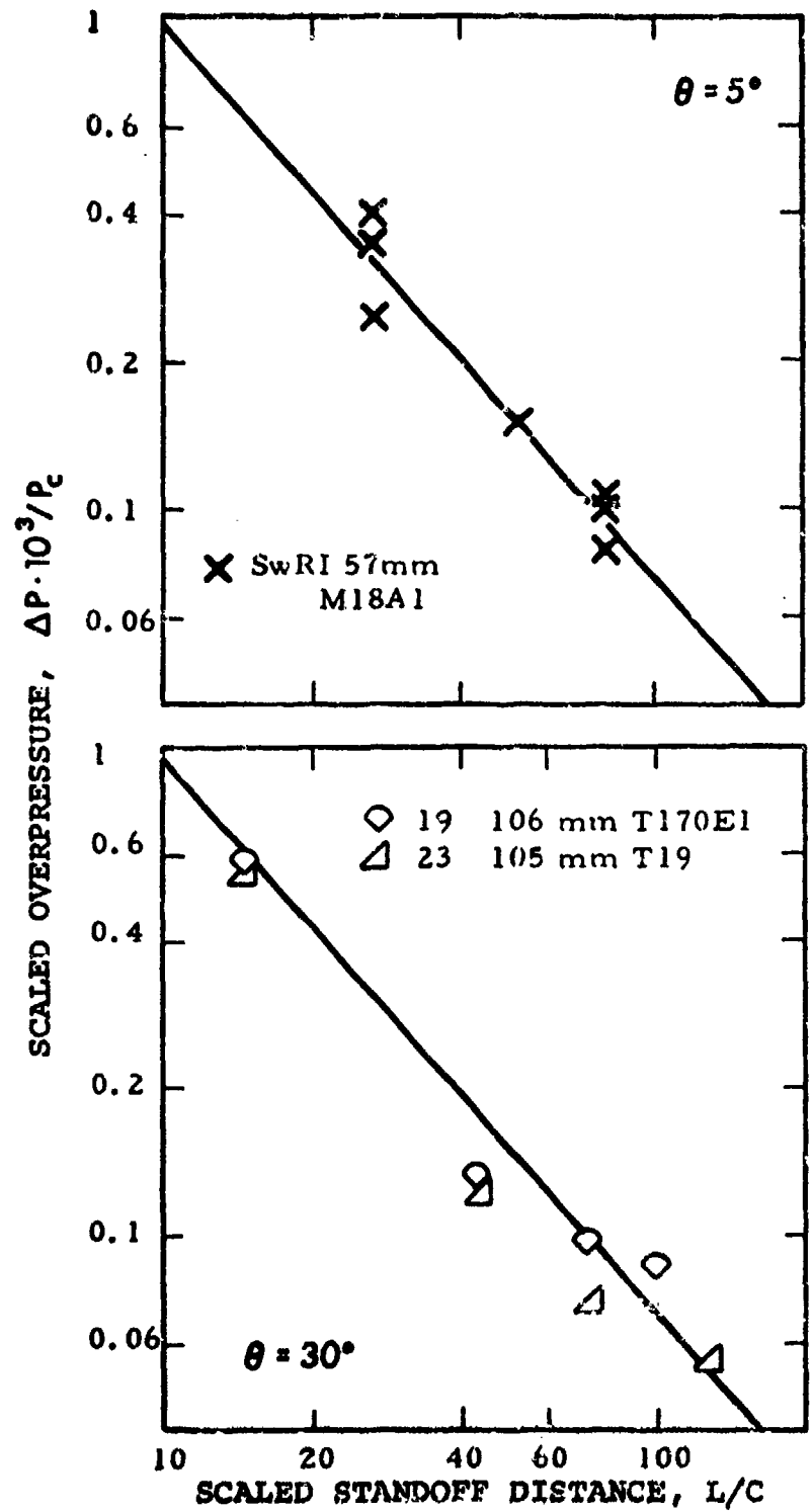
FIG. 135. OVERPRESSURES OF RECOILLESS RIFLE AHEAD OF MUZZLE AT 5^\circ AND 30^\circ FROM AXIS [138].
