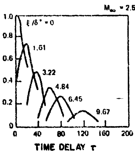
FIG. 105. NORMALIZED BROAD BAND STREAMWISE SPACE TIME CORRELATION FUNCTIONS FOR SEPARATED FLOW [112]
