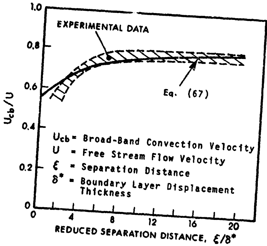
FIG. 86. VARIATION OF BROAD-BAND CONVECTION VELOCITY WITH STREAMWISE SEPARATION DISTANCE.
