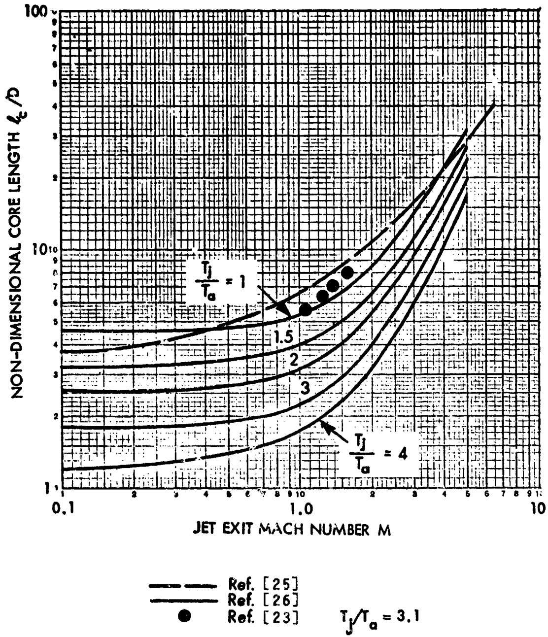
FIG. 14. JET CORE LENGTH AS FUNCTION OF JET TEMPERATURE AND MACH NUMBER.
