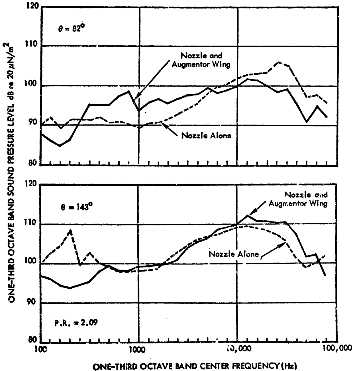
FIG. 77. FAR FIELD ACOUSTIC SPECTRA FOR MODEL NOZZLE WITH AND WITHOUT AUGMENTOR WING [85].
