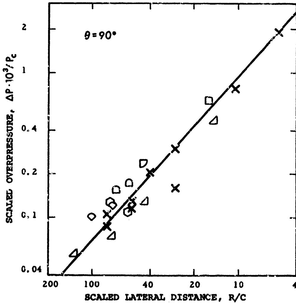
FIG. 136. OVERPRESSURES OF RECOILLESS RIFLE, TO SIDE OF MUZZLE [138].
