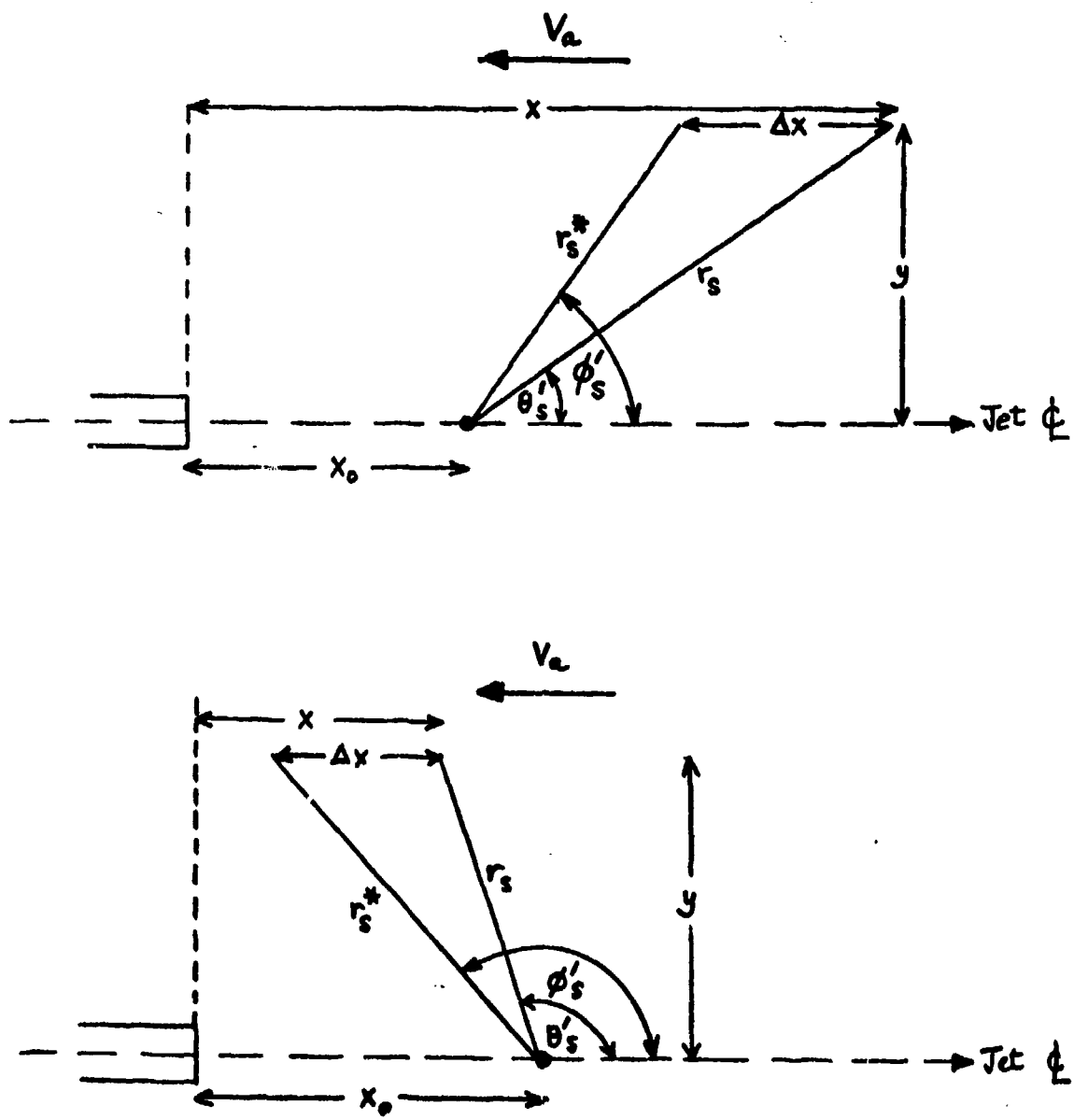
FIG. 29. GEOMETRICAL RELATIONSHIP BETWEEN RECEIVER AND SOURCE FOR FORWARD MOTION EFFECT.
