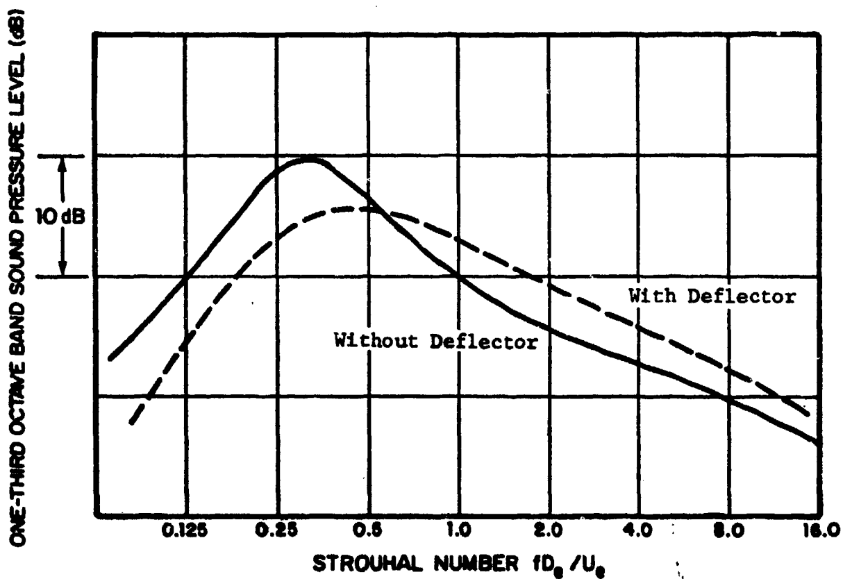
FIG. 70. EFFECT OF DEFLECTOR ON USB SPECTRUM IN FLYOVER PLANE [80].
