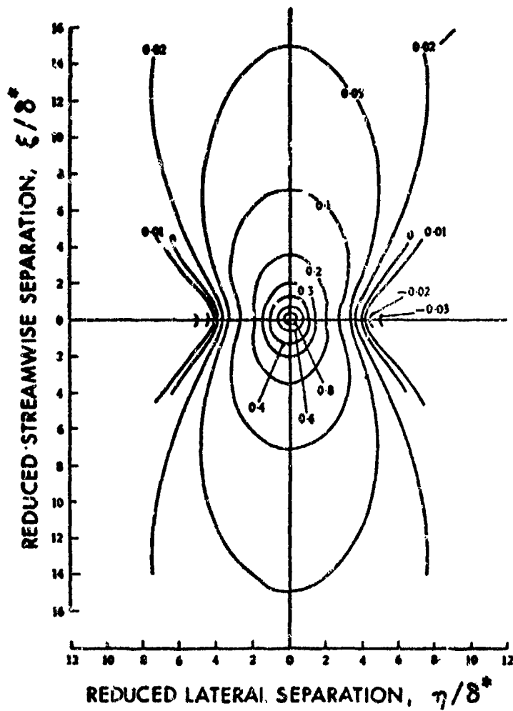
FIG. 90. CONTOURS OF CONSTANT INSTANTANEOUS BROADBAND SPATIAL CORRELATION R(\xi, \eta, 0)/R(0, 0, 0) OF THE WALL-PRESSURE FIELD.
