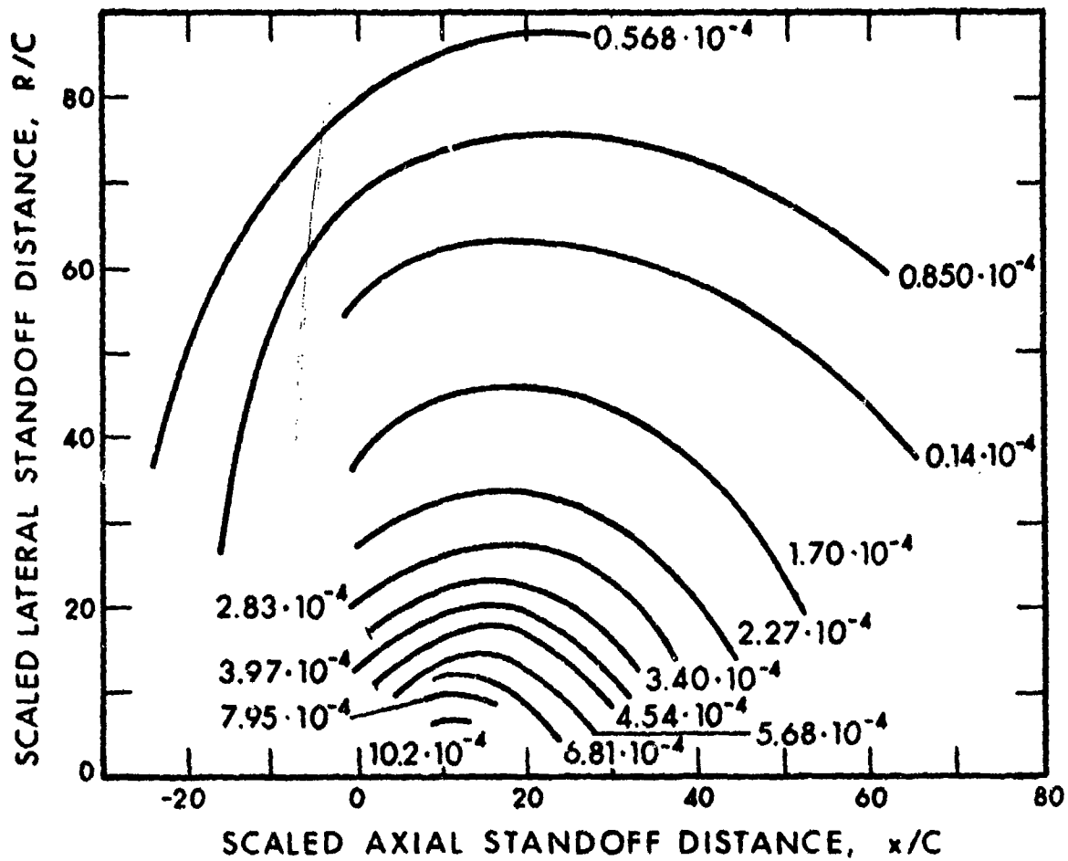
FIG. 128. CURVES OF CONSTANT SCALED OVERPRESSURE \Delta P \cdot C^2 b/E FOR CLOSED-BREECH WEAPONS [135].
