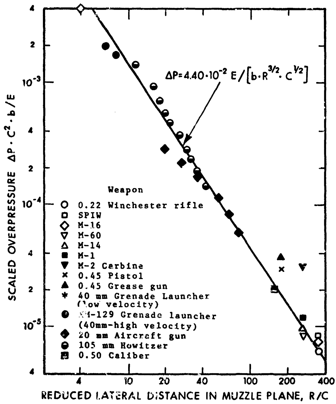
FIG. 126. SCALED SIDE-ON OVERPRESSURE FOR CLOSED-BREECH WEAPONS [135].
