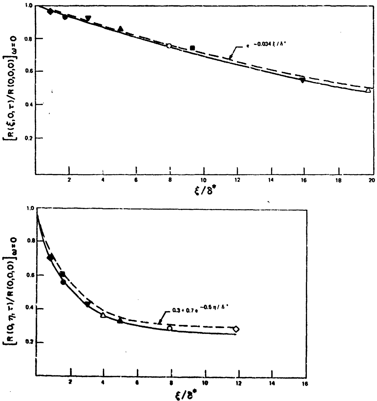
FIG. 95. LOW-FREQUENCY VALUES OF STREAMWISE AND LATERAL CORRELATIONS.
