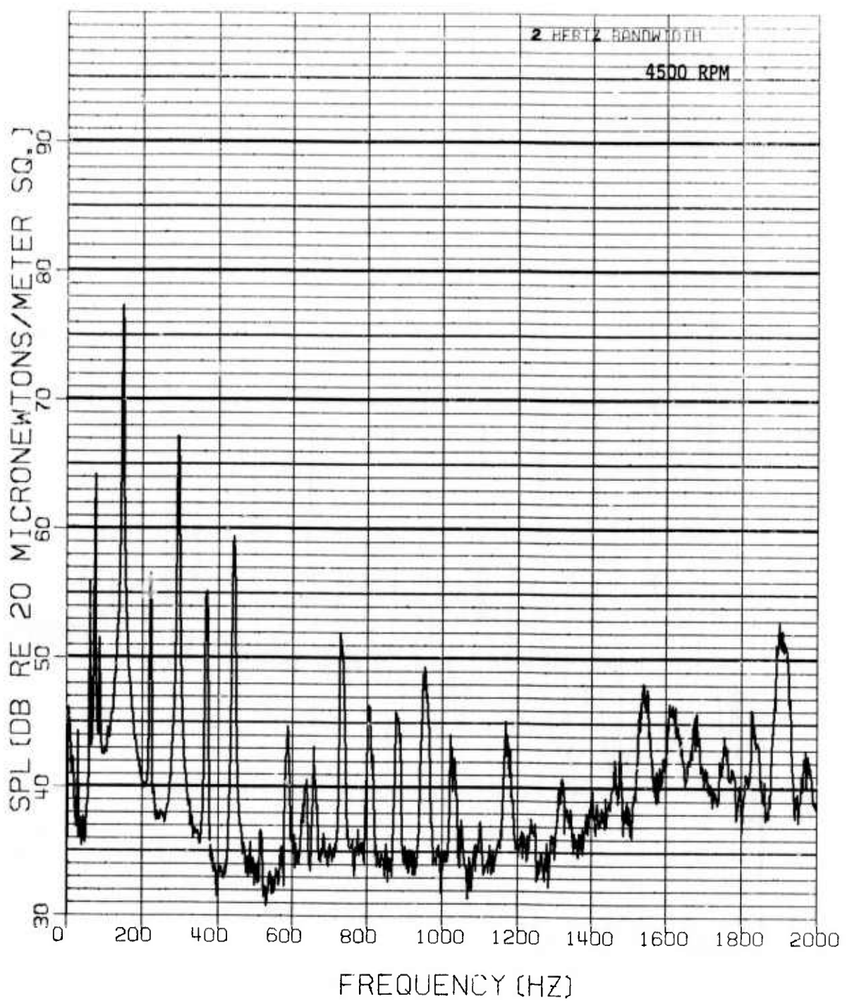
FIGURE 19 ROTARY COMBUSTION ENGINE - MAXIMUM MUFFLER NARROWBAND NOISE SPECTRA
