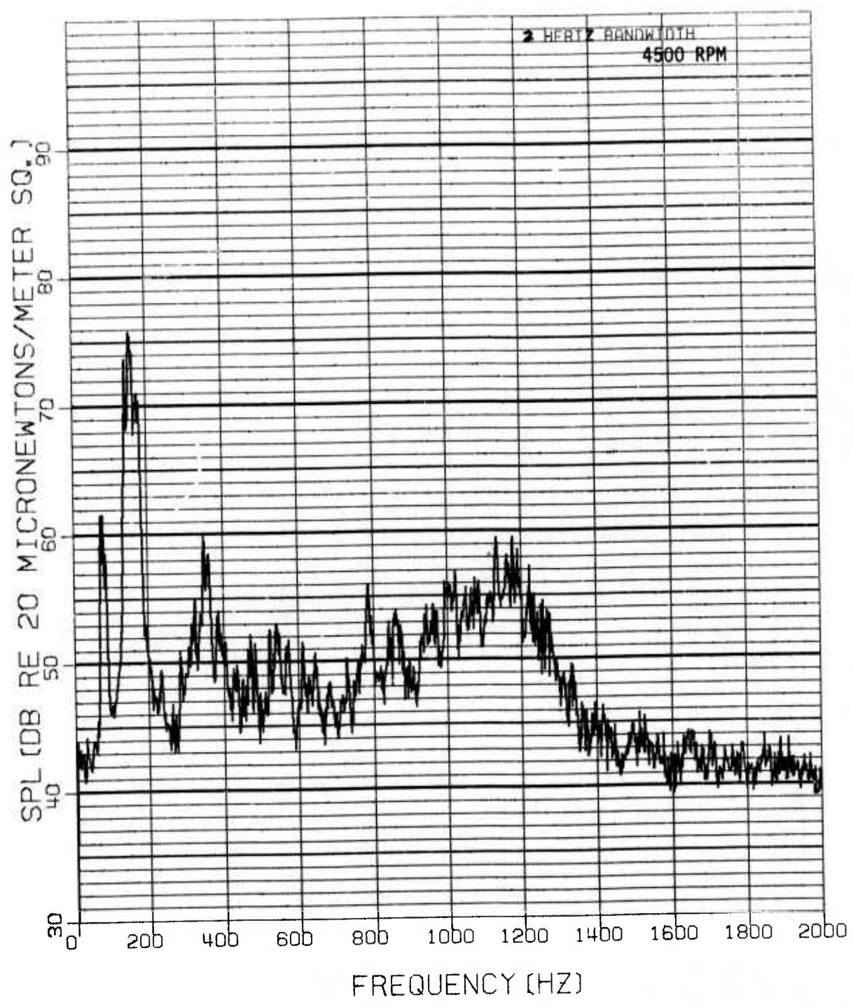
FIGURE 24 PISTON ENGINE - MAXIMUM MUFFLER NARROWBAND NOISE SPECTRA
