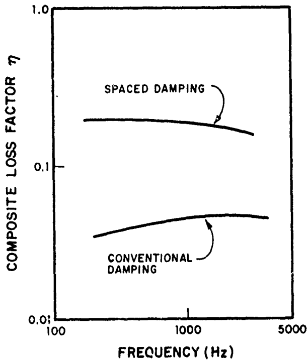
(b) COMPOSITE LOSS FACTOR VS. FREQUENCY FOR SPACED DAMPING AND CONVENTIONAL DAMPING APPLIED TO A 0" x 1/8" SQUARE TUBULAR BEAM. DAMPING MATERIALS AND COVERAGE THE SAME IN BOTH CASES
