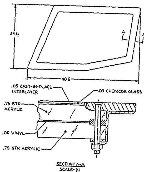
(2) SIERRACIN WINDSHIELD DESIGNED FOR 4 POUND BIRD AT 472 MPH [REFERENCE 9]
