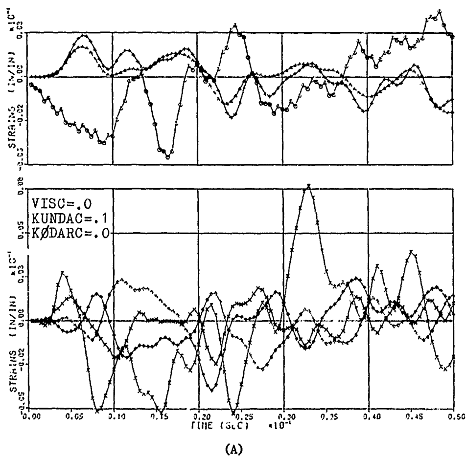
Figure 36. Theoretical Strain Gage Readings of FM-1
