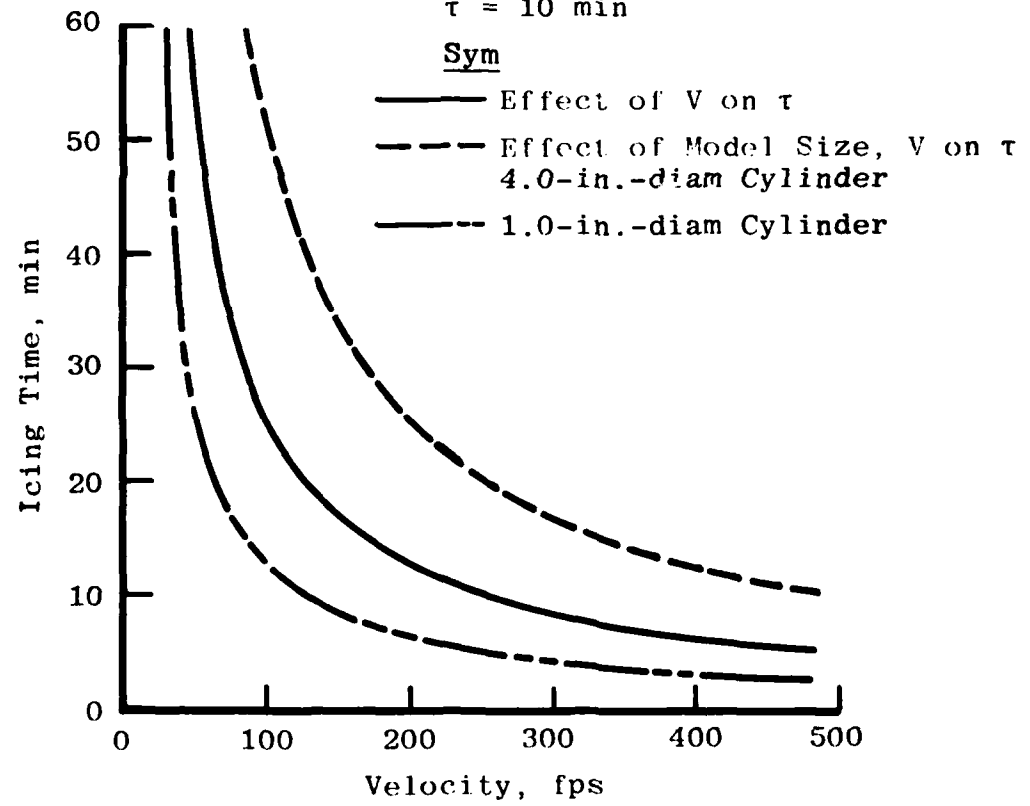
Figure 8. Effect of velocity and model size on the icing time for a constant value of accumulation parameter, A_c .
