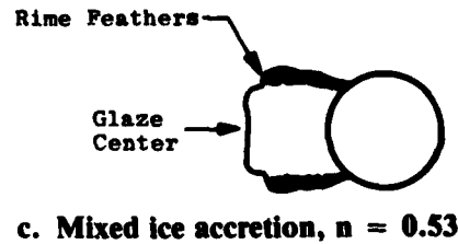
Figure 10. Examples of ice accretions formed at various values of stagnation-point freezing fraction.
