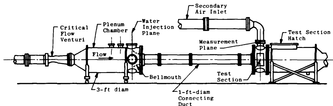
Figure 17. Icing research test cell.
