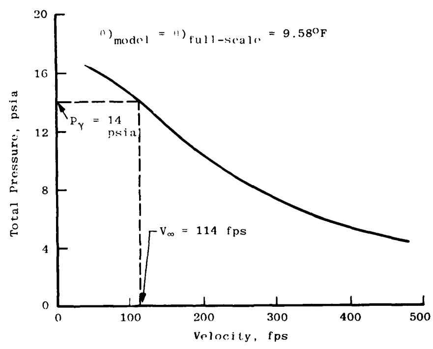
Figure 30. Sample Problem 2: Total pressure of the model as a function of model velocity for a constant value of air energy potential, \theta .
