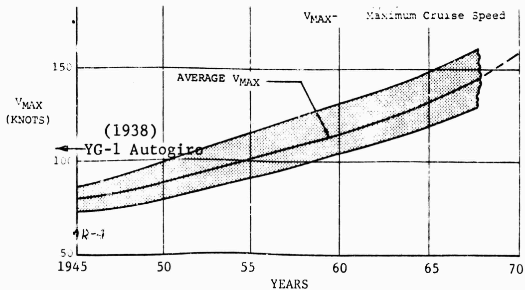
FIGURE 8. MAXIMUM SPEED
