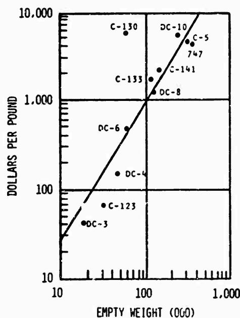
Figure 12. Transport Aircraft Development Cost Per Pound of Empty Weight (1973 Dollars)
