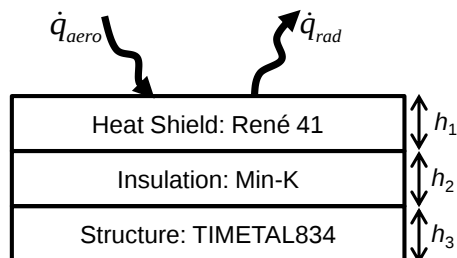
Figure 3.4: Schematic of material stacking scheme at outer mold line of structure.
