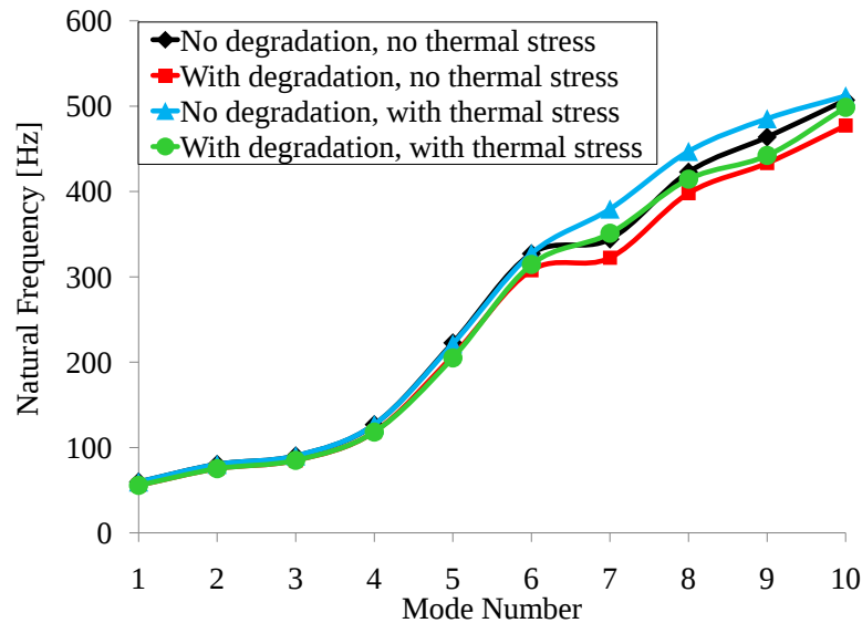
Figure 4.9: Natural frequencies of first ten free vibration modes under thermal loads at 320 s illustrating effect of both material property degradation with temperature and geometric stiffening due to thermal stresses.
