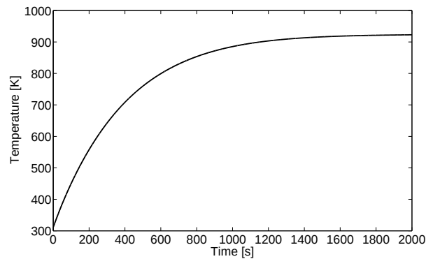
(a) Node 1 (top surface, leading edge, root).
