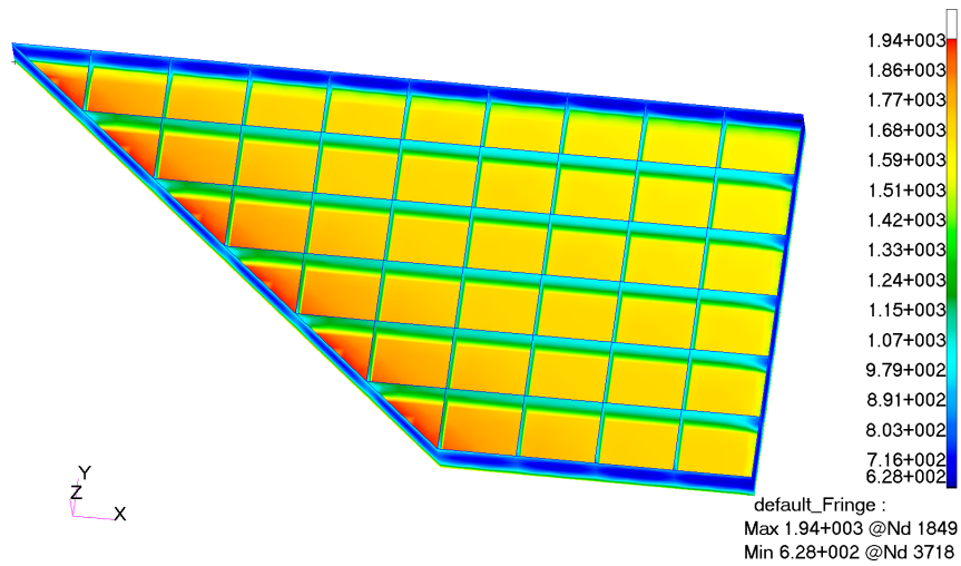
(b) Temperatures at 2,000 s.
