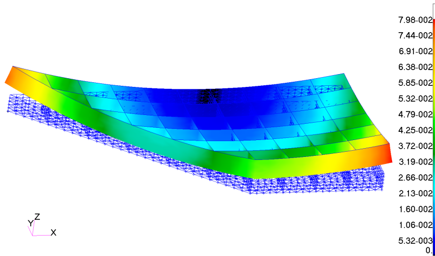
(a) Displacements at 200 s.
