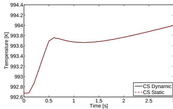
(b) Maximum nodal temperatures.
