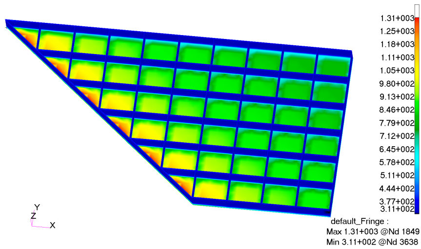
(a) Temperatures at 50 s.
