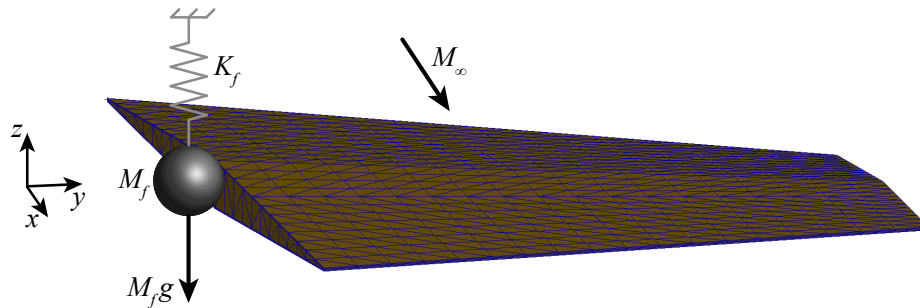
Figure 9.7: Representation of lifting surface and fuselage system.
