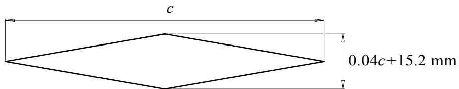
Figure 3.3: Cross-sectional geometry of control surface model.
