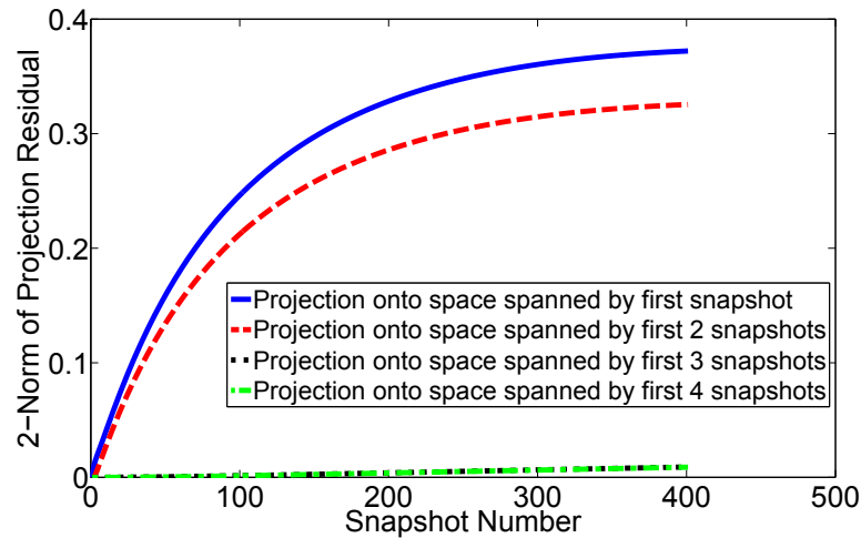
Figure 3.11: Residual of projection of snapshots onto various subspaces.
