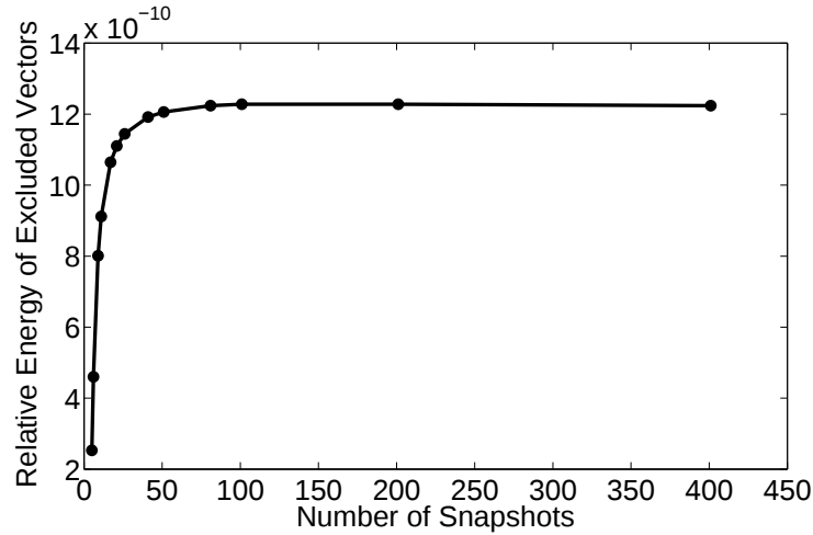
Figure 3.9: Relative energy of excluded basis vectors for varying number of snapshots at 200 s.
