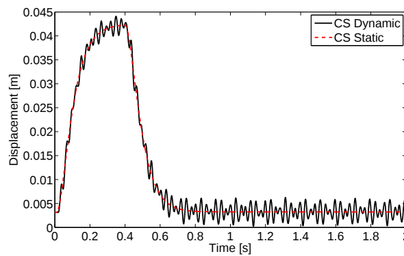
(a) Node 37 (bottom surface, tip, leading edge).
