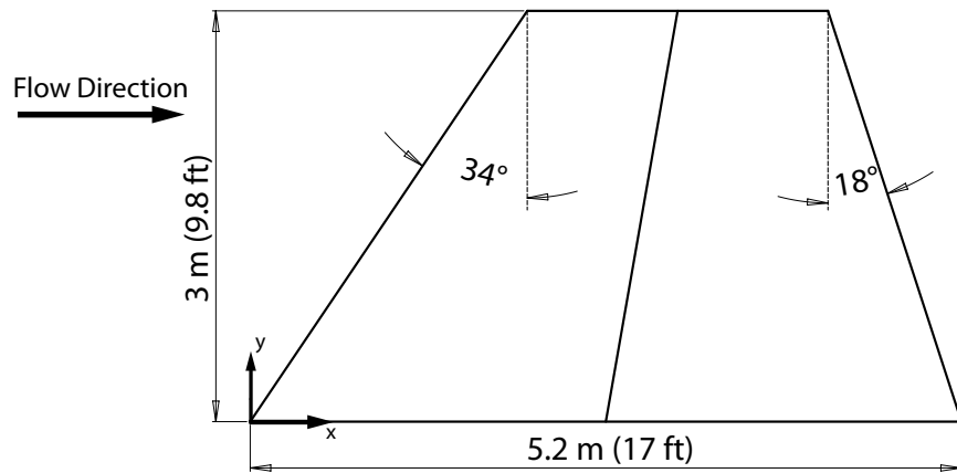
Figure 3.2: Planform geometry of control surface model.
