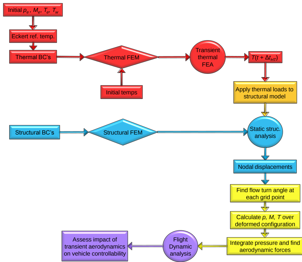
Figure 7.1: Flowchart of quasi-steady aerothermoelastic simulation framework.
