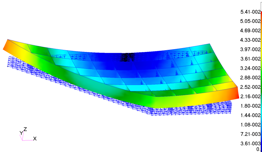
(c) Displacements at 2,000 s.
