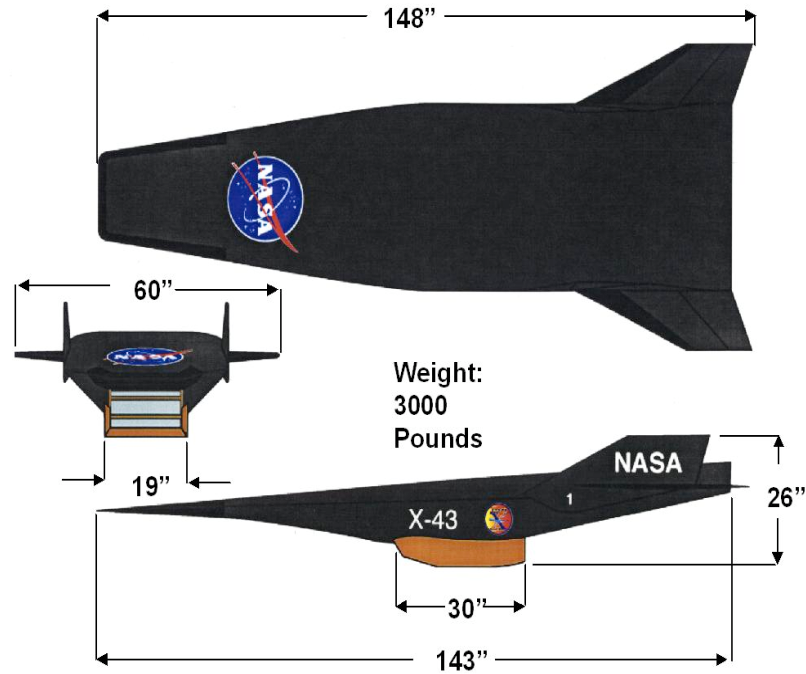
Figure 1.1: NASA X-43A Hyper-X air-breathing hypersonic vehicle [17].
