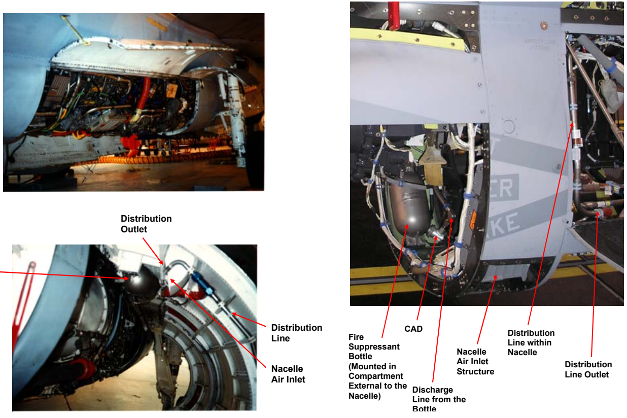
Figure 6. Examples of Contemporary Engine Nacelles and Fire Suppression Systems
