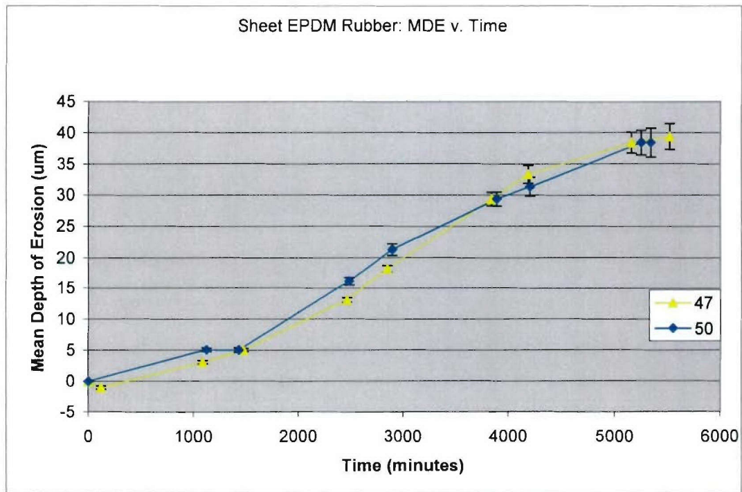
Figure 5.10 – Sheet EPDM results
