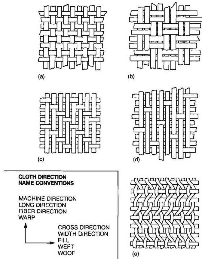
Figure 3.3 - Lamine weave geometries [Strong, 1989]
