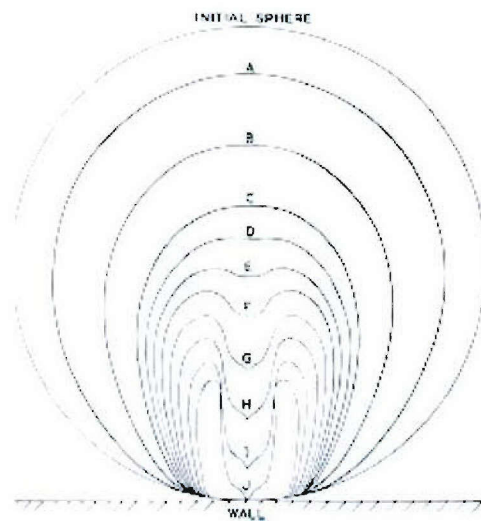
Figure 2.1 – Schematic of asymmetrical bubble collapse showing liquid jet impingement [Morch, 1979]
