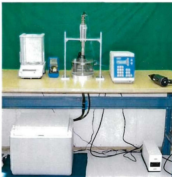
Figure 4.1 – Photograph of the experimental test apparatus
