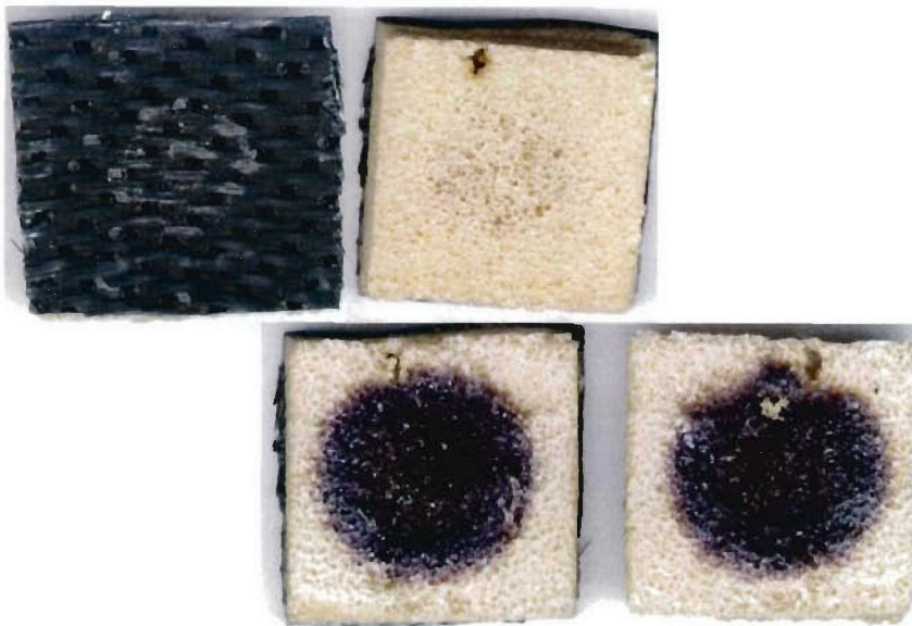
Figure 5.8 – Carbon fiber over PVC core samples showing core damage
