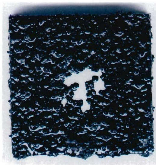
Figure 5.13 - Herculiner® sample #051 showing erosion damage
