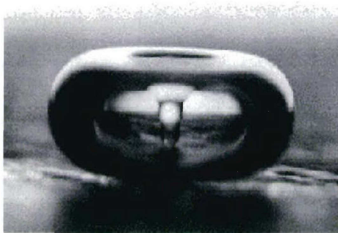
Figure 2.2 - Photograph of actual collapsing cavitation bubble. [Center for Industrial and Medical Ultrasound, University of Washington]
