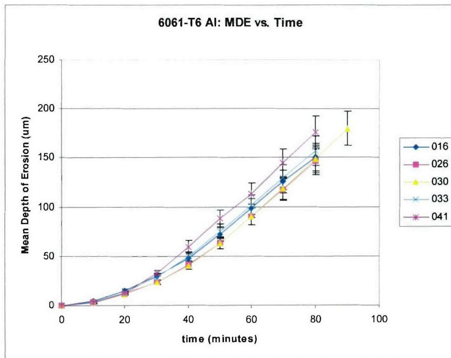
Figure 4.6 – Repeatability of 6061-T6 Aluminum Samples
