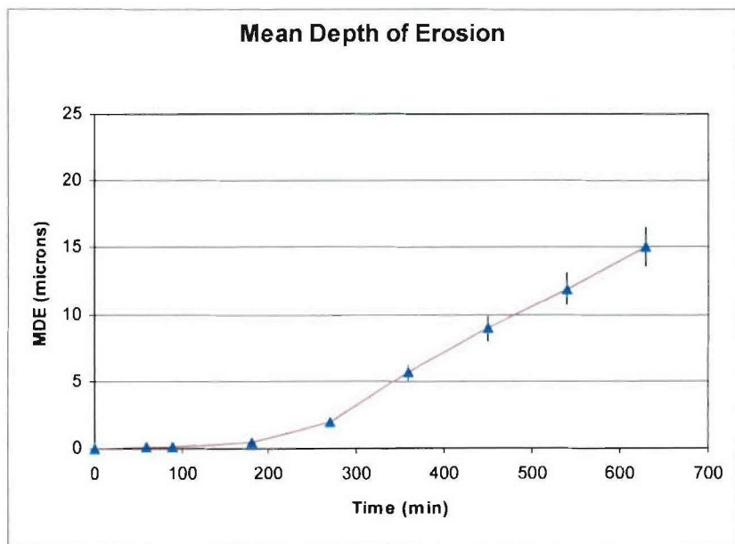
Figure 4.3 - Example Cumulative Erosion-Time Curve
