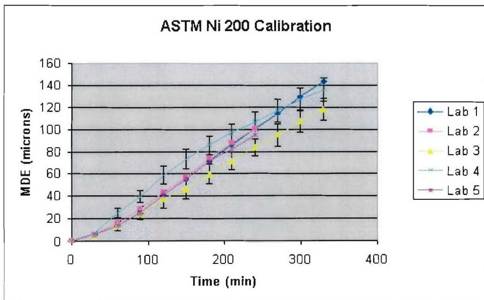
Figure 4.4 - MDE for Ni 200 from independent lab tests using ASTM procedures
