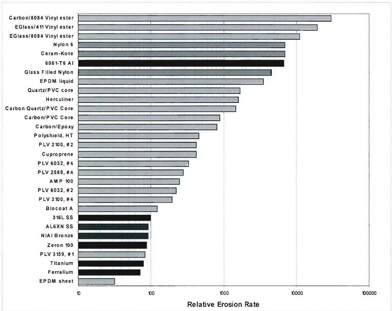
Figure 6.1 – Relative Cavitation Erosion Results.
