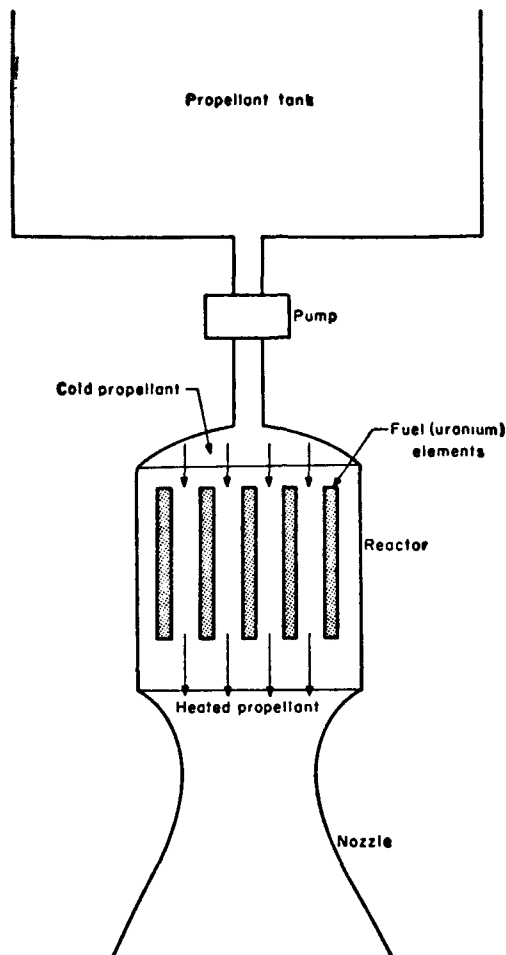
Fig. 3—Nuclear rocket
