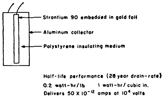
Fig.2 — Utilization of isotope power
