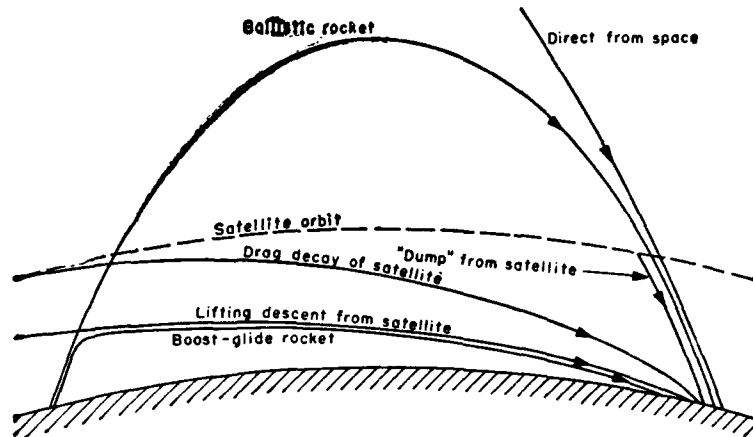
Fig.3 — Various types of atmospheric entry
