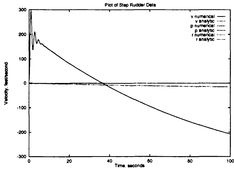
Figure 4.14: Comparison of Lateral Responses to Step Rudder Input
