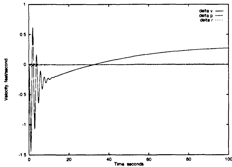
Figure 4.17: Difference in Analytic and Numerical Results, Step Rudder Input
