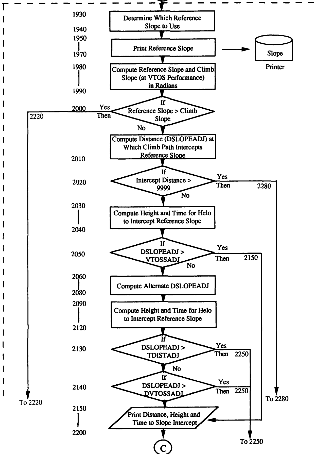
FIGURE 3 FLOW CHART FOR THE HV + 5 KNOTS PROCEDURE (CONTINUED)
