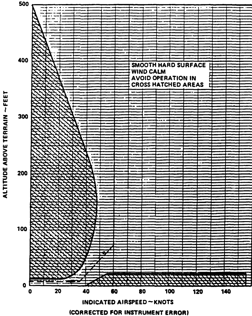
FIGURE A-1 HEIGHT VELOCITY DIAGRAM - HUGHES 500E
