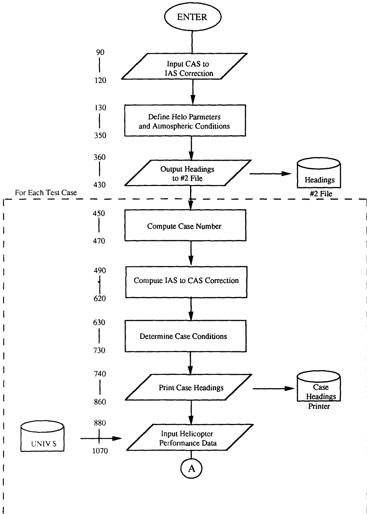
FIGURE 3 FLOW CHART FOR THE HV + 5 KNOTS PROCEDURE
