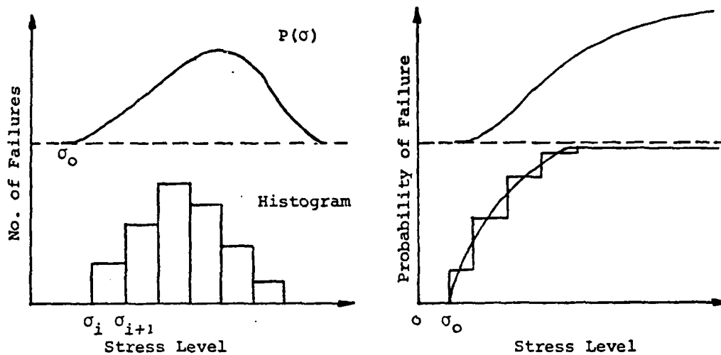
Figure C.1. Probability Distribution
