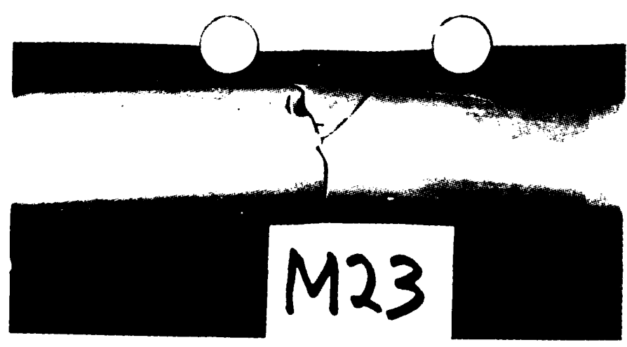
Figure 4.13: Mullite Specimen M23 After Fracture
