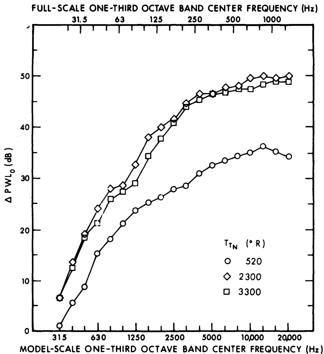
FIG. 7.6.16. \Delta PWL FOR 72-in. BBN AUGMENTER WITH 45^{\circ} RAMP, F-14 POSITION, \lambda_N = 2 , x_N = 4 in.
