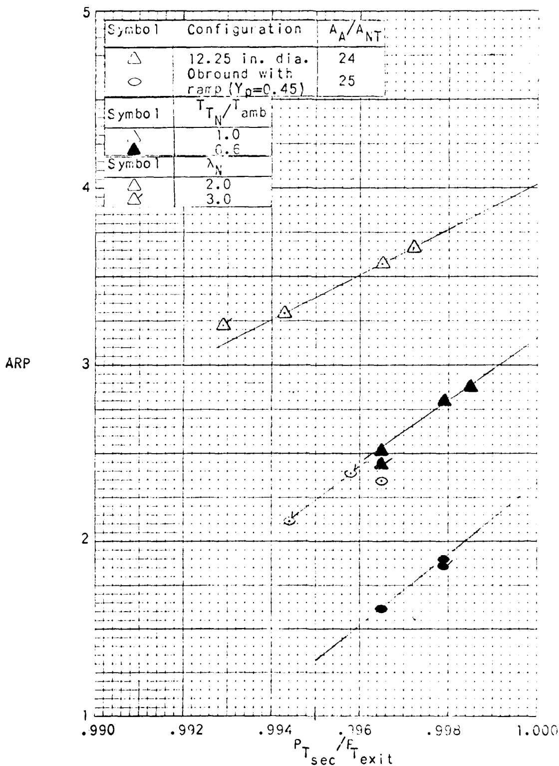
FIGURE 7.1-7. AUGMENTER PUMPING PERFORMANCE VS. AUGMENTER PRESSURE RATIO. (A_A/A_{NT} = 25, X_N/D_{NT} = 1.6, L_A/D_{AM} = 6)
