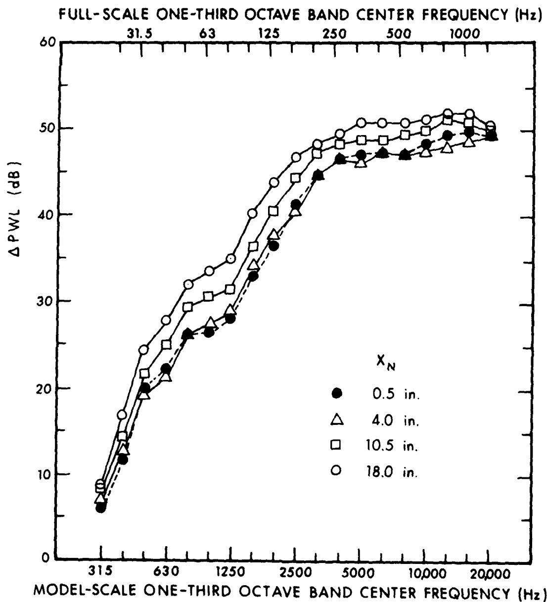
FIG. 7.6.22. \Delta PWL FOR DIFFERENT AXIAL POSITIONS OF THE NOZZLE: 72-in. BBN AUGMENTER WITH 45° RAMP, F-14 POSITION, T_{T_N} = 3300^\circ R , \lambda_N = 2 .
