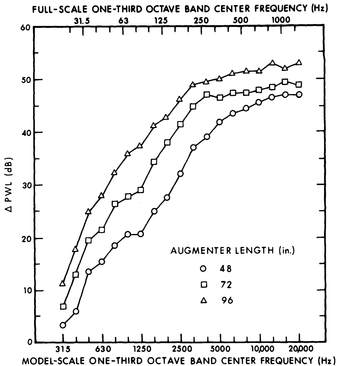
FIG. 7.6.25. \Delta PWL FOR THREE DIFFERENT LENGTHS OF LINED BBN AUG- MENTER WITH 45° RAMP: T_{TN} = 3300^\circ R , \lambda_N = 2 , x_N = 4 in.
