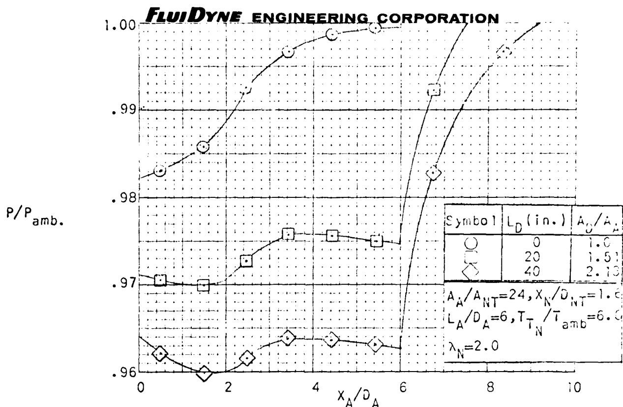
FIGURE 7.2-5. LONGITUDINAL PRESSURE DISTRIBUTION FOR THE 12.25 IN. DIAMETER AUGMENTER FOR VARIOUS EXIT SUBSONIC DIFFUSER LENGTHS
