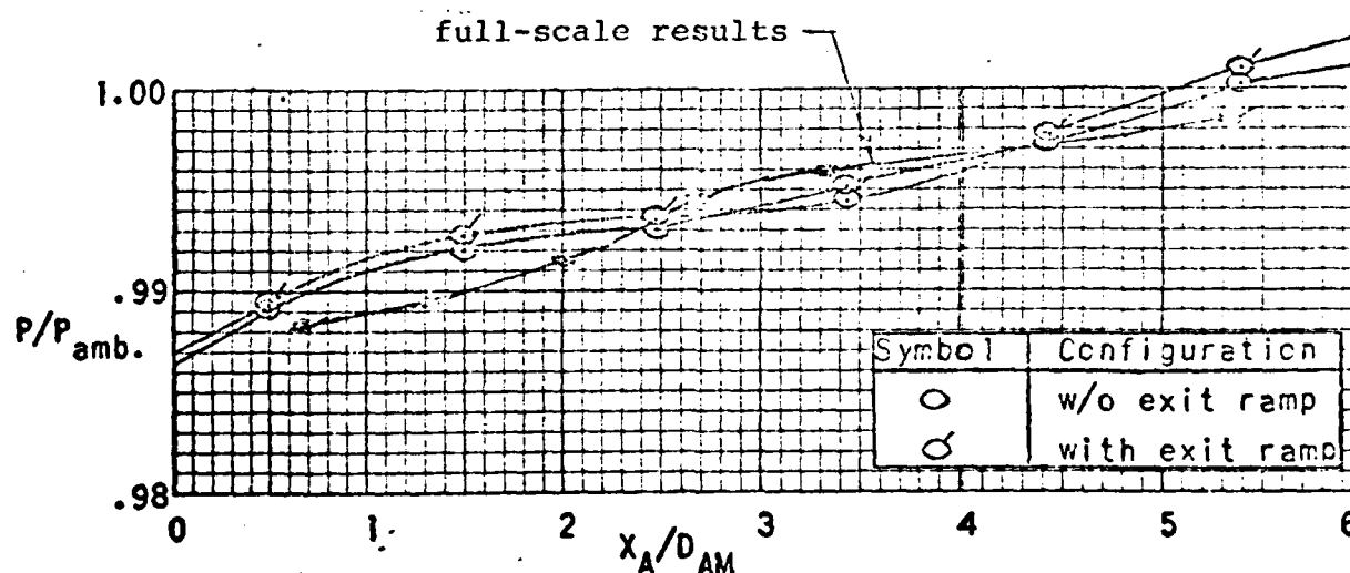
FIGURE 7.2-9. LONGITUDINAL SHELL PRESSURE DISTRIBUTION FOR THE OBROUND AUGMENTER WITH AND WITHOUT EXIT RAMP. (A_A/A_{NT}=25, X_N/D_{NT}=1.6, L_A/D_{AM}=6, T_N/T_{amb}=6.6, \lambda_N=2.0, Y_p=0.45)
