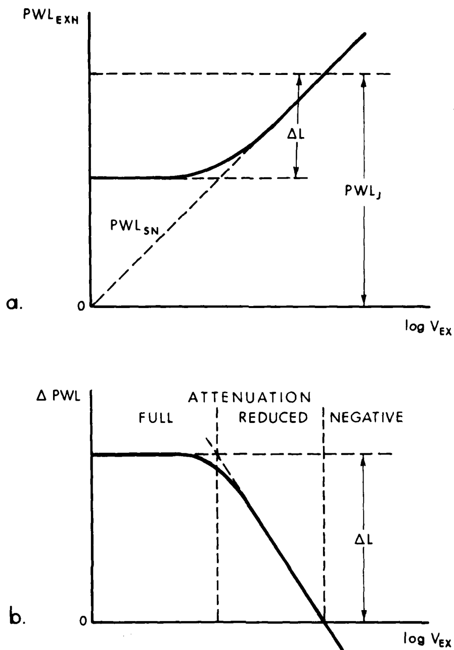
FIG. 7.6.12. EFFECT OF EXIT SPEED-GENERATED SELF-NOISE. a. EXHAUST SOUND POWER, PWL_{EXH} b. POWER LEVEL REDUCTION \Delta PWL
