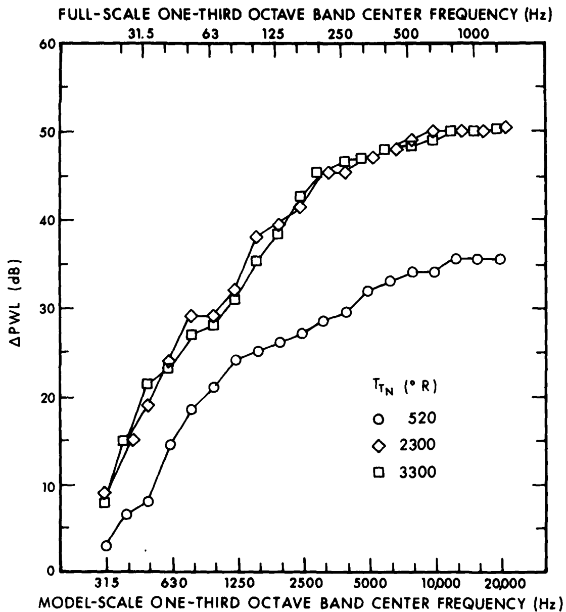
FIG. 7.6.18. \Delta PWL FOR 72-in. BBN AUGMENTER WITH 45° POROUS-BACKED RAMP: F-14 POSITION, \lambda_N = 2 , x_N = 4 in.
