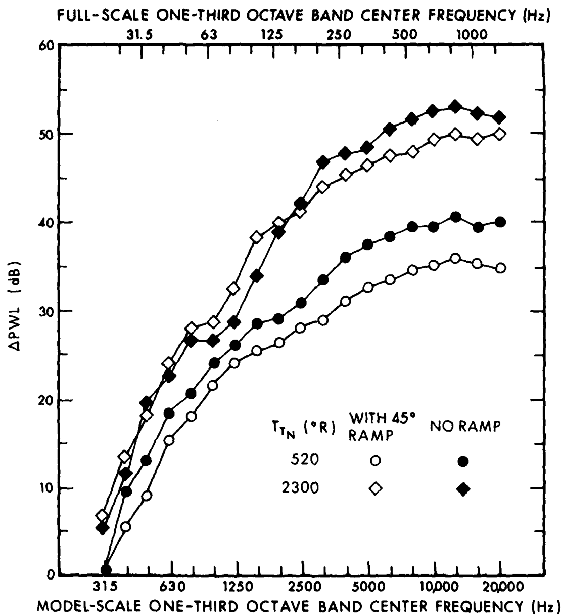
FIG. 7.6.20. \Delta PWL FOR 72-in. BBN AUGMENTER WITH AND WITHOUT 45° RAMP: F-14 POSITION, \lambda_N = 2 , x_N = 4 in.
