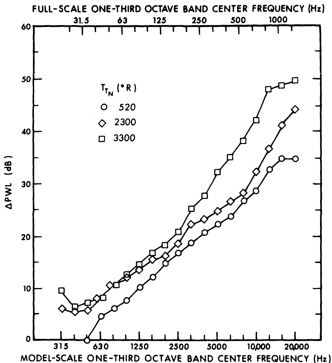
FIG. 7.6.26. \Delta PWL FOR 60-in. HARD-WALLED AUGMENTER, SUBSONIC DIFFUSER, TURNING VANES, STACK WITH BAFFLES: F-14 POSITION, \lambda_N = 2 , x_N = 4 in.
