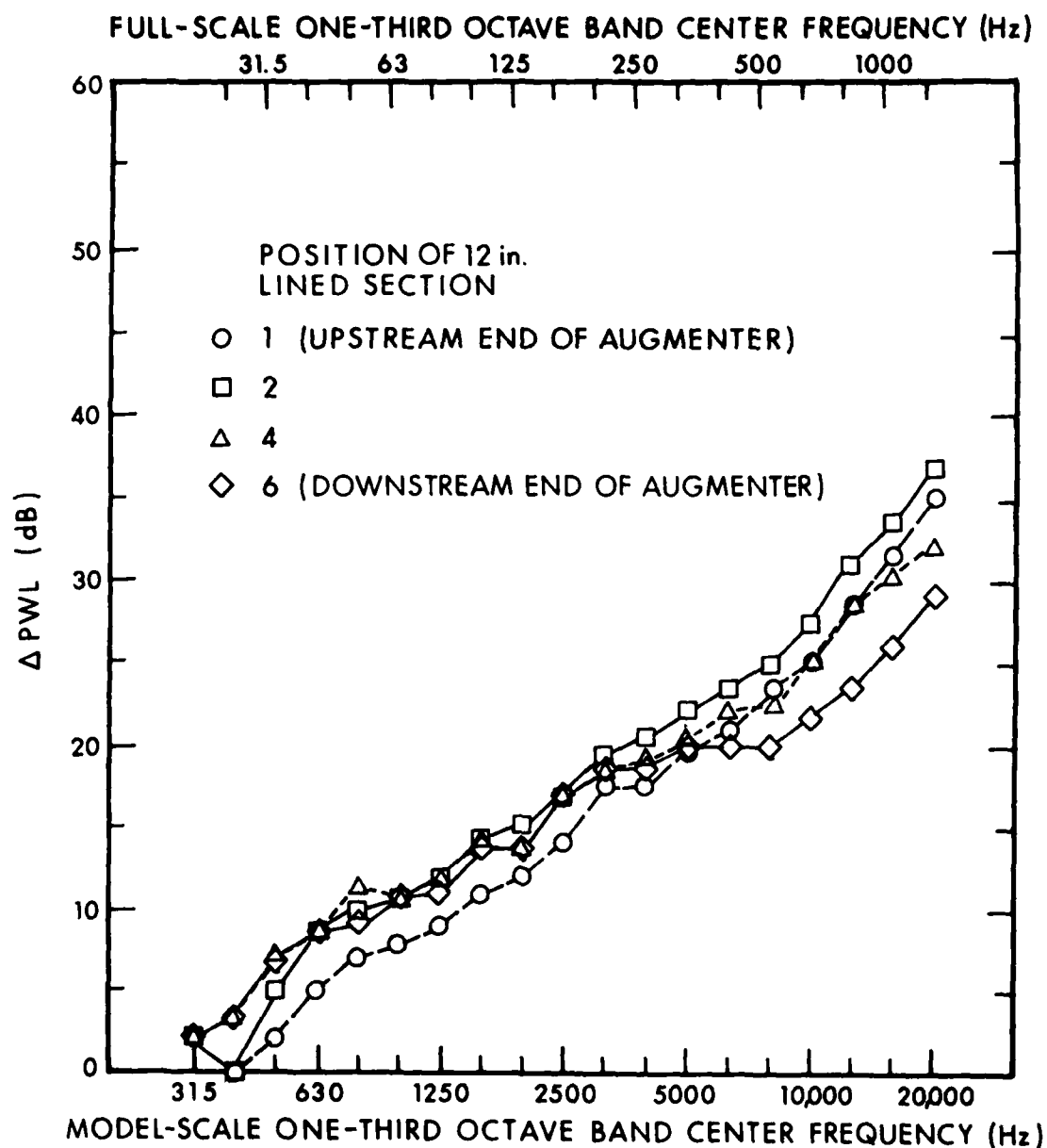
FIG. 7.6.24. \Delta PWL FOR 12-in. SECTION OF AUGMENTER WITH BBN LINER AT VARIOUS POSITION IN THE 60-in. HARD-WALLED AUGMENTER WITH 45° RAMP: F-14 POSITION, T_{TN} = 3300^\circ R , \lambda_N = 2 , X_N = 4 in.
