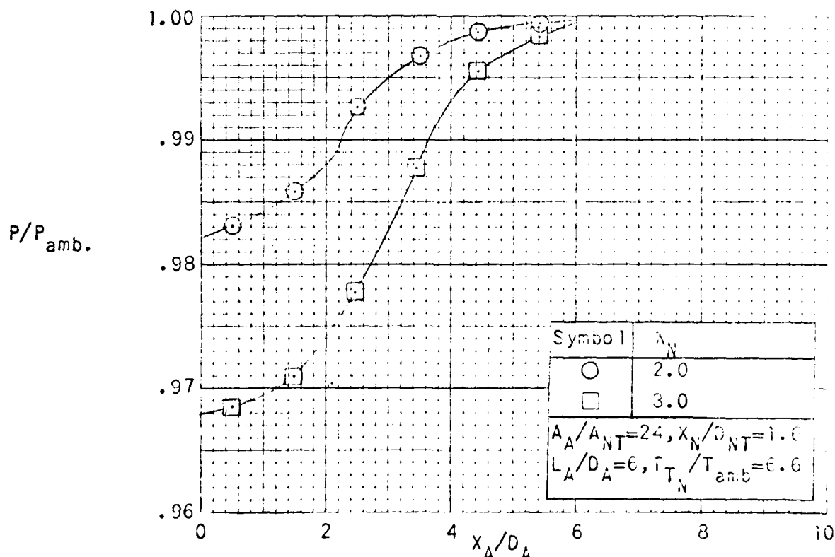
FIGURE 7.2-6. LONGITUDINAL PRESSURE DISTRIBUTION FOR THE 12.25 IN. DIAMETER AUGMENTER HAVING NO EXIT SUBSONIC DIFFUSER AT JET NOZZLE PRESSURE RATIOS OF 2.0 AND 3.0.
