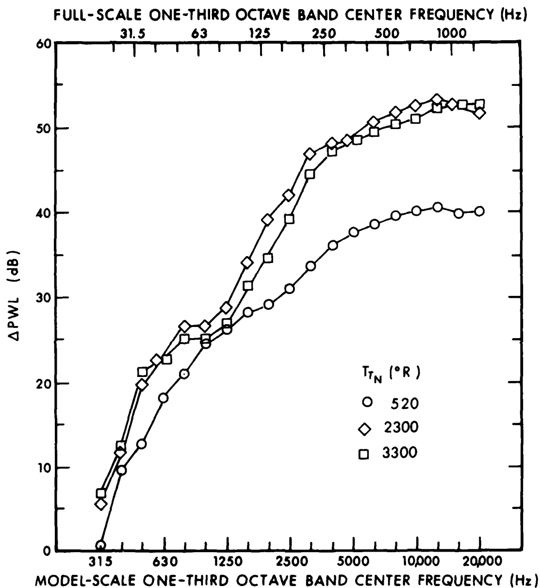
FIG. 7.6.19. \Delta PWL FOR 72-in. BBN AUGMENTER WITHOUT 45° RAMP: F-14 POSITION, \lambda_N \approx 2 , x_N = 4 in.
