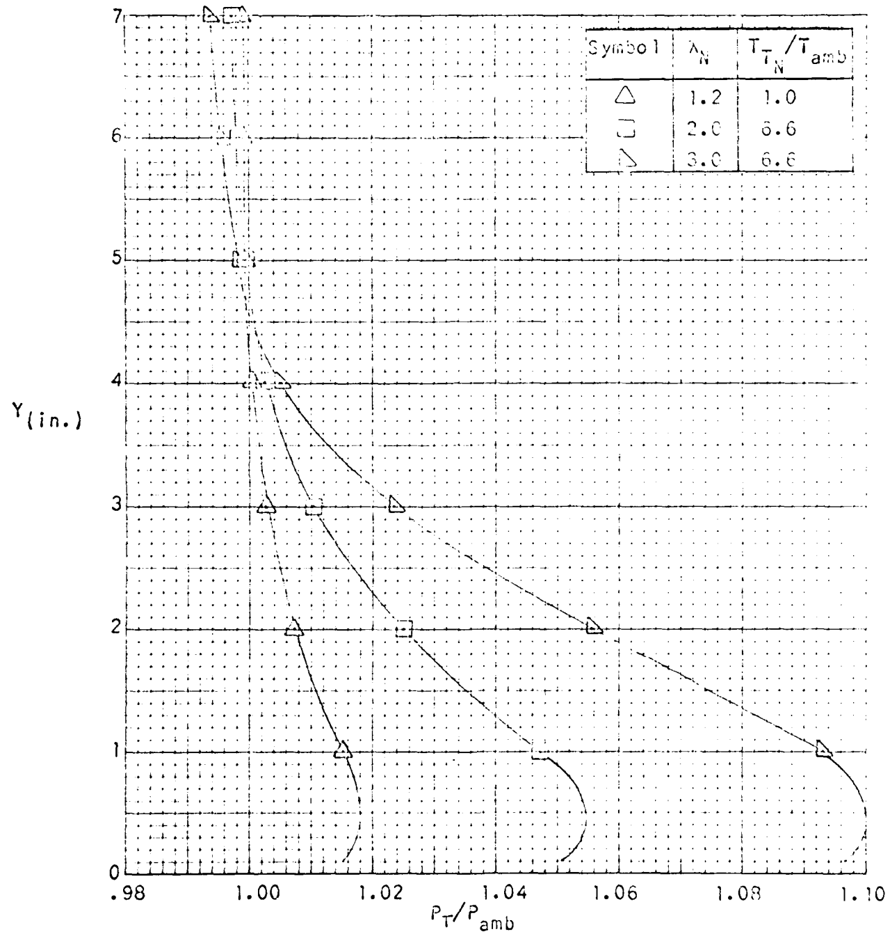
FIGURE 7.3-23. TOTAL PRESSURE DISTRIBUTION AT THE TOP OF THE OBROUND AUGMENTER EXIT RAMP FOR THREE JET NOZZLE PRESSURE RATIOS. ( A_A/A_{NT}=25, X_N/D_{NT}=1.6, L_A/D_{AM}=6, Y_p=0.45 )
