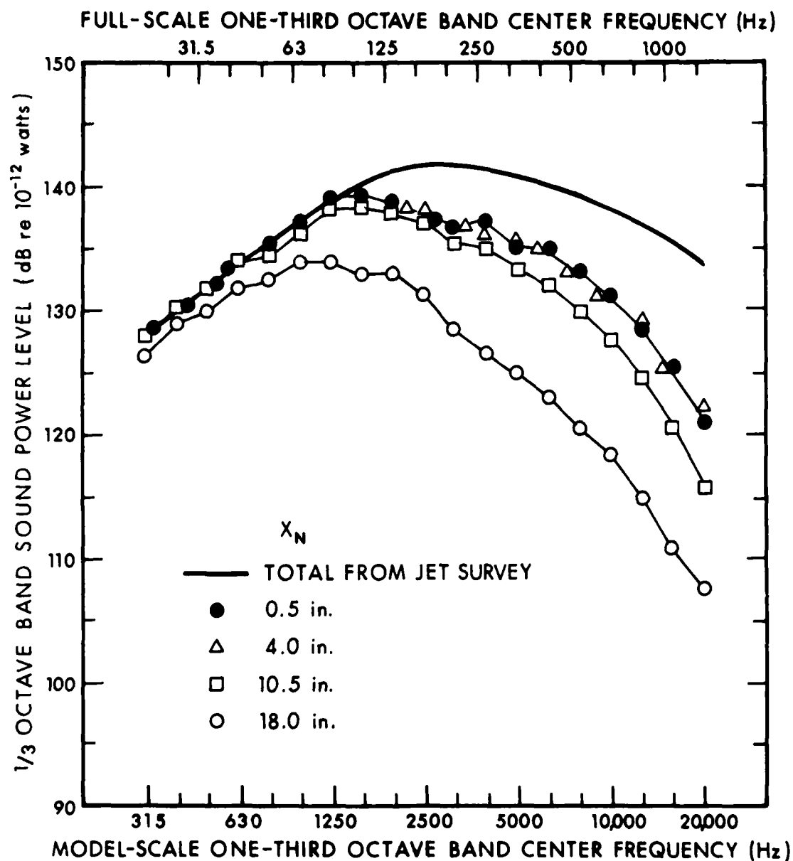
FIG. 7.6.6. EFFECT OF AXIAL DISTANCE ON THE SOUND POWER RADIATED INTO THE EXHAUST ROOM AT 3300°R, \lambda_N = 2 , D_A = 12.5 in., L_A = 72 in.
