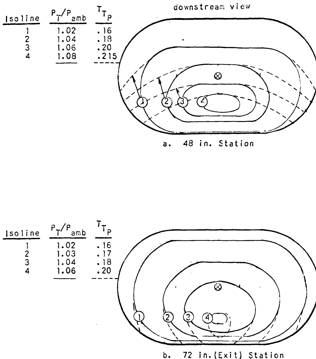
FIGURE 7.3-15. CROSS-SECTION TOTAL PRESSURE AND TEMPERATURE CONTOURS FOR THE OBROUND AUGMETER WITH THE JET CENTERED (POSITION a, Y_p = 1.0 ) AND DEFLECTED DOWNWARD 3.6^\circ . (A_A/A_{NT}=25, X_N/D_{NT}=1.6, L_A/D_{AM}=6, T_{TN}/T_{amb}=4.6, \lambda_N=2.0)
