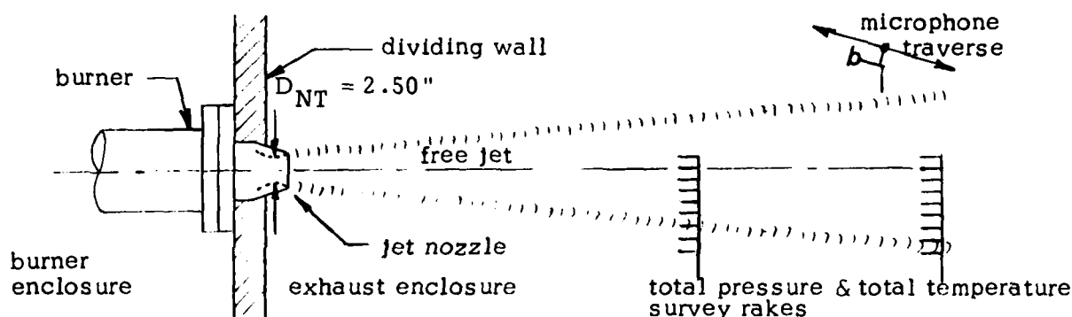
Figure 2.0-2. Experimental Arrangement for the Jet Survey Tests
