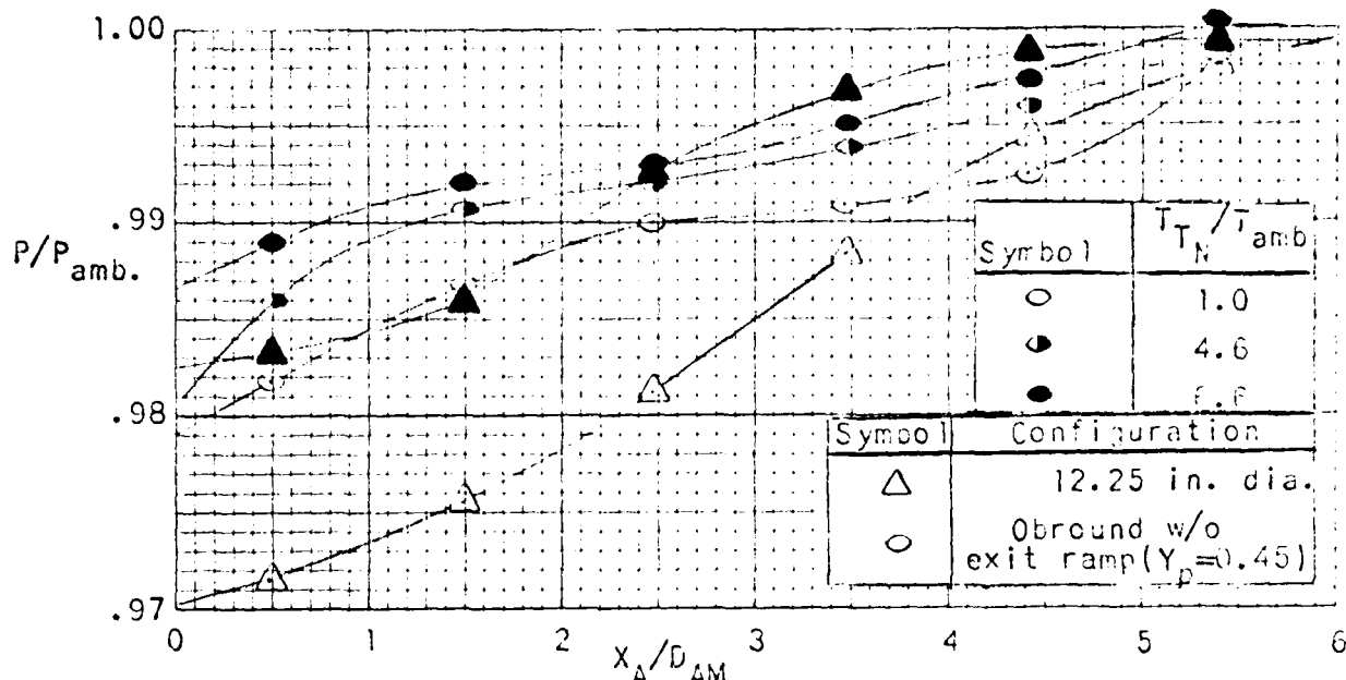
FIGURE 7.2-7. LONGITUDINAL PRESSURE DISTRIBUTION FOR BOTH THE 12.25 IN. DIAMETER AND THE OBROUND AUGMENTOR AT VARIOUS JET NOZZLE TO AMBIENT TEMPERATURE RATIOS. ( A/A_{NT}=25, X_N/D_{NT}=1.6, L_A/D_{AM}=6, \lambda_N=2.0 )
