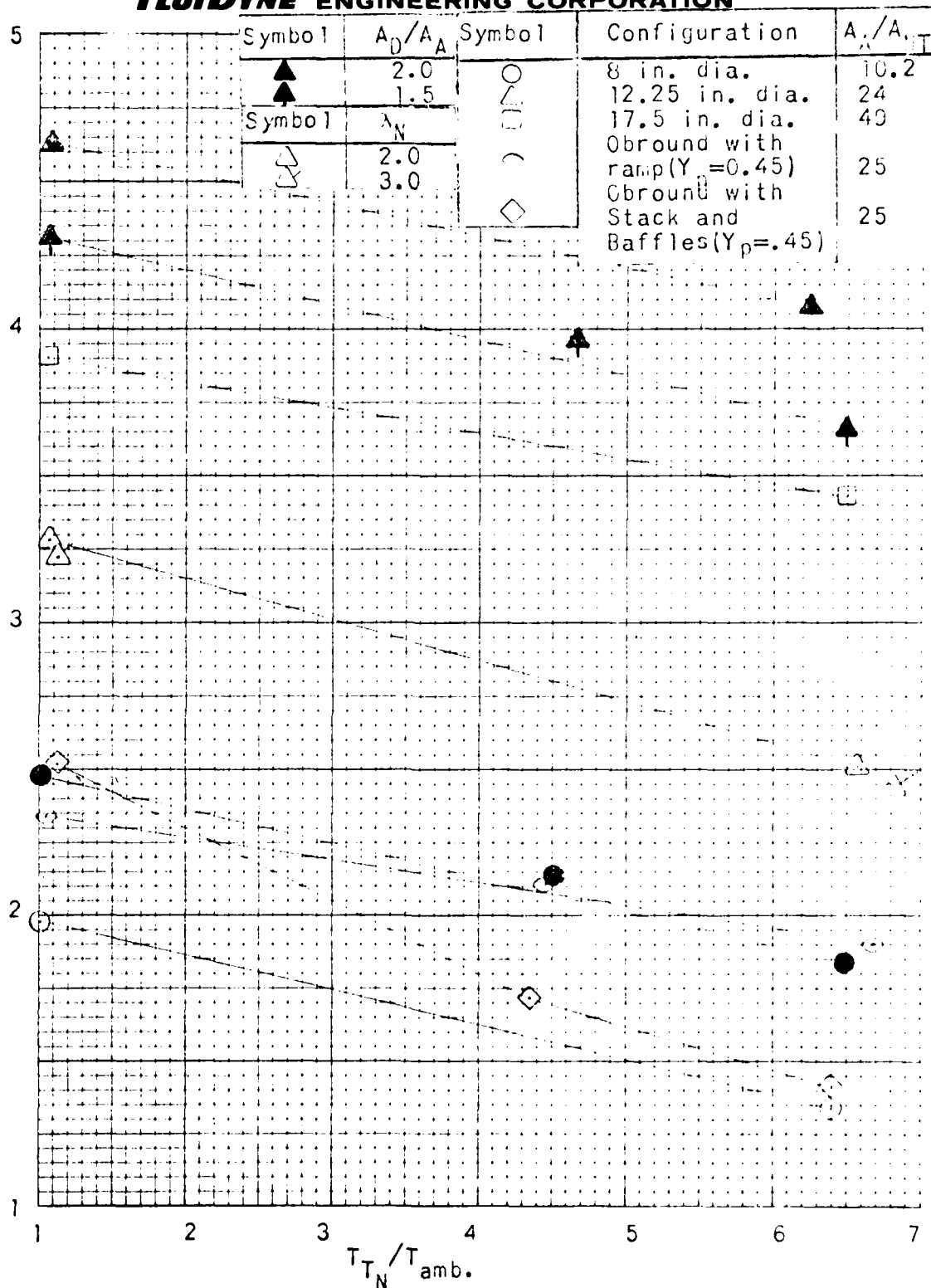
FIGURE 7.1-1. SUMMARY OF AUGMENTER PUMPING PERFORMANCE (AUGMENTATION RATIO PARAMETER, ARP, vs. T_{TN}/T_{amb.} ) ( X_N/D_{NT}=1.6, L_A/D_{AM}=6 )
