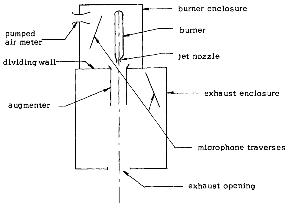
Figure 2.0-1. Arrangement of the Reverberant Rooms
