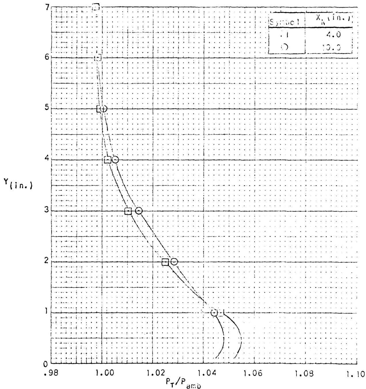
FIGURE 7.3-21. TOTAL PRESSURE DISTRIBUTION AT THE TOP OF THE OSGROUND AUGMENTER EXIT RAMP FOR TWO JET NOZZLE TO AUGMENTER ENTRANCE SPACINGS.
