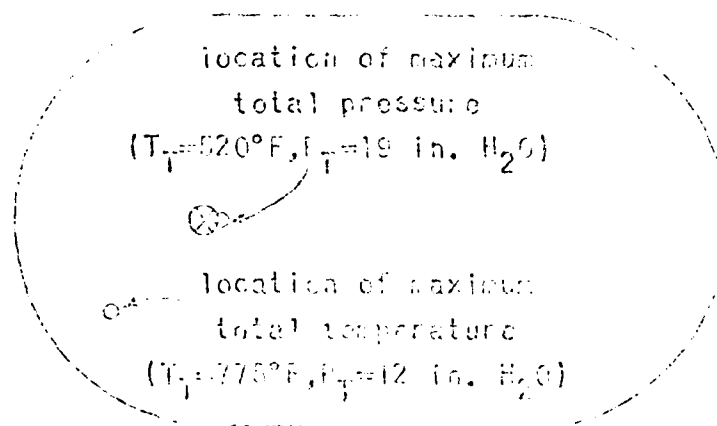
FIGURE 1. MAXIMUM TOTAL PRESSURE AND TOTAL TEMPERATURE IN THE MIRAMAR AUGMENTER EXIT CROSS-SECTION WITH THE F-14A HAVING ONE ENGINE IN MILITARY POWER SETTING.
