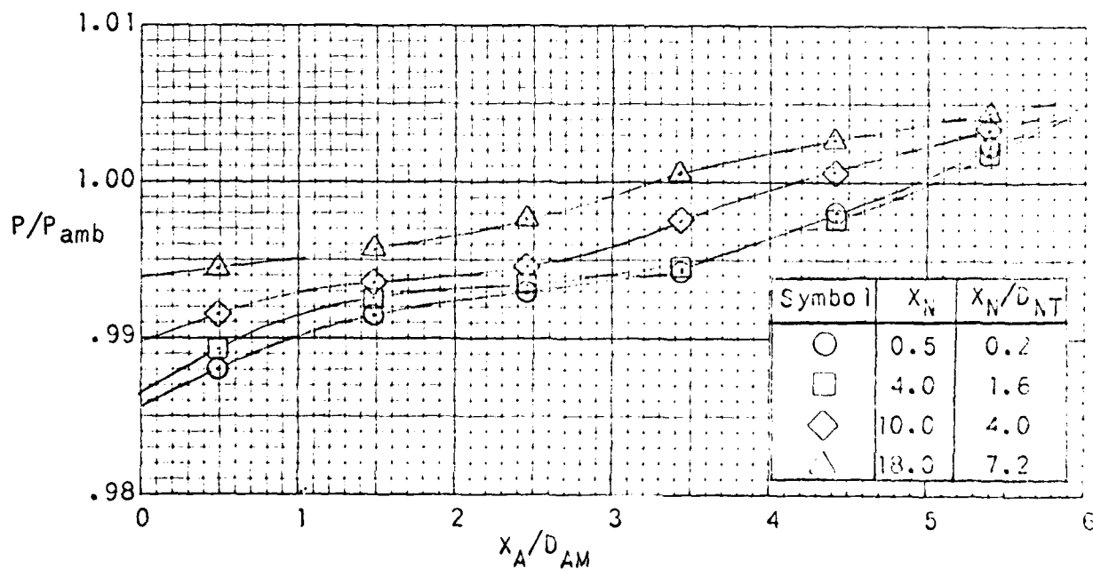
FIGURE 7.2-10. LONGITUDINAL SHELL PRESSURE DISTRIBUTION FOR THE OBOUND AUGMETER WITH EXIT RAMP AT VARIOUS JET NOZZLE EXIT TO AUGMETER ENTRANCE SPACINGS. ( A_A/A_{NT}=25 , L_A/D_{AM}=6 , T_T/T_{amb}=6.6 , \lambda_N=2.0 , Y_p=0.45 )
