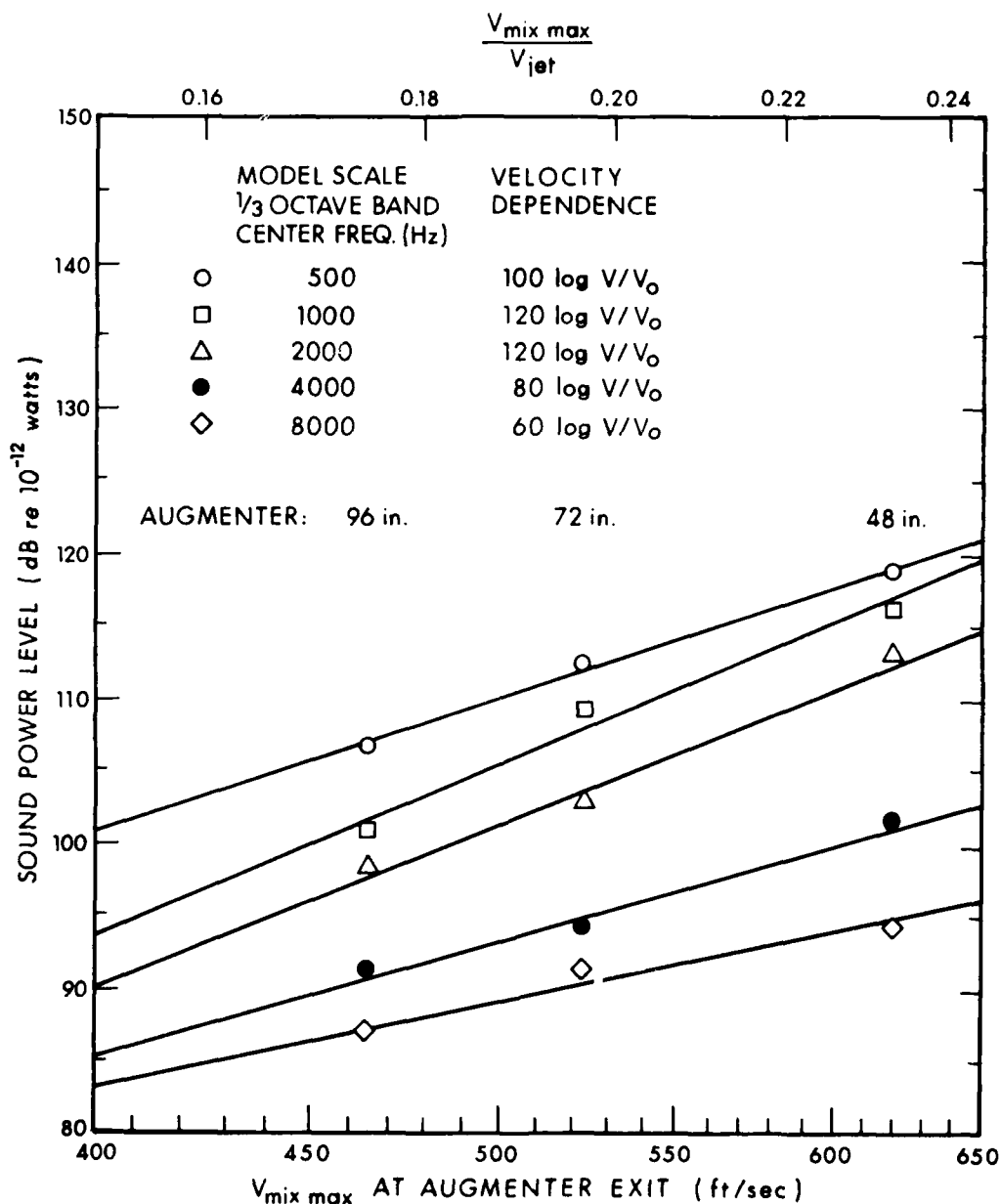
FIG. 7.6.13. DEPENDENCE OF EXHAUST ROOM PWL ON VELOCITY OF AIR EXITING FROM FULLY LINED BBN AUGMENTERS OF DIFFERENT LENGTHS: 45^\circ RAMP, T_{TN} = 3300^\circ R , \lambda_N = 2 , x_N = 4 in.
