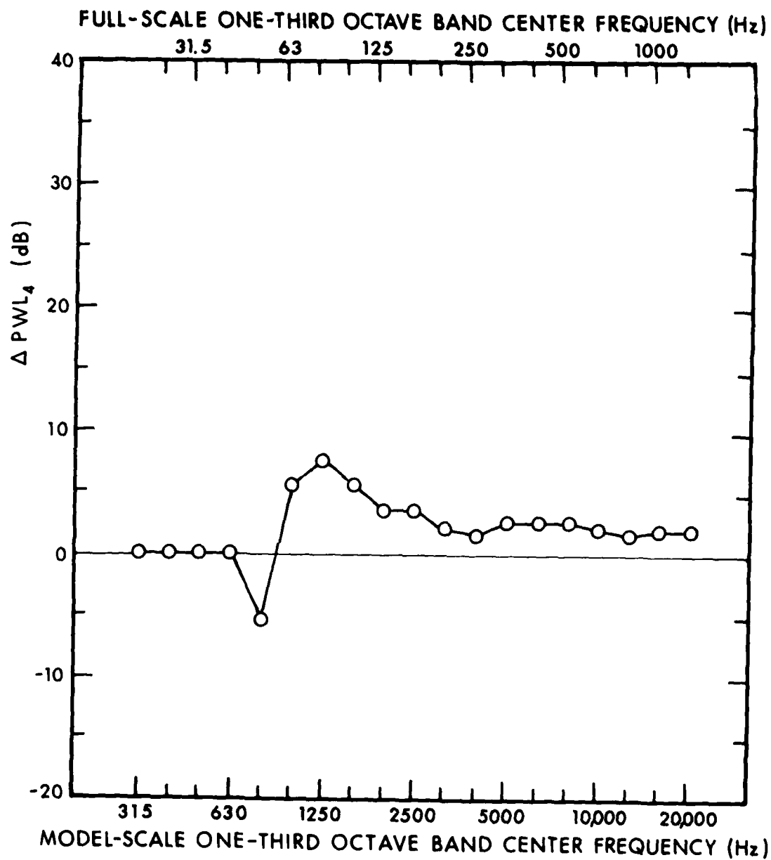
FIG. 2.3.7. CORRECTION TO \Delta \text{PWL} FOR CENTER POSITION OF JET NOZZLE.
