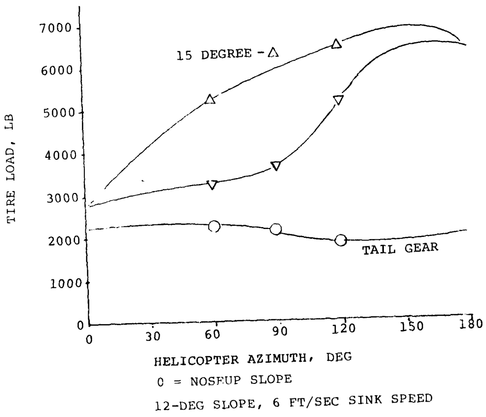
Figure 10. Slope landing gear loads.
