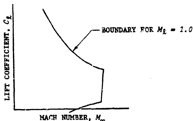
Figure 6. Critical Mach number boundary
