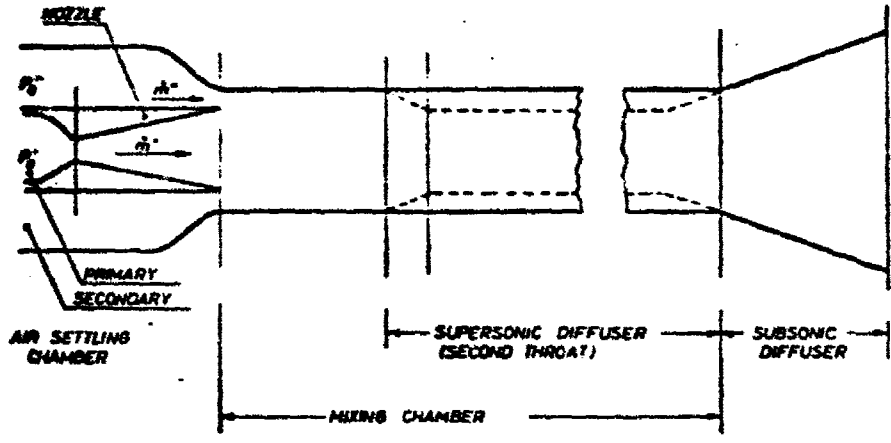
Diagram of a supersonic ejector and reference stations
