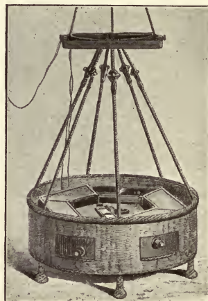
FIG. 216.—Panoramic apparatus for a balloon without observers.
