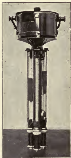
FIG. 151.—Assmann's aspirator-psychrometer.
