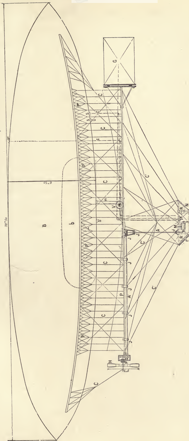
FIG. 45.—Count de la Vaulx's dirigible balloon.
