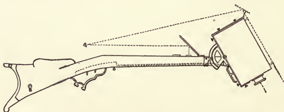
FIG. 191.—Baron von Bassus' rifle apparatus.
