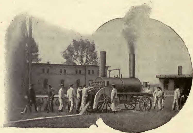
FIG. 88.—Steam winch for pulling in a captive balloon.
