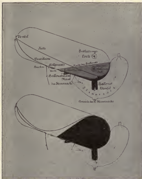
Fig. 116.—Drawing showing the design of the kite-balloon.
