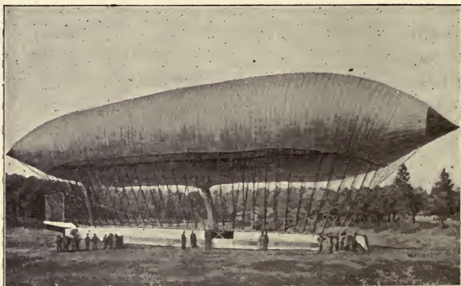
FIG. 28.—The balloon "La France," built by Renard and Krebs.
