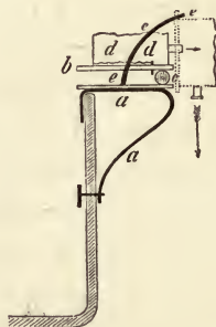
FIG. 189.—Hagen's method of mounting the camera.
