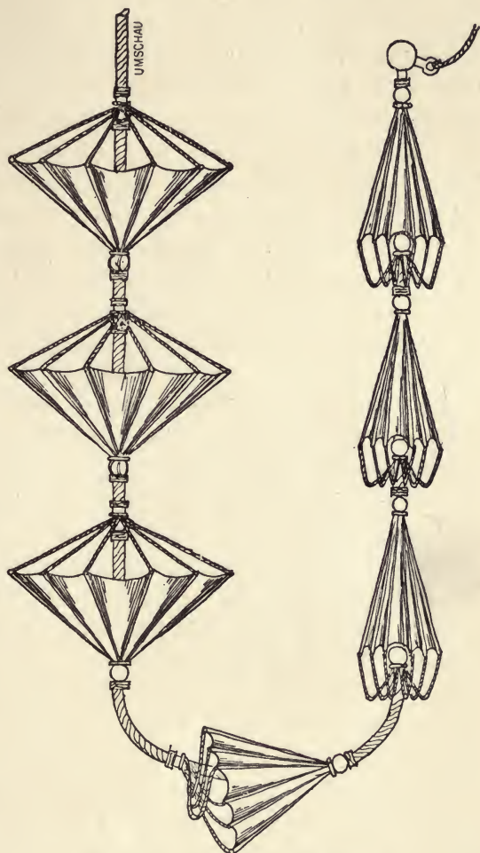
FIG. 129.—Water anchor for balloon.
