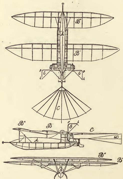
FIG. 54.—Kress's flying machine.
