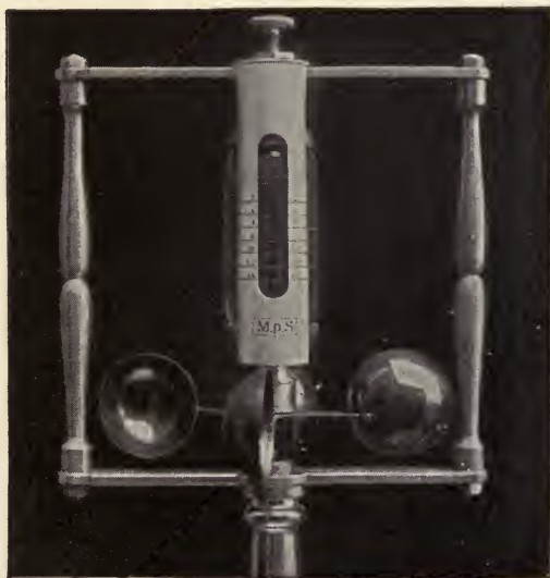
FIG. 37.—Gradenwitz anemometer.
