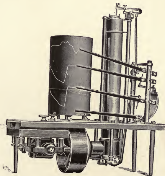
FIG. 169.—Baro-thermo-hygrograph, designed for balloons with observers by Dr. Hergesell, and made by Bosch, of Strassburg.
