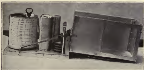
FIG. 119.—Barograph, or recording barometer.
