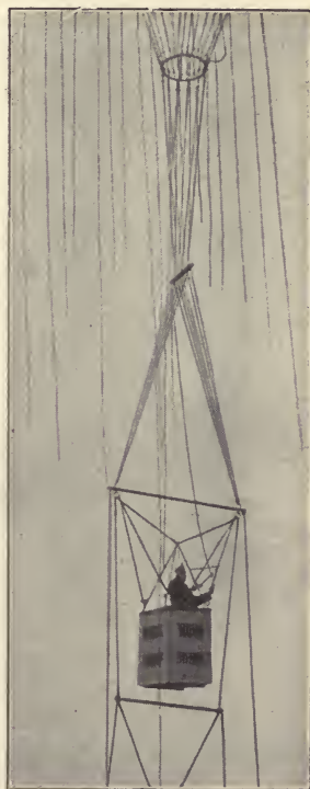
FIG. 94.—French method of suspending the basket for an observer.
