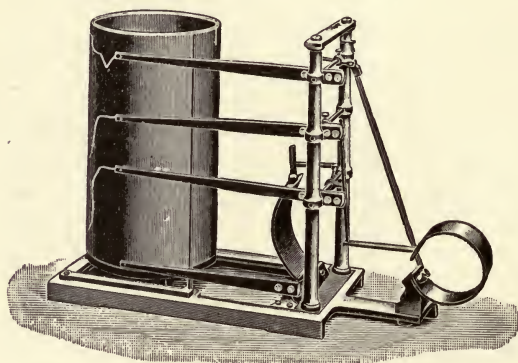
FIG. 170.—Baro-thermo-hygrograph, designed for kites by Dr. Hergesell, and made by Bosch, of Strassburg.
