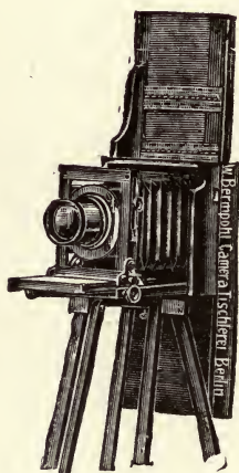
FIG. 211. — Camera for three-colour photography.
