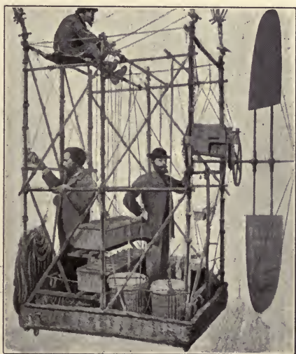
FIG. 26.—The basket of Tissandier's dirigible balloon.
