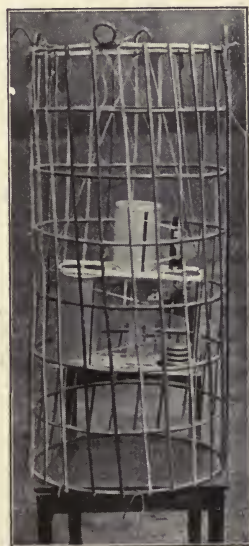
FIG. 158.—A wickerwork basket with instruments for a recording balloon.
