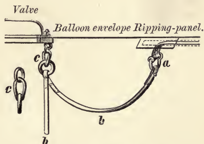
FIG. 112.—Arrangements for ripping-panel.
