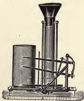
FIG. 171.—Baro-thermo-hygrograph, designed for recording balloons by Dr. Hergesell, and made by Bosch, of Strassburg.
