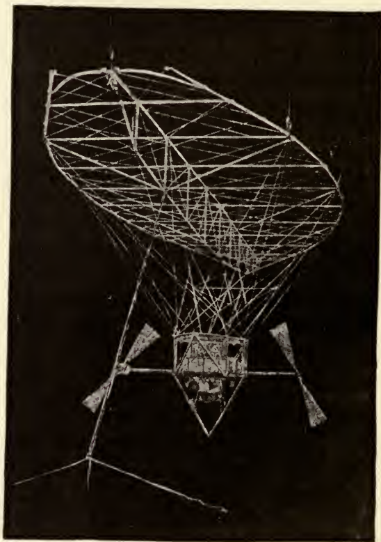
FIG. 40.—Framework and car of Lébaudy's dirigible balloon.
