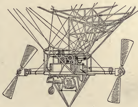
FIG. 41.—Car of Lébaudy's balloon.
