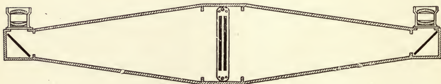
FIG. 214.—Boulade's stereoscopic camera.
