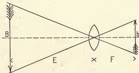
FIG. 197.—Diagram showing the relation between the focal length of the lens, the size of the image, and the distance of the object.
