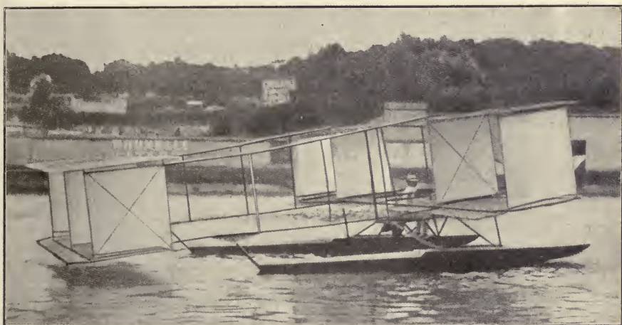
FIG. 65.—Archdeacon's experiments on the Seine.
