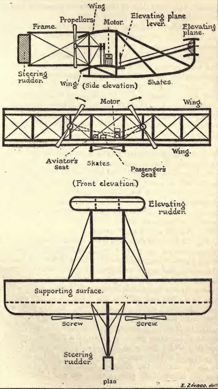
FIG. 71. The Wright Brothers' aeroplane
