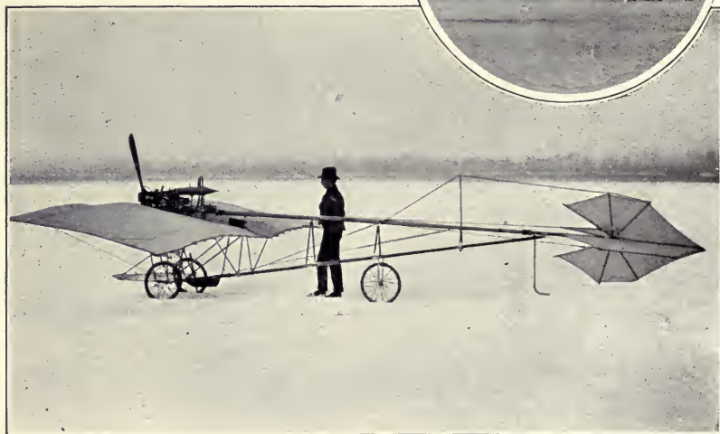
SANTOS-DUMONT'S "DEMOISELLE"
