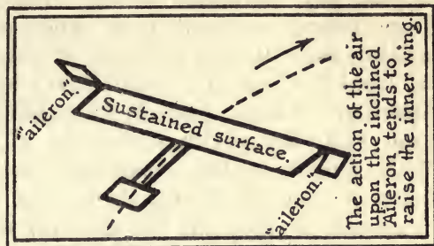
FIG. 57. Blériot's correcting ailerons
