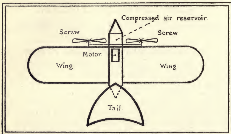
FIG. 79. Victor Tatin's aeroplane model driven by compressed air made a flight at Mendon in 1879
