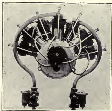
THE ESNAULT-PELTERIE LIGHT MOTOR
